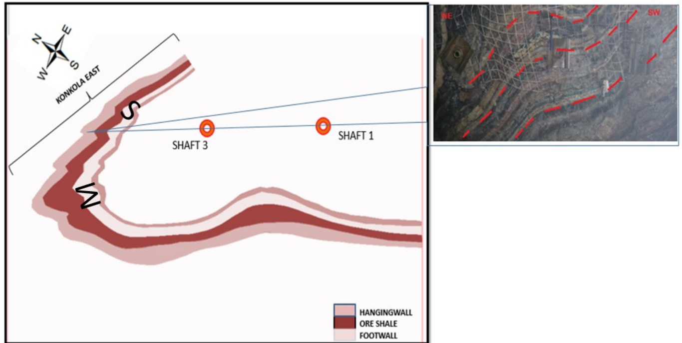
Figure 6-7: Schematic map of the Kirilabombwe anticline (not to scale) showing the location of Konkola east and the parasitic fold along the main fold.
