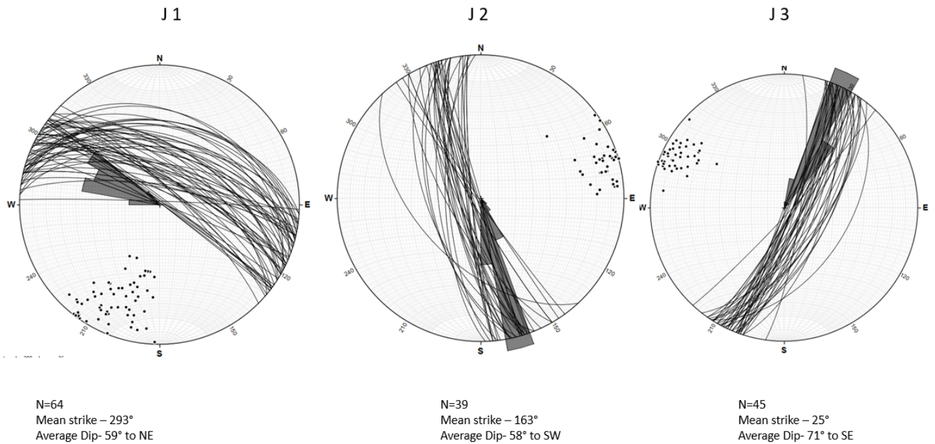
Figure 6-17: Lower hemisphere plot of the orientation of the established joint sets.
