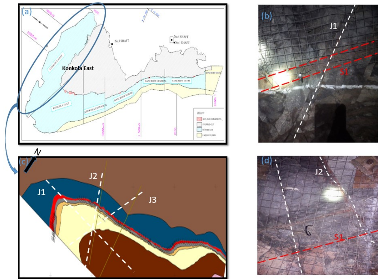
Figure 6-16 Jointing pattern in Konkola East. (a) General map showing the location of Konkola east. (b) Underground photo showing the relationship between S_1 and J_1 . (c) Geological map of Konkola East showing the general trend of the identified major joint sets, J_1 , J_2 and J_3 . (d) Underground picture showing the Orientation of J_3 and J_2 in relation to the bedding parallel S_1 .
