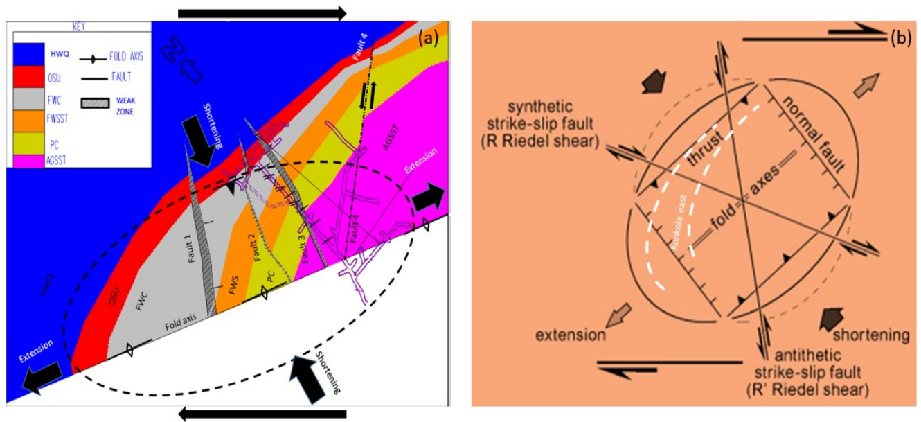
Figure 8-1: Structural pattern of Konkola East compared to the expected structural pattern of a typical dextral strike slip fault. (a) structural pattern observed and mapped at Konkola east in this study. (b) Structural pattern of a typical dextral strike slip fault (Eggers, 2016)
