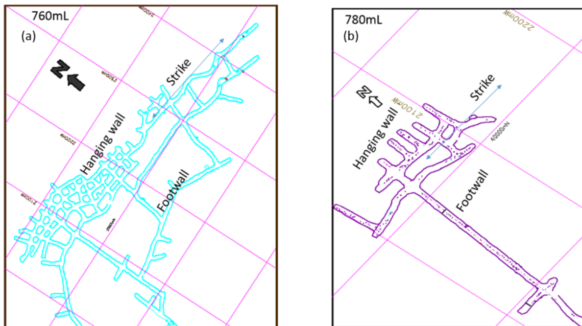
Figure 3-1 Microstation (dgn) mine plans of Konkola East mining block showing the two levels which were mapped during this study. (a) 760mL showing the mine development in relation to the general strike (b) 780mL showing the mine development in relation to the general strike.
