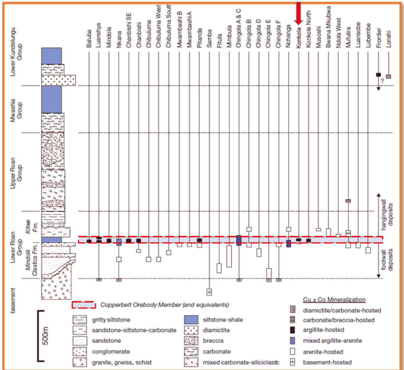
Figure 2-2: Lithostratigraphy of the Zambian Copperbelt showing the distribution of copper-cobalt mineralization (Selley et al., 2005). The figure also shows the stratigraphic position of the Copperbelt Orebody Member (highlighted in red).
