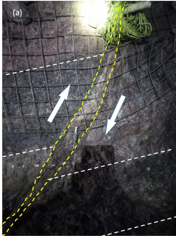
Figure 6-12 Mapped fault zones from underground. (a) Minor fault zone with a reverse shear sense and minor displacement. (b) Medium sized fault zone with a normal shear sense and displacement above 5 meters.
