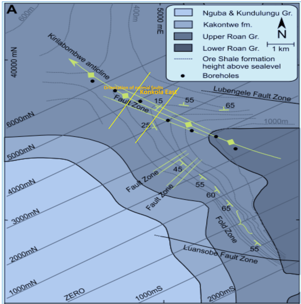
Figure 2-7: Map of structural elements associated with the Konkola ore deposit showing the surface trace of the Kirilabombwe anticline (Torremans et al., 2012)
