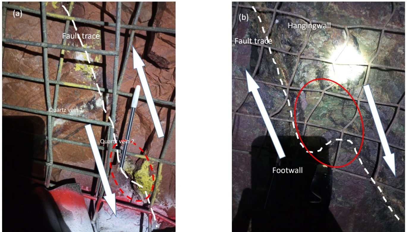
Figure 6-11: High angle faults observed in Konkola east. (a) Steep reverse fault with a releasing bend (circled in red) observed facing east. (b) A normal fault with a restraining bend (circled in red) as observed on the 2400mW pillar cross cut 3 facing northwest.
