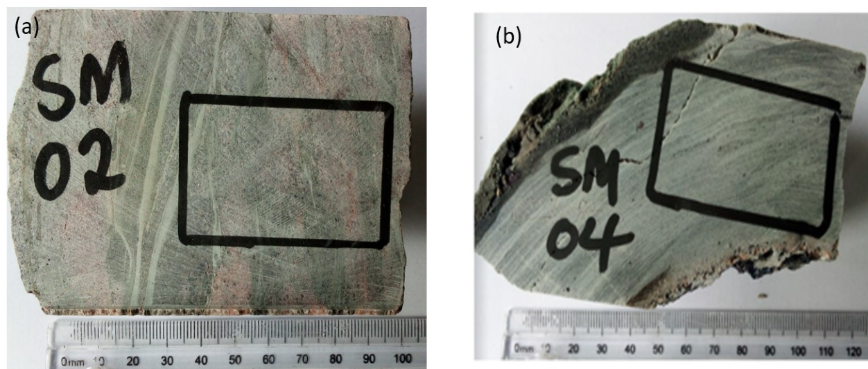
Figure 5-1: Core samples showing where the photomicrographs discussed in this chapter were prepared from. (a) SM 02 sample of footwall conglomerate from borehole BPN 881 (b) SM 04 sample of the Ore Shale Unit.
