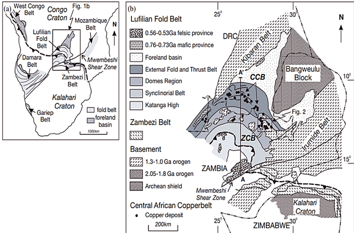
Figure 2-1: Simplified geological maps showing the tectonic setting and structural architecture of the Lufilian arc (Selley et al., 2005)
