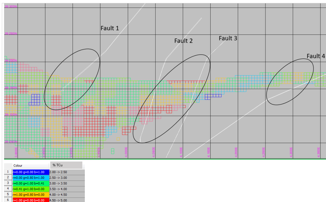
Figure 6-20: Grade maps showing grade in relation to the four major faults modelled on 609m level elevation. The circled areas show range associated with the faults.
