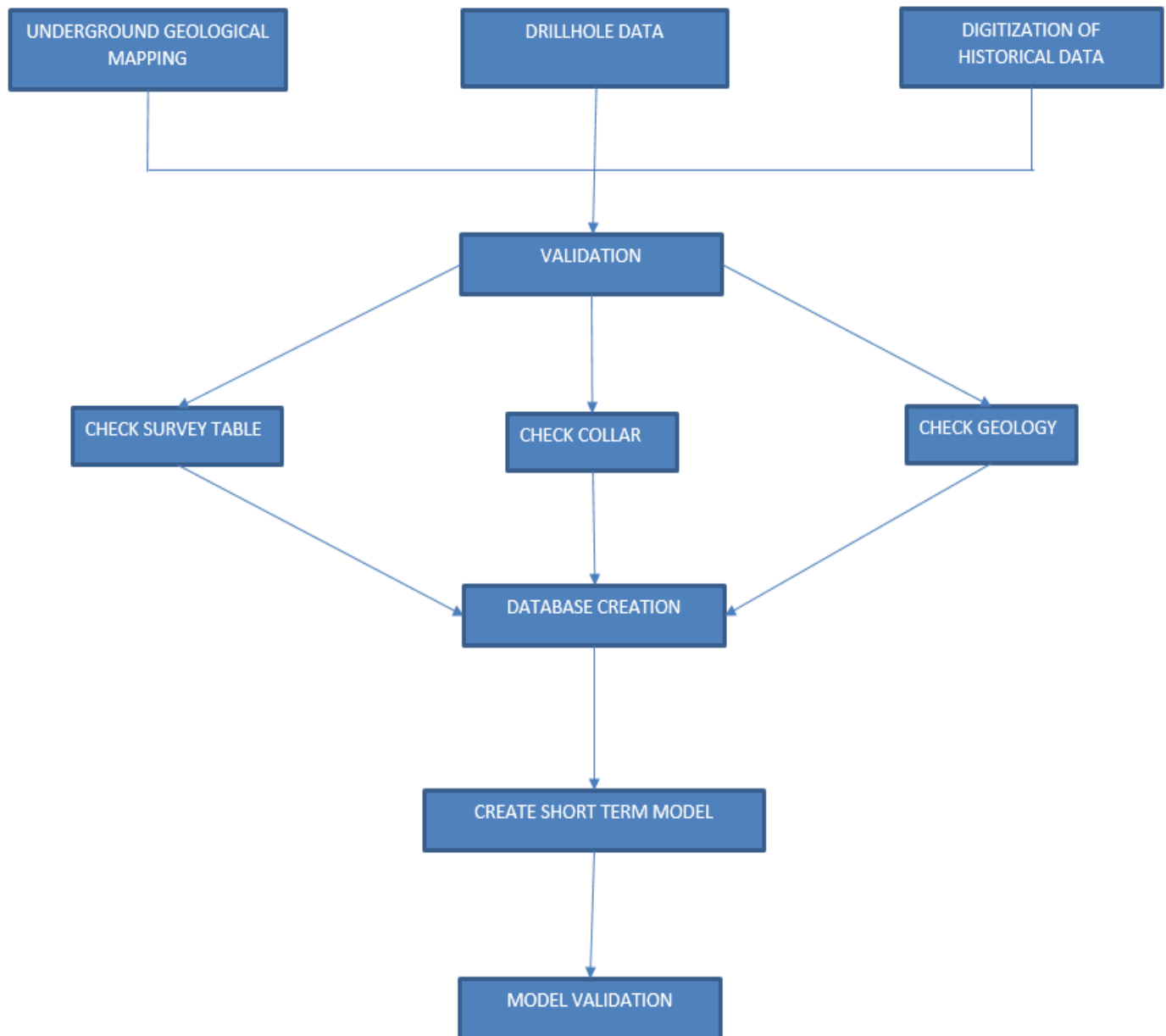
Figure 7-1: Workflow followed in generating the short term geological model.
