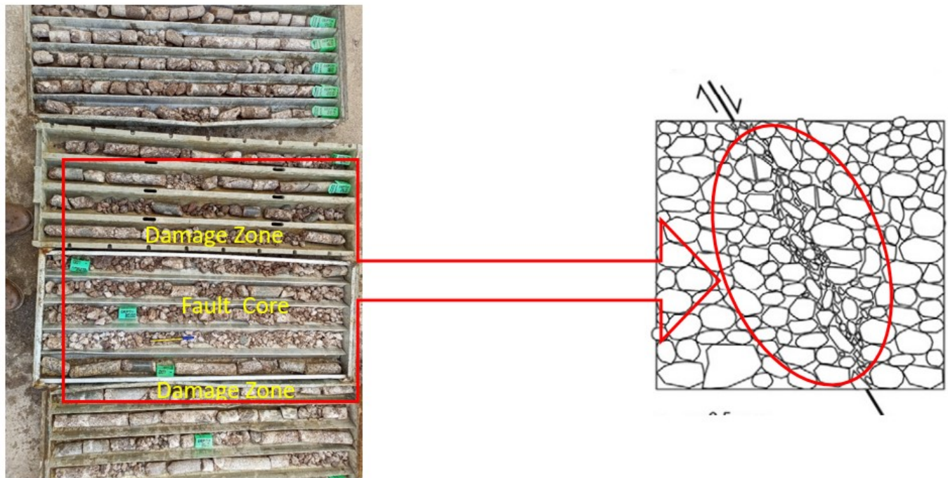
Figure 6-13: Observed brecciated Fault zone in DVN 1592 with relatively low intensity of cataclasis.
