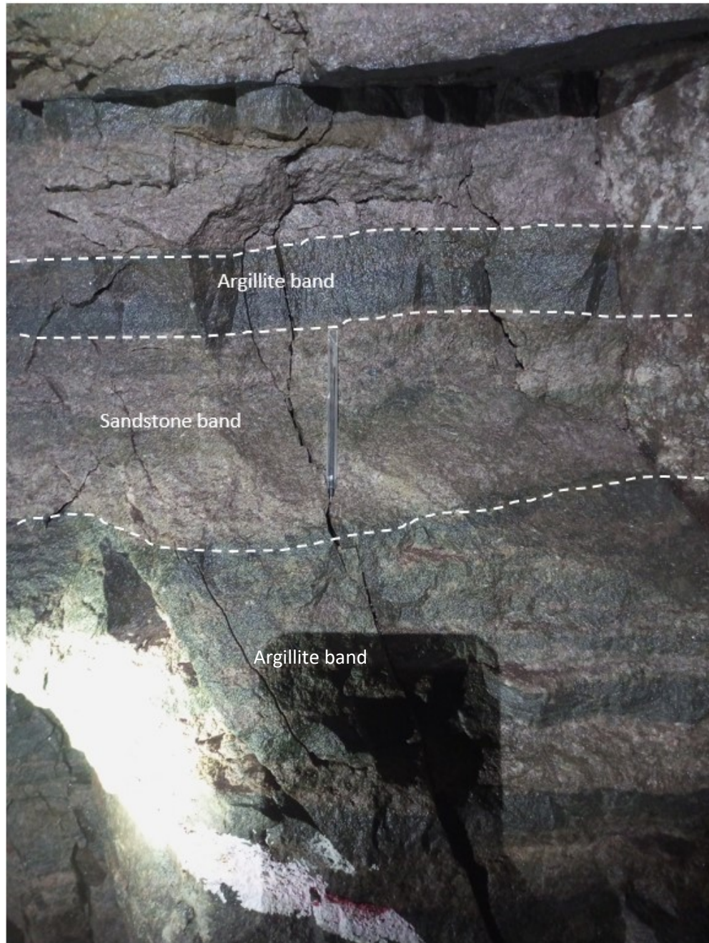
Figure 4-3: Underground picture of Argillaceous Sandstone exposure showing argillite bands interbedded with sandstone. The picture was taken from 760mL, 2400mW (Figure 1-3) crosscut facing north.
