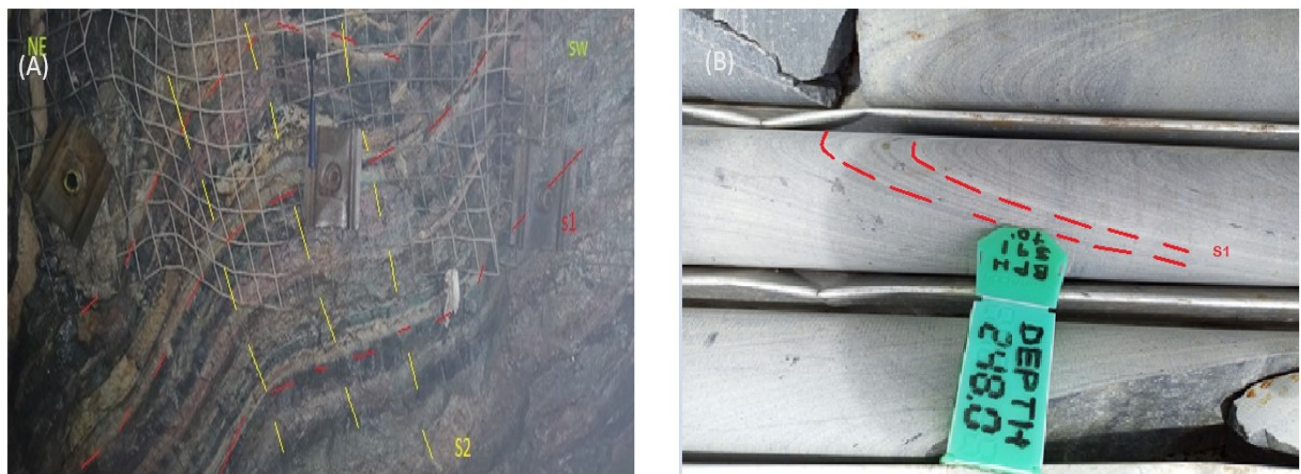
Figure 6-3: (A) 780mL 2400mw pillar cross cut 6 showing the S_1 fabric strongly developed in the ore shale and the fairly to poorly developed S_2 fabric. (B) Strongly developed S_1 fabric in ore shale as observed in core.
