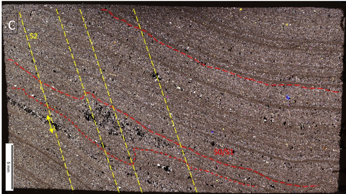
Figure 6-4 : Cross polarized light thin section of SM 04 showing S_0/S_1 fabric and S_2 fabric shown by the elongation of sulphide minerals appearing black. The yellow line represents S_2 and the yellow arrows shows the elongation direction.
