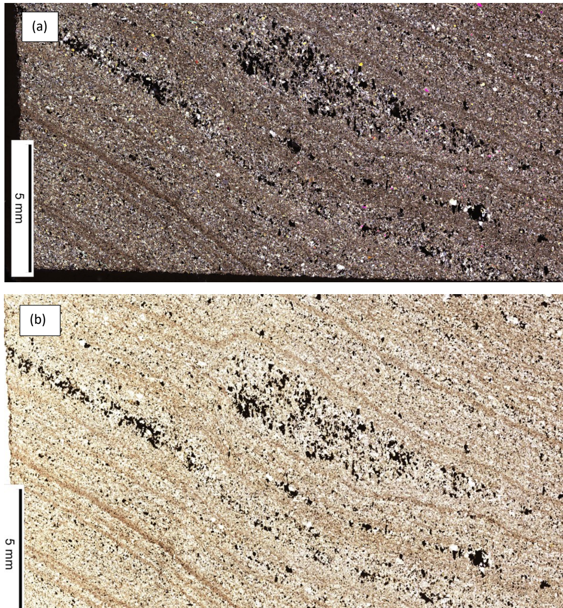
Figure 5-4: Photomicrograph of SM 04 as observed under (a) cross polarized light and (b) plane polarized light. Ore minerals appear dark in both cross polarized light and plane polarized light and occur mainly along layers.
