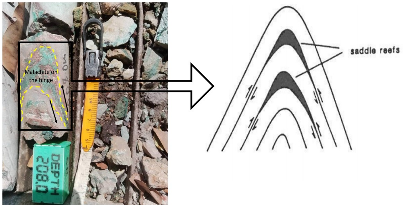
Figure 6-18: Photo from BPN 891 showing crescentic saddles created through flexural slip and hinge dilation through the folding process. Malachite mineralization is observed to be concentrated on the fold hinge. Schematic illustration done after(Cox et al., 1991)
