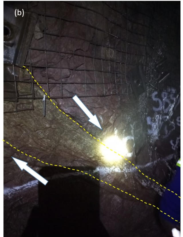
Figure 6-12 Mapped fault zones from underground. (a) Minor fault zone with a reverse shear sense and minor displacement. (b) Medium sized fault zone with a normal shear sense and displacement above 5 meters.
