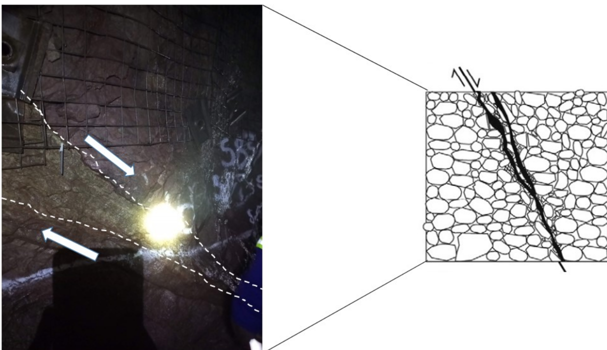
Figure 6-14: Underground photo from 2400mW Konkola east showing a normal fault with relatively high intensity of cataclasis.
