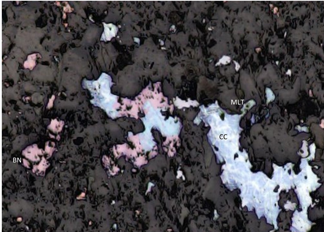
Figure 5-6 : Part of the photomicrograph (SM04), an extract from figure 8.3 showing textural relationship between bornite (BN), chalcocite (CC) and malachite (MLT)
