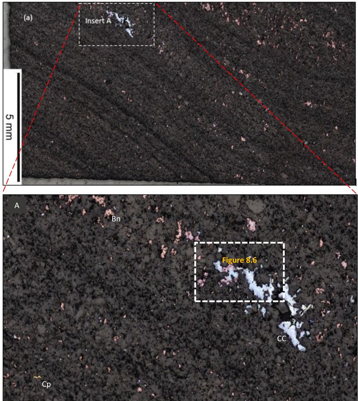
Figure 5-5: Photomicrograph of SM 04 viewed under Reflected light showing the major ore minerals being bornite (pinkish brown), chalcocite (whitish grey) and chalcopyrite (yellow). In insert A in the bottom, chalcocite is observed to be replacing the relic bornite grains.
