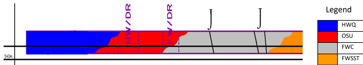
Figure 6-1: Eastern Sidewall mapping of 2400mW showing the lithologies and joints observed in the cross cut. Two drives, hanging wall drive (HW/DR) and foot wall drive (FW/DR) are shown by the dotted lines.
