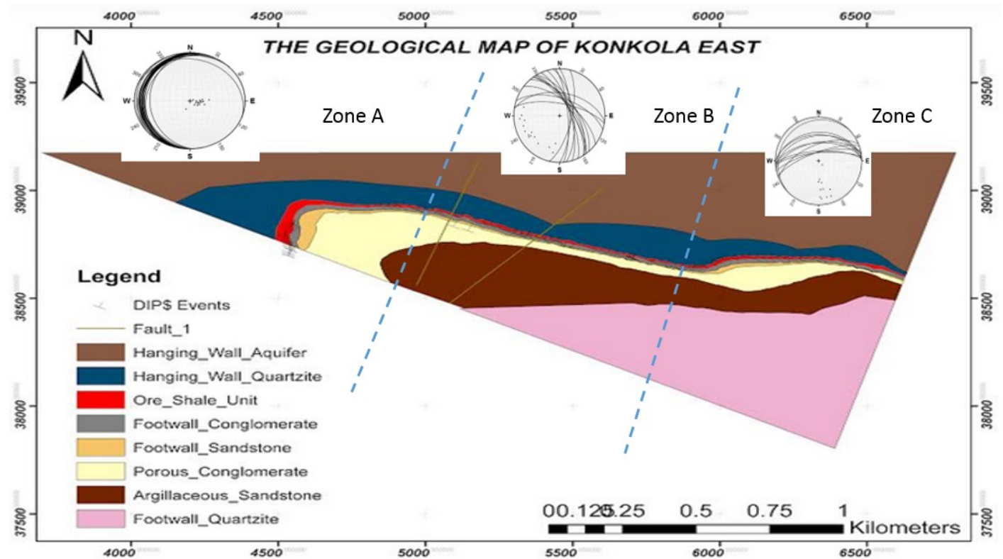
Figure 4-1: Geological map of Konkola East showing the major lithologies and structural features of Konkola east. The area was subdivided into 3 zones, Zone A, Zone B and Zone C based on the average dip and strike of the bedding of the Ore Shale Unit (red).
