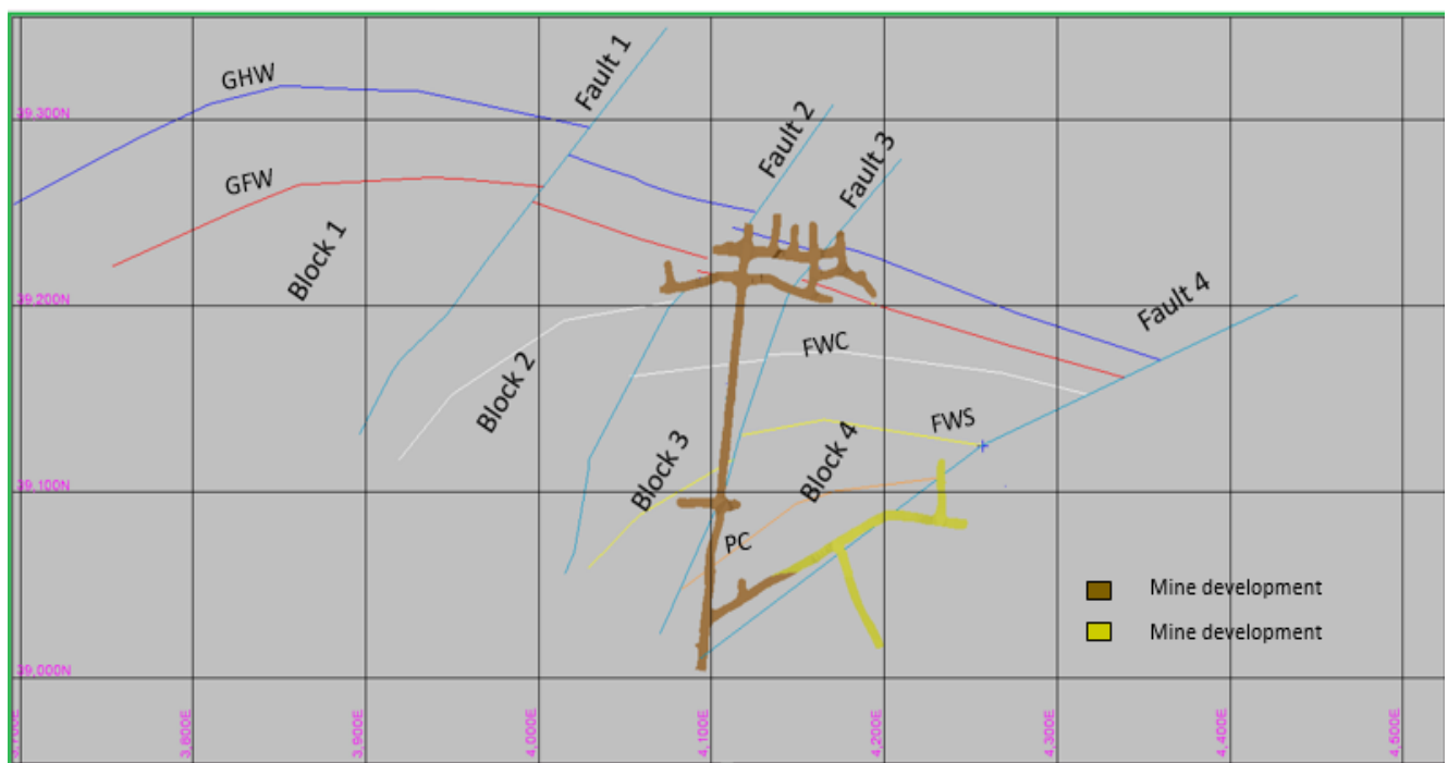
Figure 7-2: Surpac plan view of 780 m level showing the 4 blocks and the 4 major faults. The lines indicate lithological contacts.
