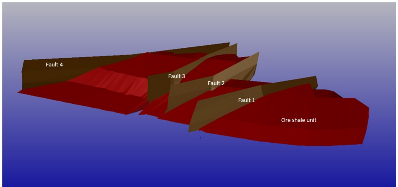
Figure 7-5: Isometric view of the created model facing south-west the four main faults identified (in brown) and the ore shale unit lithology in red.
