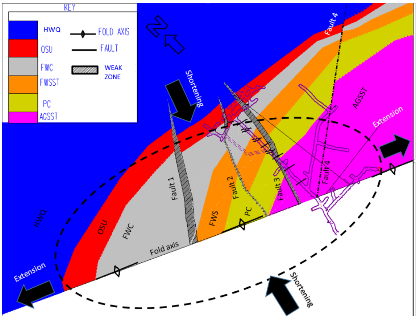
Figure 6-10: 780mL geological map showing the major structures and the ellipse demonstrating zones of extension and zones of compression
