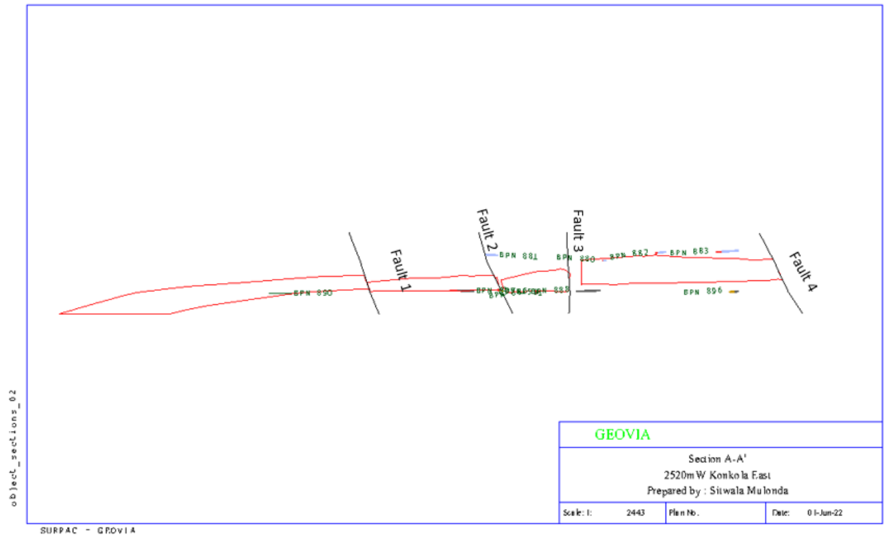
Figure 7-4: Section along A-A' showing the four major faults identified in the study and the ore shale lithology
