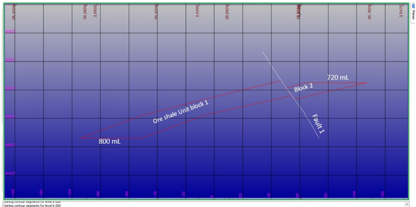
Figure 7-6 : Random section of the created model used for validation purposes showing the ore shale lithology displaced in a normal way along fault 1.
