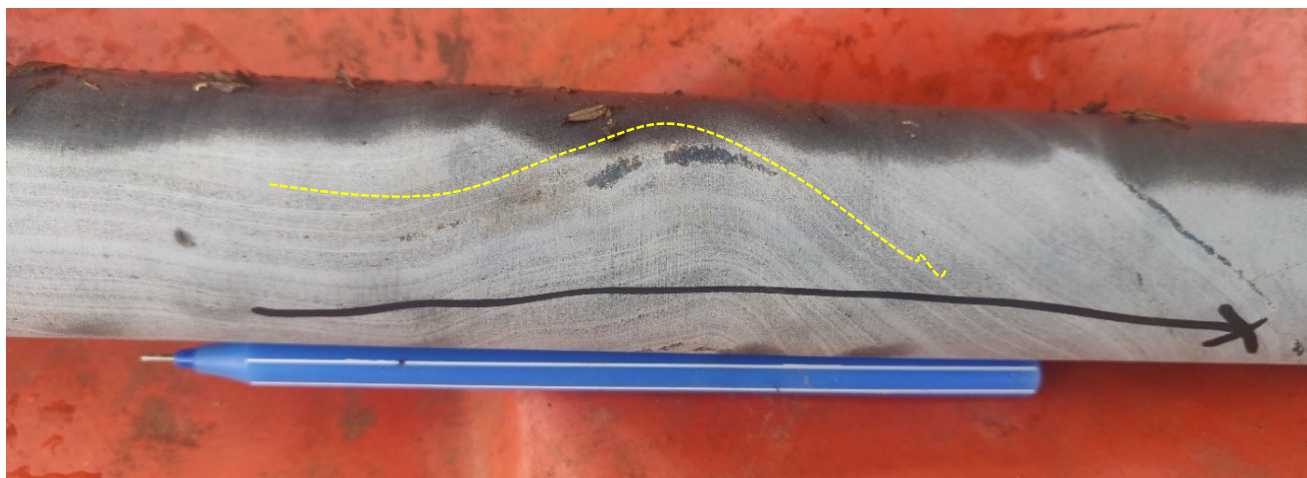
Figure 6-8: A relatively open fold observed from borehole BPN 881.
