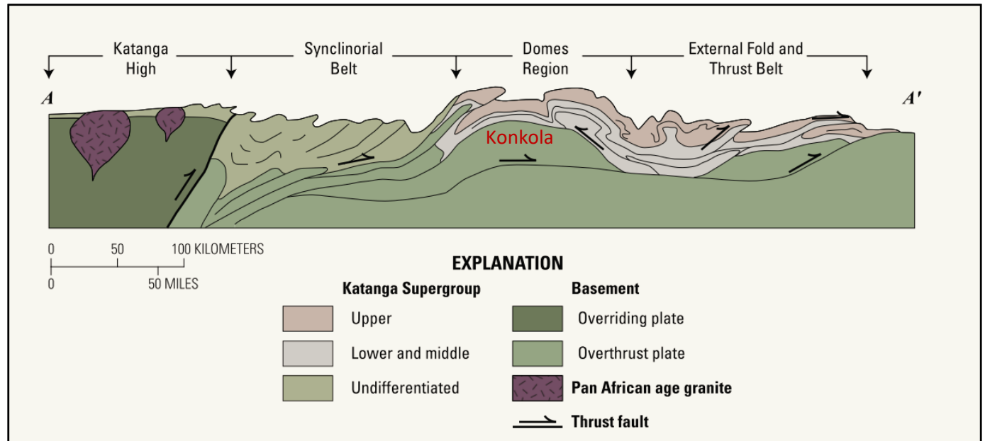
Figure 2-4: South to north cross section across the Lufilian arc showing the four subdivisions including the domes region where Konkola east lies (Zientek et al., 2010).
