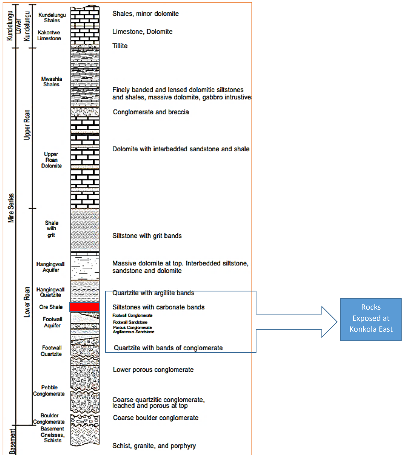
Figure 2-6: stratigraphic column for Konkola Mine also showing the part of the stratigraphy that is exposed by mine developments at Konkola east (Greyling, 2009)
