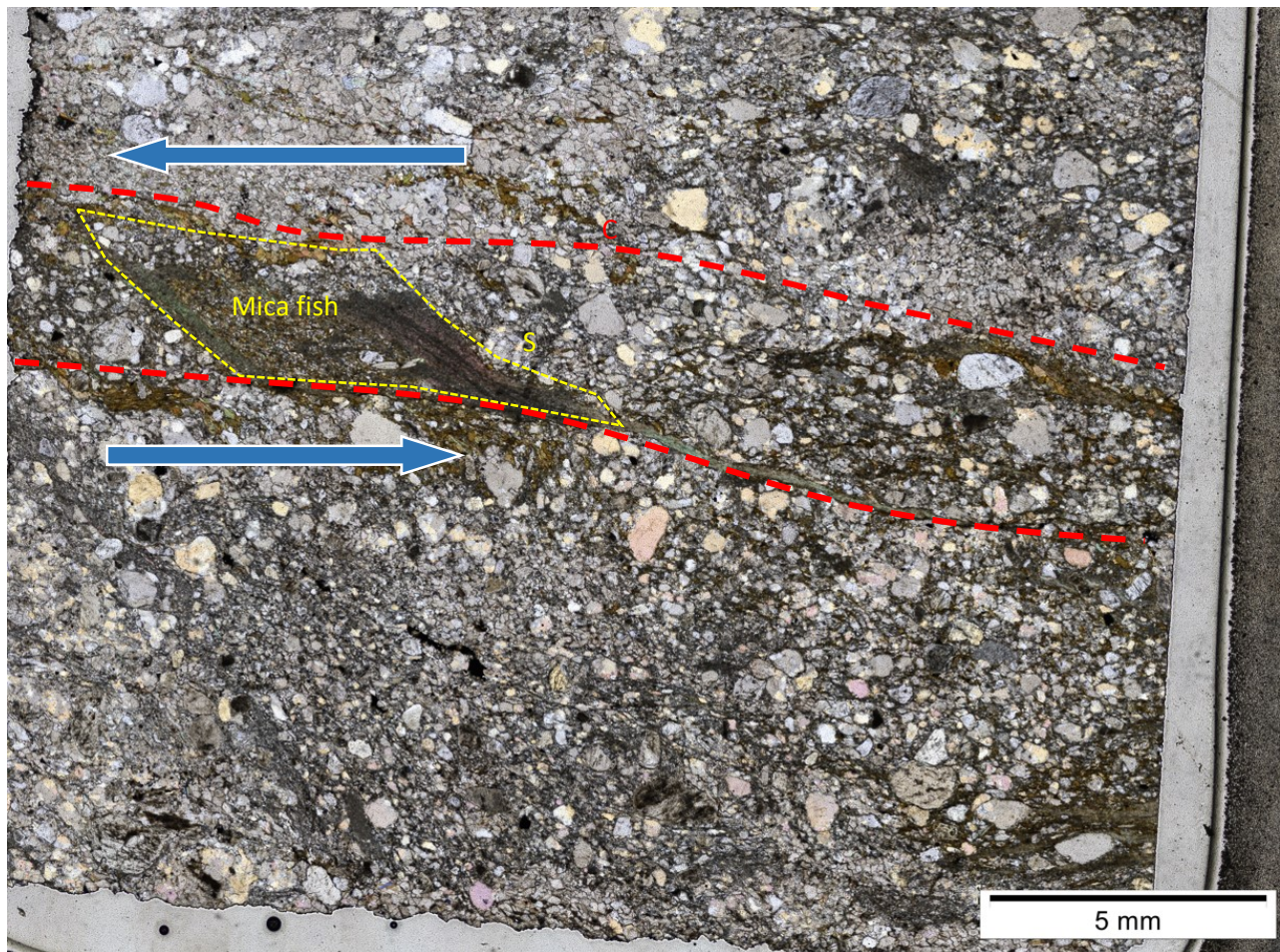
Figure 6-6: Photomicrograph SM 02, of the footwall conglomerate viewed under plane polarized showing mica fish developed and interpreted as a shear sense indicator of a left lateral shear.
