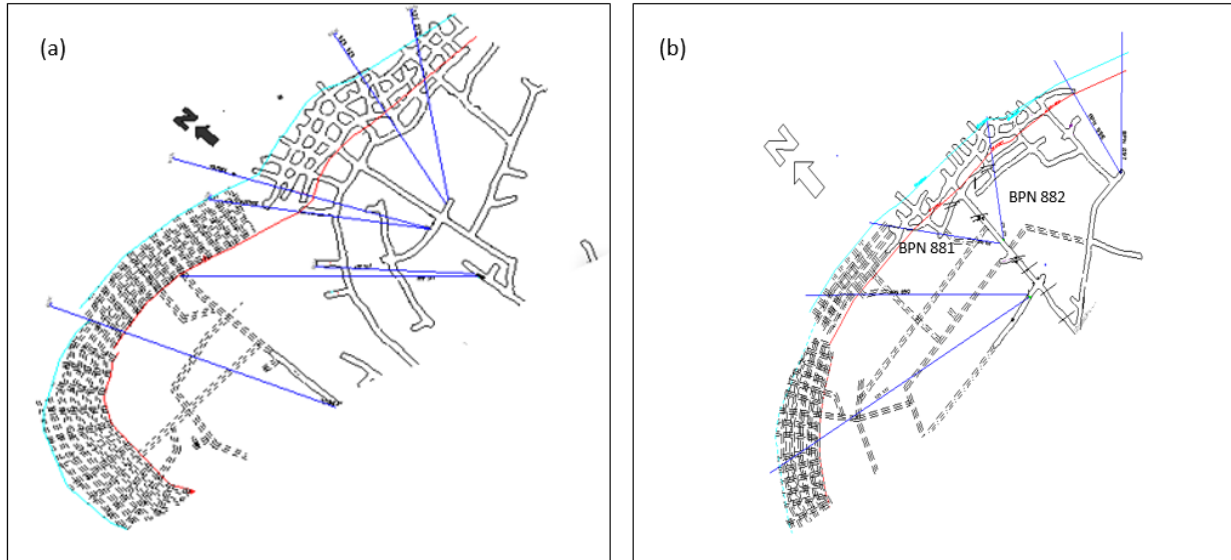
Figure 3-2: Location of some of the boreholes used in this study shown in plan-view on underground working levels. (a) 760 mL showing the collar position and orientation of some of the boreholes drilled on this level. (b) 780 mL showing boreholes drilled on this level and used in this study. Samples for petrographic analysis were gotten from BPN 881 and BPN 882.
