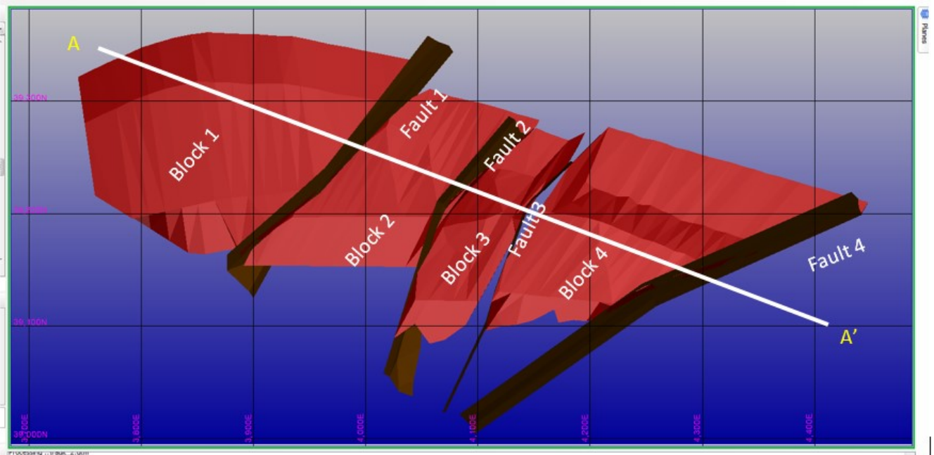
Figure 7-3: Plan view of the created geological model showing the four faults and the 4 blocks.
