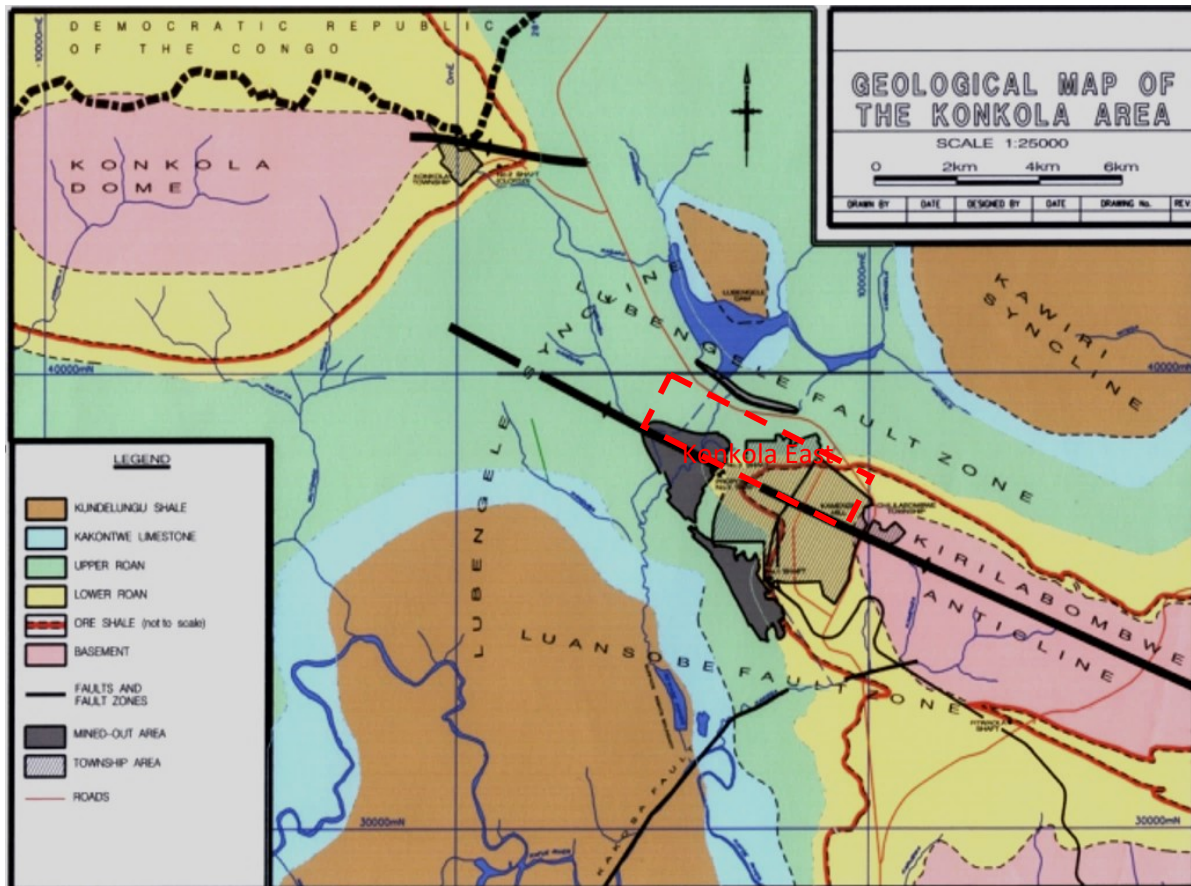
Figure 2-5: Geological Map of the Konkola area also showing the location of Konkola East. (Konkola Copper Mines, 2013)
