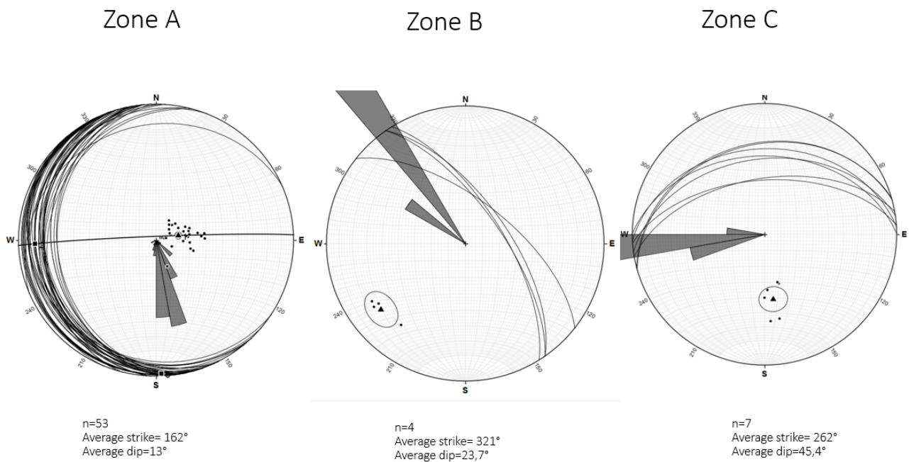
Figure 6-5: Lower hemisphere Stereo plots of S_1 on the 3 zones identified as shown in Figure 4-1
