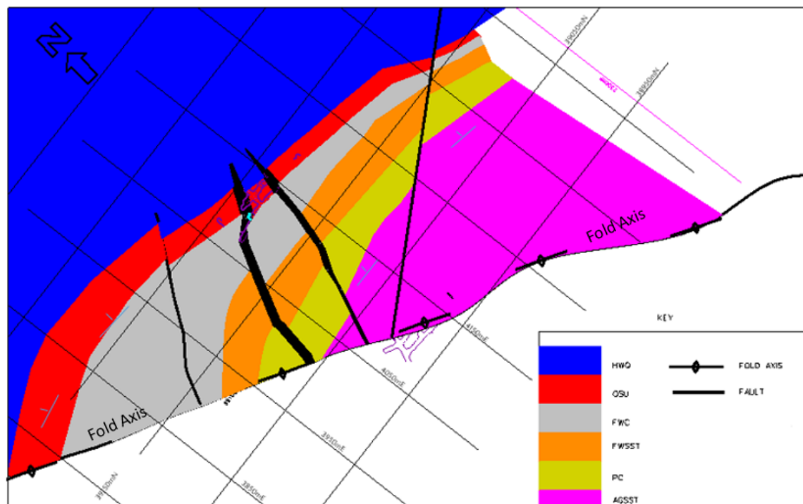
Figure 6-2: Geological map of 780 ml produced after mapping the mining excavations.
