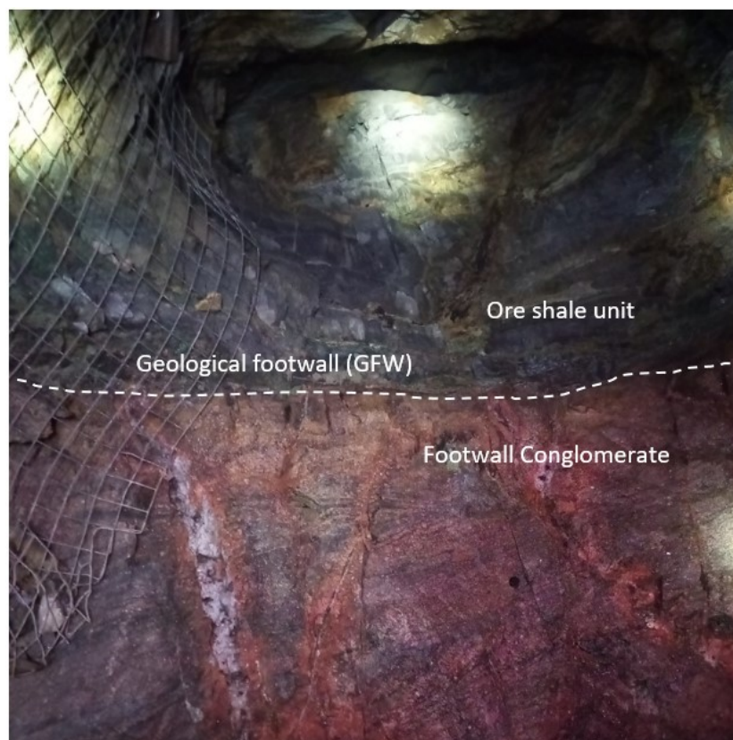
Figure 4-6: Underground face mapping. 760mL 2400mW access to orebody showing the top part of the Footwall Conglomerate where it makes contact with the Ore Shale unit. This contact is also called the Geological Footwall (GFW).
