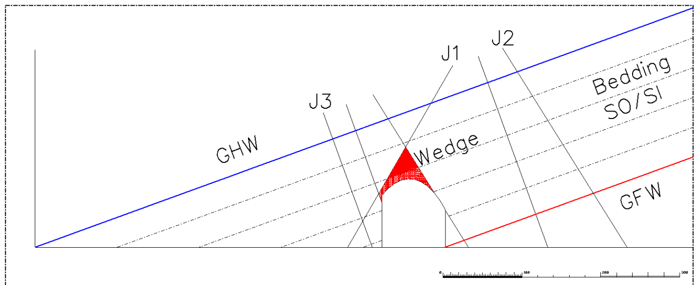
Figure 8-2: Cross section view (facing east) illustrating formation of wedge failure as a result of the interaction of the bedding planes and the joint orientation.
