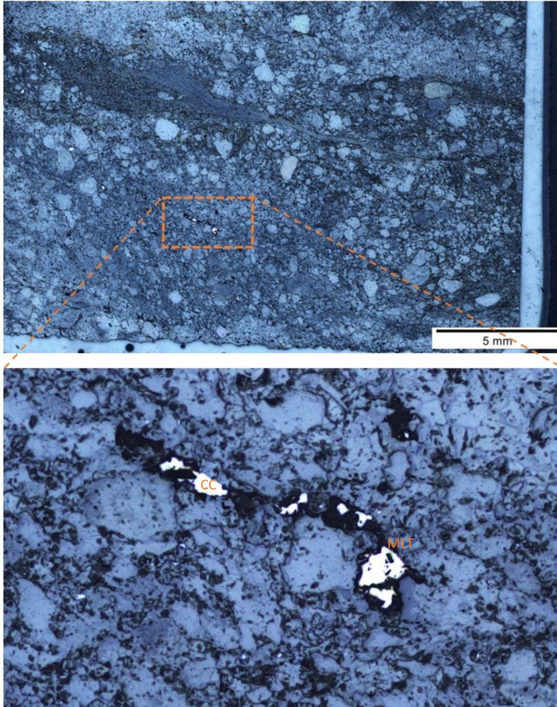
Figure 5-3: Photomicrograph of SM 02 (Footwall conglomerate) viewed under reflected light showing chalcocite (whitish grey) being replaced by malachite (green) along the grain boundaries.
