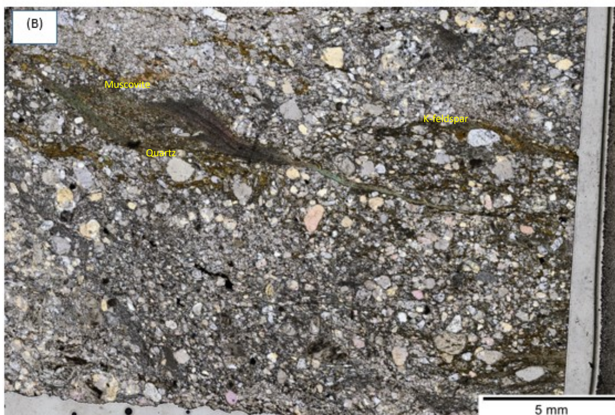
Figure 5-2: Photomicrographs of the footwall Conglomerate, SM02 showing sinusoidal mica. (A) Viewed under cross polarized light. (B) Viewed under plane polarized light.
