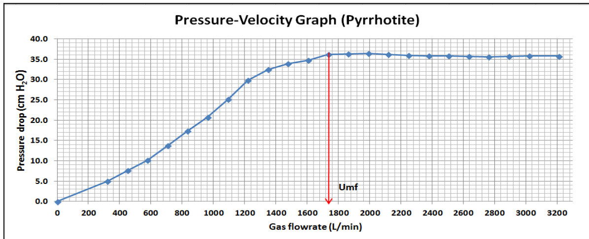
Figure 4-2: Illustration of minimum fluidization velocity
