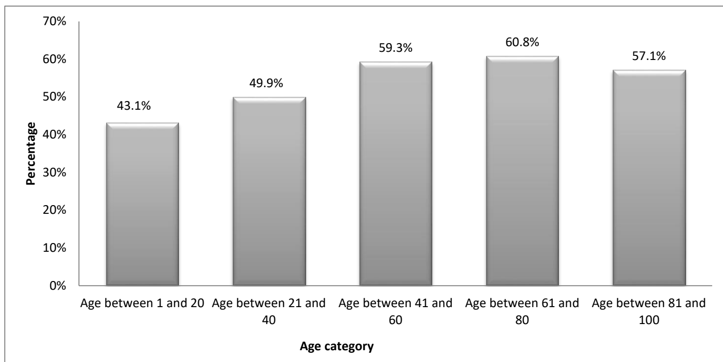
Figure 2: Positive scans according to age categories
