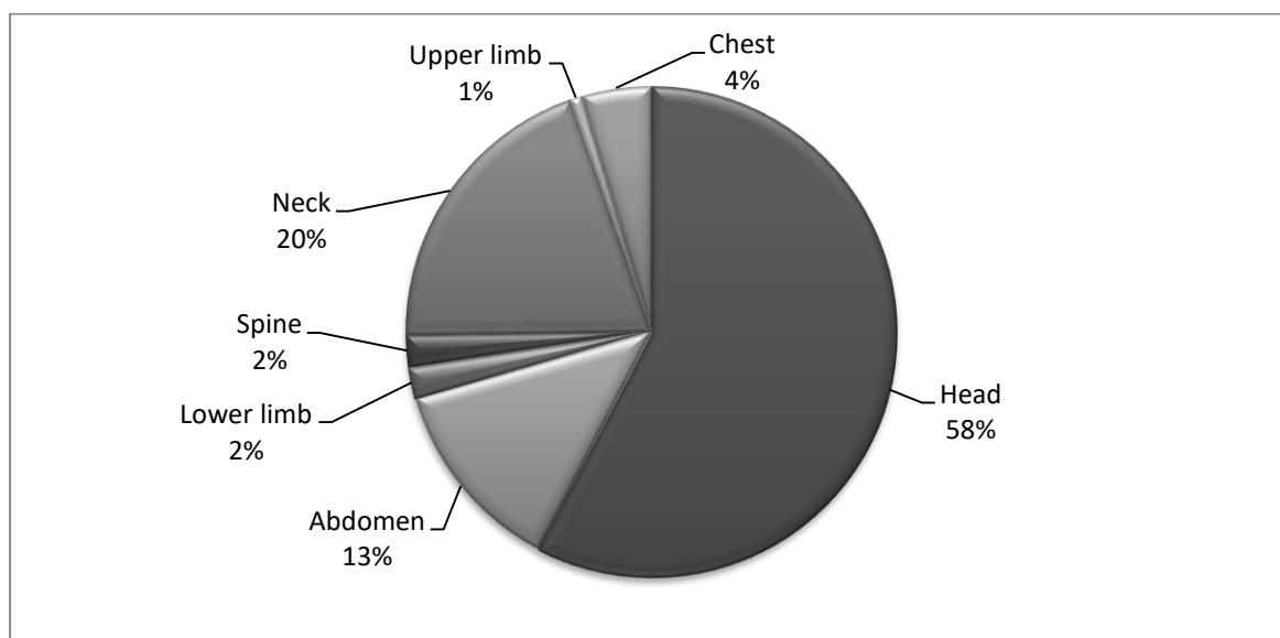
Figure 3: Division of anatomy scanned
