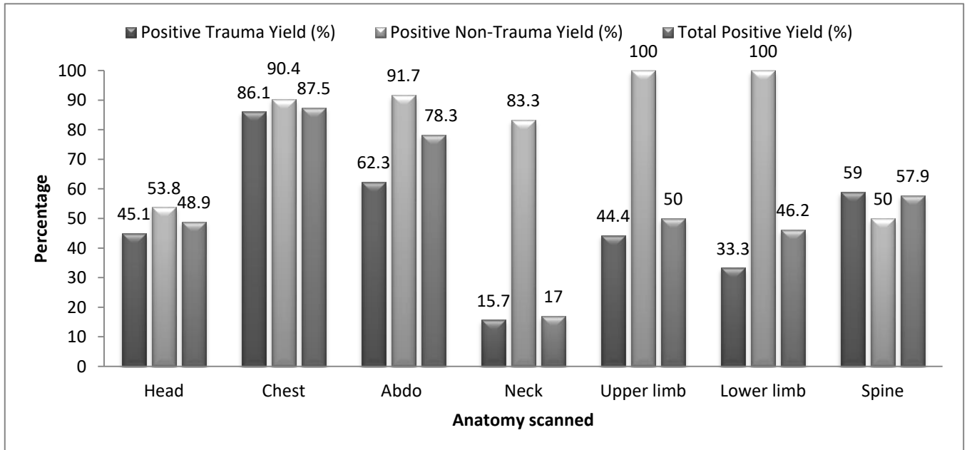
Figure 4: Positive findings according to anatomical region scanned.
