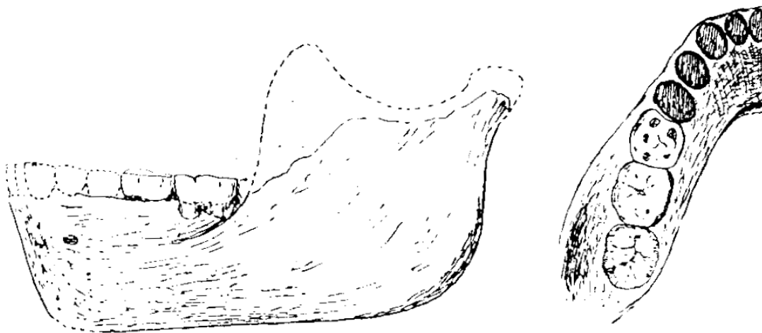
Figure 2. Side view of mandible (L) and occlusal view of teeth (R) of Telanthropus . (not scaled). From Broom and Robinson, 1949.
