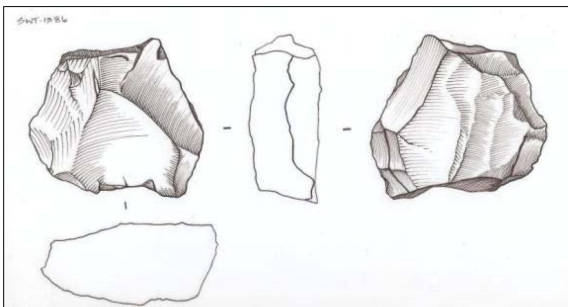
Figure 46. Quartzite prepared core. Image in figure 32 (b). Drawn by A. Sumner.
