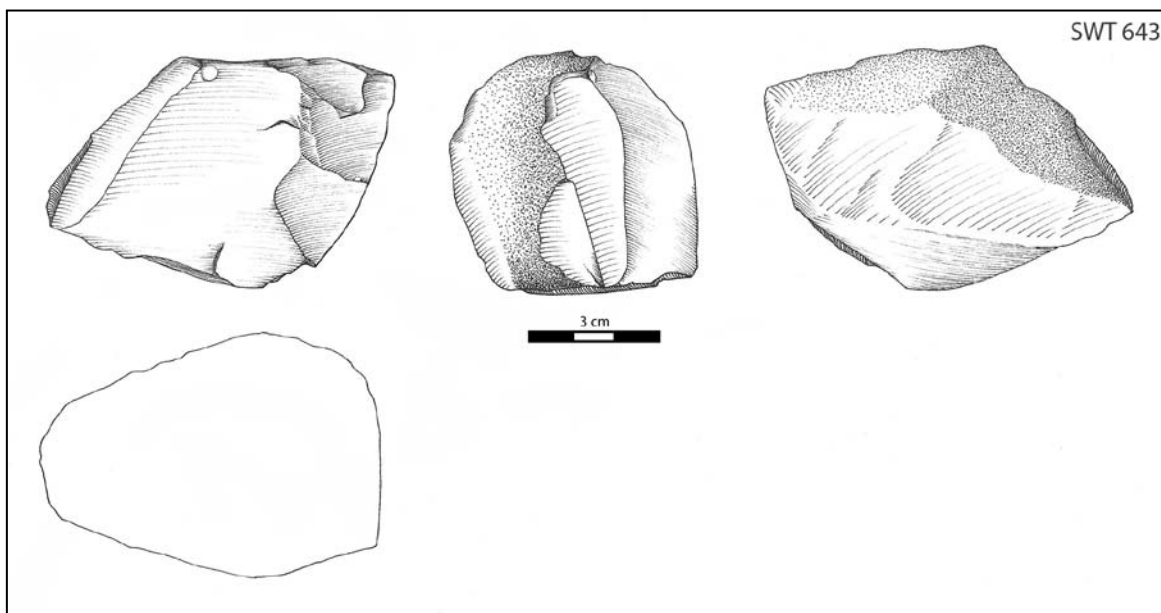
Figure 22. SWT 643, a chert casual or tested core from the Lower Bank of Member 1 with only one removal and associated breakage. Drawn by A. Sumner.
