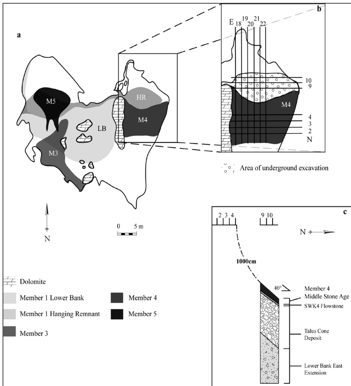
Figure 35. Plan view of Swartkrans Cave showing the relationship of Member 4 to the other areas of the site. (b) Detail of the Member 4 area, with the excavation grid superimposed. The Member 4 area includes the MSA surface excavation (shaded) and the underlying Talus Cone Deposit and Lower Bank East Extension deposit, exposed in our excavations to the north (open circles) of the surface excavation. (c) The Member 4 area stratigraphy is shown schematically in profile. Drawn by Jason Heaton.
