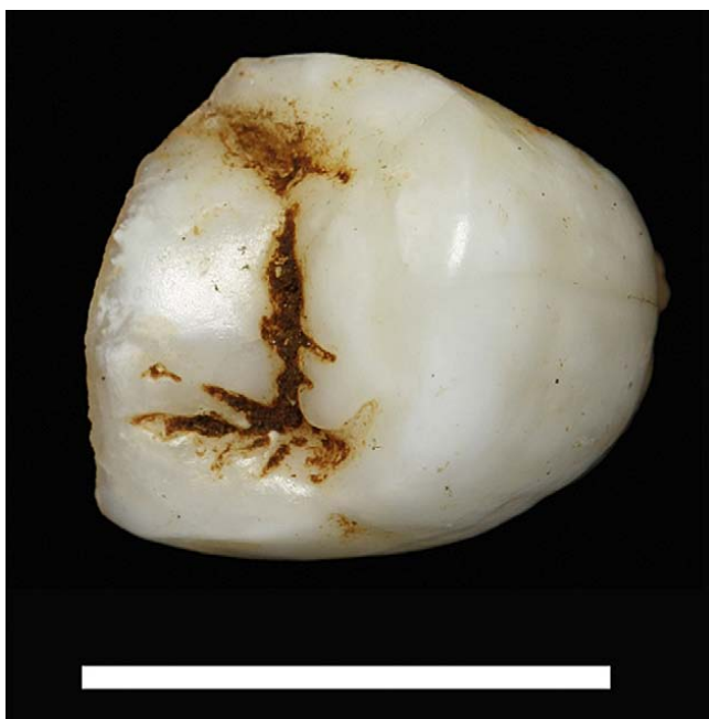
Figure 28. SWT1/LB-12 (occlusal view), a lingual crown fragment of a Paranthropus robustus right upper third premolar (missing its buccal ridge) from the Lower Bank of Swartkrans Member 1. Bar scale \frac{1}{4} 1 cm. From Pickering et al. 2012.
