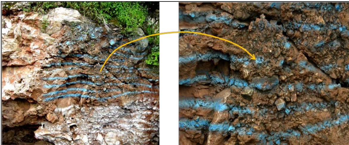
Figure 8. View of HR calcified conglomerate adjacent and east of newly exposed section (seen on far left).
