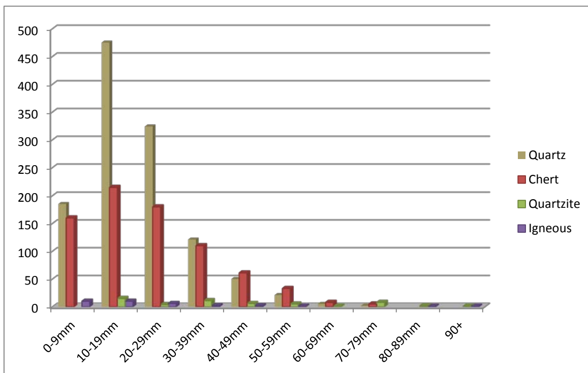
Figure 19. Maximum length of the newly excavated LB assemblage, excluding cores and manuports. The collection is dominated by small pieces but has a full range of debitage indicating a near complete assemblage.
