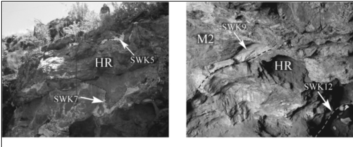
Figure 12. Photos showing the position of the flowstones and the locations from which the dating samples were taken. The left photo is the newly exposed central portion of the HR. SWK 7 was taken from the base of the deposit. SWK 5 was taken from near the top of the deposit. The right photo is the HR along the west wall in the northwest corner of the cave. Sample SWK 12 was taken from the distal portion of the large speleothem removed by the miners. SWK 9 was taken from the flowstone at the top of the HR where it is overlain by Member 2. Photo on left taken by R. Pickering.
