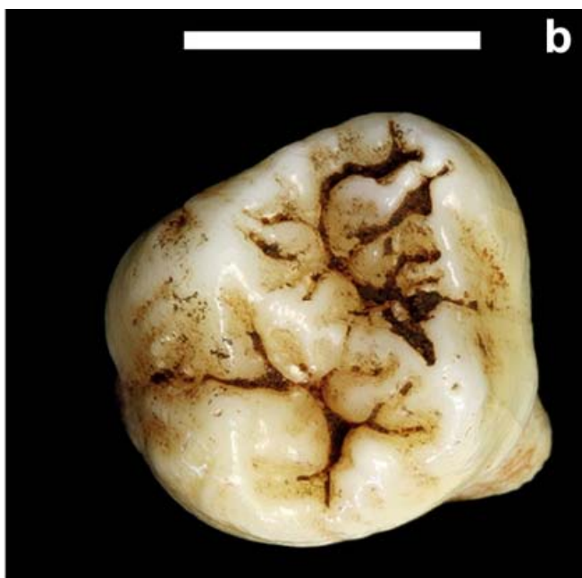
Figure 31. SWT1/LB-11 (occlusal view), unerupted left upper molar of Paranthropus robustus from the Lower Bank of Swartkrans Member 1. Bar scale \frac{1}{4} 1 cm. From Pickering et al. 2012.
