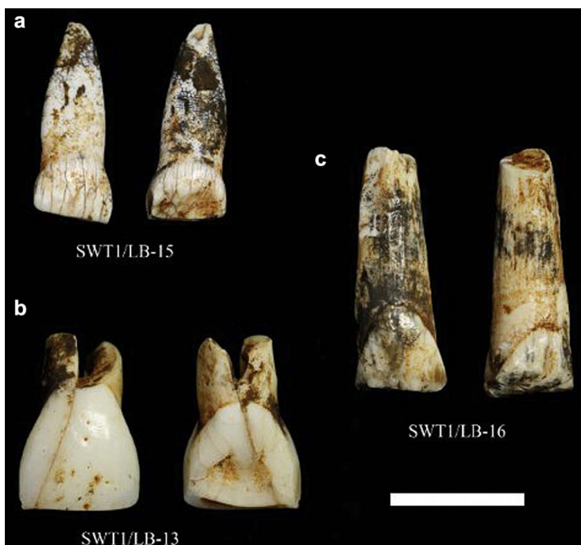
Figure 26. Paranthropus robustus upper central incisor fossils from the Lower Bank of Swartkrans Member 1. SWT1/LB-15 is a right deciduous (a), SWT1/LB-13 is a left permanent (b) and SWT1/LB-16 is a right permanent (c). Bar scale \frac{1}{4} 1 cm. From Pickering et al. 2012.
