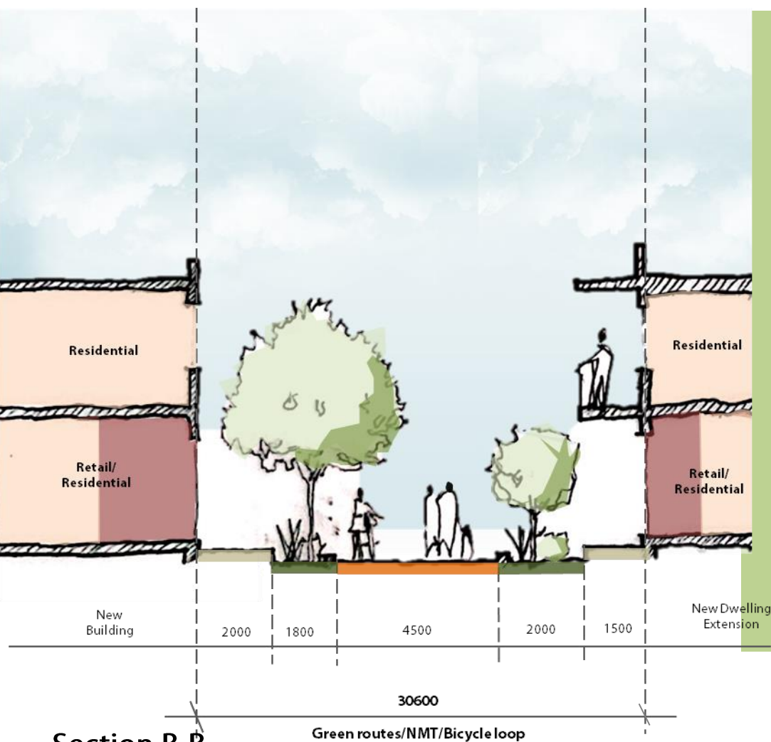
Section B-B
