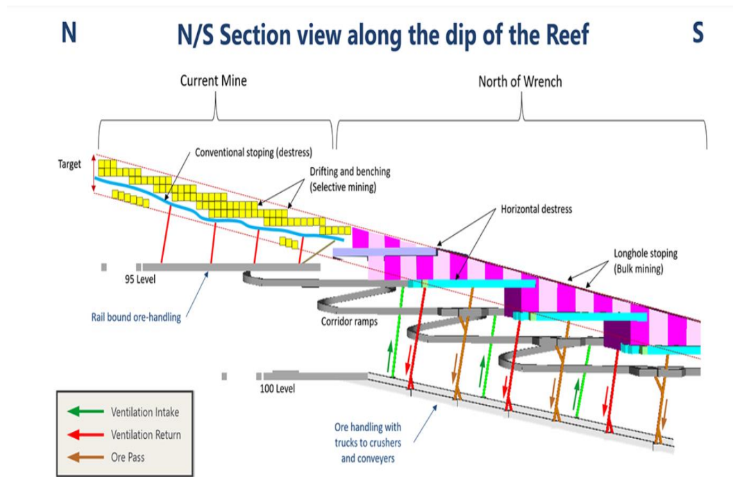
Figure 1-7: Illustration of mining methods at South Deep Gold Mine (Gold Fields, 2022c)
