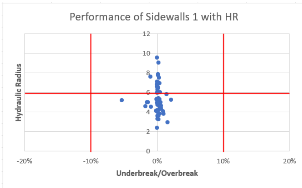
Figure 4-43: Performance of sidewalls 1 with HR
