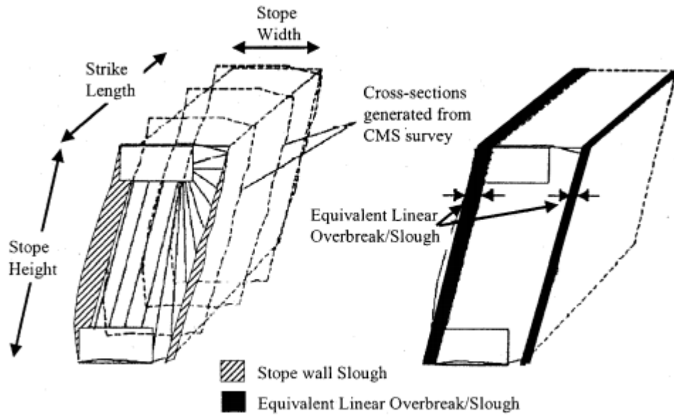
Figure 2-8: Schematic of ELOS (Clark & Pakalnis, 1997)
