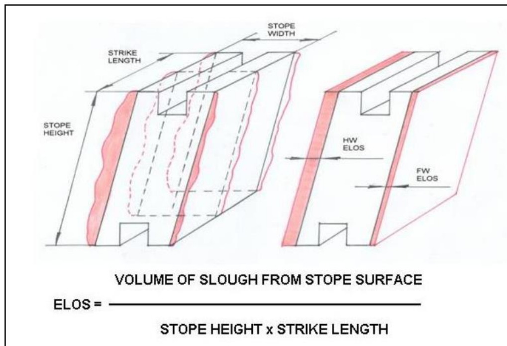
Figure 2-9: Concept of ELOS (Andrews and Barsanti, 2008)
