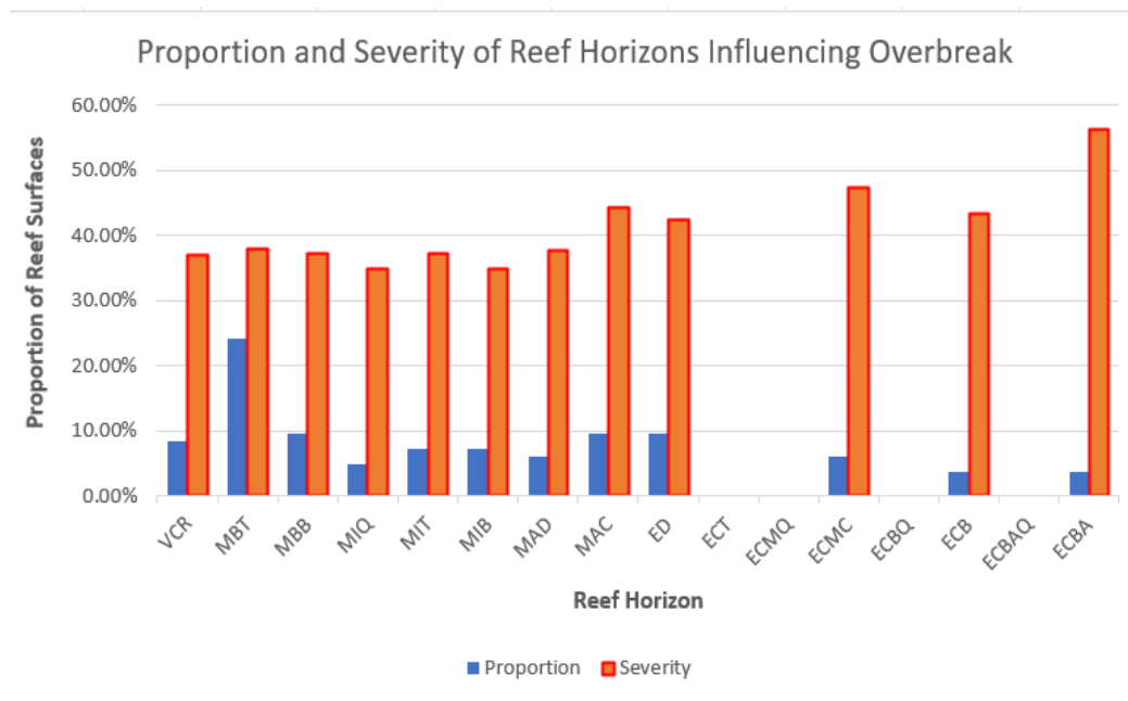
Figure 4-14: Proportion and severity of reef horizons influencing over-break
