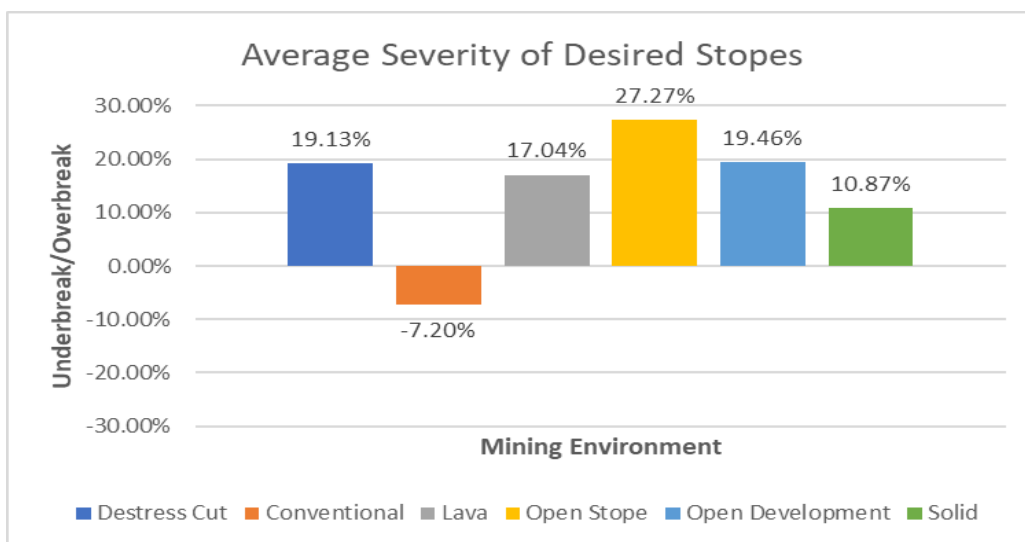
Figure 4-11: Severity of desired stopes by environment
