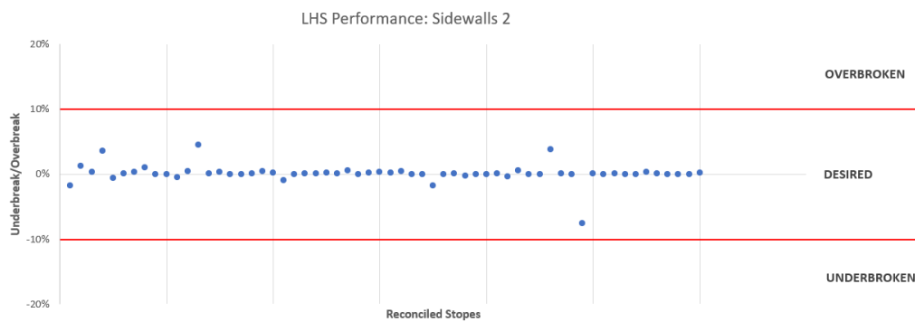
Figure 4-21: LHS performance and sidewalls 2
