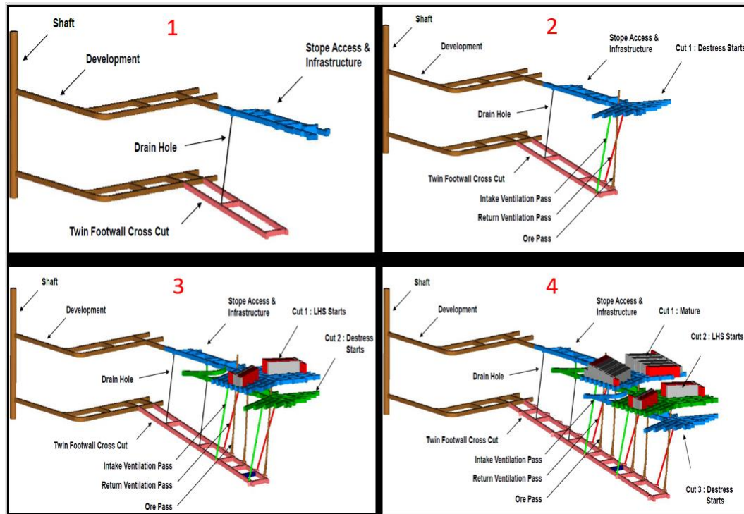
Figure 1-10: High-profile de-stress and long-hole stoping (Collated from Gold Fields (2017))
