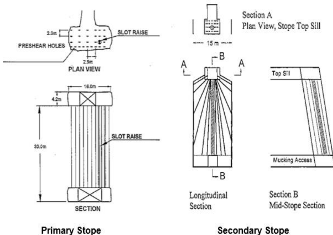
Figure 2-13: Primary and secondary stoping drilling patterns (Ibarra et al., 1996)
