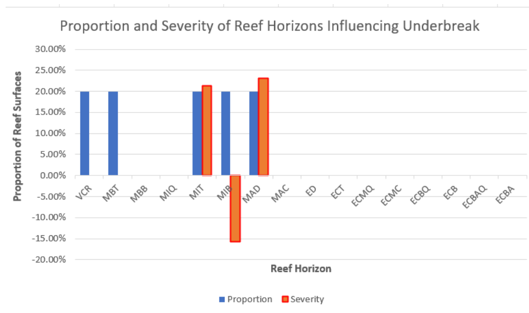
Figure 4-16: Proportion and severity of reef horizons influencing under-break
