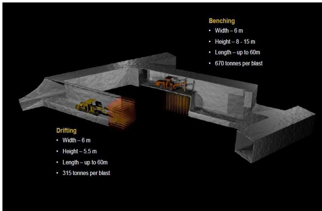
Figure 1-13: Adjacent drifting and benching faces (Gold Fields, 2017)
