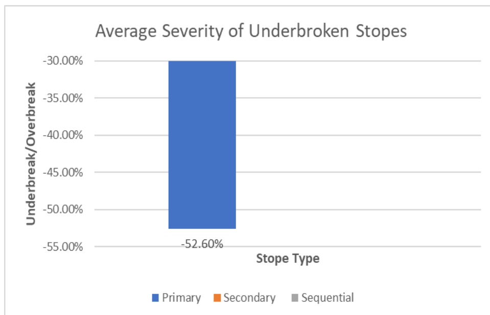
Figure 4-39: Severity of under-broken stopes by mining sequence
