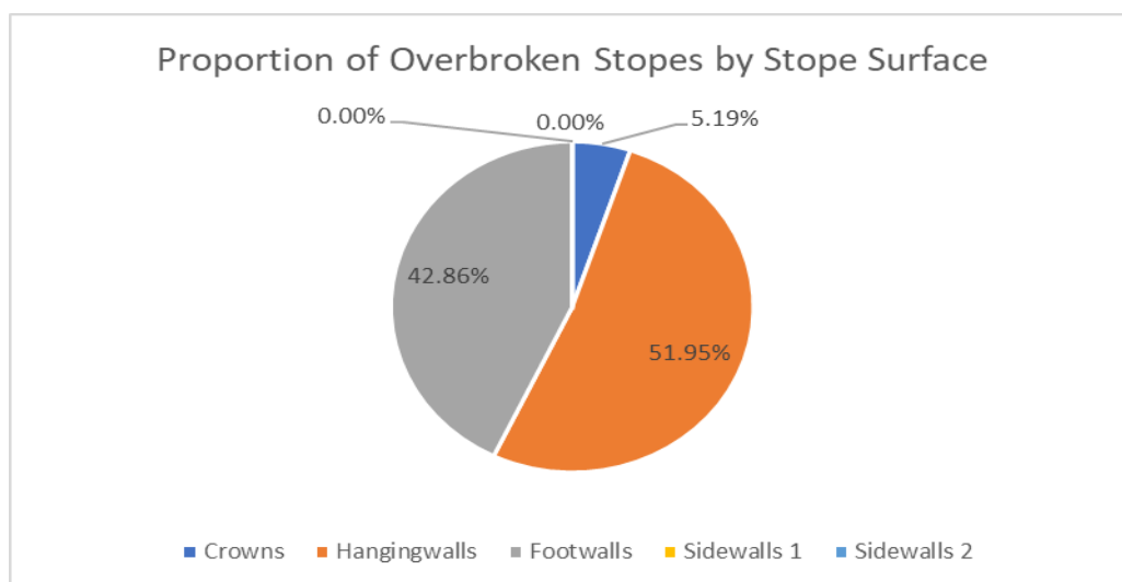
Figure 4-22: Proportion of over-broken stopes by stope surface
