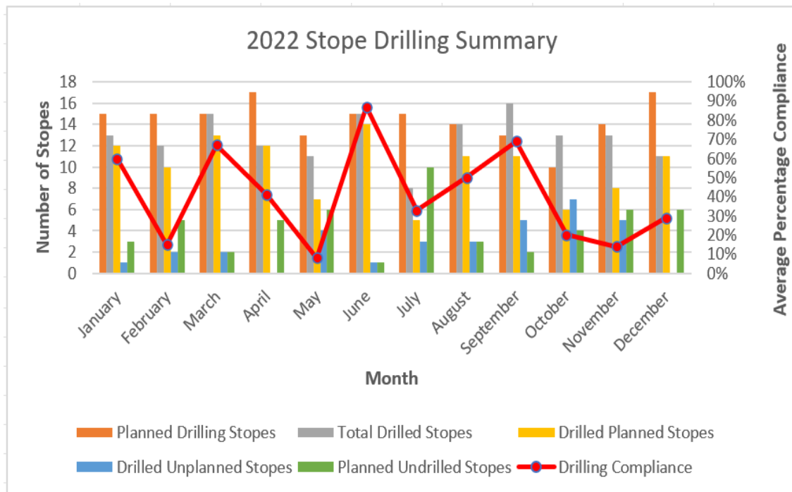
Figure 4-25: 2022 stope drilling summary
