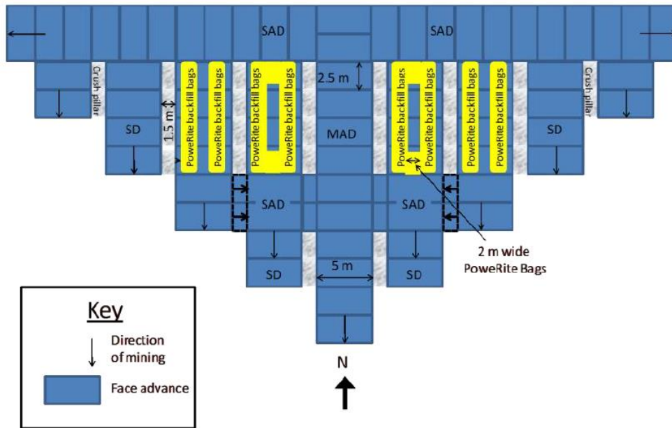
Figure 1-8: Plan view of horizontal de-stress with crush pillar layout (Watson et al., 2014)
