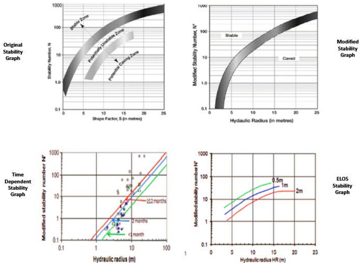
Figure 2-12: Types of stability graphs (Suorineni, 2010)
