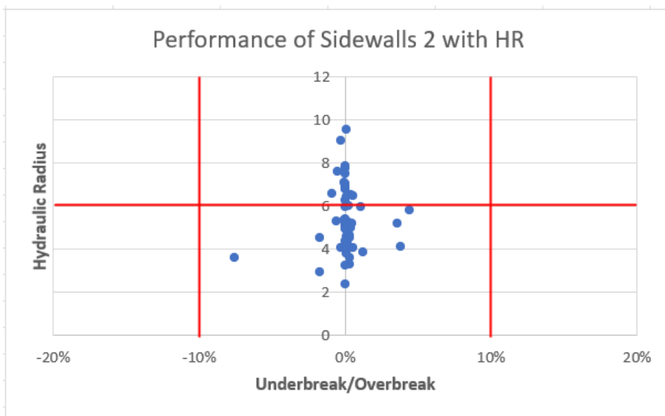
Figure 4-44: Performance of sidewalls 2 with HR
