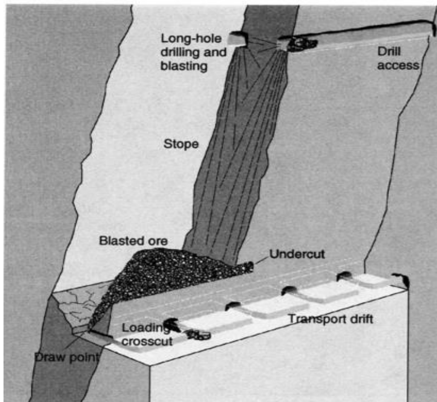
Figure 2-2: Long-hole stoping (Hamrin, 1982)
