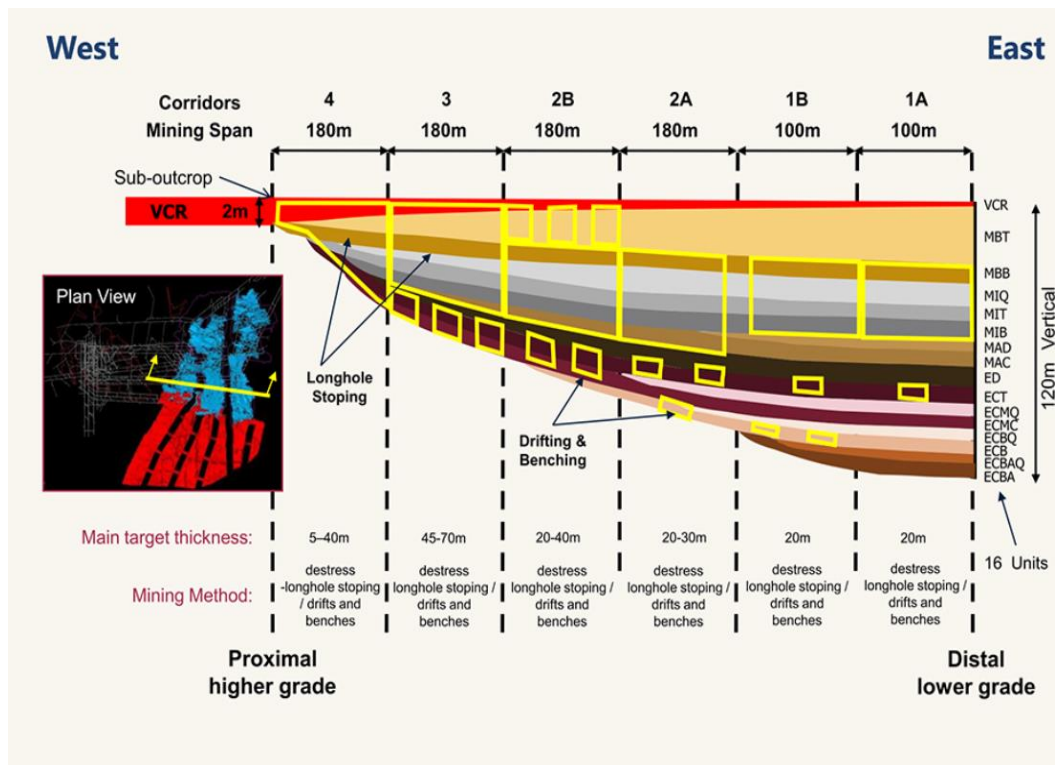
Figure 1-6: Cross-section of the Upper Elsburg orebody (Gold Fields, 2022c)
