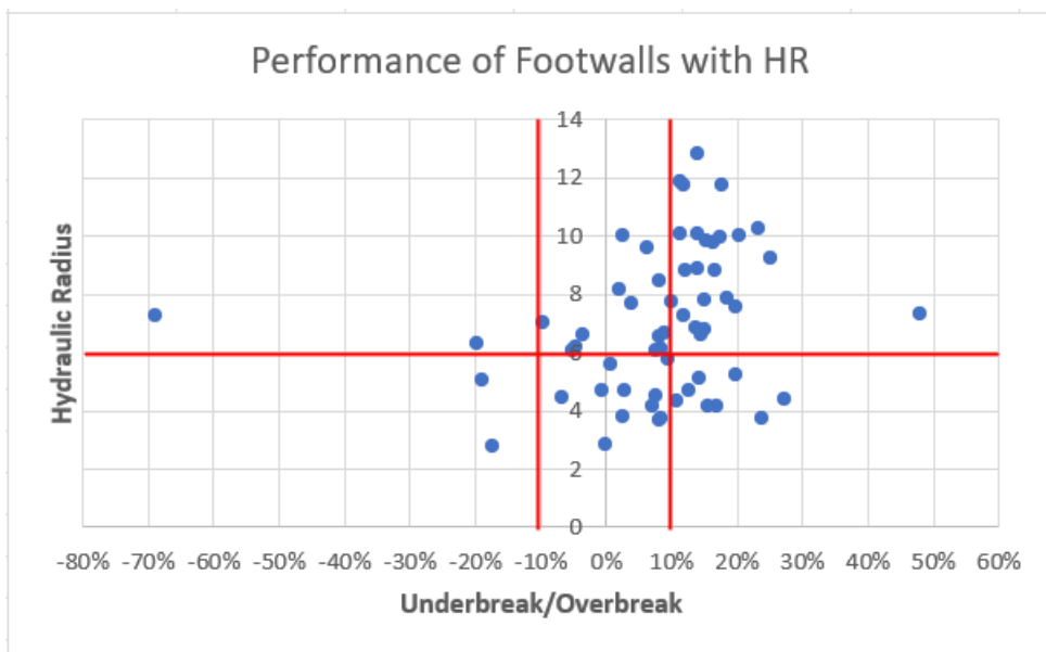
Figure 4-42: Performance of footwalls with HR
