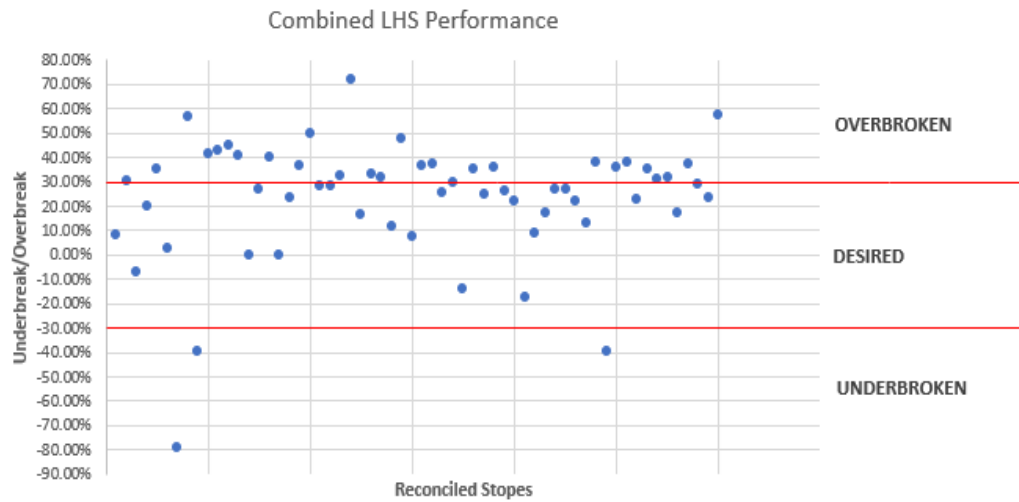
Figure 4-1: Overall LHS performance
