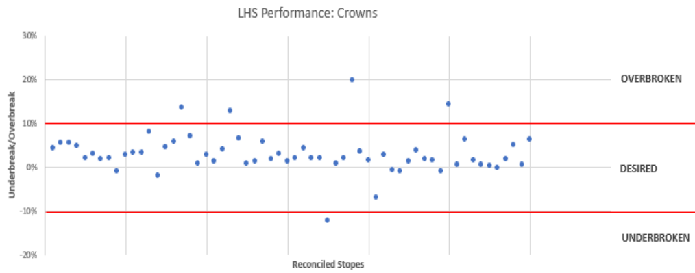
Figure 4-17: LHS performance and crowns
