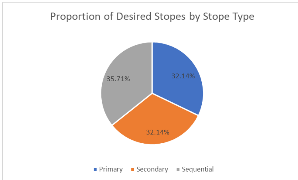
Figure 4-36: Proportion of desired stopes by mining sequence
