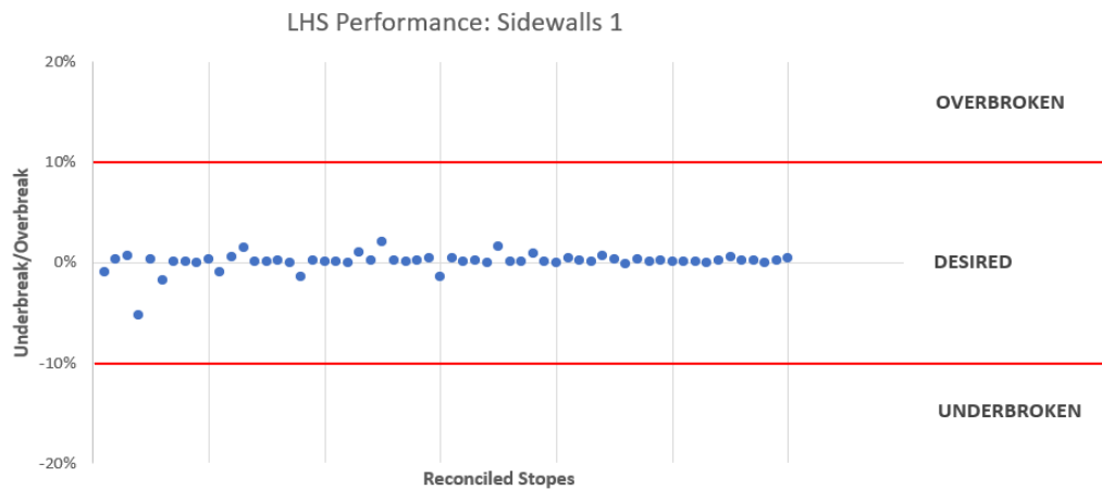
Figure 4-20: LHS performance and sidewalls 1
