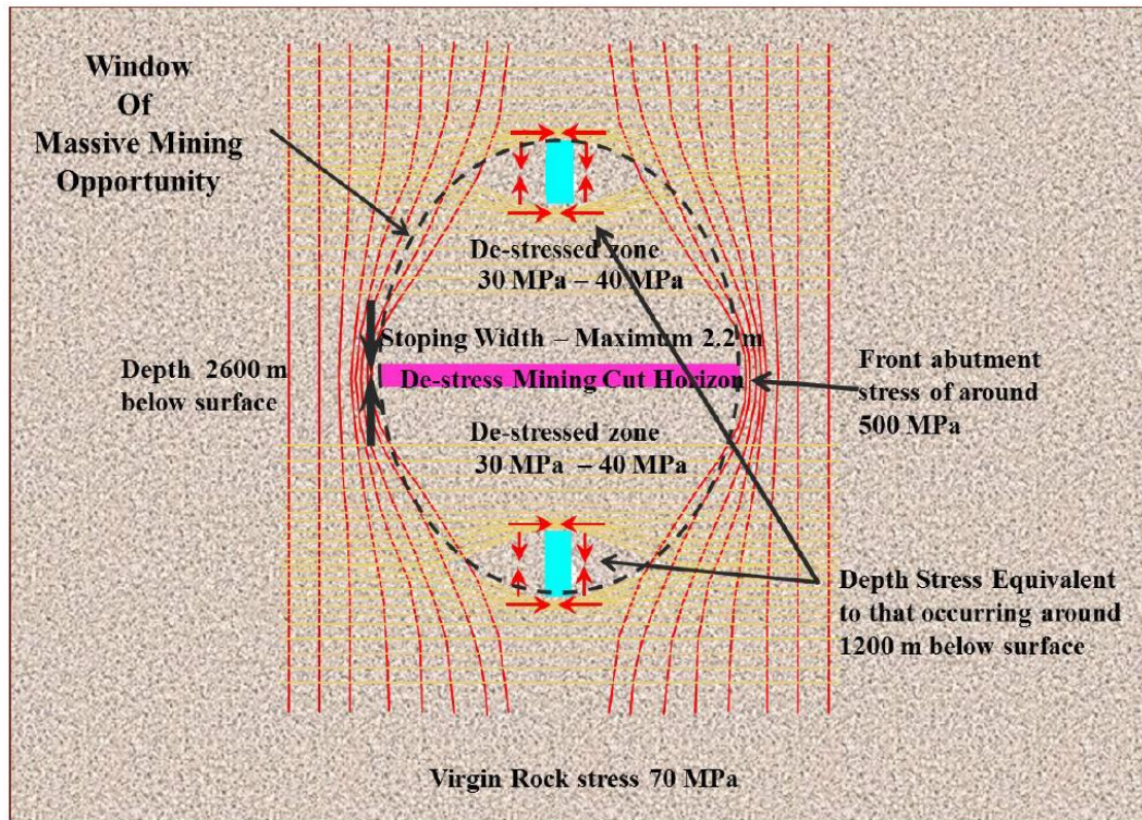
Figure 1-9: South Deep Gold Mine de-stress concept (Watson et al., 2014)
