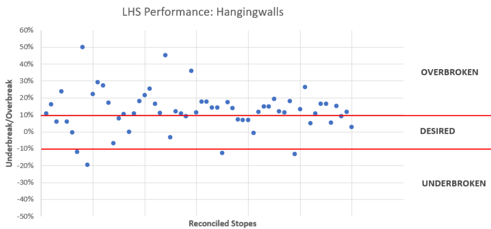
Figure 4-18: LHS performance and hanging walls
