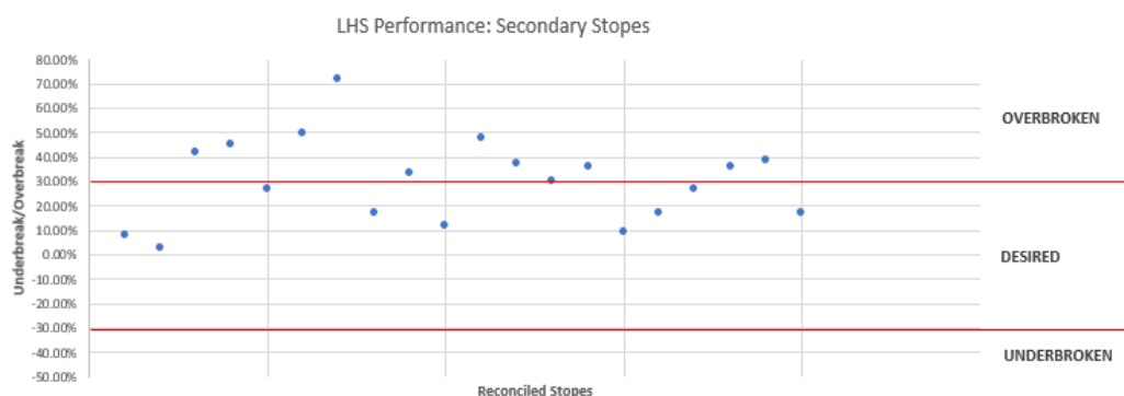
Figure 4-32: LHS performance and secondary stopes
