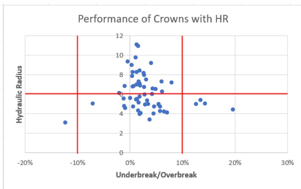
Figure 4-40: Performance of crowns with HR
