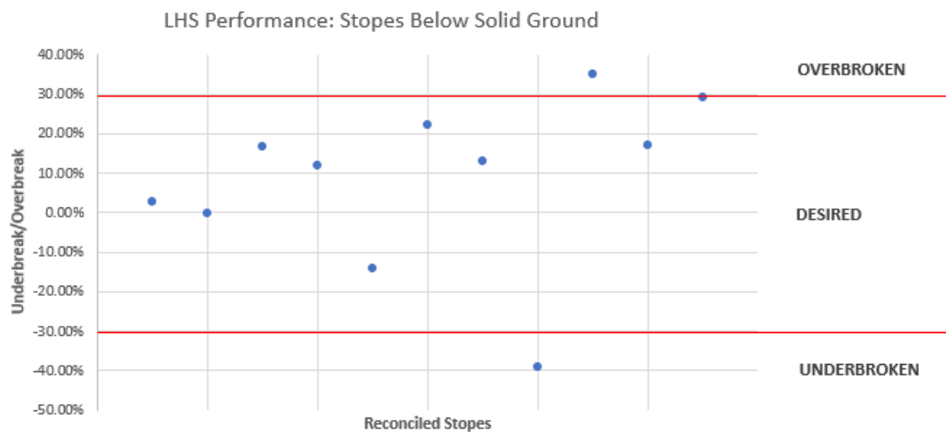
Figure 4-6: Stopes below solid ground
