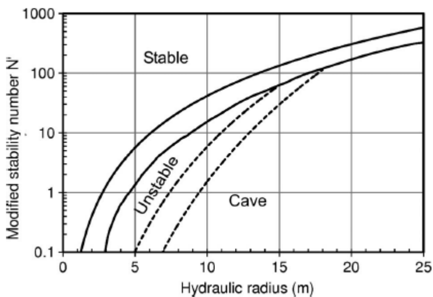
Figure 2-10: Standard stability graph (Suorineni, 2010)
