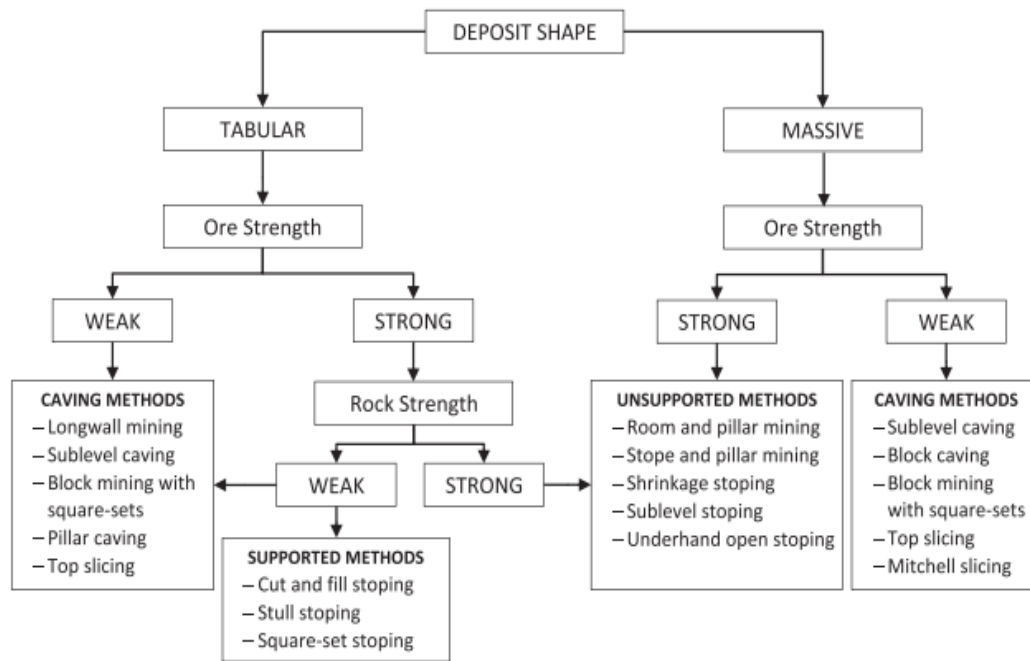
Figure 2-1: Hartman and Mutmanský selection chart (Hartman & Mutmanský, 2002)
