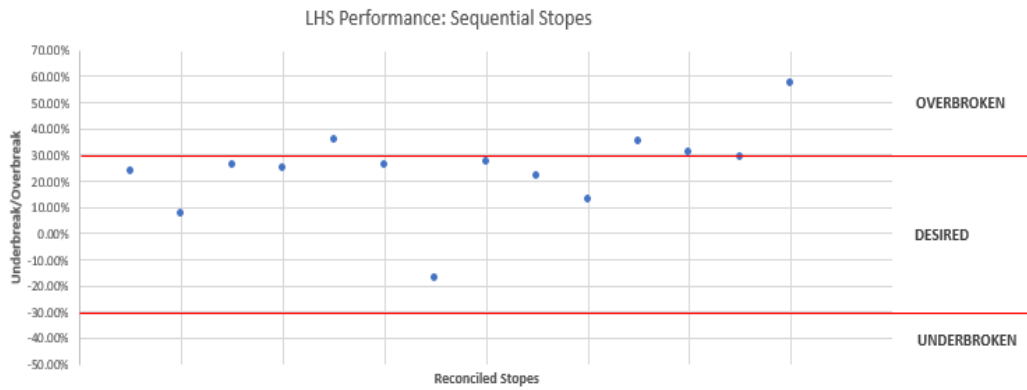
Figure 4-33: LHS performance and sequential stopes
