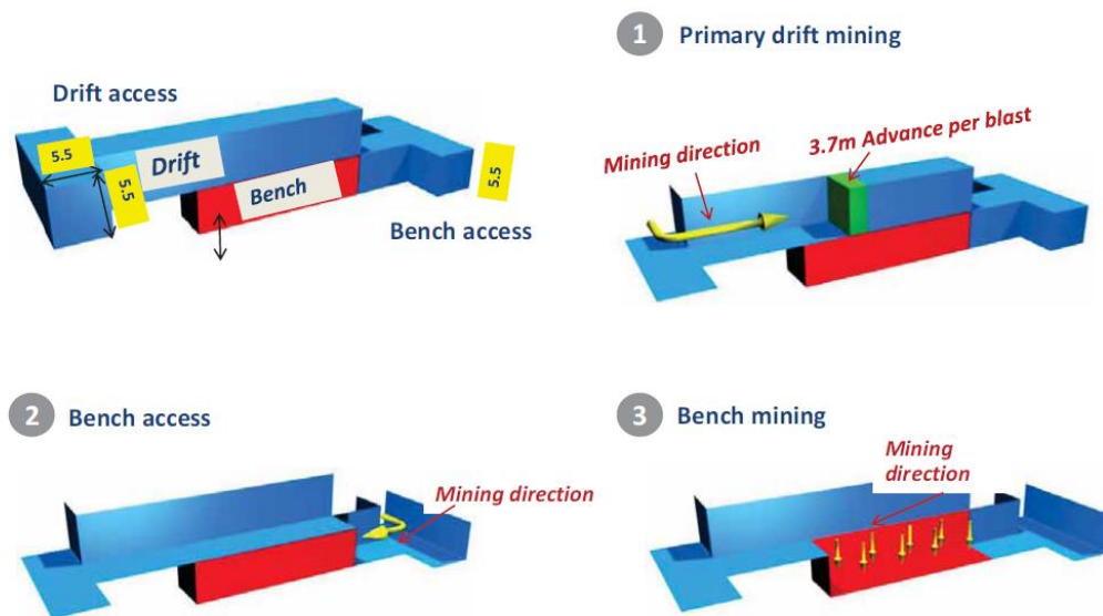
Figure 1-12: Stages and direction of mining in drift and bench mining (Gold Fields, 2013)
