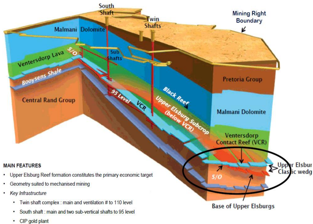
Figure 1-5: Stratigraphic view of the orebody at South Deep Gold Mine (Gold Fields, 2022c)
