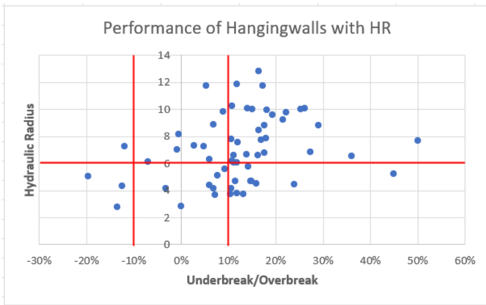
Figure 4-41: Performance of hanging walls with HR
