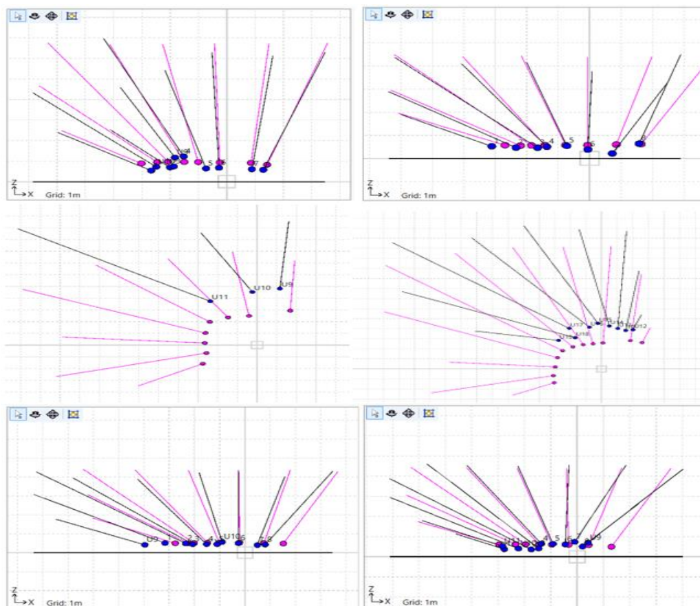
Figure 4-30: Drilling setup report. Planned (purple) and drilled (black) holes
