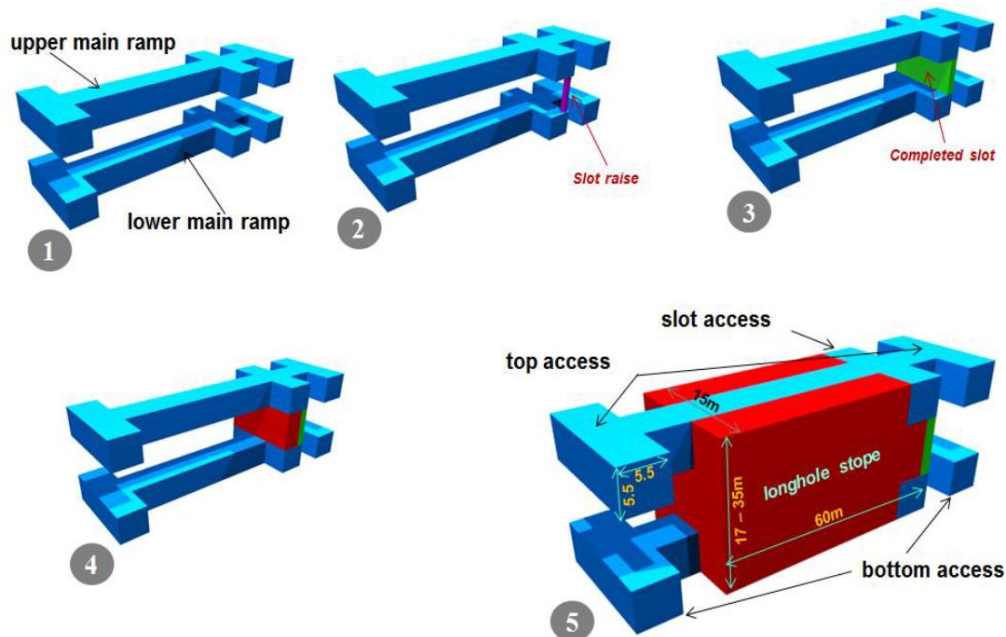
Figure 1-11: Long-hole stope development (Osburn et al., 2014)
