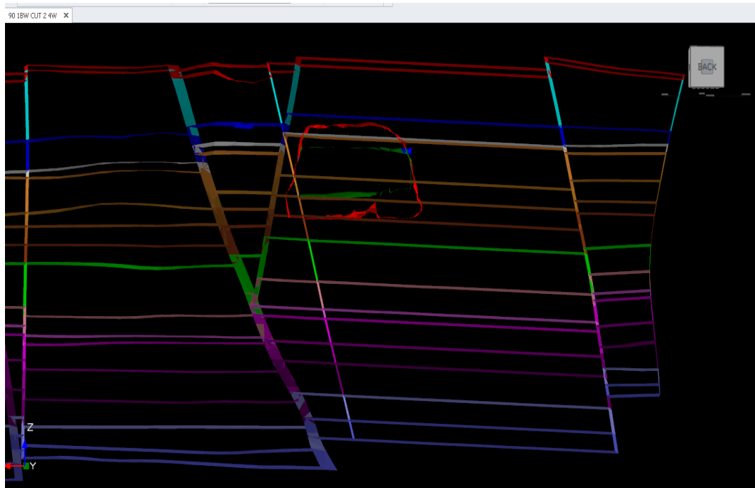
Figure 3-3: LHS cross-section after reef horizon mapping (LHS data files, 2022)
