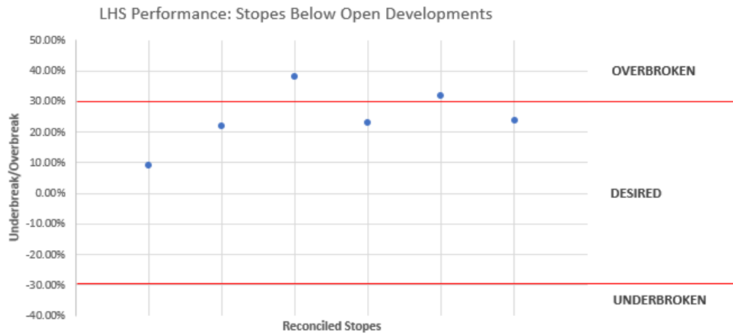
Figure 4-5: Stopes below open developments
