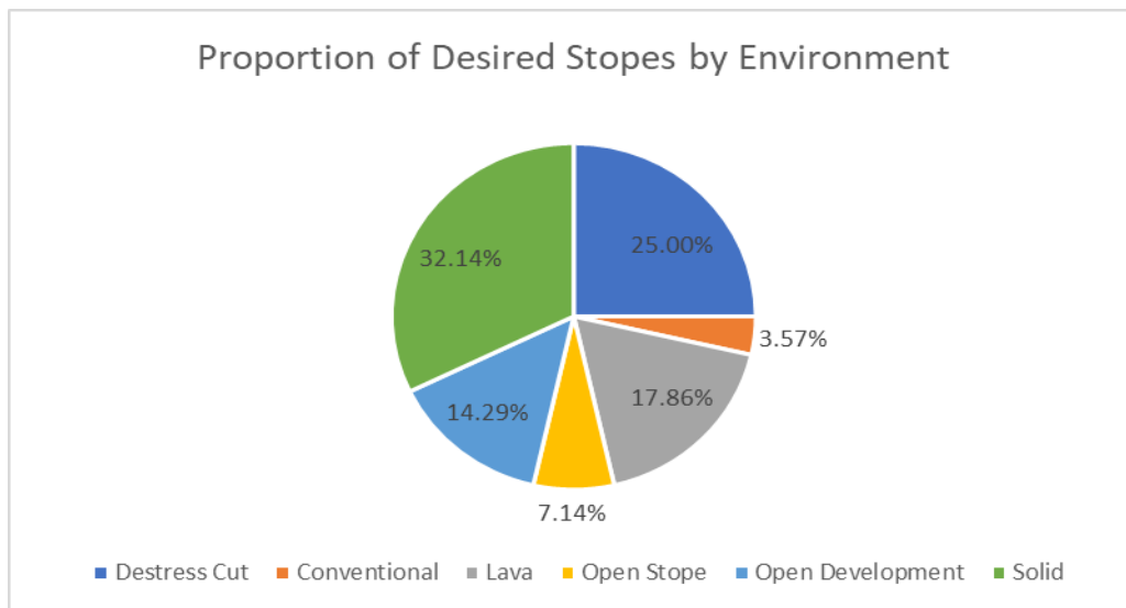
Figure 4-10: Proportion of desired stopes by environment
