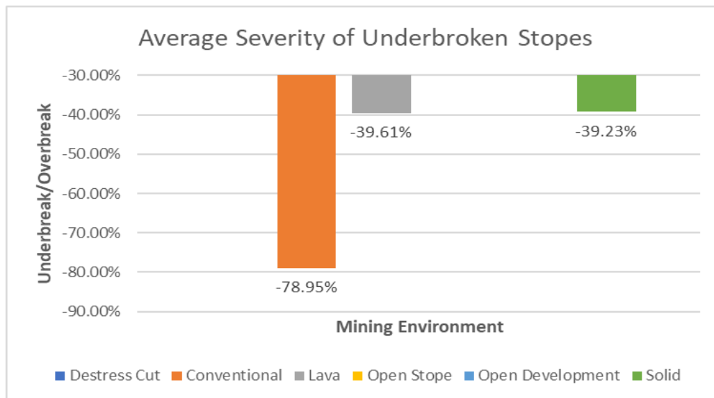
Figure 4-13: Severity of under-broken stopes by environment
