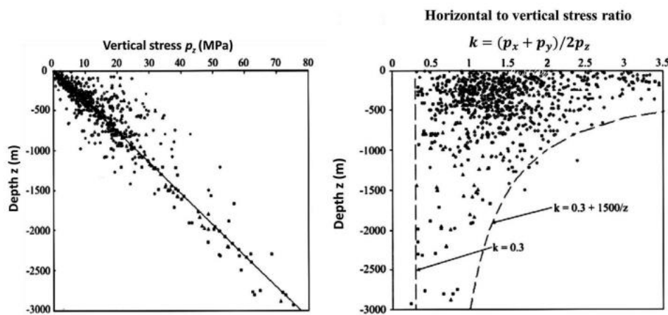
Figure 2-3: Variation of rock stress with depth (Brady & Brown, 2004)
