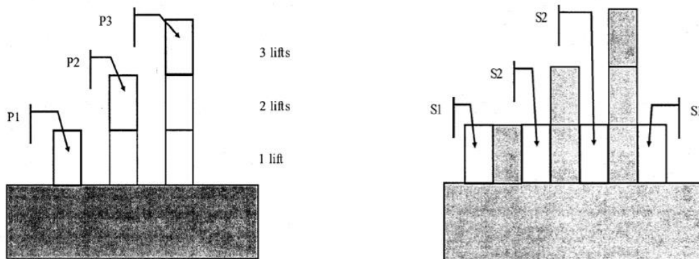
Figure 2-5: Primary and secondary stope mining sequence category (Henning, 2007)
