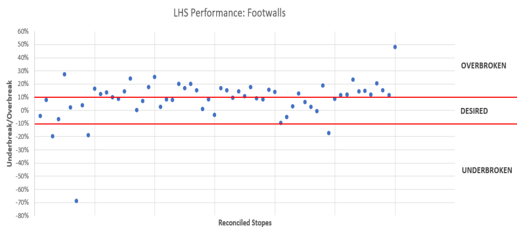
Figure 4-19: LHS performance and footwalls
