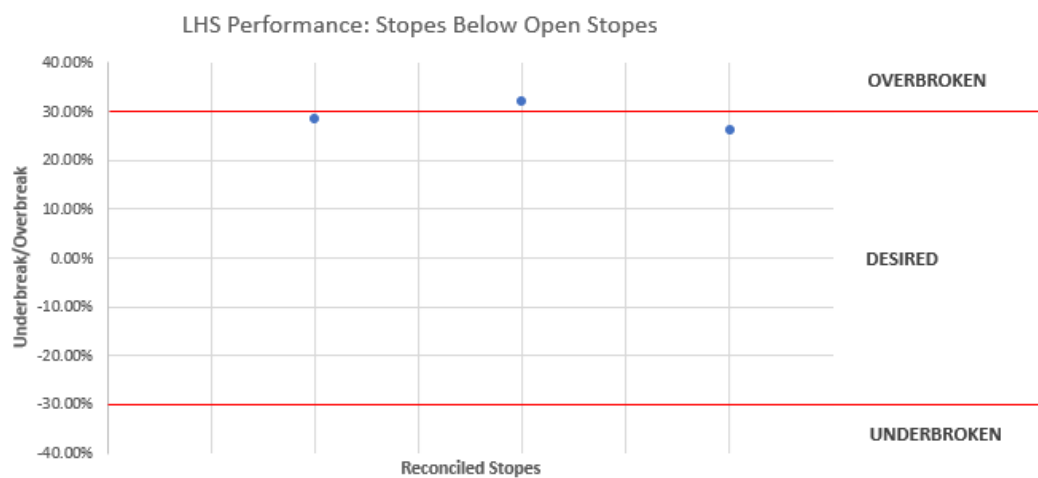
Figure 4-4: Stopes below open stopes
