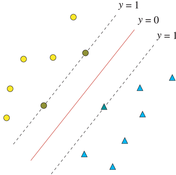
FIGURE 3.4: SVM Hyperplane
