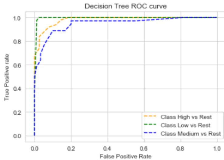
FIGURE 4.9: Decision Tree ROC
