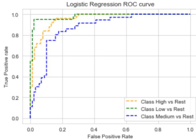
FIGURE 4.6: Logistic Regression ROC
