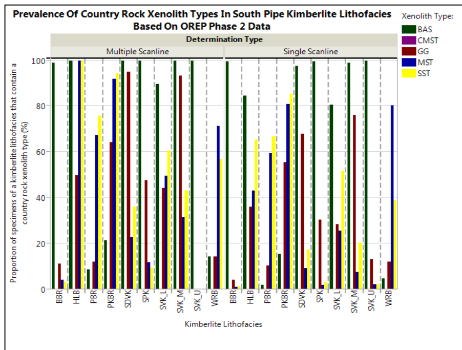
Figure 6.4: Plot of prevalence of country rock xenolith types in South Pipe kimberlite lithofacies based on OREP-2 data.
