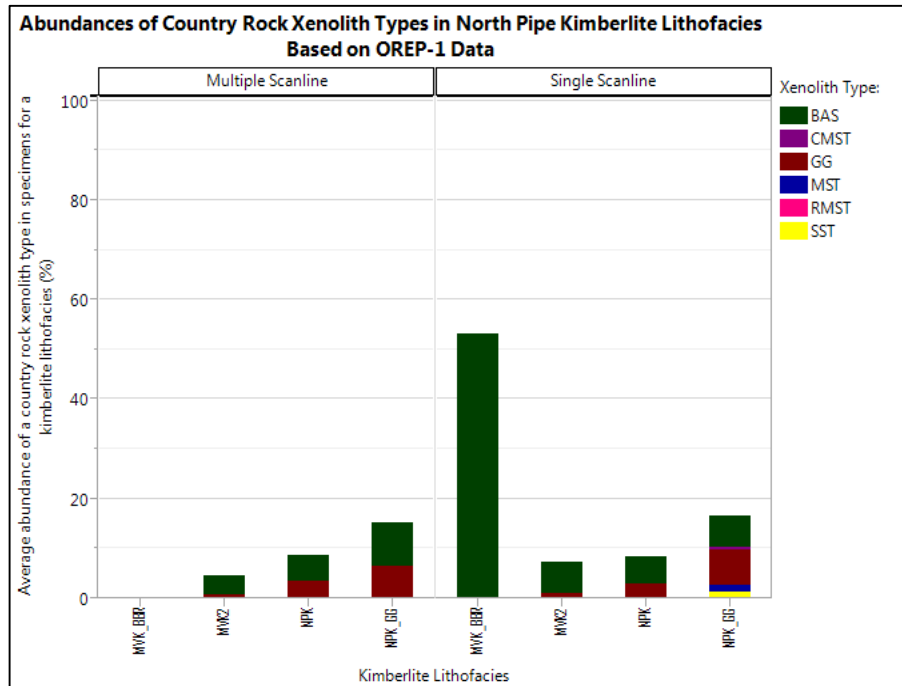
Figure 6.5: Plot of abundances of country rock xenolith types in North Pipe kimberlite lithofacies based on OREP-1 data.
