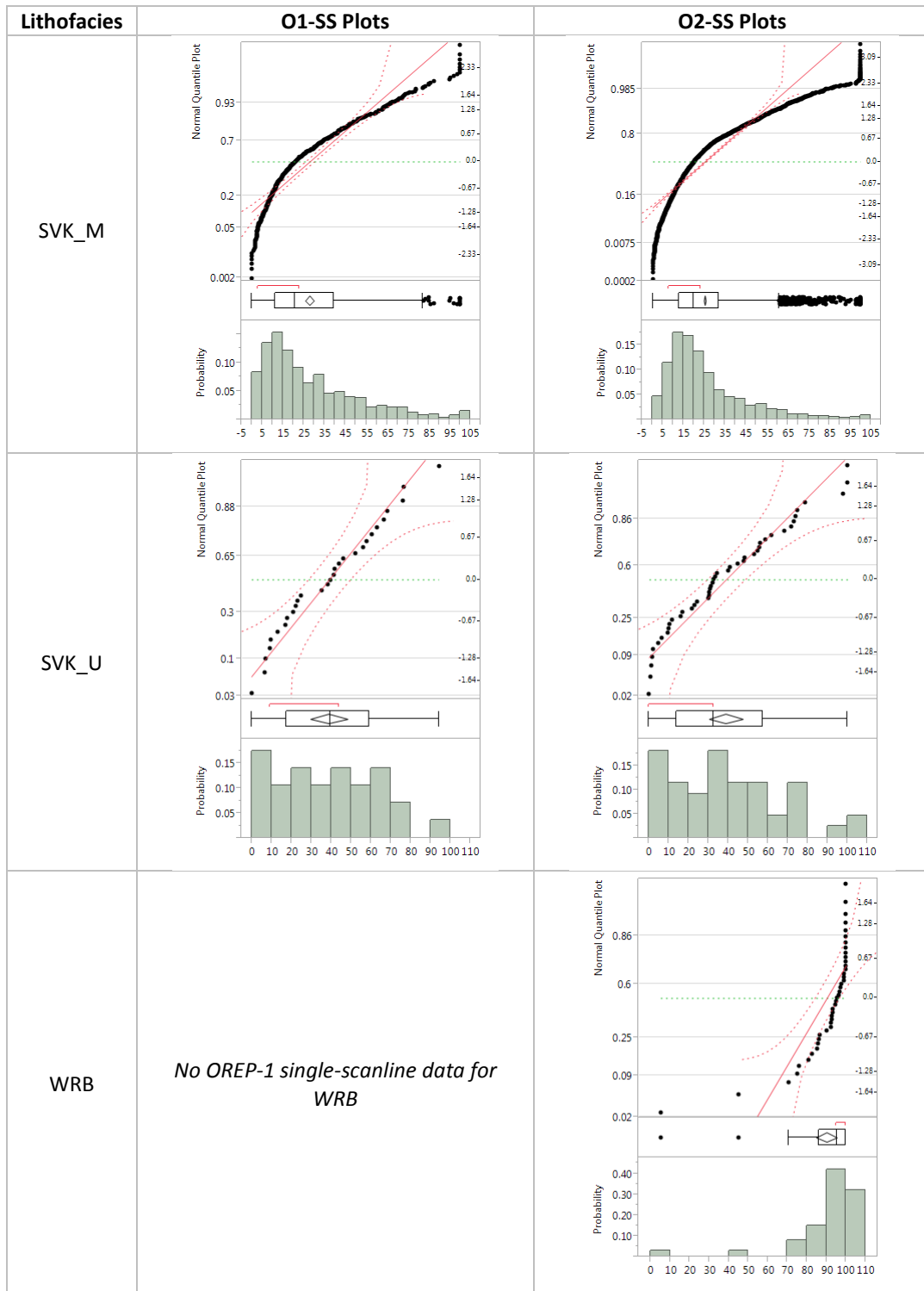
Figure 6.17: Histograms and Q-Q plots of Internal Dilution % for SVK_M, SVK_U and WRB based on single-scanline data.
