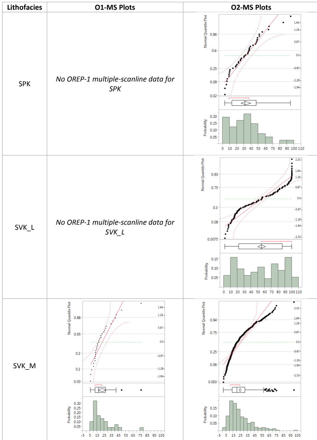
Figure 6.20: Histograms and Q-Q plots of internal dilution for SPK, SVK_L and SVK_M based on multiple-scanline data.
