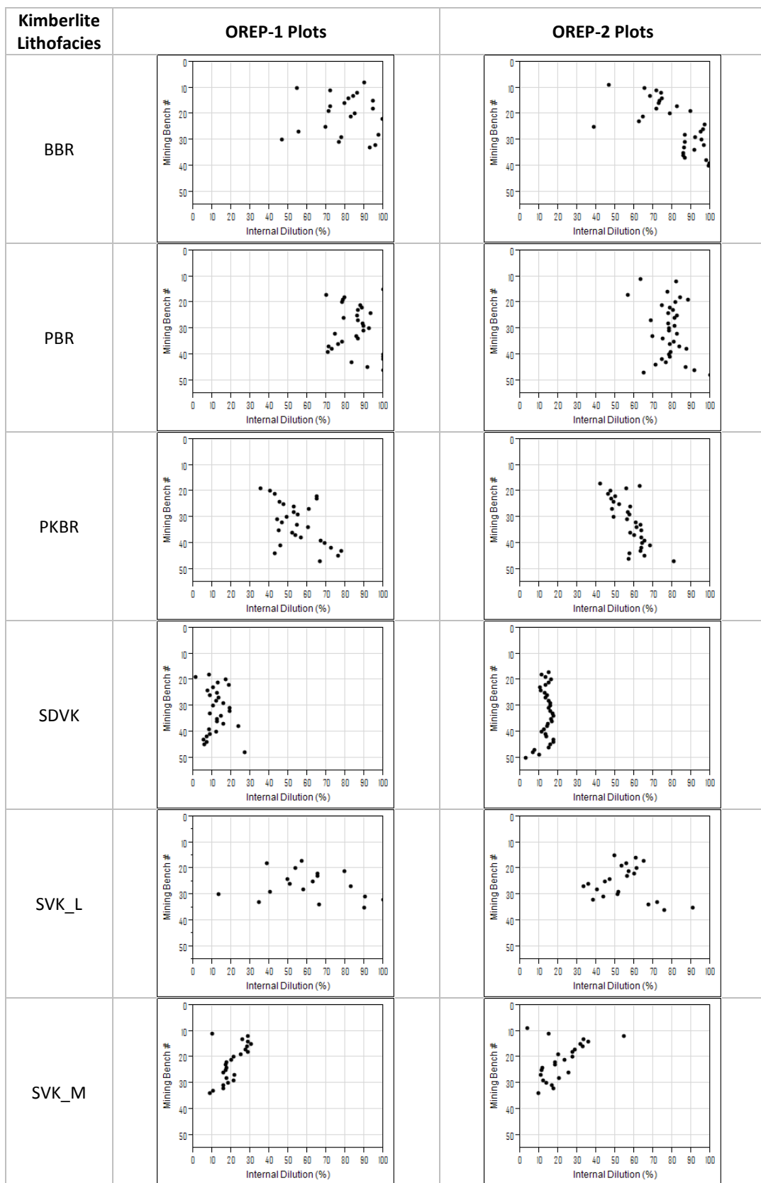
Figure 6.22: Plots of abundances of internal dilution in South Pipe kimberlite lithofacies against mining bench based on single-scanline data.
