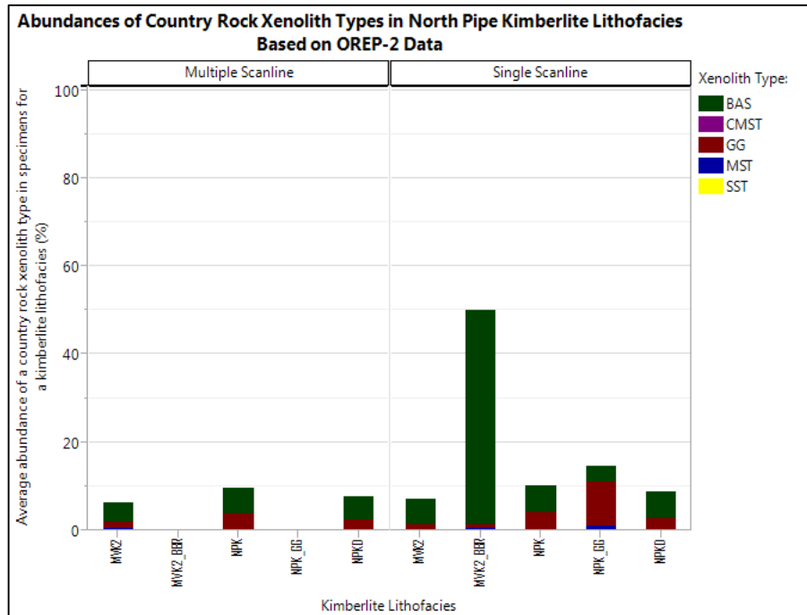
Figure 6.7: Plot of abundances of country rock xenolith types in North Pipe kimberlite lithofacies based on OREP-2 data.
