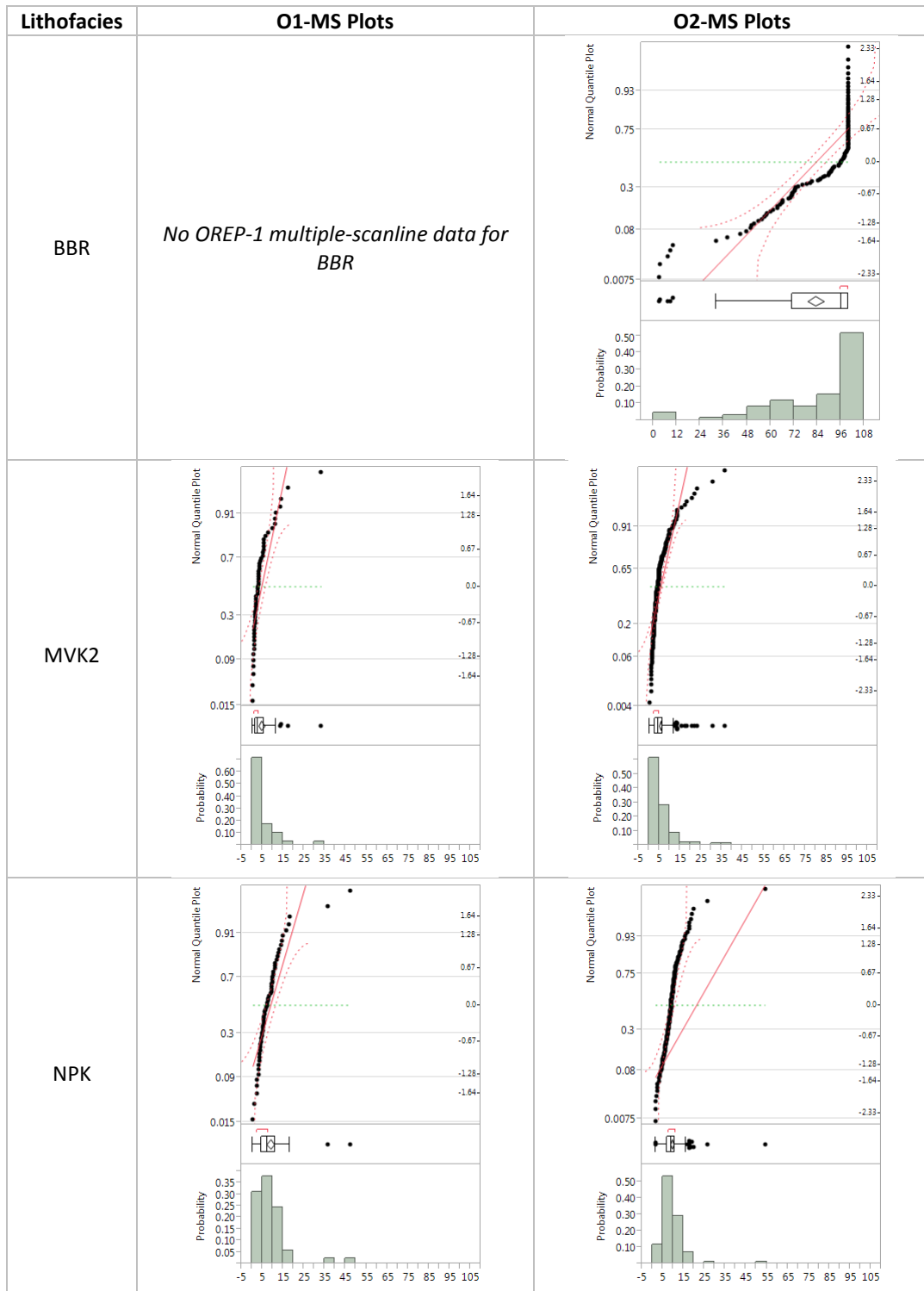
Figure 6.18: Histograms and Q-Q plots of Internal Dilution % for BBR, MVK2 and NPK based on multiple-scanline data.
