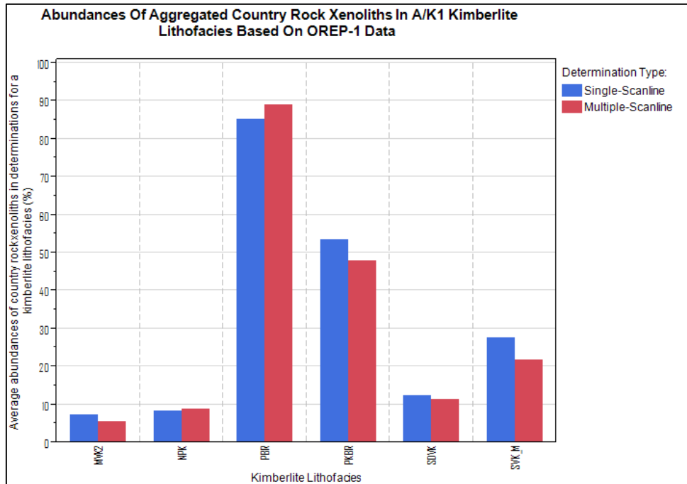
Figure 6.9: Plot of abundances of country rock xenoliths in A/K1 kimberlite lithofacies based on OREP-1 data.
