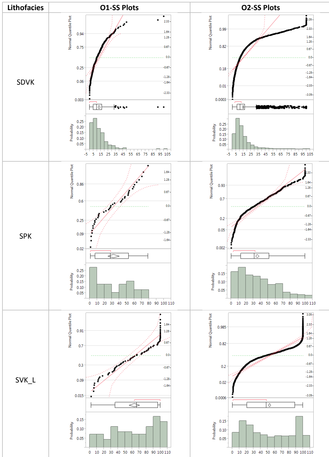
Figure 6.16: Histograms and Q-Q plots of Internal Dilution % for SDVK, SPK and SVK_L based on single-scanline data.
