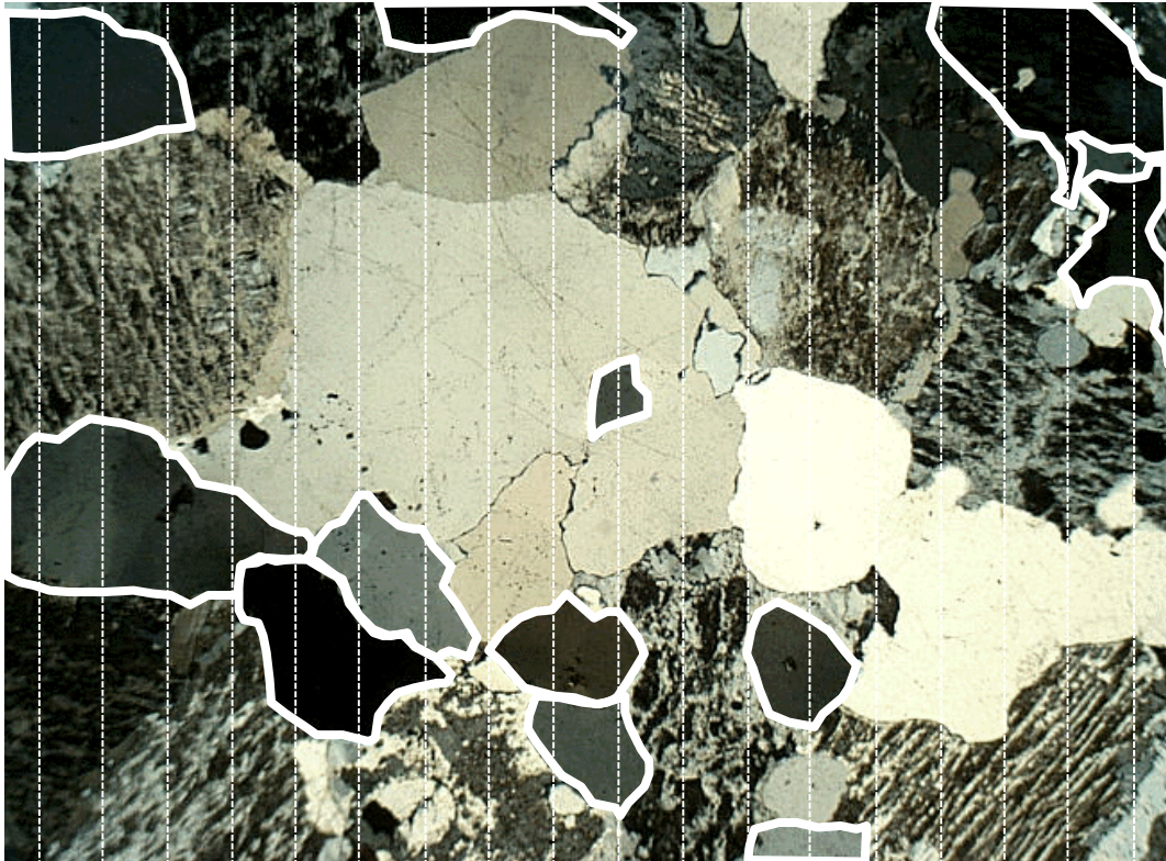
Figure 4.2: Illustration of Rosiwal's transects (lines) based stereological technique (NB. The lengths of the dashed lines over the white-rimmed target particles were measured).
