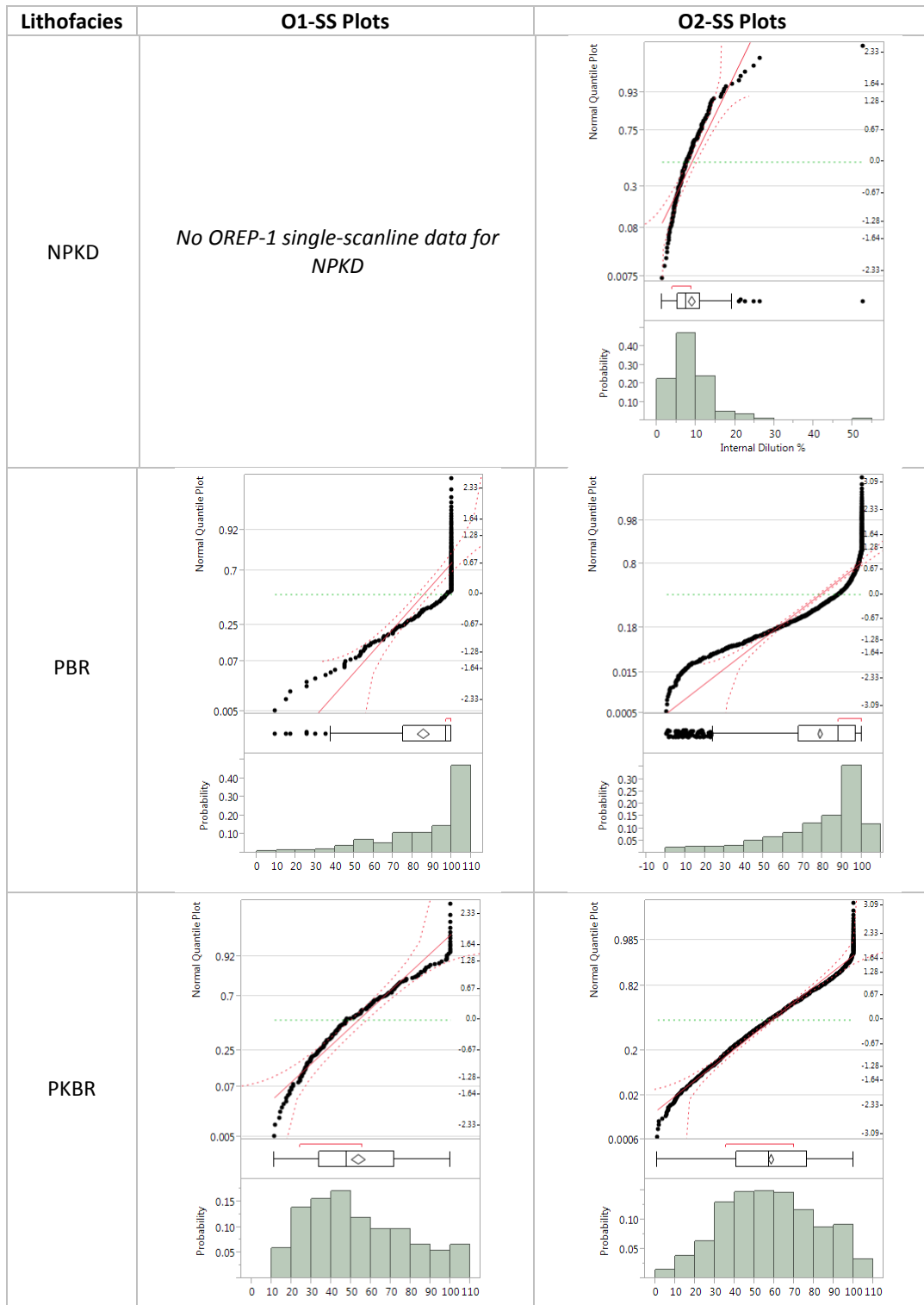
Figure 6.15: Histograms and Q-Q plots of Internal Dilution % for NPKD, PBR and PKBR based on single-scanline data.
