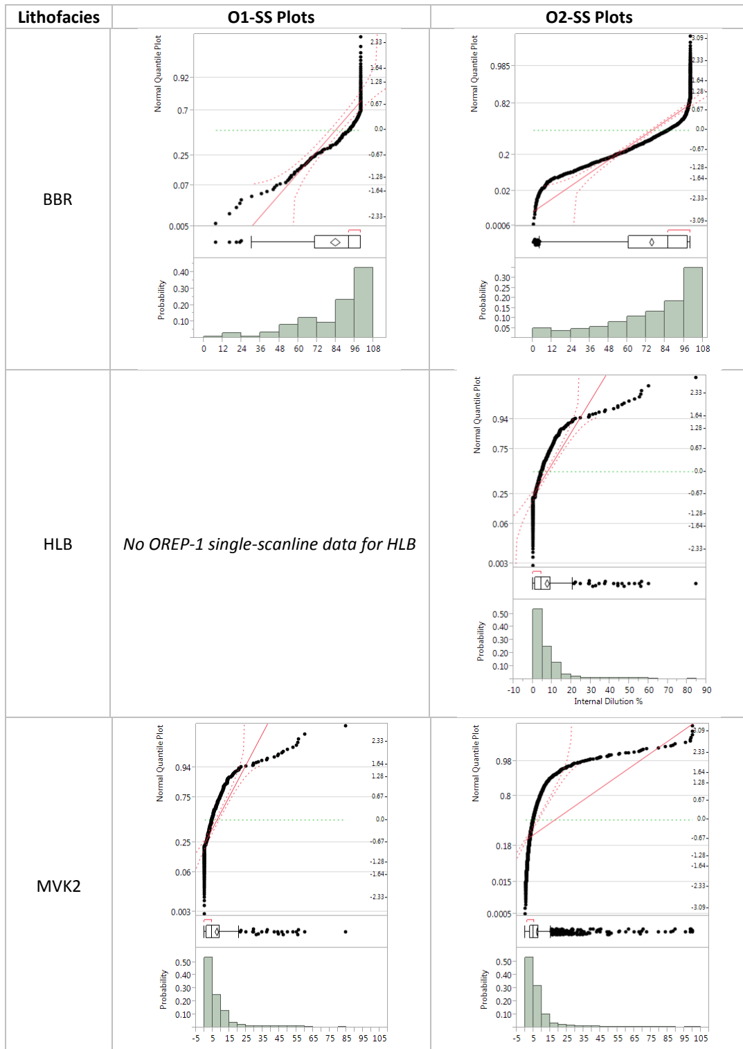
Figure 6.13: Histograms and Q-Q plots of Internal Dilution % for BBR, HLB and MVK2 based on single-scanline data.
