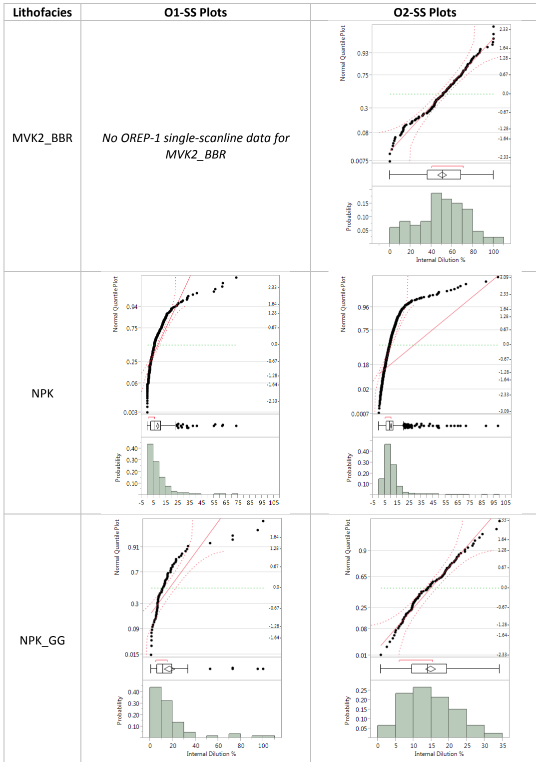
Figure 6.14: Histograms and Q-Q plots of Internal Dilution % for MVK2_BBR, NPK_GG and NPK based on single-scanline data.
