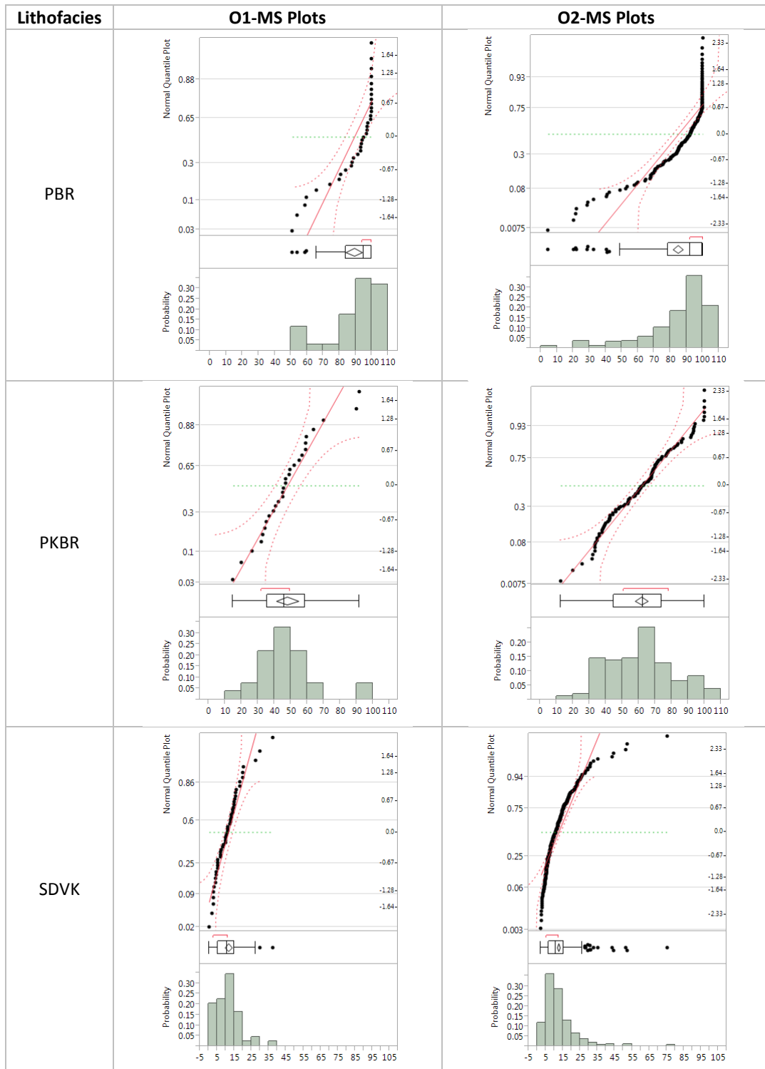
Figure 6.19: Histograms and Q-Q plots of Internal Dilution % for PBR, PKBR and SDVK based on multiple-scanline data.
