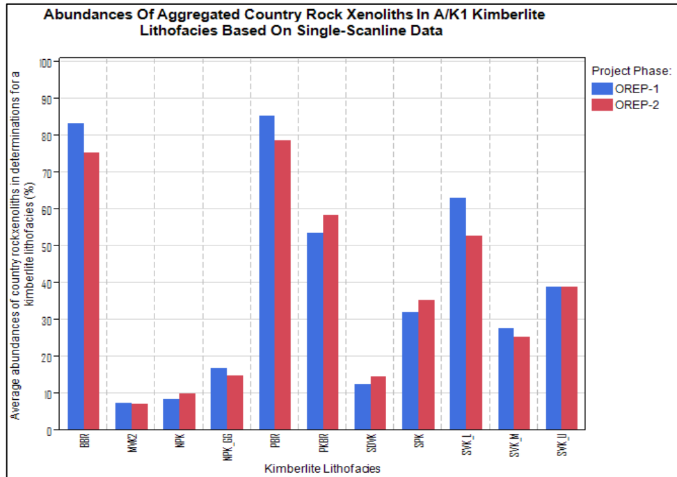
Figure 6.11: Plot of abundances of country rock xenoliths in A/K1 kimberlite lithofacies based on single-scanline data.
