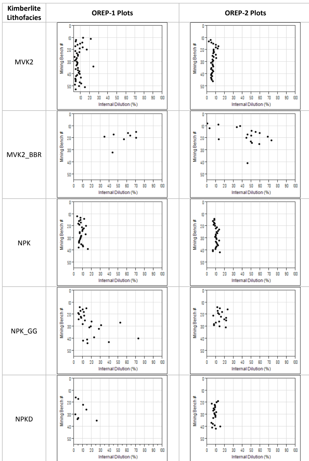
Figure 6.21: Plots of abundances of internal dilution in North Pipe kimberlite lithofacies against mining bench based on single-scanline data.
