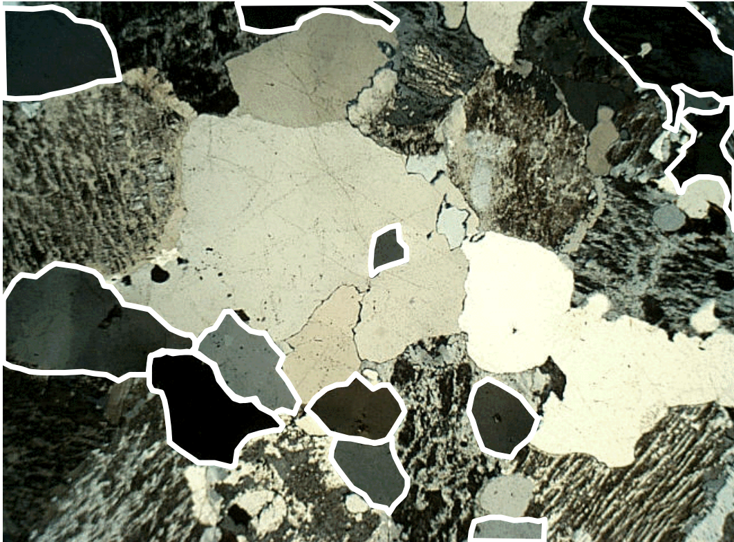
Figure 4.1: Illustration of Delesse's area based stereological technique (NB. The areas of the white-rimmed target particles were measured).
