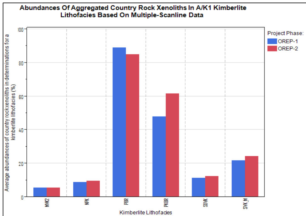
Figure 6.12: Plot of abundances of country rock xenoliths in A/K1 kimberlite lithofacies based on multiple-scanline data.
