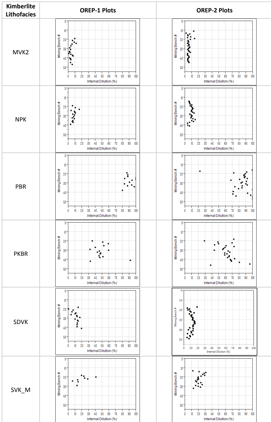
Figure 6.23: Plots of abundances of internal dilution in A/K1 kimberlite lithofacies against mining bench based on multiple-scanline data.
