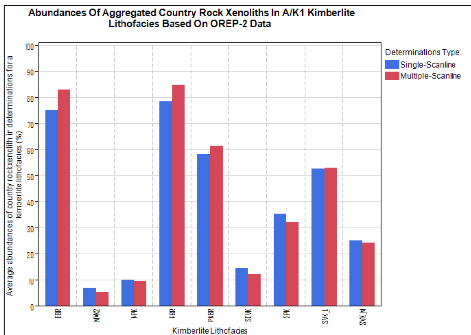
Figure 6.10: Plot of abundances of country rock xenoliths in A/K1 kimberlite lithofacies based on OREP-2 data.
