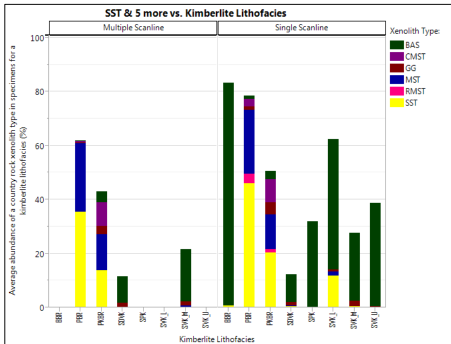
Figure 6.6: Plot of abundances of country rock xenolith types in South Pipe kimberlite lithofacies based on OREP-1 data.
