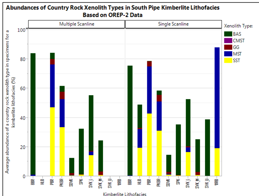
Figure 6.8: Plot of abundances of country rock xenolith types in South Pipe kimberlite lithofacies based on OREP-2 data.
