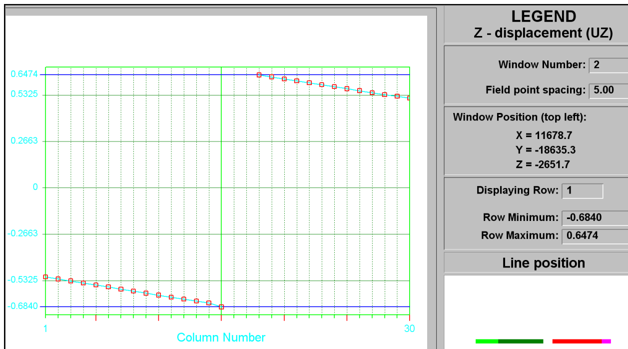
Figure C-57 UZ closure at STEP 12
