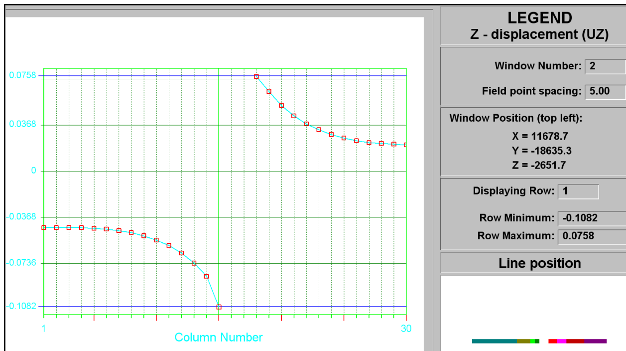
Figure C-47 UZ closure at STEP 2
