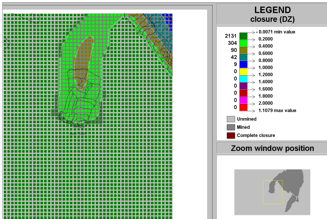
Figure C-183 Contour plot of closure (DZ) of Ya Rona shaft barrel area in Block E at STEP 3
