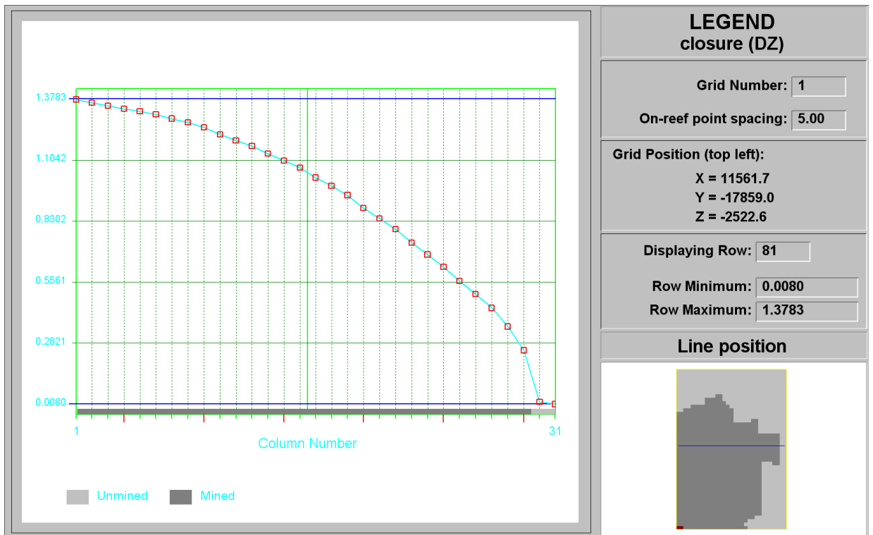
Figure C-202 Contour plot of closure (DZ) of Ya Rona shaft barrel area in Block F at STEP 15
