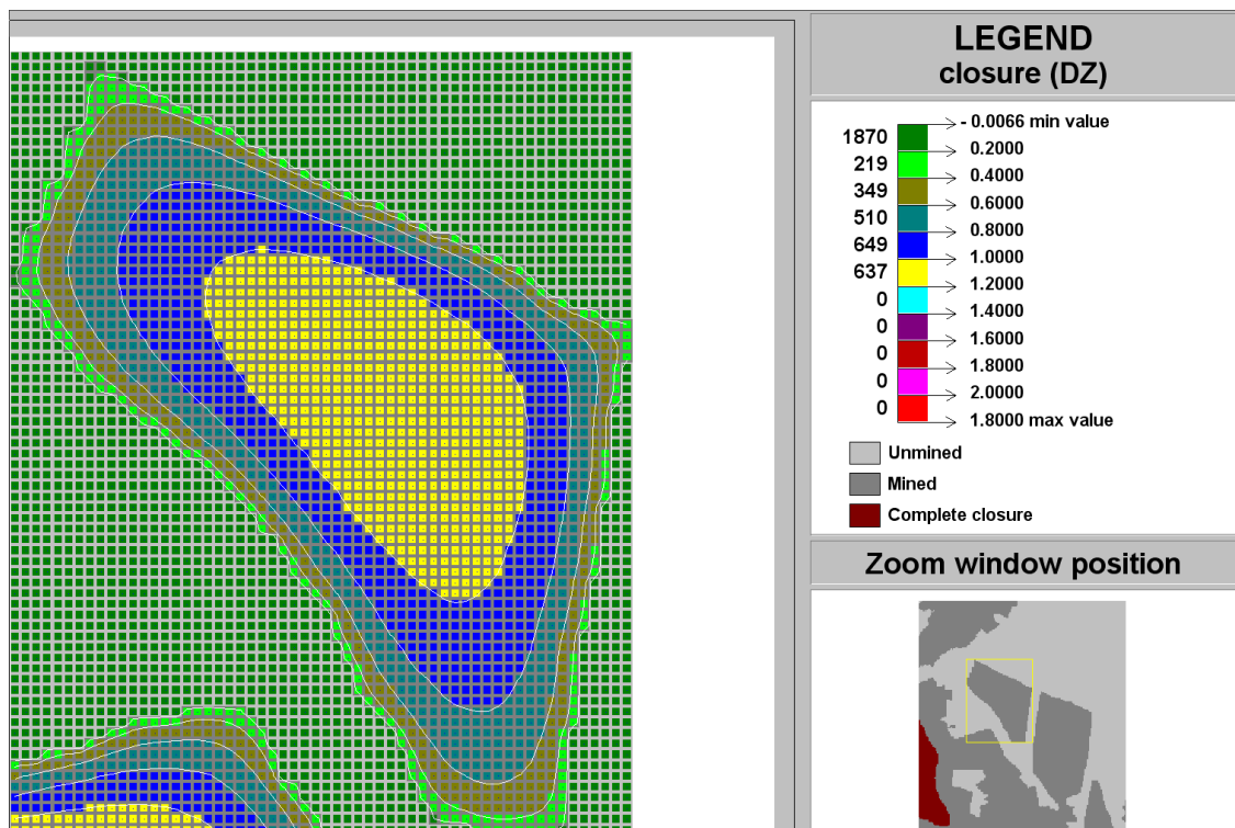
Figure C-167 Contour plot of closure (DZ) of Ya Rona shaft barrel area in Block C at STEP 15
