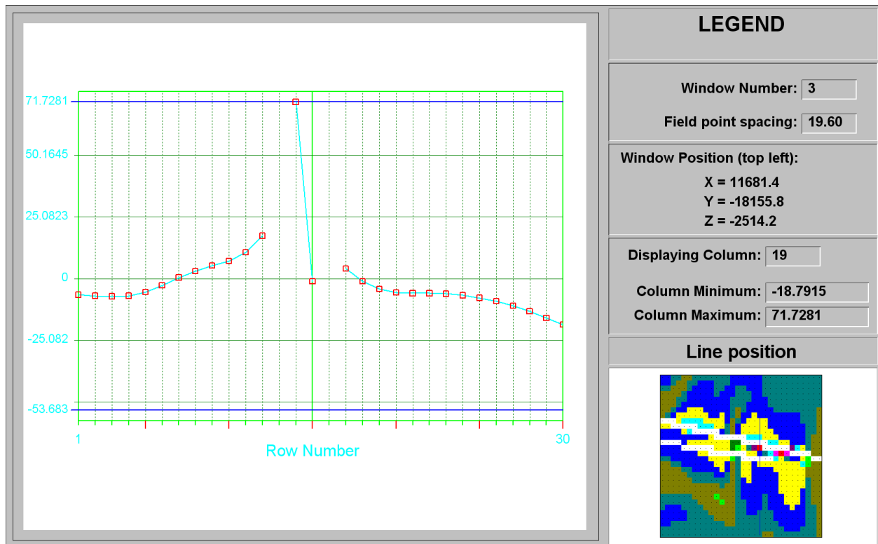
Figure C-90 ESS line plot at column 19 of Murray Fault at STEP 15
