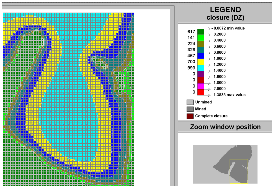
Figure C-179 Contour plot of closure (DZ) of Ya Rona shaft barrel area in Block D at STEP 14
