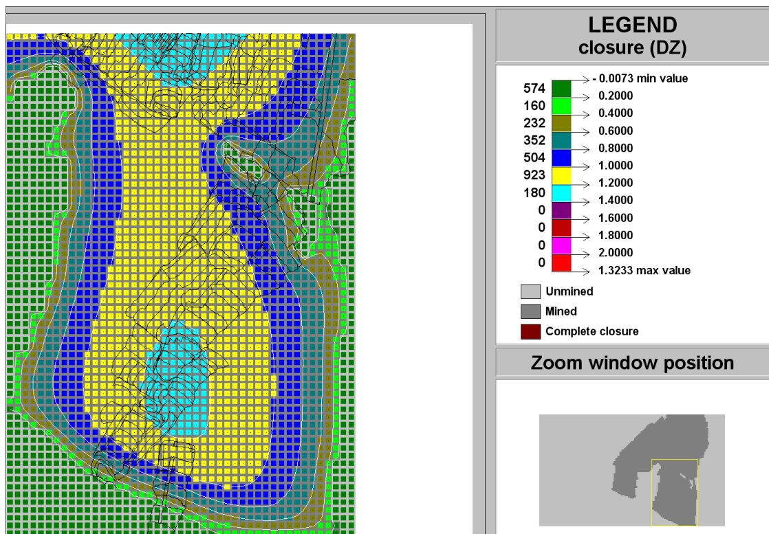
Figure C-177 Contour plot of closure (DZ) of Ya Rona shaft barrel area in Block D at STEP 12
