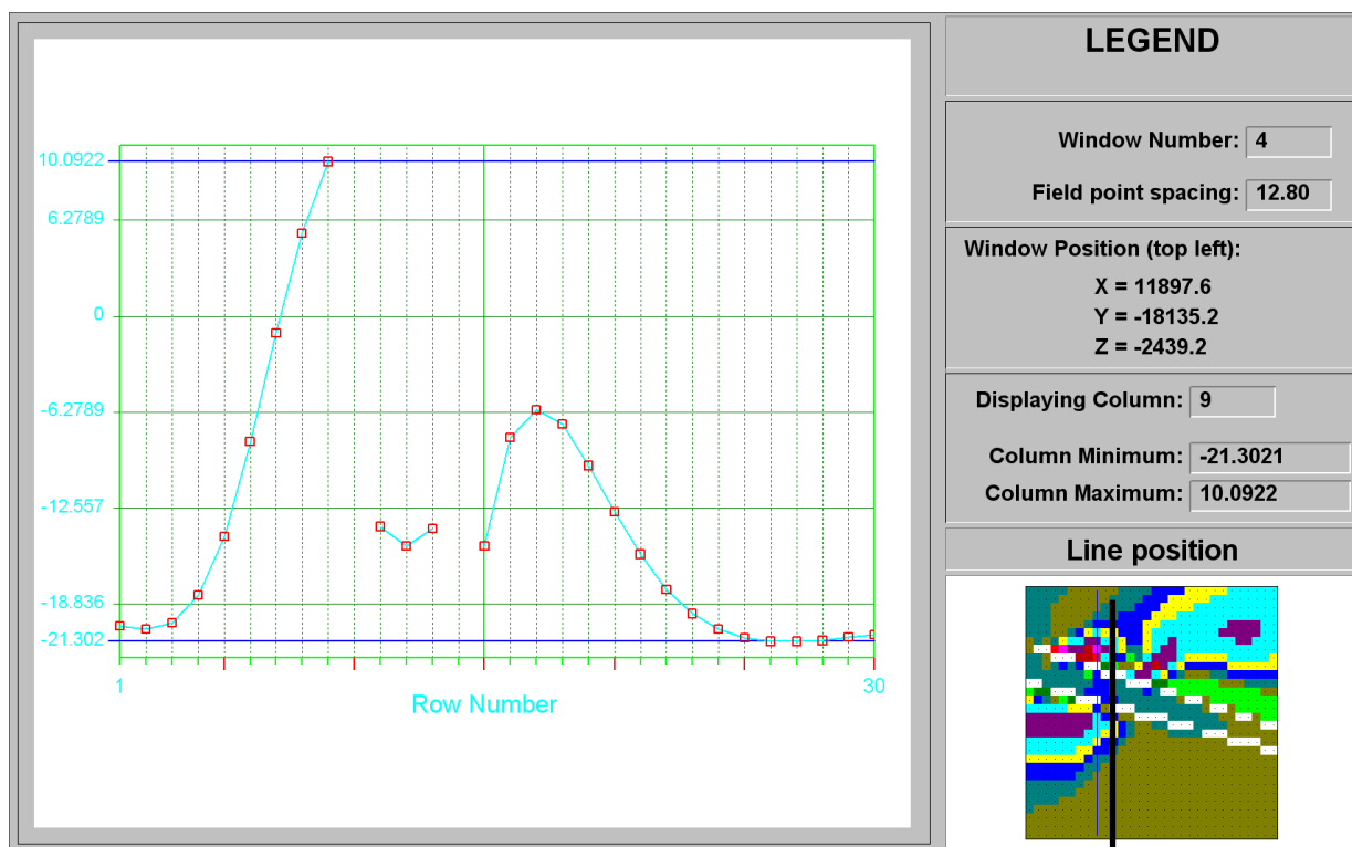
Figure C-66 ESS line plot at column 9 of Kate's Fault at STEP 6
