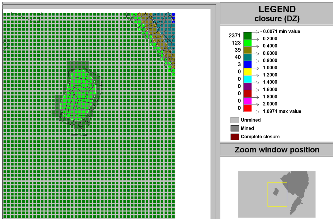
Figure C-181 Contour plot of closure (DZ) of Ya Rona shaft barrel area in Block E at STEP 1
