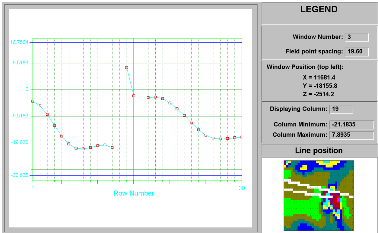
Figure C-80 ESS line plot at column 19 of Murray Fault at STEP 5
