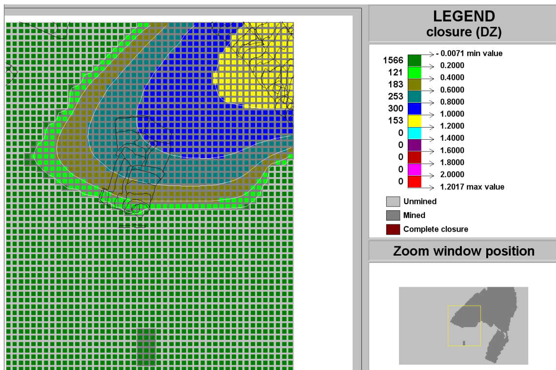
Figure C-188 Contour plot of closure (DZ) of Ya Rona shaft barrel area in Block E at STEP 8
