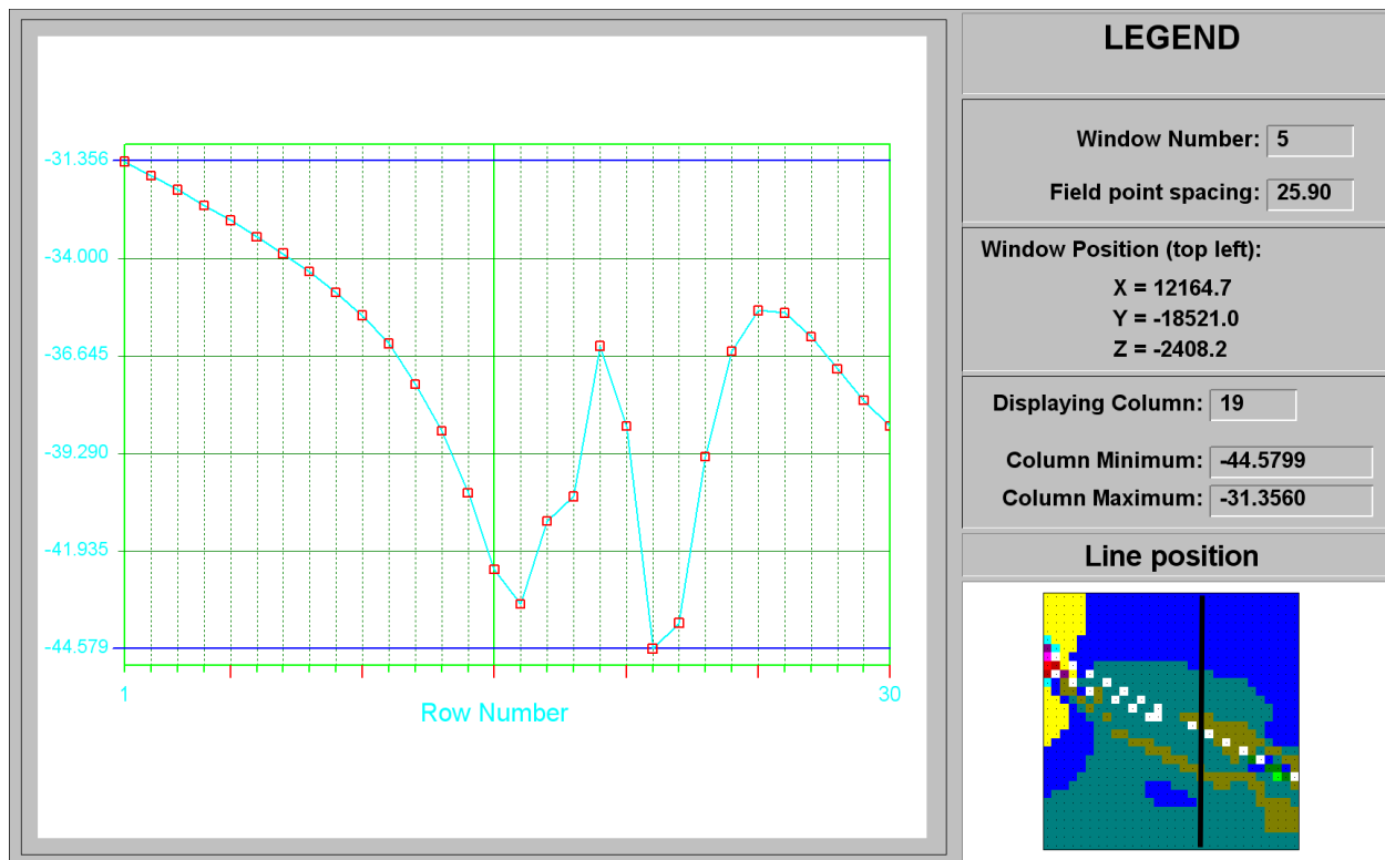
Figure C-95 ESS line plot at column 19 of Smith Fault at STEP 5
