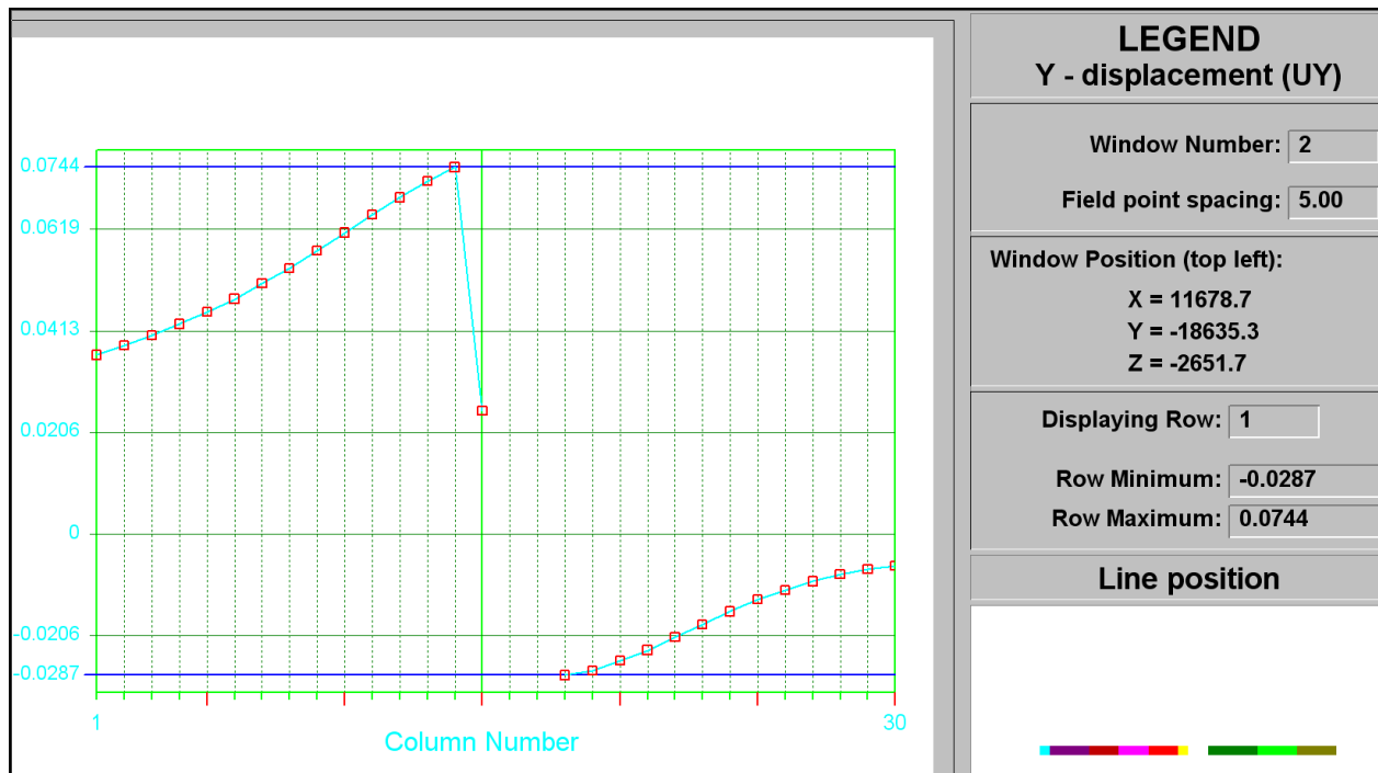
Figure C-18 UY closure at STEP 3
