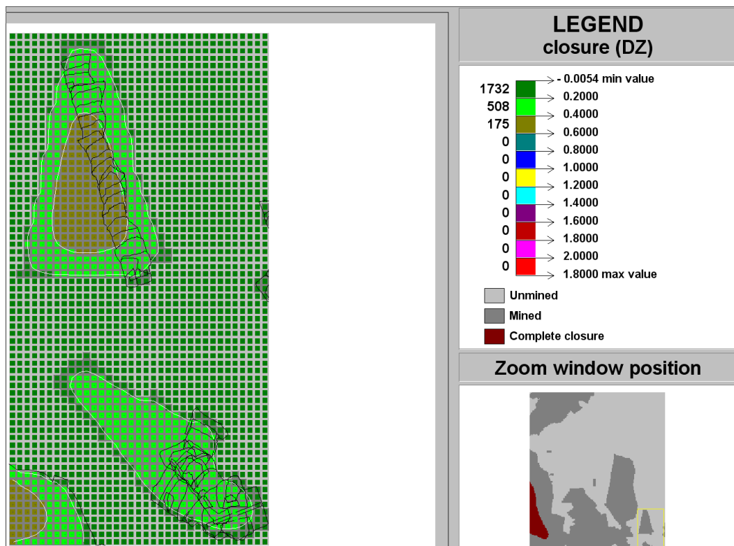
Figure C-150 Contour plot of closure (DZ) of Ya Rona shaft barrel area in Block B at STEP 6
