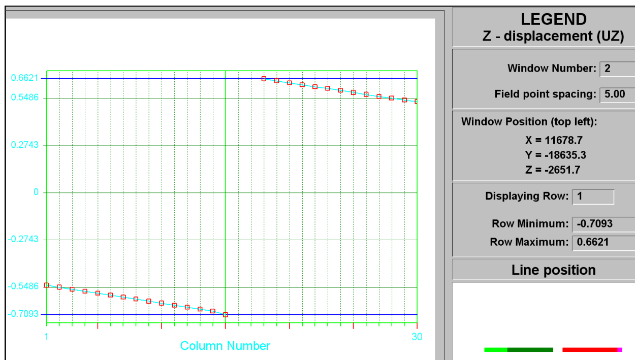
Figure C-60 UZ closure at STEP 15
