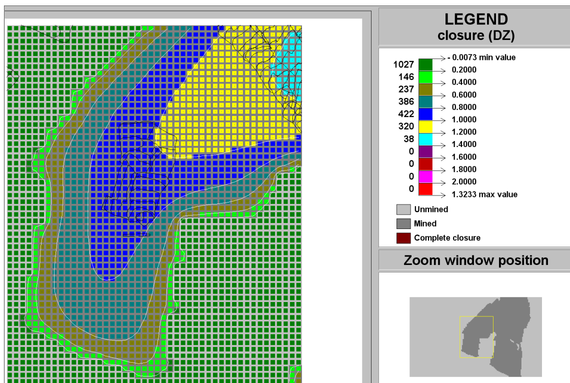
Figure C-192 Contour plot of closure (DZ) of Ya Rona shaft barrel area in Block E at STEP 12
