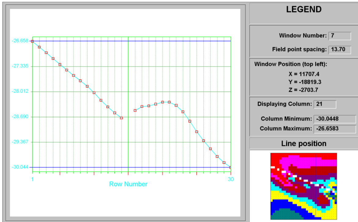
Figure C-106 ESS line plot at column 21 of Shane's Fault at STEP 1
