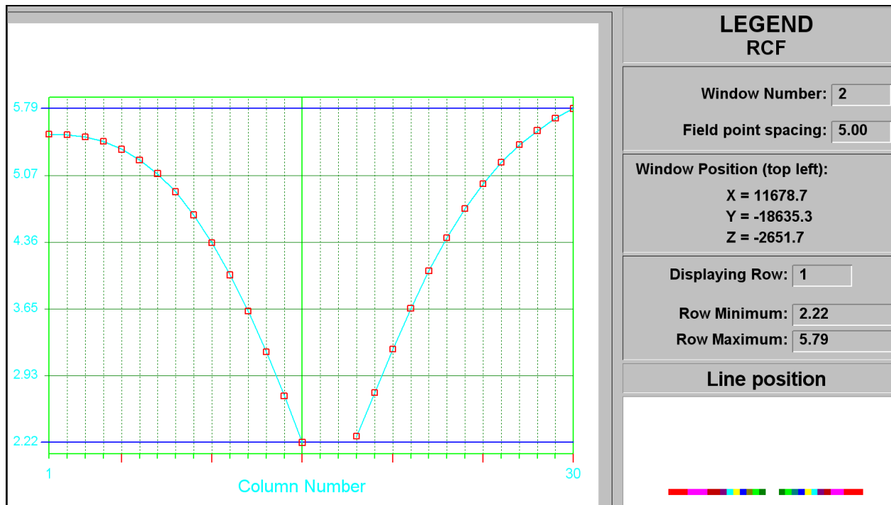
Figure C-7 RCF of shaft barrel at STEP 7
