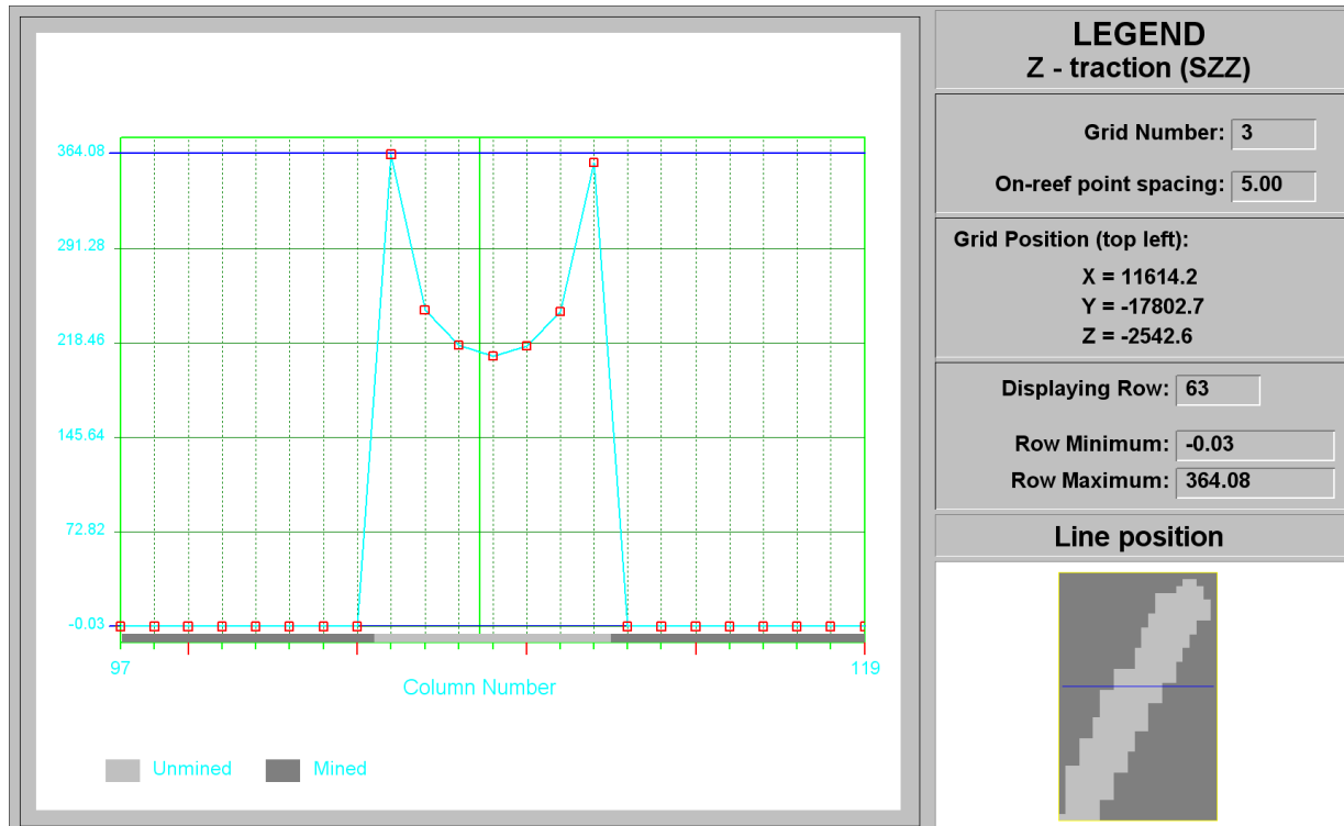
Figure C-128 Line plot at row 52 (SECTION R-S) of Regional Stability Pillar ZZ at STEP 14
