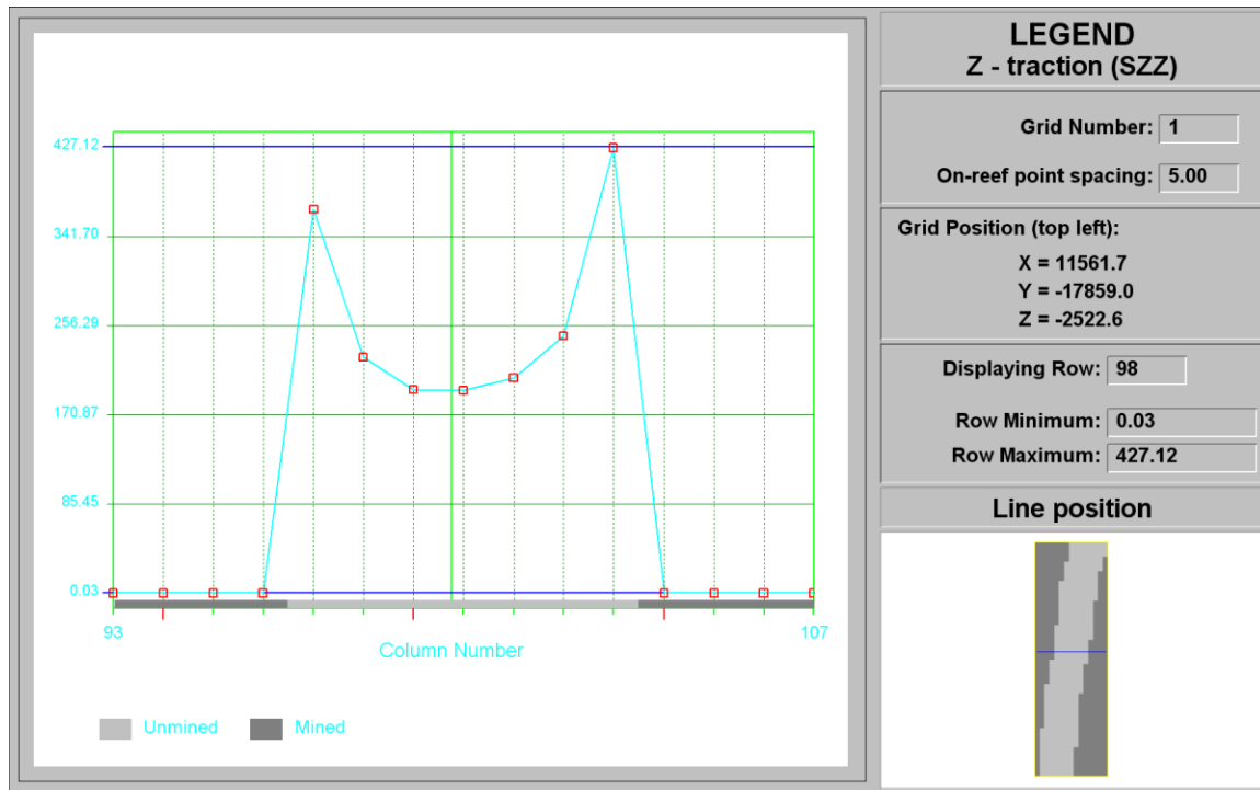
Figure C-123 Line plot at row 98 of Regional Stability Pillar XX at STEP 12
