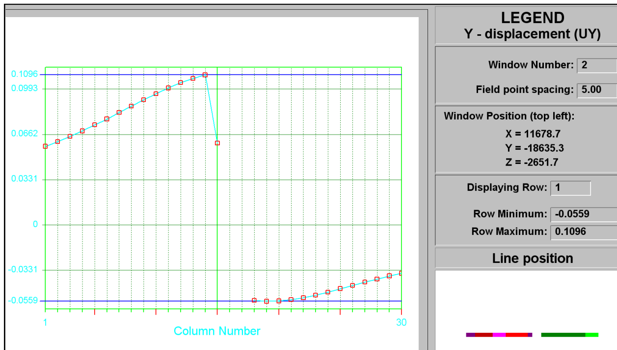
Figure C-19 UY closure at STEP 4
