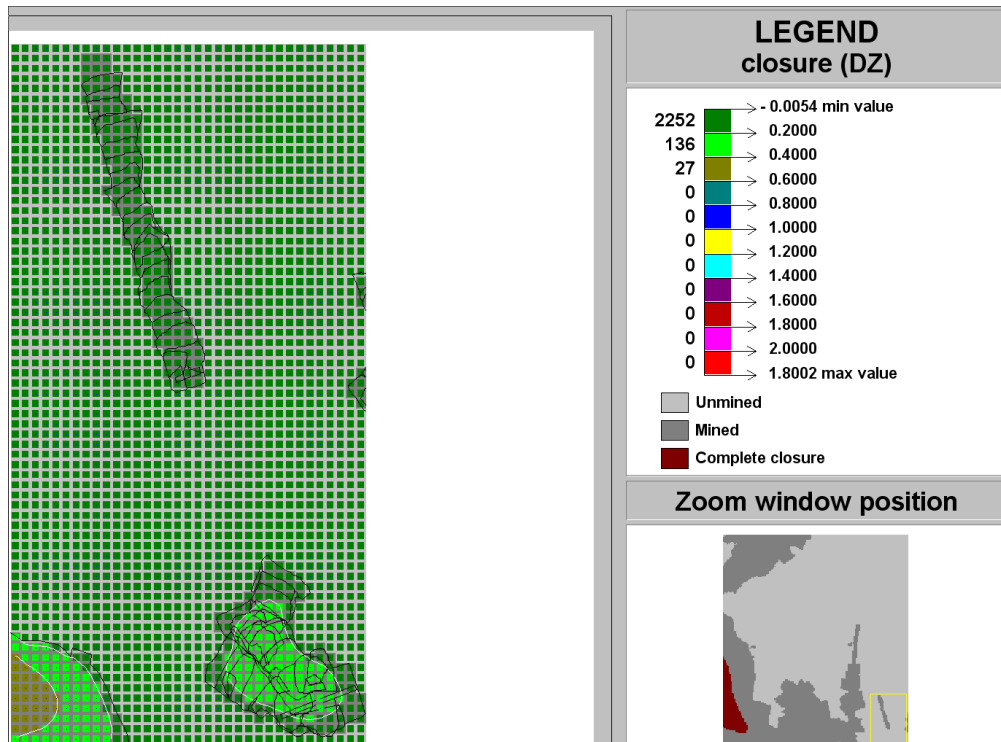
Figure C-145 Contour plot of closure (DZ) of Ya Rona shaft barrel area in Block B at STEP 1
