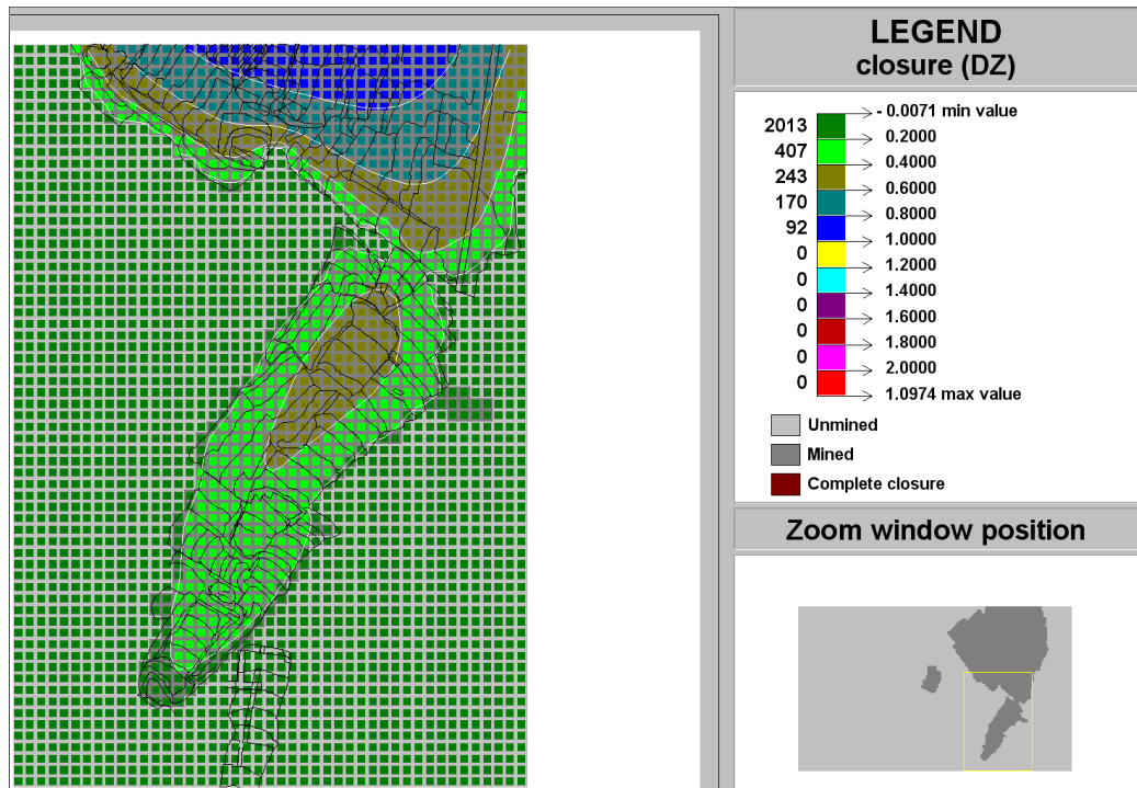
Figure C-168 Contour plot of closure (DZ) of Ya Rona shaft barrel area in Block D at STEP 1
