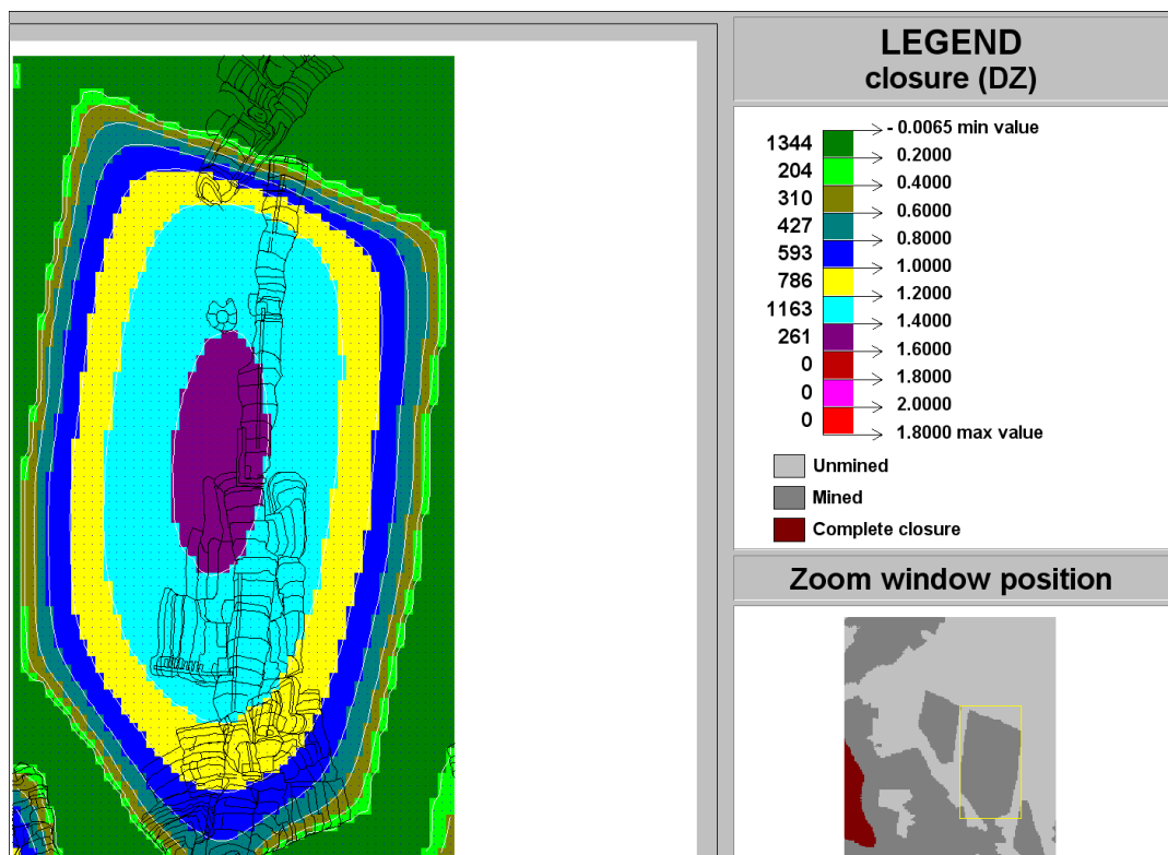
Figure C-141 Contour plot of closure (DZ) of Ya Rona shaft barrel area in Block A at STEP 12
