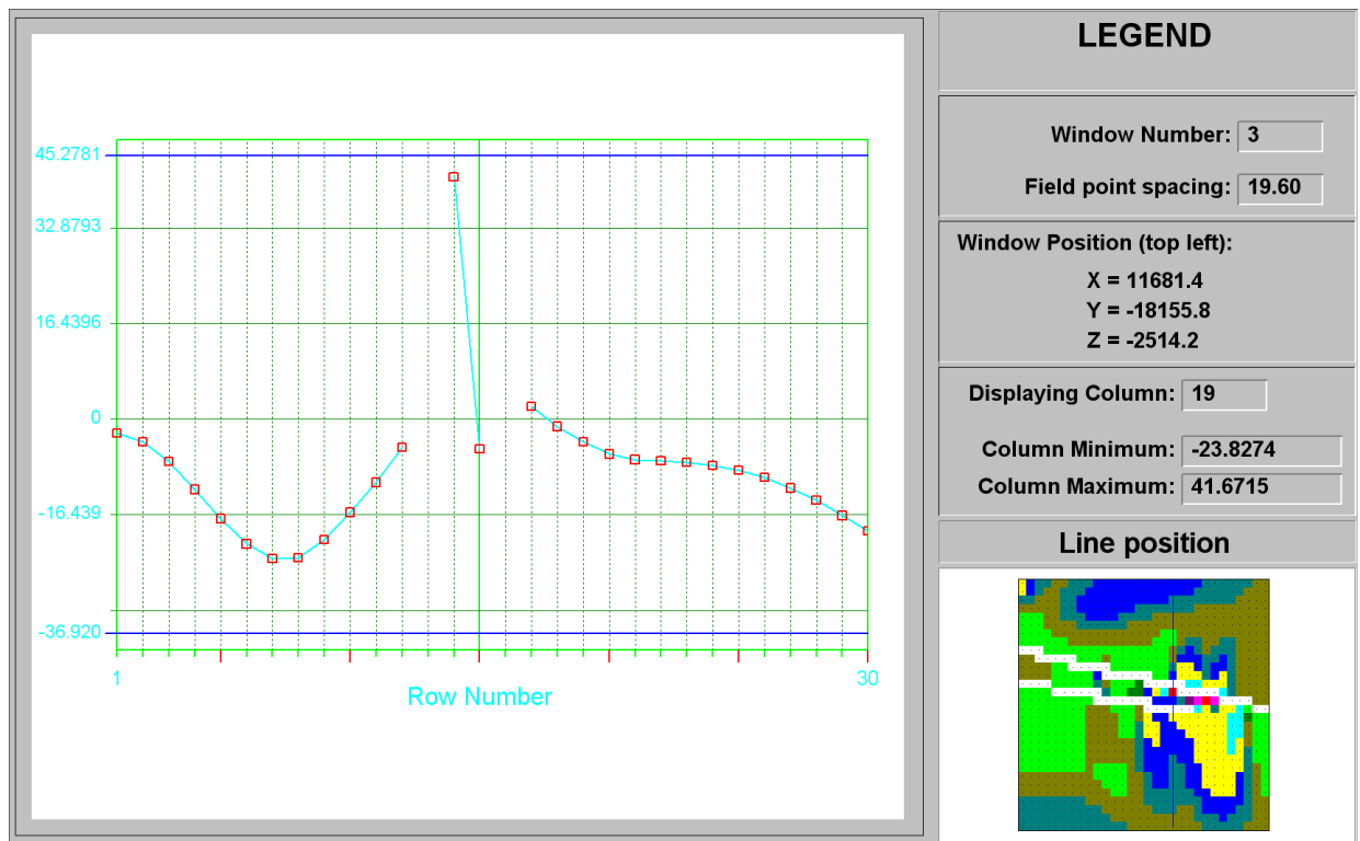
Figure C-84 ESS line plot at column 19 of Murray Fault at STEP 9
