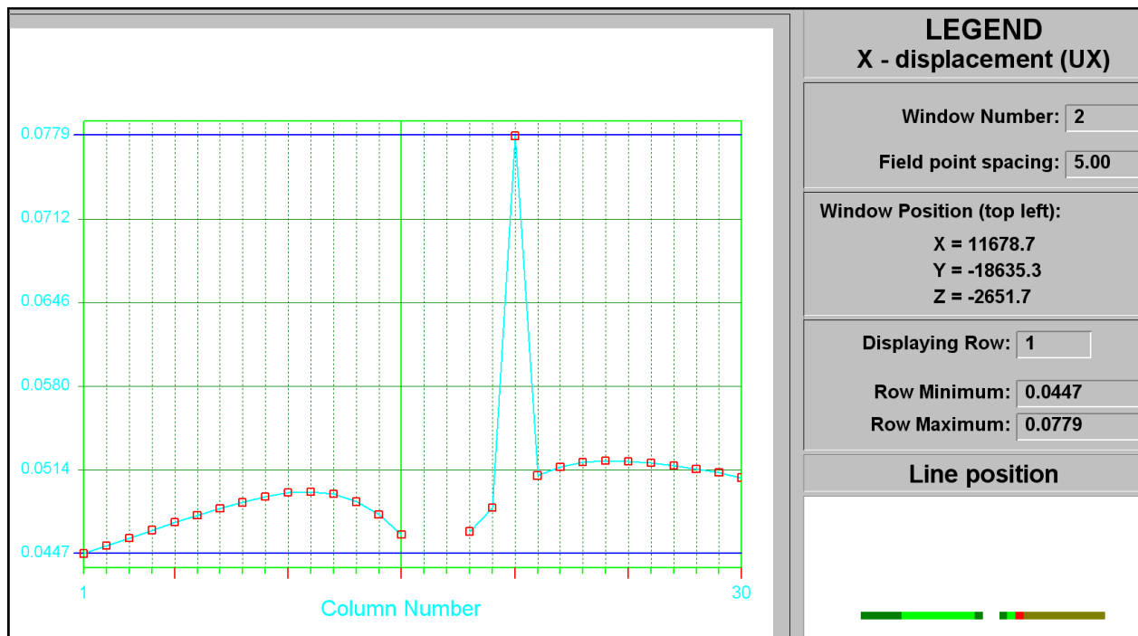
Figure C-31 UX closure at STEP 1
