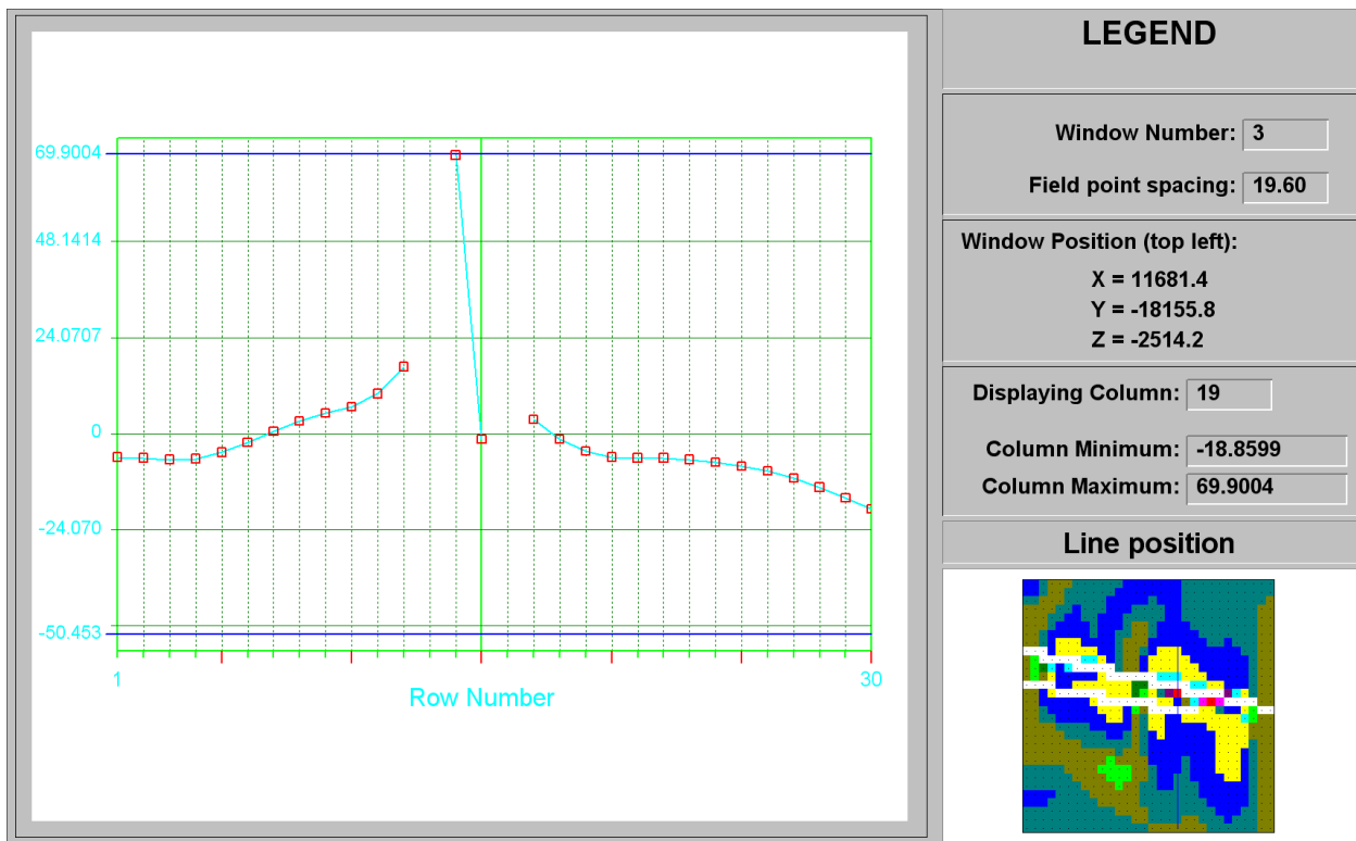
Figure C-88 ESS line plot at column 19 of Murray Fault at STEP 13
