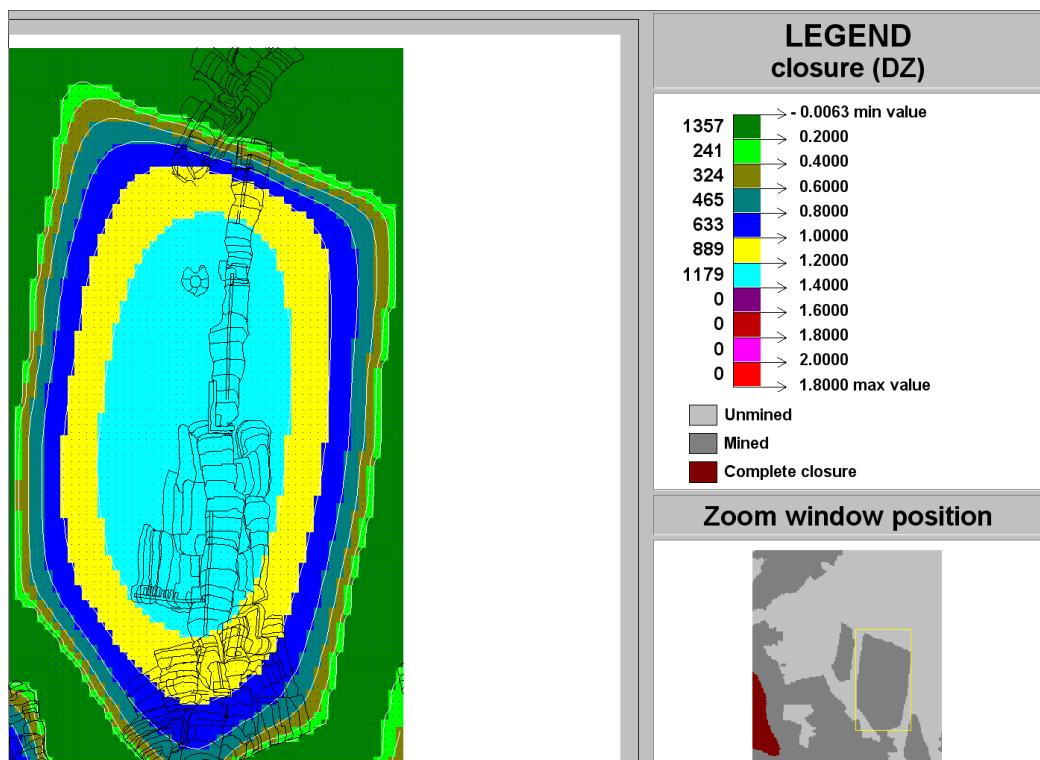
Figure C-139 Contour plot of closure (DZ) of Ya Rona shaft barrel area in Block A at STEP 10
