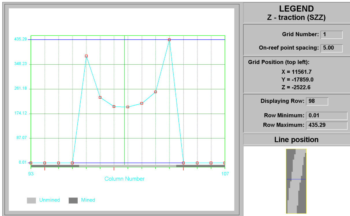
Figure C-125 Line plot at row 98 of Regional Stability Pillar XX at STEP 15
