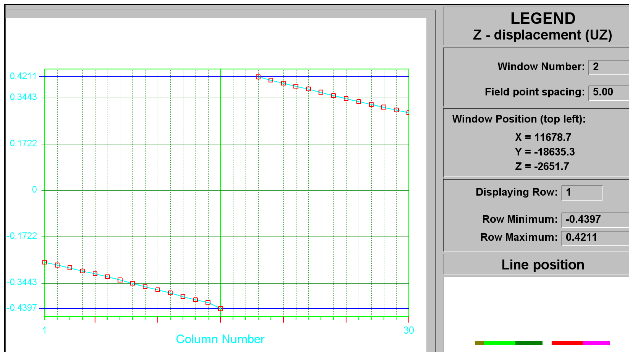
Figure C-51 UZ closure at STEP 6
