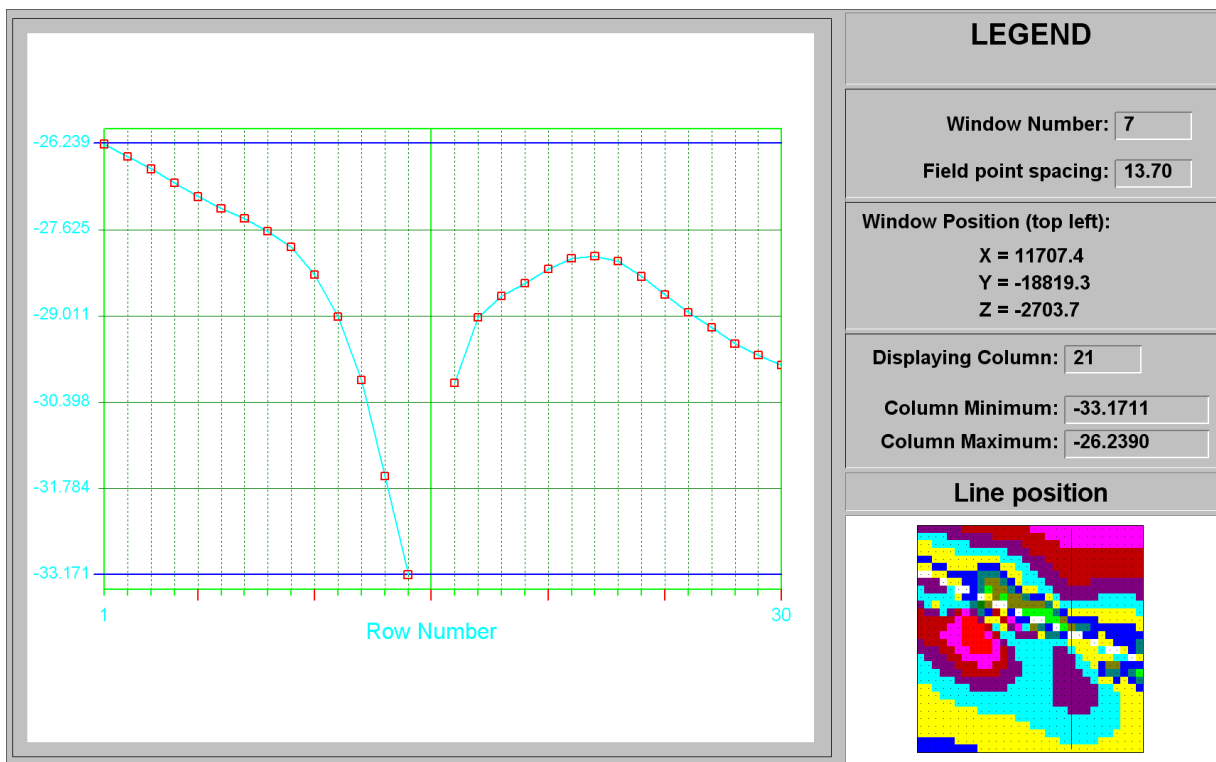
Figure C-111 ESS line plot at column 21 of Shane's Fault at STEP 6
