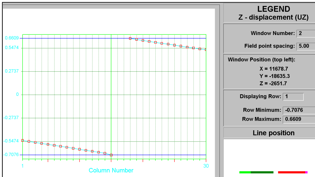
Figure C-59 UZ closure at STEP 14
