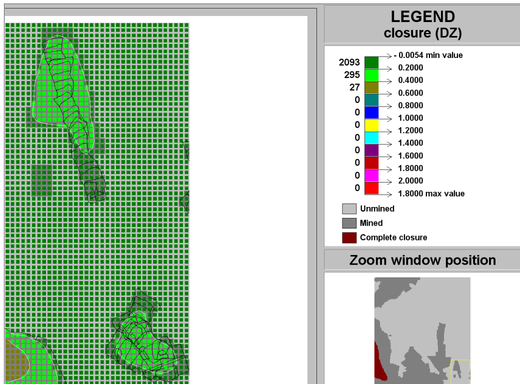
Figure C-147 Contour plot of closure (DZ) of Ya Rona shaft barrel area in Block B at STEP 3
