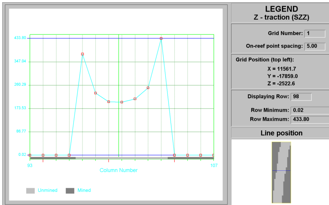
Figure C-124 Line plot at row 98 of Regional Stability Pillar XX at STEP 13
