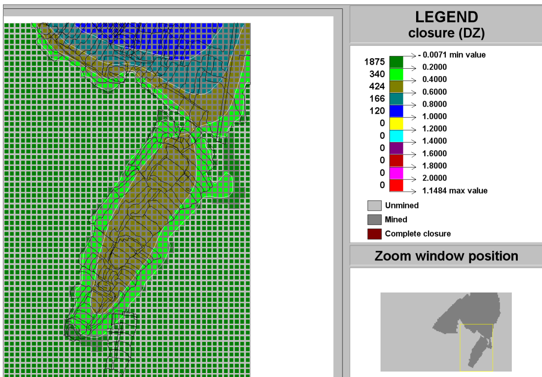
Figure C-171 Contour plot of closure (DZ) of Ya Rona shaft barrel area in Block D at STEP 4
