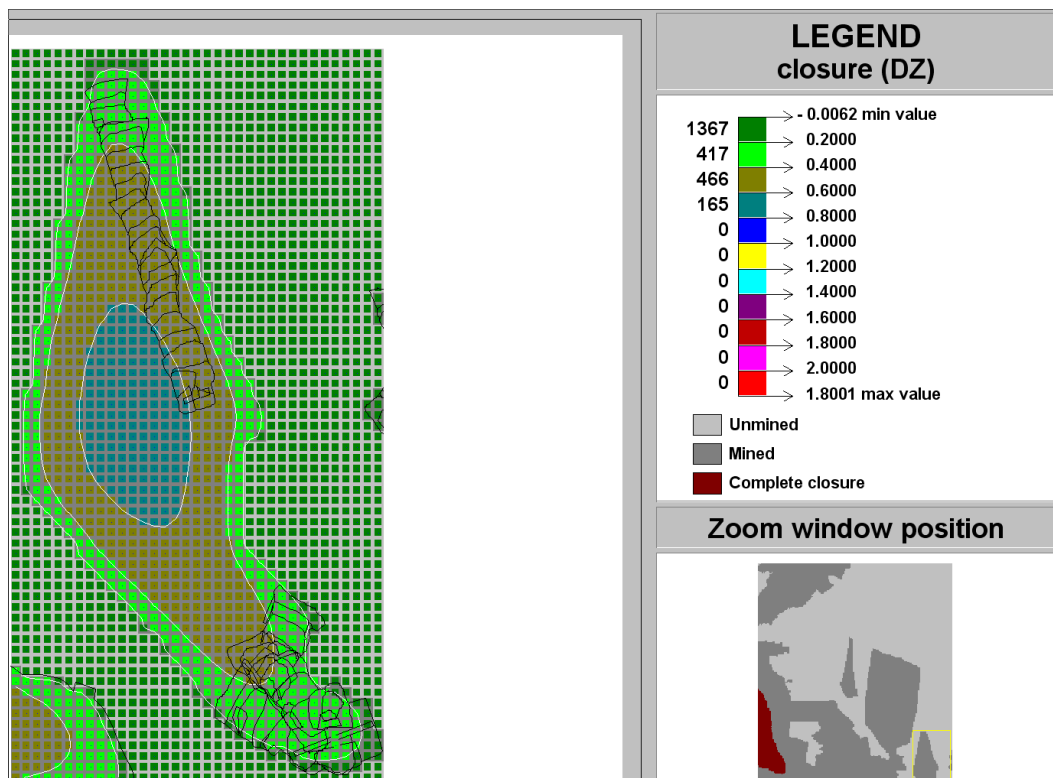
Figure C-153 Contour plot of closure (DZ) of Ya Rona shaft barrel area in Block B at STEP 9
