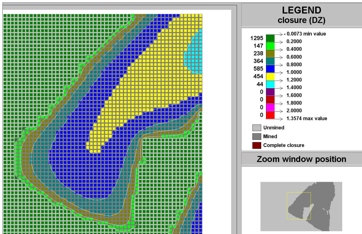
Figure C-193 Contour plot of closure (DZ) of Ya Rona shaft barrel area in Block E at STEP 13
