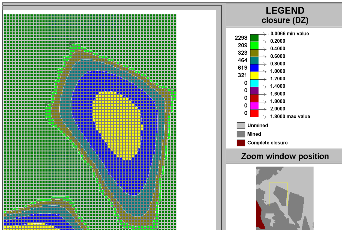
Figure C-165 Contour plot of closure (DZ) of Ya Rona shaft barrel area in Block C at STEP 13
