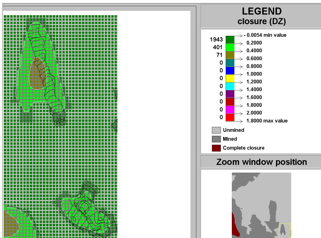
Figure C-148 Contour plot of closure (DZ) of Ya Rona shaft barrel area in Block B at STEP 4
