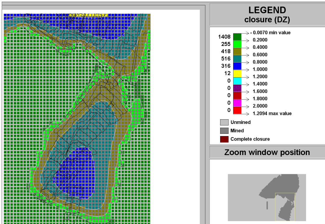
Figure C-174 Contour plot of closure (DZ) of Ya Rona shaft barrel area in Block D at STEP 9
