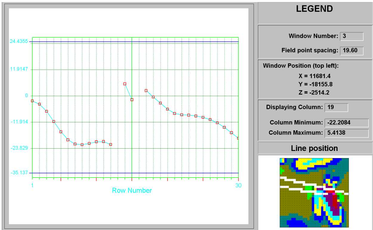
Figure C-83 ESS line plot at column 19 of Murray Fault at STEP 8
