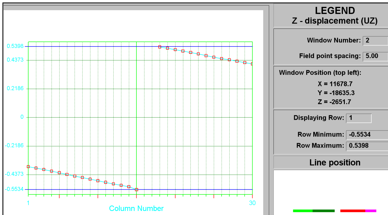
Figure C-53 UZ closure at STEP 8
