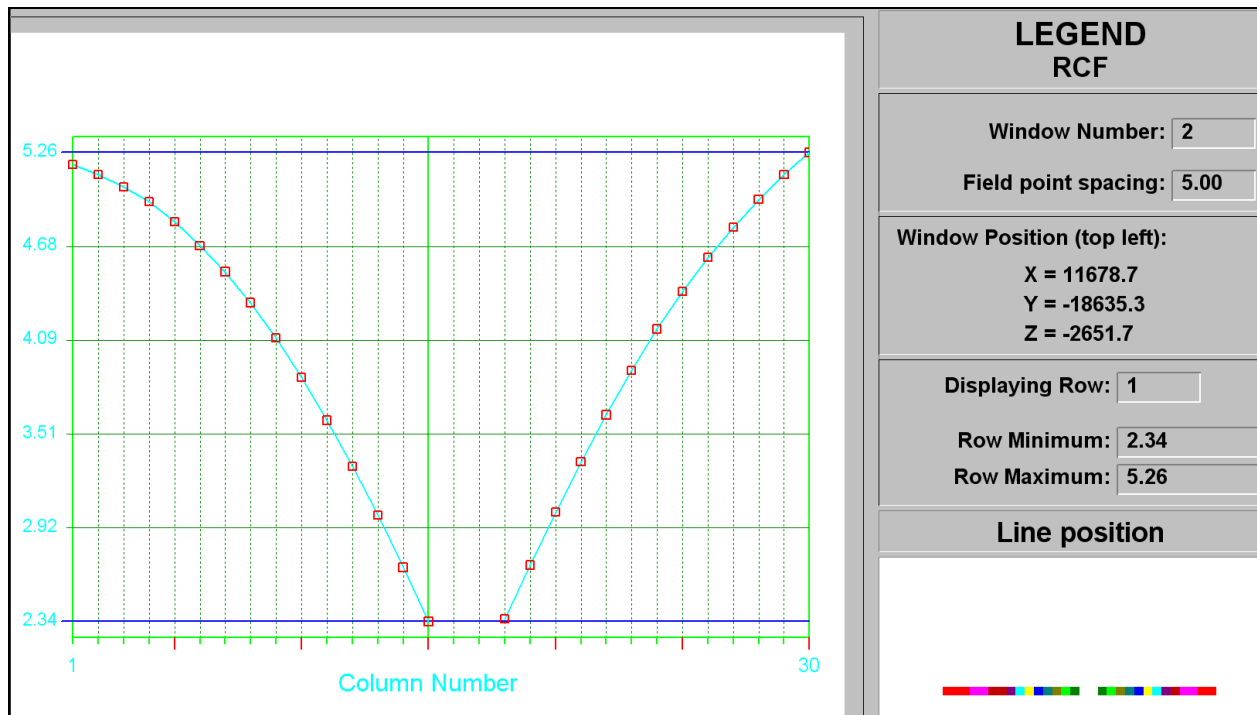
Figure C-11 RCF of shaft barrel at STEP 11
