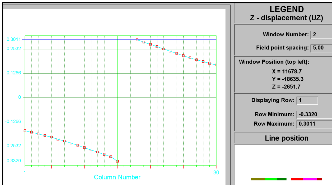
Figure C-49 UZ closure at STEP 4
