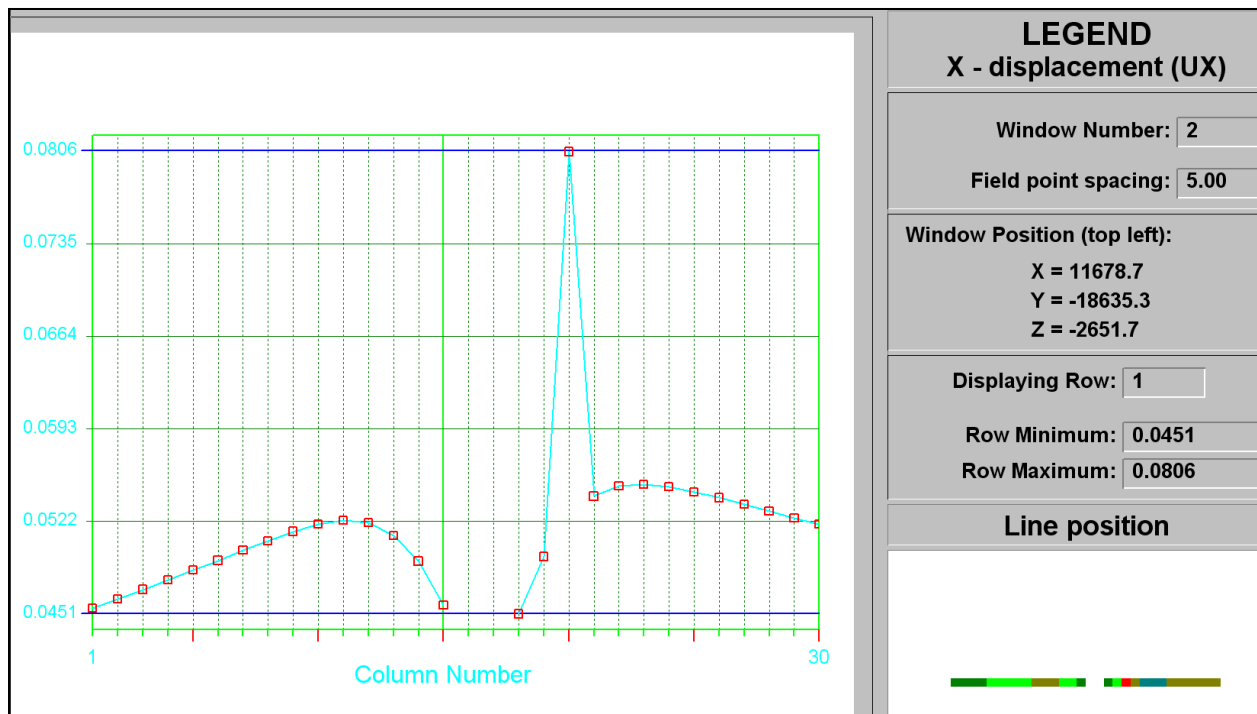
Figure C-32 UX closure at STEP 2
