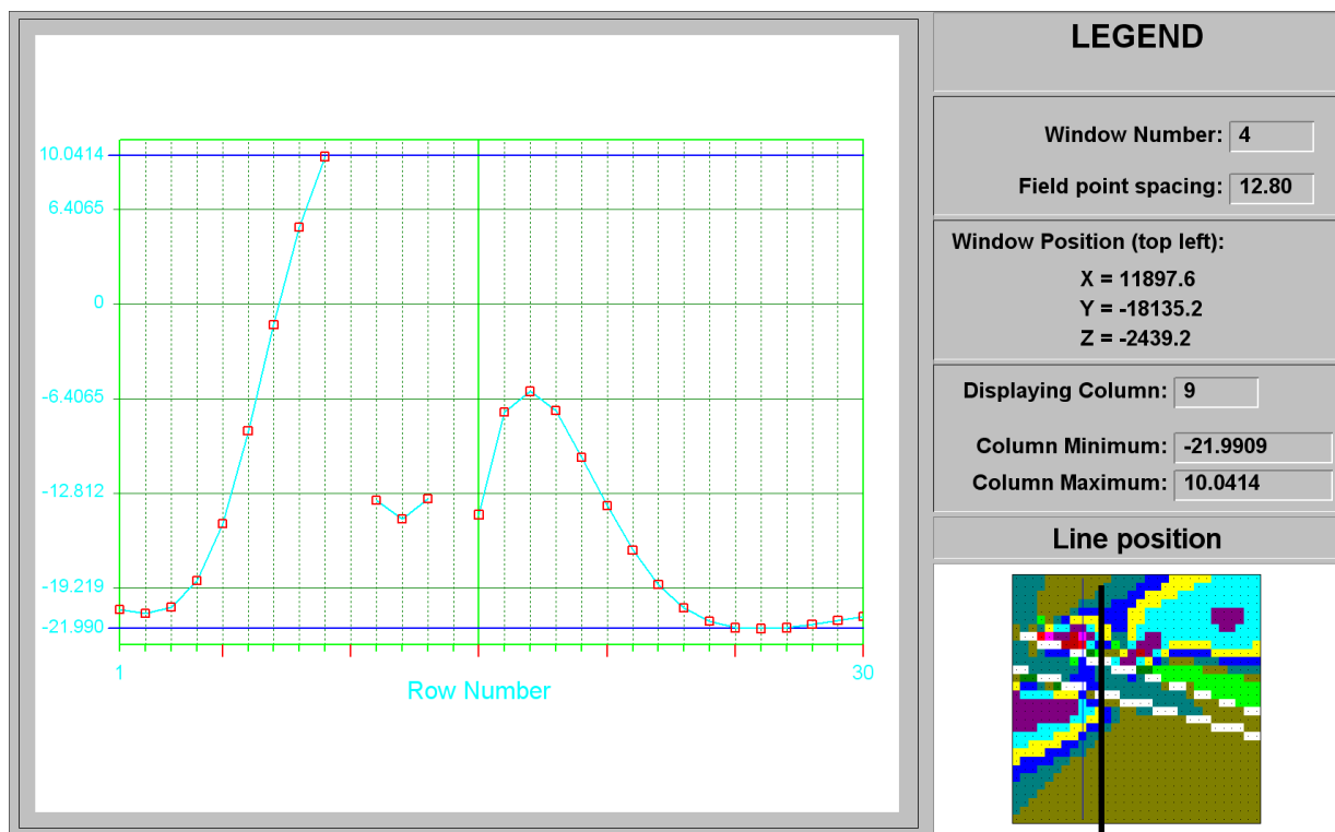
Figure C-68 ESS line plot at column 9 of Kate's Fault at STEP 8
