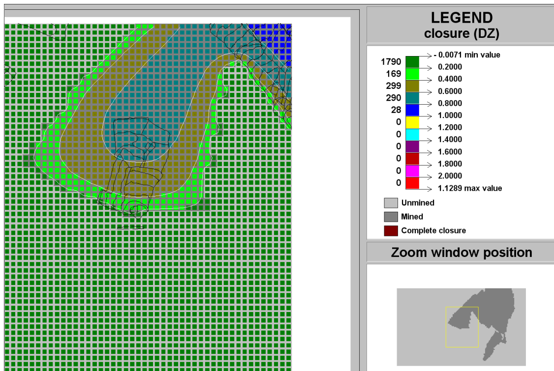
Figure C-185 Contour plot of closure (DZ) of Ya Rona shaft barrel area in Block E at STEP 5
