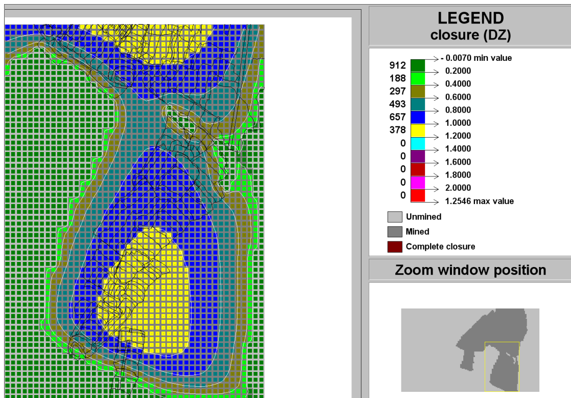
Figure C-176 Contour plot of closure (DZ) of Ya Rona shaft barrel area in Block D at STEP 11
