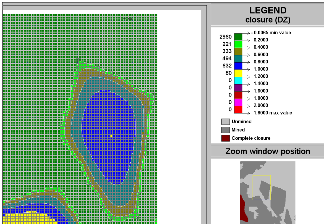
Figure C-164 Contour plot of closure (DZ) of Ya Rona shaft barrel area in Block C at STEP 12
