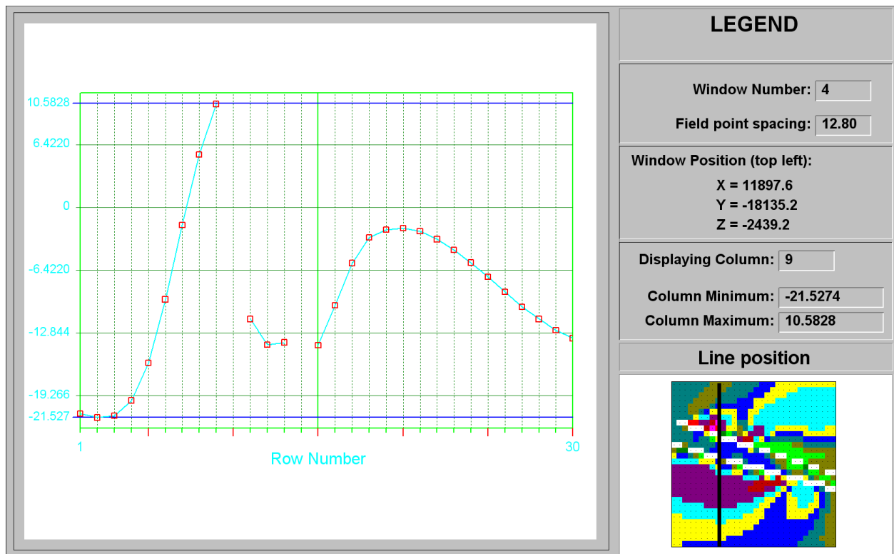
Figure C-75 ESS line plot at column 9 of Kate's Fault at STEP 15
