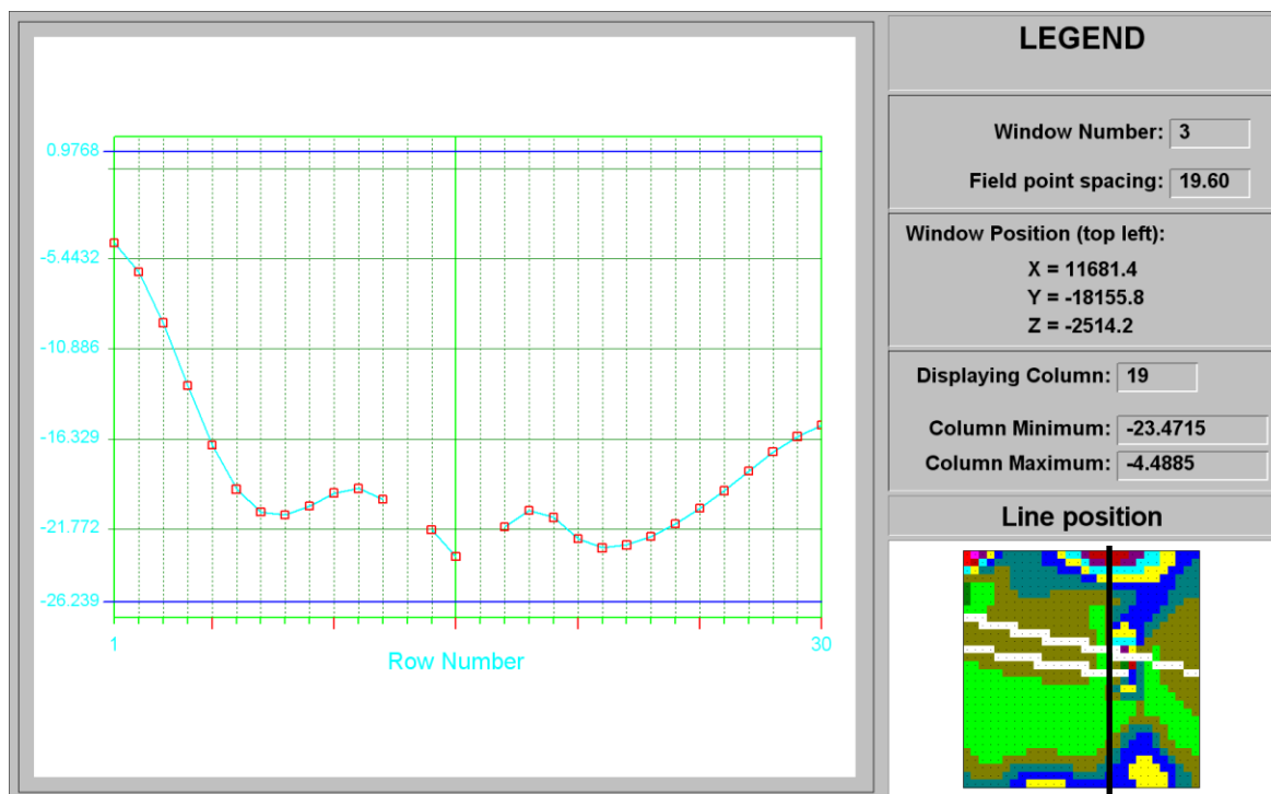
Figure C-77 ESS line plot at column 19 of Murray Fault at STEP 2
