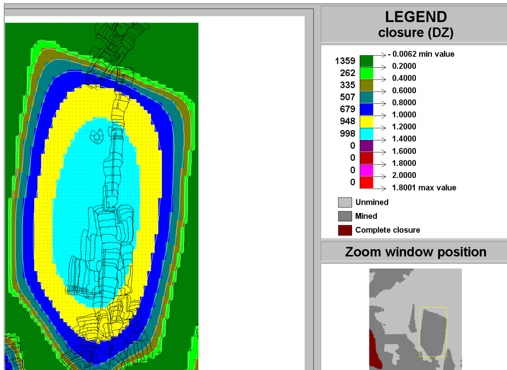
Figure C-138 Contour plot of closure (DZ) of Ya Rona shaft barrel area in Block A at STEP 9
