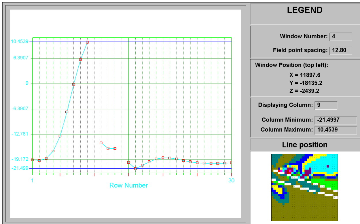
Figure C-63 ESS line plot at column 9 of Kate's Fault at STEP 3
