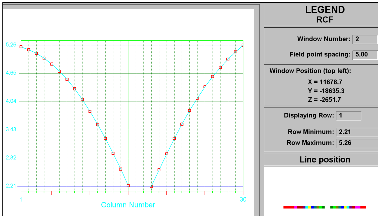
Figure C-13 RCF of shaft barrel at STEP 13
