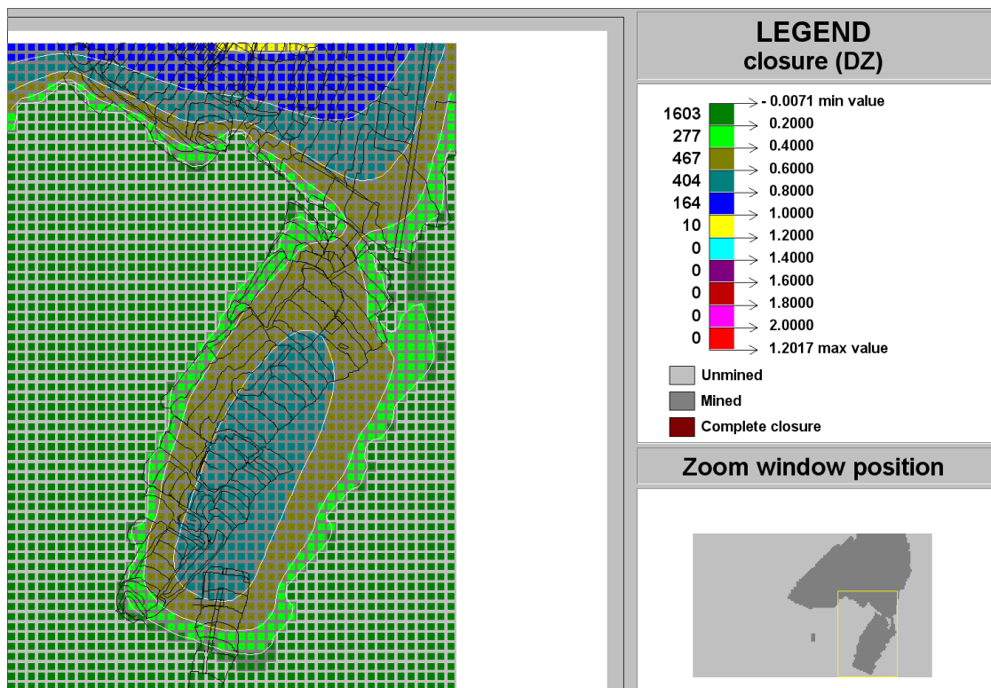
Figure C-173 Contour plot of closure (DZ) of Ya Rona shaft barrel area in Block D at STEP 8
