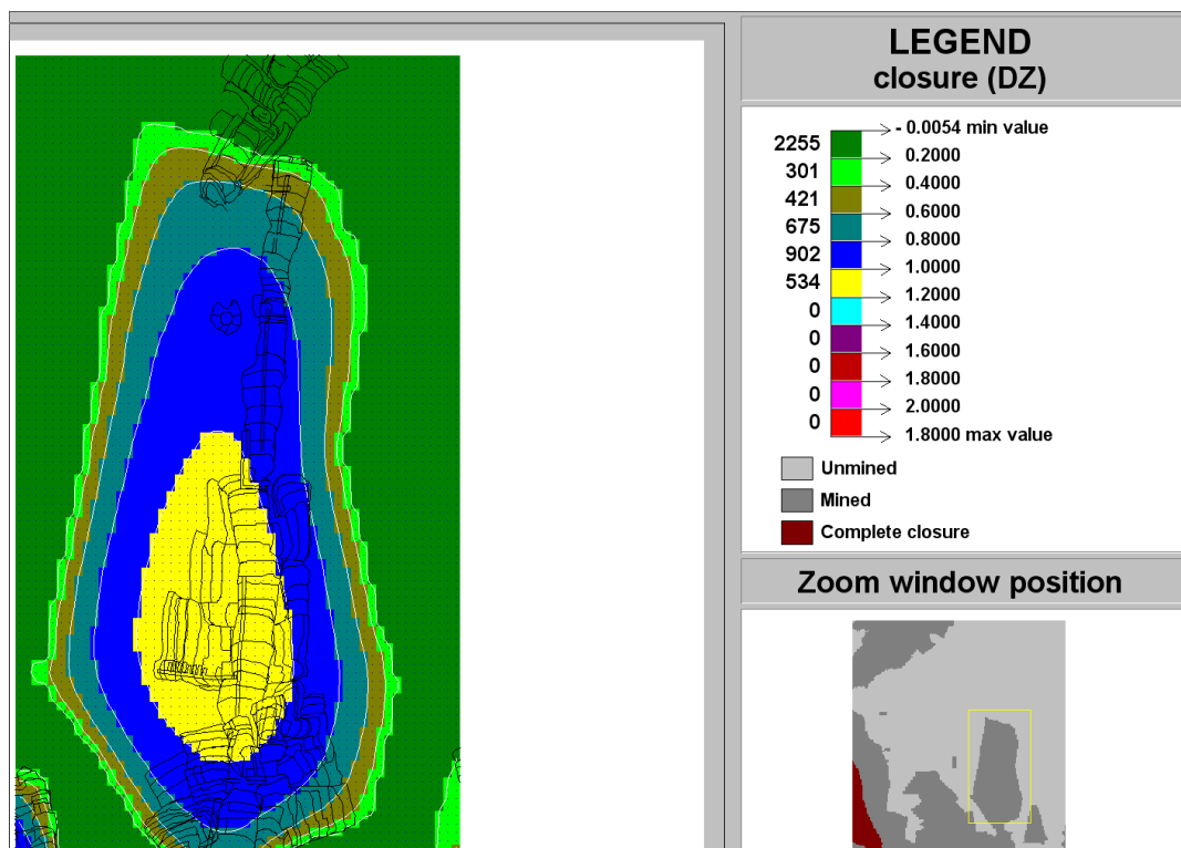
Figure C-135 Contour plot of closure (DZ) of Ya Rona shaft barrel area in Block A at STEP 6
