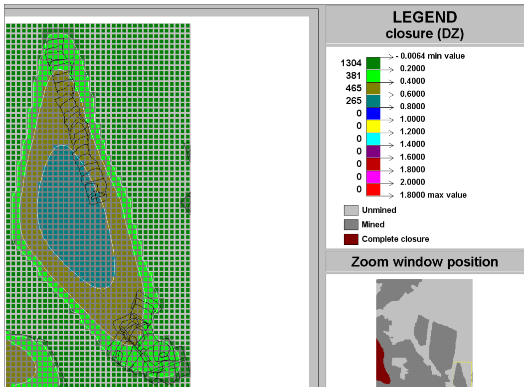
Figure C-155 Contour plot of closure (DZ) of Ya Rona shaft barrel area in Block B at STEP 11
