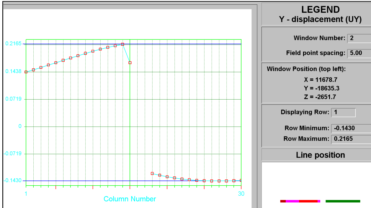
Figure C-25 UY closure at STEP 10
