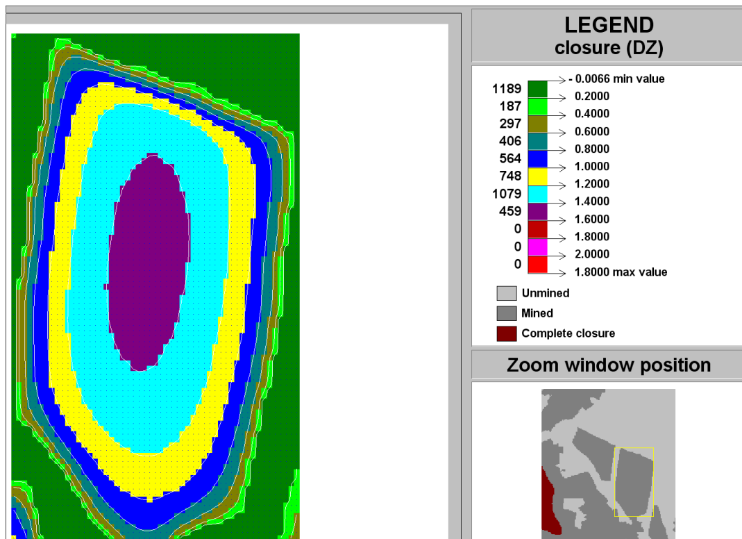
Figure C-144 Contour plot of closure (DZ) of Ya Rona shaft barrel area in Block A at STEP 15
