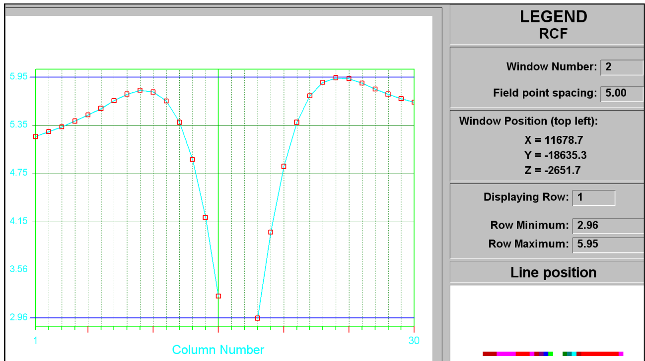
Figure C-3 RCF of shaft barrel at STEP 3
