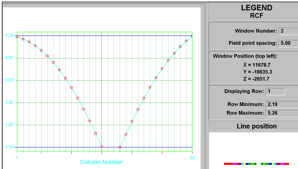
Figure C-15 RCF of shaft barrel at STEP 15
