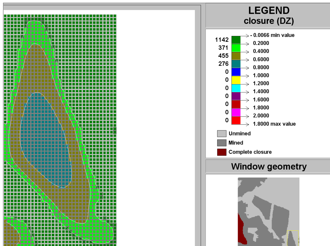
Figure C-159 Contour plot of closure (DZ) of Ya Rona shaft barrel area in Block B at STEP 15
