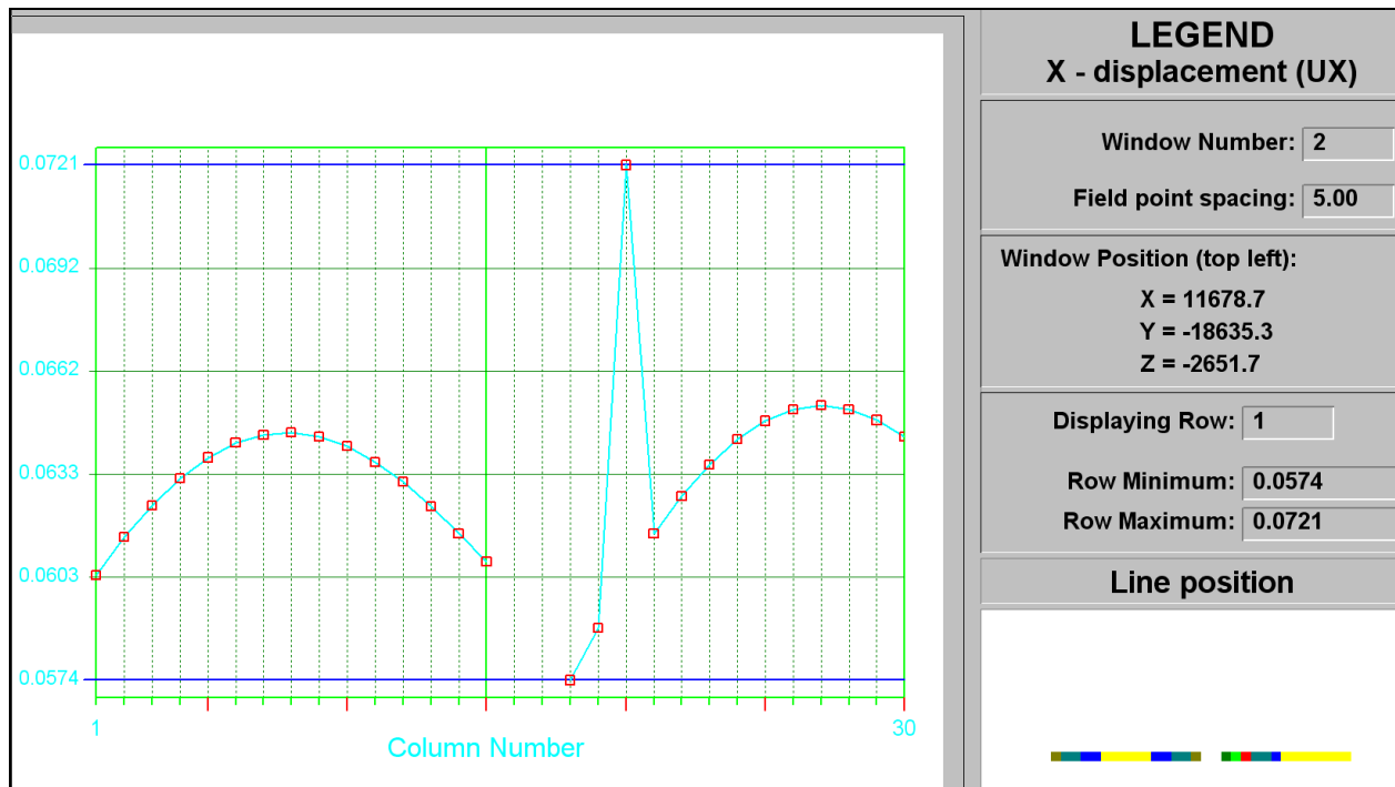
Figure C-42 UX closure at STEP 12
