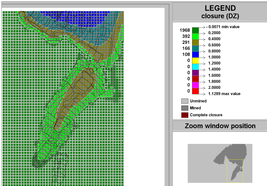
Figure C-170 Contour plot of closure (DZ) of Ya Rona shaft barrel area in Block D at STEP 3
