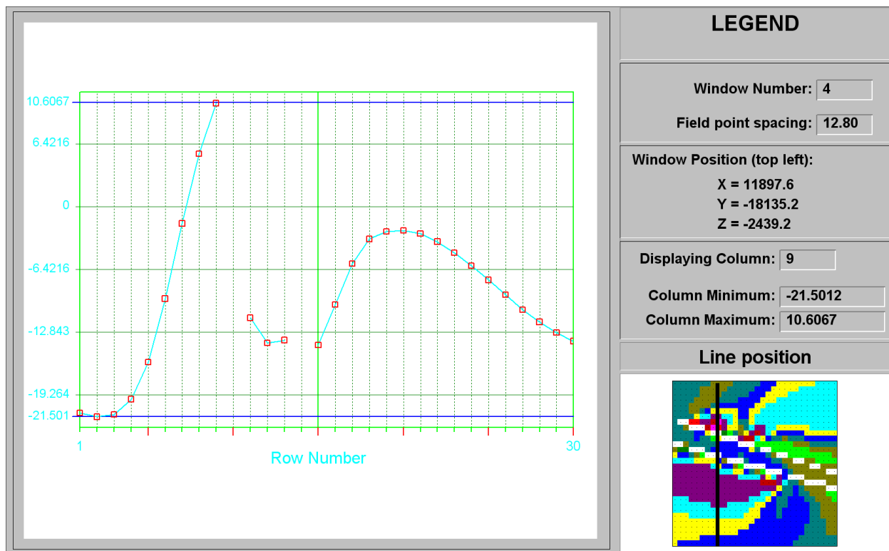
Figure C-74 ESS line plot at column 9 of Kate's Fault at STEP 14
