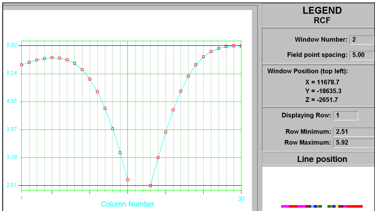
Figure C-4 RCF of shaft barrel at STEP 4
