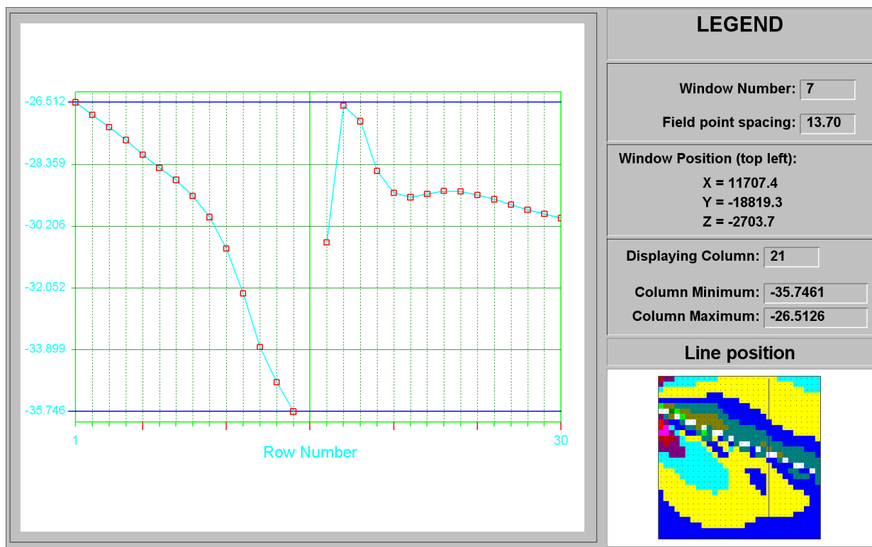
Figure C-114 ESS line plot at column 21 of Shane's Fault at STEP 9
