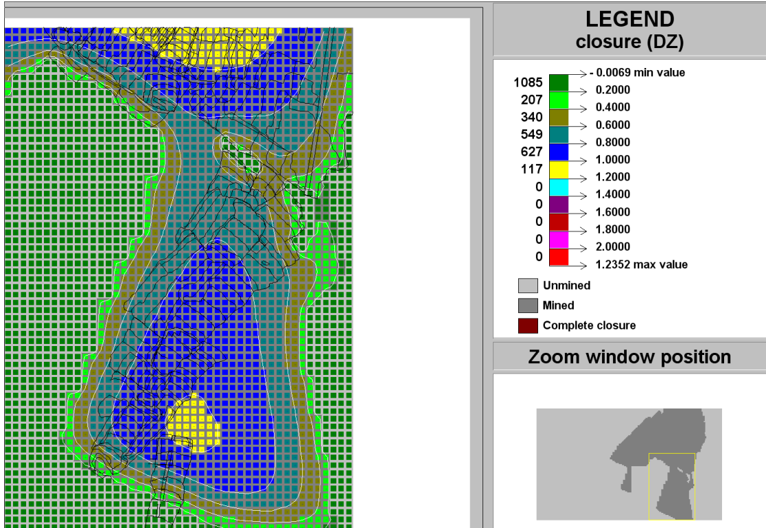
Figure C-175 Contour plot of closure (DZ) of Ya Rona shaft barrel area in Block D at STEP 10
