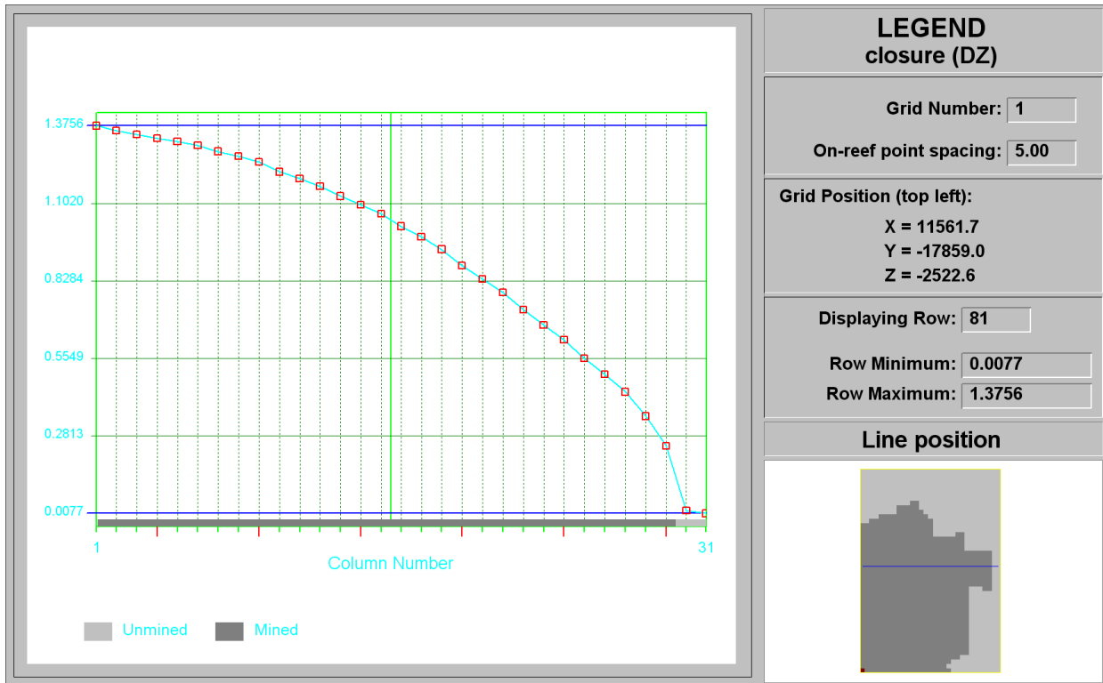
Figure C-201 Contour plot of closure (DZ) of Ya Rona shaft barrel area in Block F at STEP 14
