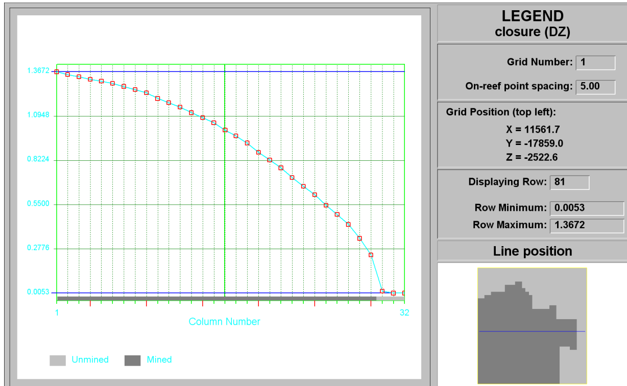
Figure C-201 Contour plot of closure (DZ) of Ya Rona shaft barrel area in Block F at STEP 13
