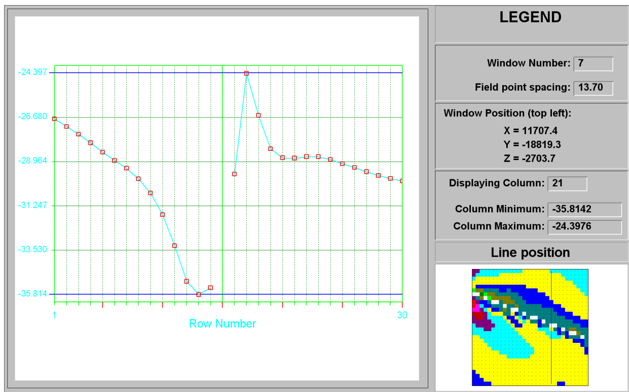
Figure C-116 ESS line plot at column 21 of Shane's Fault at STEP 11
