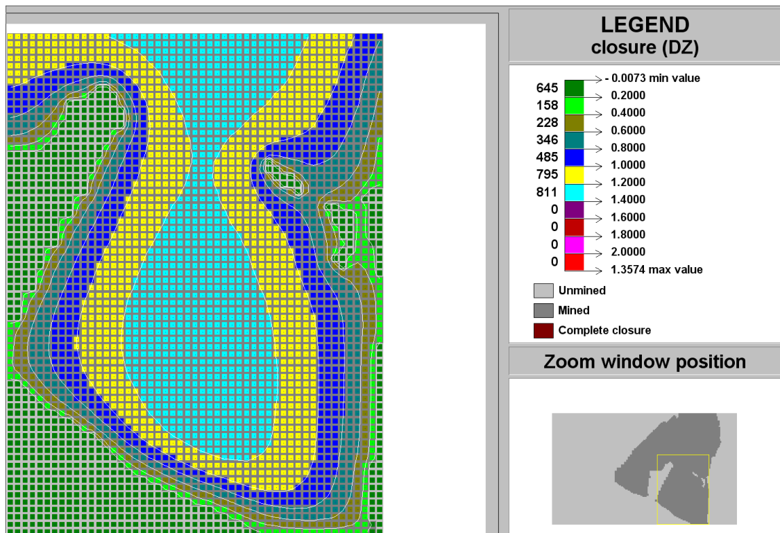
Figure C-178 Contour plot of closure (DZ) of Ya Rona shaft barrel area in Block D at STEP 13
