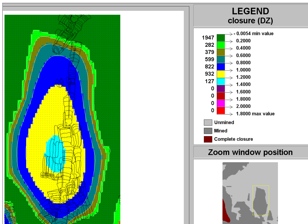
Figure C-136 Contour plot of closure (DZ) of Ya Rona shaft barrel area in Block A at STEP 7
