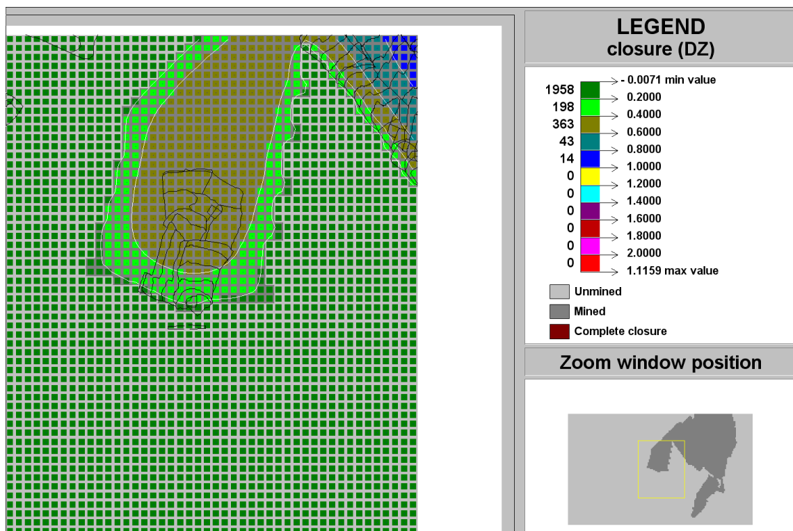
Figure C-184 Contour plot of closure (DZ) of Ya Rona shaft barrel area in Block E at STEP 4
