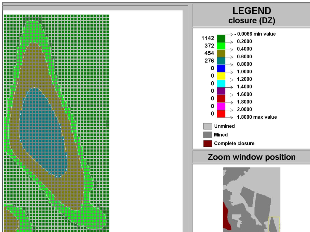
Figure C-157 Contour plot of closure (DZ) of Ya Rona shaft barrel area in Block B at STEP 13
