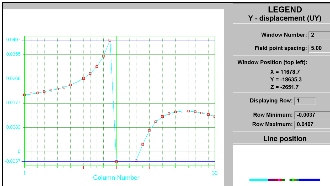
Figure C-17 UY closure at STEP 2
