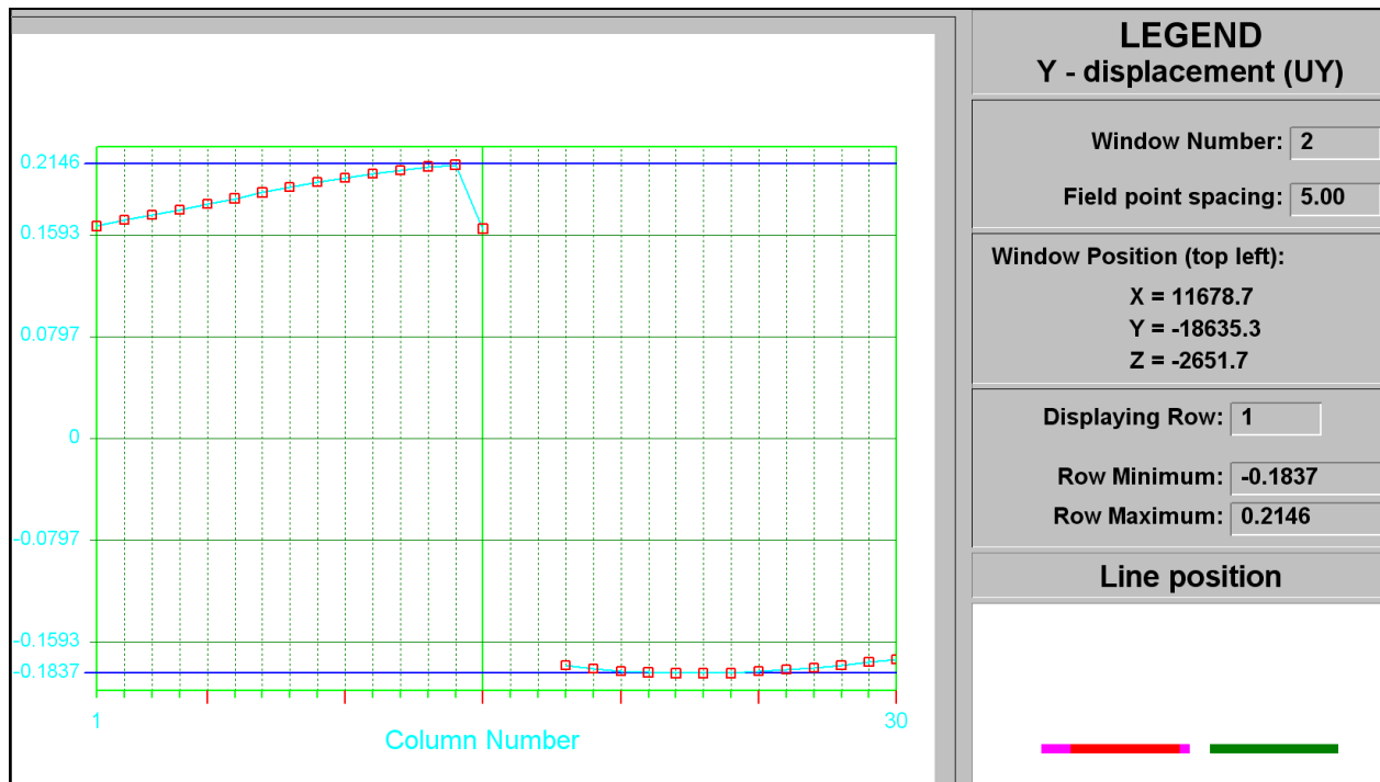
Figure C-30 UY closure at STEP 15
