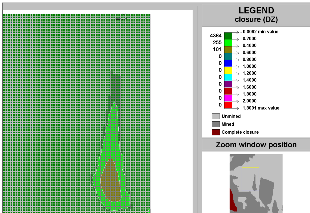
Figure C-161 Contour plot of closure (DZ) of Ya Rona shaft barrel area in Block C at STEP 9
