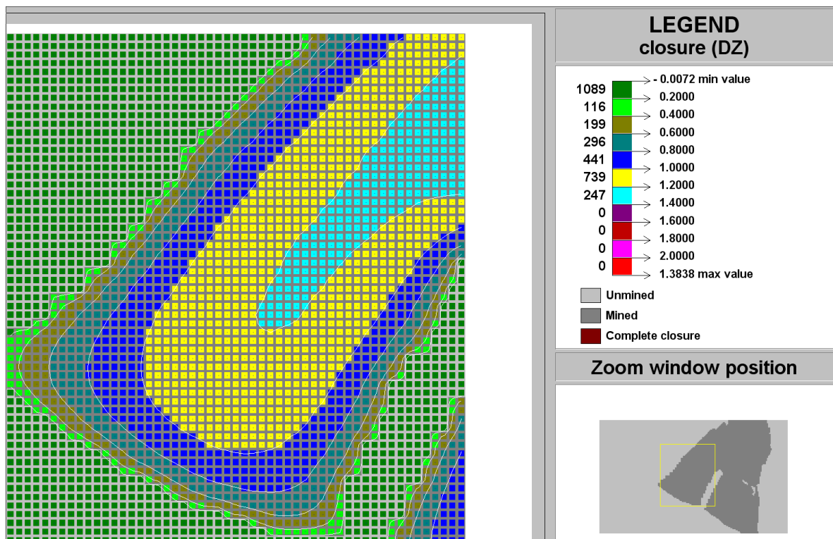
Figure C-194 Contour plot of closure (DZ) of Ya Rona shaft barrel area in Block E at STEP 14
