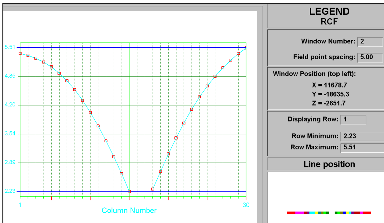
Figure C-8 RCF of shaft barrel at STEP 8
