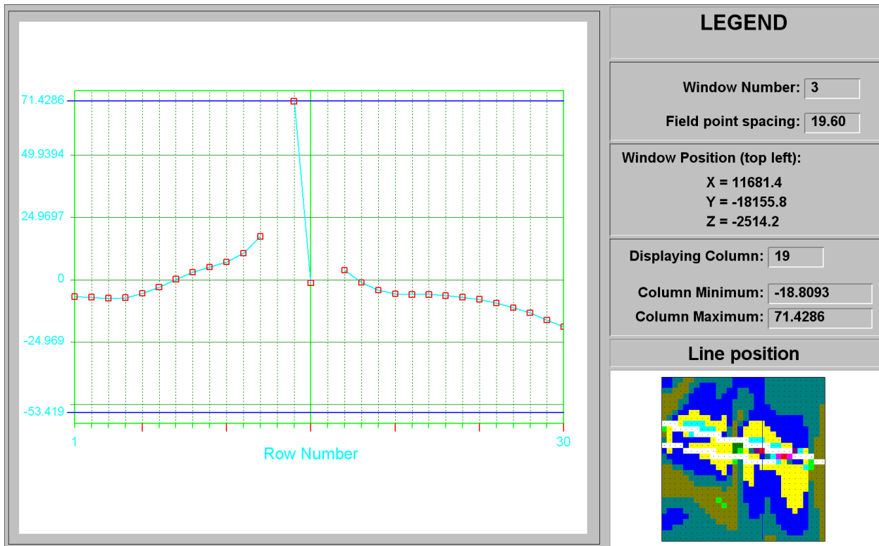
Figure C-89 ESS line plot at column 19 of Murray Fault at STEP 14
