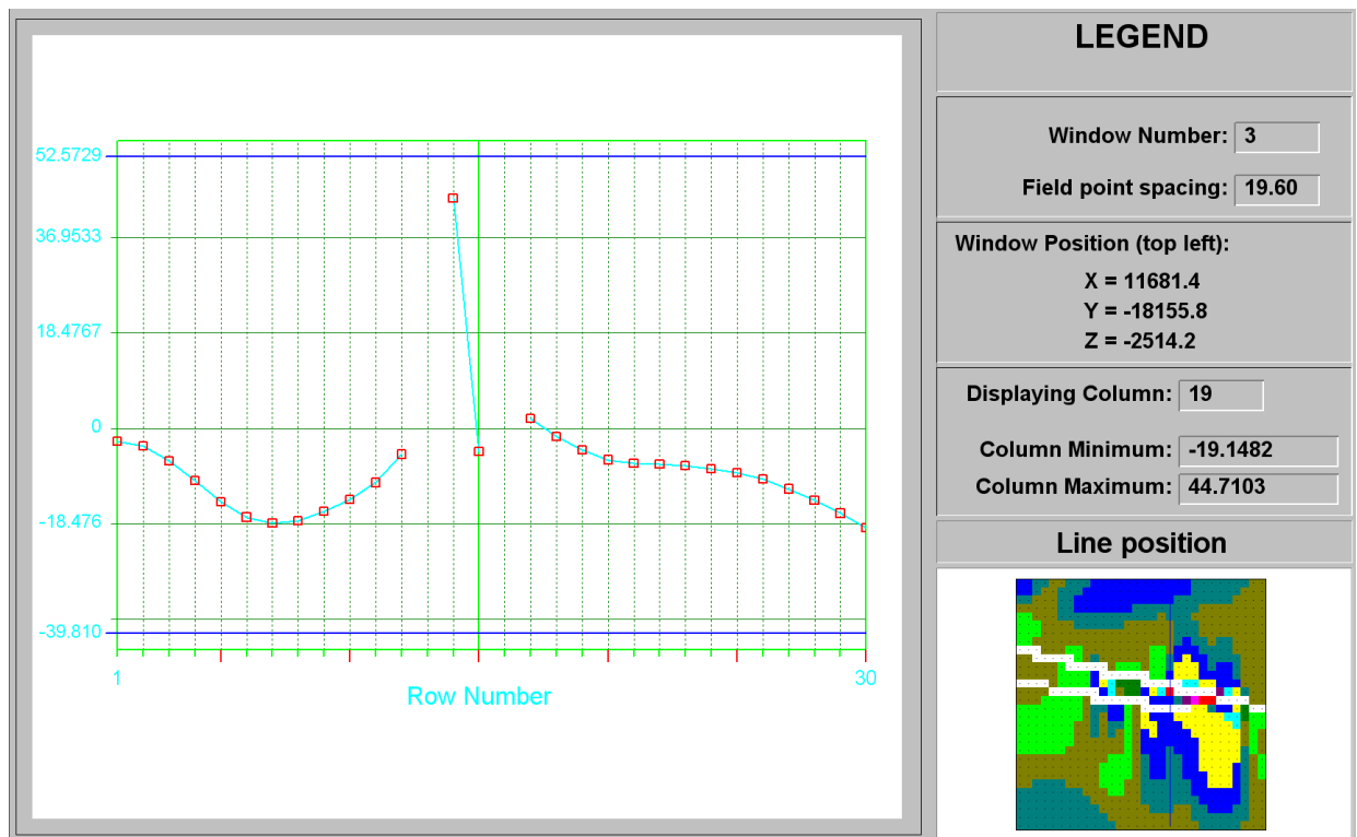
Figure C-85 ESS line plot at column 19 of Murray Fault at STEP 10
