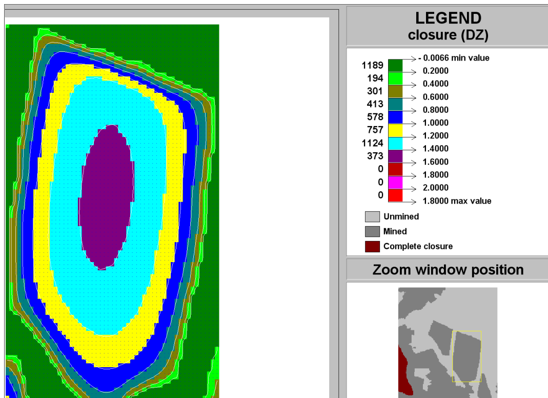
Figure C-142 Contour plot of closure (DZ) of Ya Rona shaft barrel area in Block A at STEP 13
