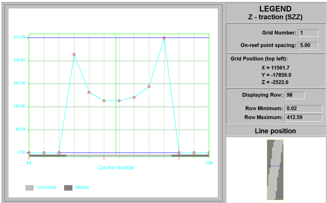
Figure C-122 Line plot at row 98 of Regional Stability Pillar XX at STEP 11
