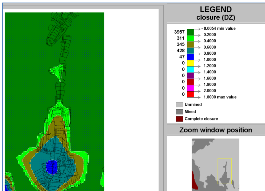
Figure C-131 Contour plot of closure (DZ) of Ya Rona shaft barrel area in Block A at STEP 2
