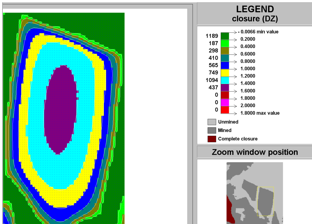
Figure C-143 Contour plot of closure (DZ) of Ya Rona shaft barrel area in Block A at STEP 14
