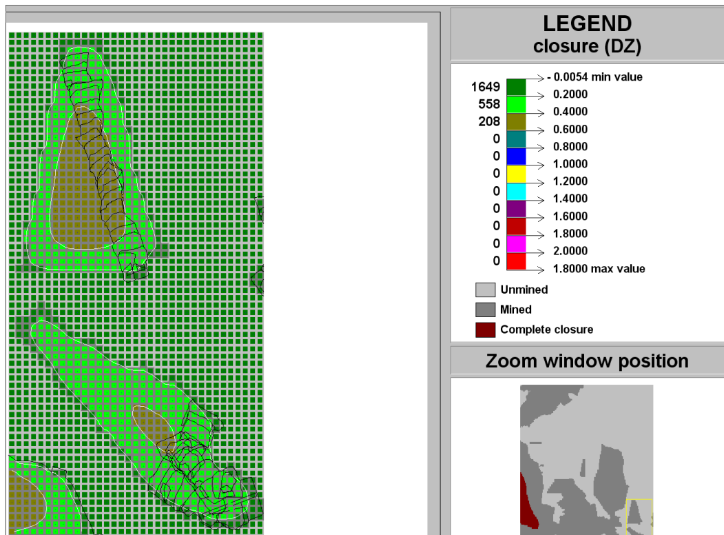
Figure C-151 Contour plot of closure (DZ) of Ya Rona shaft barrel area in Block B at STEP 7
