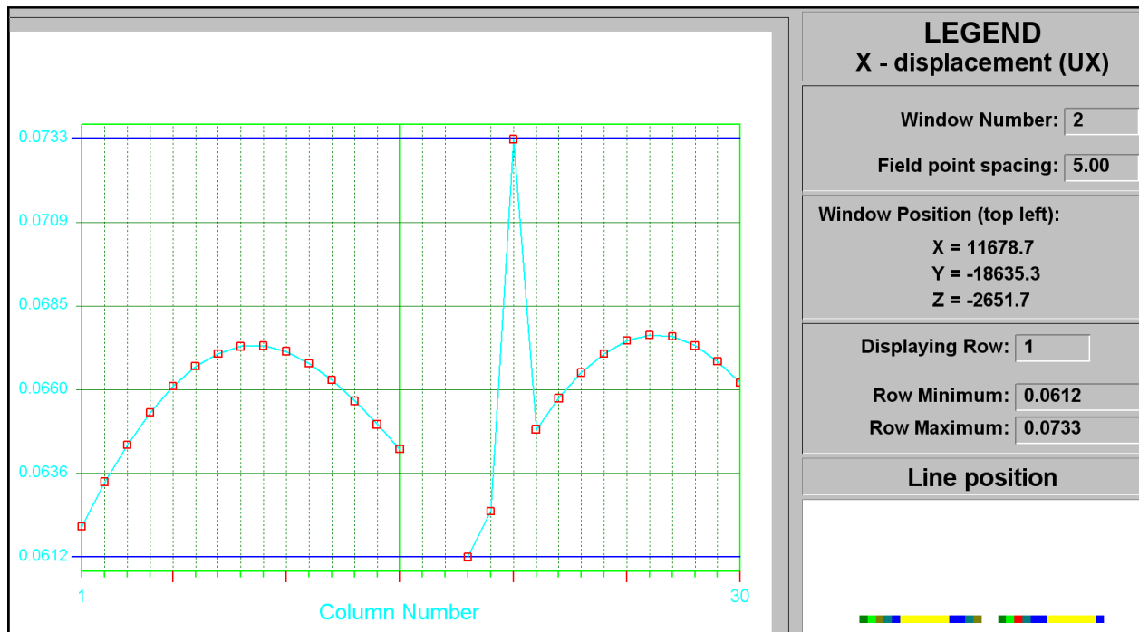
Figure C-43 UX closure at STEP 13
