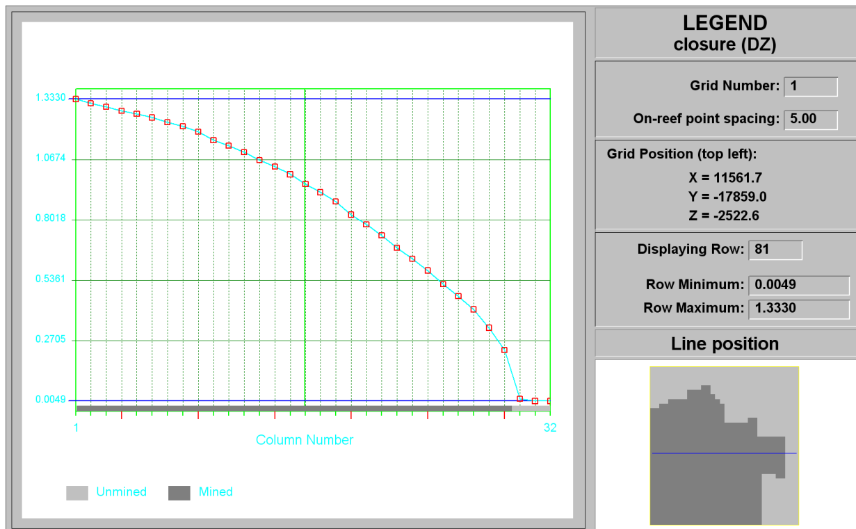
Figure C-199 Contour plot of closure (DZ) of Ya Rona shaft barrel area in Block F at STEP 11
