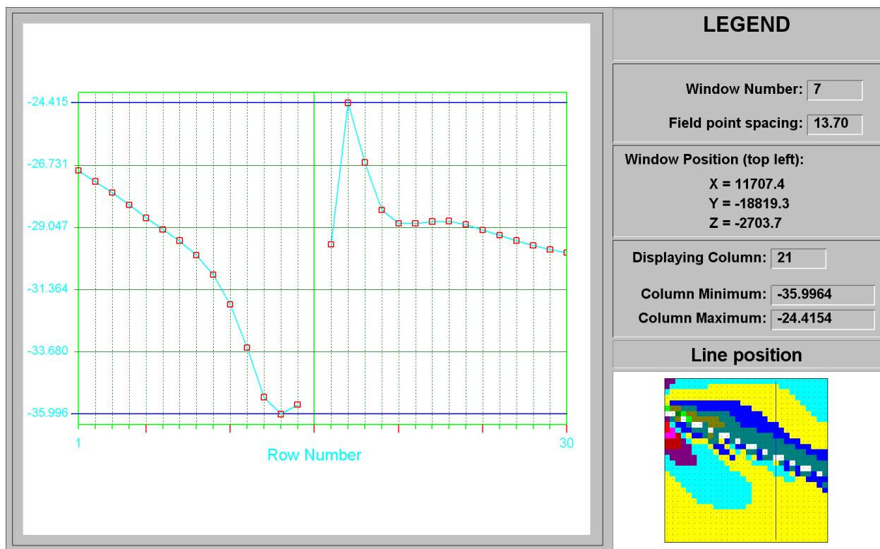
Figure C-118 ESS line plot at column 21 of Shane's Fault at STEP 13
