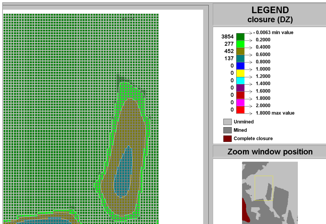
Figure C-162 Contour plot of closure (DZ) of Ya Rona shaft barrel area in Block C at STEP 10
