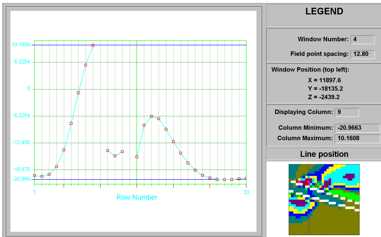
Figure C-65 ESS line plot at column 9 of Kate's Fault at STEP 5
