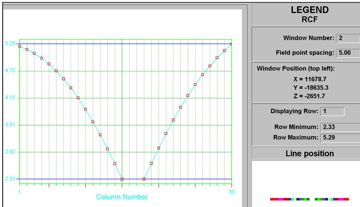
Figure C-9 RCF of shaft barrel at STEP 9
