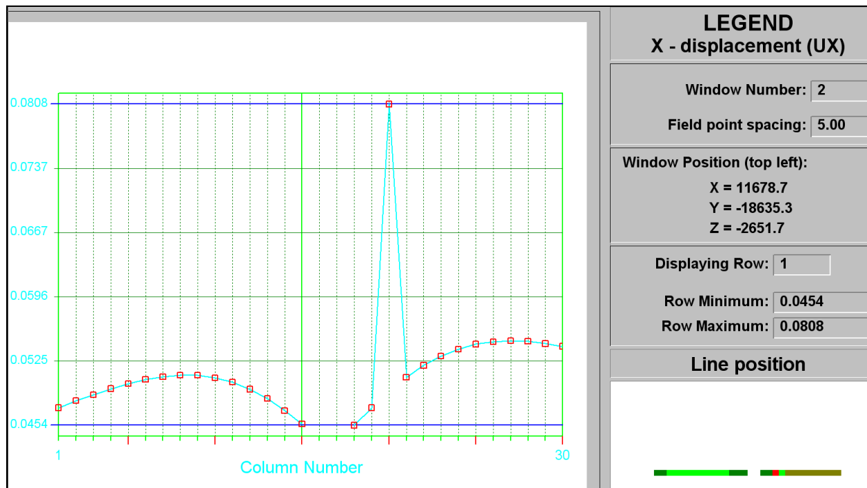
Figure C-34 UX closure at STEP 4
