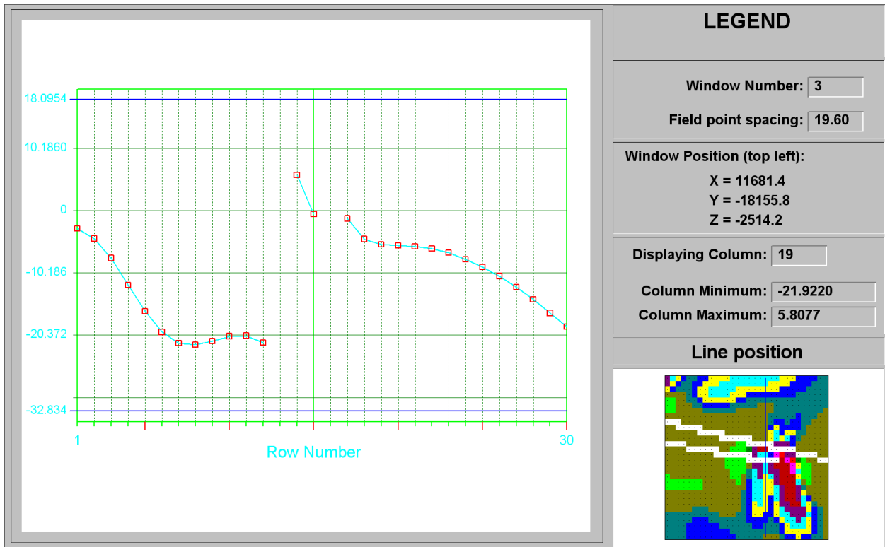
Figure C-82 ESS line plot at column 19 of Murray Fault at STEP 7
