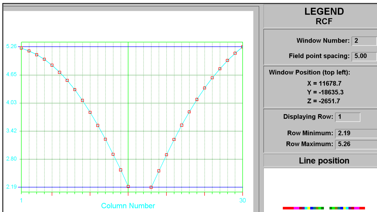
Figure C-14 RCF of shaft barrel at STEP 14
