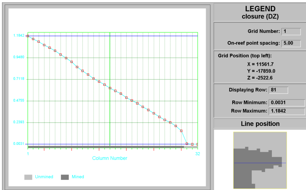
Figure C-197 Contour plot of closure (DZ) of Ya Rona shaft barrel area in Block F at STEP 9
