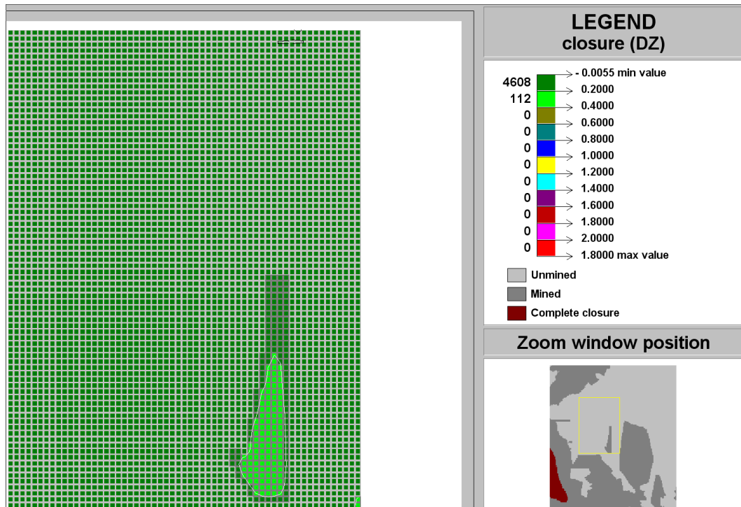
Figure C-160 Contour plot of closure (DZ) of Ya Rona shaft barrel area in Block C at STEP 8
