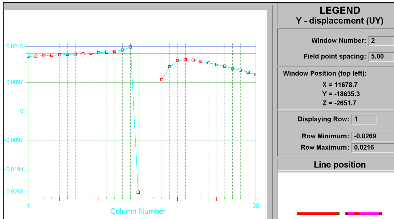
Figure C-16 UY closure at STEP 1
