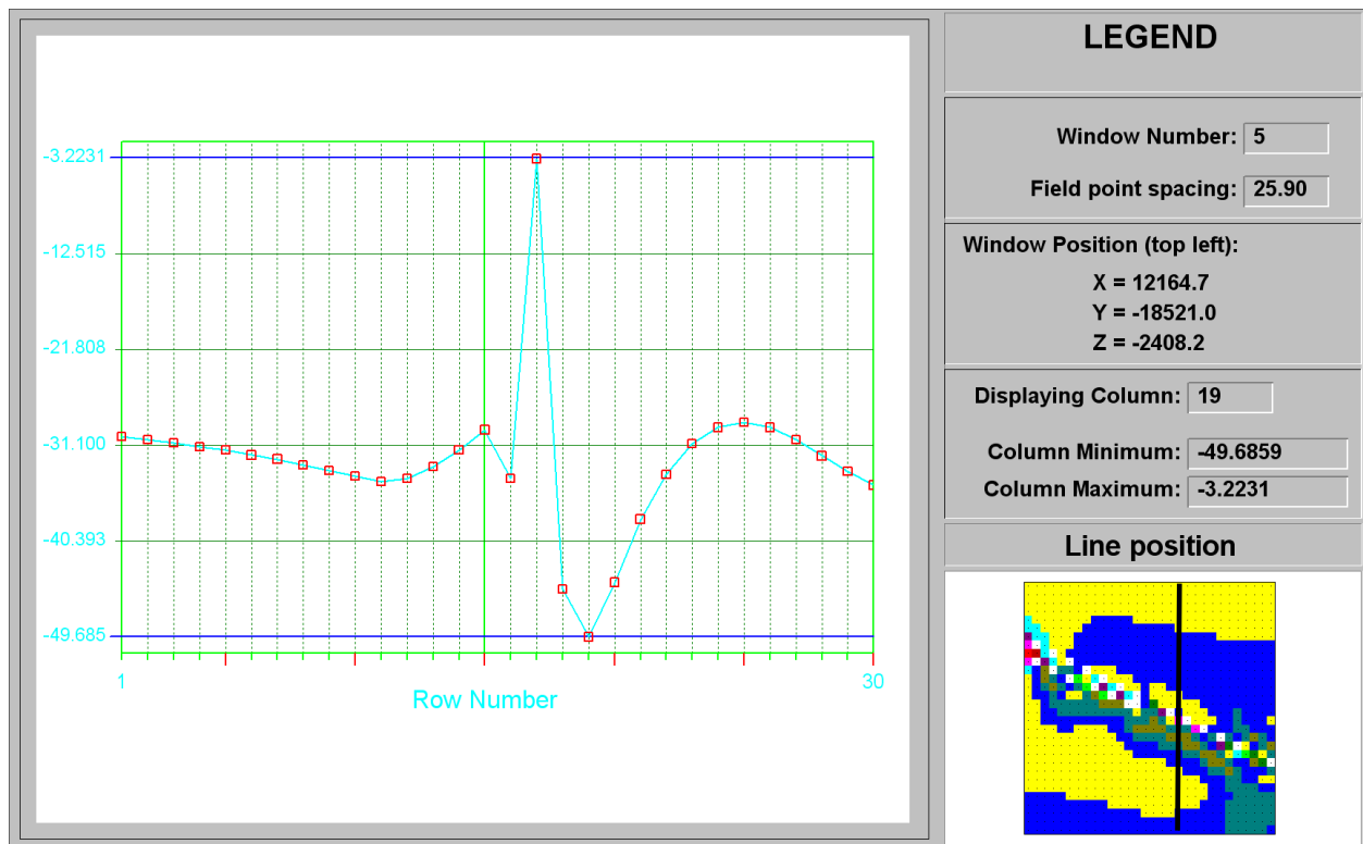
Figure C-105 ESS line plot at column 19 of Smith Fault at STEP 15
