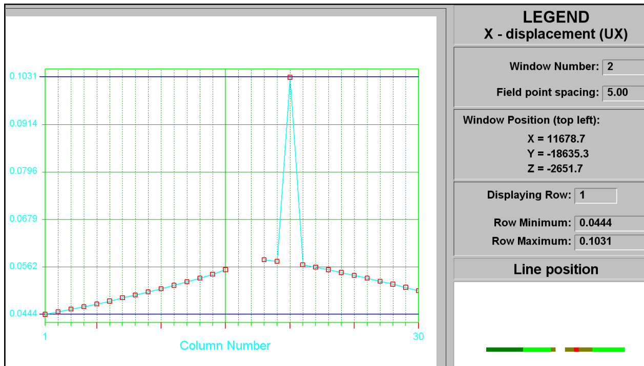
Figure C-37 UX closure at STEP 7
