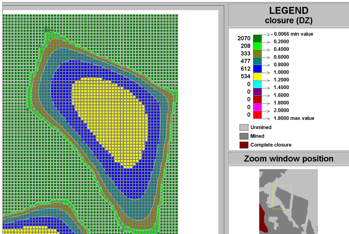
Figure C-166 Contour plot of closure (DZ) of Ya Rona shaft barrel area in Block C at STEP 14
