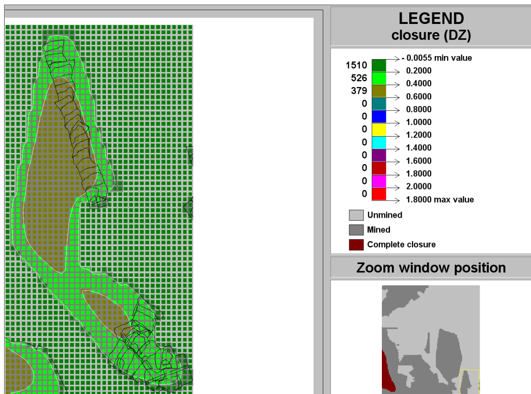
Figure C-152 Contour plot of closure (DZ) of Ya Rona shaft barrel area in Block B at STEP 8
