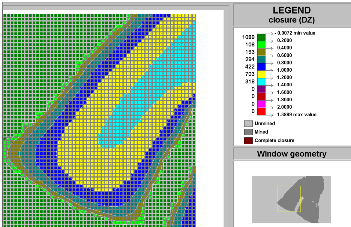
Figure C-195 Contour plot of closure (DZ) of Ya Rona shaft barrel area in Block E at STEP 15
