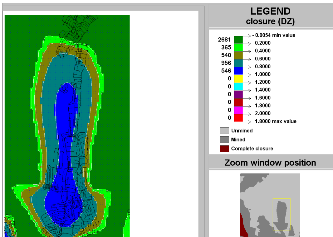
Figure C-134 Contour plot of closure (DZ) of Ya Rona shaft barrel area in Block A at STEP 5
