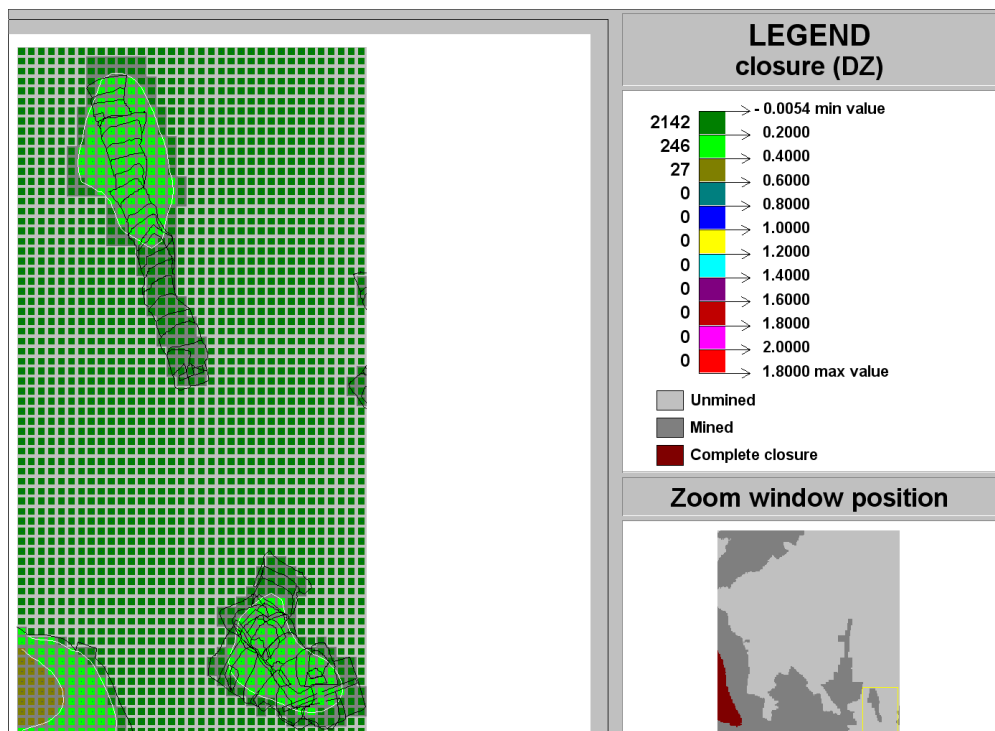
Figure C-146 Contour plot of closure (DZ) of Ya Rona shaft barrel area in Block B at STEP 2
