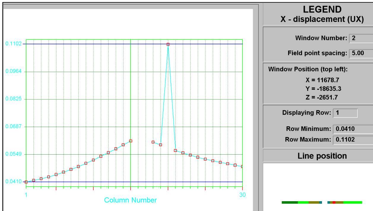
Figure C-38 UX closure at STEP 8
