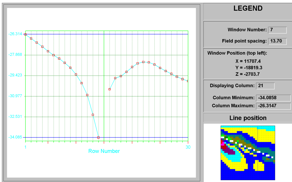
Figure C-113 ESS line plot at column 21 of Shane's Fault at STEP 8
