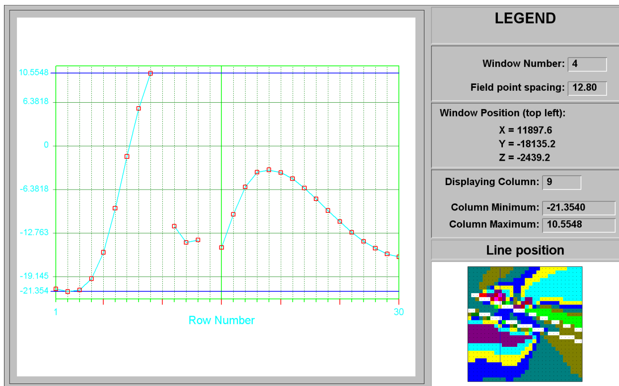
Figure C-73 ESS line plot at column 9 of Kate's Fault at STEP 13
