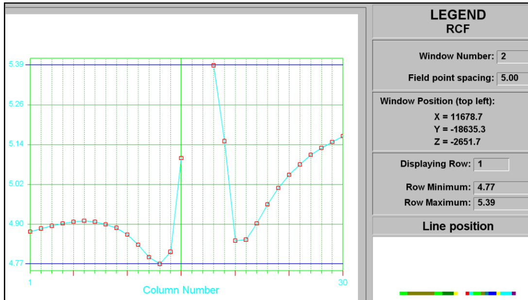
Figure C-1 RCF of shaft barrel at STEP 1
