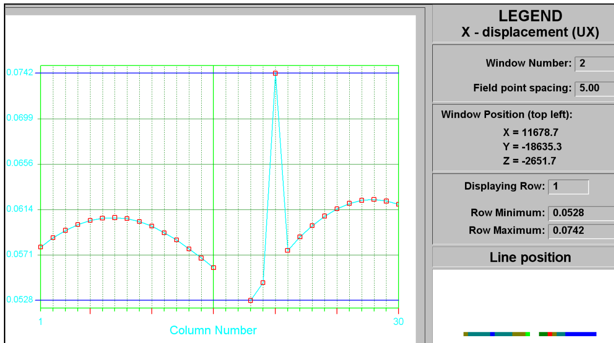
Figure C-41 UX closure at STEP 11
