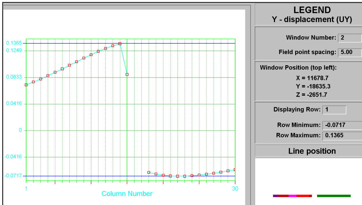
Figure C-20 UY closure at STEP 5
