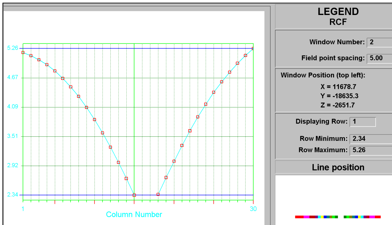
Figure C-10 RCF of shaft barrel at STEP 10
