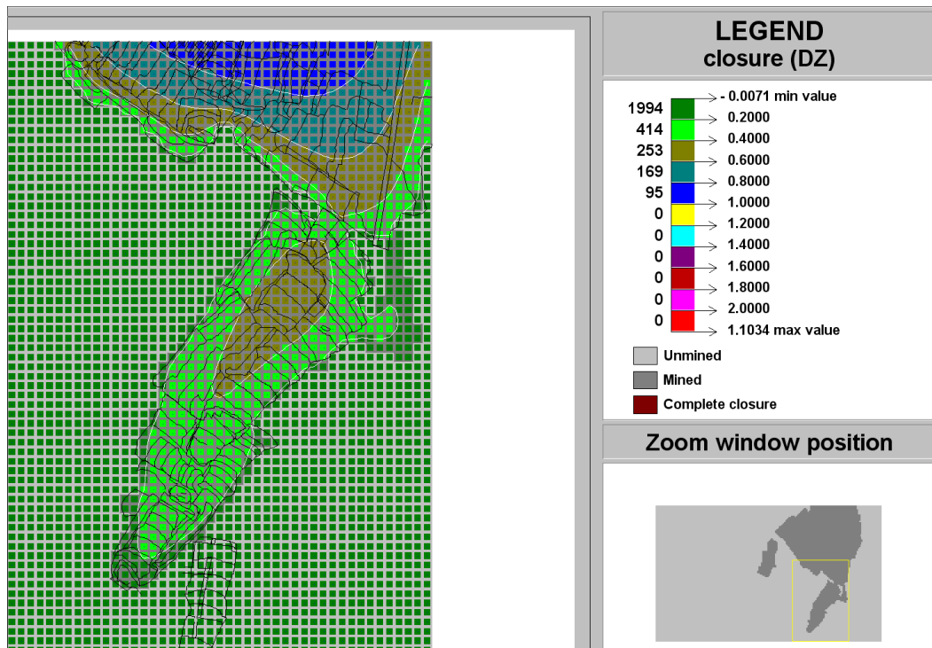
Figure C-169 Contour plot of closure (DZ) of Ya Rona shaft barrel area in Block D at STEP 2
