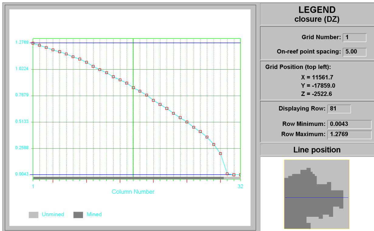
Figure C-198 Contour plot of closure (DZ) of Ya Rona shaft barrel area in Block F at STEP 10
