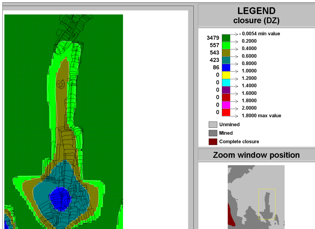
Figure C-132 Contour plot of closure (DZ) of Ya Rona shaft barrel area in Block A at STEP 3
