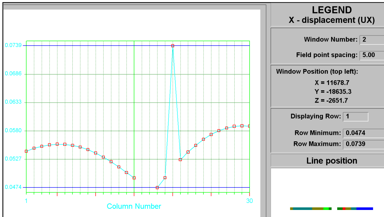
Figure C-40 UX closure at STEP 10
