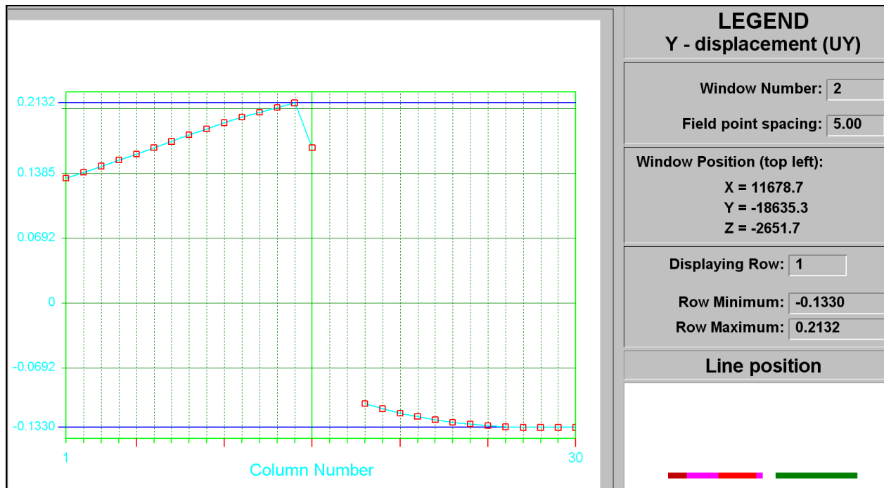
Figure C-24 UY closure at STEP 9
