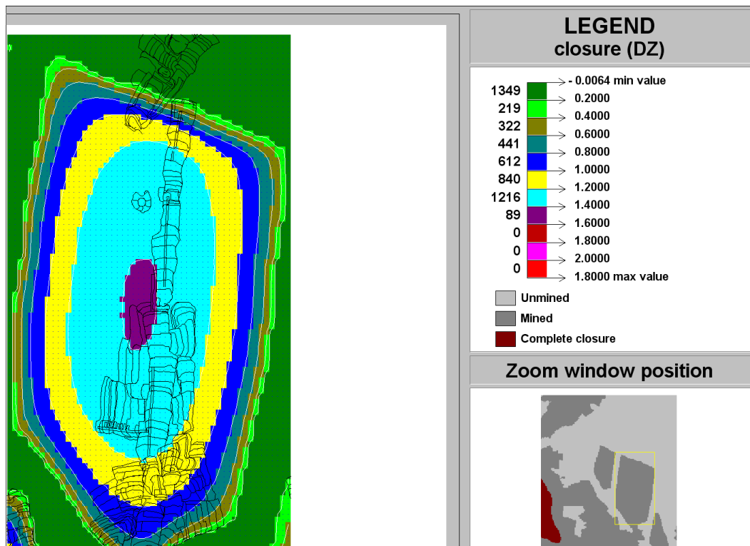
Figure C-140 Contour plot of closure (DZ) of Ya Rona shaft barrel area in Block A at STEP 11
