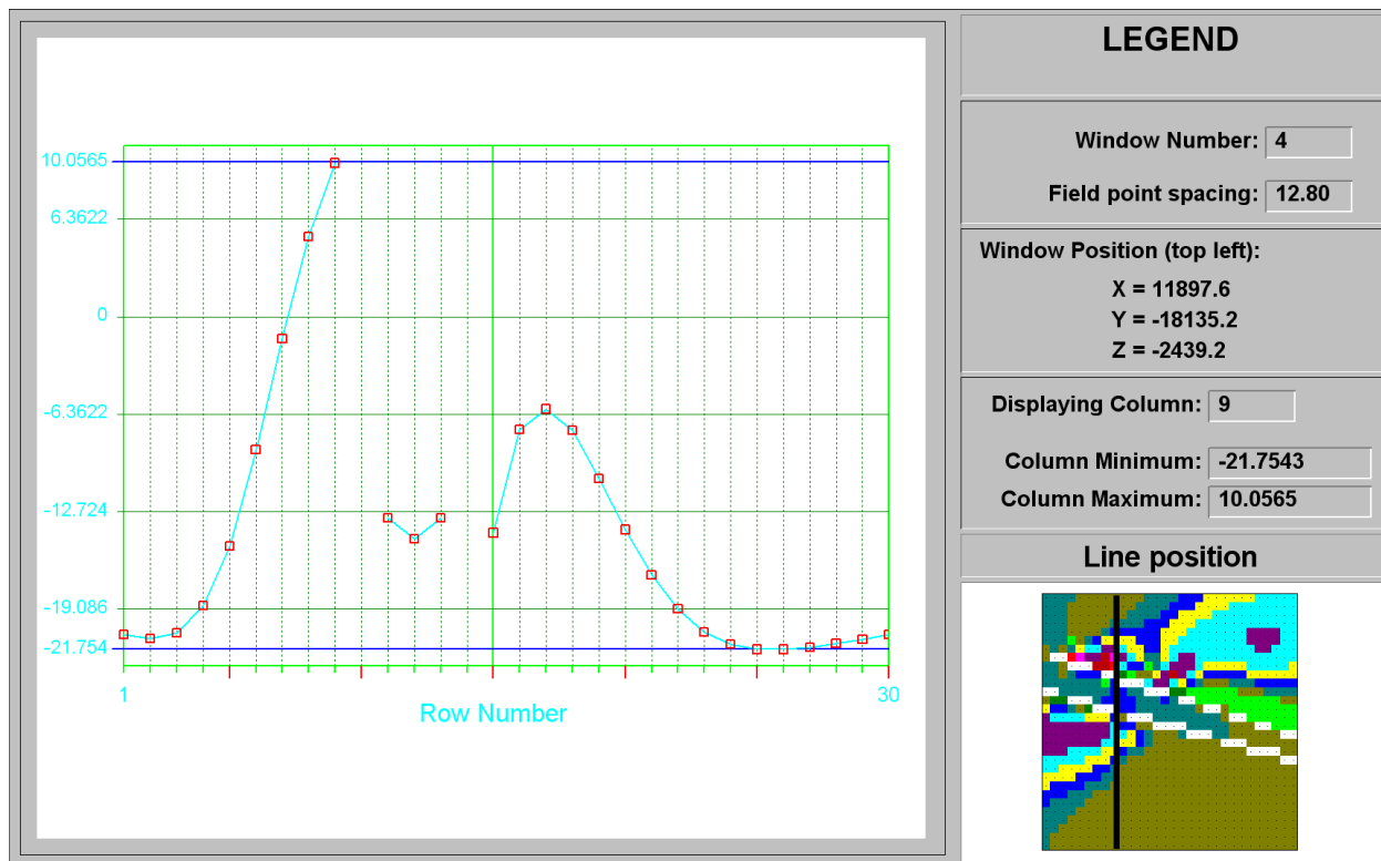
Figure C-70 ESS line plot at column 9 of Kate's Fault at STEP 10
