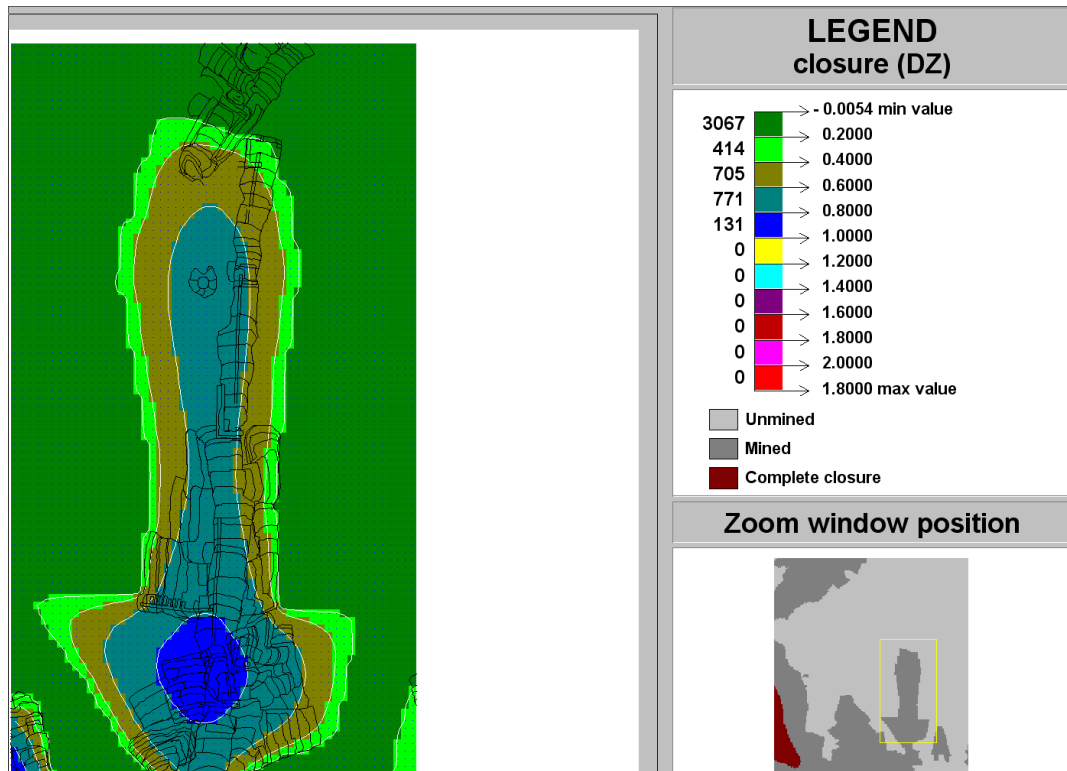
Figure C-133 Contour plot of closure (DZ) of Ya Rona shaft barrel area in Block A at STEP 4
