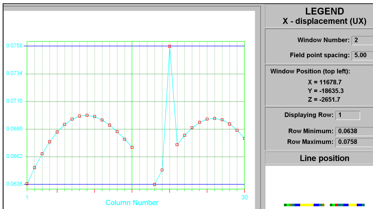
Figure C-44 UX closure at STEP 14
