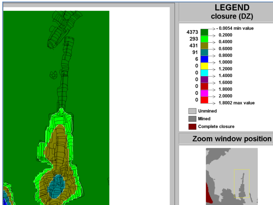
Figure C-130 Contour plot of closure (DZ) of Ya Rona shaft barrel area in Block A at STEP 1
