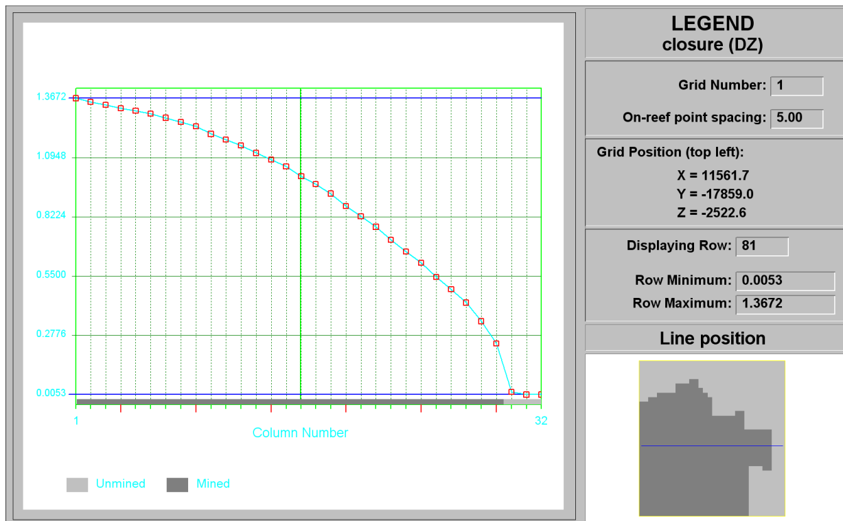
Figure C-200 Contour plot of closure (DZ) of Ya Rona shaft barrel area in Block F at STEP 12
