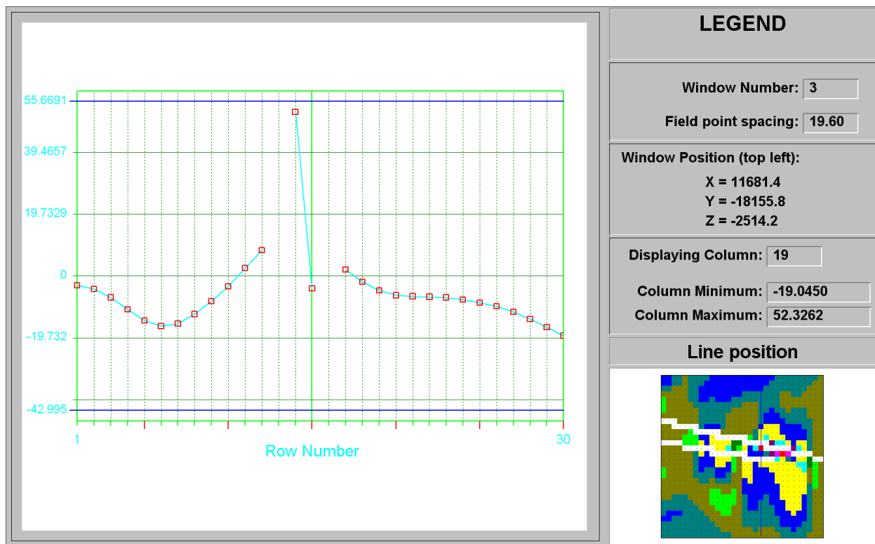
Figure C-86 ESS line plot at column 19 of Murray Fault at STEP 11
