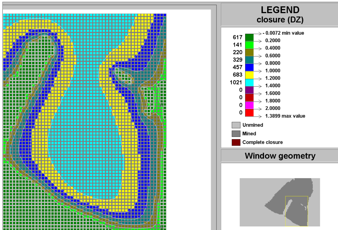
Figure C-180 Contour plot of closure (DZ) of Ya Rona shaft barrel area in Block D at STEP 15
