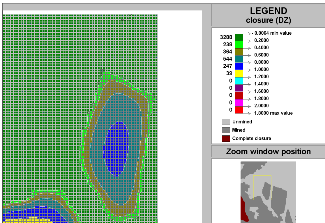
Figure C-163 Contour plot of closure (DZ) of Ya Rona shaft barrel area in Block C at STEP 11
