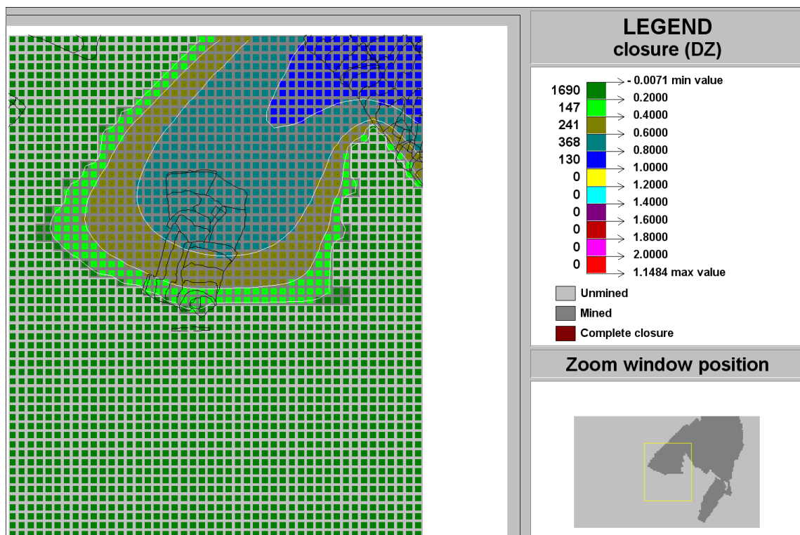
Figure C-186 Contour plot of closure (DZ) of Ya Rona shaft barrel area in Block E at STEP 6
