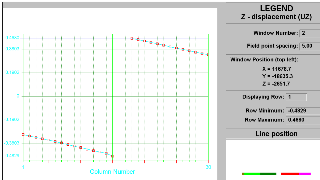
Figure C-52 UZ closure at STEP 7
