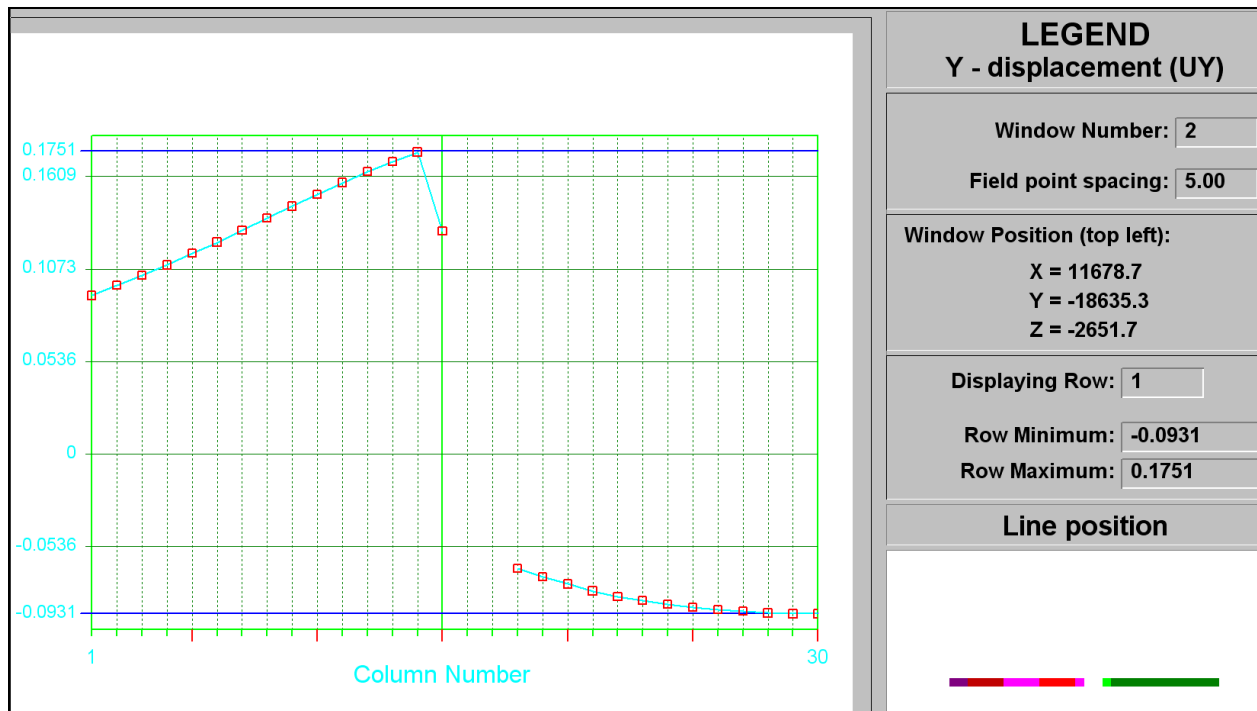
Figure C-22 UY closure at STEP 7
