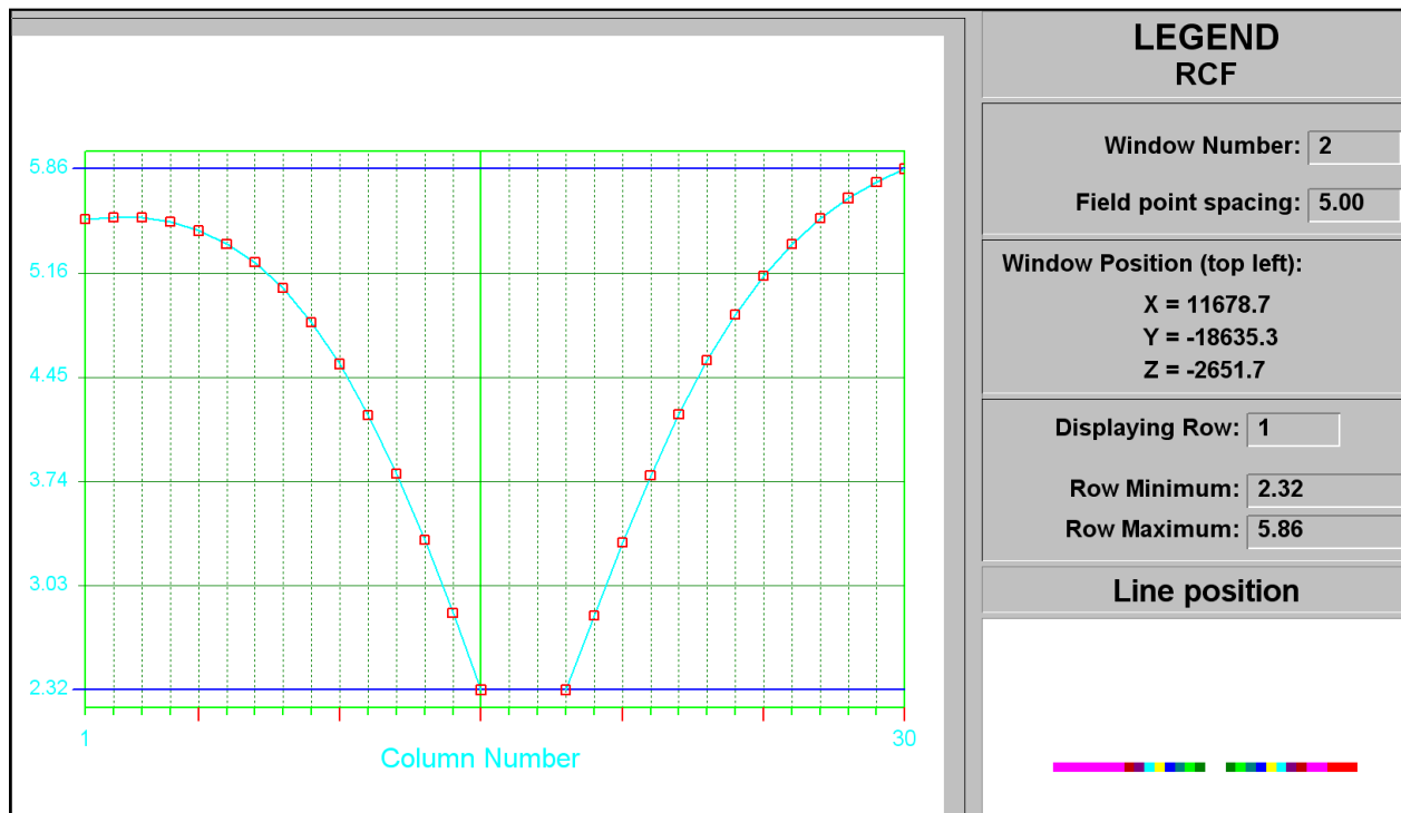
Figure C-6 RCF of shaft barrel at STEP 6
