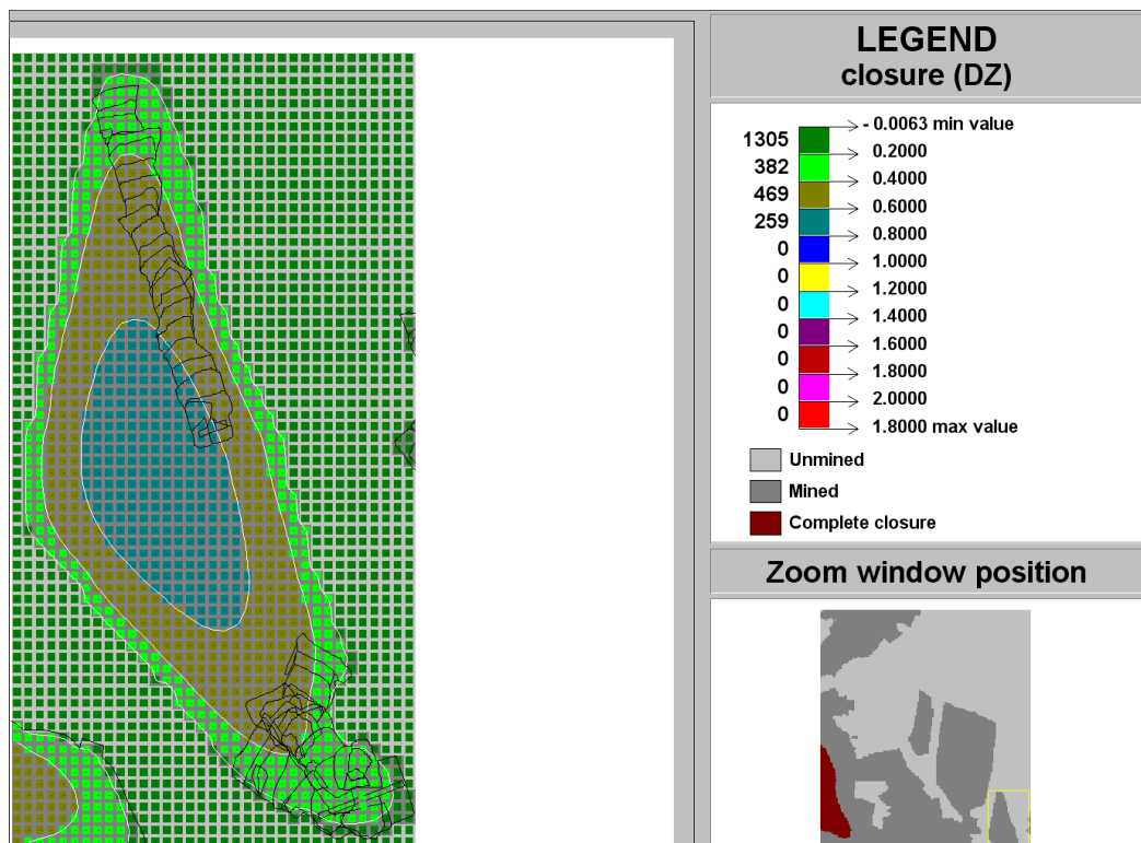
Figure C-154 Contour plot of closure (DZ) of Ya Rona shaft barrel area in Block B at STEP 10
