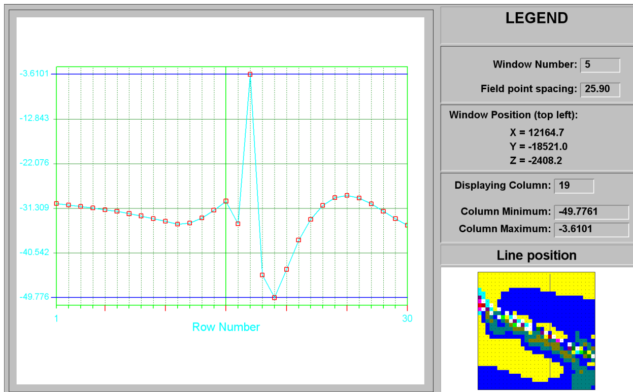
Figure C-102 ESS line plot at column 19 of Smith Fault at STEP 12
