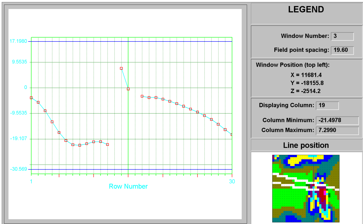
Figure C-81 ESS line plot at column 19 of Murray Fault at STEP 6
