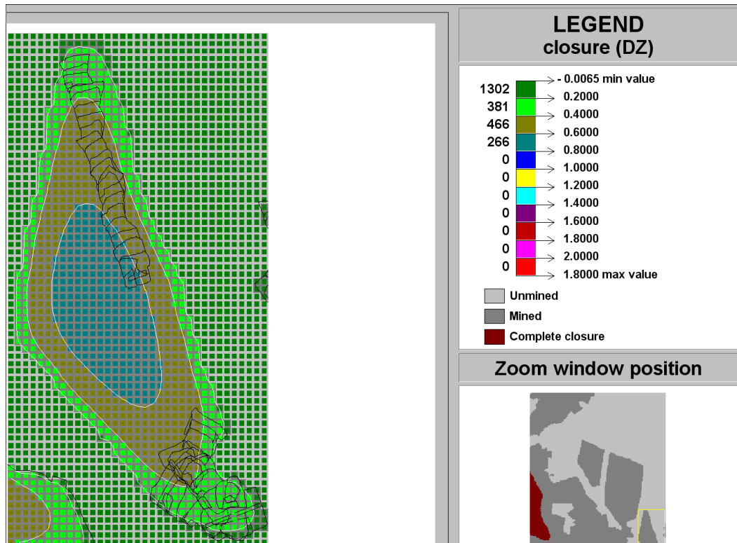
Figure C-156 Contour plot of closure (DZ) of Ya Rona shaft barrel area in Block B at STEP 12
