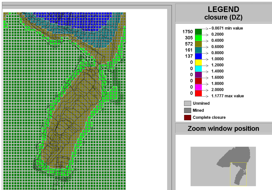
Figure C-172 Contour plot of closure (DZ) of Ya Rona shaft barrel area in Block D at STEP 5
