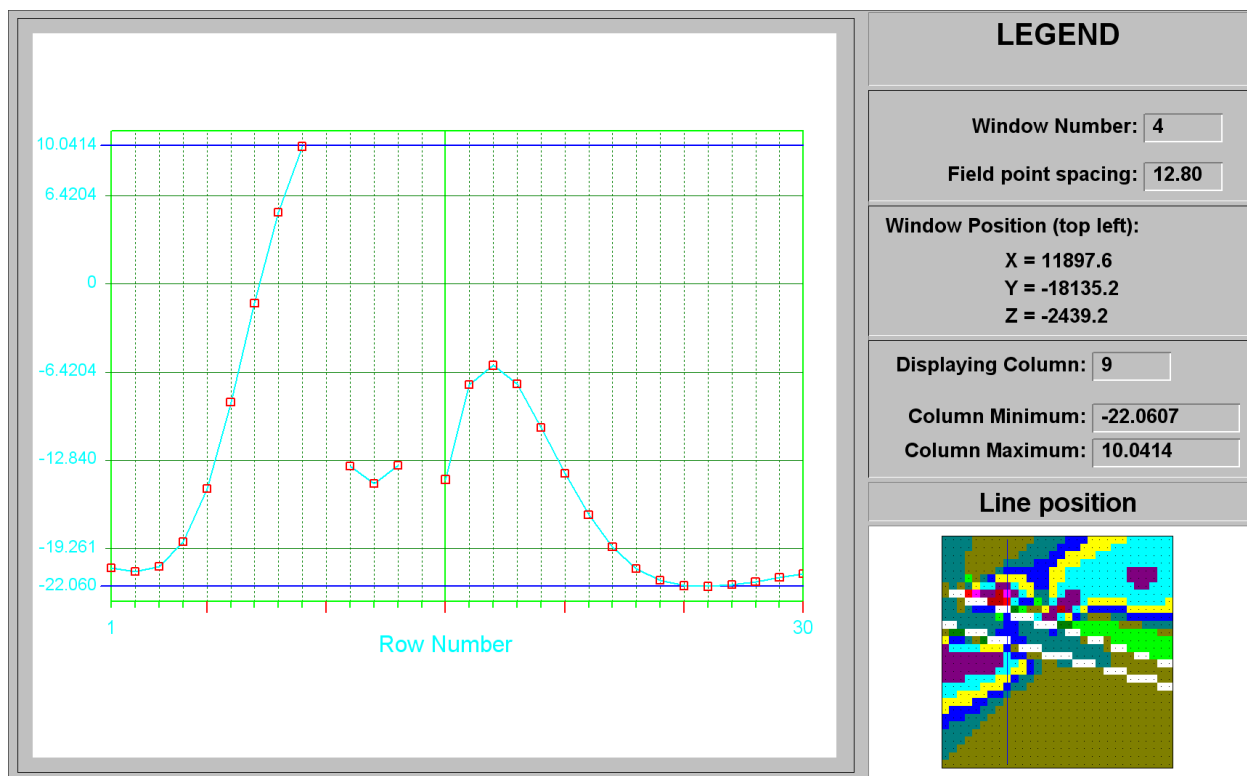
Figure C-69 ESS line plot at column 9 of Kate's Fault at STEP 9
