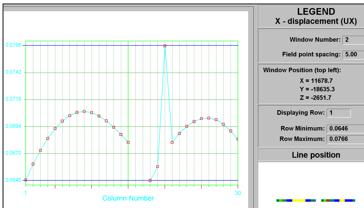
Figure C-45 UX closure at STEP 15
