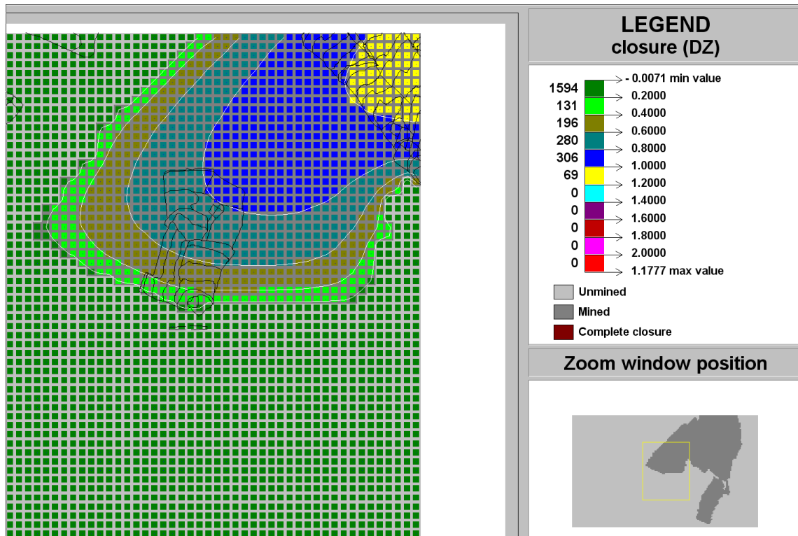
Figure C-187 Contour plot of closure (DZ) of Ya Rona shaft barrel area in Block E at STEP 7
