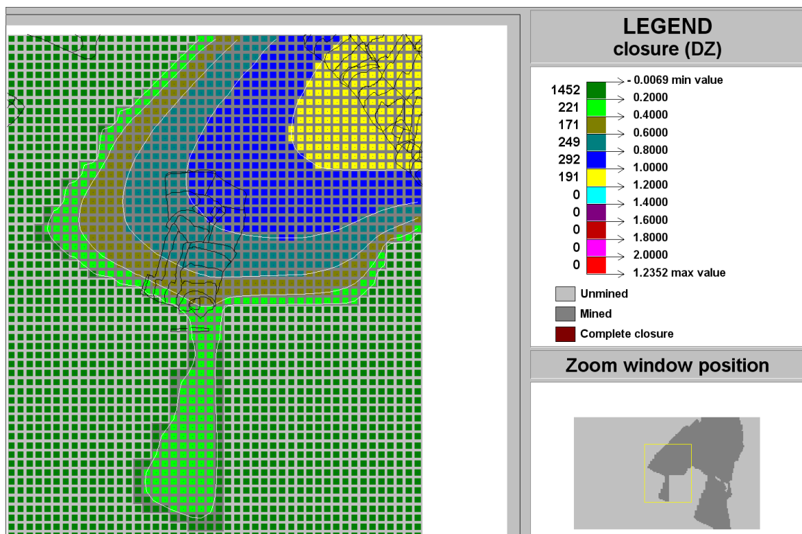
Figure C-190 Contour plot of closure (DZ) of Ya Rona shaft barrel area in Block E at STEP 10
