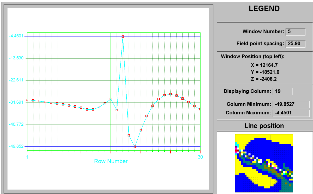
Figure C-100 ESS line plot at column 19 of Smith Fault at STEP 10
