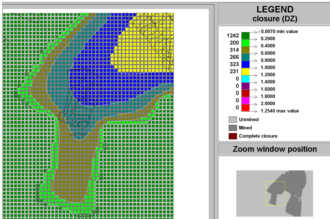
Figure C-191 Contour plot of closure (DZ) of Ya Rona shaft barrel area in Block E at STEP 11
