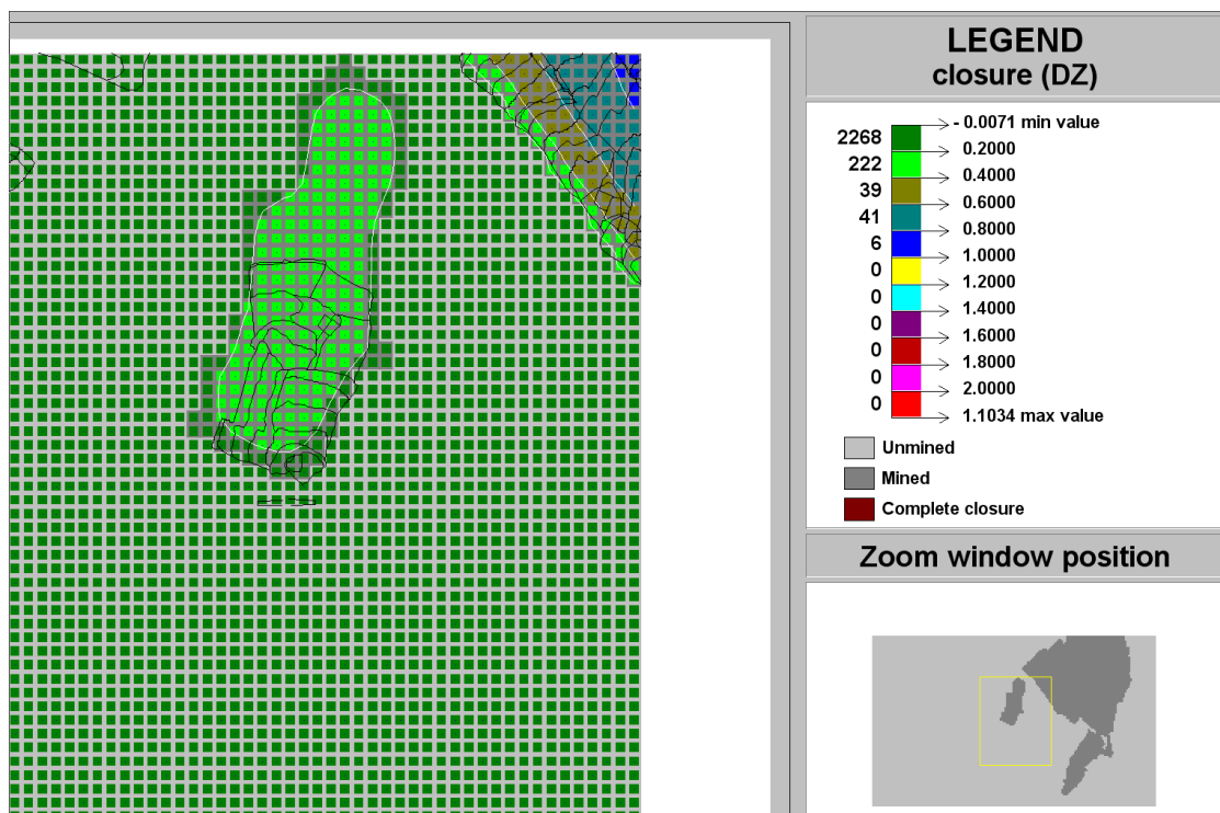
Figure C-182 Contour plot of closure (DZ) of Ya Rona shaft barrel area in Block E at STEP 2
