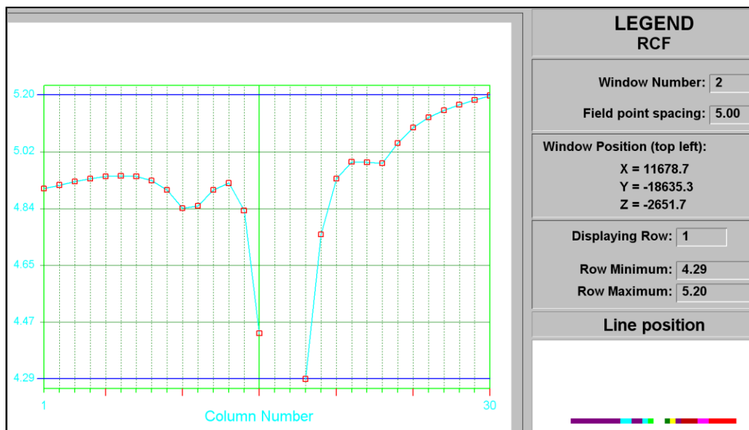
Figure C-2 RCF of shaft barrel at STEP 2
