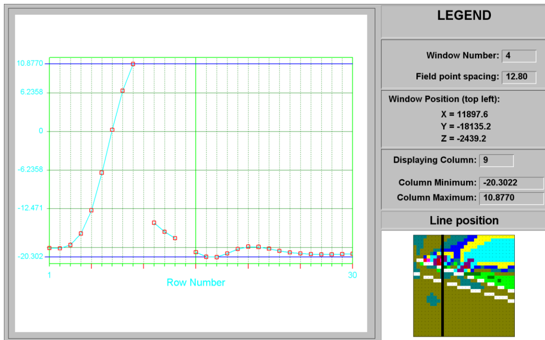
Figure C-61 ESS line plot at column 9 of Kate's Fault at STEP 1
