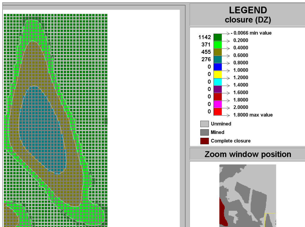
Figure C-158 Contour plot of closure (DZ) of Ya Rona shaft barrel area in Block B at STEP 14
