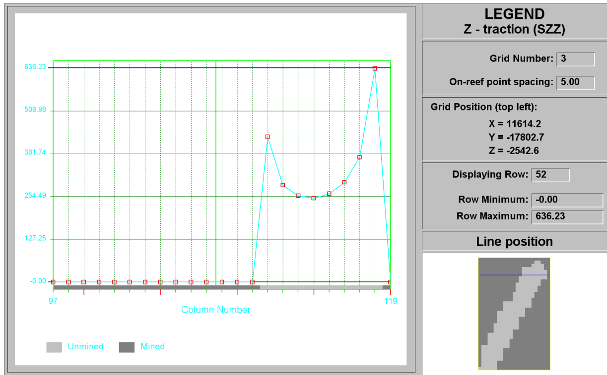
Figure C-127 Line plot at row 52 (SECTION P-Q) of Regional Stability Pillar ZZ at STEP 15
