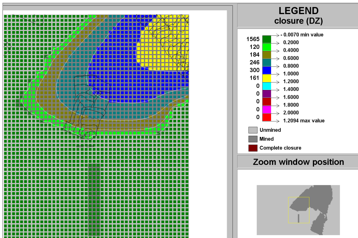
Figure C-189 Contour plot of closure (DZ) of Ya Rona shaft barrel area in Block E at STEP 9
