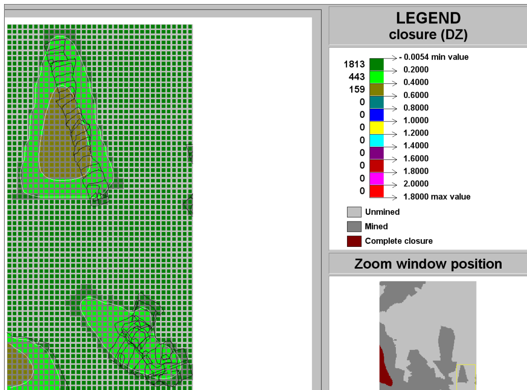
Figure C-149 Contour plot of closure (DZ) of Ya Rona shaft barrel area in Block B at STEP 5
