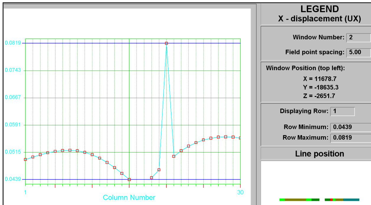
Figure C-35 UX closure at STEP 5
