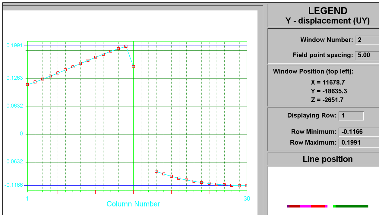
Figure C-23 UY closure at STEP 8
