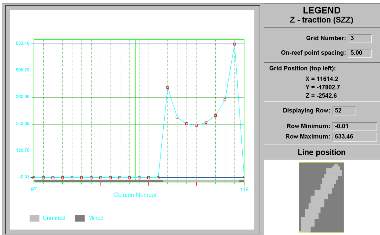
Figure C-126 Line plot at row 52 (SECTION P-Q) of Regional Stability Pillar ZZ at STEP 14
