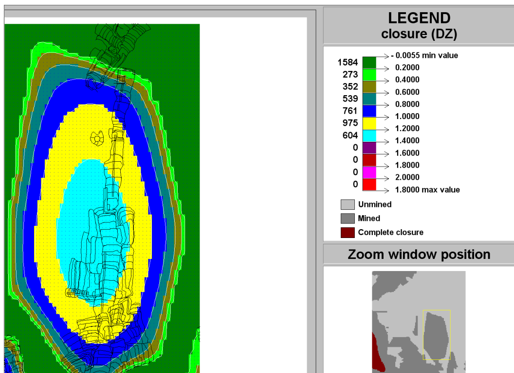
Figure C-137 Contour plot of closure (DZ) of Ya Rona shaft barrel area in Block A at STEP 8
