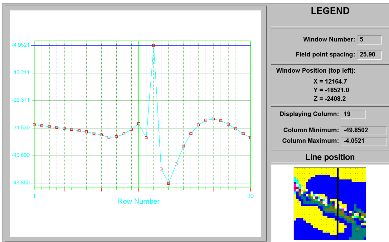
Figure C-101 ESS line plot at column 19 of Smith Fault at STEP 11
