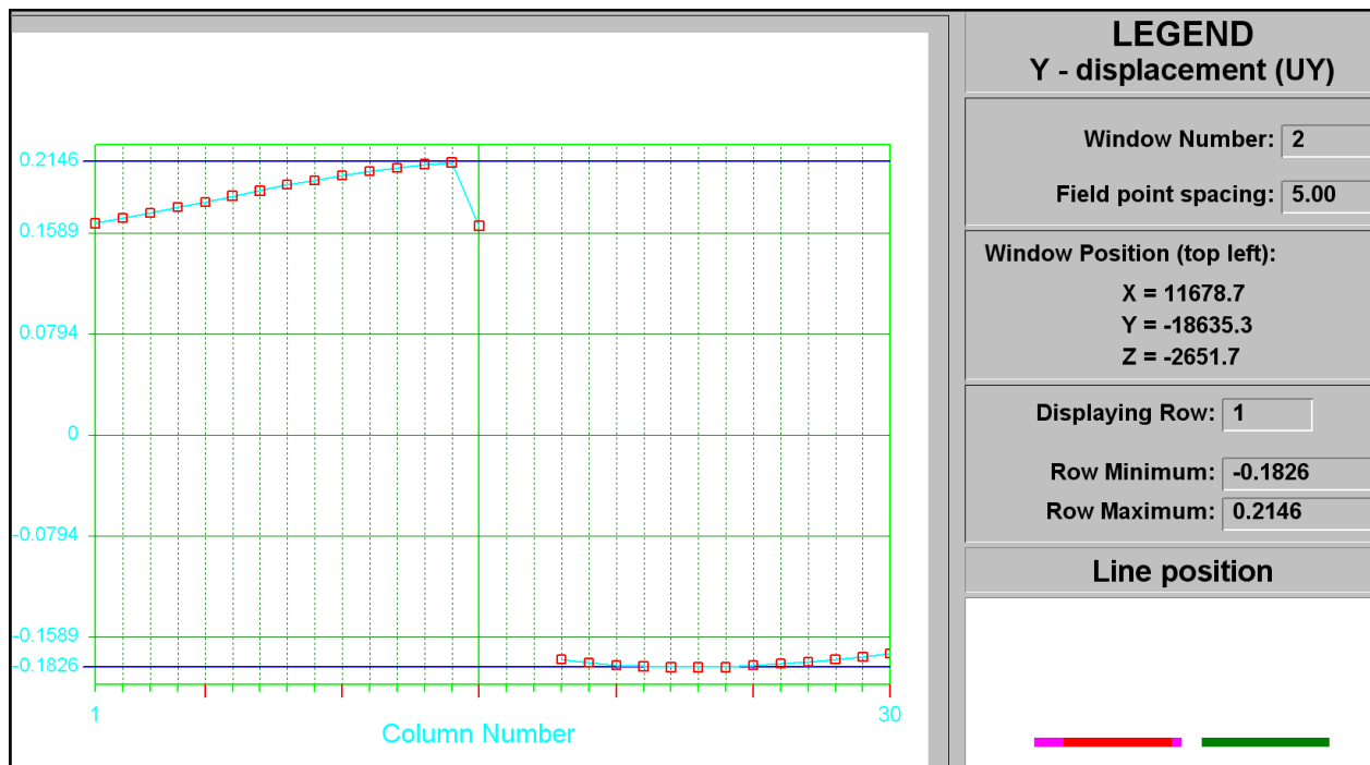
Figure C-29 UY closure at STEP 14
