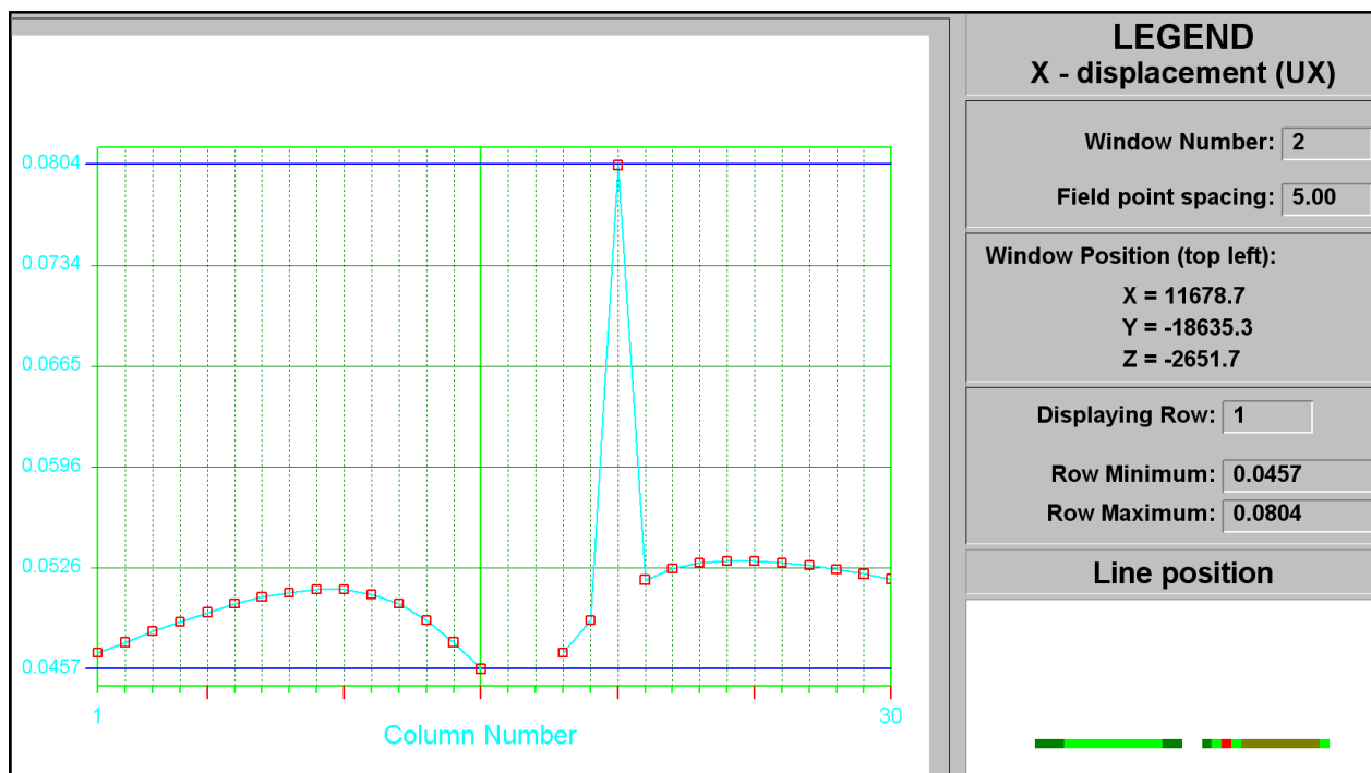
Figure C-33 UX closure at STEP 3
