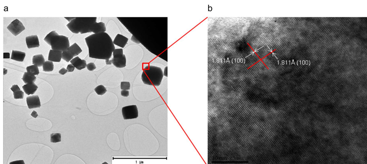
Figure 5.3: a) cube-shaped copper nanocrystals; b) lattice fringes and spacing of 1.811 Å (100).
