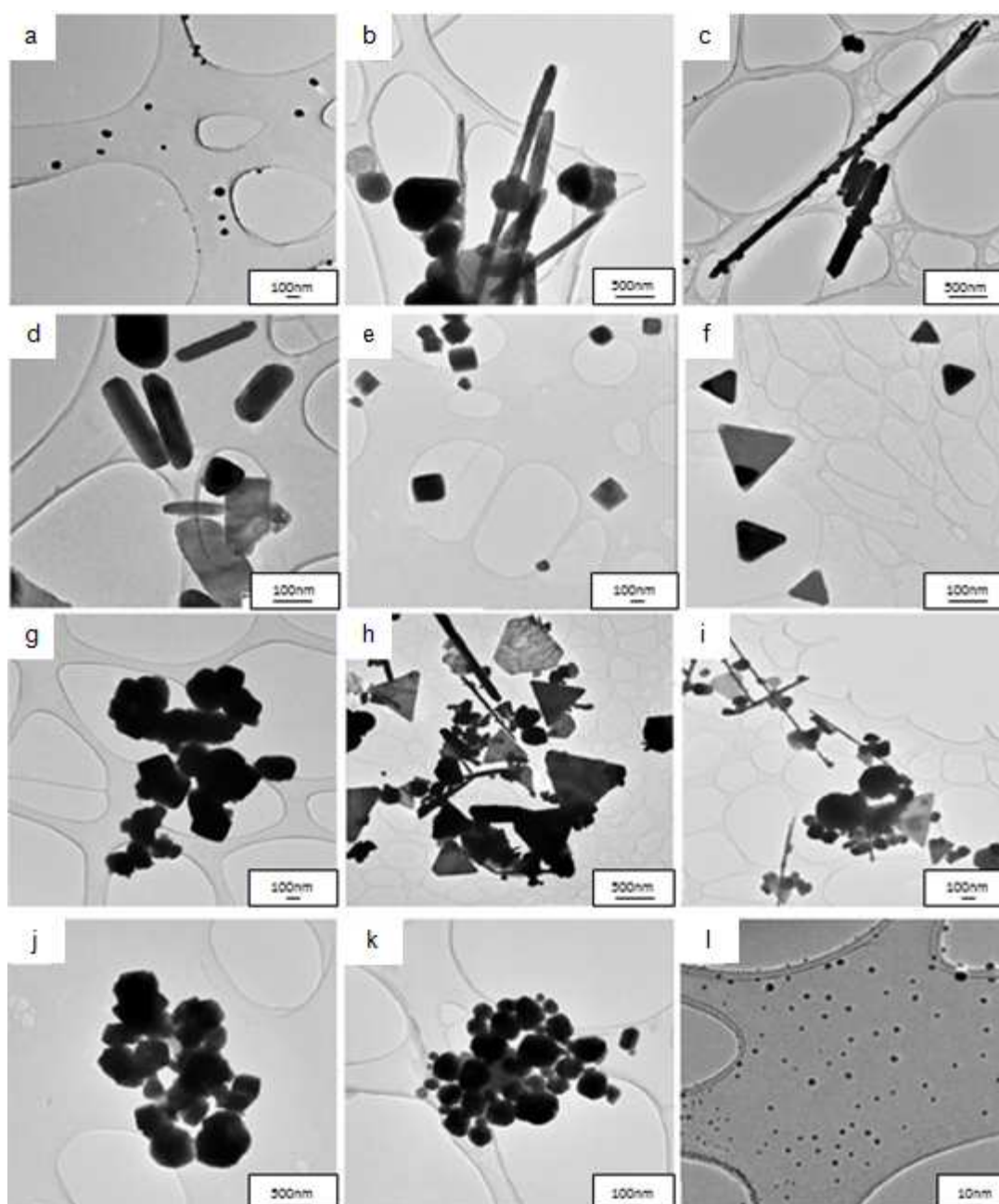
Figure 3.1: a) sample S1, spherical nanoparticles (90nm); b) sample S2, combination of spheres and rods; c) sample S3, combination spheres and rods with predominant rods; d) sample S4, rod-like nanoparticles; e) sample S5, cubic-shaped nanoparticles; f) sample S6, pyramidal nanoparticles; g) sample S7, irregular spherical particles; h) sample S8, combination of neo-geometrical nanoparticles; i) sample S9, combination of neo-geometrical nanoparticles at reduced size range; j) sample S10, irregular nanospheres; k) sample S11, spherical nanoparticles (250–300nm); l) sample S12, spherical nanoparticles (5nm).
