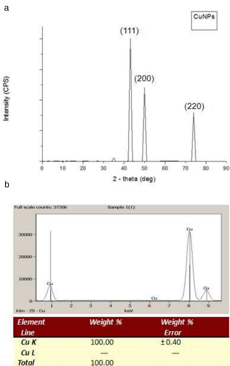
Figure 3.4: a) powder X-Ray diffraction patterns of synthesized copper nanocrystals; b) energy dispersive spectra showing pure elemental copper.
