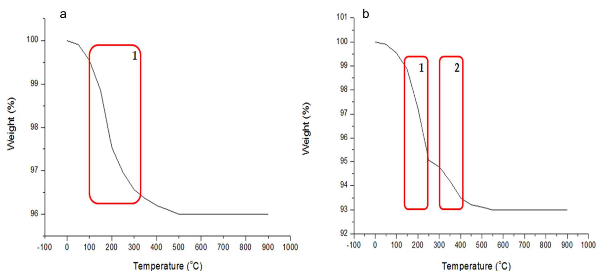
Figure 4.4: TGA analysis confirming the surfactant adsorption on the CuNPs.
