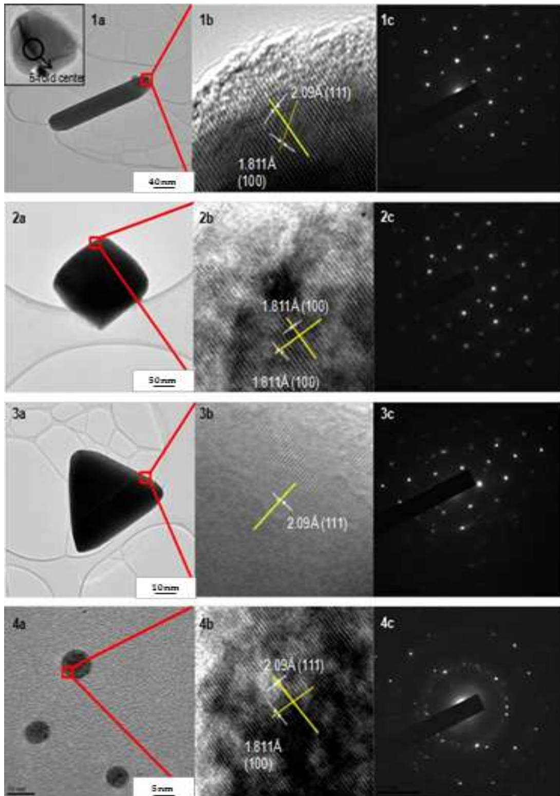
Figure 3.3: 1a) rod-shaped nanoparticle and inset showing 5-fold center of the decahedral geometry at (111); 1b) lattice fringes and spacing of rod-shaped nanoparticle; 1c) uniform SAED patterns; 2a) Cube-shaped nanoparticle; 2b) lattice fringes and spacing of cube-shaped nanoparticle; 2c) uniform SAED patterns; 3a) Pyramid-shaped nanoparticle; 3b) lattice fringes and spacing of pyramid-shaped nanoparticle; 3c) uniform SAED patterns; 4a) Spherically-shaped nanoparticles; 4b) lattice fringes and spacing of spherical nanoparticles; 4c) uniform SAED patterns.
