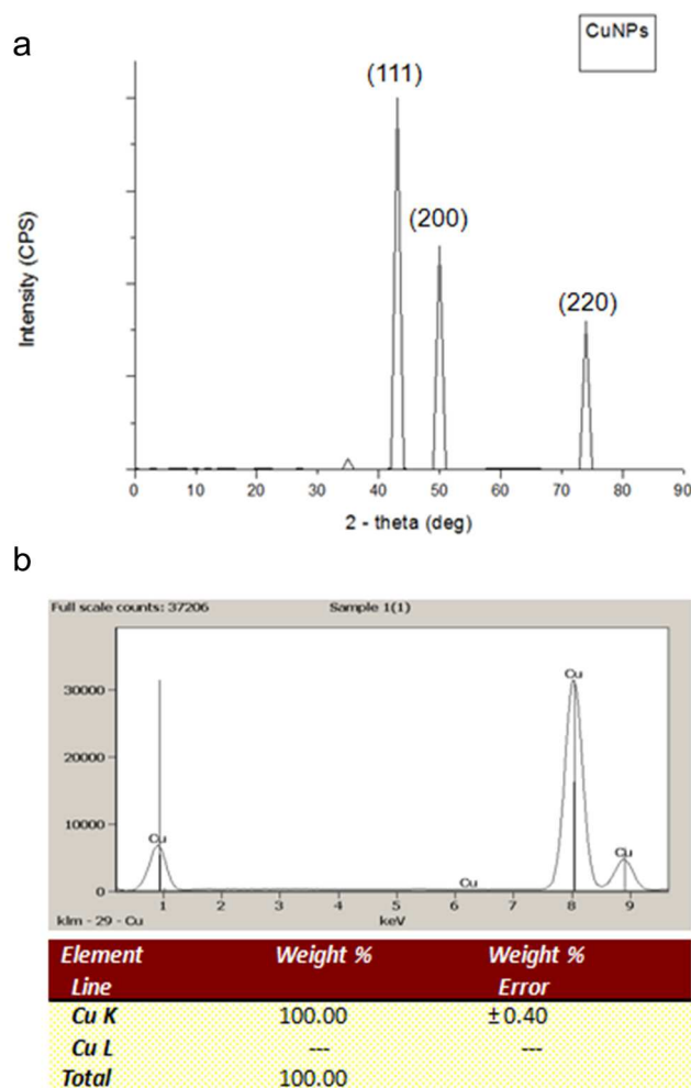
Figure 4.3: a) XRD patterns of the neo-geometric nanosystems; b) energy dispersive spectra indicating elemental analysis.
