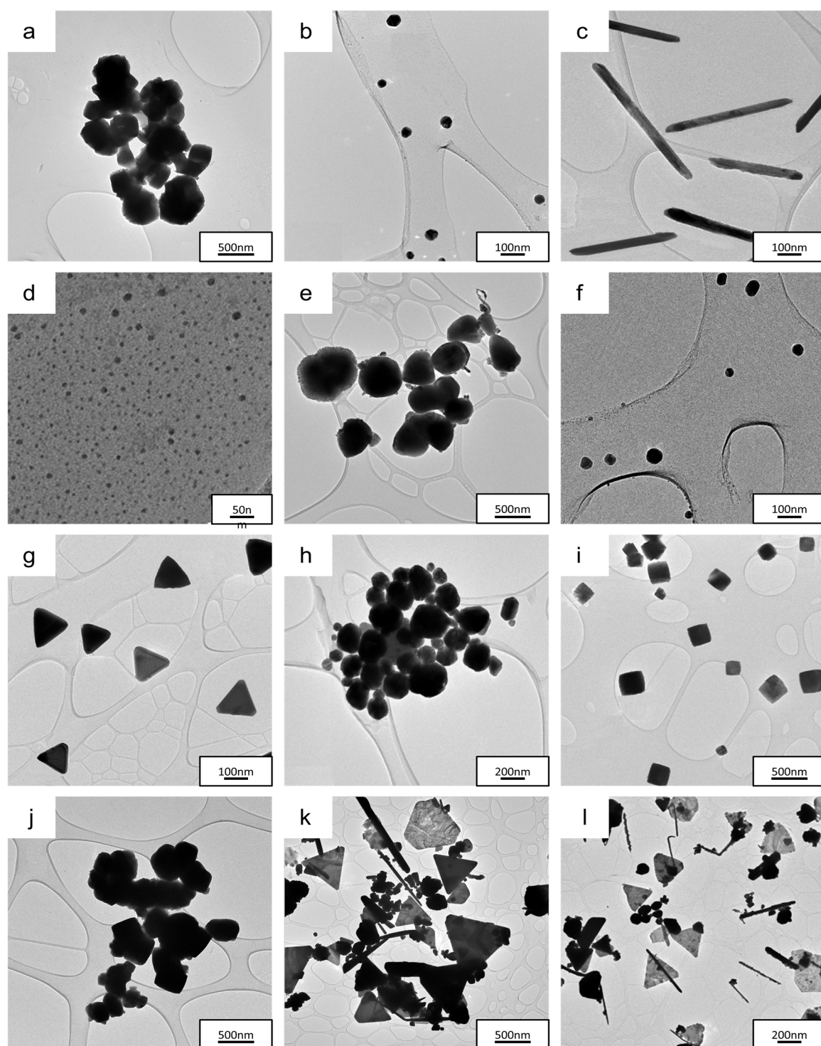
Figure 4.1: TEM images of the nanoparticles synthesized from 12 formulations as per the Full Factorial Design.
