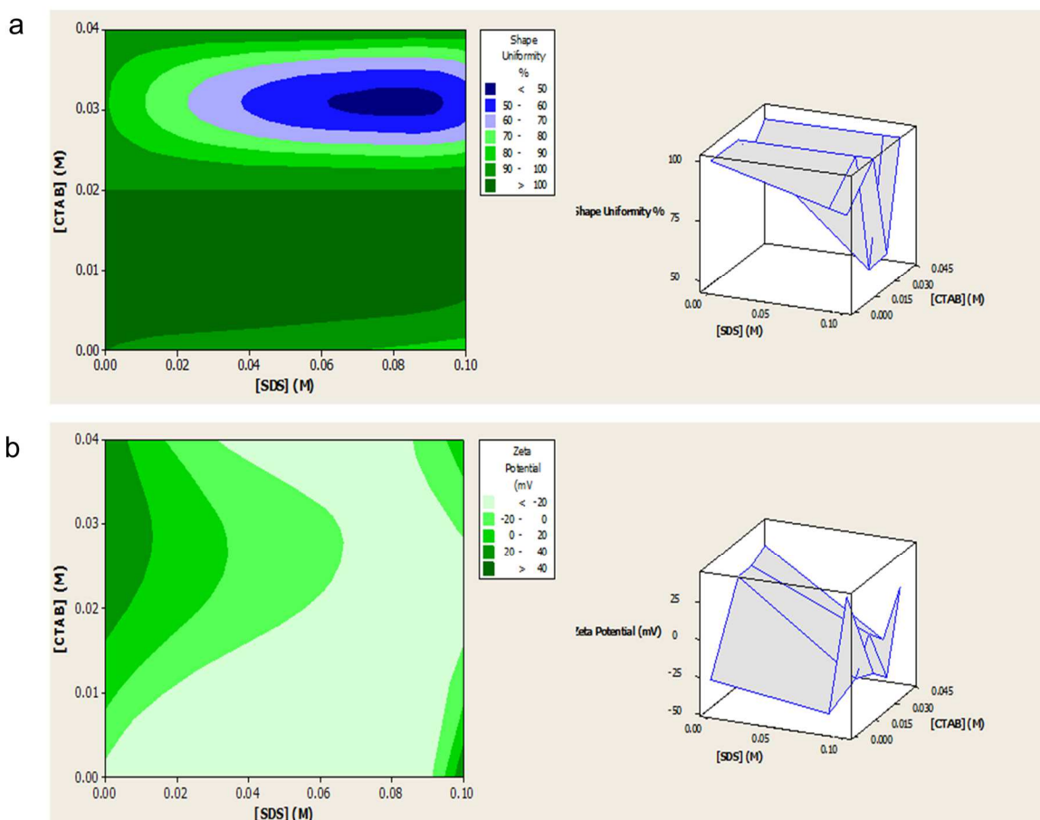
Figure 4.8: Contour plot and response surface plots. a) shape uniformity per sample; b) zeta potential.
