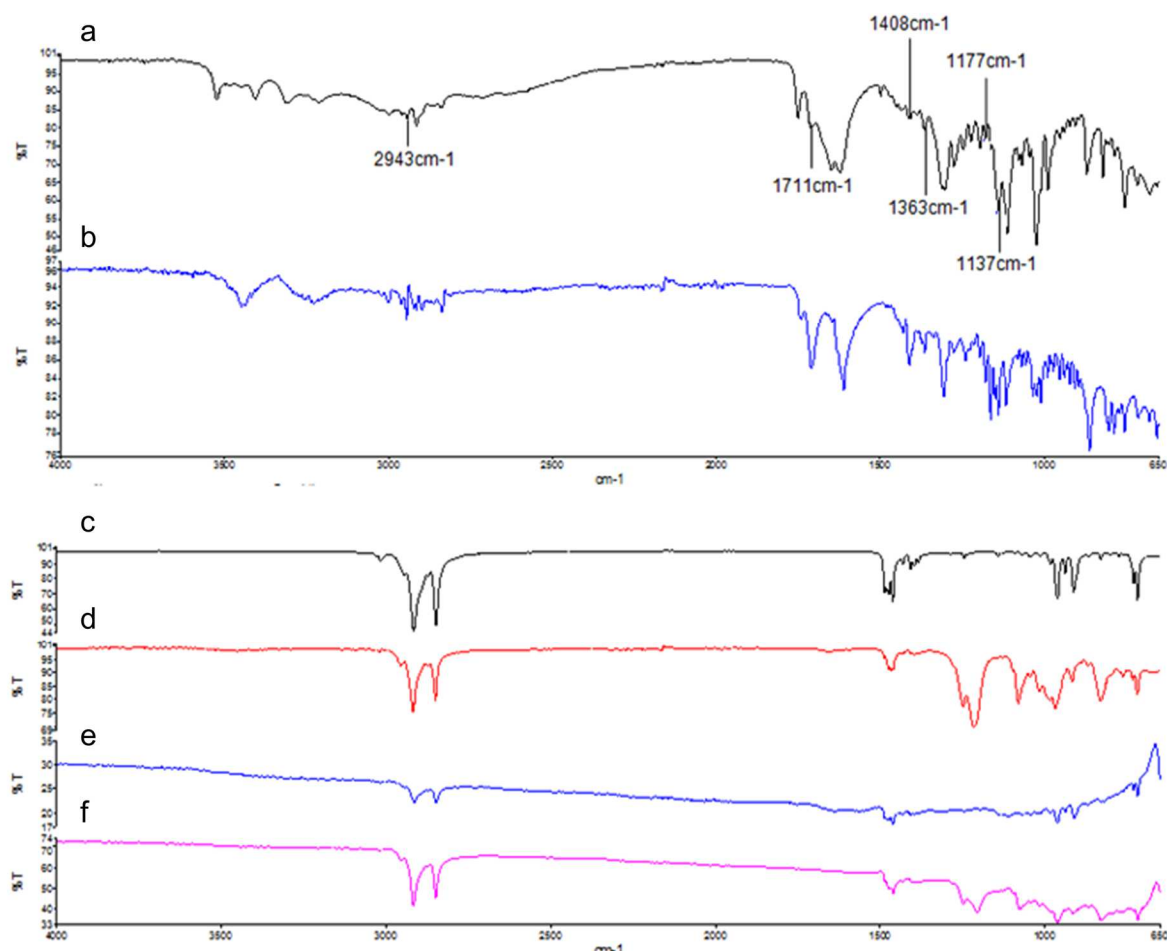
Figure 3.5: FTIR spectra of: a) ascorbic acid; b) sample S1; c) CTAB; d) SDS; e) sample S4; f) sample S5.
