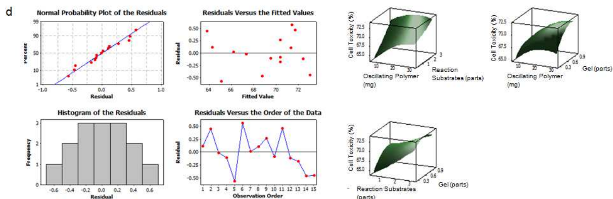
Figure 5.2: Residual (left panel) and surface plots (right panel) of a) average oscillation amplitude; b) duration of oscillations; c) permeation rate; d) cell toxicity.
