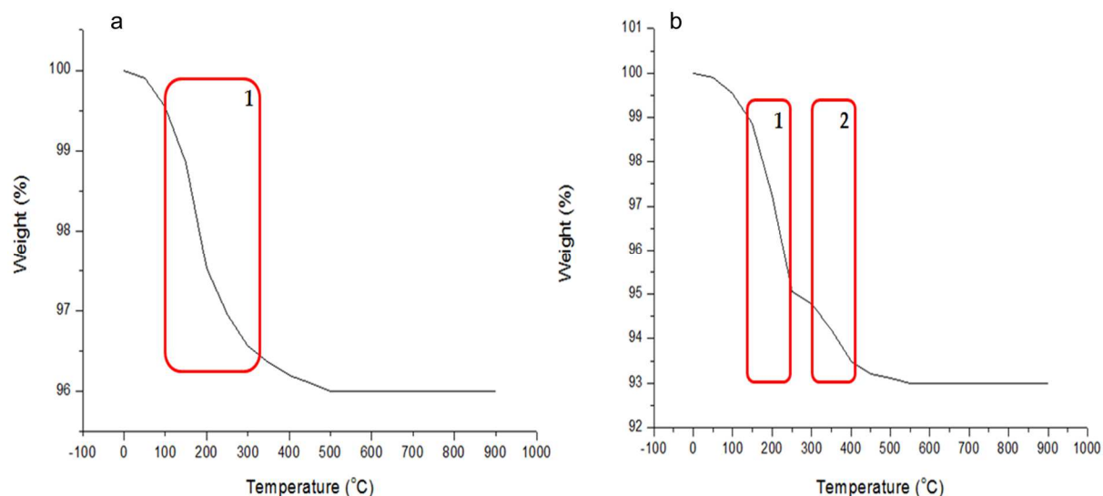
Figure 3.6: TGA curves of: a) sample S1 showing degradation of reducing agent; b) sample S2 showing degradation of surfactants on the nanoparticle surface.
