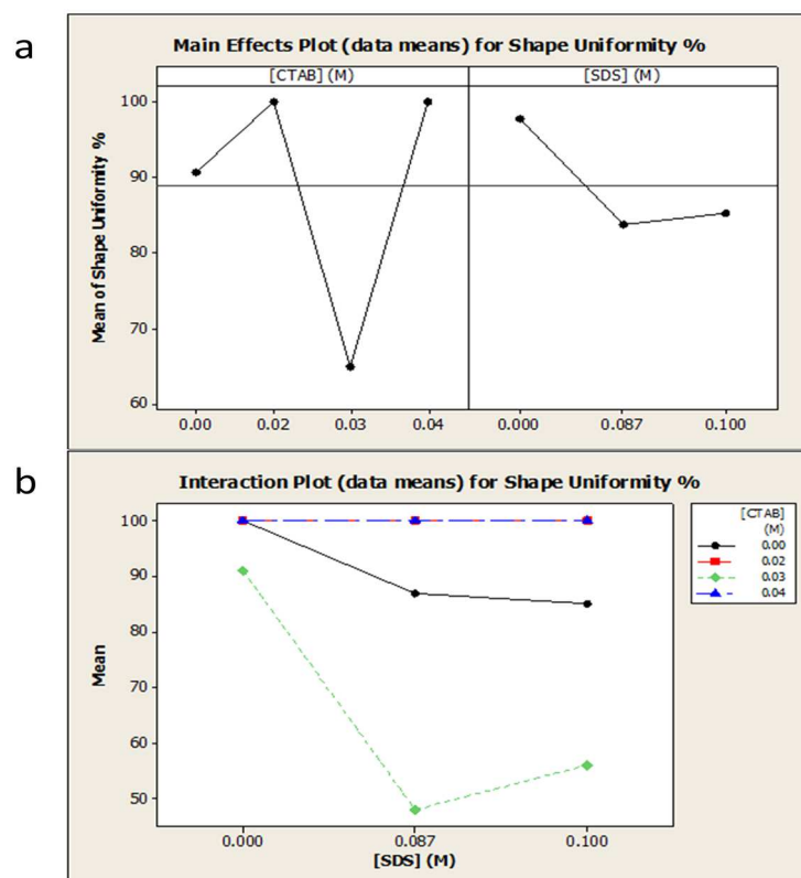
Figure 4.6: a) main effects; b) interaction plots for shape uniformity.
