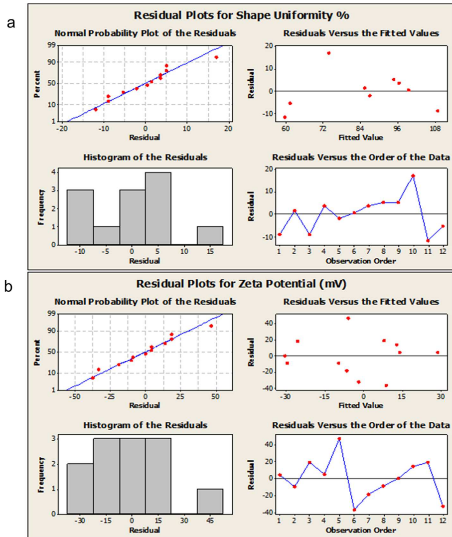
Figure 4.5: Residual plots: a) shape uniformity per sample; b) zeta potential.
