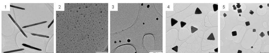
Figure 1. TEM micrographs of monodisperse neo-geometric copper nanoparticles. 1) Rods, 2) 5nm spheres, 3) 100nm spheres, 4) 500nm pyramids, 5) 200nm cubes
