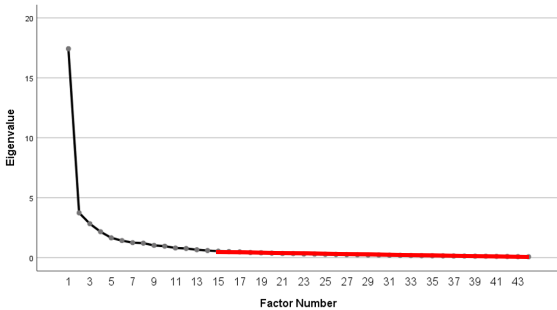
Figure 10: EFA – Scree Plot
