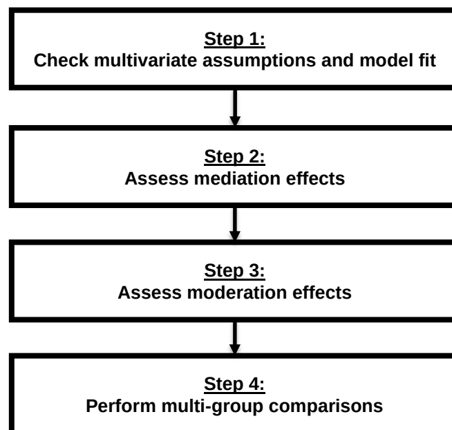
Figure 6: SEM protocol employed
