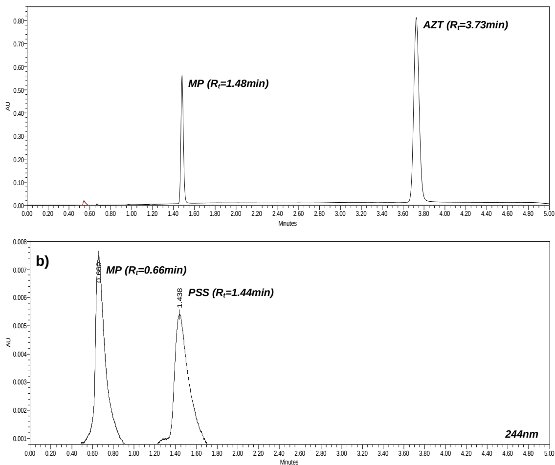
Figure 6.15: UPLC chromatograms depicting the separation of a) AZT and MP (internal standard) and b) PSS and MP (internal standard) in simulated vaginal fluid (pH 4.5; 37°C).
