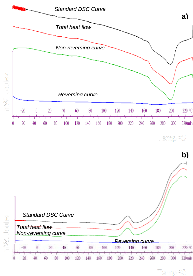
Figure 6.13: TMDSC thermogram for a) the unhydrated physical polymer blend, b) the unhydrated IBPD.
