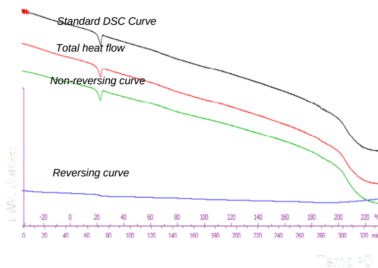
Figure 6.8: TMDSC thermogram for the unhydrated poly (lactic-co-glycolic acid).
