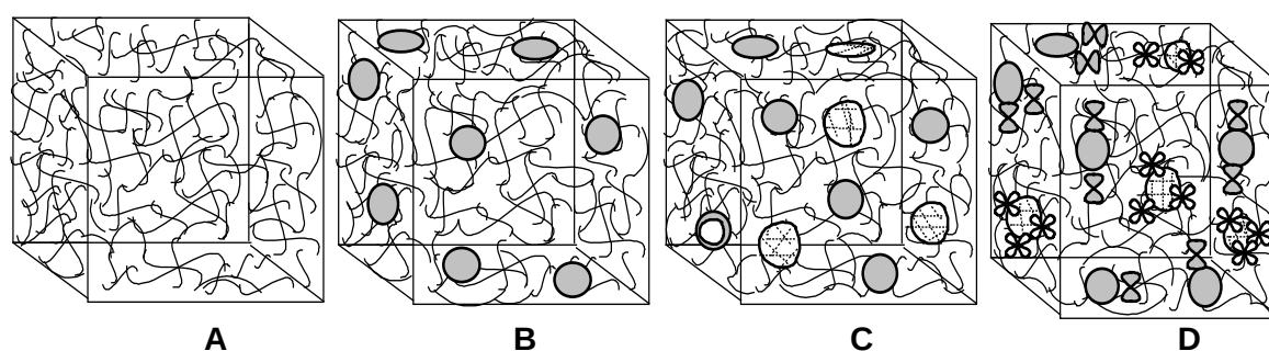
Figure 6.22: A 3D model representing the IBPD matrix under dissolution along with drug associations: a) the polymer matrix, b) fluid interactions producing hydrophilic pockets and swelling of the device, c) generation of hydrophobic areas in the matrix due to critical formulation excipients and d) the drug molecule (AZT) in association at hydrophilic sites prior to release.
