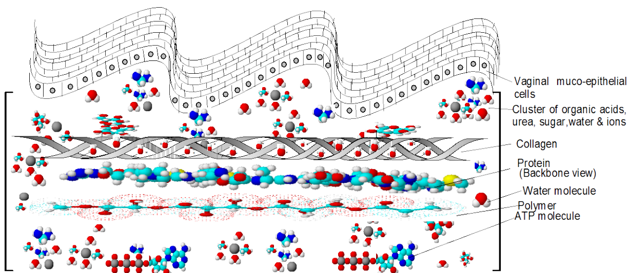
Figure 5.8: A chemometric structural model developed in our laboratories depicting caplet bioadhesion to freshly excised pig vaginal tissue with muco-epithelial cell secretions and surface bio-molecule interactions.
