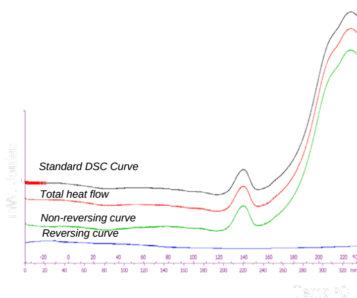
Figure 6.11: TMDSC thermogram for the unhydrated IBPD.
