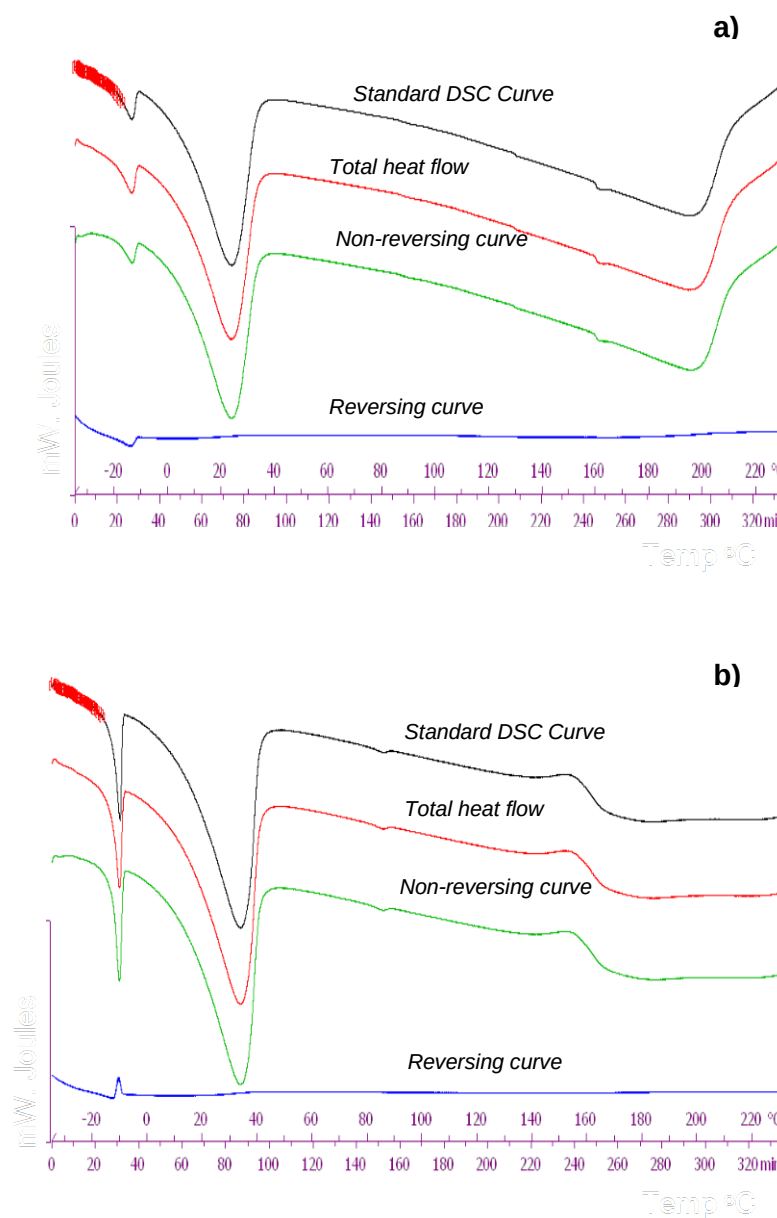
Figure 6.12: TMDSC thermogram for a) the hydrated physical polymer blend, b) the hydrated IBPD.
