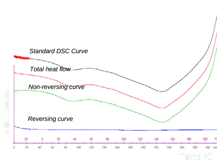
Figure 6.10: TMDSC thermogram for the unhydrated allyl penta erythritol-crosslinked poly(acrylic acid).
