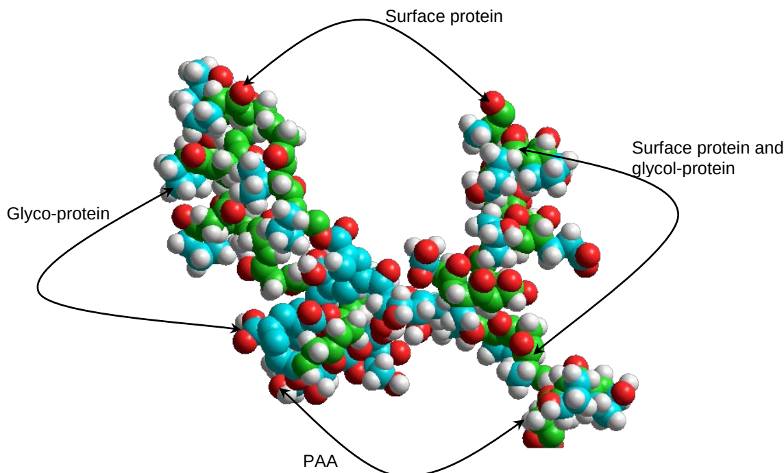
Figure 4.4: A chemometric structural model developed in our laboratories for a glyco-protein structure showing attachment of cellular surface protein (red) bound to the saccharide part of the glyco-protein (blue) and both (surface) protein and glyco-protein (green) bound to the polymer (here PAA) (white) for non-evenly distributed applied force during adhesion, with non-smooth and unevenly contacted two interacting surfaces with non-evenly distributed and non-constant, non-steadily (applied) force for the adhesion shown in a 3D optimized state with ball model. The coiling loop distortions for both protein and glycoprotein are also shown.
