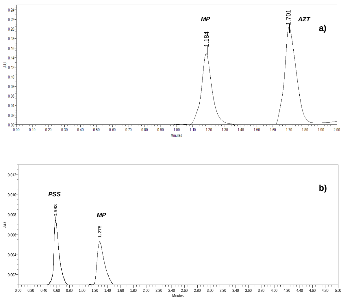
Figure 7.4: UPLC chromatograms depicting the retention times for the standard solutions of a) AZT, b) PSS and MP as an internal standard in blank plasma.
