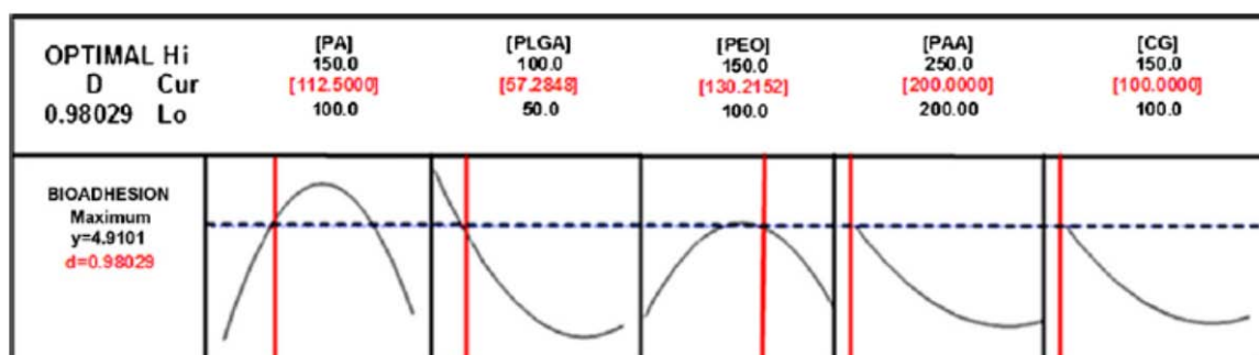
Figure 5.4: A typical response optimization plot for the AS-PAA and APE-PAA caplets.
