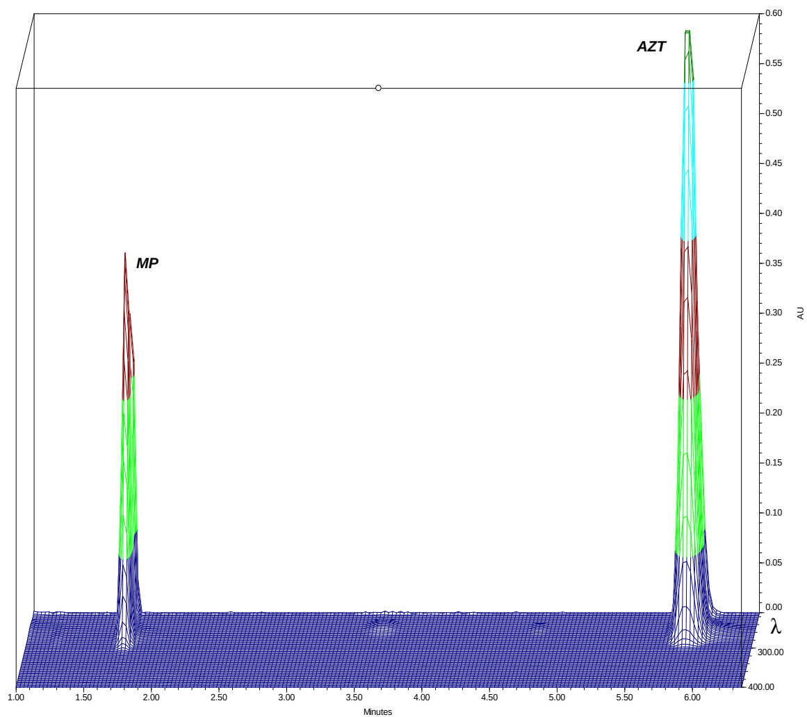
Figure 6.14: A typical 3D UPLC profile showing a complete separation between AZT and MP (internal standard).
