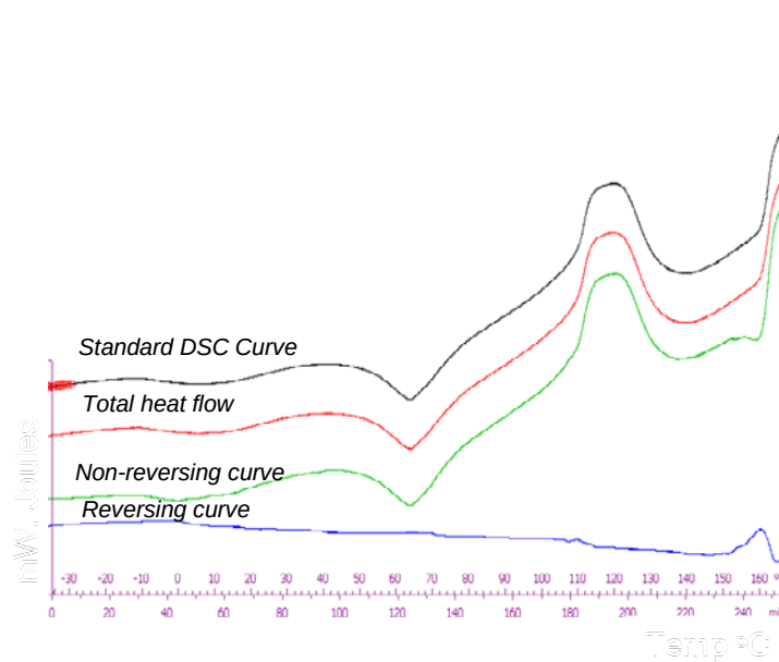
Figure 6.7: TMDSC thermogram for the unhydrated polyamide 6,10 (PA 6,10).
