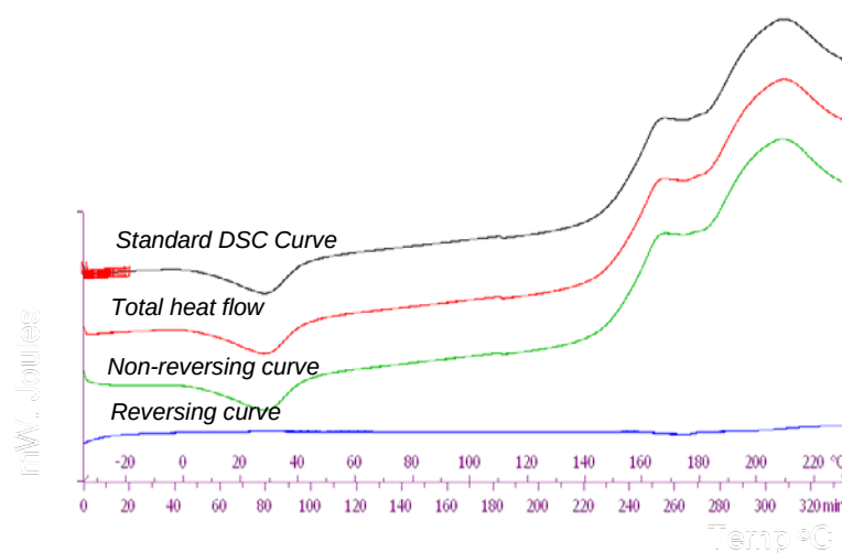
Figure 6.9: TMDSC thermogram for the unhydrated polyvinyl alcohol.
