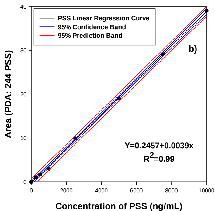
Figure 6.2: a) Calibration curves for: a) AZT in simulated vaginal fluid 267nm (N=3, SD<0.001 in all cases); b) PSS in simulated vaginal fluid 244nm (N=3, SD<0.003 in all cases).
