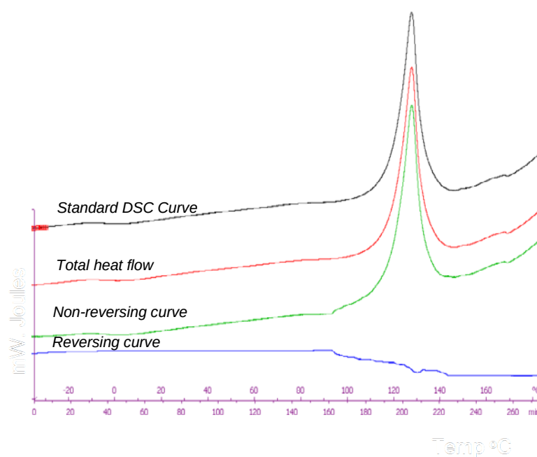
Figure 6.6: TMDSC thermogram for the unhydrated ethylcellulose.
