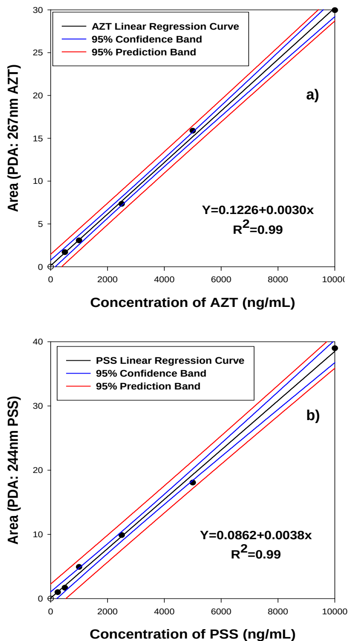
Figure 6.4: a) Calibration curves for: a) AZT in simulated plasma fluid 267nm (N=3, SD<0.001 in all cases); b) PSS in simulated plasma fluid 244nm (N=3, SD<0.003 in all cases).
