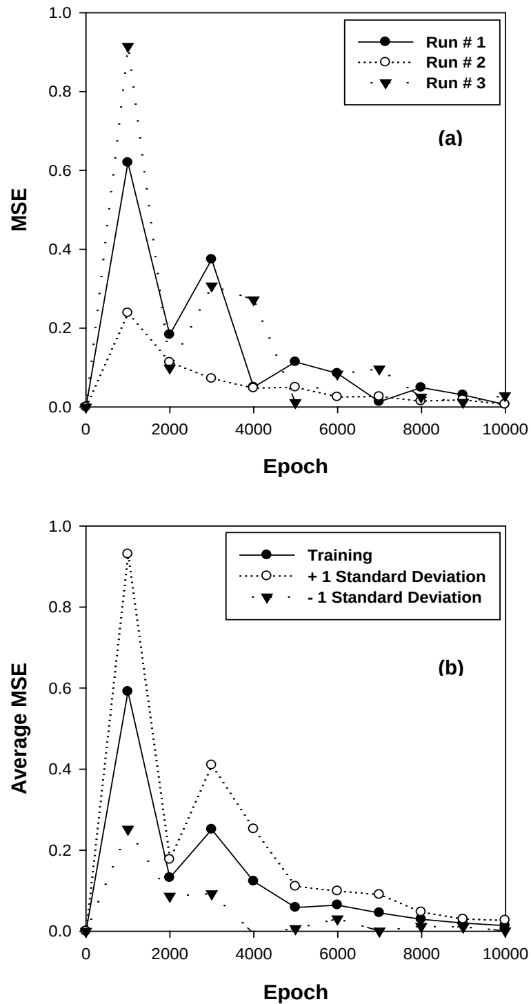
Figure 4.8: a) MSE for the secondary ANN training, b) Average MSE for the secondary training with standard deviations for 10,000 epochs.
