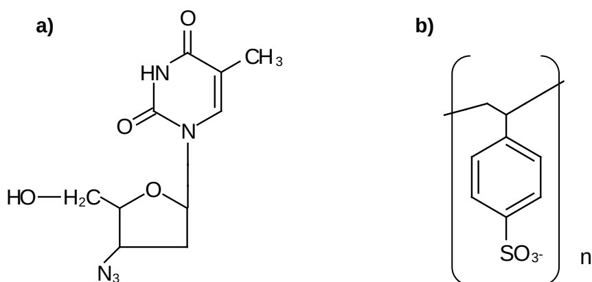
Figure 3.3: a) 3'-azido-3'-deoxythymidine (AZT), molecular weight 267.24 and a solubility 20.1 mg/mL, b) Polystyrene Sulfonate (PSS) molecular weight 70,000, water soluble.
