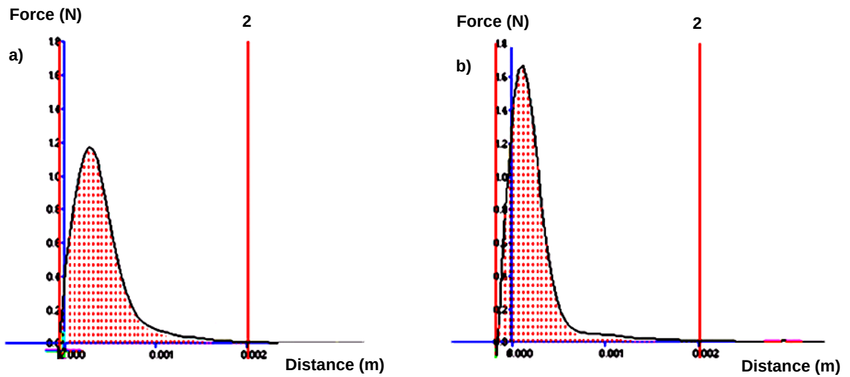
Figure 5.5: Typical textural profiles elucidating the peak adhesive force (PAF) (N) and work of adhesion ( \text{AUC}_{\text{FD}} ) (J) for the optimized composed of: a) AS-PAA, and b) APE-PAA.
