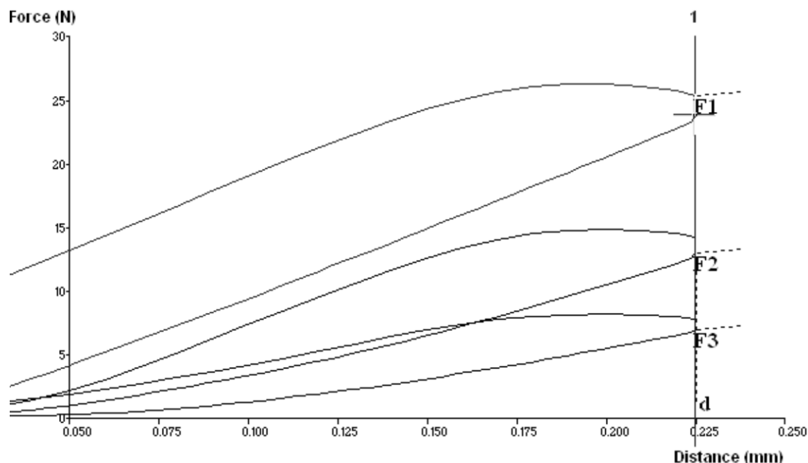
Figure 4.1: Typical force-distance profiles employed in the determination of matrix indentation hardness of the IBPD.
