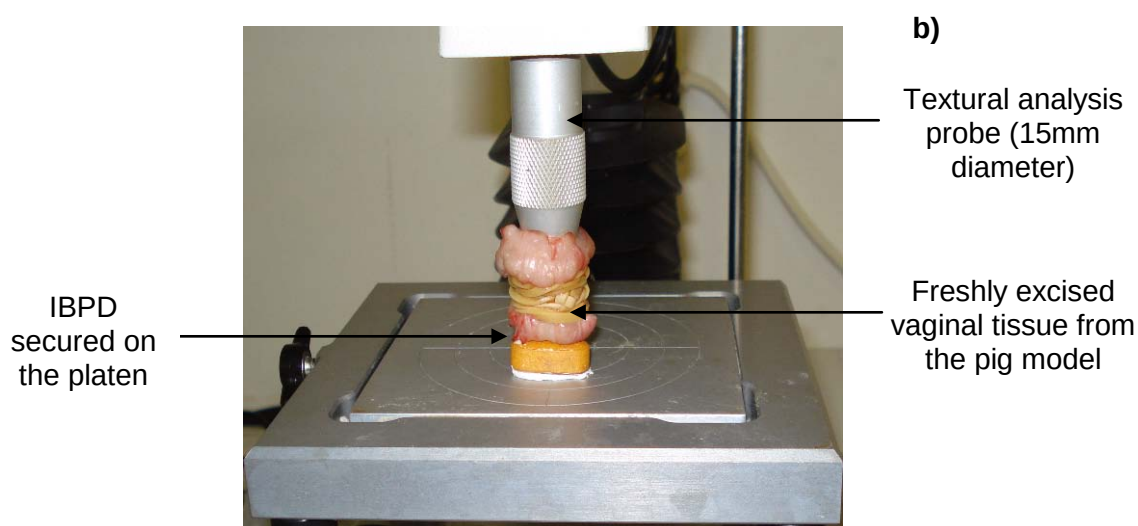
Figure 5.2: Textural analysis method employed to generate Force-Distance profiles for assessing the caplet bioadhesivity to freshly excised pig vaginal tissue indicating a) blue paint design, b) actual process.
