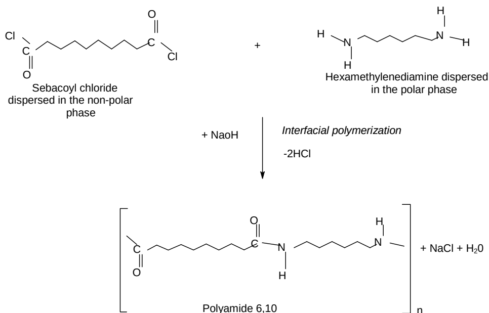
Figure 3.2: Synthesis of modified polyamide 6,10 by interfacial polymerization.
