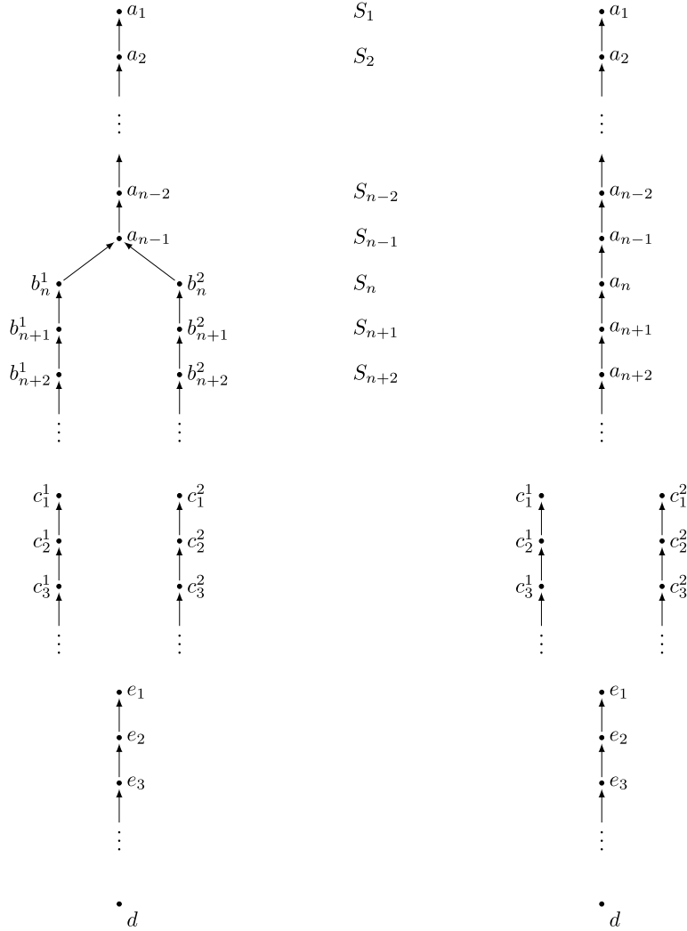
Fig. 1. Frames \mathfrak{F}_n^2 (left) and \mathfrak{F}_\omega^2 (right).
