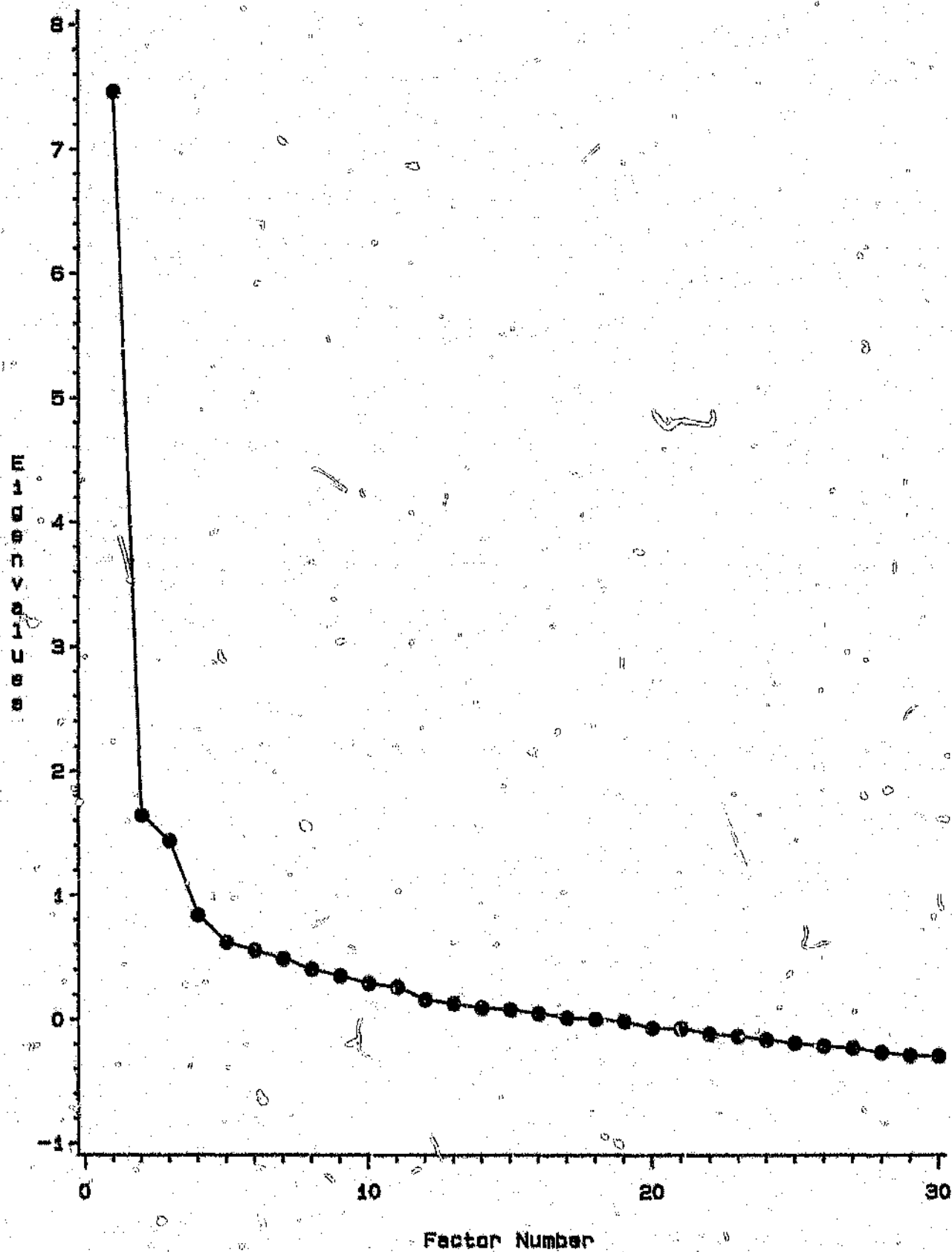
Figure 13: Scree plot of eigenvalues
