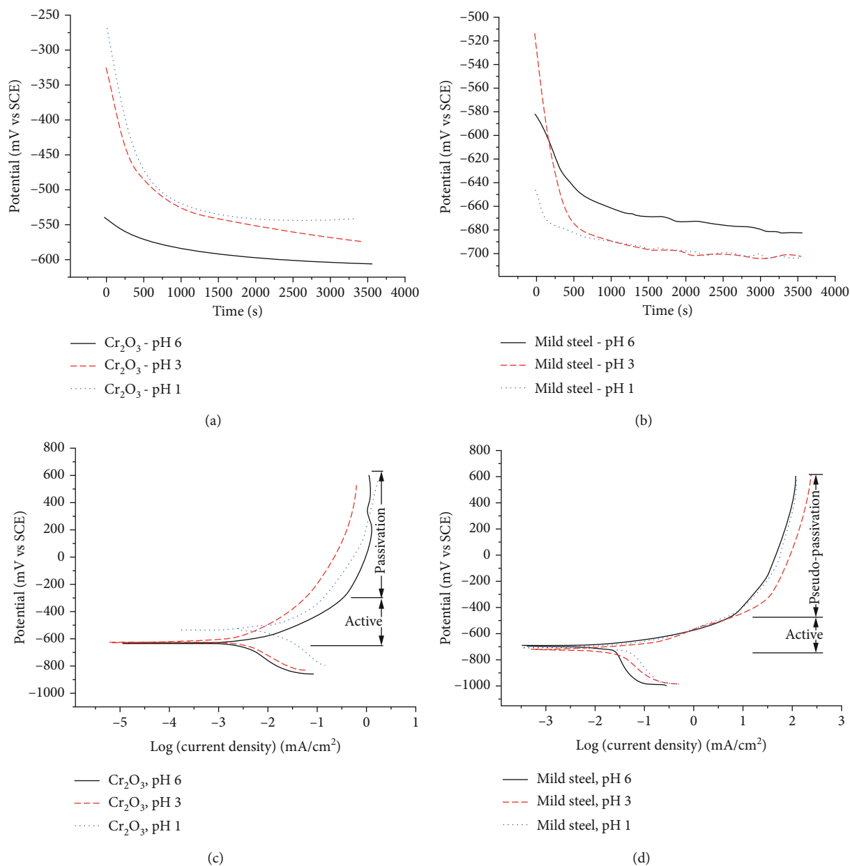
FIGURE 5: Open circuit potentials of (a) \text{Cr}_2\text{O}_3 coating and (b) mild steel substrate and potentiodynamic polarisation responses for (c) \text{Cr}_2\text{O}_3 coating and (d) mild steel substrate in synthetic mine water at pH 6, 3, and 1 [26].
