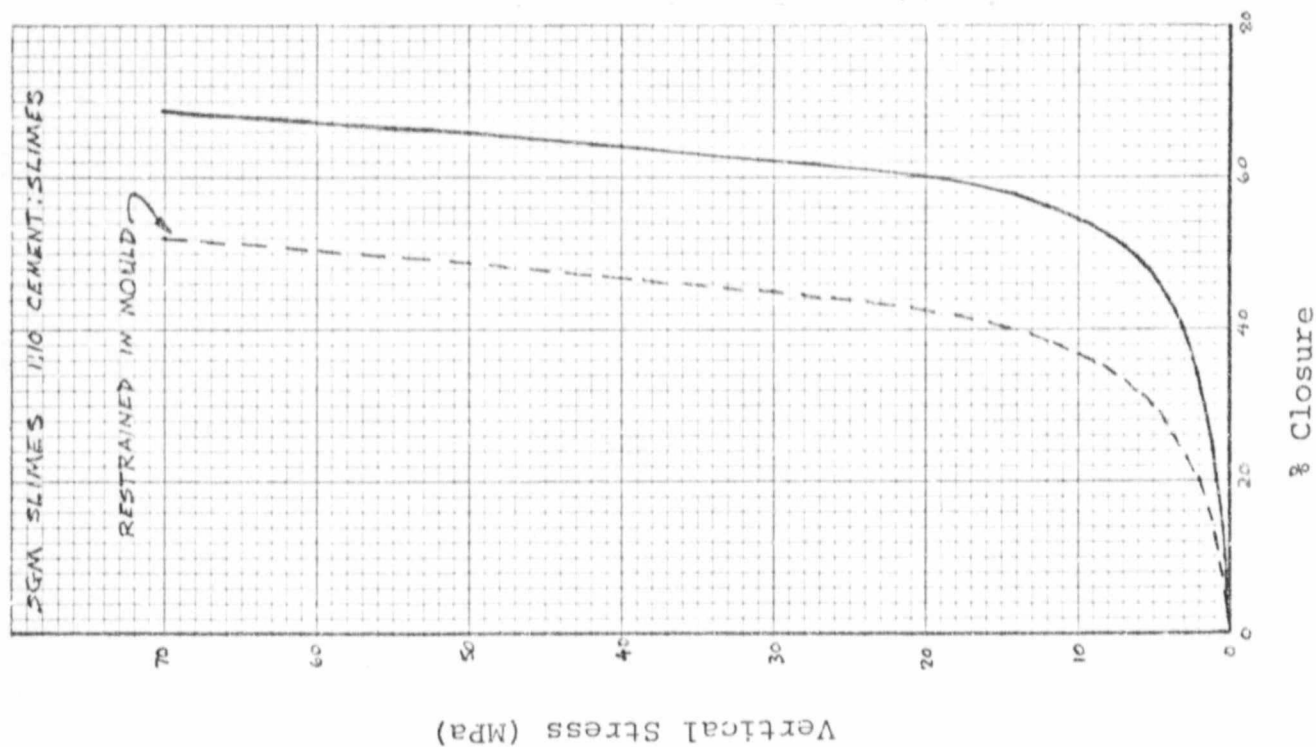
Fig. 25a Stress-Strain Curve
