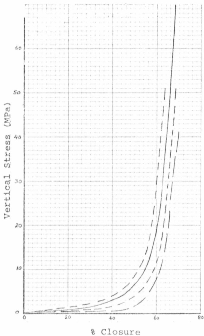
Fig. 17 Stress-Strain Curves for SGM Slimes with Cement, Lime-Flyash and Gypsum-Lime-Flyash
