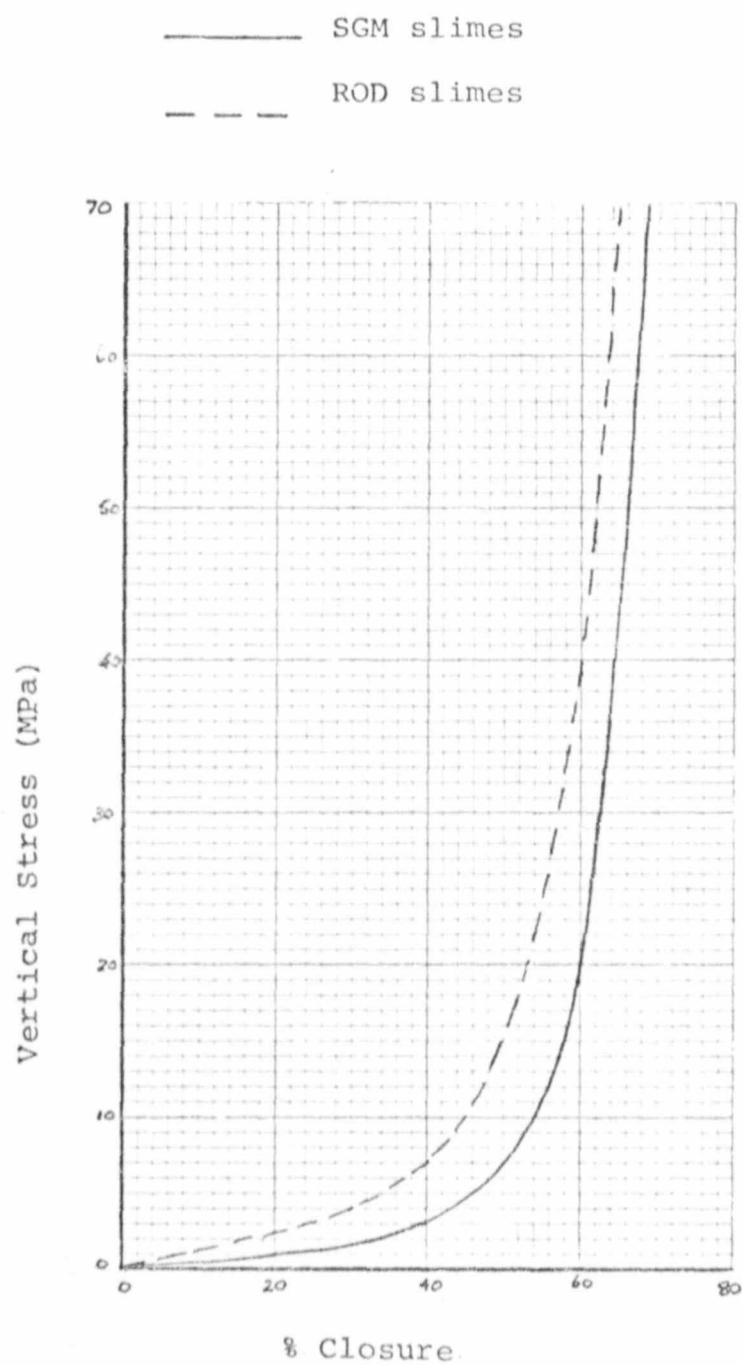
Fig. 18 Stress-Strain Curves for SGM and ROD slimes with Cement (1:10 Cement:Slimes Ratio)
