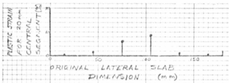
Fig. 23c Central plastic strain of wires across section B-B after loading to 80 MPa
