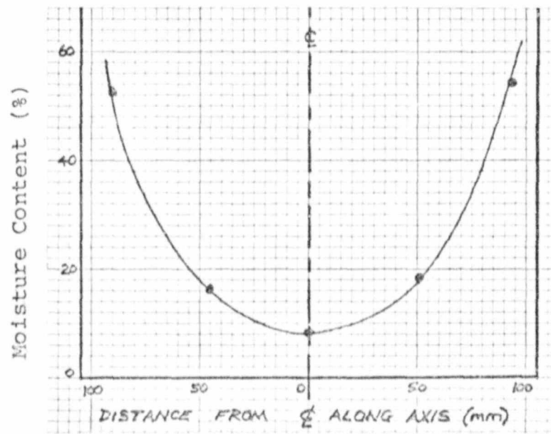
Fig. 20 Typical Moisture Content Profile (after loading to about 70 MPa)
