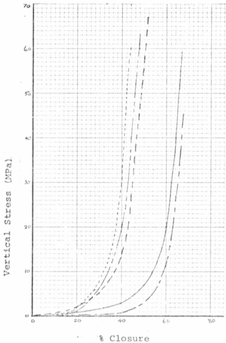
Fig. 26 Effect of Mould-Restraint and Cementing Agent on Strength Development
