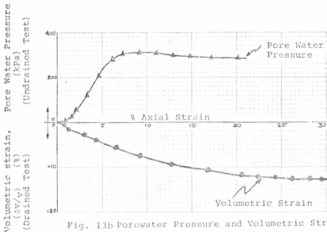
Fig. 13 Typical Curves for Drained and Undrained Triaxial Tests on SGM slimes
