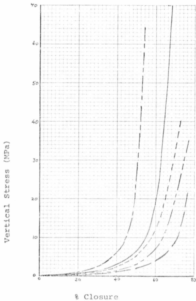
Fig. 16 Stress-strain Curves for SGM slimes with Cement and Cement-Flyash
