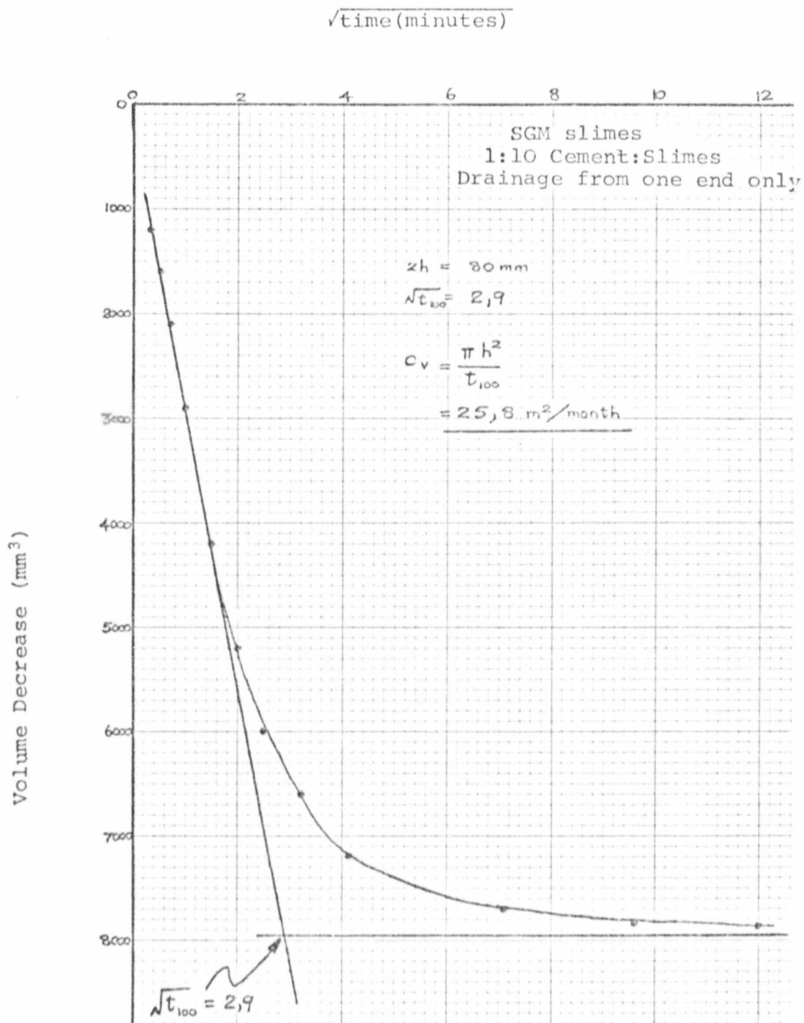
Fig. 12 Typical Curve and Calculation for Coefficient of Consolidation
