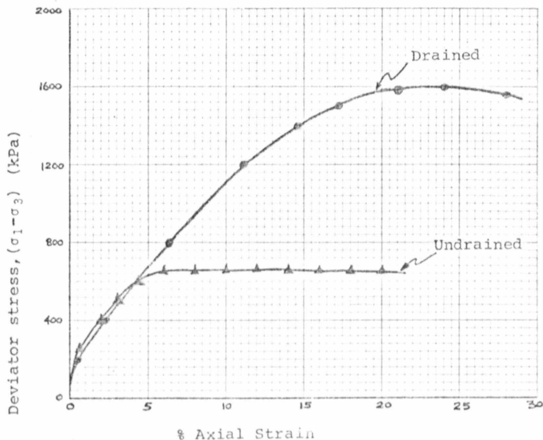
Fig. 13a Stress-Strain Curves
