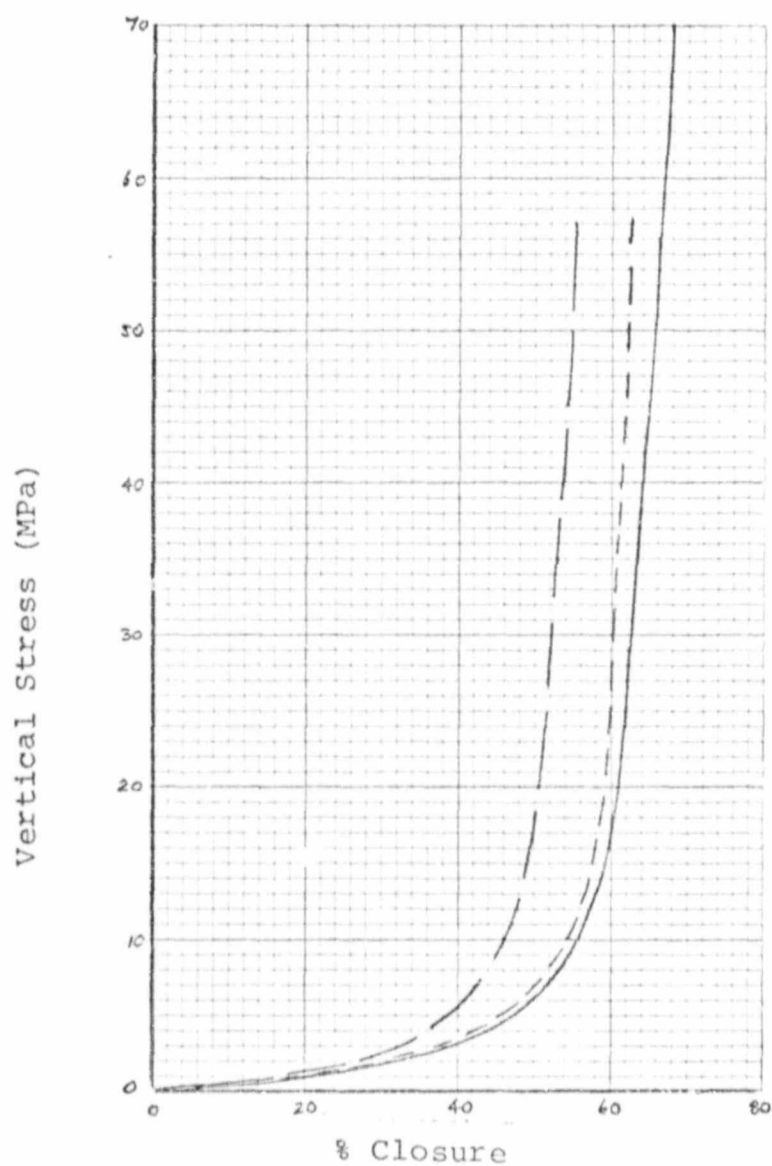
Fig. 19 Effect of Moisture Content Reduction on Strength Development (SGM Slimes)
