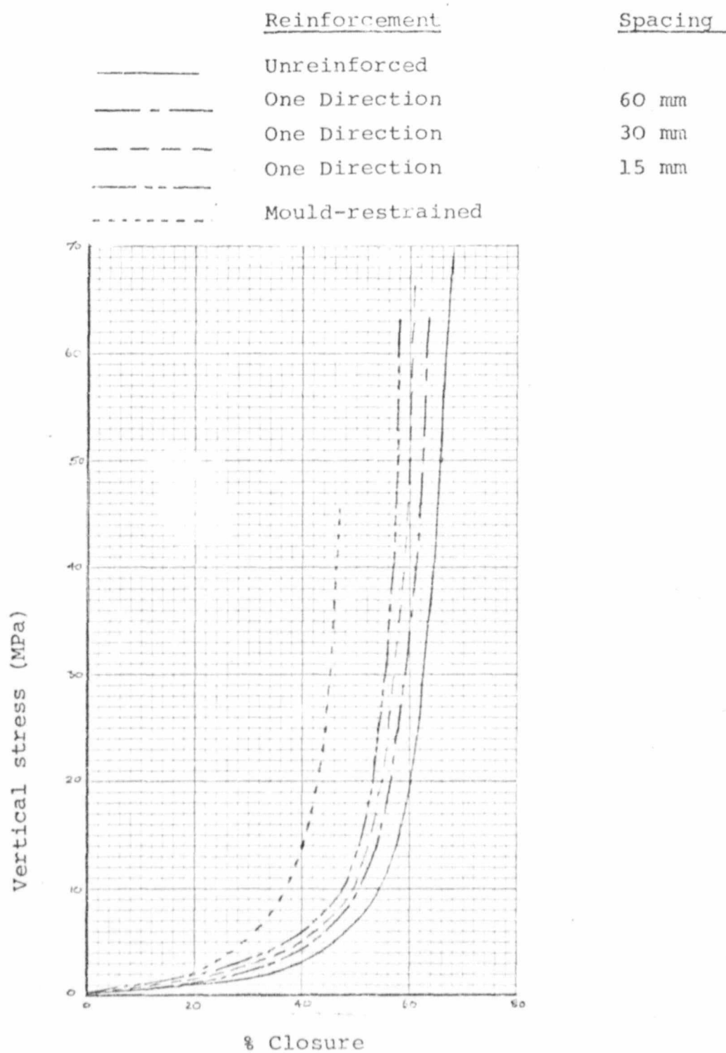
Fig. 22 Effect of Reinforcement Spacing on Strength Development (SGM slimes, 1:10 cement:slimes)
