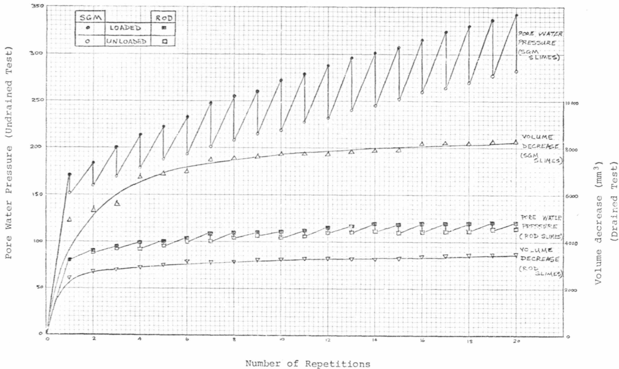
Fig. 30 Pore Water Pressure and Volume Decrease Curves during Cyclic Loading (1:10 Cement:slimes ratio, 7-11 days curing period, Cell Pressure = 493 kPa, Consolidation Pore Pressure = Atmospheric)
