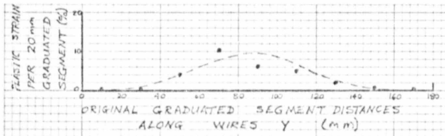
Fig. 23b Average plastic strain along wires Y after loading to 80 MPa
