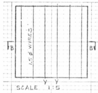
Fig. 23a Plan on Slab
