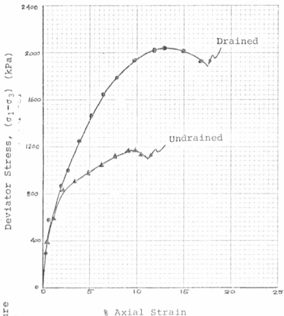
Fig. 14a Stress-strain curves
