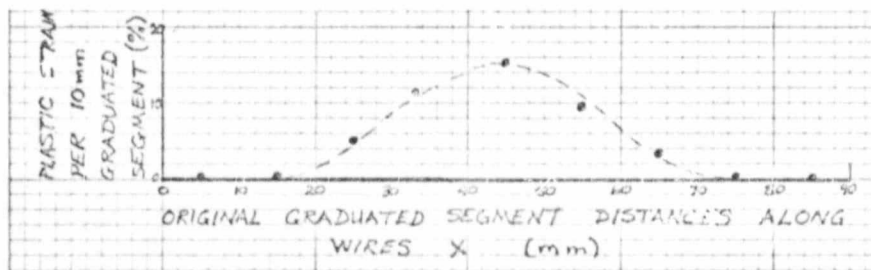
Fig. 24b Average plastic strain along wires X after loading to 80 MPa
