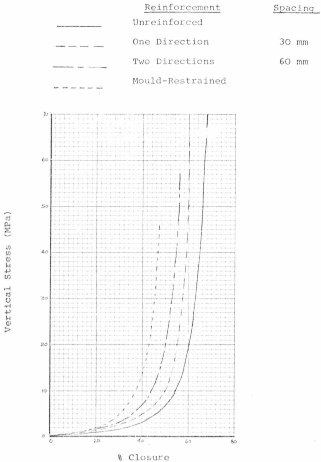
Fig. 21 Effect of One-and Two-Directional Reinforcement on Strength Development
