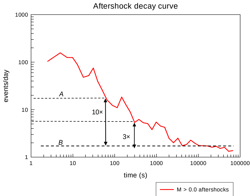
Figure 6.12: Determination of time periods where the event rate has decreased to background levels.
