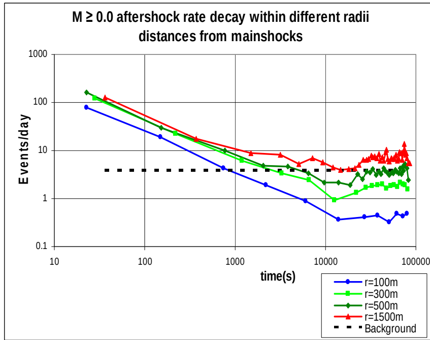
Figure 6.7: M \geq 0.0 aftershock rate decay within different radial distances from M \geq 1.0 mainshocks. The line representing the estimated background level is also shown.
