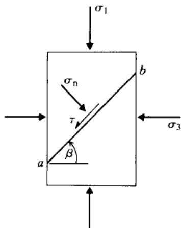
Figure 2.2: Shear failure along a plane due to the applied stresses.
