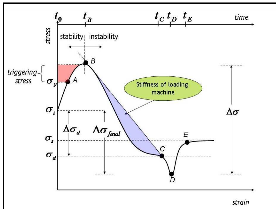
Figure 2.4: Stress-strain behaviour of a rock sample.
