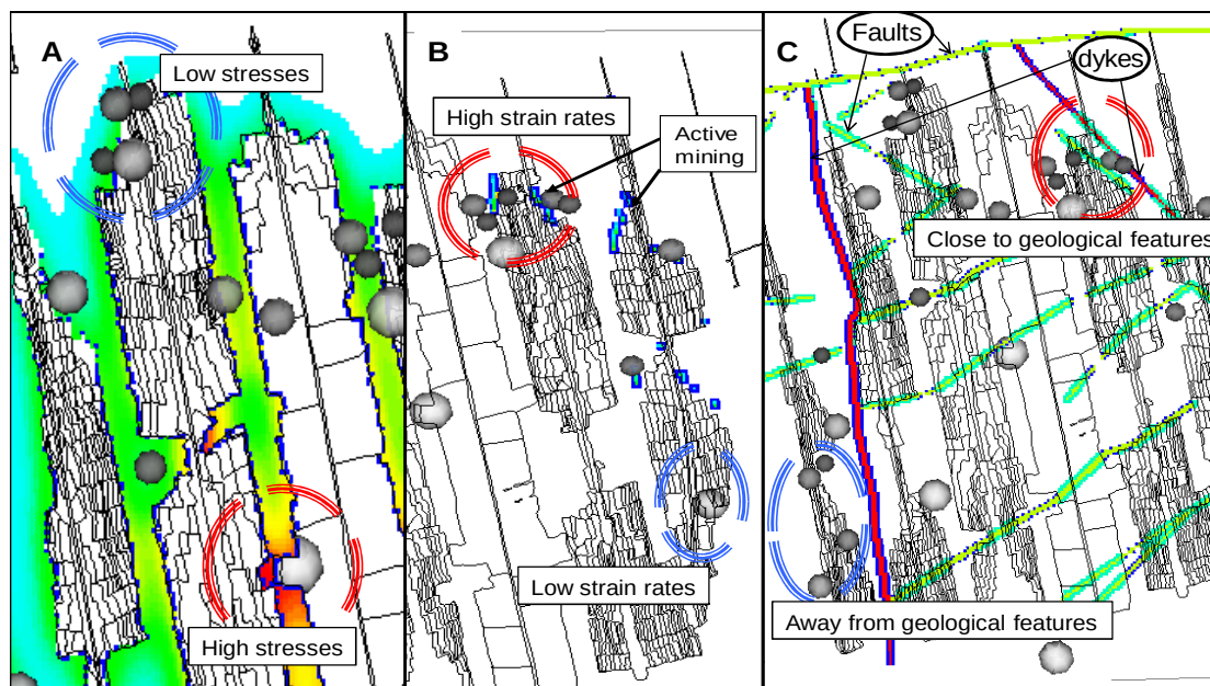
Figure 9.2: Subsets defining three mining conditions. (A) Stress influence (red and blue colour represent high and low stress conditions respectively), (B) Strain rate influence (blue colour represent active mining) and (C) Geological discontinuity influence.
