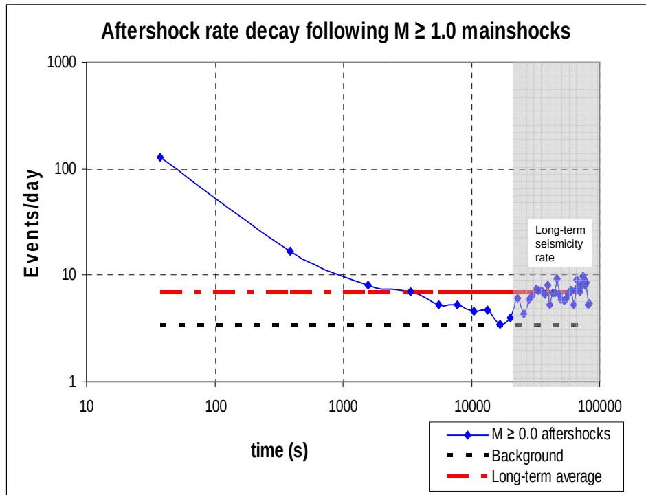
Figure 6.2: Estimation of the background rate. Long-term average determined by averaging over long-term seismicity (shaded area).
