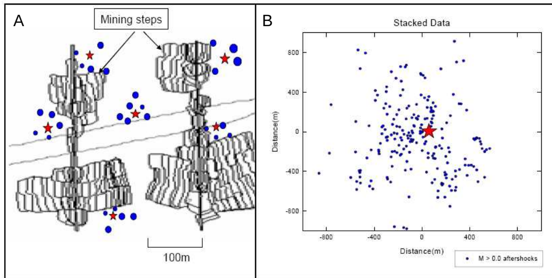
Figure 3.2: Stacking of different mainshock-aftershock sequences.
