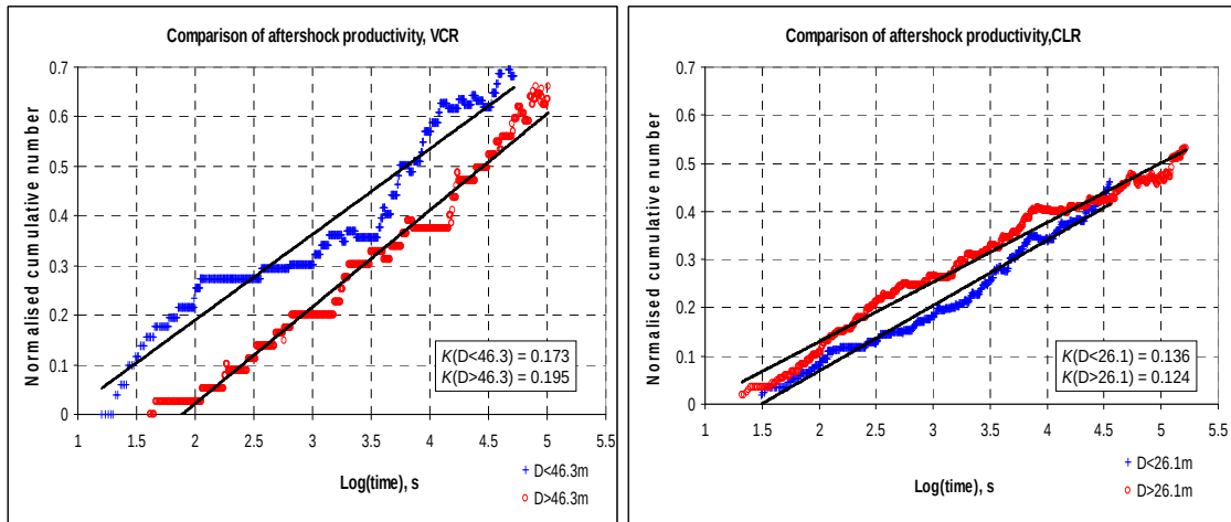
Figure 9.7: Aftershock productivity dependency on geological discontinuities.
