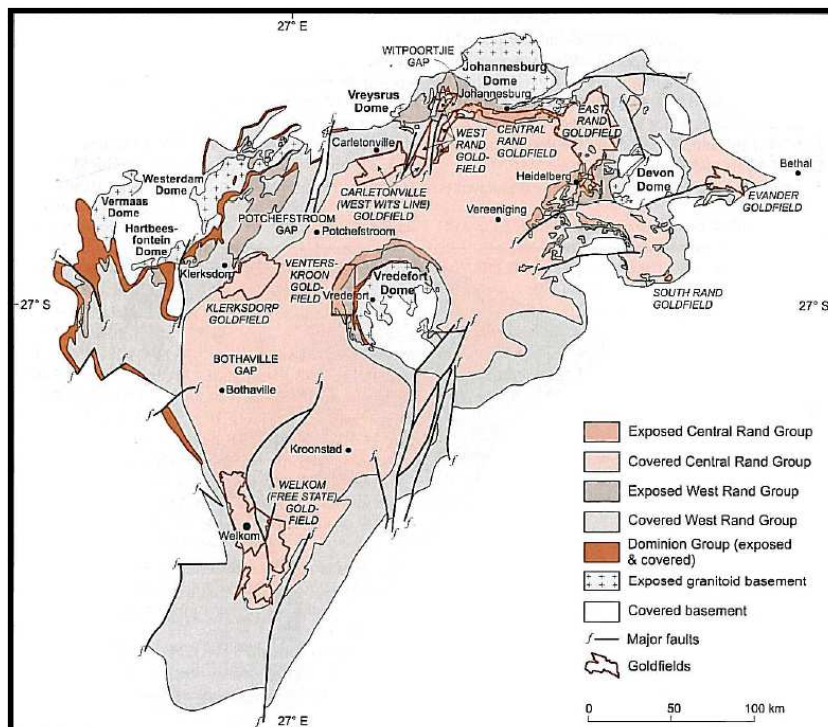
Figure 2.5: The geology of the Witwatersrand basin.
