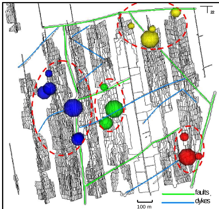
Figure 3.1: Aftershock-mainshock sequences showing the typical small number of aftershocks following each mainshock.
