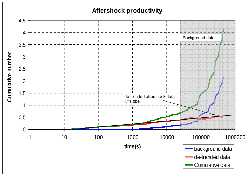
Figure 9.5: Aftershock productivity within 1000 m and 1 day following M \geq 2.0 mainshocks.
