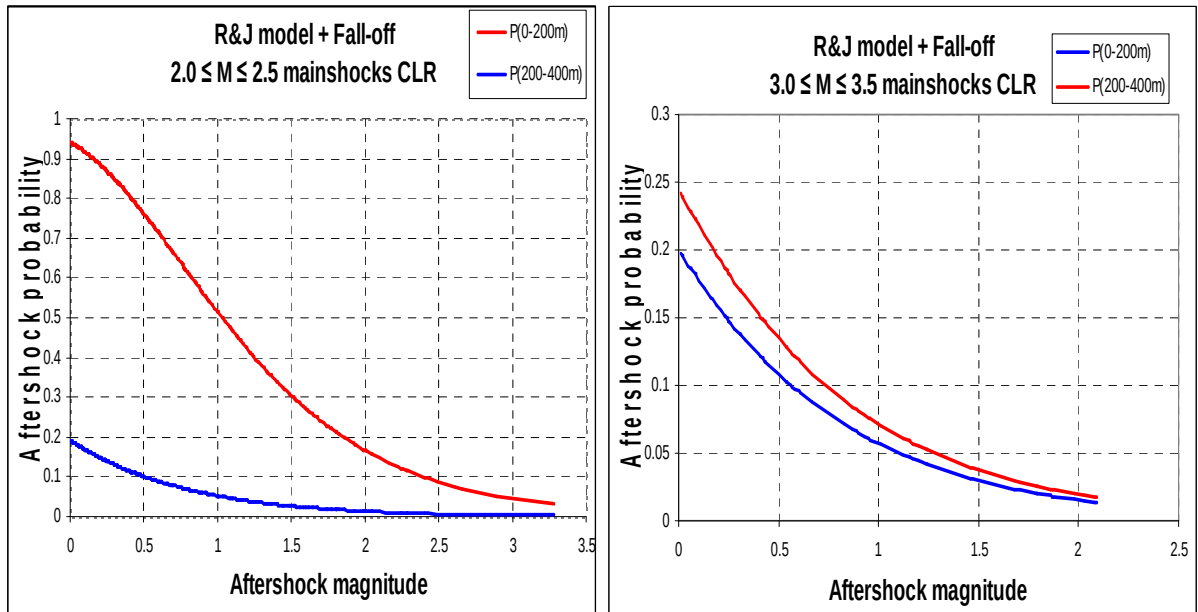
Figure 8.2: M \geq 0.0 Aftershock probabilities for CLR mine within 1 day following, (a) 2.0 \leq M \leq 2.5 mainshocks and (b) 3.0 \leq M \leq 3.5 mainshocks.
