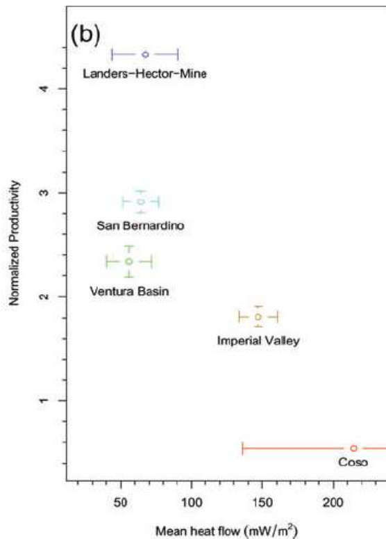
Figure 9.1: Dependency of aftershock productivity on mean heat flow for 5 regions in Southern California.
