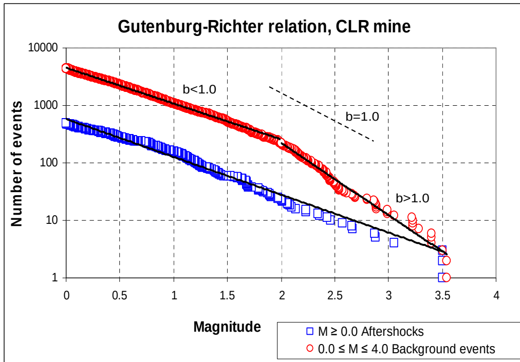
Figure 4.2: Gutenberg-Richter frequency-magnitude relation of aftershock and background seismicity at the CLR mine.
