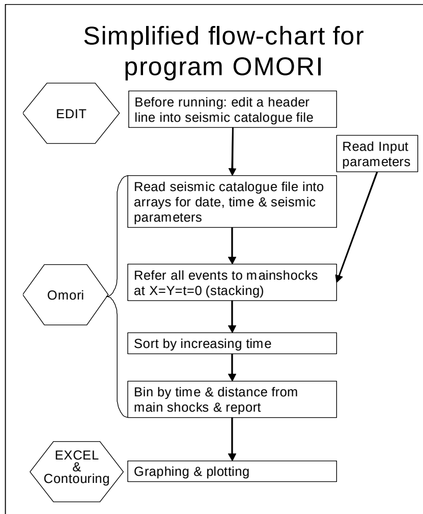
Figure 3.3: A simplified flow chart for the program Omori.
