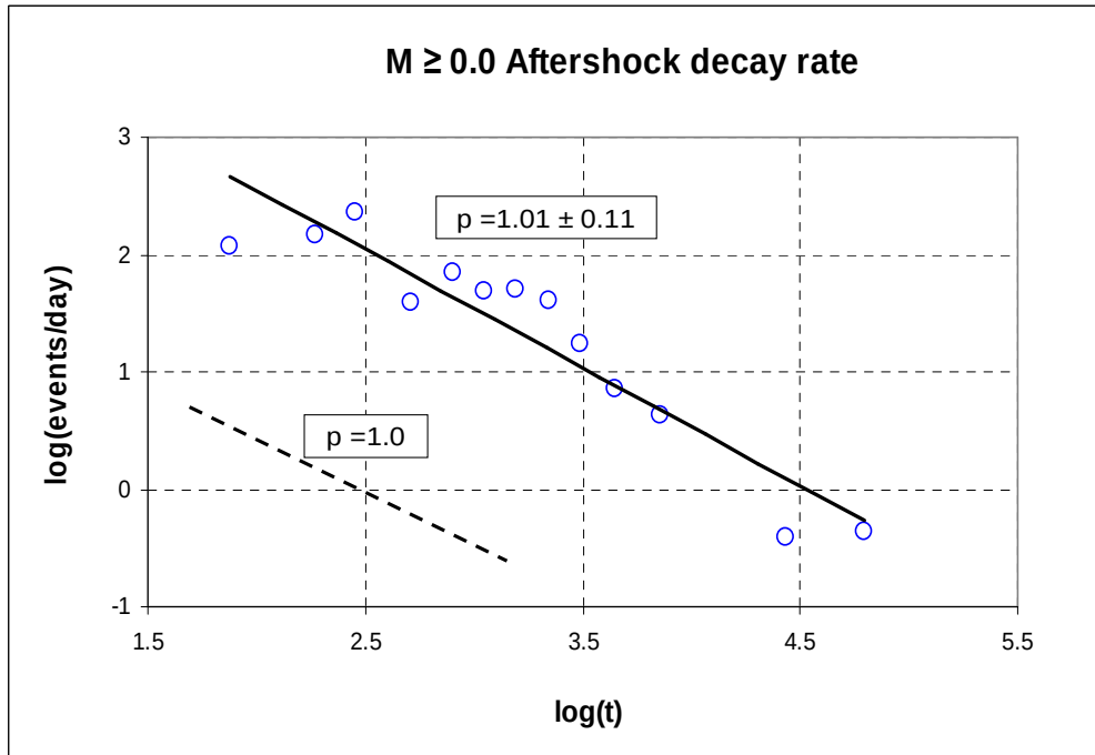
Figure 9.4: M \geq 0.0 aftershock decay rate following 2.0 \leq M \leq 3.0 mainshocks.
