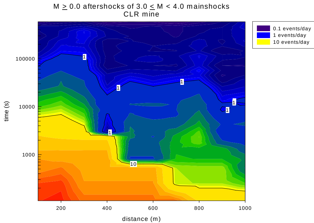
Figure 6.11: Event rate contour plots as a function of time and distance from 3.0 \leq M \leq 4.0 mainshocks (CLR mine).
