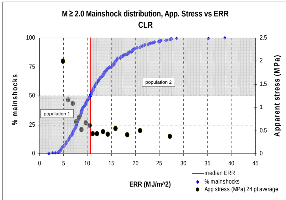
Figure 9.3: Division of mainshocks into two populations to study the influence of geological discontinuities on aftershock productivity.
