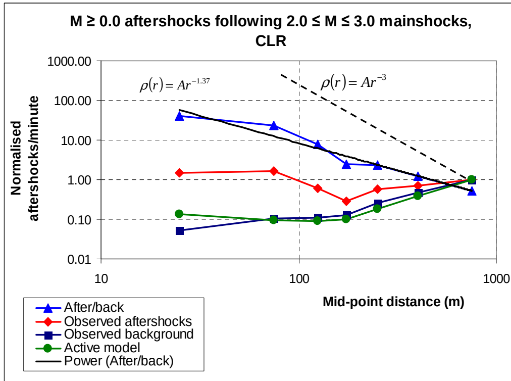
Figure 7.1: Aftershock density as a function of distance from the mainshock.
