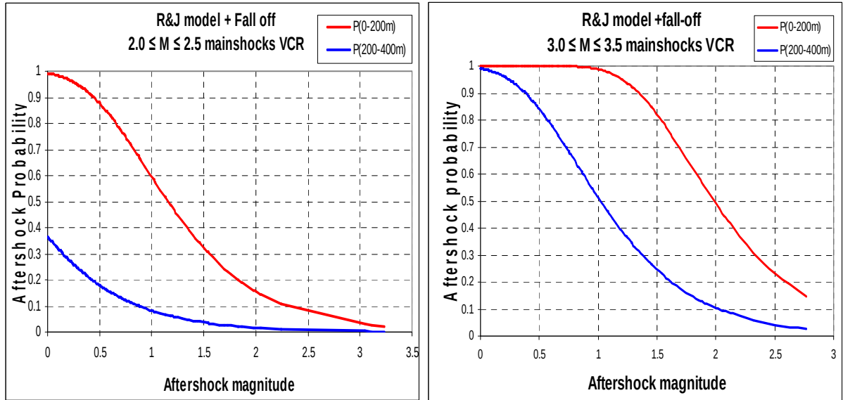
Figure 8.1: M \geq 0.0 Aftershock probabilities for VCR mine within 1 day following, (a) 2.0 \leq M \leq 2.5 mainshocks and (b) 3.0 \leq M \leq 3.5 mainshocks) 2.0 \leq M \leq 2.5 mainshocks and (b) 3.0 \leq M \leq 3.5 mainshocks..
