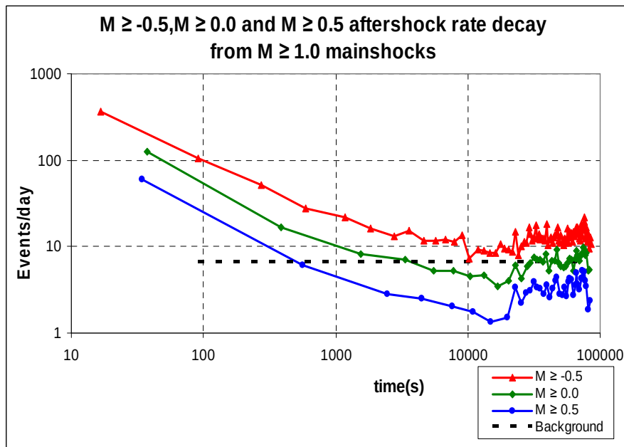
Figure 6.6: M \geq -0.5 , M \geq 0.0 and M \geq 0.5 aftershock rate decay following mainshocks with magnitude M \geq 1.0 . The line representing the estimated background level is also shown.
