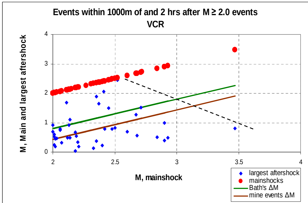
Figure 5.1: Bath's law analysis of M \geq 0.0 aftershocks within 1000 m of and 2 hour following 163 M \geq 2.0 mainshocks (VCR mine).
