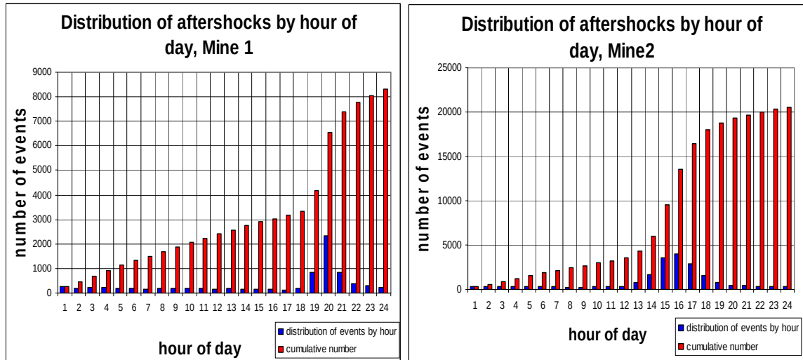
Figure 3.4: Distribution of M_L \geq 0.0 aftershocks by hour of day within 1000 m of the mainshock epicentre.
