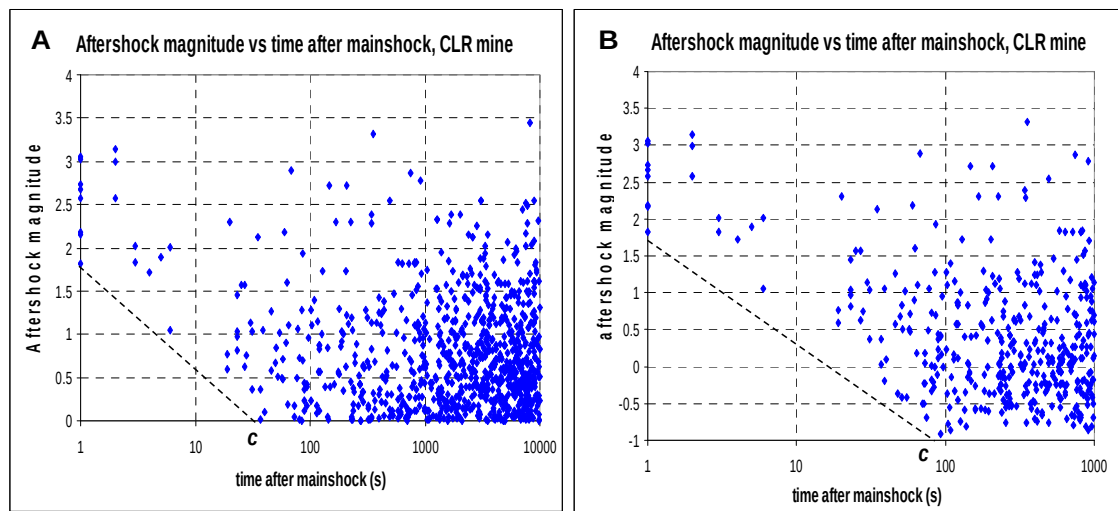
Figure 6.3: Time-magnitude distribution of aftershocks (CLR mine).
