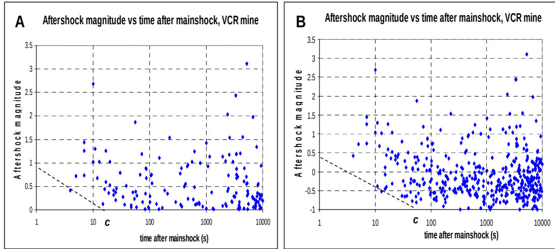
Figure 6.4: Time-magnitude distribution of aftershocks (VCR mine).
