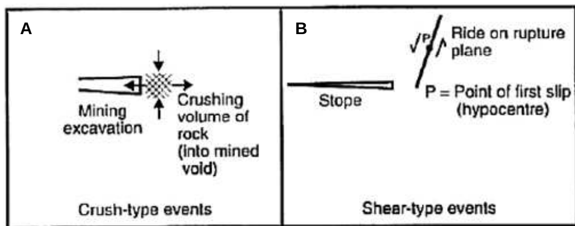
Figure 2.1: Simplified events mechanisms encountered in mining environments (section views).
