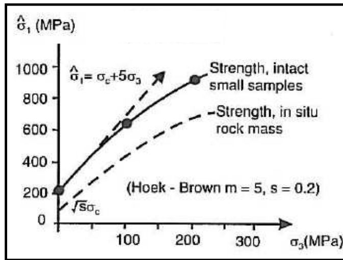
Figure 2.3: Strength behaviour of a rock sample.
