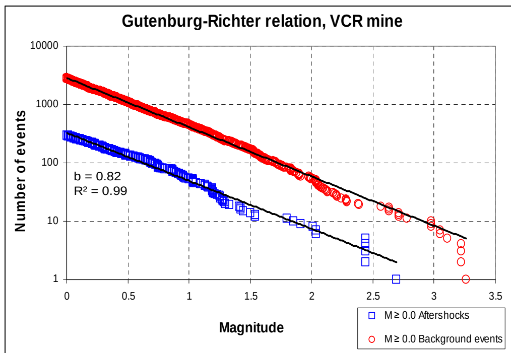
Figure 4.1: Gutenberg-Richter frequency-magnitude relation of aftershock and background seismicity at the VCR mine.
