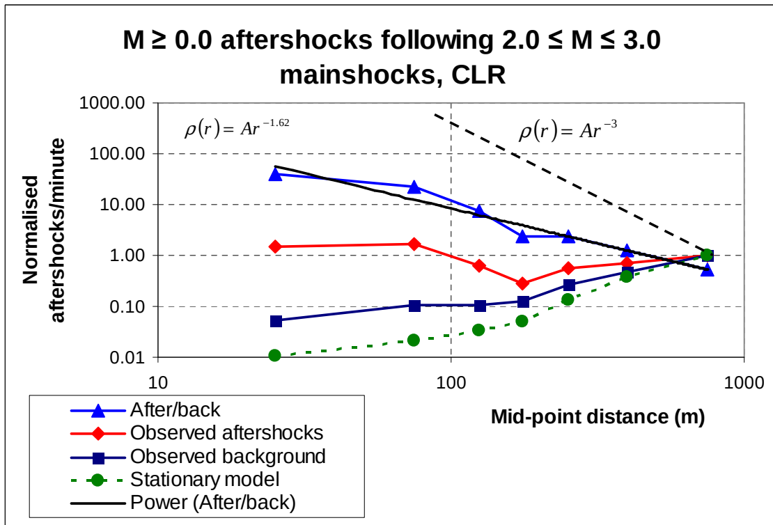
Figure 7.2: Aftershock density as a function of distance from the mainshock.
