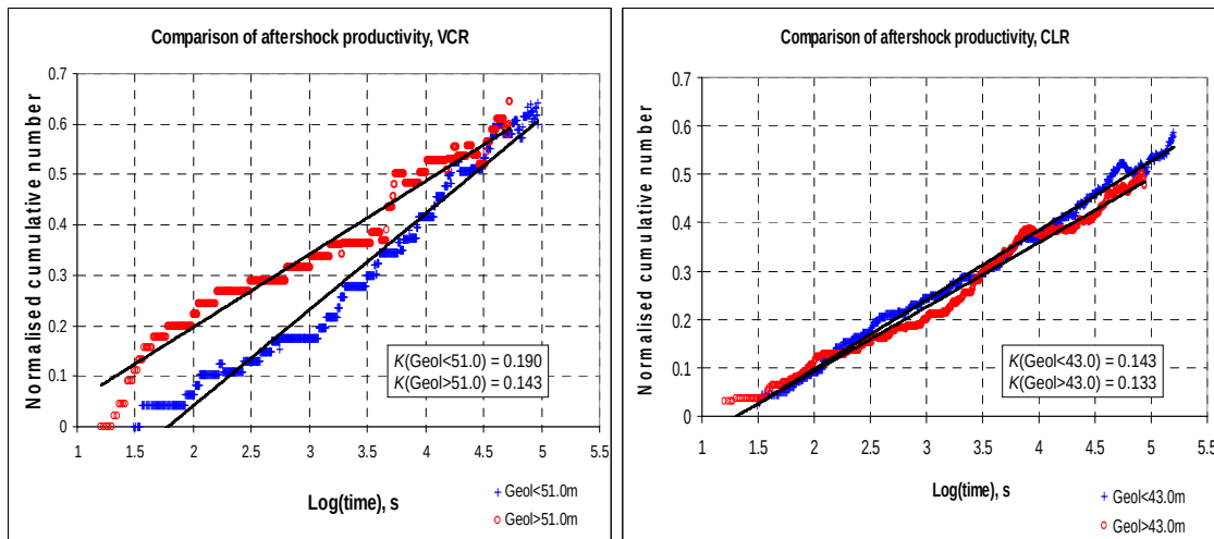
Figure 9.8: Aftershock productivity dependency on strain environments.
