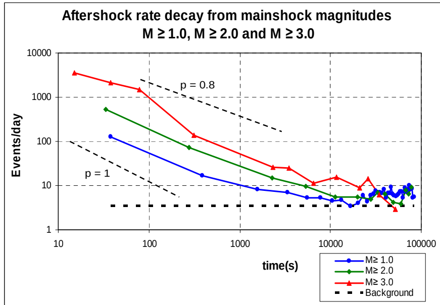
Figure 6.5: M \geq 0.0 aftershock rate decay following mainshocks with threshold magnitudes M \geq 1.0 , M \geq 2.0 , and M \geq 3.0 . The lines representing p = 1 and the estimated background level are also shown.
