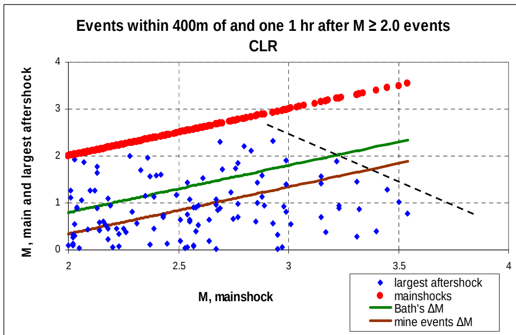
Figure 5.2: Bath's law analysis of M \geq 0.0 aftershocks within 400 m of and 1 hour following 517 M \geq 2.0 mainshocks (CLR mine).
