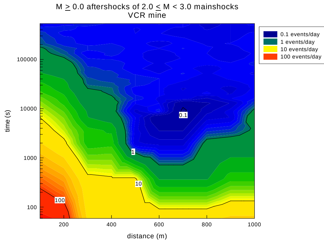
Figure 6.8: Event rate contour plots as a function of time and distance from 2.0 \leq M \leq 3.0 mainshocks (VCR mine).
