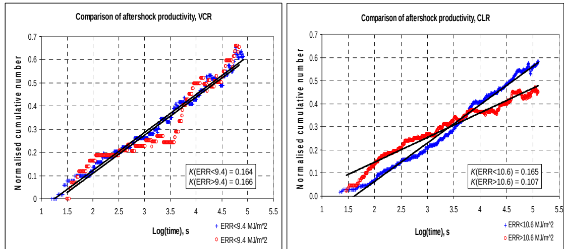
Figure 9.6: Aftershock productivity dependency on stress environments.
