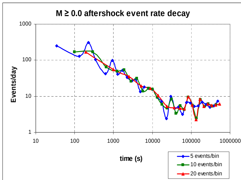
Figure 6.1: Effect of number of events per bin on the event rate decay curve.
