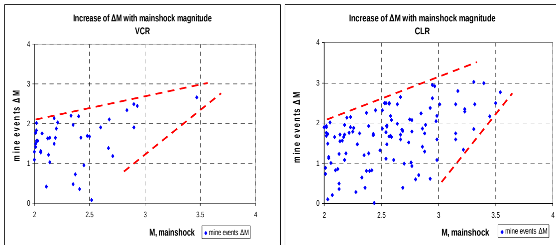
Figure 5.3: Increase of \Delta M with increasing mainshock magnitude.
