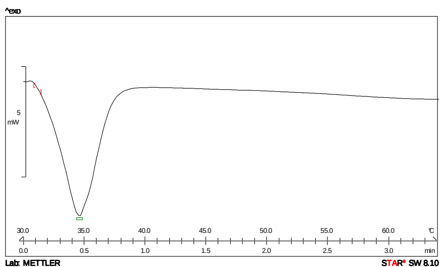
Figure 5.3. DSC profile for \text{CH}_3\text{CpFe(CO)}_2\text{I} + \text{PPh}_3 1: 1 ratio
