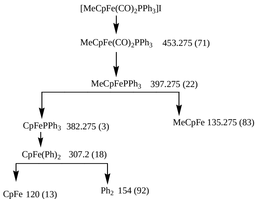
Scheme 5.2 Fragmentation patterns for [\text{CH}_3\text{CpFe(CO)}_2\text{PPh}_3]\text{I}
