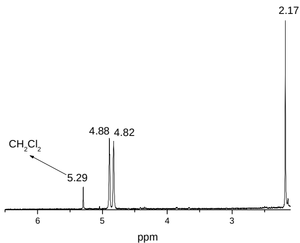
Figure 5.2. ^1\text{H} NMR spectrum of \text{CH}_3\text{CpFe(CO)}_2\text{I} + \text{PPh}_3 before heating
