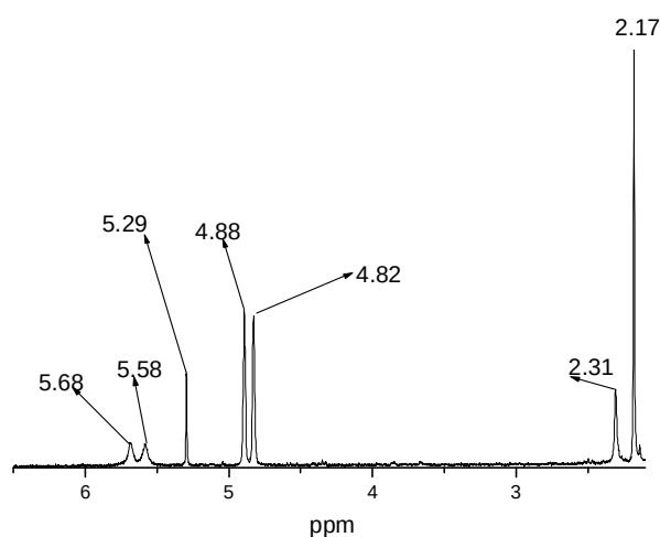
Figure 5.4. ^1\text{H} NMR spectrum of \text{CH}_3\text{CpFe(CO)}_2\text{I} + \text{PPh}_3 at 60^\circ\text{C} after 3 hours
