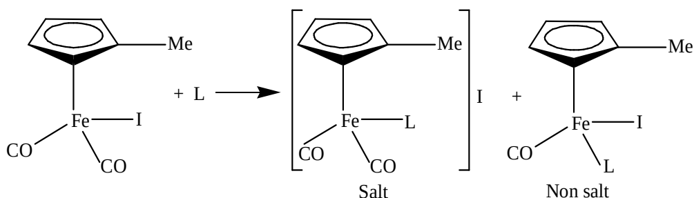
Scheme 5.1. Reaction between \text{MeCpFe(CO)}_2\text{I} and electron donor ligands.
