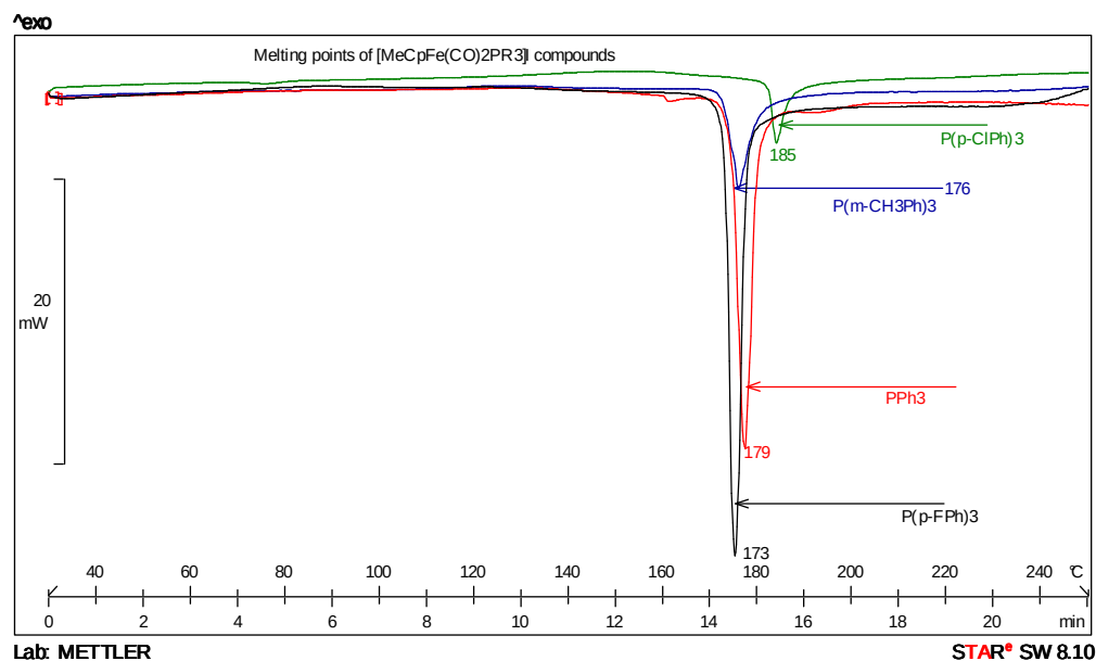
Figure 5.5. DSC profiles for [\text{CH}_3\text{CpFe(CO)}_2\text{PR}_3]\text{I} compounds
