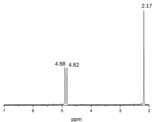
Figure 5.1. ^1\text{H} NMR spectrum of \text{CH}_3\text{CpFe(CO)}_2\text{I}
