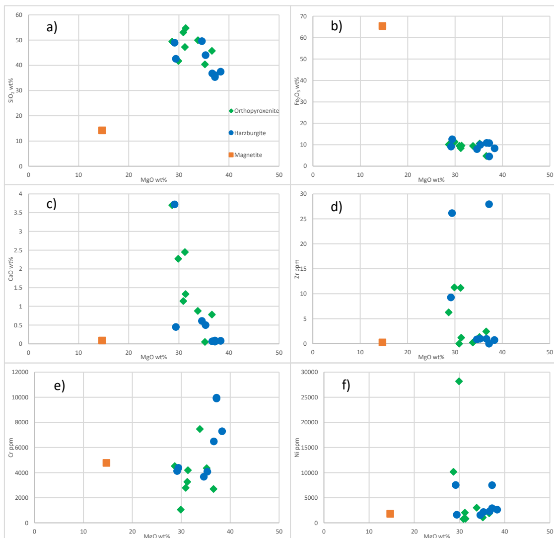
Figure 12: XRF compositional data of orthopyroxenite (green), harzburgite (blue) and magnetite vein (orange): a) SiO 2 vs MgO (wt%); b) Fe 2 O 3 vs MgO (wt%); c) CaO vs MgO (wt%); d) Zr ppm vs MgO wt%; e) Cr ppm vs MgO wt%; f) Ni ppm vs MgO wt%.
