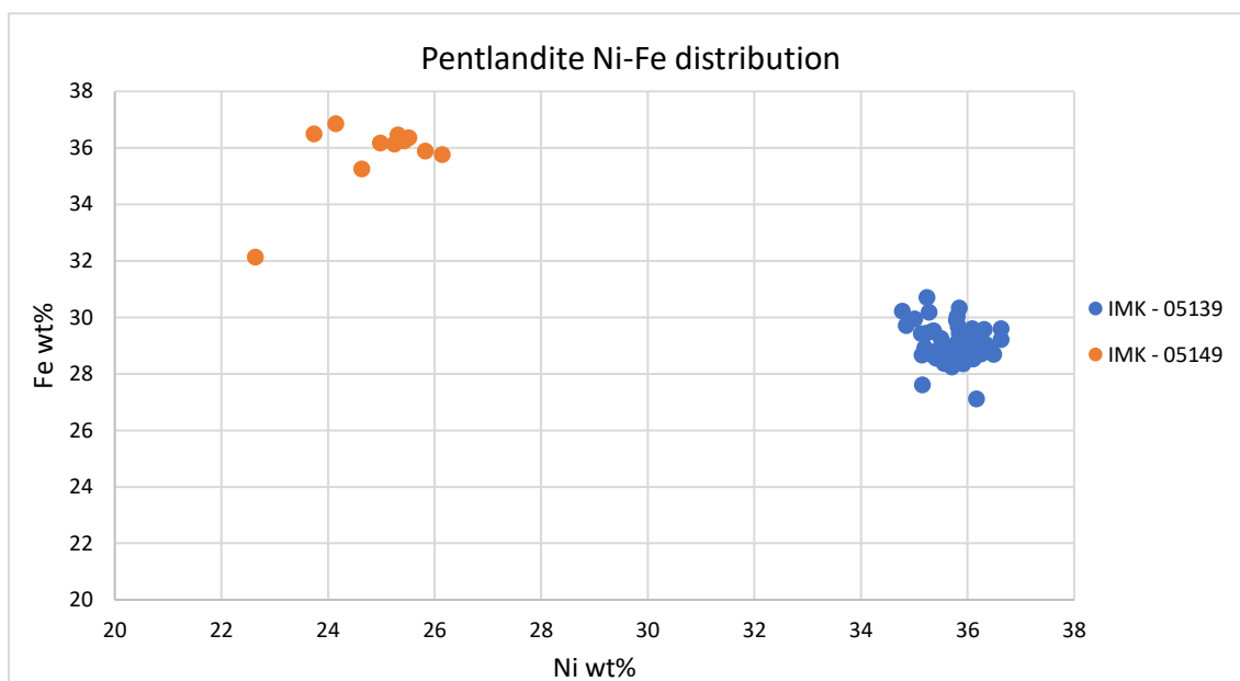
Figure 33: Ni-Fe (Ni wt% and Fe wt%) distribution in pentlandite from samples IMK – 05139 and IMK – 05149
