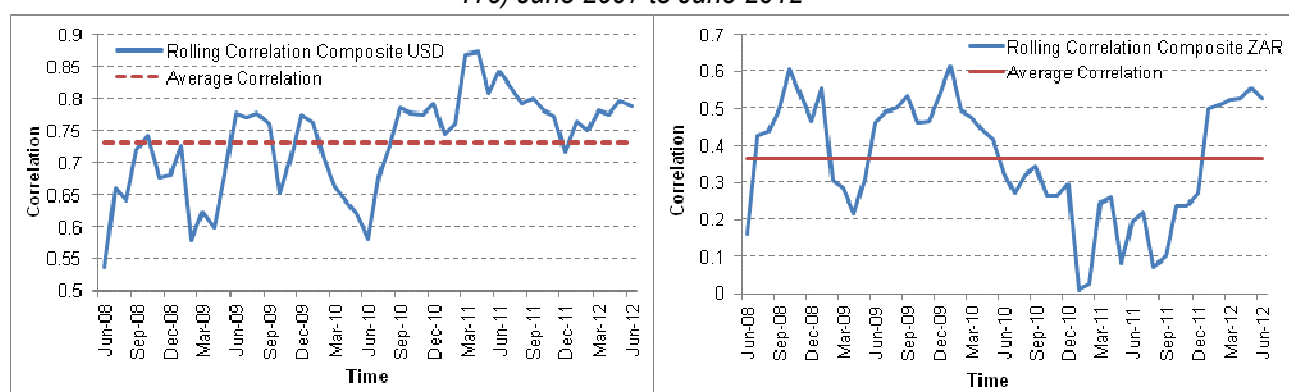
Figure 17: Rolling Correlations – Equities versus commodity indices
