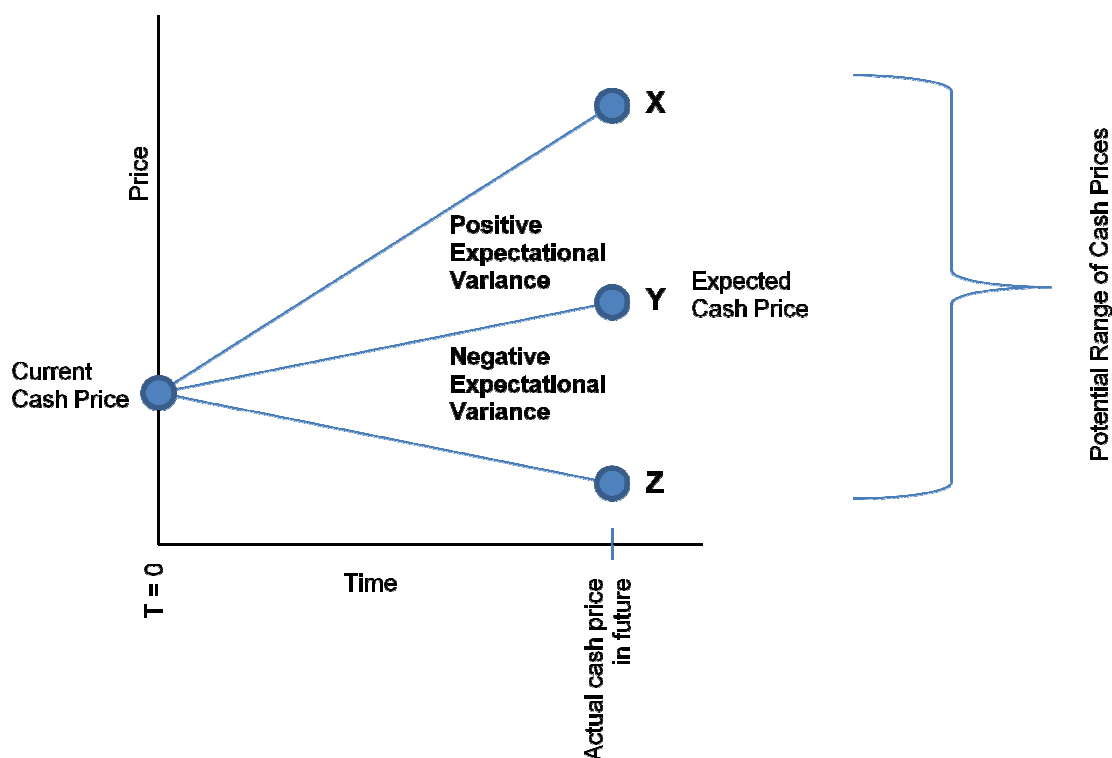
Figure 9: Expectational Variance 8
