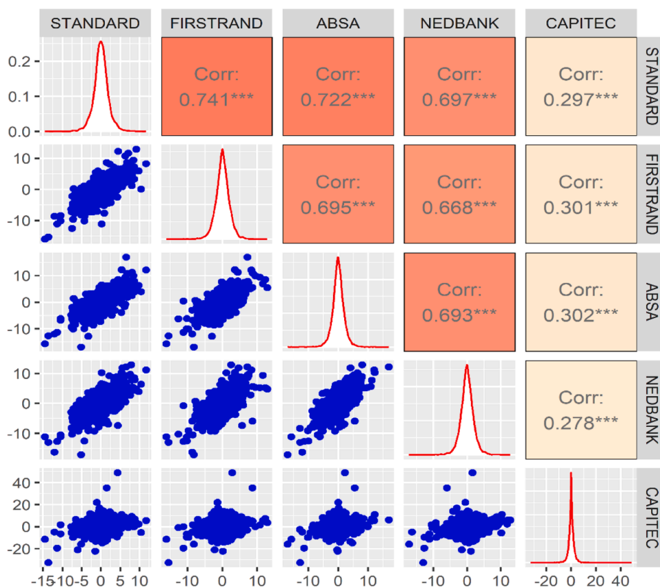
Fig. 2. Pairwise correlations.
