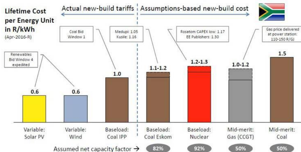
Figure 20: Cost comparison of different electricity technologies (CSIR 2016)
