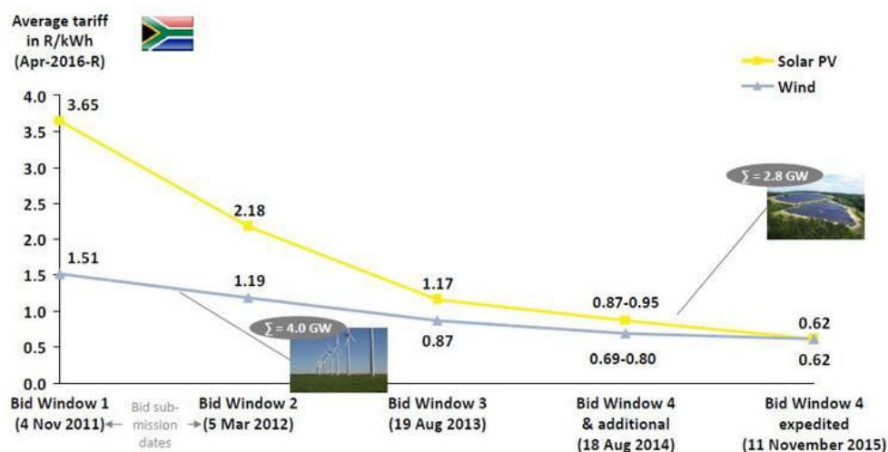
Figure 19: Cost of solar PV and wind from 2011 to 2015 (CSIR 2016)
