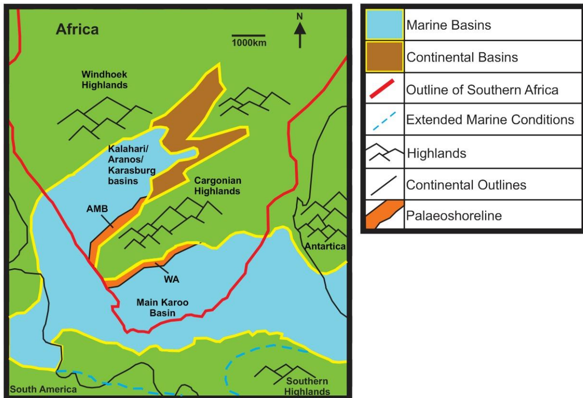
Figure 5.2. Palaeogeographic reconstruction of southern Gondwana during the Late Palaeozoic (based on Visser and Praekelt, 1996 and Scheffler et al., 2006). Note the connectivity of the Aranos, Karasburg and Main Karoo basins as well as shoreline orientations along the Cargonian Highlands (AMB – Amibberg Formation; WA – Waterford Formation).
