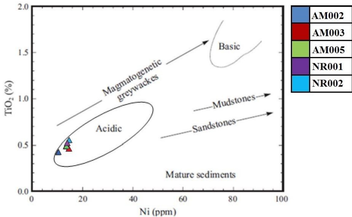
Figure 3.19. \text{TiO}_2 vs Ni bivariate plot for the mudstones of the upper Aussenkjer Formation and the Amibberg Formation (fields after Floyd et al., 1989). Triangles indicate plotted samples.
