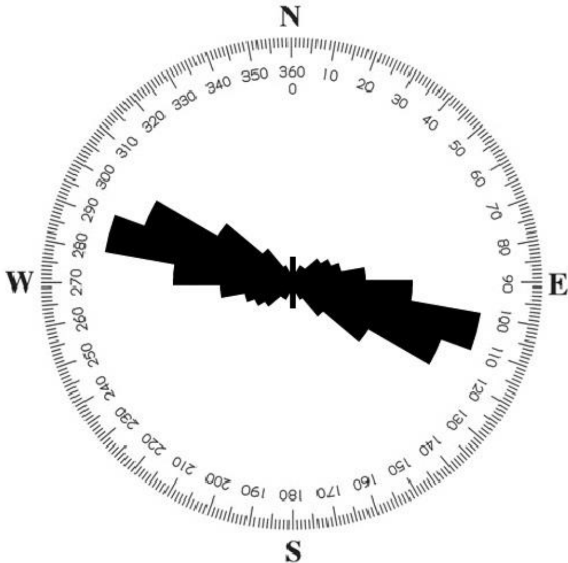
Figure 2.28. Symmetrical wave ripple palaeocurrents. 106 palaeocurrent readings obtained from symmetrical wave ripples and displayed on a rose diagram. A general trend WNW-ESE is observed as well as outliers of the data set.
