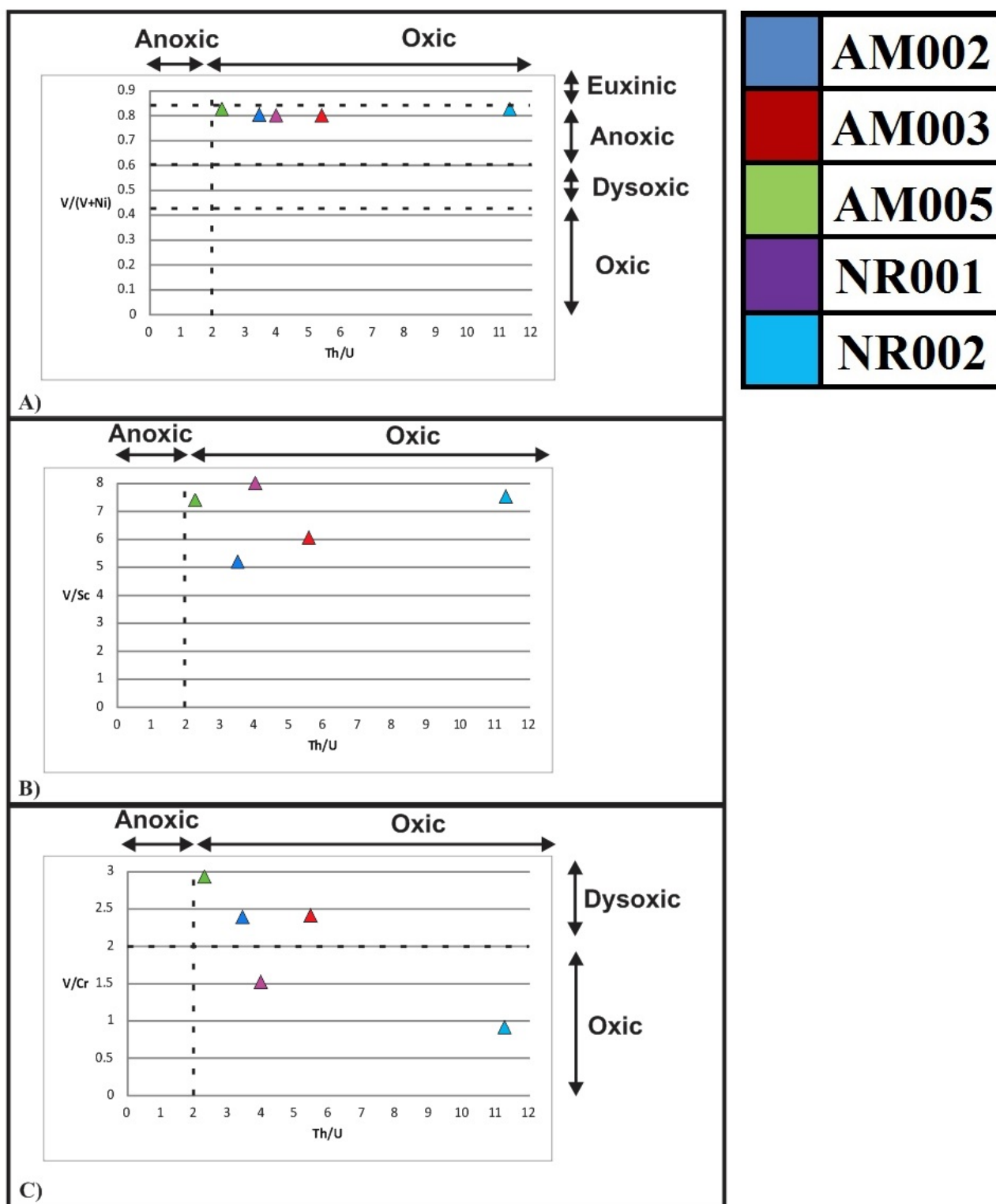
Figure 3.23. Crossplots of various trace element ratios used as palaeoredox proxies. A) Th/U vs V/(V+Ni). B) Th/U vs V/Sc. C) Th/U vs V/Cr.
