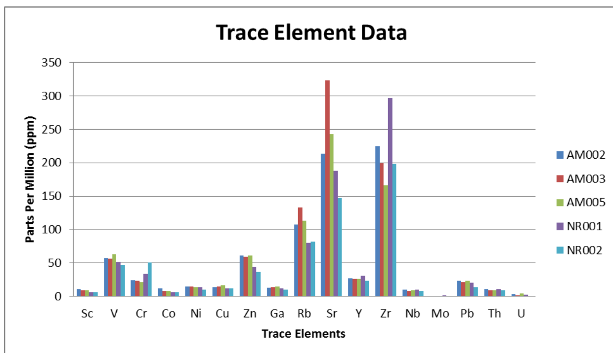
Figure 7.7. Bar graph of various trace elements (in ppm) from mudstones.
