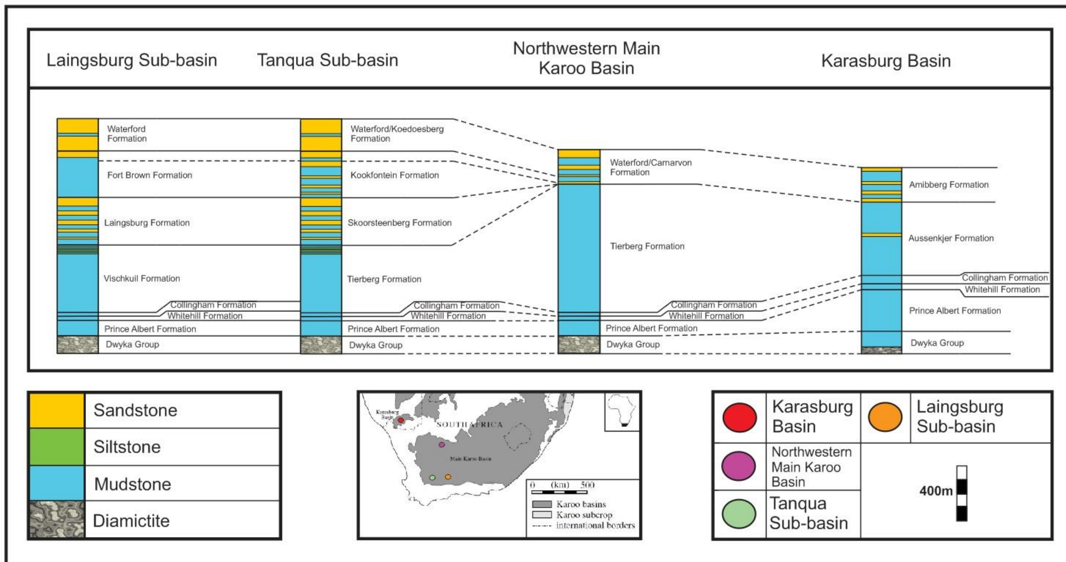
Figure 5.3. Final lithostratigraphic correlation between the Karasburg and Main Karoo basins as well as the Tanqua and Laingsburg sub-basins. Inset map of southern Africa displays the location of the various stratigraphic sections. Note that thickness of formations may vary within a given basin.
