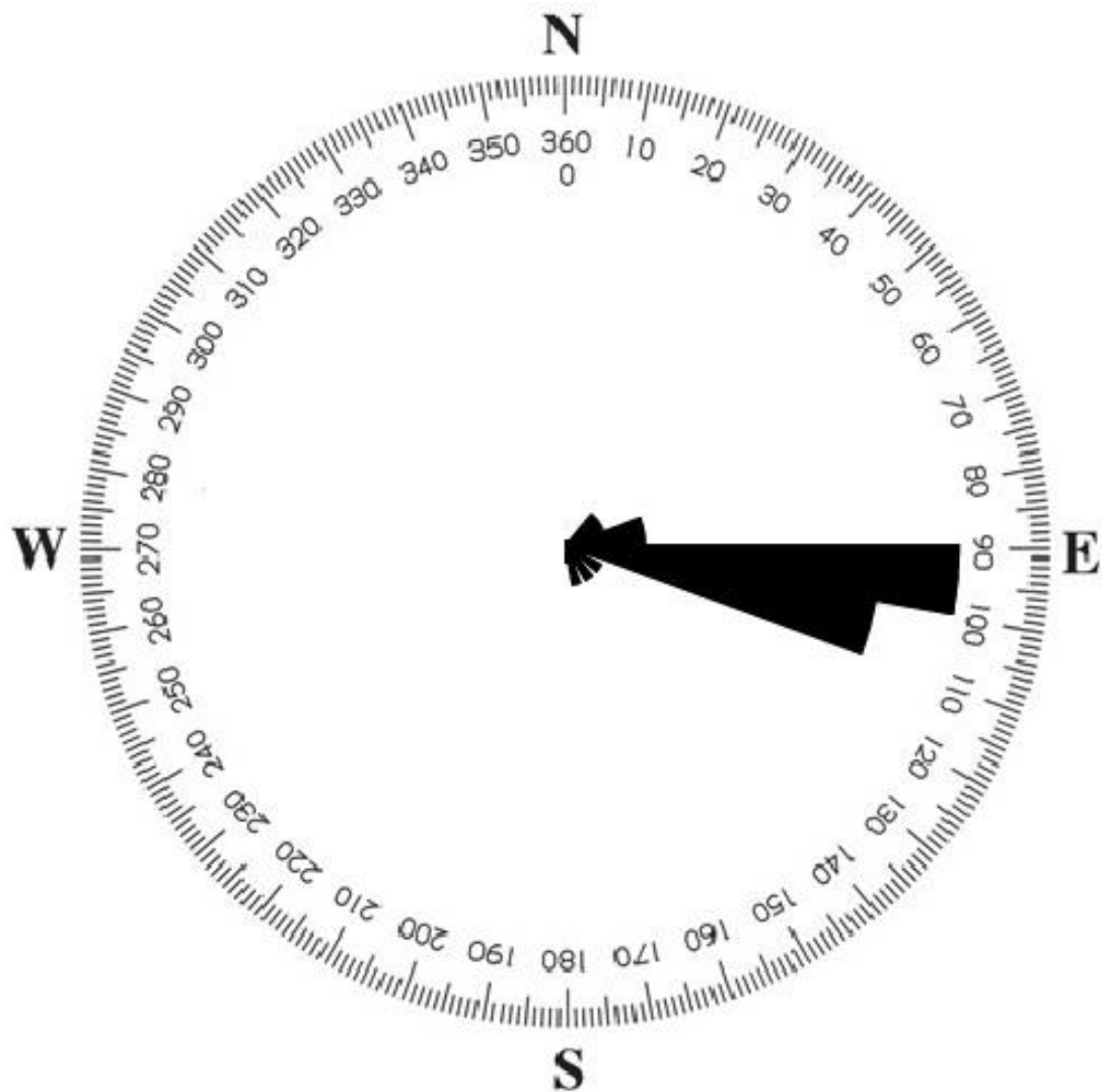
Figure 2.29. Asymmetrical wave ripple palaeocurrents. 28 palaeocurrent readings obtained from asymmetrical wave ripples and displayed on a rose diagram. A general ESE trend is observed as well as outliers of the data set.
