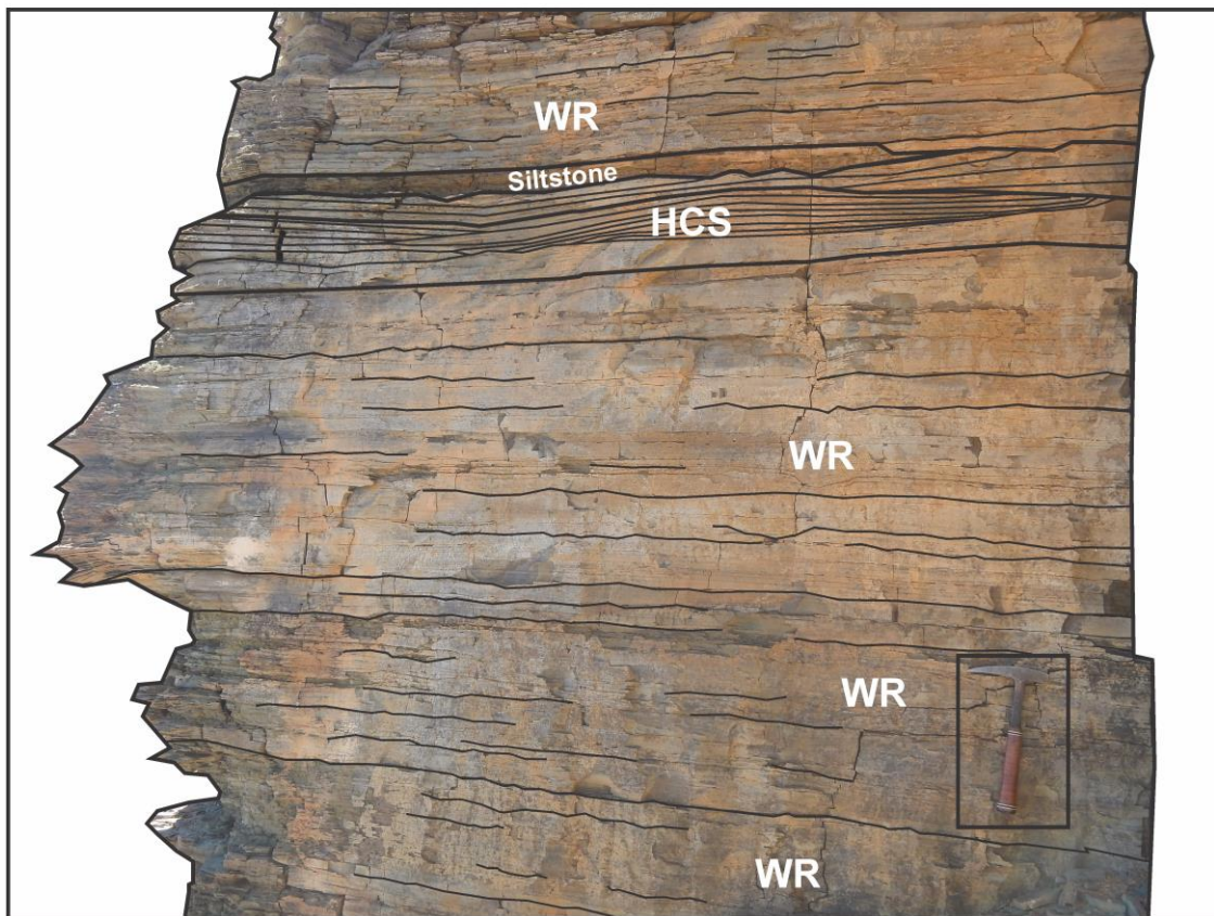
Figure 2.22. Interpreted photograph of an amalgamated HCS and wave rippled unit. 20cm zone of HCS and minor siltstone bed in a unit of amalgamated wave ripples (hammer for scale is 32cm long).
