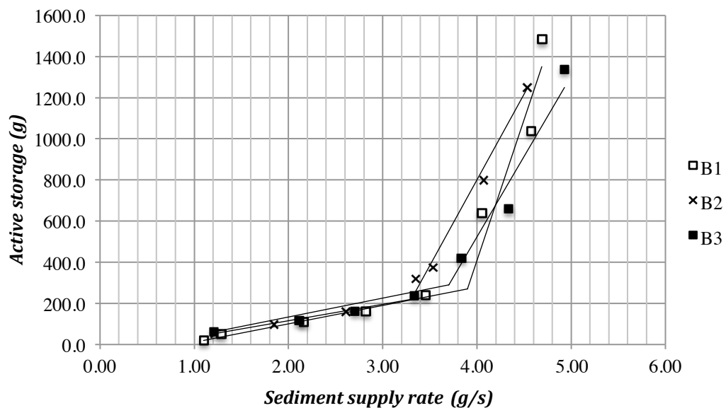
Figure 3-8 Active storage in discrete and collective modes of bed load transport for Series B experiments (quartz sediment)
