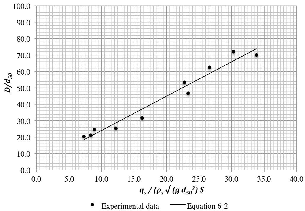
Figure 6-1 Dimensionless relationship for minimum flow depth
