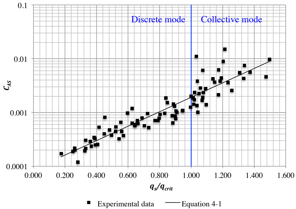
Figure 4-1 Dimensionless relationship for active storage
