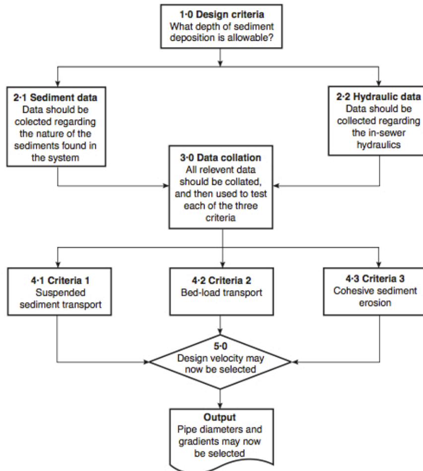
Figure 2-1 Schematic application of CIRIA design procedure (Arthur et al., 1999)
