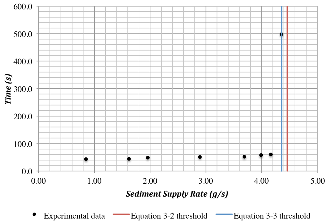
Figure 5-1 Time taken for active storage in Series T1 to be cleared
