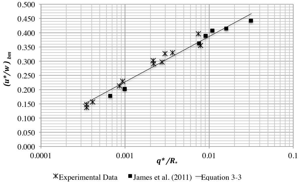
Figure 3-15 Threshold conditions between discrete and collective movement for experimental data and James et al. (2011) data
