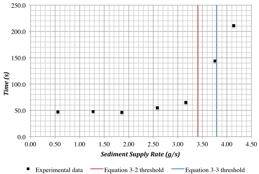
Figure 5-2 Time taken for active storage in Series T2 to be cleared
