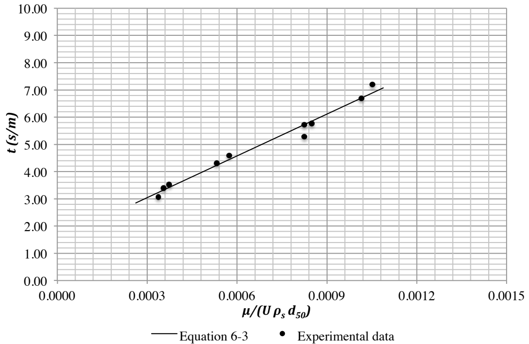
Figure 6-3 Flushing duration relationship
