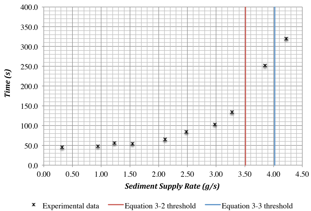
Figure 5-3 Time taken for active storage in Series T3 to be cleared
