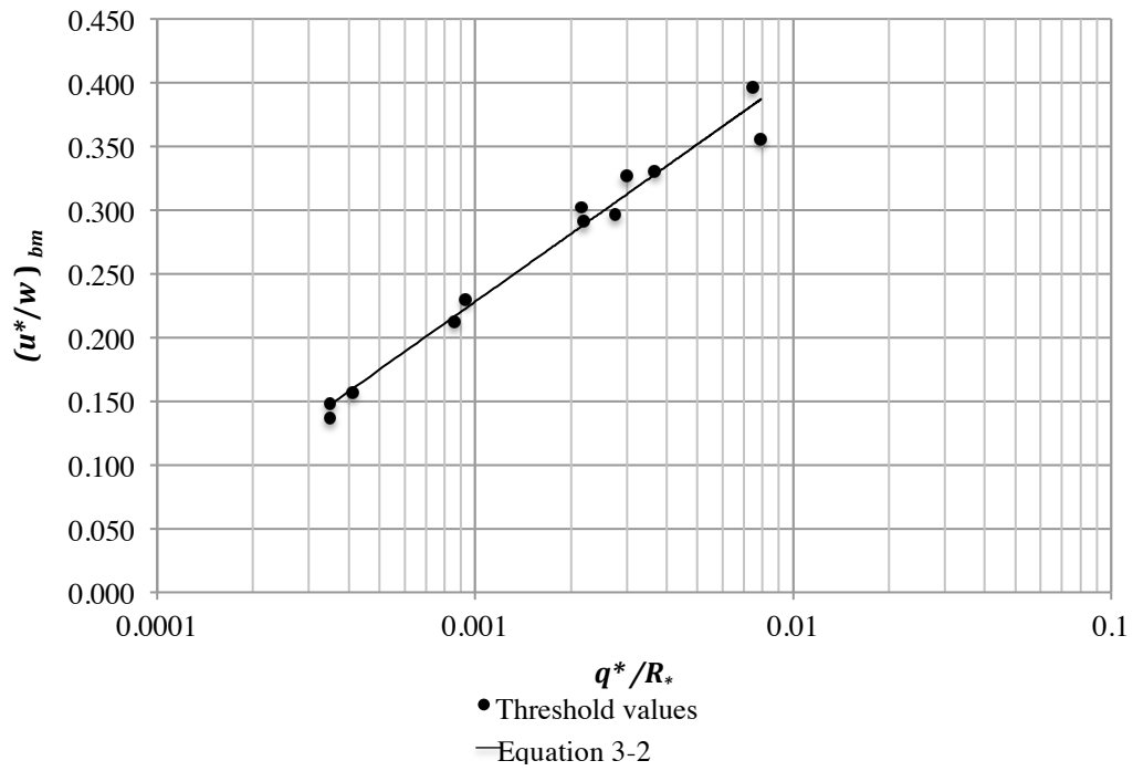
Figure 3-14 Threshold conditions between discrete and collective bed load movement
