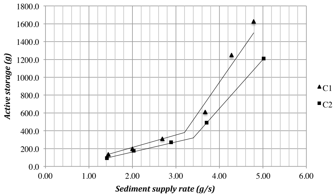
Figure 3-11 Active storage in discrete and collective modes of bed load transport for Series C experiments (coal sediment)
