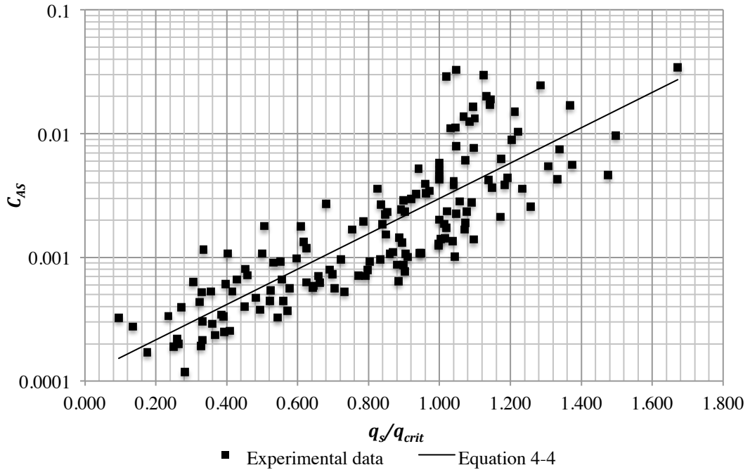
Figure 4-3 Dimensionless relationship for active storage for combined data
