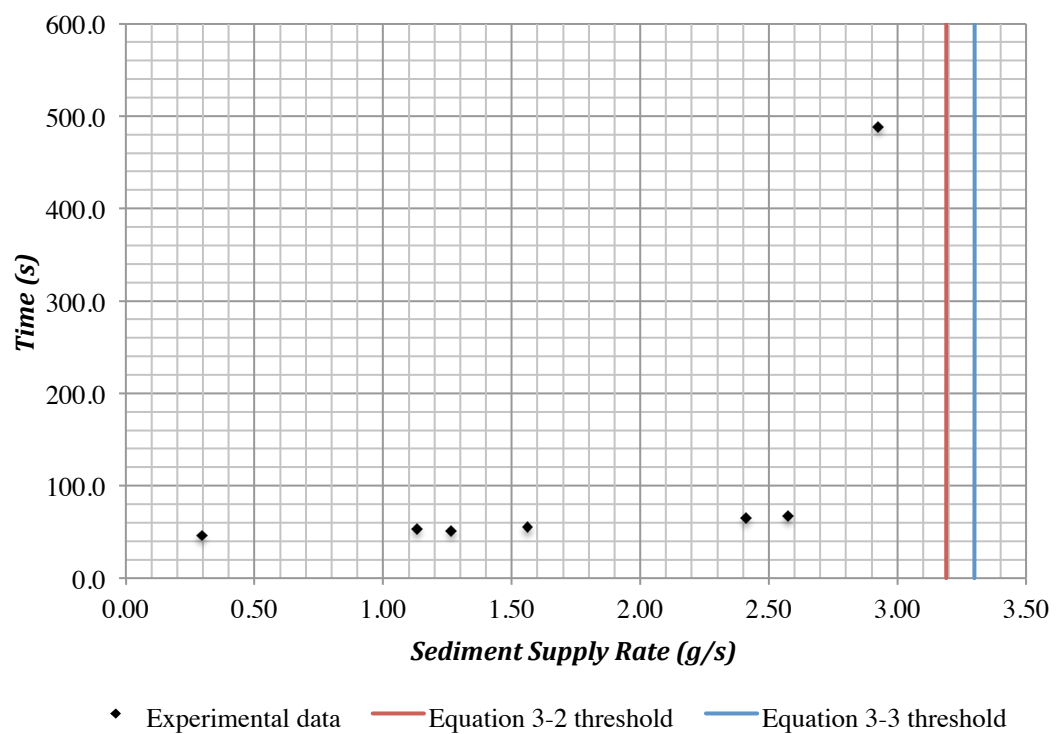
Figure 5-4 Time taken for active storage in Series T4 to be cleared
