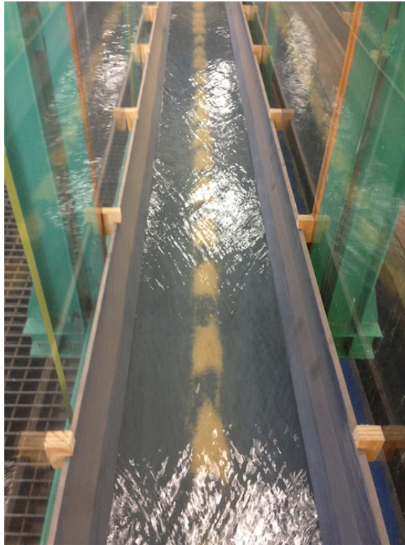
Figure 3-13 Collective bed load movement
