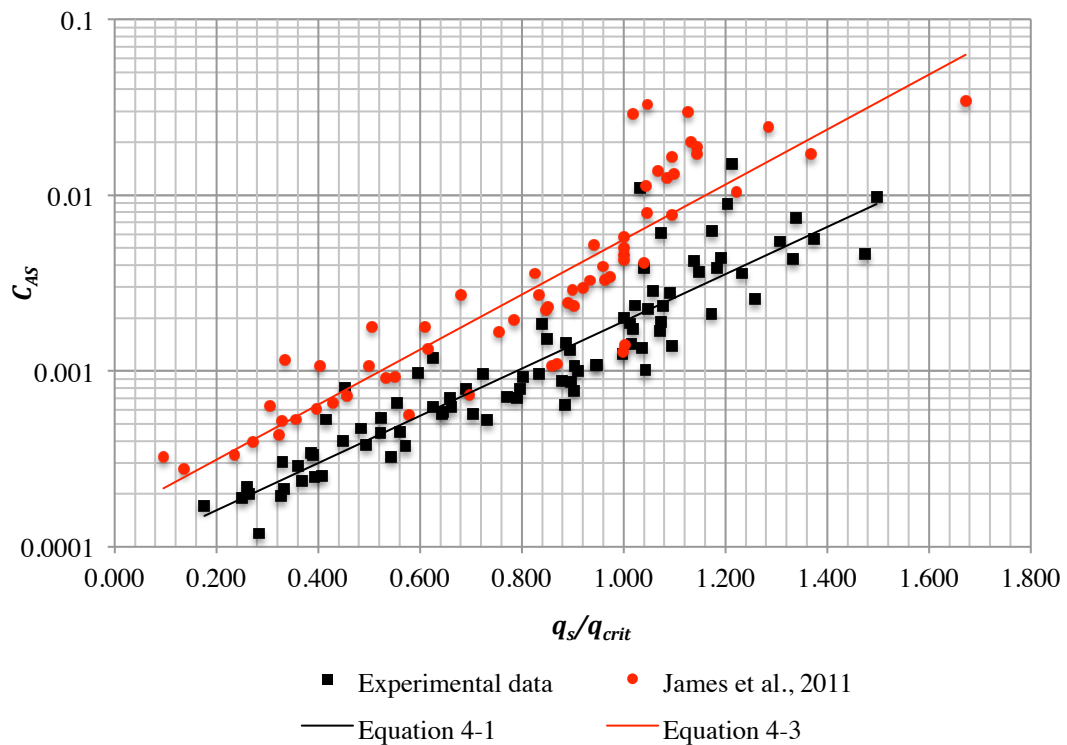
Figure 4-2 Dimensionless relationship for active storage compared to James et al. (2011) data
