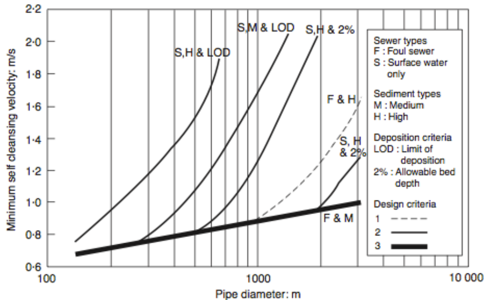
Figure 2-2 Minimum required flow for different sediment transport criteria (Arthur et al., 1999)
