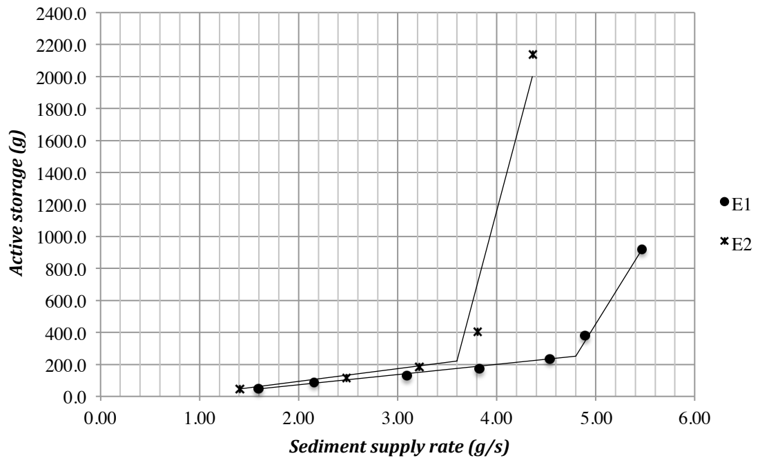
Figure 3-10 Active storage in discrete and collective modes of bed load transport for Series E experiments (quartz sediment)
