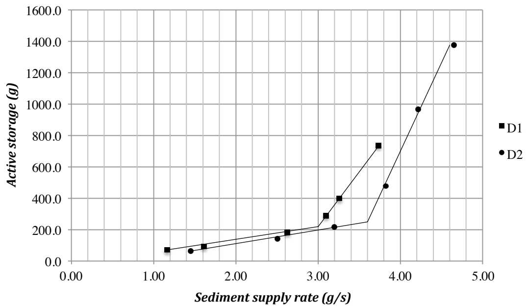
Figure 3-9 Active storage in discrete and collective modes of bed load transport for Series D experiments (quartz sediment)
