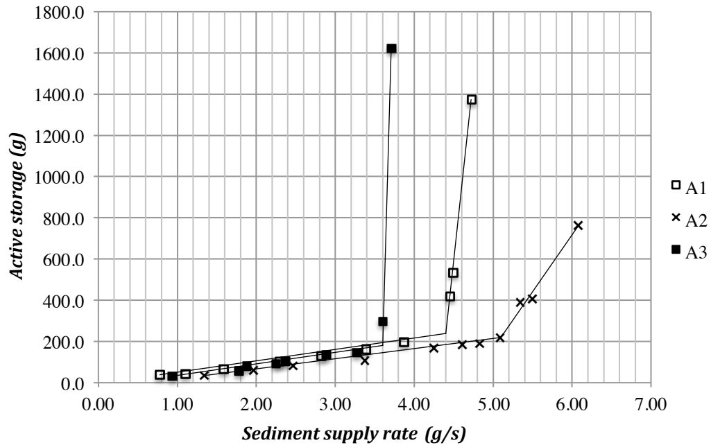
Figure 3-7 Active storage in discrete and collective modes of bed load transport for Series A experiments (quartz sediment)
