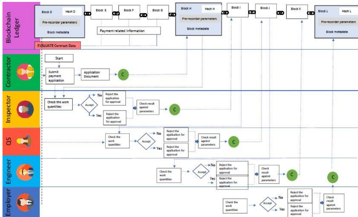
Figure 2.5: Proposed Execution flow of semi-automated payments. Source: (Luo et al., 2019)
