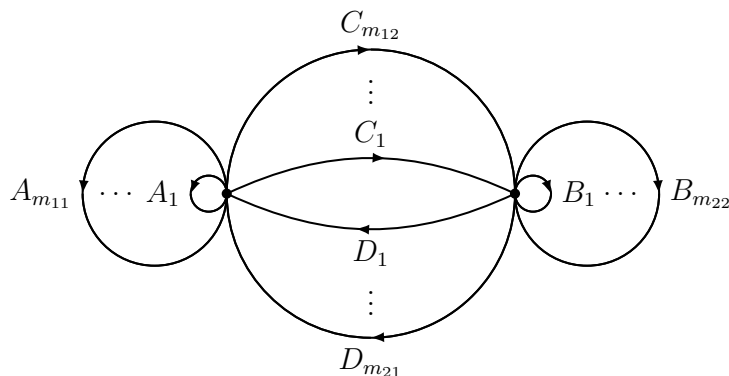
Figure 1. This figure gives a graphical representation of the excited brane bound states described by the generating function (2.35). The node on the left represents the brane with momentum p_1 while the node on the right is for the brane of momentum p_2 .
