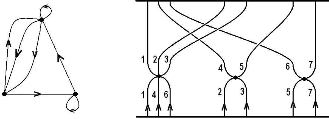
Figure 2. Any open string configuration can be mapped to a labelled graph as shown. The two bold horizontal lines in the figure on the right are identified. Rows of R form nodes in the graph. For the graph shown, R has three rows. There are 7 open strings, so the operator is constructed using 7 Y fields. The graph determines a permutation, so each open string configuration maps to a permutation. For the graph shown the permutation, in cycle notation, is \sigma = (24)(536) . A nice example is the configuration in which all open strings loop back to the brane they start from, described by the identity permutation.
