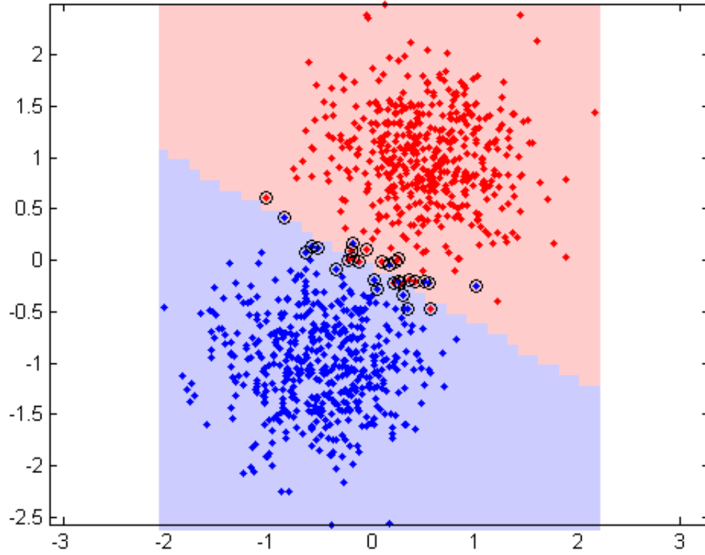
FIGURE 3.4: An example of a linear classification border trained by SVM . Blue and red dots represent different clusters, and circled dots are support vectors.
