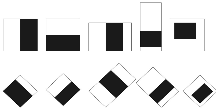
FIGURE 4.11: Some examples of filters for extracting Haar-Like features.
