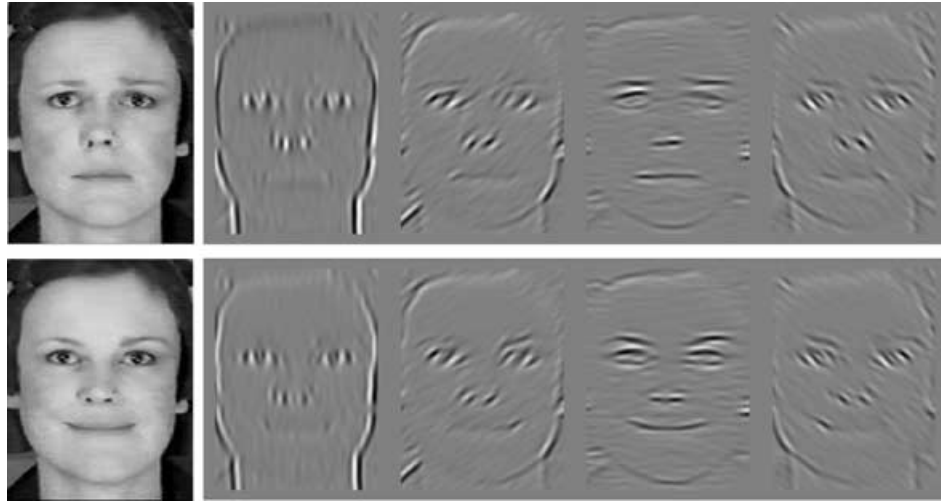
FIGURE 4.10: Gabor responses on images [11].
