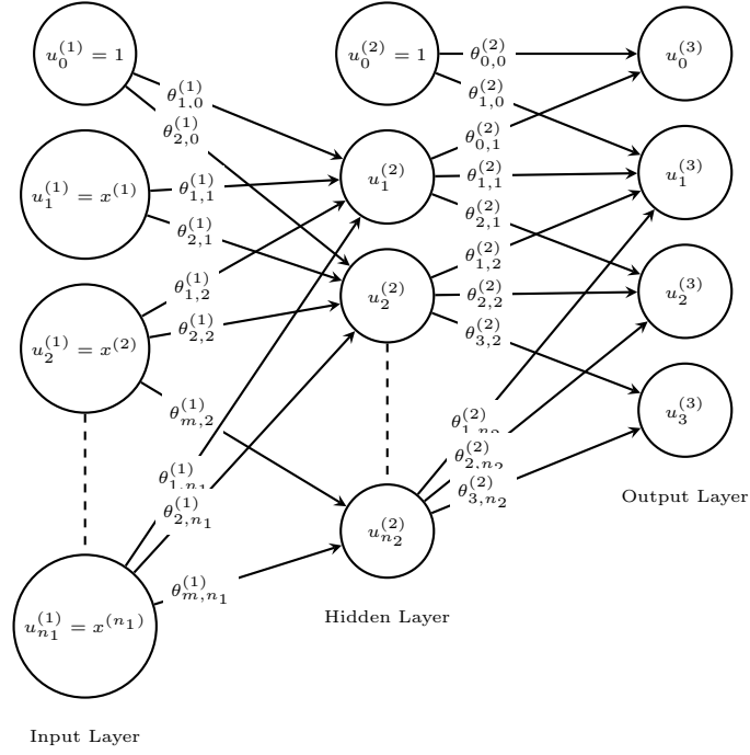
FIGURE 5.6: The structure of the 1 hidden layer, multi-class neural network
