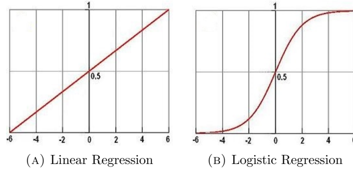
FIGURE 3.5: Linear and Logistic Regression Analysis comparison.
