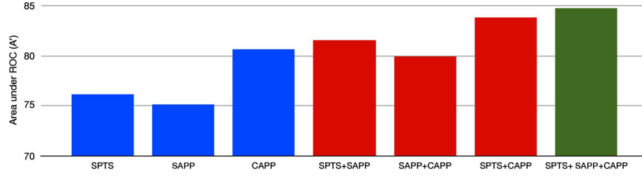
FIGURE 6.4: The results of Lucey et al. [16] by means of area under the ROC curve.
