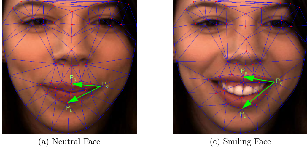
FIGURE 5.3: Example P_C , P_L , P_R points, and vectors for feature extraction [8].
