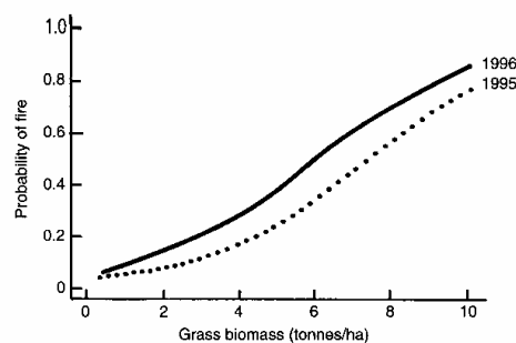
Fig. 14. The relationship between grass biomass (fuel) and the probability of fire in two individual years in the Kruger National Park. Severe fire weather conditions occurred in 1996, but not in 1995. The regression equations were P(f) = e^Z / (1 + e^Z) , where P(f) is the probability of fire, e is the base of natural logarithms, and Z = -3.47 + 0.00047b for 1995, and -2.47 + 0.00051b for 1996 ( b = grass biomass in kg ha -1 ).
