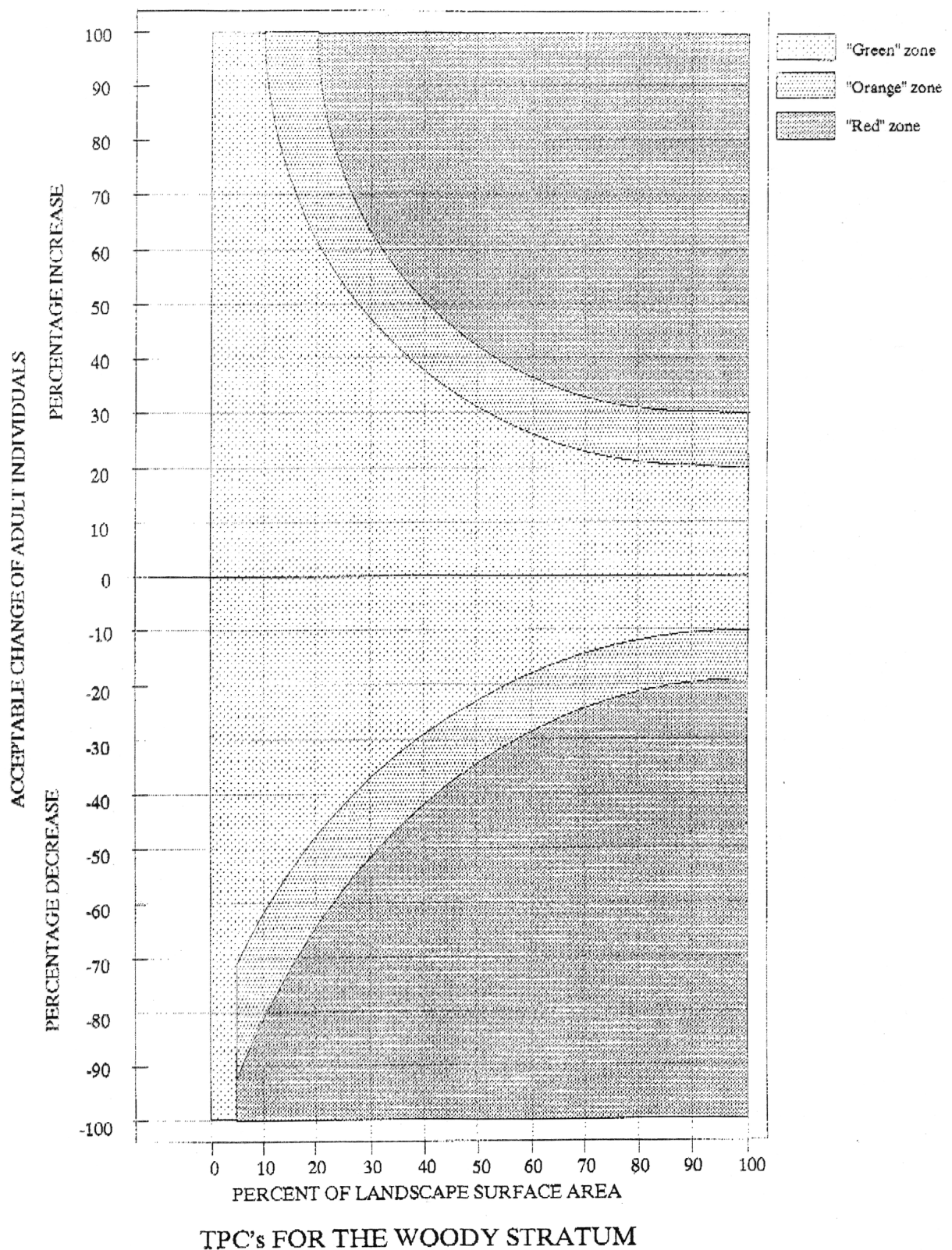
Figure 17-3: Change over area graph modelling the suggested Thresholds of Potential Concern for the density of the woody vegetation in the KNP (Provided by N Zambatis KNP Scientific Services).
