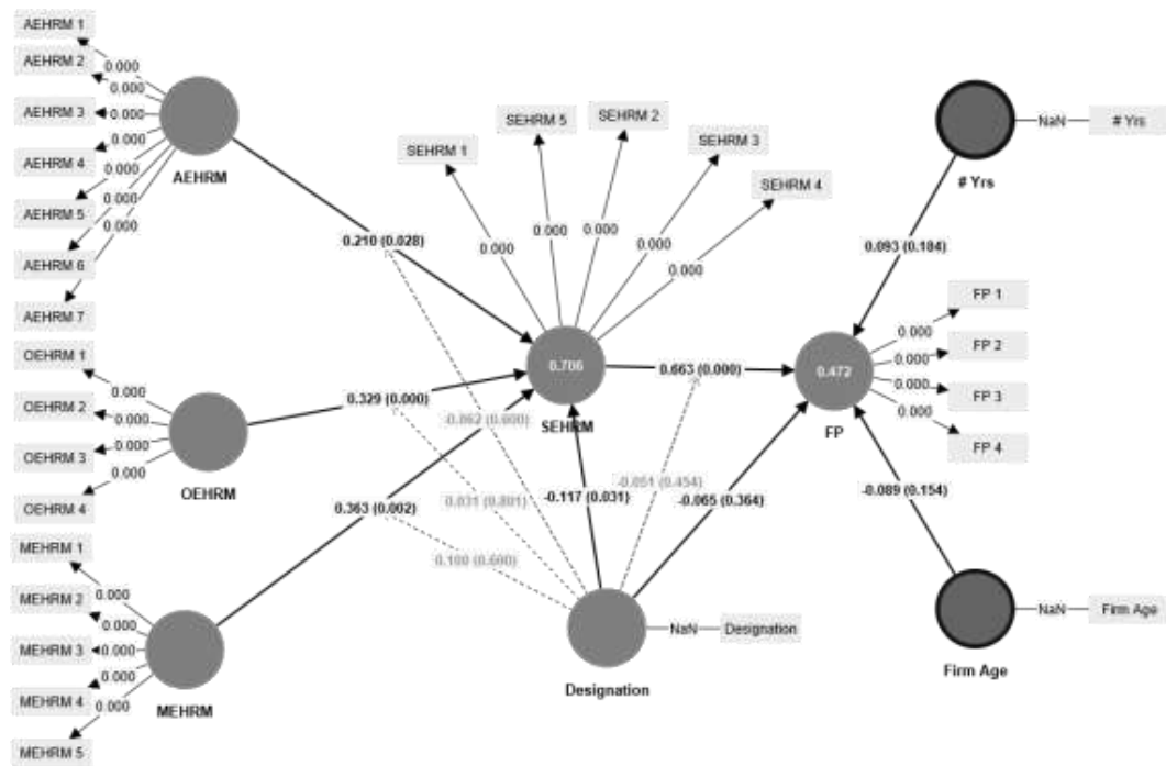
Figure 10: Structural Model
