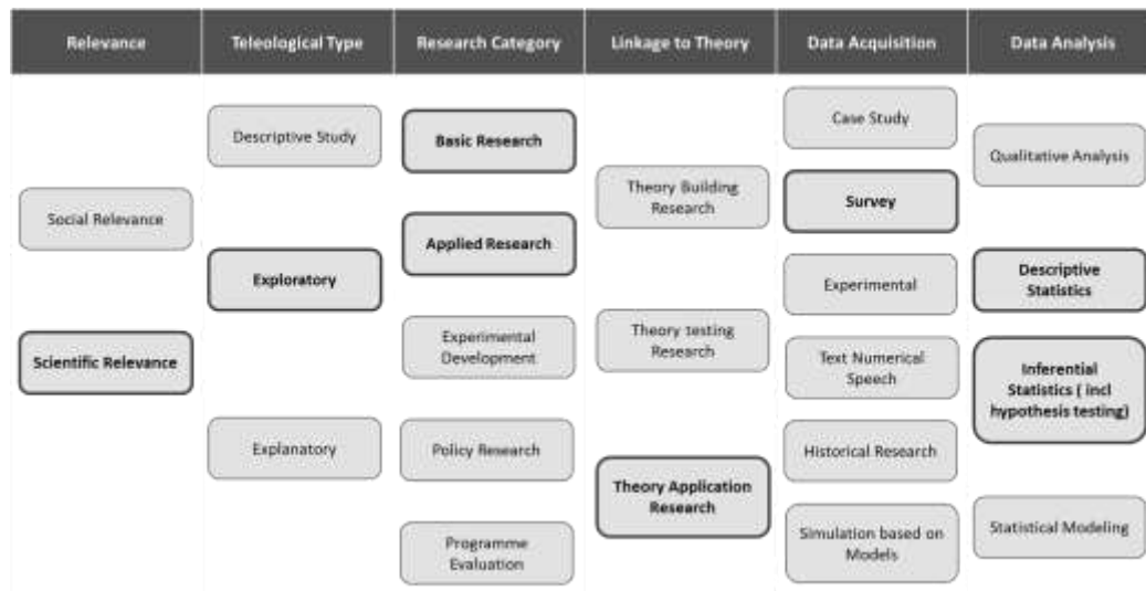
Figure 4: Summary of Research Methodology
