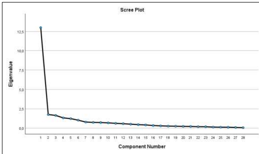
Figure 8: Scree Plot
