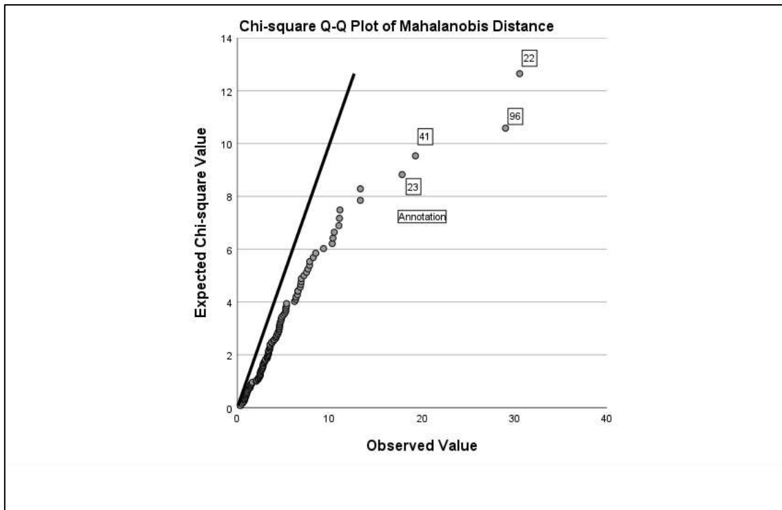
Figure 5: Q-Q Plot of the Mahalanobis Distance
