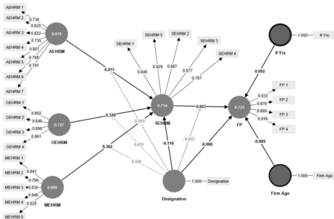
Figure 9: PLS Measurement Model
