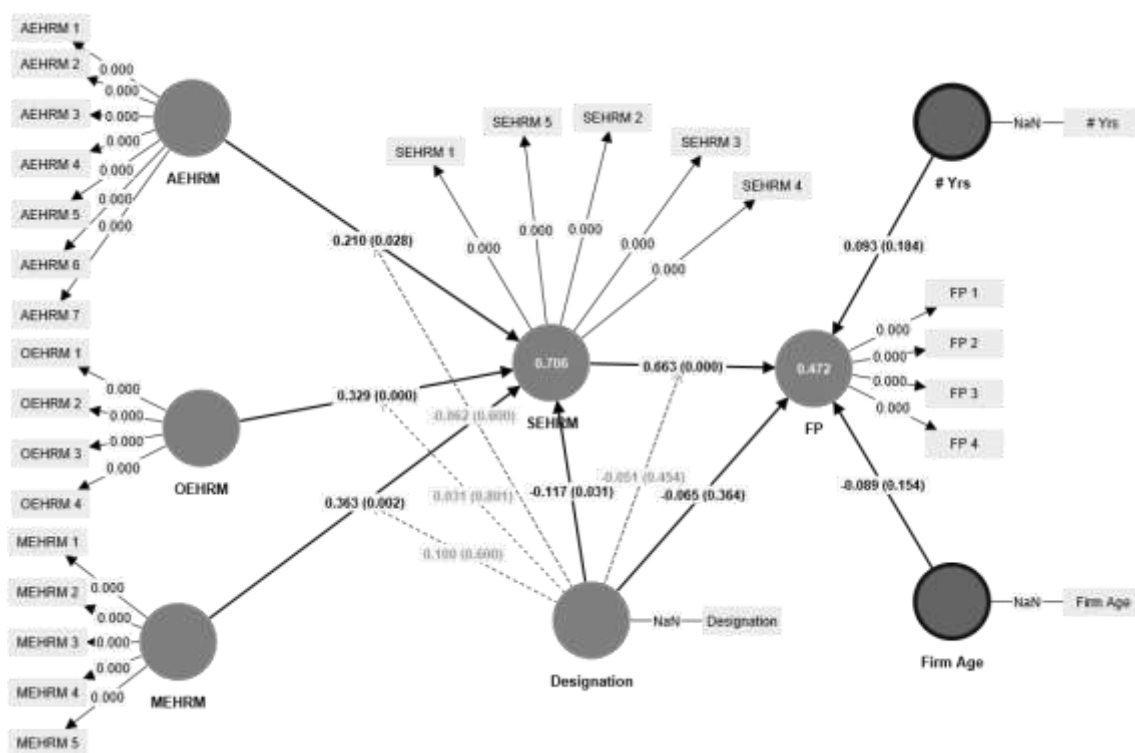
Figure 11: Model Showing the R^2 Explained
