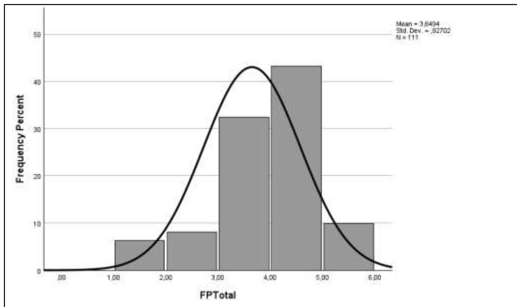
Figure 6: Test for Normality
