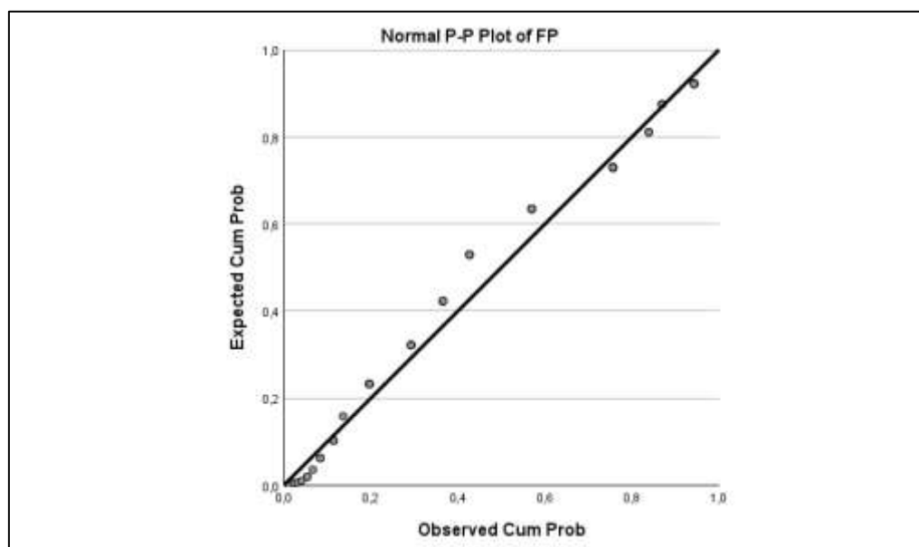
Figure 7: Normal P-P Plot of FP
