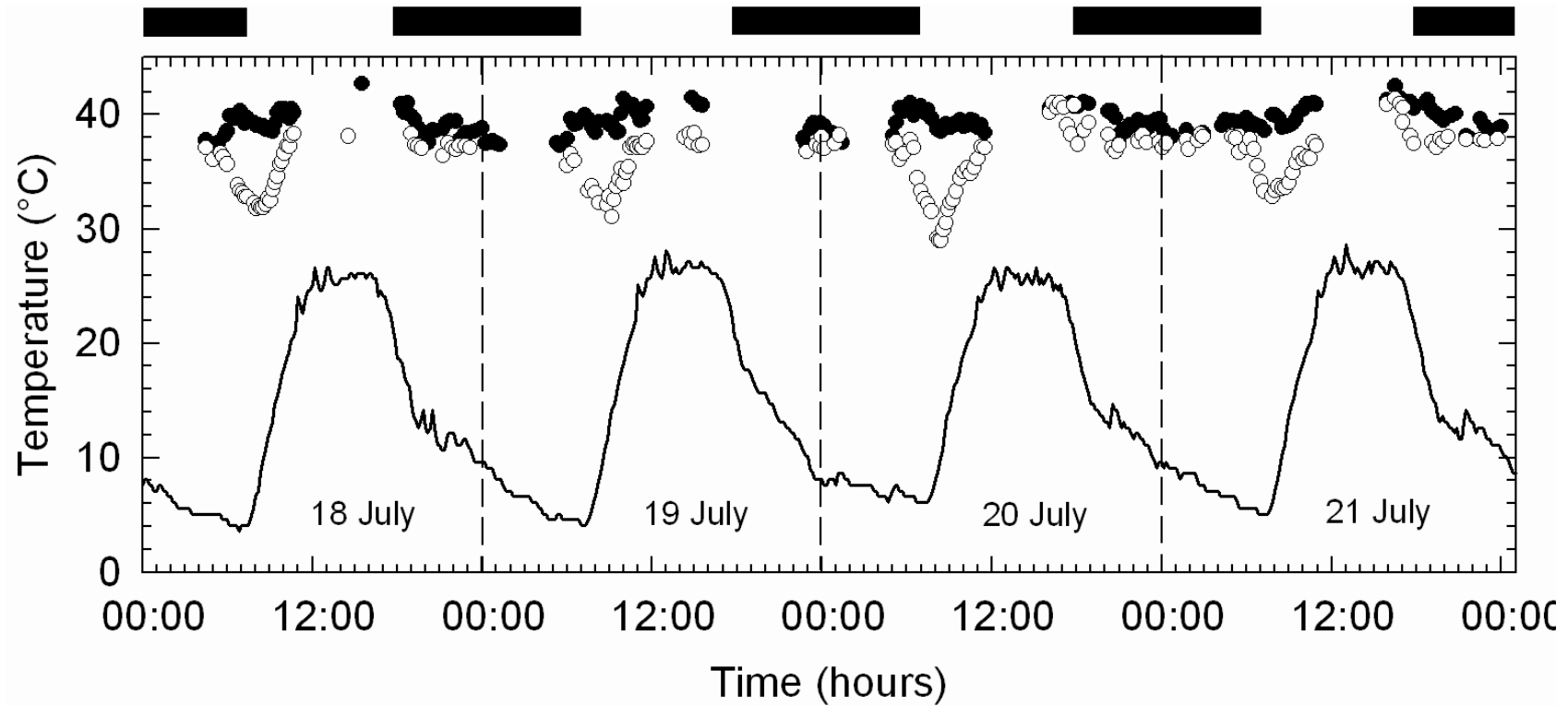
Figure 3: Skin temperature ( T_{\text{skin}} ) in a single Pearl-spotted Owlet (filled circles) and African Scops-Owl (clear circles) on four consecutive days during July 2007 at Molopo Nature Reserve. Air temperature ( T_a ) measured at the study site is represented by the solid line. The black bar at the top of the expanded figure indicates night-time. The Pearl-spotted Owlet typically remained homeothermic, whereas the African Scops-Owl showed shallow bouts of torpor every morning after sunrise. After sunrise on the morning of 20 July 2007 the African Scops-Owl reduced T_{\text{skin}} to 29.0°C.
