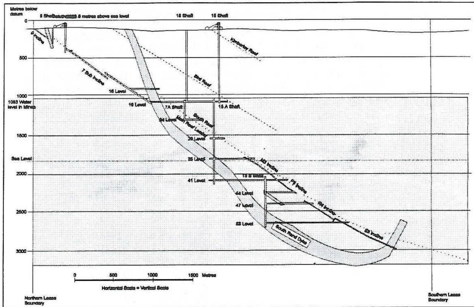
Figure 2.8. Cross section through Crown Mines property (Scott, 1995)
