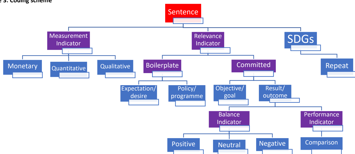
Figure 3: Coding scheme
