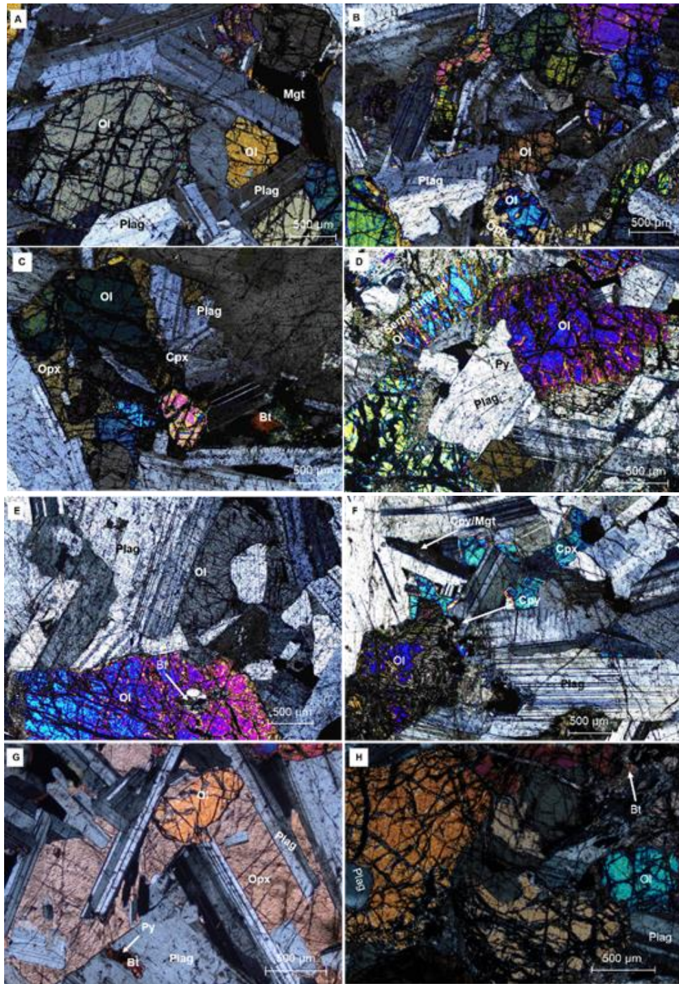
Figure 19: Transmitted-Light Photomicrographs (all XPL; 4x magnification) of two samples from Ohamaremba. A) Fine- to medium- grained and subhedral to anhedral olivine and subhedral to anhedral plagioclase laths to give a cumulate texture in the leucotroctolite. B) Fine-grained subhedral to anhedral olivine and mainly anhedral, partially enclosed plagioclase, with olivine showing orthopyroxene reaction rims. C)
