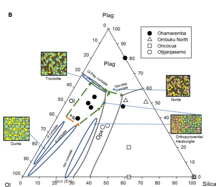
Figure 14: The modal abundances of the MUM intrusions plotted on mineral ternary plots (A, Ol-Plag-Cpx; B, Ol-Plag-Silica) modified from Barnes (2023). This plot included only samples that were relatively unaltered and described petrographically. These ternary diagrams show the crystallisation sequences of basaltic liquids. The ellipse-like shapes are zones of cumulates (dark blue). The MUM intrusions are plotted (Ohamaremba, Otijjanjasemo, Oncocua and Ombuku North). Ol=Olivine, Plag=Plagioclase, Cpx=Clinopyroxene and Opx=Orthopyroxene.
