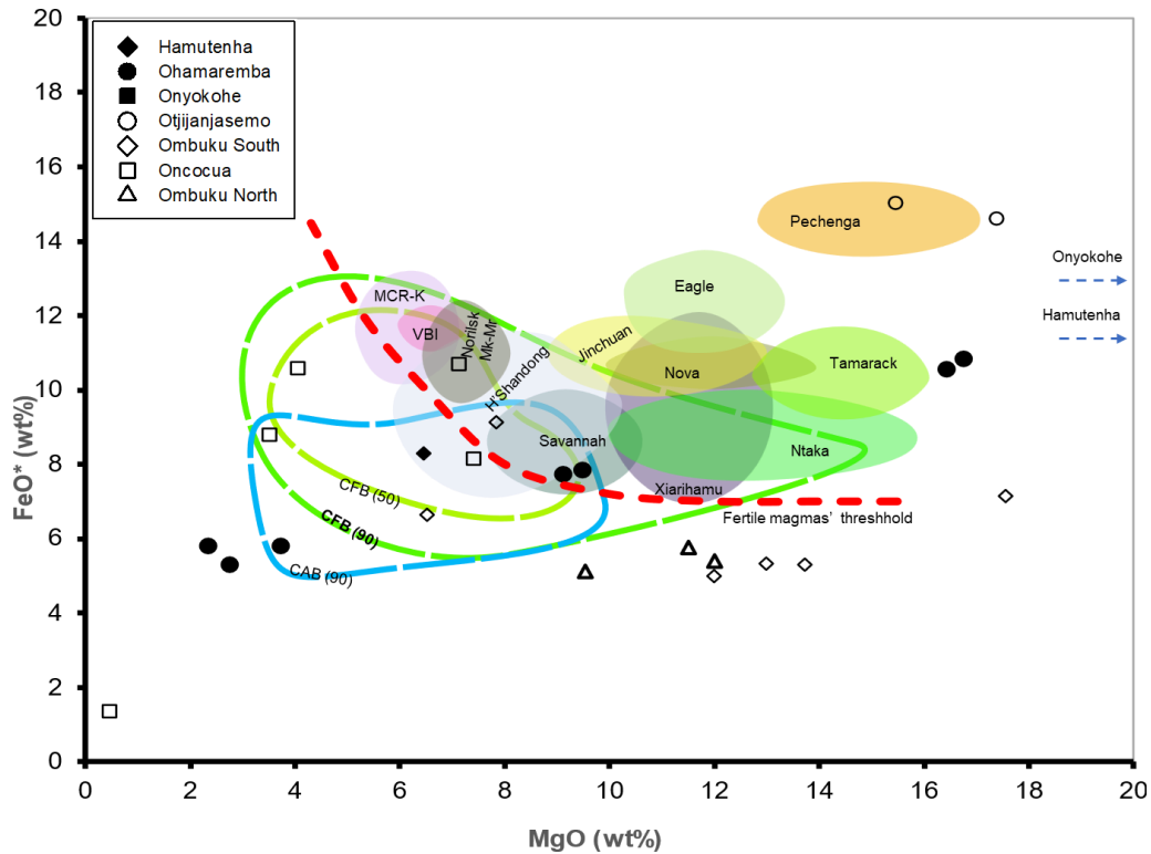
Figure 23: A FeO*-MgO (wt%) diagram that includes the parent magma compositions of world-class magmatic Nickel sulphide mineralised intrusions globally. The MUM intrusions associated with the KC are also plotted for comparison (1 sample of Onyokohe and 2 samples of Hamutenha plot outside the diagram as indicated by blue dashed arrow). The liquid composition curve (red dashed line) is the empirical threshold for 'fertile magma' with most Ni-enriched deposits plotting above this line. MCR = Mid-Continent Rift; VBI = Voisey's Bay Intrusion. The circled fields (dashed lines) represent the MgO and FeO* compositional fields of Continental Flood Basalts (CFB) and Continental Arc Basalts (CAB). The plot is modified from Barnes (2023). FeO* represents the total ferrous iron content which was calculated from the total iron content (assuming a ferrous iron proportion of 0.9 in the total iron content).
