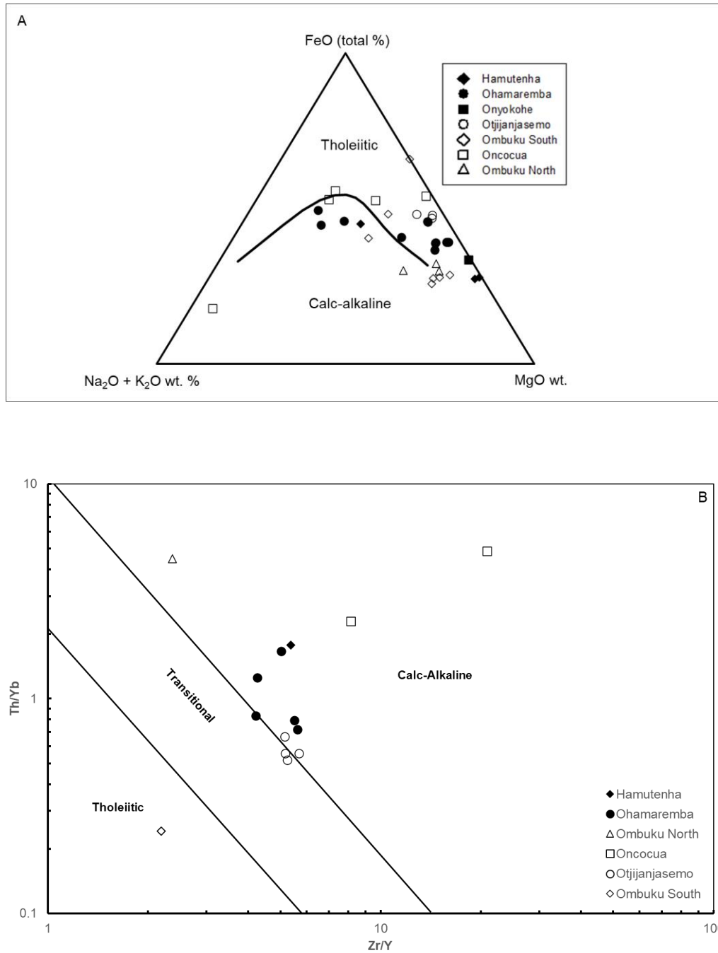
Figure 27: Major oxides and trace element ratio diagrams to assess the magmatic affinity of the MUM intrusions. A) Ternary AFM diagram (after Irvine and Baragar, 1971) shows that most of the MUM samples follow a calc-alkaline trend, towards alkali-enrichment whereas some plot on a tholeiitic trend, towards Fe-enrichment. B) A Zr/Y vs Th/Yb diagram (e.g., Ross and Bédard, 2008; Sappin et al., 2022) showing that most of the MUM samples plot in the transitional and calc-alkaline fields. AFM: A(Na 2 O+K 2 O); F(FeO+Fe 2 O 3 ); M(MgO).
