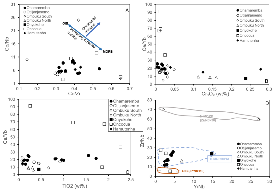
Figure 28: Trace element ratios and major oxides of the MUM intrusions to assess magma sources and magma evolution in the crust. A) Ce/Zr vs Ce/Nb evaluates the degree of partial-melting (negative blue double-arrow line) with two possible end-member sources (OIB = Ocean Island Basalt and MORB = Mid-Ocean Ridge Basalt),
