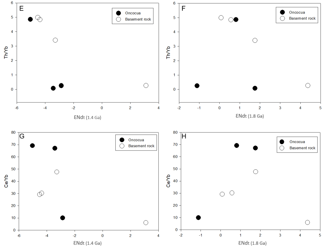
Figure 35: Covariant plots of \epsilon_{Nd(t)} for Oncocua and its basement rocks (corrected at 1.4 Ga and 1.8 Ga) versus \delta^{34}S and selected trace element ratios. A-B) \epsilon_{Nd(t)} vs \delta^{34}S showing negative correlation at 1.4 Ga and positive correlation at 1.8 Ga. C-D) \epsilon_{Nd(t)} vs La/Sm showing negative correlation at 1.4 Ga and positive correlation at 1.8 Ga. E-F) \epsilon_{Nd(t)} vs Th/Yb showing negative correlation at 1.4 Ga and the basement rocks showing negative correlation at a 1.8 Ga. G-H) \epsilon_{Nd(t)} vs Ce/Yb showing negative correlation at 1.4 Ga and positive correlation at 1.8 Ga.
