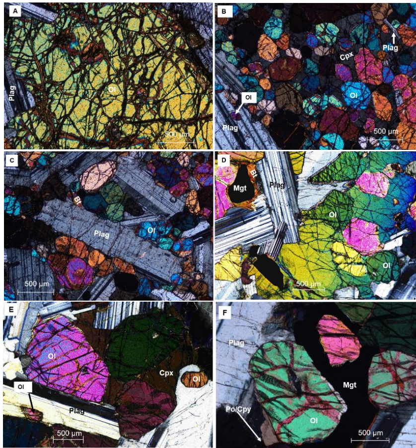
Figure 20: Transmitted light photomicrographs (all XPL; 4x magnification) of two samples from Otjijanasemo. A) Medium-grained anhedral olivine partially enclosing plagioclase to give a sub-ophitic texture locally in the serpentinised troctolite. B) euhedral fine-grained olivine enclosed by clinopyroxene to give a poikilitic texture and locally by plagioclase laths in serpentinised troctolite. C) Medium- to fine-grained plagioclase laths and fine-grained subhedral olivine in the serpentinised troctolite. D) euhedral olivine and plagioclase laths in the troctolite. E) Subhedral to euhedral medium- to fine-grained olivine and medium-grained plagioclase with interstitial clinopyroxene and locally fine-grained olivine enclosed by plagioclase. F) Medium- to fine-grained olivine and medium-grained plagioclase with interstitial magnetite in the troctolite. Ol (Olivine), Cpx (Clinopyroxene), Opx (Orthopyroxene), Plag (Plagioclase), Bt (Biotite), Ap (Apatite), Mgt (Magnetite), Cpy (Chalcopyrite), Po (Pyrrhotite).
