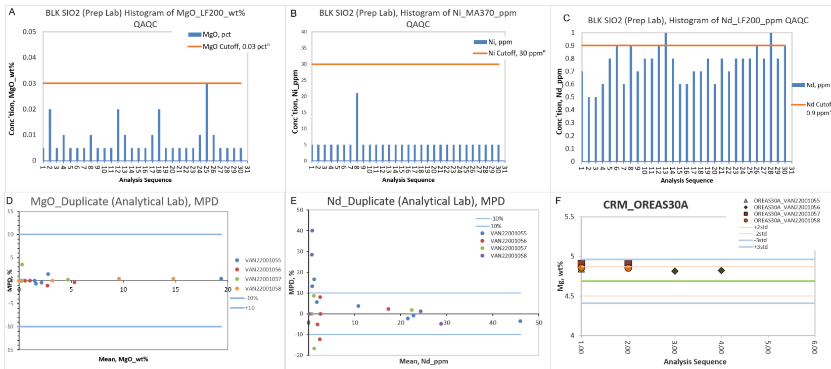
Figure IV.1: QAQC of the samples analysed for major oxides and trace elements at Bureau Veritas. A-C) Blank QAQC samples inserted in the sample batches with approximately 98.76 wt% SiO 2 to assess the level and source of introduced contamination in the method; D-E) Duplicates of routine samples inserted in the sample batches by the lab to assess the precision of the analytical method; F) Certified Reference Material (CRM: OREAS30A) inserted in the sample batches to assess the accuracy of the analytical method. The Mg concentration was converted from MgO ( 0.6031 \cdot \text{MgO} ) to standardise with the OREAS30A certificate. MPD = Mean Percentage Differences.
