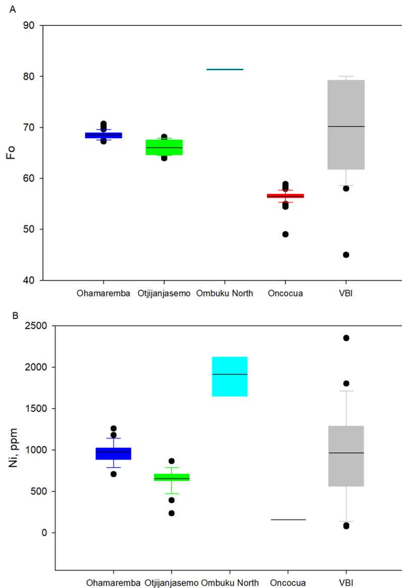
Figure 16: Boxplots showing the range of the Fo composition of olivine (A, Molar Fo; B, Ni in ppm) with outliers (black dots). Olivine Fo-Ni data from the Voisey's Bay intrusion (VBI) are shown for comparison (these data are from Bulle & Layne, 2015).
