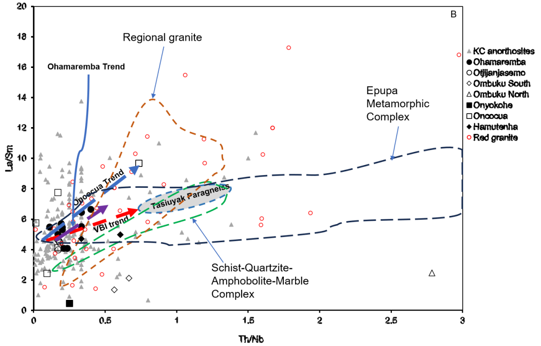
Figure 30: Trace element ratio diagrams to assess magma sources and magma-crust interaction for the MUM intrusions. A) The MUM intrusions plotted on a Th-Yb vs Nb/Yb diagram showing various mantle reservoirs (modified from Pearce, 2008; Sappin et al., 2022); and B) The MUM intrusions plotted on a La/Sm vs Th/Nb diagram that assesses the evidence of crustal contamination. The Regional Granite and Schist-Quartzite-Amphibolite-Marble Complex (SQAMC: green dashed circle) are the basement rocks surrounding Oncócu. The Epupa Metamorphic Complex (EMC: dark blue dashed circle) is the basement rock surrounding Ohamaremba. The Voisey's Bay intrusion contamination trajectory (VBI) towards the Tasiuyak paragneiss is shown for comparison (modified from Li et al., 2000).
