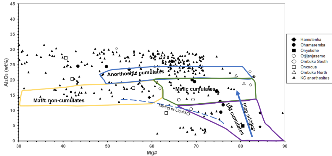
Figure 24: Mg# vs \text{Al}_2\text{O}_3 plot to discriminate the compositions of cumulate and non-cumulate rocks (from Barnes, 2022). A curve showing the mixing of olivine (“ol”) with liquid is shown (dashed blue line). An arrow pointing towards plagioclase addition is also shown. UM = Ultramafic.
