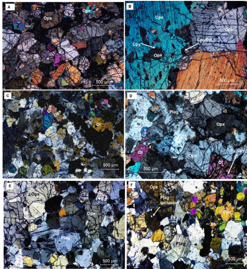
Figure 21: Transmitted-Light Photomicrographs (all XPL; 4x magnification) of three samples from Ombuku North and South. A) Fine-grained subhedral to anhedral orthopyroxene and interstitial clinopyroxene in serpentinitised websterite. B) Coarse-grained clinopyroxene and orthopyroxene with clinopyroxene showing orthopyroxene exsolution lamellae and orthopyroxene enclosed by clinopyroxene oikocrysts in serpentinitised websterite. C) Subhedral to anhedral fine-grained olivine and fine-grained orthopyroxene, clinopyroxene and fine-grained granular plagioclase in the leucotroctolite. D) Fine-grained olivine, subhedral to anhedral fine-grained orthopyroxene and granular fine-grained plagioclase with interstitial clinopyroxene and a larger olivine grain associated with a larger orthopyroxene in the leucotroctolite. E) Subhedral to anhedral orthopyroxene and granular plagioclase in the (leuco) norite. F) Fine-grained orthopyroxene, granular plagioclase and fine-grained clinopyroxene with clinopyroxene mainly interstitial in the (leuco) norite. Ol (Olivine), Cpx (Clinopyroxene), Opx (Orthopyroxene), Plag (Plagioclase), Bt (Biotite), Mgt (Magnetite), Cpy (Chalcopyrite), Pn (Pentlandite).
