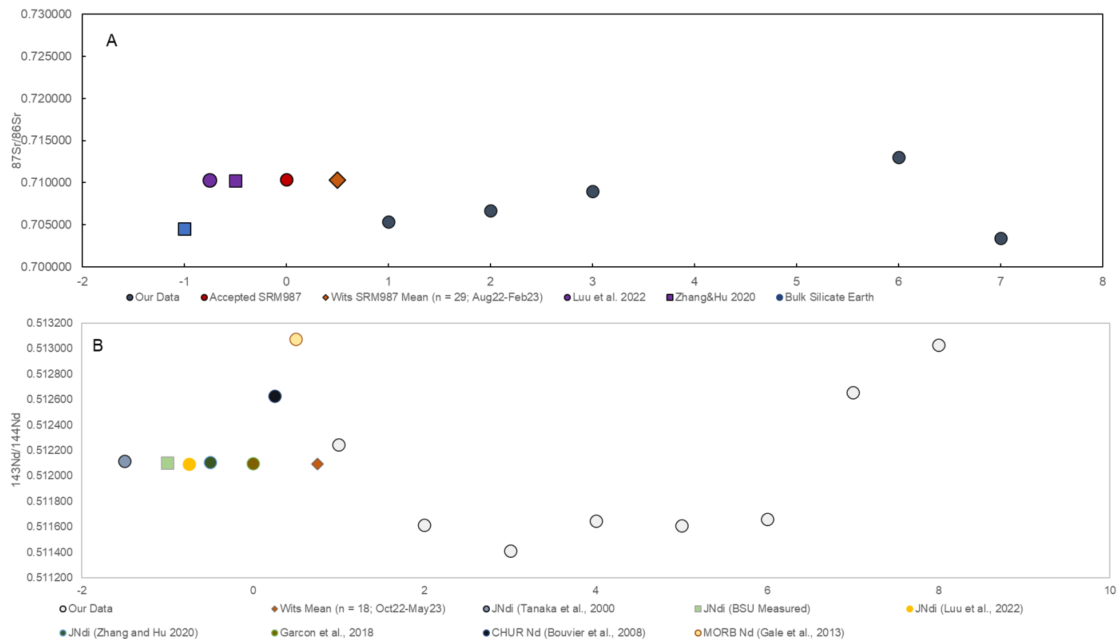
Figure III.2: Performance of standards and reference materials during the Sr-Nd isotope measurements in the lab at Wits. A) ^{87}\text{Sr}/^{86}\text{Sr} ; B) ^{143}\text{Nd}/^{144}\text{Nd} .
