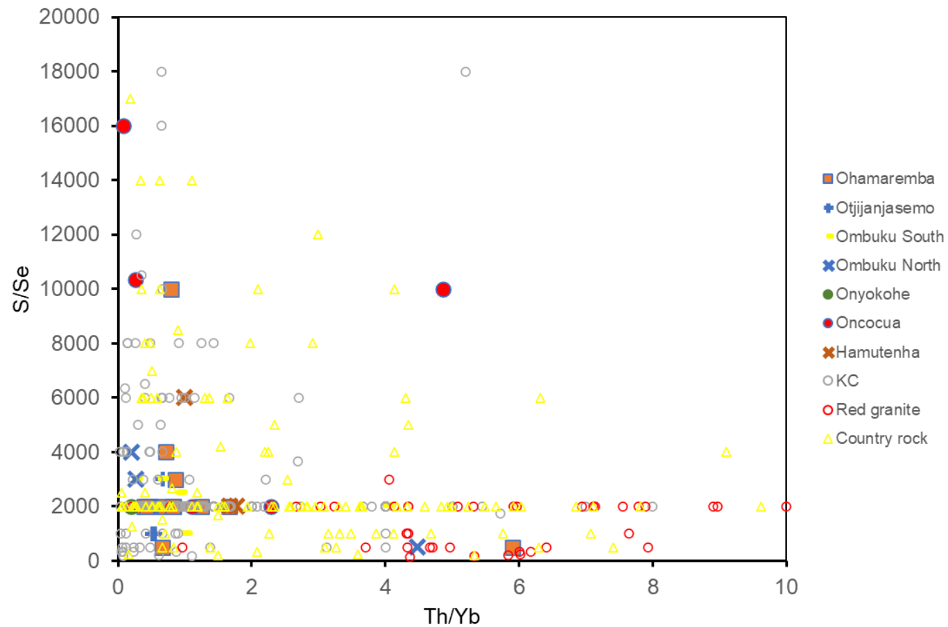
Figure IV.2- Whole rock trace elemental ratios of Th/Yb vs S/Se to assess possible sources of contamination.
