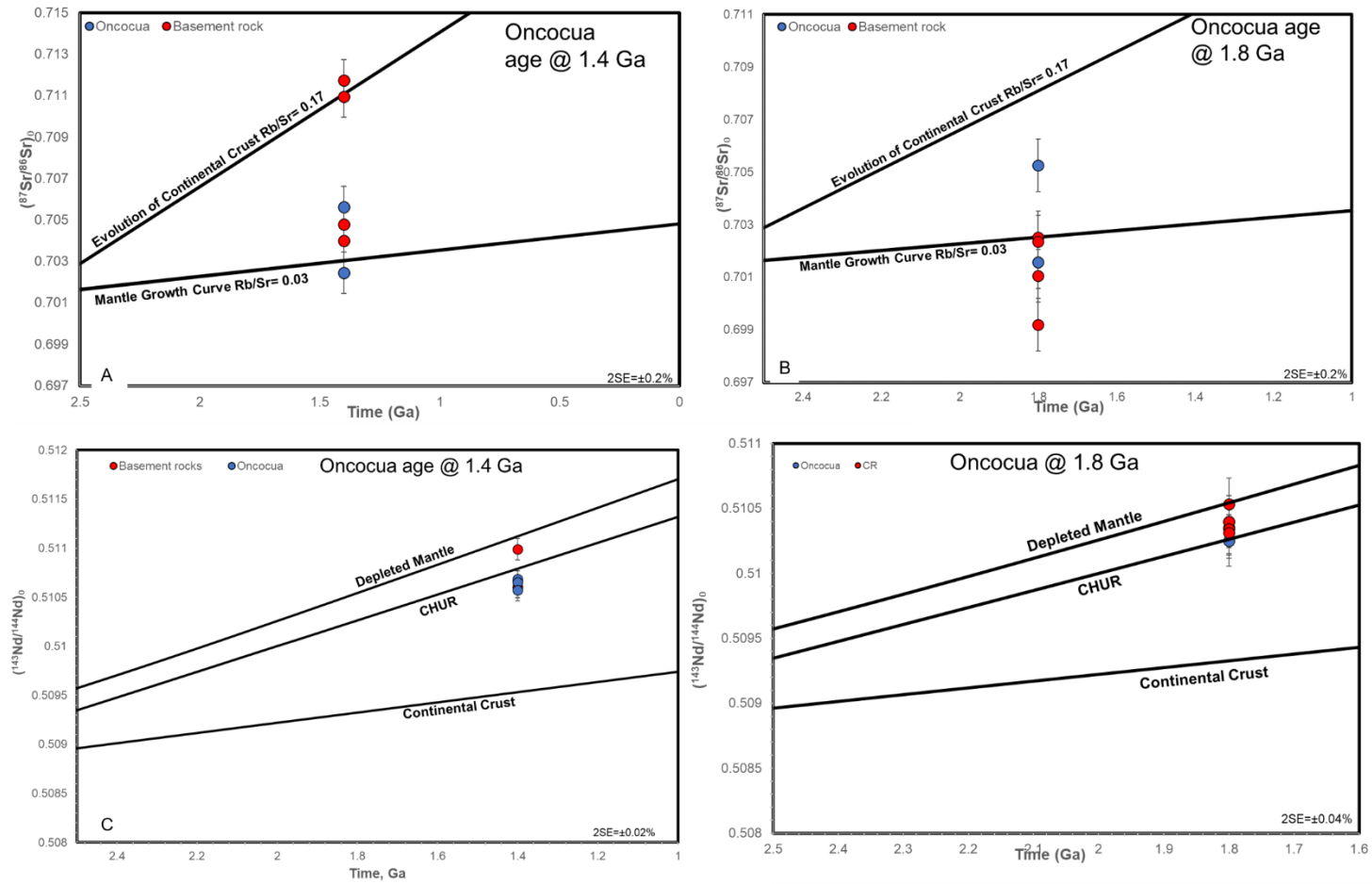
Figure III.1: Sr-Nd isotope composition data for Oncocua and its basement rocks. A-B) Initial ^{87}\text{Sr}/^{86}\text{Sr} Isotopic Compositions corrected to 1.4 Ga and 1.8 Ga. C-D) Initial ^{143}\text{Nd}/^{144}\text{Nd} Isotopic Compositions corrected to 1.4 Ga and 1.8 Ga.
