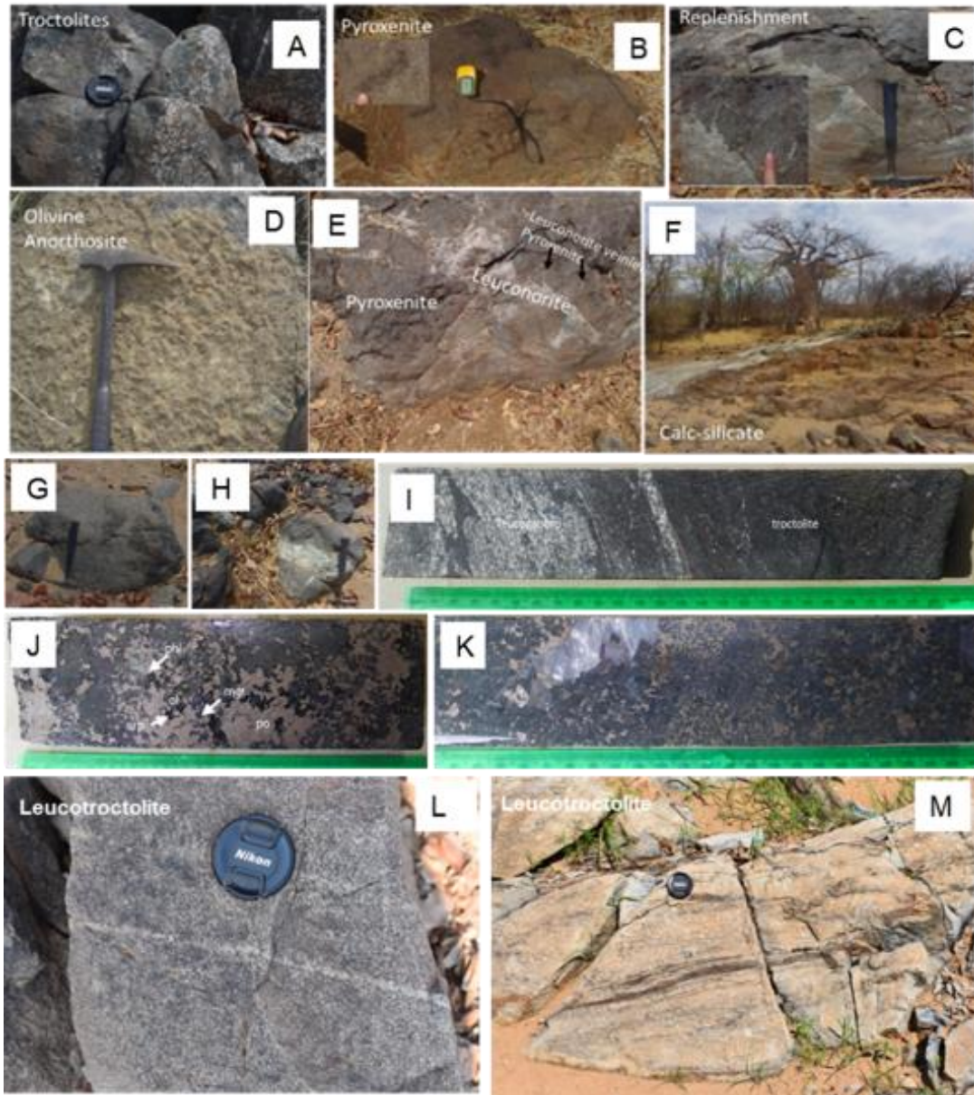
Figure 12: Photographs of outcrops (A-H & L-M) and drillcores (I-K) taken during fieldwork in the Mafic-Ultramafic intrusions (mainly Oncócuá intrusion) of the Kunene Complex that show a range of mafic to ultramafic lithologies and textures. A) Troctolite at Ombuku North with wehrlite bands showing plagioclase-rich and plagioclase-poor zonation; B) Orthopyroxene-rich outcrop at Oncócuá intrusion with coarse-grained orthopyroxenite xenoliths/autoliths; C & E) Feldspathic pyroxenite at Oncócuá in contact with leuconoritic vein and veinlets connected to the interstitial plagioclase of the pyroxenite; D) Olivine anorthosite at Ohamaremba; F) Calc-silicate at the contact between the basement rock in
