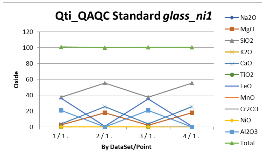
Figure 1.1- Plot of the standard used to assess the in situ mineral chemistry data.
