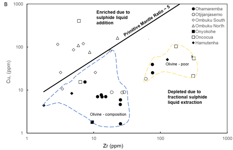
Figure 31: Diagrams of primitive mantle normalised PGE (Platinum Group Elements) and some base metals. A) Plot of Primitive Mantle normalised PGE. B) Plot showing Zr vs Cu to assess evidence of sulphide liquid addition or extraction from sulphur-undersaturated magmas in the MUM intrusions. Primitive Mantle values are from Barnes and Maier (1999). The dashed fields represent clusters of high Zr (> 60 ppm) of olivine-poor rocks and low Zr (< 60 ppm) of olivine-rich rocks. The Cu-Zr plot is modified from Barnes (2023) and Li and Naldrett (1999).
