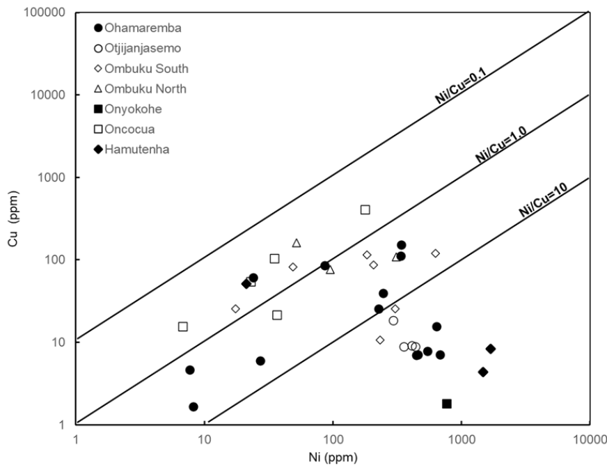
Figure 32: Plot of Ni vs Cu to assess metal enrichment in the MUM intrusions showing which intrusions are likely to be Ni enriched over Cu.
