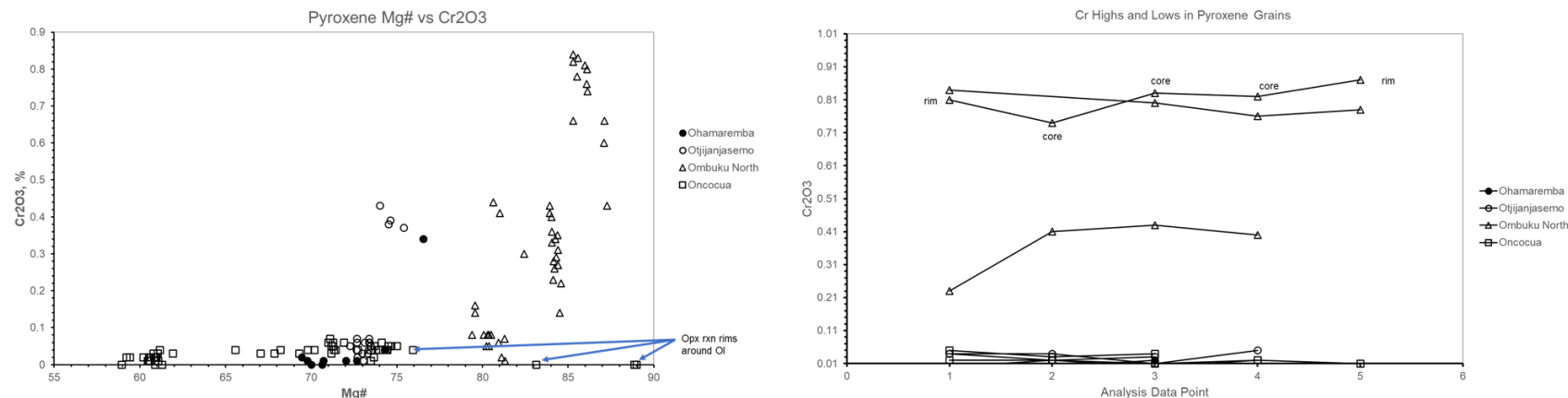
Figure I.2: A) Plot to assess Mg# and Cr 2 O 3 ; B) Cr 2 O 3 profiles in pyroxene.
