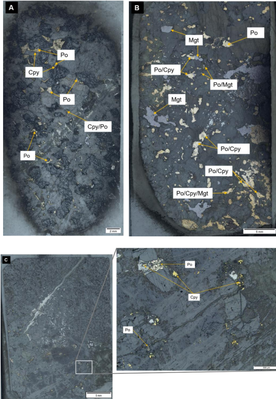
Figure 22: Reflected-Light Photomicrographs (all PPL; 4x magnification) of three drillcore samples from Ohamaremba (KSAT-157), Oncocua (ONC1-59) and Ombuku North (4-778). A) (Leuco) troctolite from Ohamaremba with 3–5% fine-grained anhedral pyrrhotite and minor subhedral blebs/stringers of chalcopryite; B) Feldspathic
