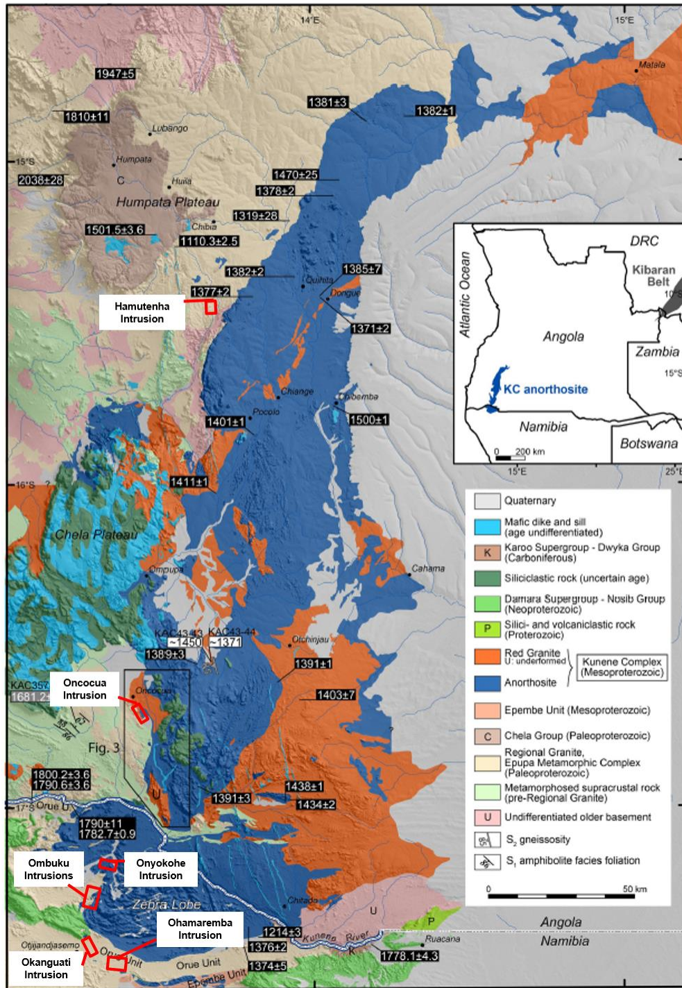
Figure 2: Geological map of the Kunene Anorthosite-Mangerite-Charnockite-Granite (AMCG) Complex showing the locations of the peripheral mafic-ultramafic intrusions (red boxes) in this study. Various ^{40}\text{Ar}/^{39}\text{Ar} ages (grey boxes) and U-Pb ages (white boxes) and age data from past publications (black boxes) are also shown. This map has been modified after Lehmann et al. (2020).
