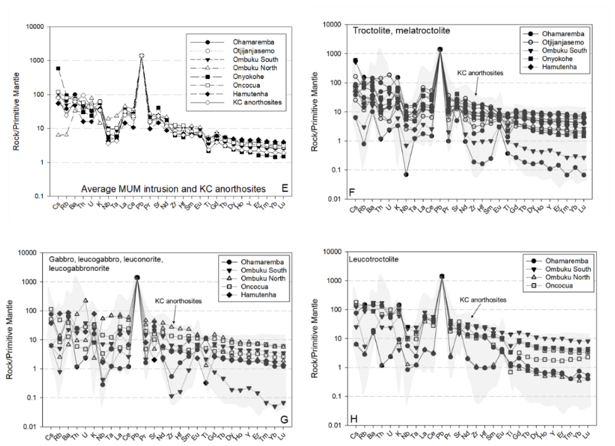
Figure 29: Primitive mantle normalised multi-element diagrams of the MUM intrusions (average values for particular rock types from each intrusion are shown in each diagram) and the KC anorthosite suite. A-D) Primitive Mantle normalised Rare Earth Element (REE) diagrams of selected samples of the MUM intrusions. E-H) Primitive Mantle normalised multi-element diagrams of selected samples of the MUM intrusions. The numbers in brackets represent the number of samples in the calculated average. The grey shaded area in each rock-type represents the range of the 25 KC anorthosite suite samples. Primitive Mantle values are from Sun & McDonough (1989).
