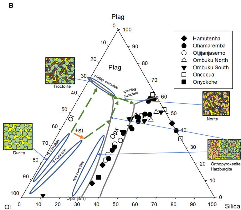
Figure 25: Whole rock data of the MUM intrusions used to determine the normative mineralogy of the samples by CIPW (Cross, Iddings, Pirsson and Washington) Norm and plotted in the ternary plots of crystallisation sequences of basaltic liquids modified from Barnes (2023) (A and B). The ellipsoidal circles are zones of cumulates (dark blue). A) Basalt Tetrahedron System of Ol-Plag-Cpx following a normal pathway of crystallisation sequences; B) Basalt Tetrahedron System Ol-Plag-Silica (silica includes Opx) of crystallisation sequences after addition of silica (e.g., Crustal input). Ol = Olivine, Plag = Plagioclase. Cpx = Clinopyroxene and Opx = Orthopyroxene.
