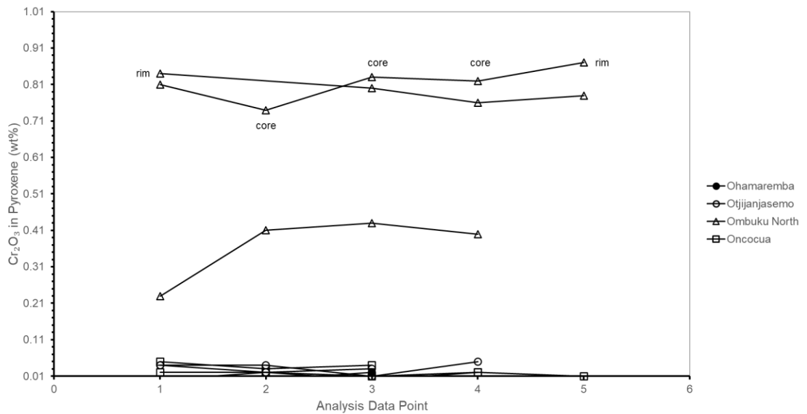
Figure 38: Chromium profiles in pyroxene grains of the MUM intrusions for chromium zoning.
