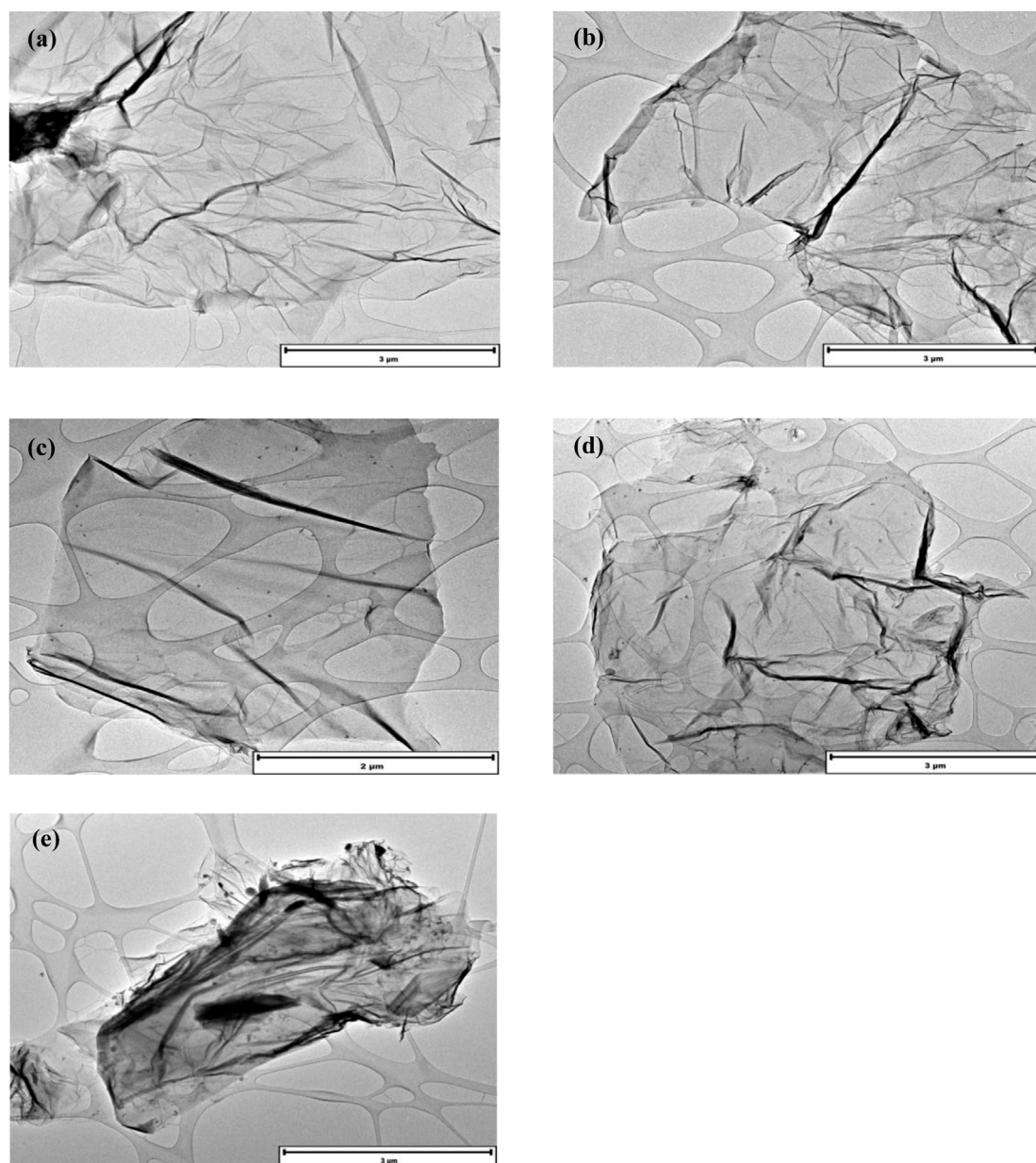
FIGURE 1 TEM images of pristine GO (a), GO-Br (b), GO-GLU 50 (c), GO-GLU 100 (d) and GO-GLU 200 (e).
