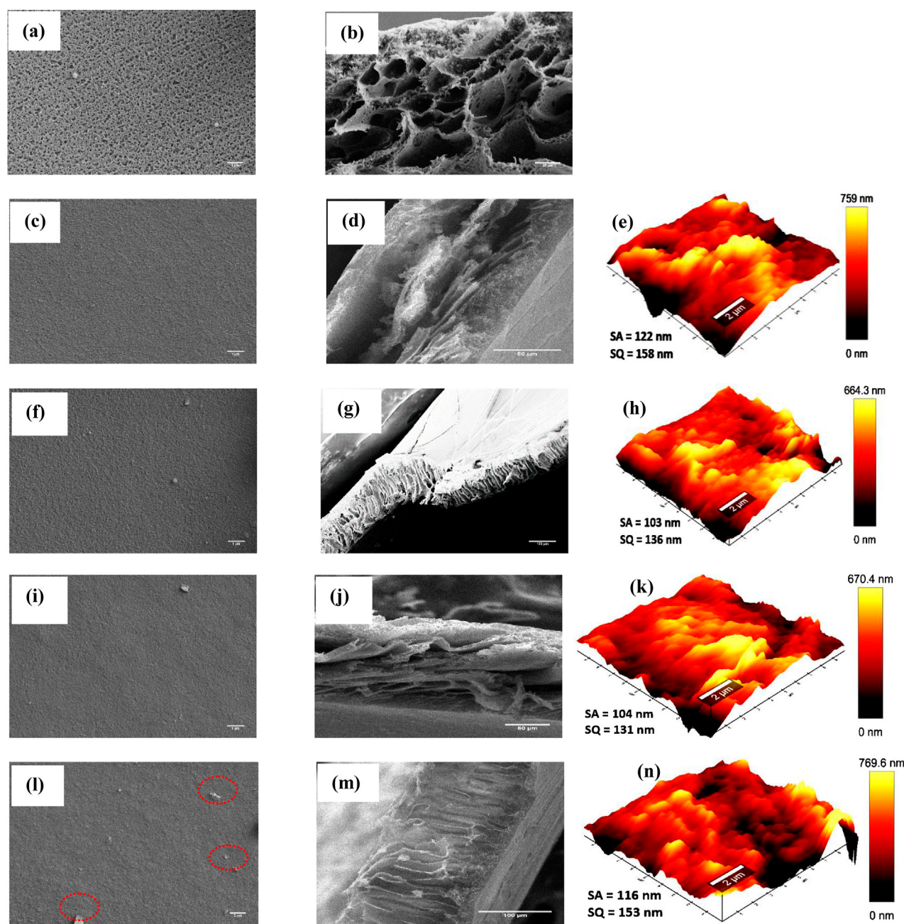
FIGURE 2 Surface, cross section morphologies and AFM images of PSF (a,b), TFC (c–e), TFN-1 (f–h), TFN-2 (i–k) and TFN-3 (l–n).
