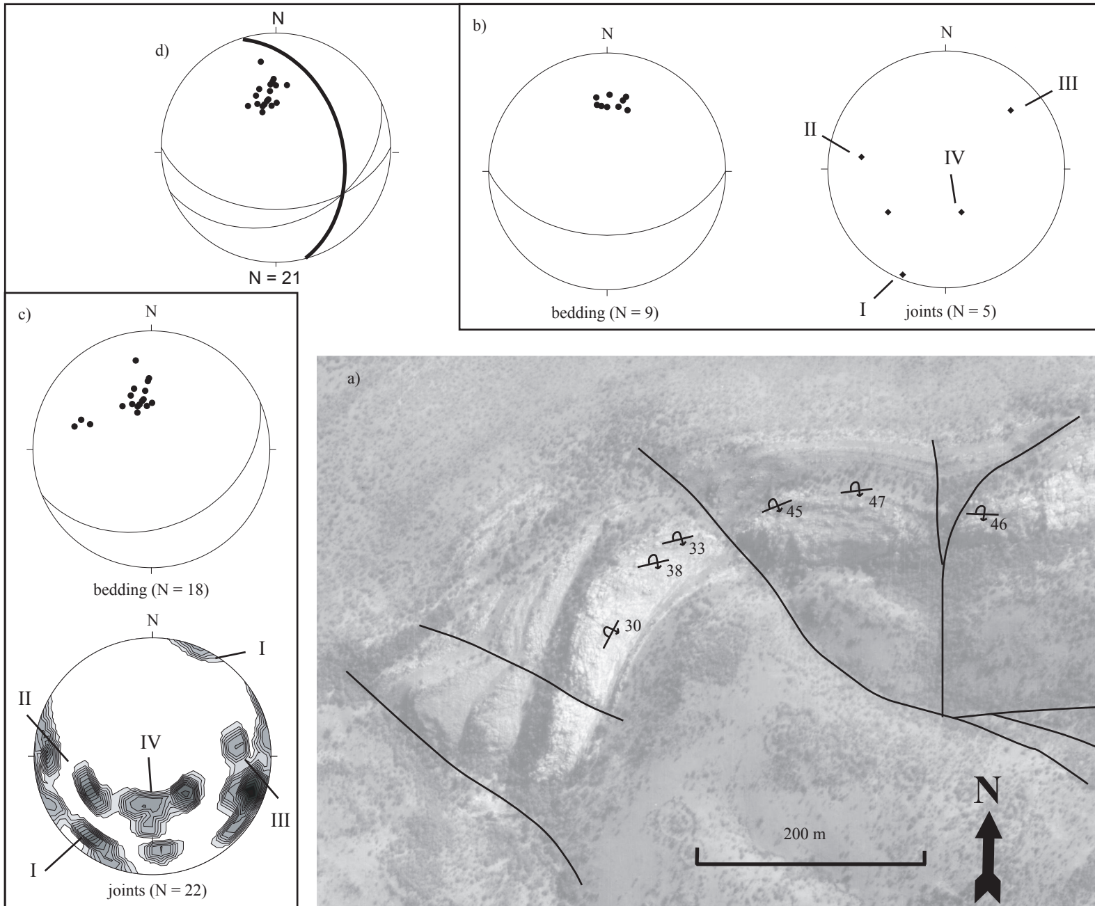
Fig. 2.16: Symmetrical fold D in the northwestern part of the collar, as mapped during this study. The fold is less faulted on the limbs than the other folds in the collar. (a) 1: 25 000 aerial photograph of the fold structure (locations 555-560, see Appendix No. 6). (b) and (c) Lower hemisphere equal area stereographic projection of the poles to bedding and the joint pattern on the northern (b) and as contour plot for joints on the western (c) limbs of the fold structure. (d) Axial plane is given as bold great circle
