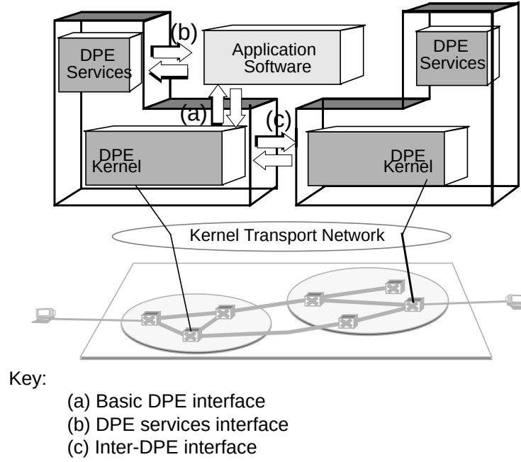
Figure 5.1: DPE Architecture
