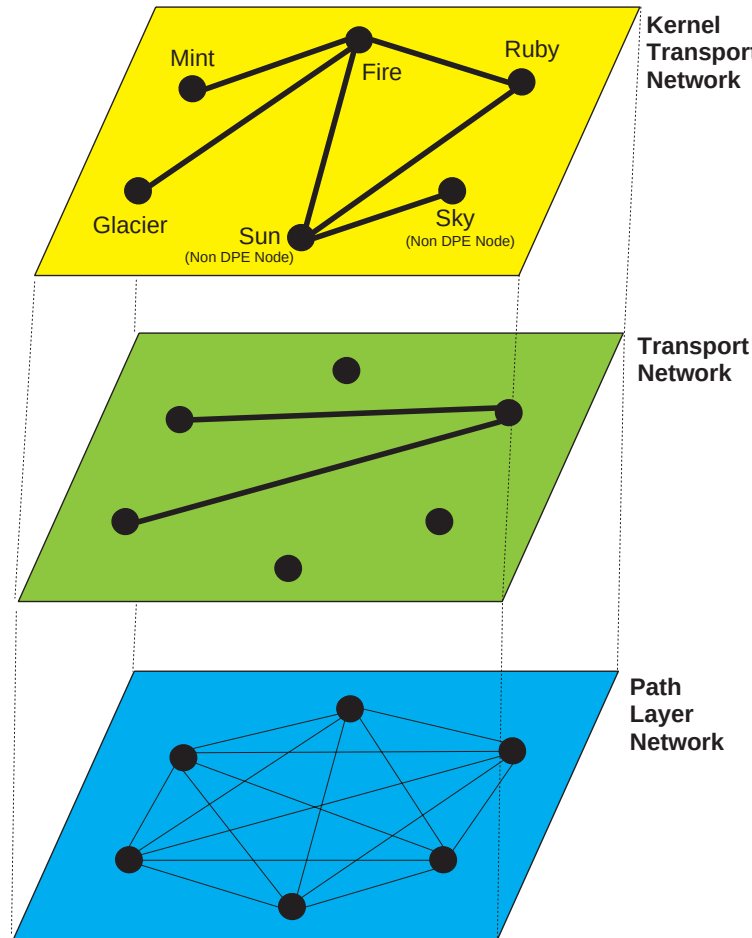
Figure 6.2: Logical Network Planes
