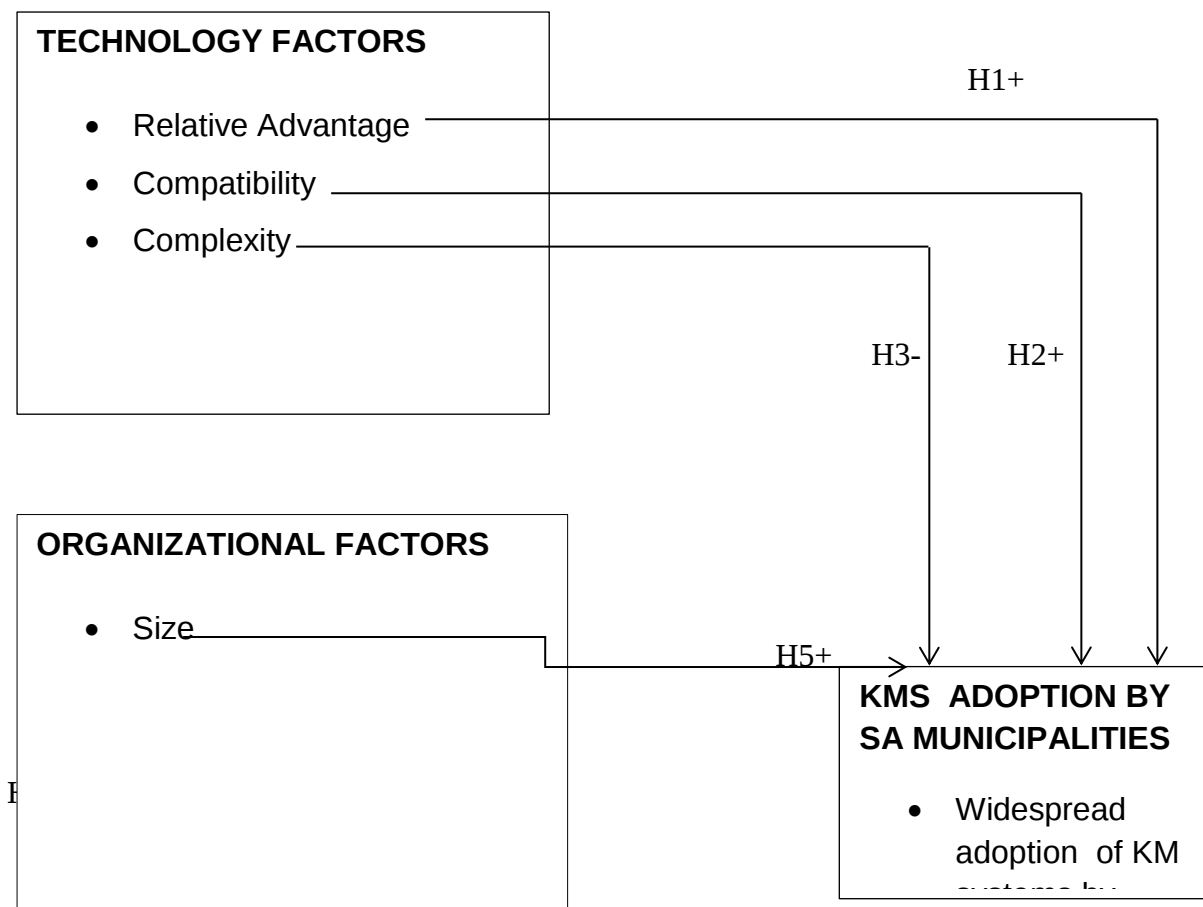
Figure 9: Supported hypotheses
