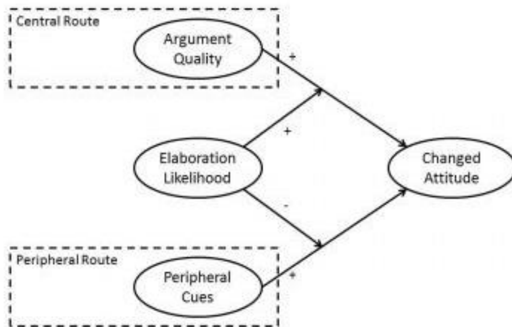
Figure 3.1: Elaboration Likelihood Model
