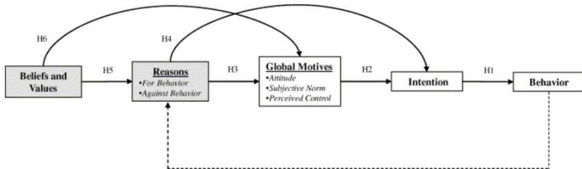
Figure 3.2: Behavioural Reasoning Model
