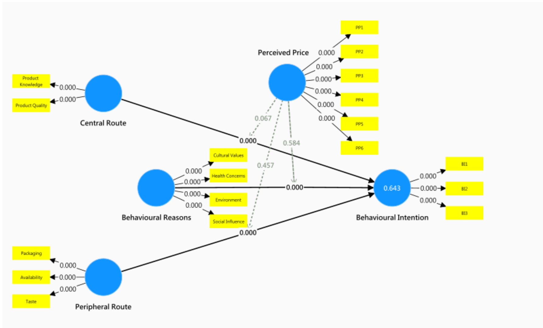
Figure 6.3: Bootstrapping Results for HOC
