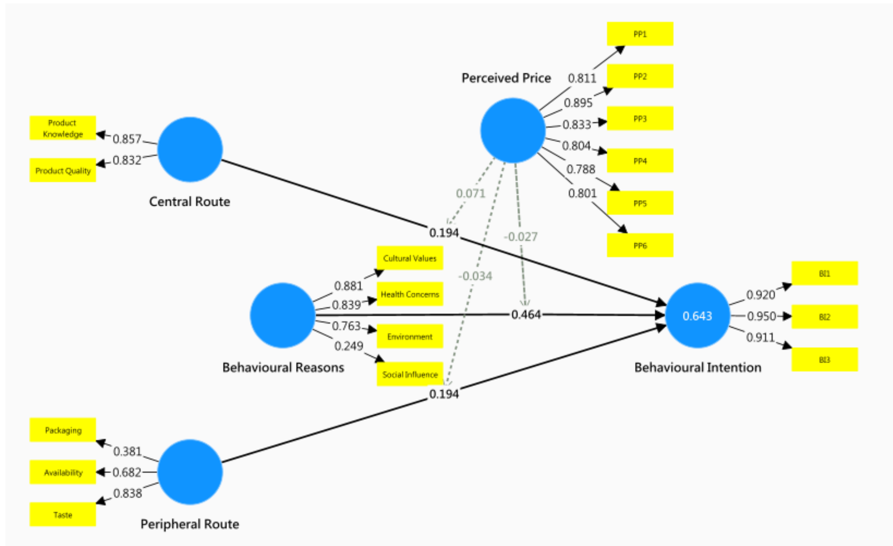
Figure 6.2: 2-Stage Disjoint Approach: Stage 2 - HOC
