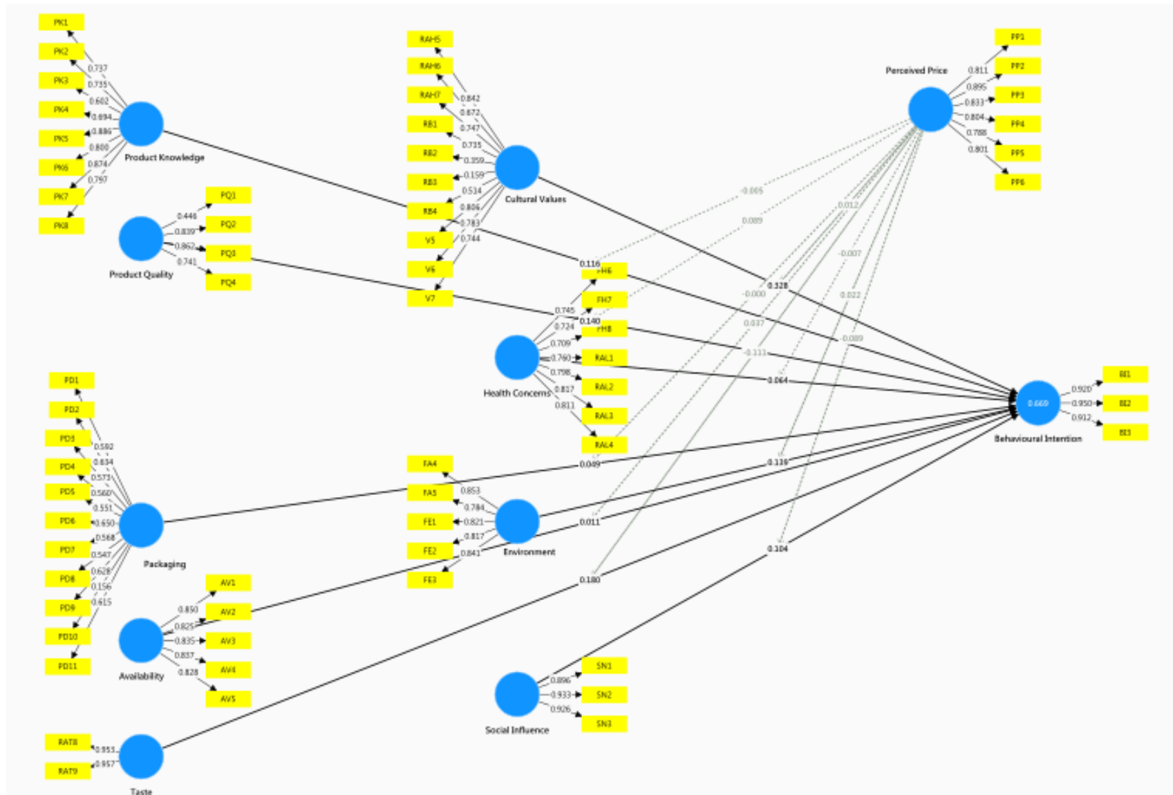
Figure 6.1: Stage 1 - Reflective Conceptual Model (LOC)
