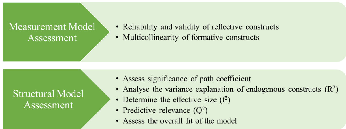
Figure 4.5: Two-Step Process of PLS-SEM Assessment
