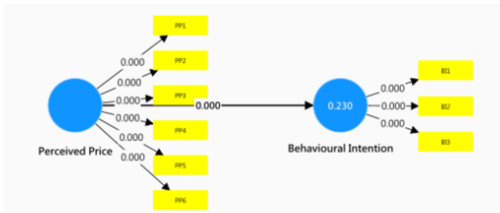
Figure 6.4: Bootstrapping Results of Perceived Price on Behavioural Intentions
