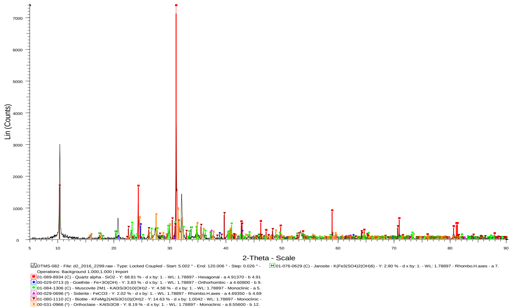
Figure 83: The result of sample DTMS-082 indicates the presents of silica, goethite, muscovite, siderite and biotite minerals.
