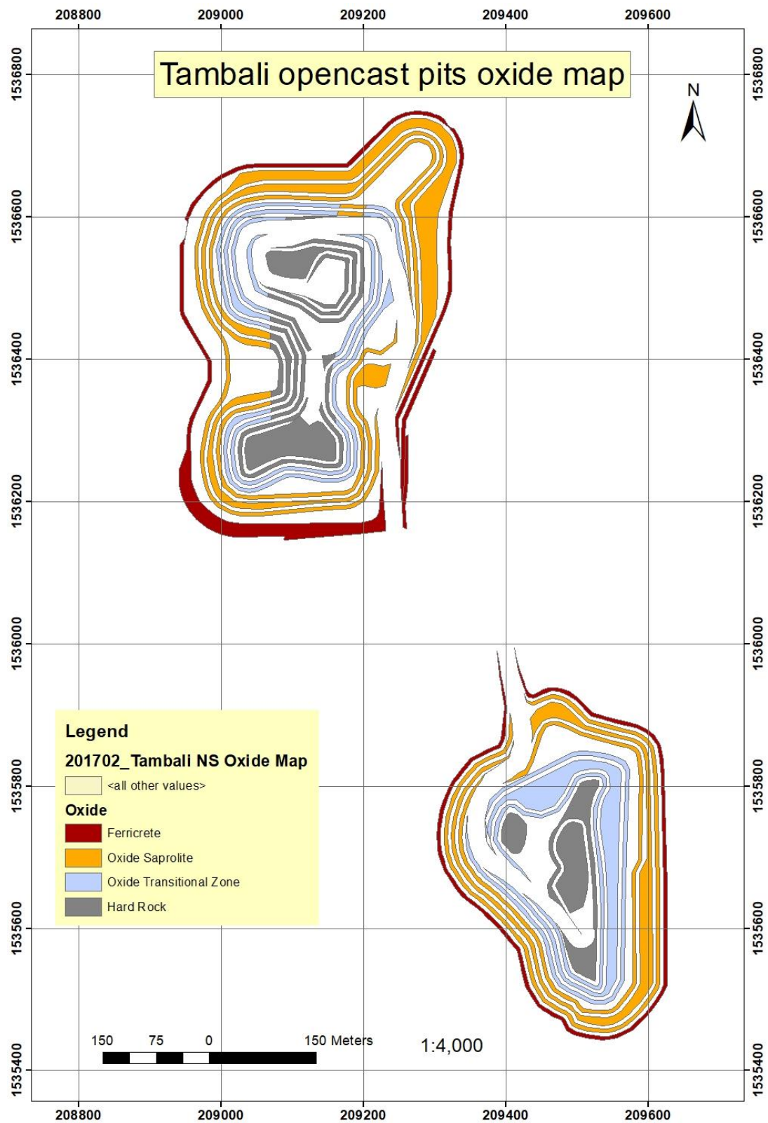
Figure 29: A plan view of oxide map for Tambali north and south pits, composed of ferricrete in red colour, the oxide saprolite, the oxide transitional zone is the light blue colour and the hard rock is represented by the grey colour.
