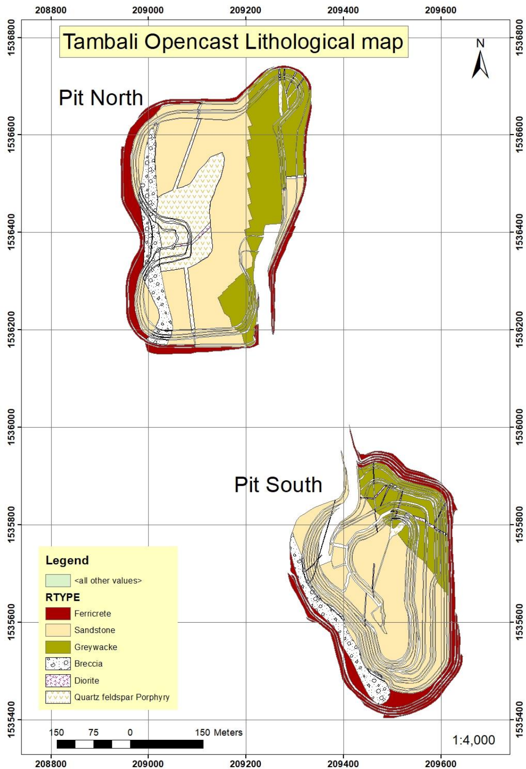
Figure 23: Lithological map of the Tambali opencast pits. The pits are composed mainly of sandstone and greywacke. The dyke of diorite and quartz-feldspar porphyry across the sedimentary rock.
