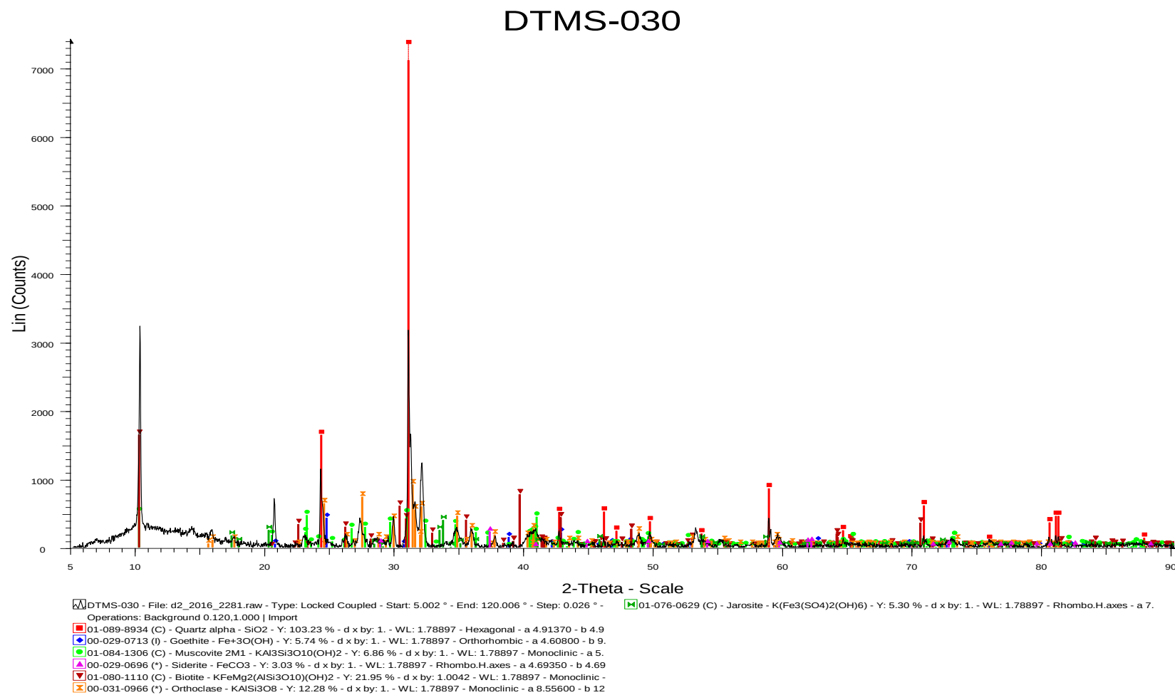
Figure 68: The result of sample DTMS-030 indicates the presents of silica, goethite, muscovite, siderite and biotite minerals.
