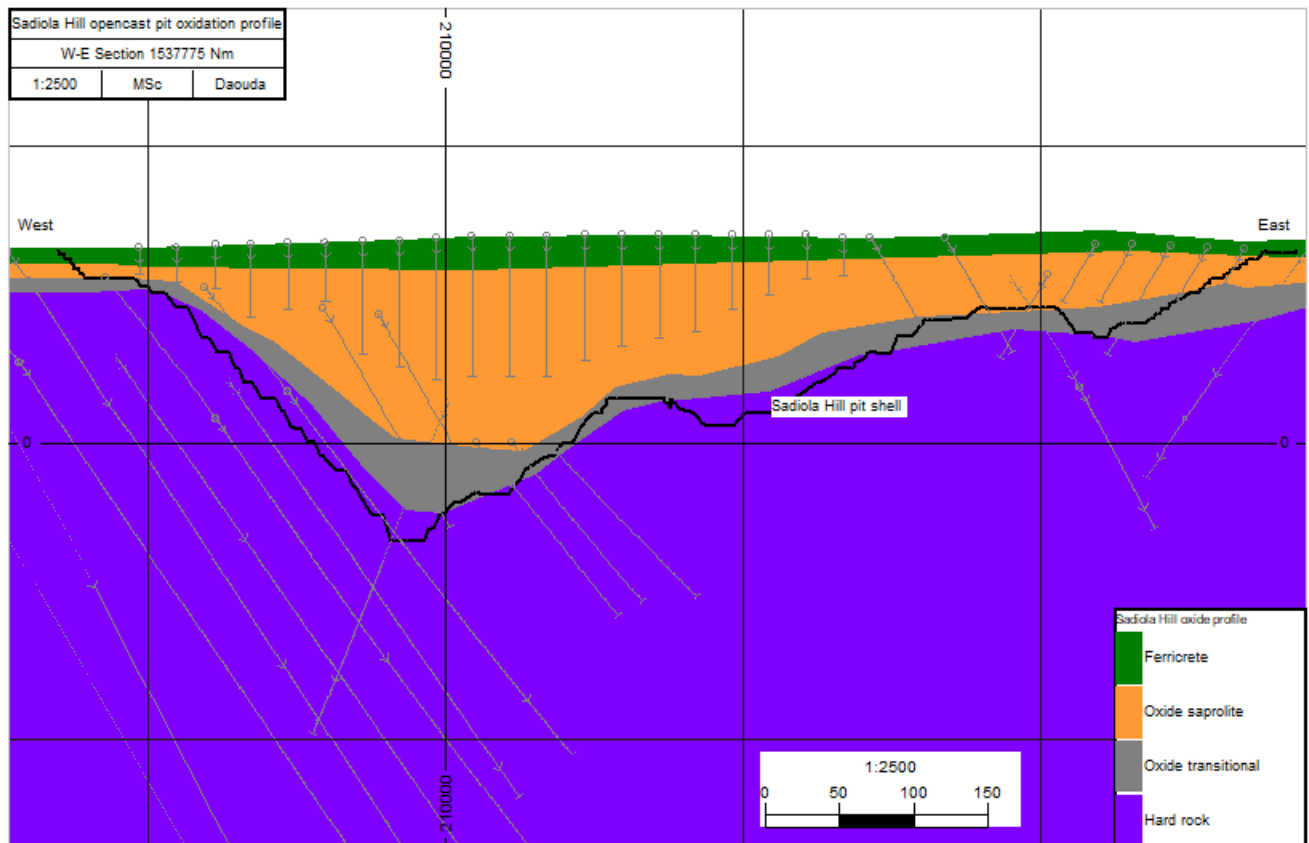
Figure 27: West-east vertical cross section along a 1537775 Nm latitude line showing the Sadiola Hill opencast oxide profile. All the four domains are well depicted from the hard rock to the ferricrete horizon.
