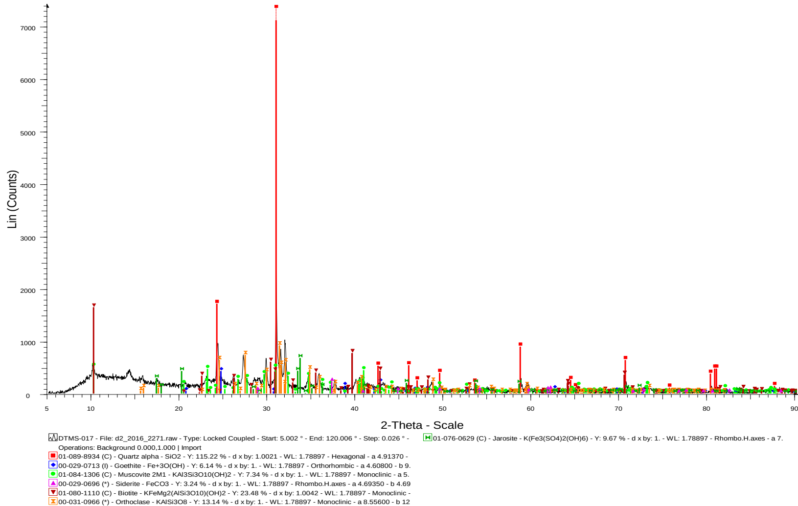
Figure 59: The result of sample DTMS-017 indicates the presents of silica, goethite, muscovite, siderite and biotite minerals.
