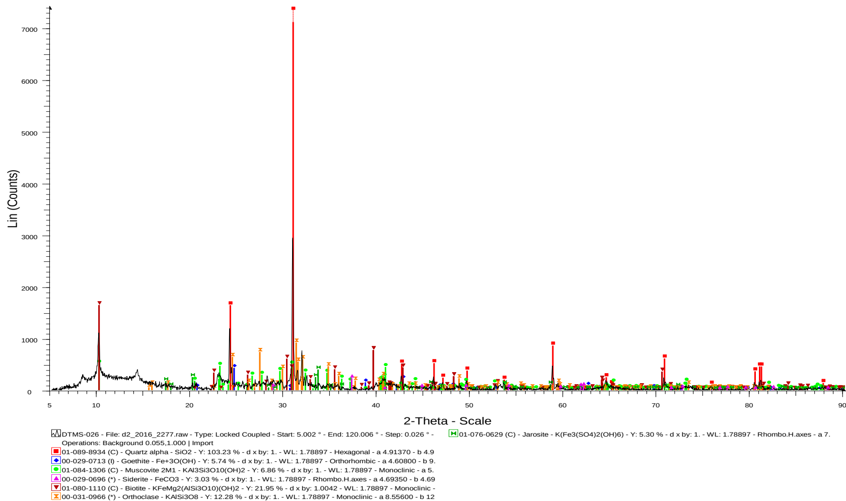
Figure 64: The result of sample DTMS-026 indicates the presents of silica, goethite, muscovite, siderite and biotite minerals.
