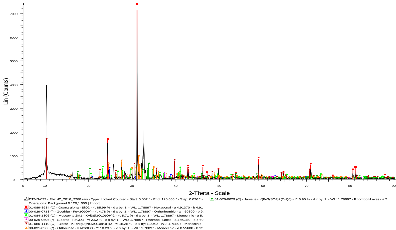
Figure 72: The result of sample DTMS-037 indicates the presents of silica, goethite, muscovite, siderite and biotite minerals.
