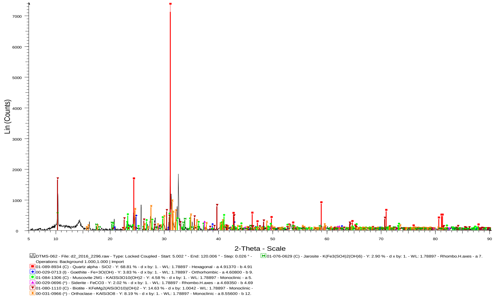
Figure 80: The result of sample DTMS-062 indicates the presents of silica, goethite, muscovite, siderite and biotite minerals.
