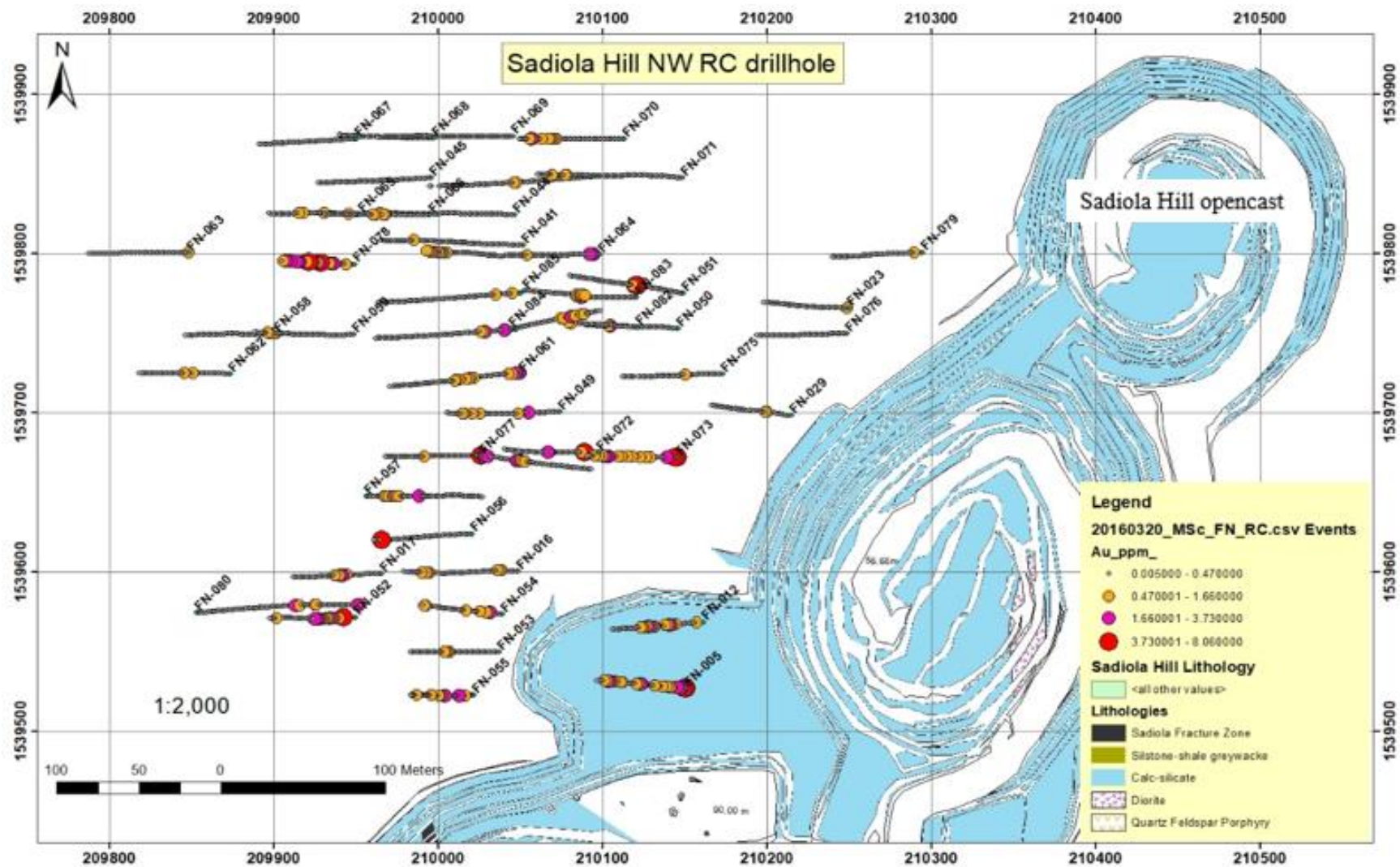
Figure 20: Position of the forty-four RC holes drilled in the Sadiola Hill NW, the holes were logged for stratigraphic definition purposes.
