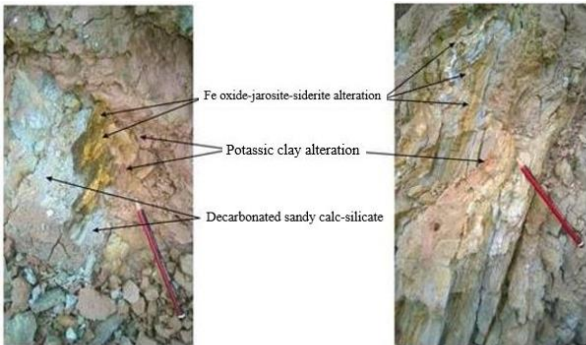
Figure 51: The three-oxide facies developed in the Sadiola Hill opencast pit. The blue colour is decarbonated calc-silicate rocks, crosscut by the red Fe-oxide alteration zones, which are in turn crosscut by zones of pink colour potassic clay alteration.
