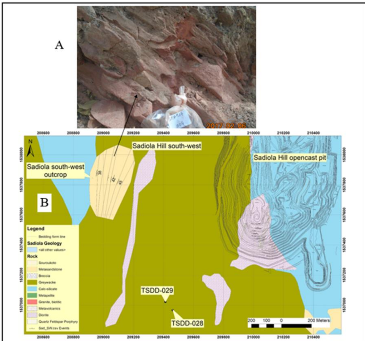
Figure 24: The red sandstone mapped at the southwest of the Sadiola Hill. (A) present the photograph of the sandstone and (B) the position of the map.
