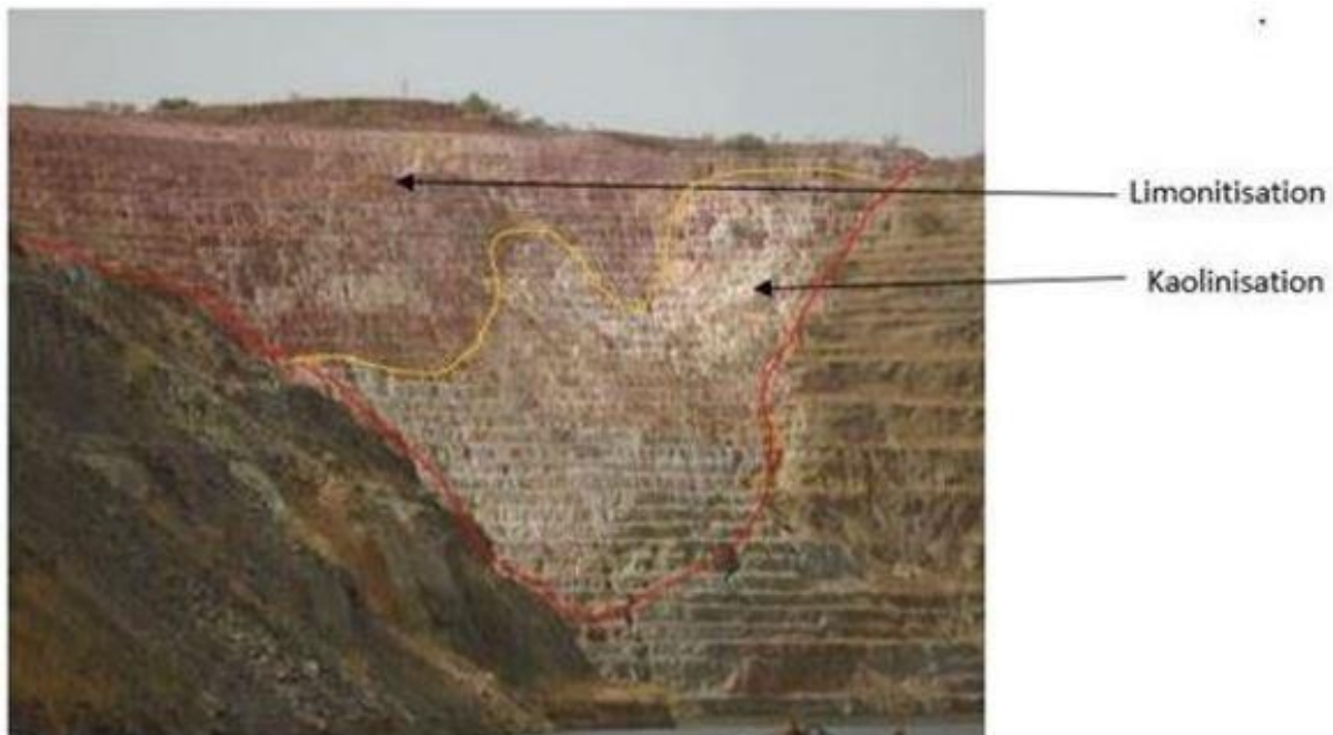
Figure 32: Photograph of the weathering profile on the southern wall of the Sadiola Hill opencast pit. The shape is presented as a funnel of the meteoric water penetration.
