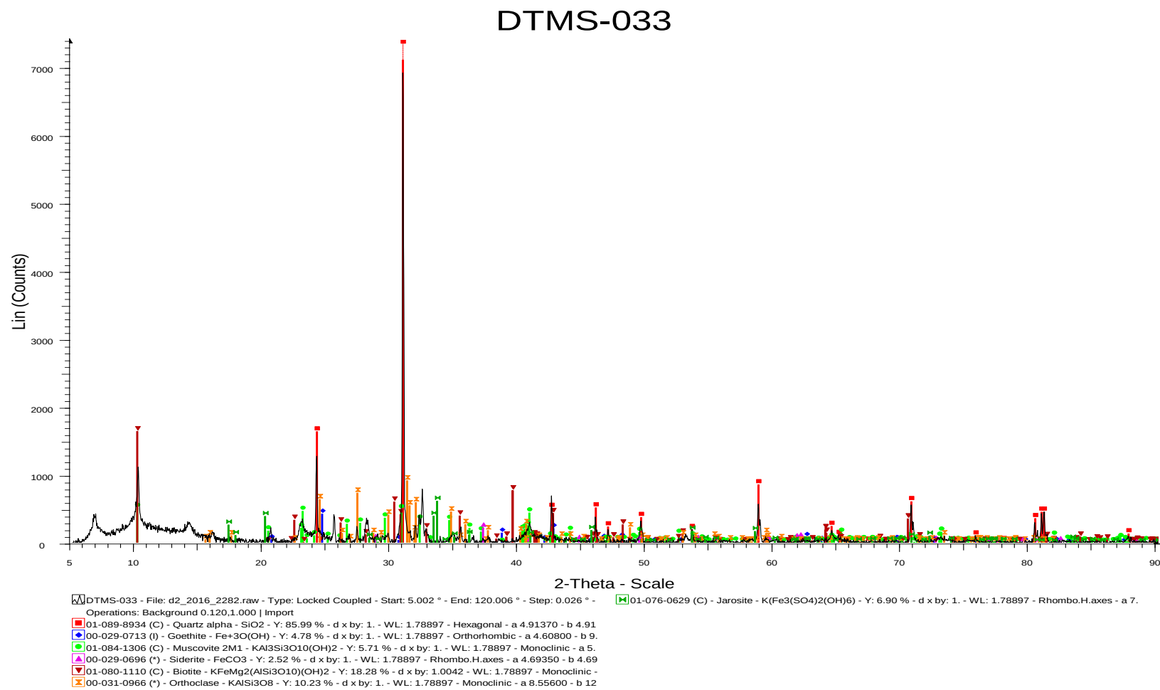
Figure 69: The result of sample DTMS-033 indicates the presents of silica, goethite, muscovite, siderite and biotite minerals.
