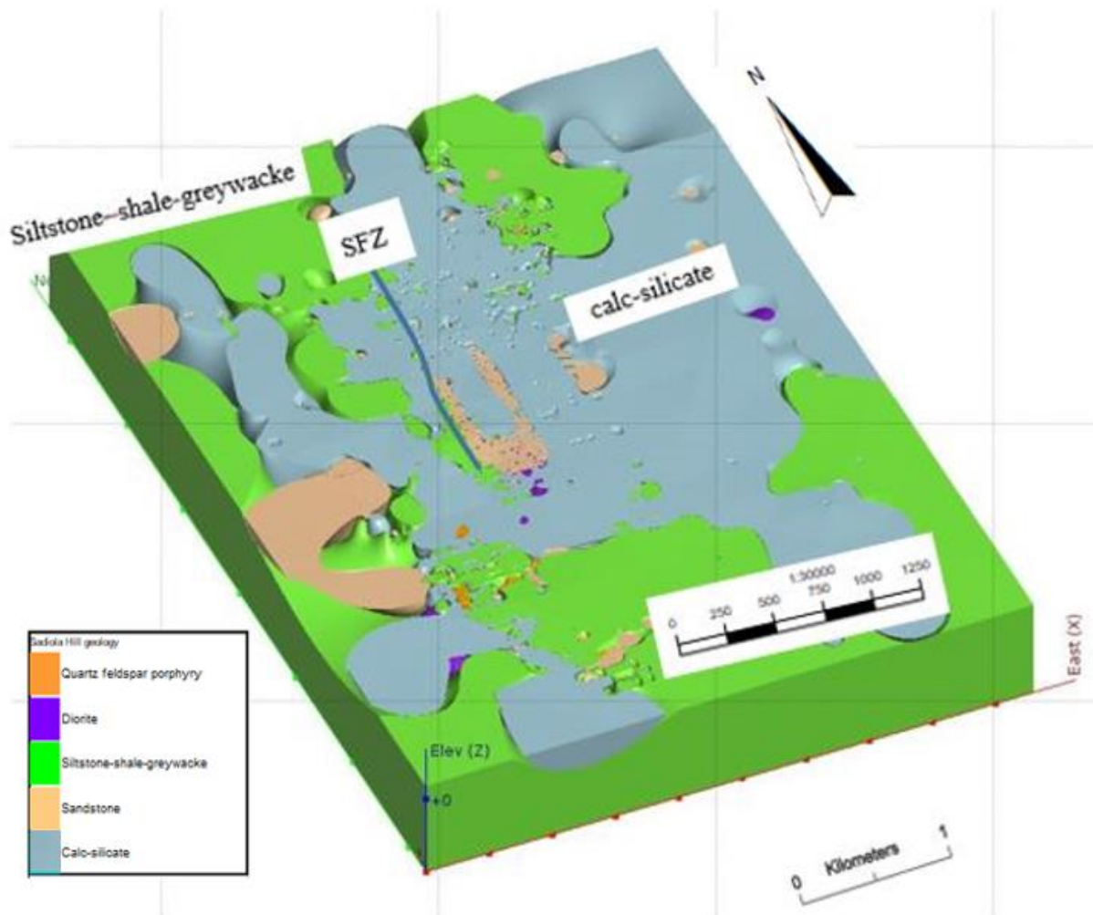
Figure 45: The 3D Sadiola goldfield lithology model. The green at the west represents the siltstone-shale-greywacke, while the calc-silicate is located mostly in the east with the blue colour.
