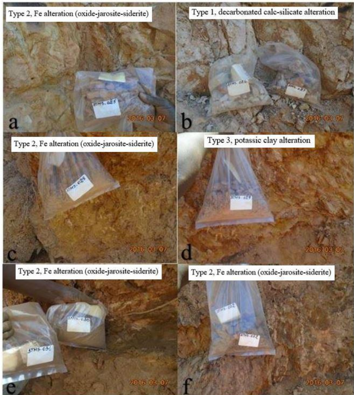
Figure 9: Photograph of the samples according to the alteration profile.
