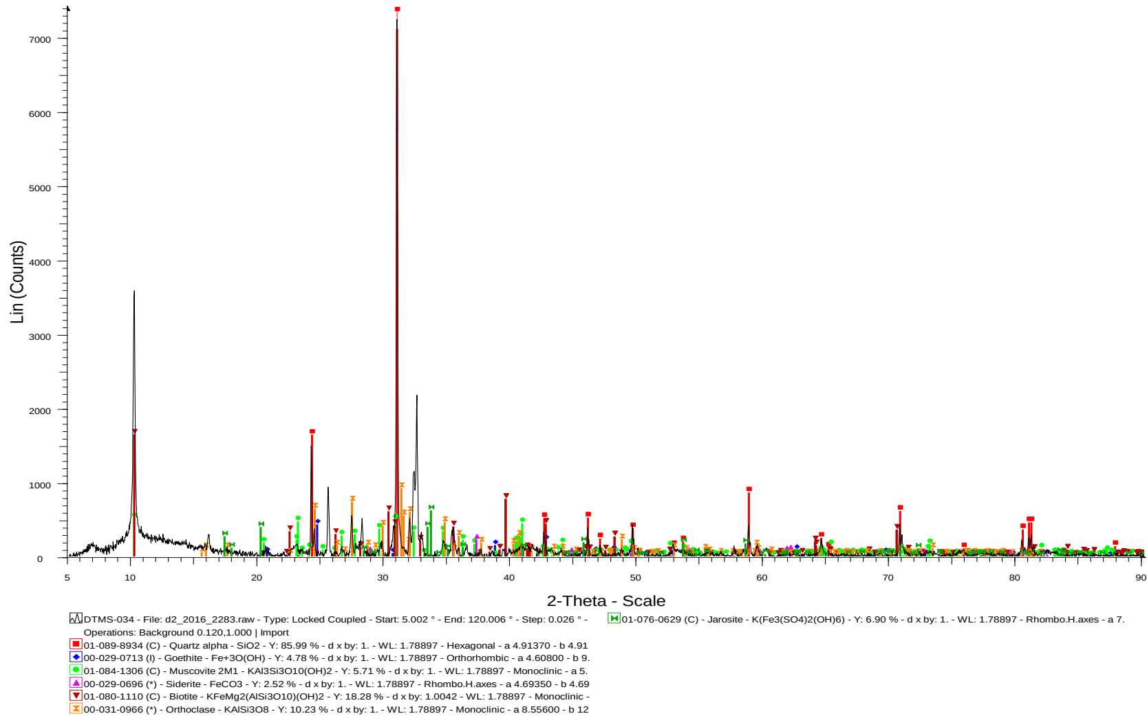
Figure 70: The result of sample DTMS-034 indicates the presents of silica, goethite, muscovite, siderite and biotite minerals.
