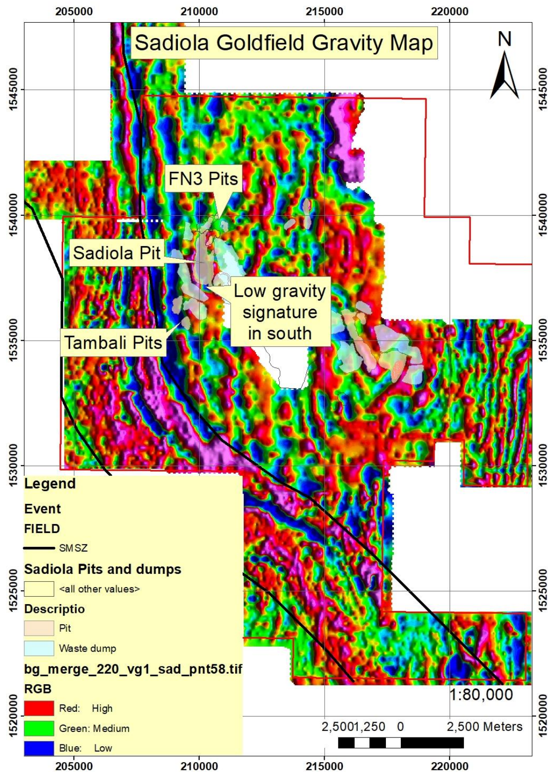
Figure 17: Sadiola goldfield regional gravity map. The blue colour represents low gravity, while the red the high gravity. Each open cast pit is located on area of low gravity, where oxides are
