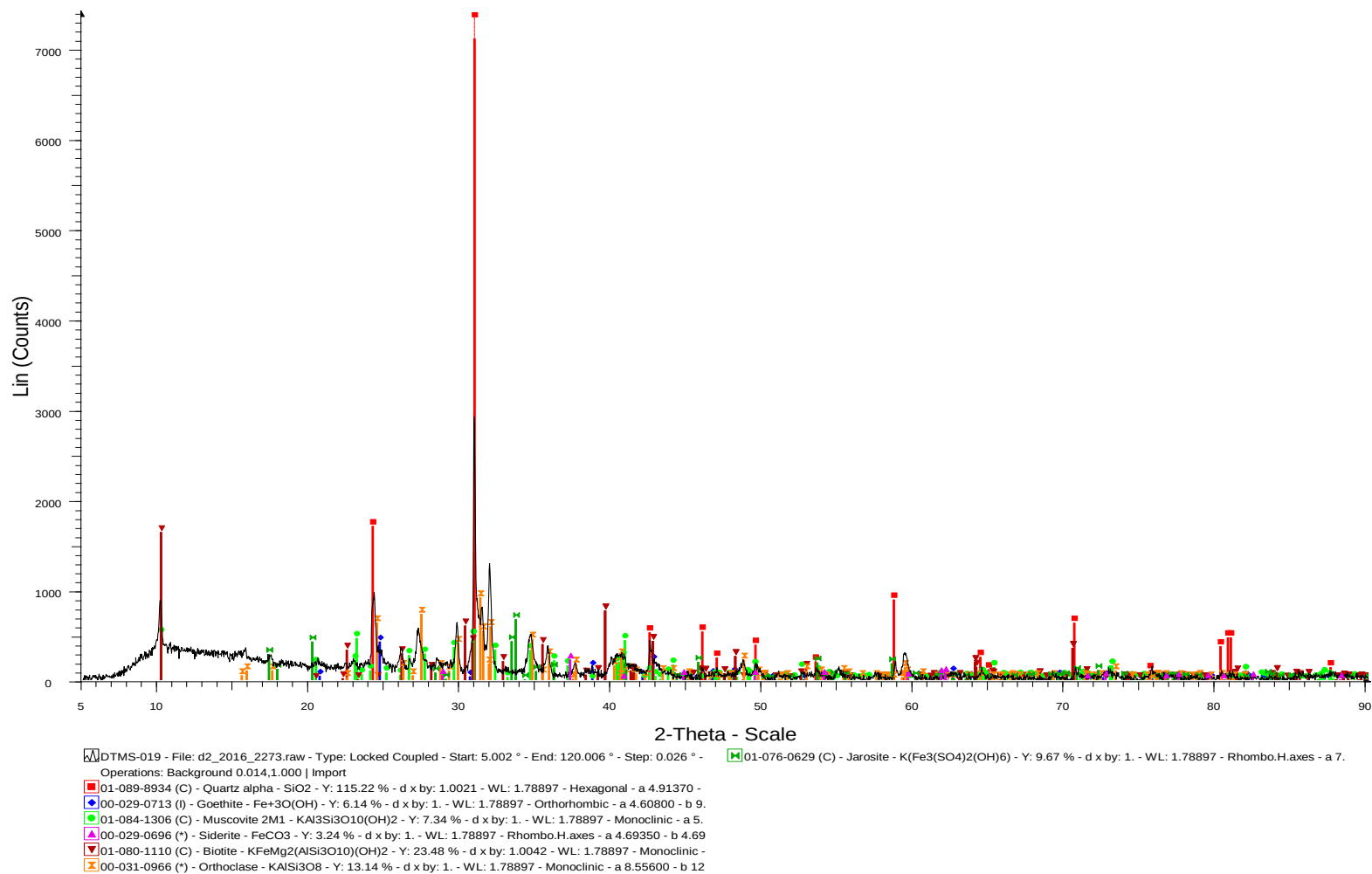
Figure 61: The result of sample DTMS-019 indicates the presents of silica, goethite, muscovite, siderite and biotite minerals.
