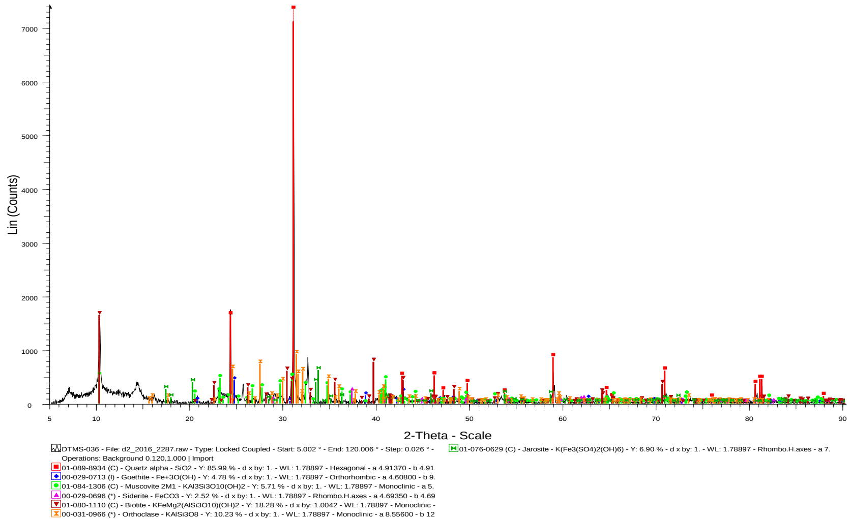
Figure 71: The result of sample DTMS-036 indicates the presents of silica, goethite, muscovite, siderite and biotite minerals.
