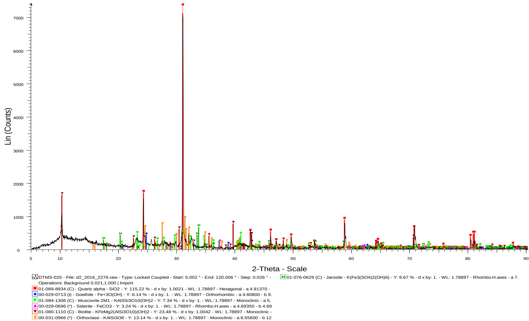
Figure 63: The result of sample DTMS-025 indicates the presents of silica, goethite, muscovite, siderite and biotite minerals.
