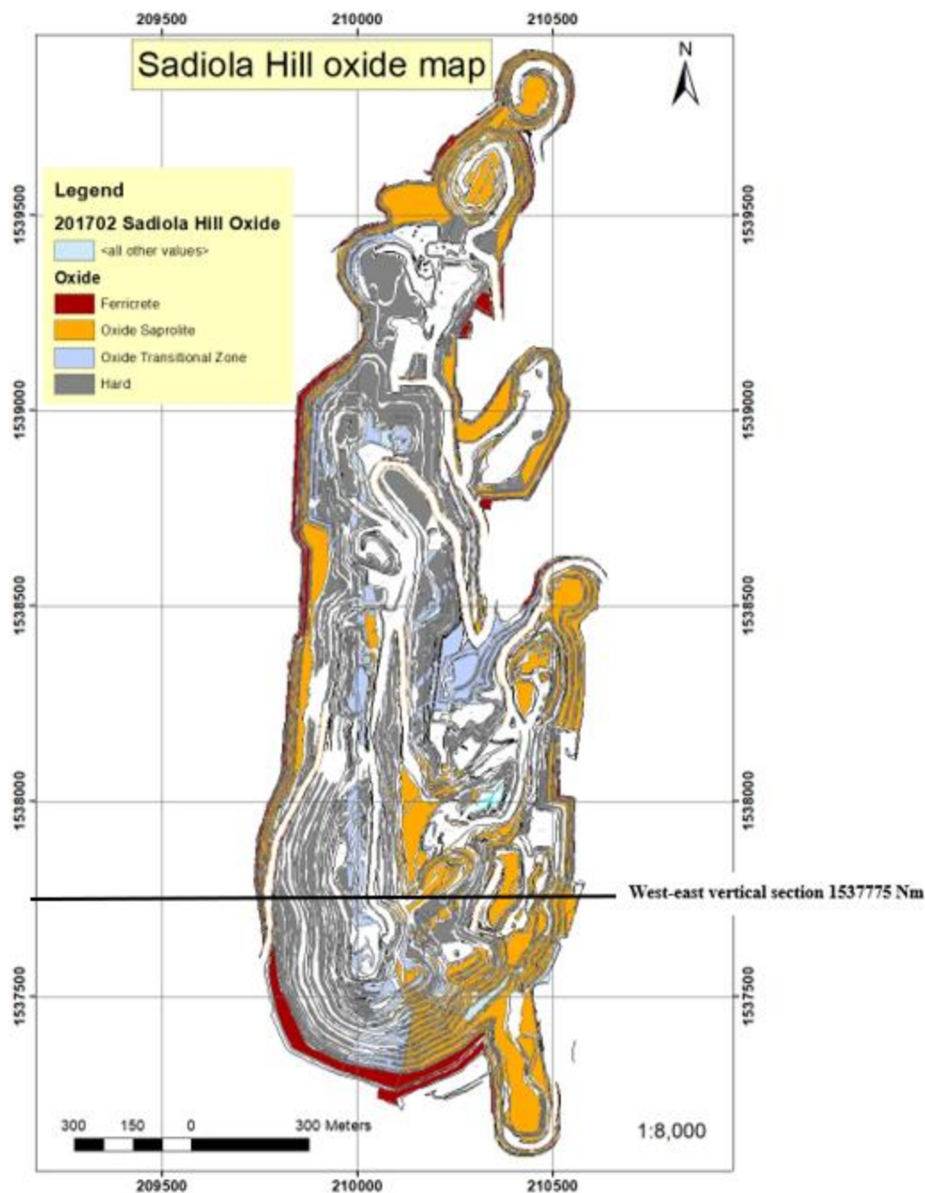
Figure 30: The oxide map of the Sadiola Hill opencast pit, composed of ferricrete in red colour, the oxide saprolite, the oxide transitional zone is the light blue colour and the hard rock in grey colour.
