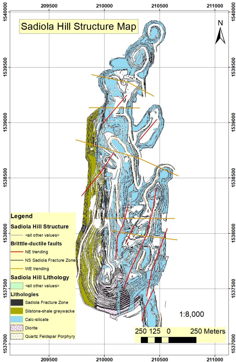
Figure 41: The SFZ, northeast trending faults and west east trending faults plotted on the Sadiola Hill opencast pit geological map. The SFZ is located along the contact between the siltstone-shale-greywacke in the west and the calc-silicate in the east.
