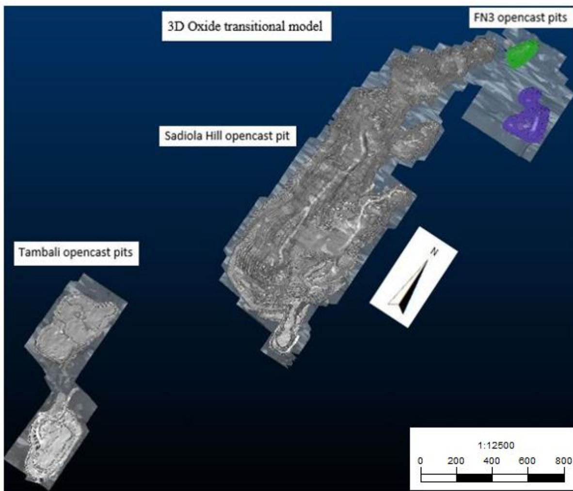
Figure 48: The 3D oxide transitional zone for Sadiola goldfield (FN3 in the northern, Sadiola Hill open cast in the middle, and the Tambali pits in the southern part).
