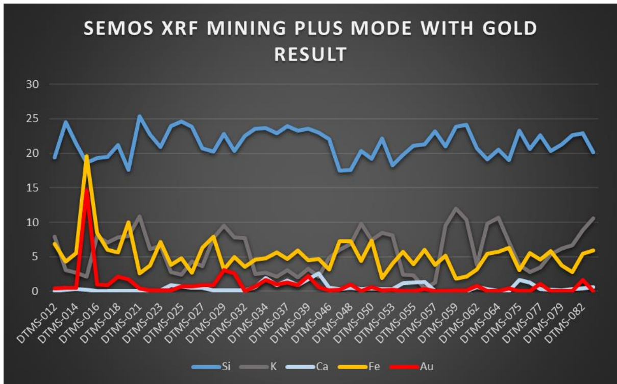
Figure 52: Diagram of SEMOS XRF “Mining Plus” showing silica (Si), potassium (K), calcium (Ca), and the iron (Fe) with gold result. There is a strong correlation, between gold and iron alteration and a second correlation with Au and potassium K, while no correlation with calcium (Ca) was examined due to the absence or weakness of Ca due to the oxidation.
