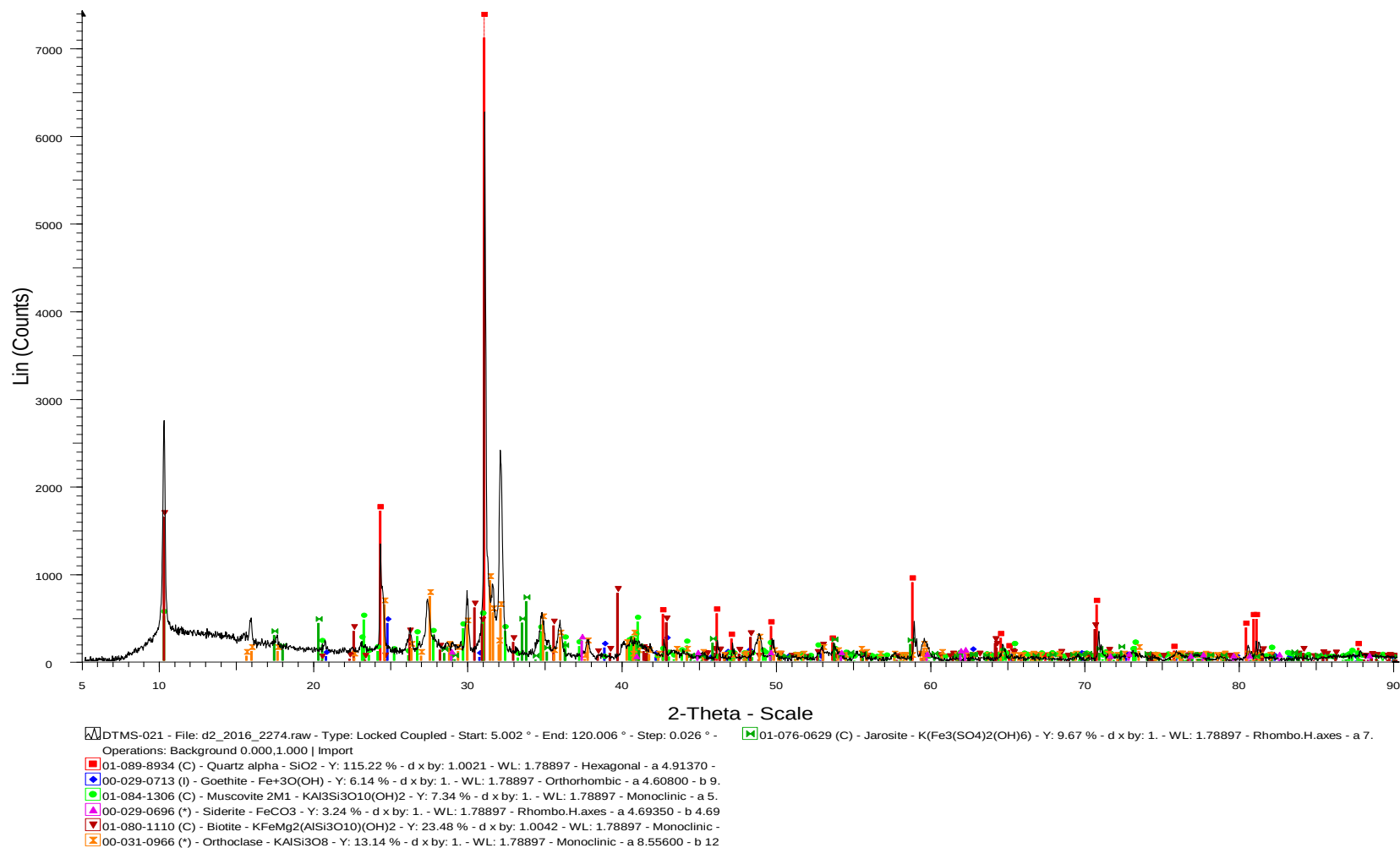
Figure 62: The result of sample DTMS-021 indicates the presents of silica, goethite, muscovite, siderite and biotite minerals.
