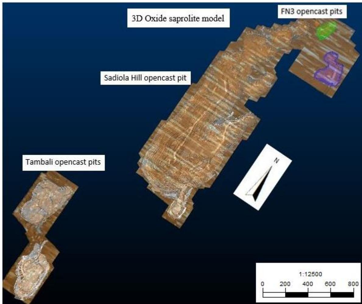
Figure 47: The 3D oxide saprolite model for Sadiola goldfield (FN3 in the northern, Sadiola Hill open cast in the middle, and the Tambali pits in the southern).
