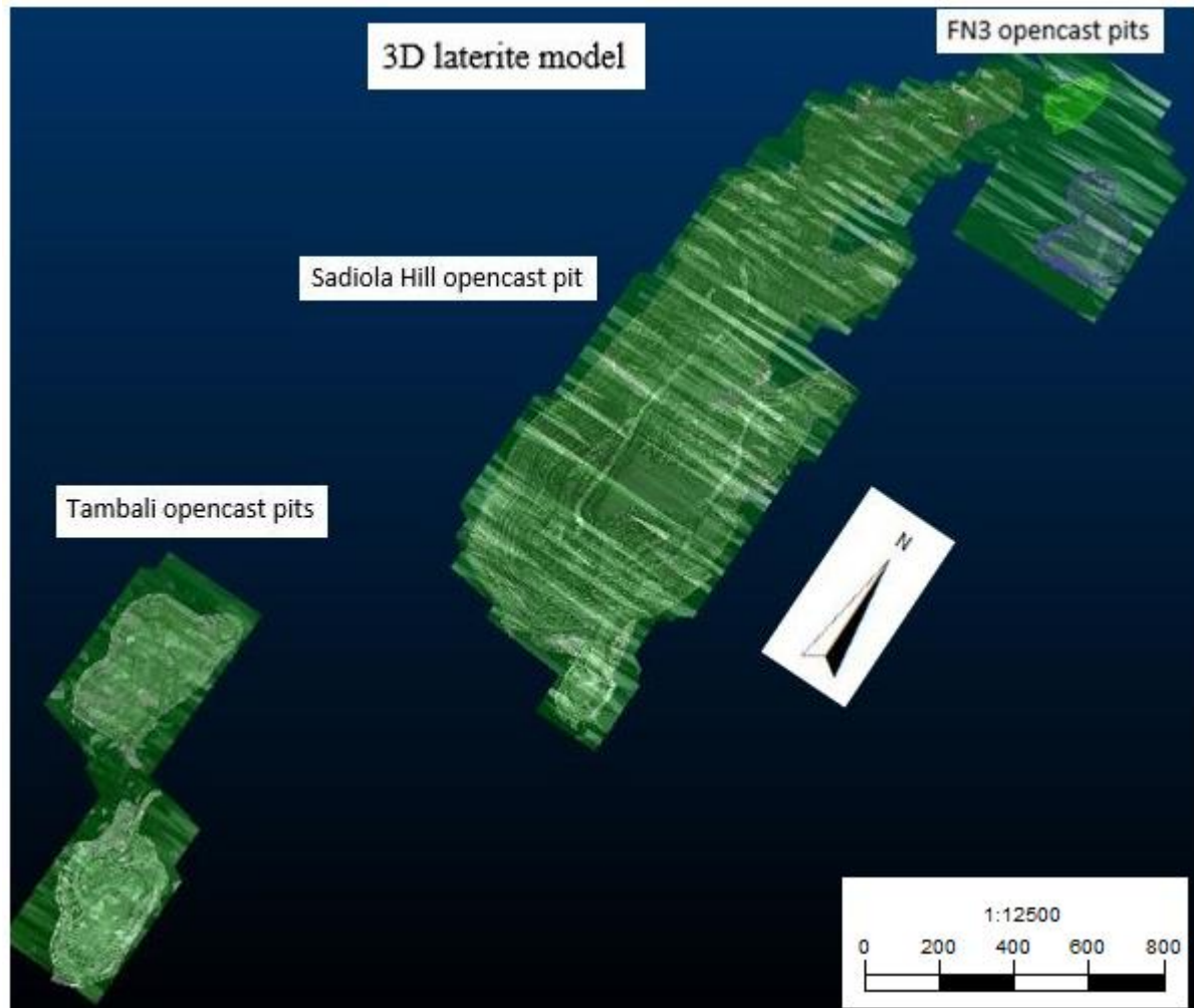
Figure 46: The 3D laterite model for Sadiola goldfield (FN3 in the northern, Sadiola Hill open cast in the middle, and the Tambali pits in the southern part).
