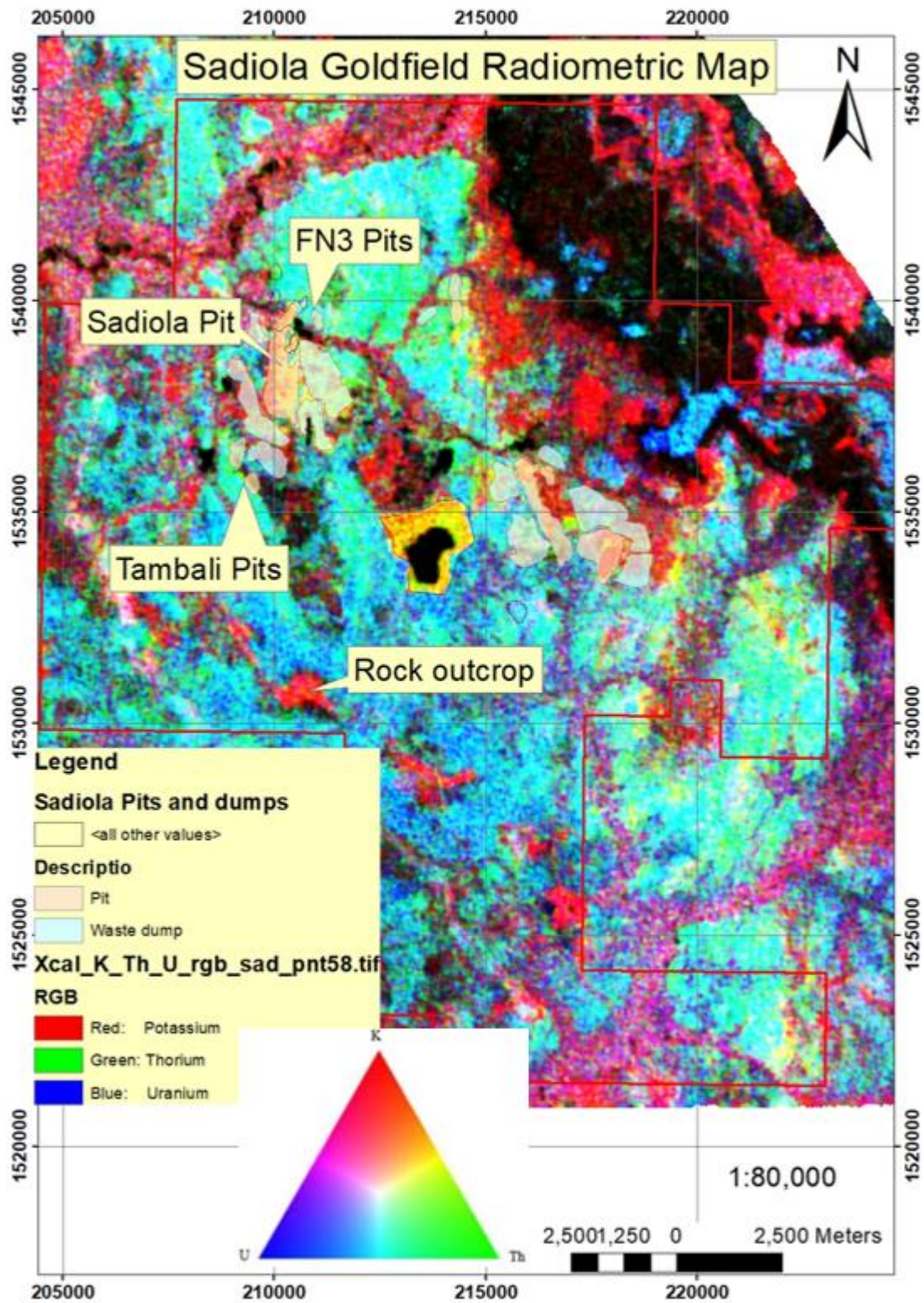
Figure 19: The regional radiometric data across the Sadiola goldfield. The blue light colour shows the ferricrete which cover most parts of the goldfield. The red colour represents some outcrop through the goldfield.
