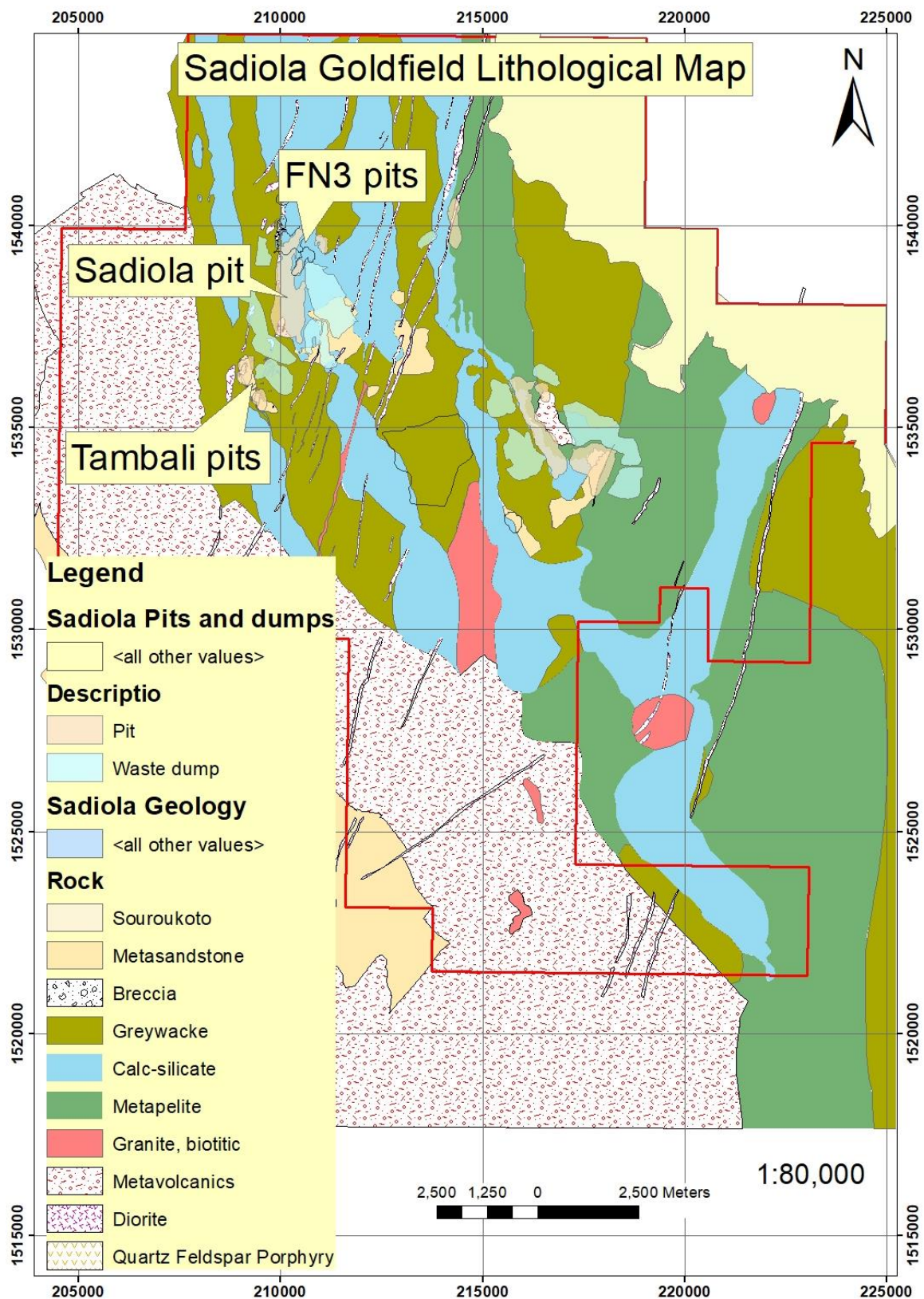
Figure 6: Sadiola goldfield local geological map, this map is established by a compilation of the field mapping and drilling data.
