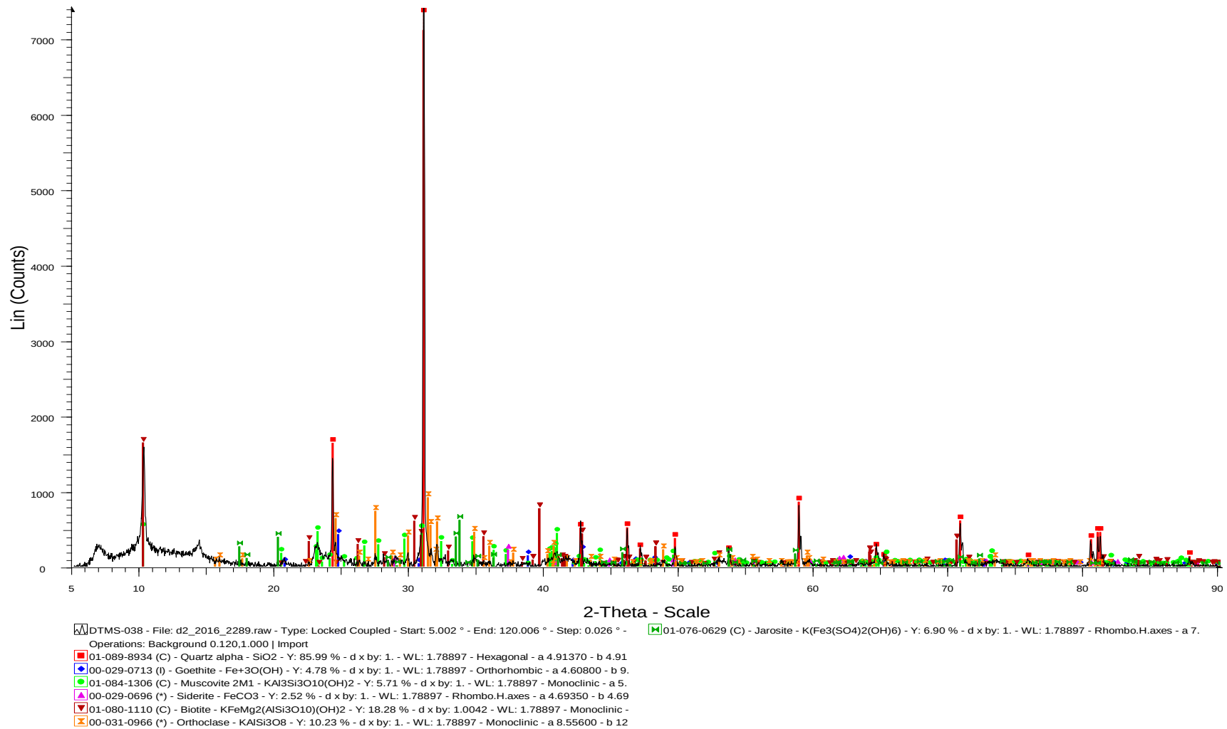
Figure 73: The result of sample DTMS-038 indicates the presents of silica, goethite, muscovite, siderite and biotite minerals.
