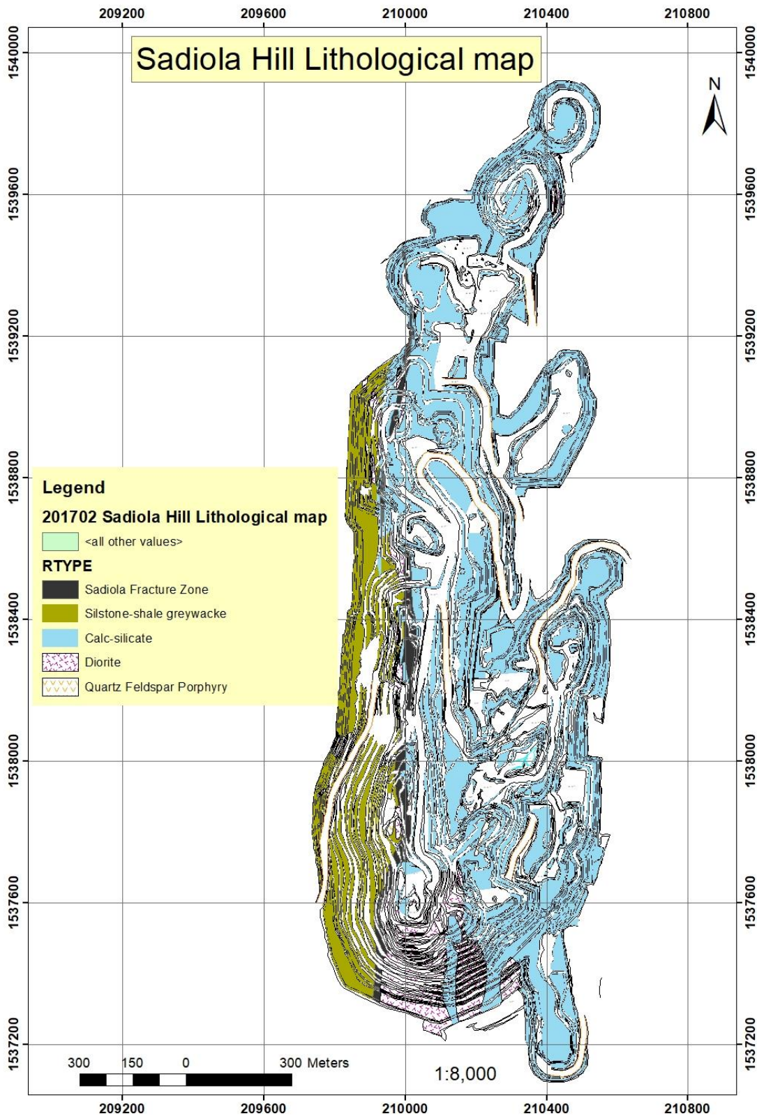
Figure 22: Sadiola Hill opencast pit geological map. The eastern part of the pit is the altered and unaltered calc-silicate, while the western part is the siltstone-shale greywacke. The contact is structurally defined by the SFZ. The sedimentary rocks are cross cut by a dyke and sill of diorite and quartz-feldspar porphyry dyke.
