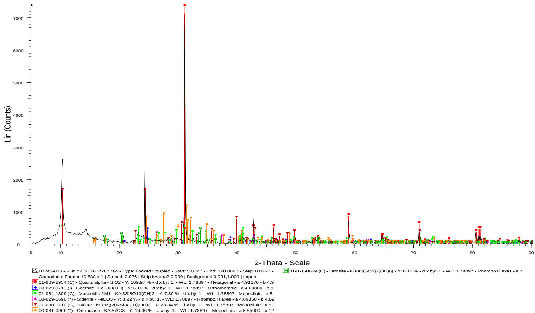
Figure 55: The result of sample DTMS-013 contains silica, goethite, muscovite, siderite and biotite minerals.
