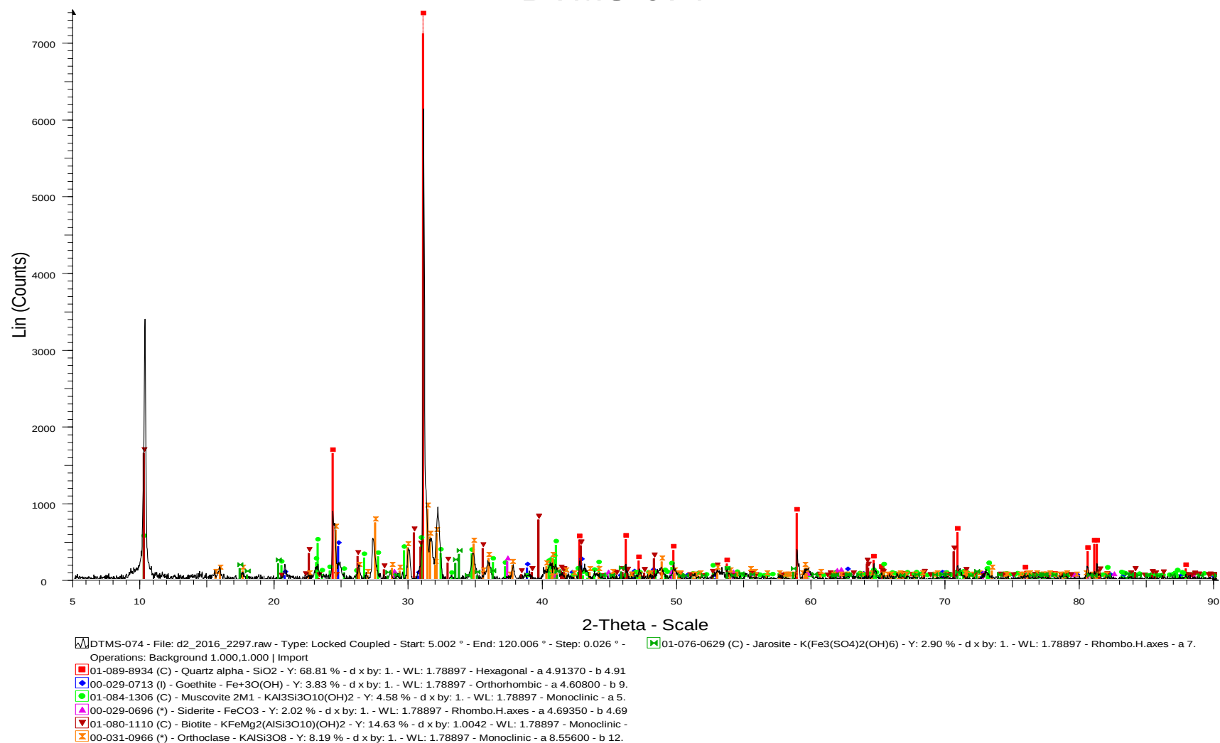
Figure 81: The result of sample DTMS-074 indicates the presents of silica, goethite, muscovite, siderite and biotite minerals.
