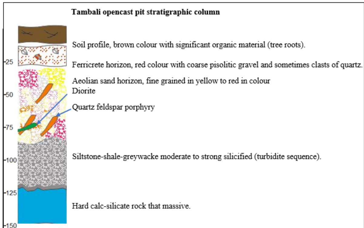
Figure 35: Tambali opencast pit stratigraphic column. The column was established by the compilation of the pit mapping data and RC and diamond). drilling data.
