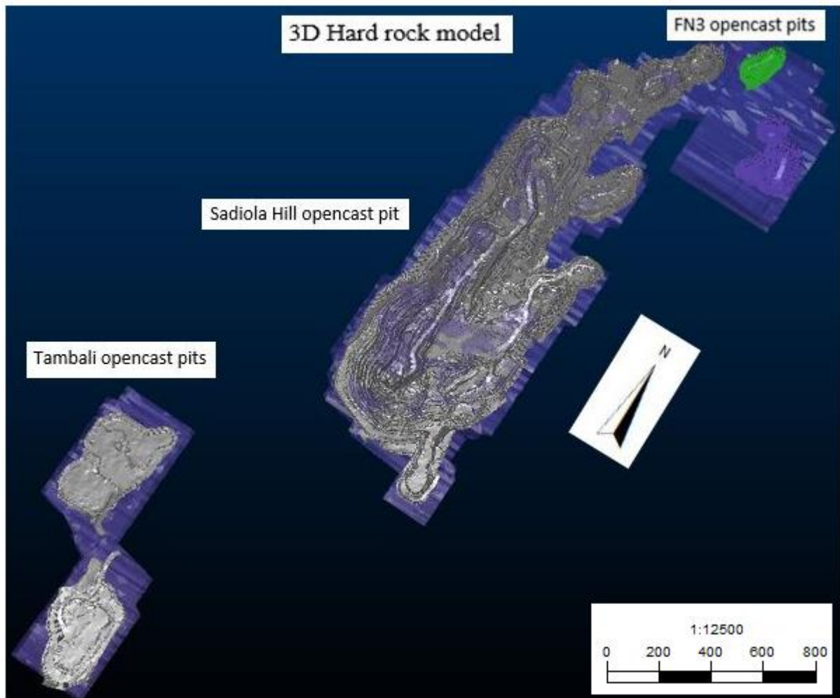
Figure 49: The 3D hard rock model for Sadiola goldfield (FN3 in the northern, Sadiola Hill open cast in the middle, and the Tambali pits in the south).
