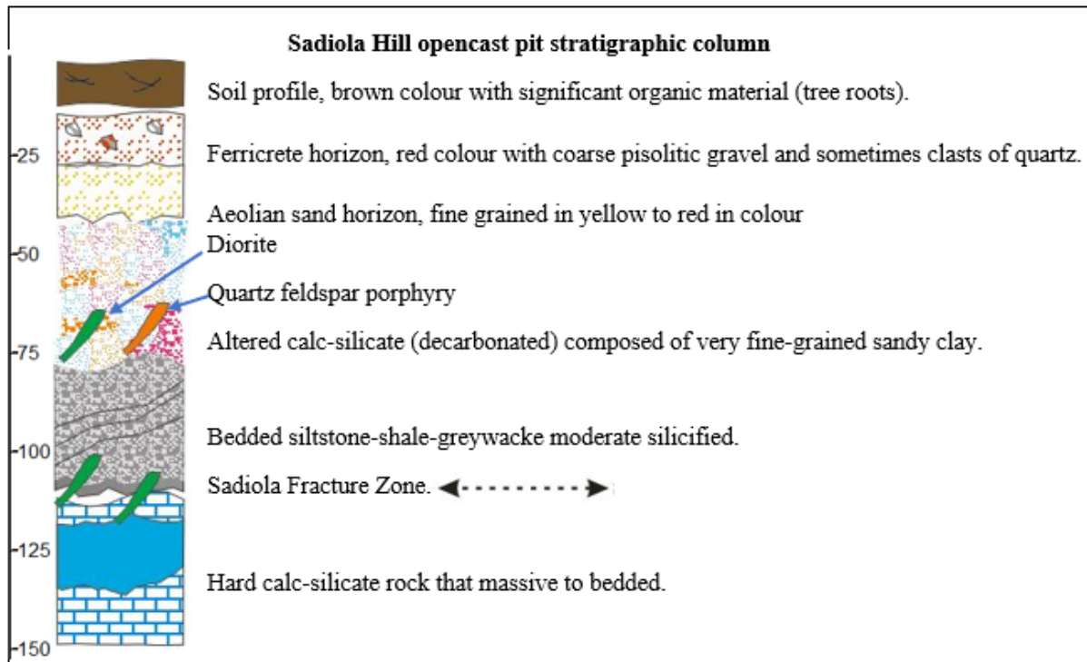
Figure 34: Sadiola Hill opencast stratigraphic column. The column was established by the compilation of the pit mapping data and RC and diamond drilling data.
