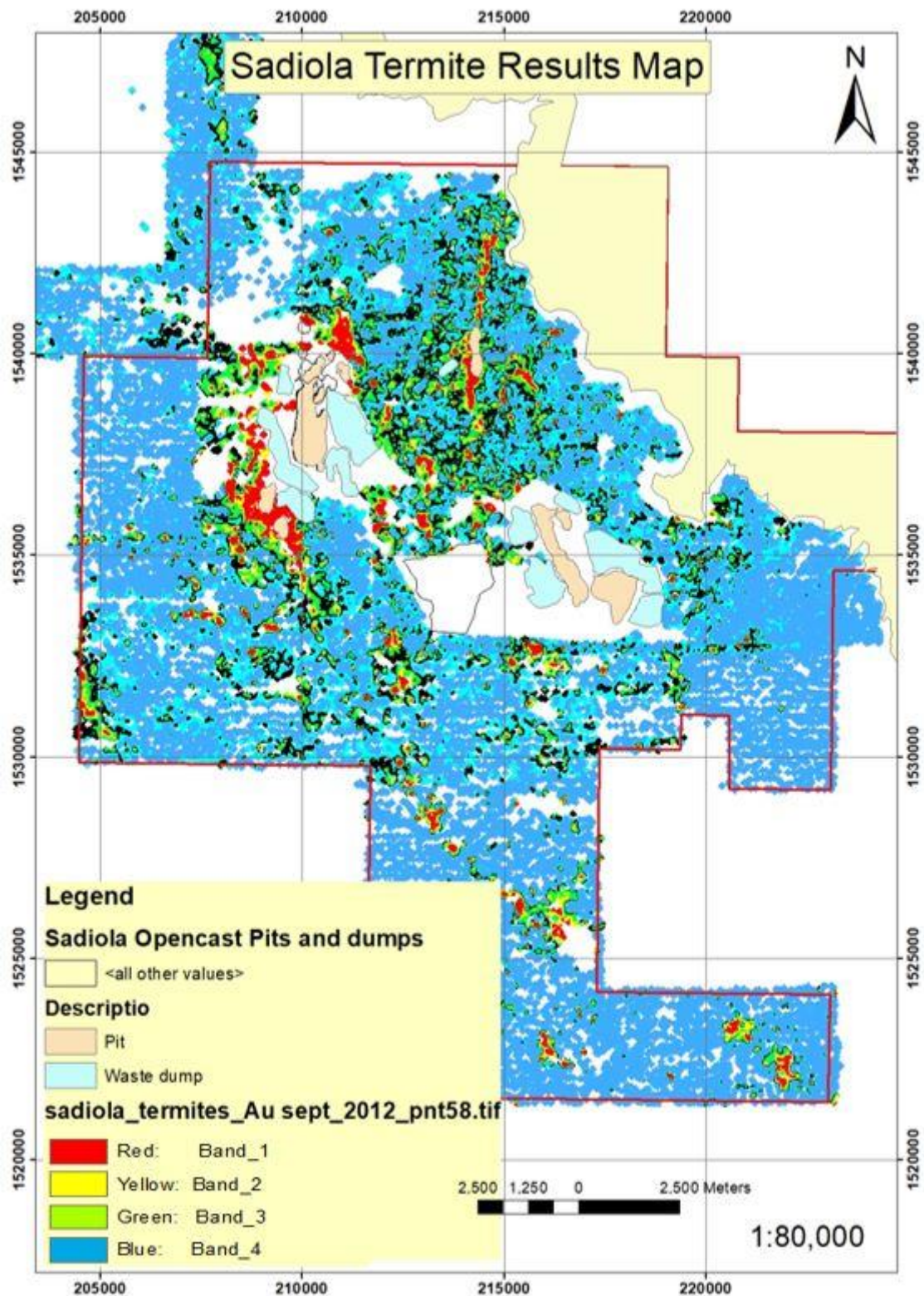
Figure 36: Map of termite mounds sample result in the Sadiola exploration permit. The red (high value), (2) yellow (medium), (3) green (Low) and (4) blue (zero) of gold. This value is overprinted on each open cast pit in the Sadiola goldfield.
