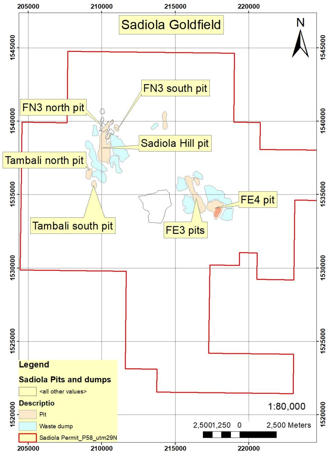
Figure 2: Sadiola goldfield with ancillary opencast pits. Each pit is indicated by its name. The pits shapes were plotted in the ArcGIS to represent their position in the Sadiola district.
