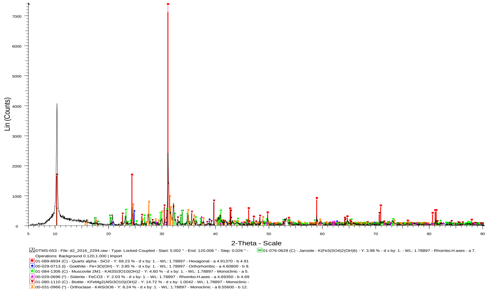
Figure 78: The result of sample DTMS-053 indicates the presents of silica, goethite, muscovite, siderite and biotite minerals.
