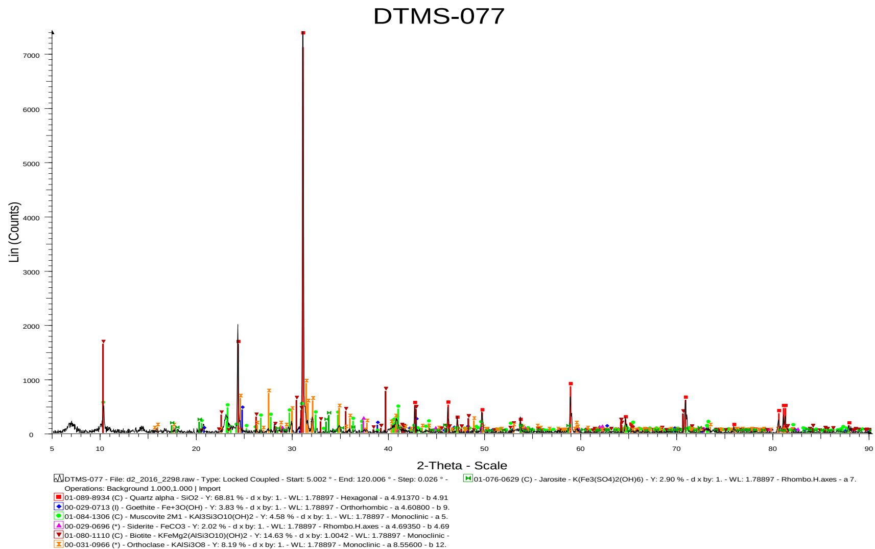
Figure 82: The result of sample DTMS-077 indicates the presents of silica, goethite, muscovite, siderite and biotite minerals.
