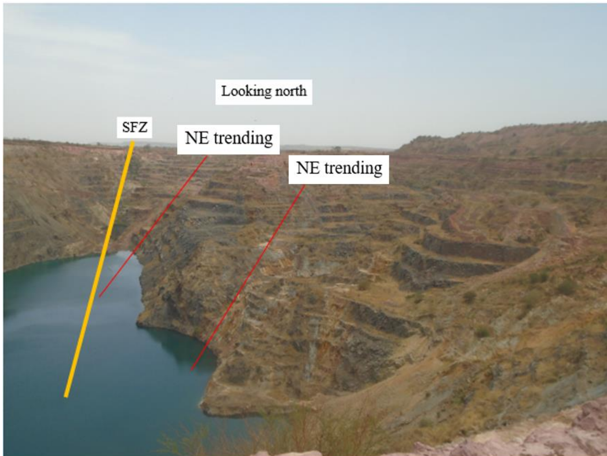
Figure 50: The supergene alteration presents in the calc-silicate rock from the southern area to north of the Sadiola Hill opencast pit.
