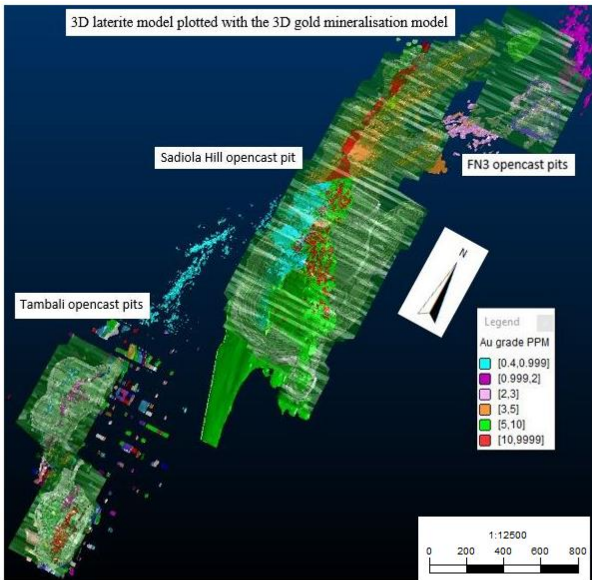
Figure 38: The 3D laterite model plotted with the 3D gold mineralisation model for Sadiola goldfield (FN3 in the northern, Sadiola Hill open cast in the middle, and the Tambali pits in the southern).
