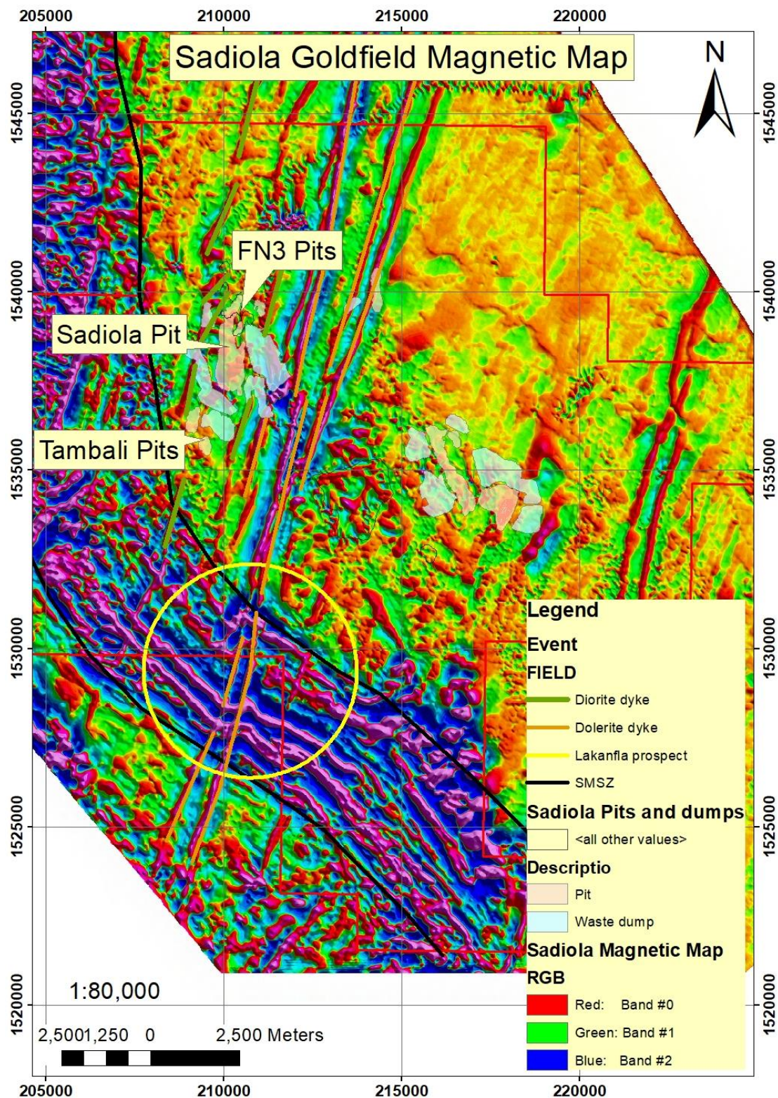
Figure 18: Regional Magnetic data and interpretation map on the Sadiola goldfield shows the shape and width of the SMSZ. The SMSZ is located on the western side of the map. This Sadiola total field is GradEnh_0p05_NEW_RTPLL_UC50_1VD.ecw.
