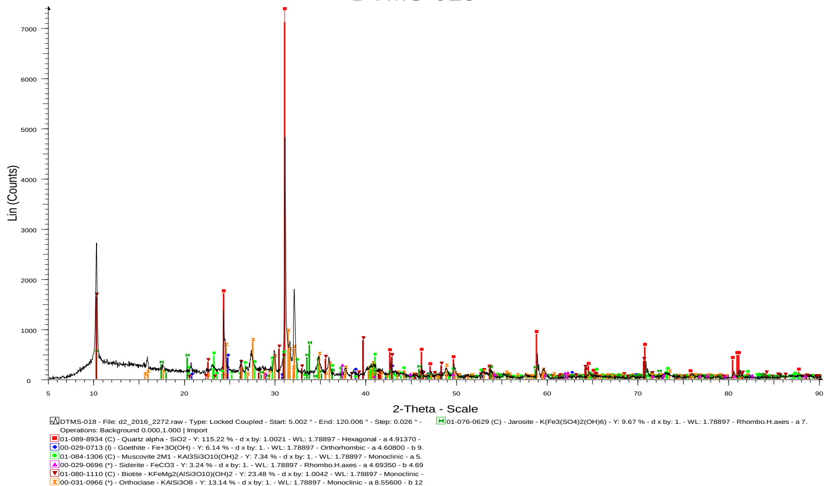
Figure 60: The result of sample DTMS-018 indicates the presents of silica, goethite, muscovite, siderite and biotite minerals.
