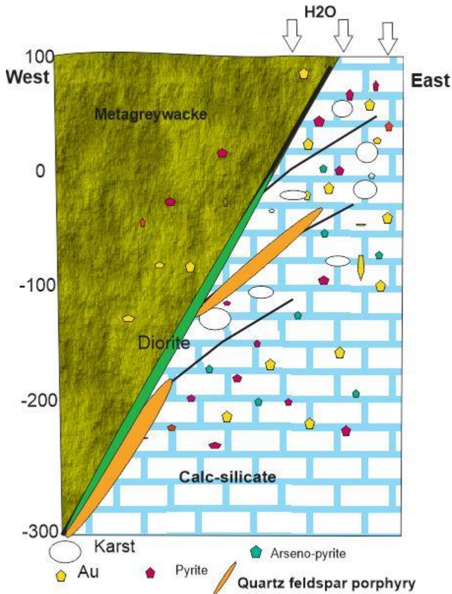
Figure 42: West-east cross-sectional sketch of the Sadiola Hill genetic model for the supergene enrichment phase. The surface water penetrated the calc-silicate rock through the SFZ and northeast trending structures. The pyrite in the presence of H_2O and O_2 can active some reactions and cause the oxidation of calc-silicate.
