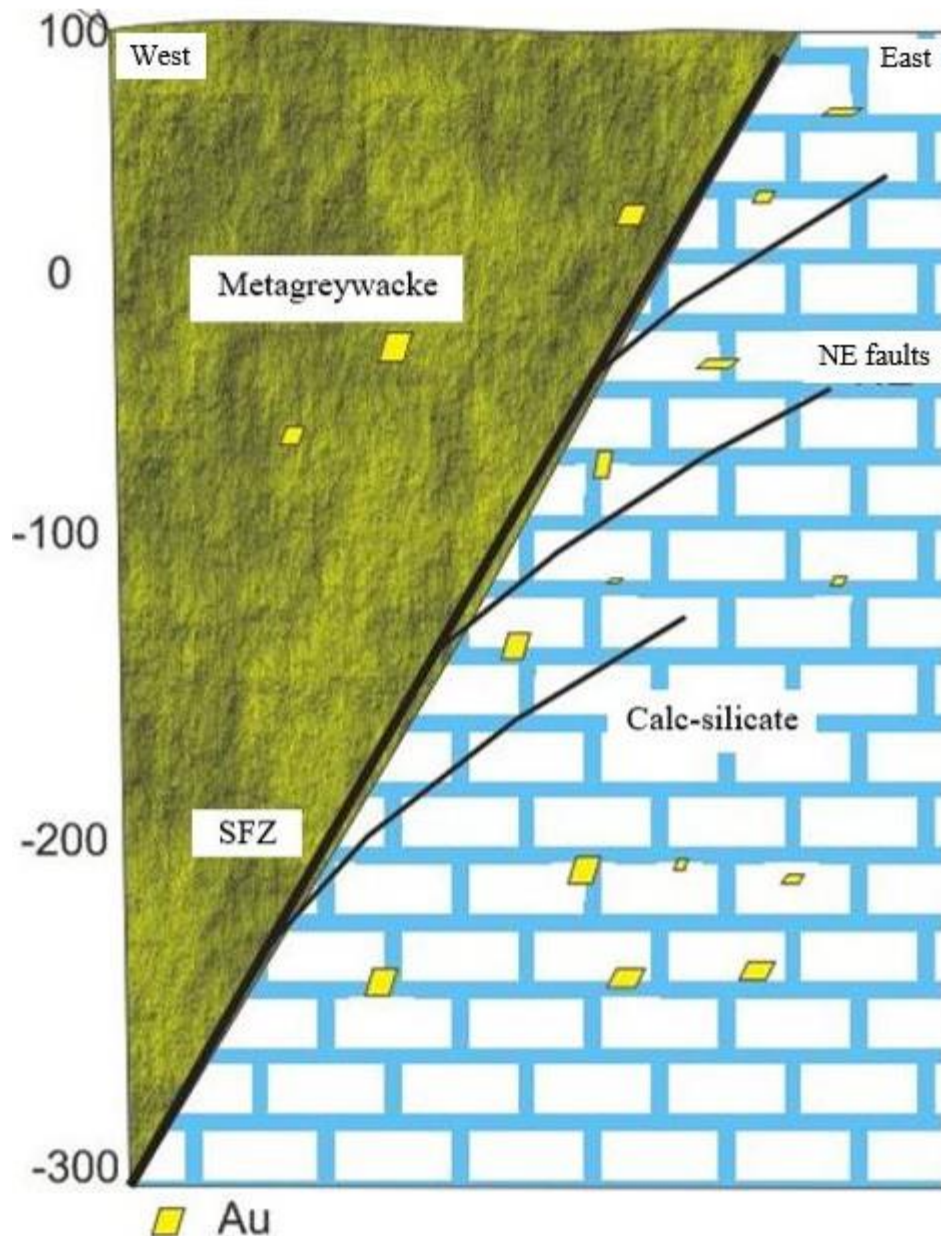
Figure 33: West-east cross-sectional sketch of the Sadiola Hill genetic model for the supergene enrichment phase. The D2 deformation related to northwest-southeast compression, probably associated with the Eburnean orogeny, produced an effect on the SFZ, and north-northeast trending faults. The SFZ and north-northeast trending faults seem to be syn-genetic. The source of the gold in the Sadiola Hill opencast pit was concluded by Hein (2007) as hydrothermal.
