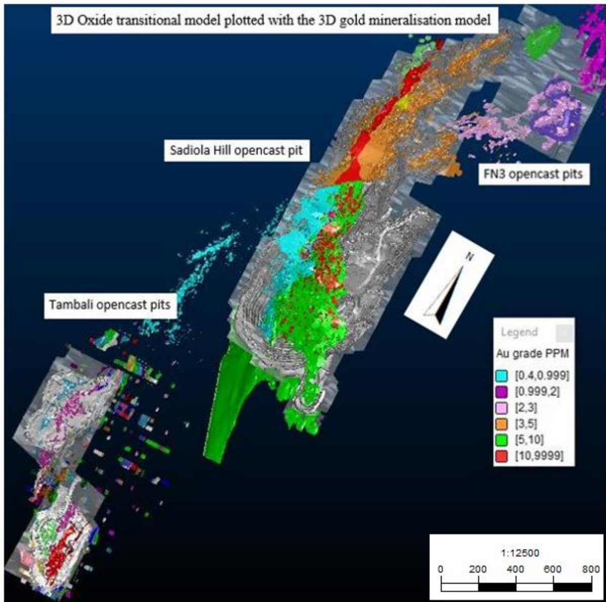
Figure 40: The 3D oxide transitional zone plotted with the 3D gold mineralisation model for Sadiola goldfield (FN3 in the northern, Sadiola Hill open cast in the middle, and the Tambali pits in the southern part).
