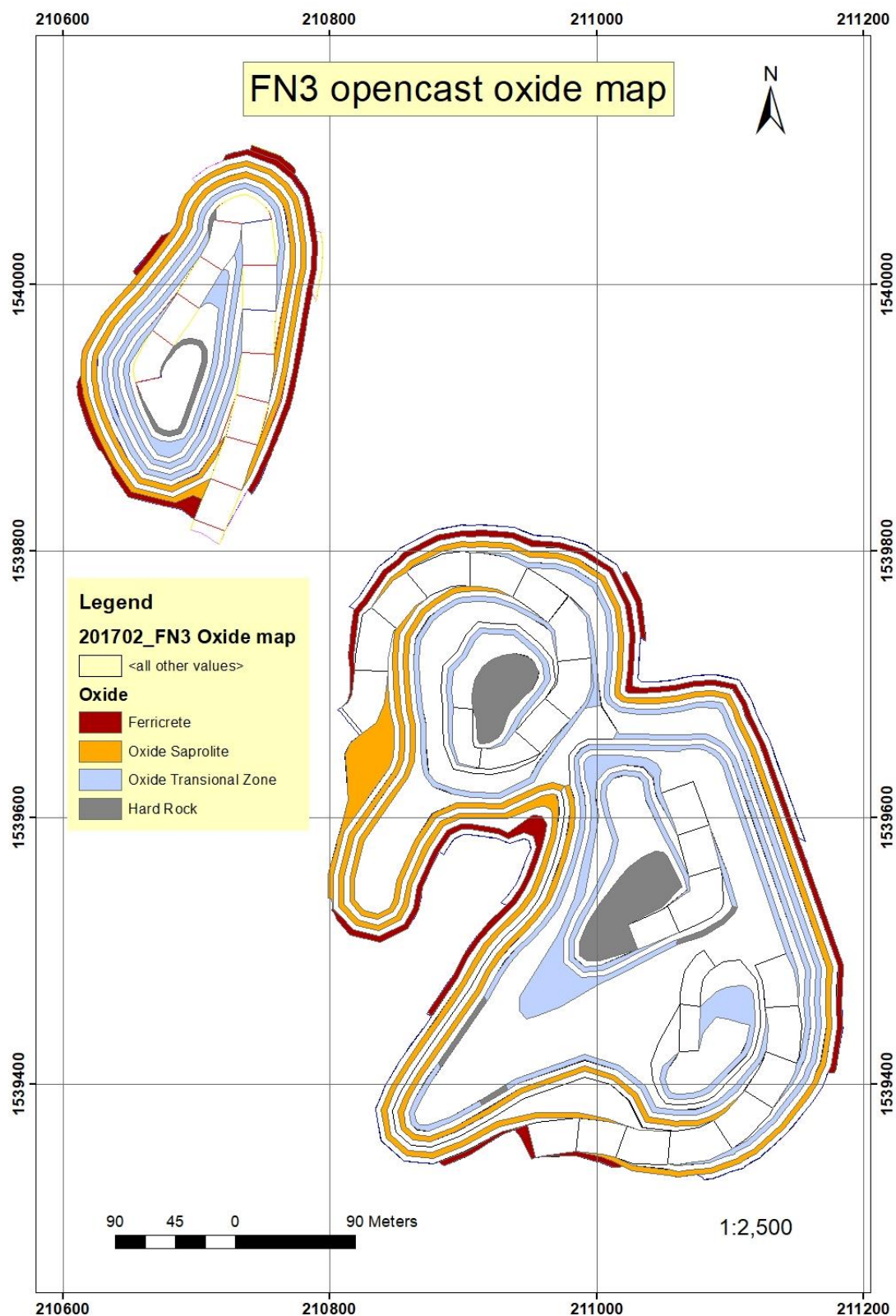
Figure 31: The oxide map for FN3 north and south pits, composed of ferricrete in red colour, the oxide saprolite, the oxide transitional zone is the light blue colour and the hard rock in grey colour.
