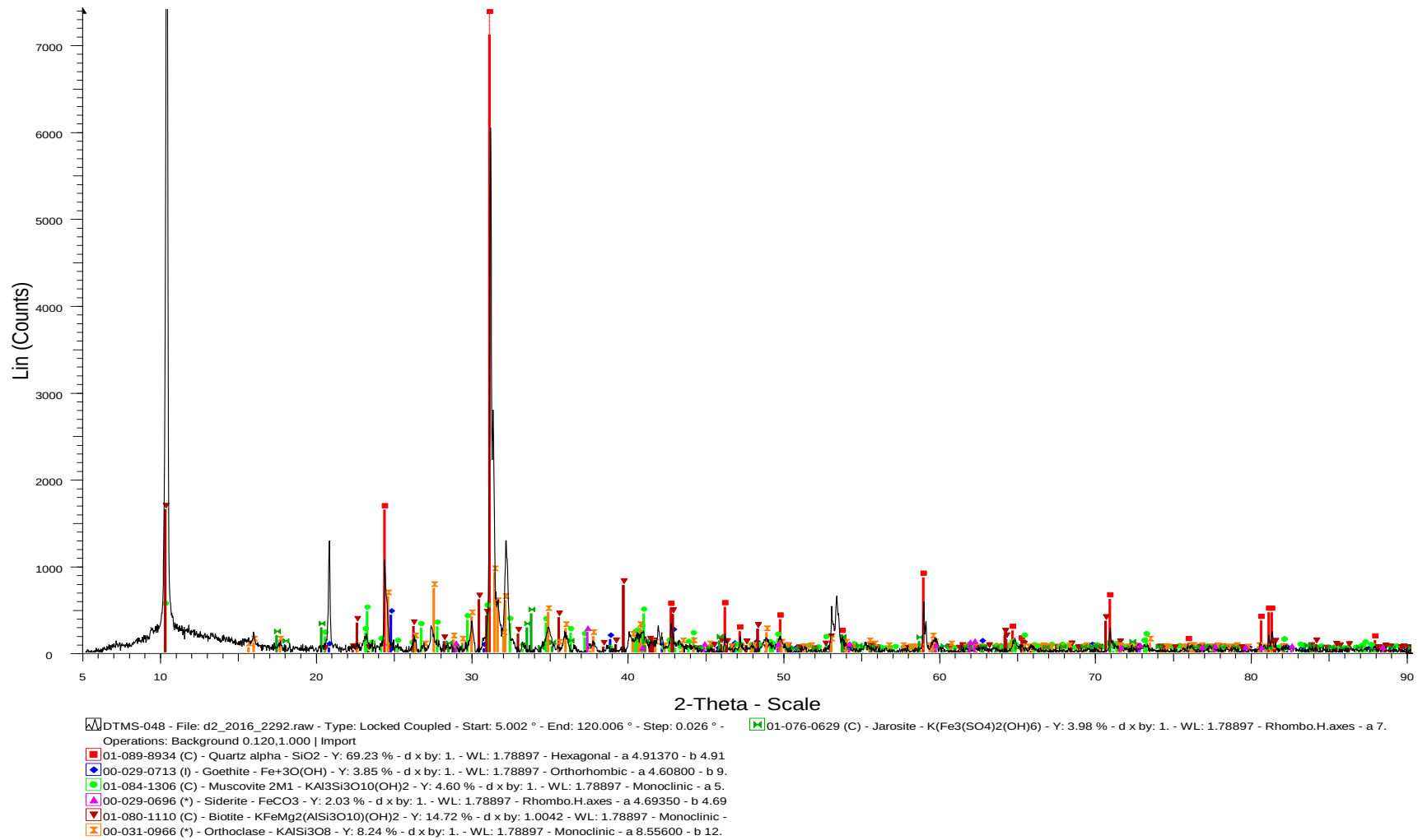
Figure 76: The result of sample DTMS-048 indicates the presents of silica, goethite, muscovite, siderite and biotite minerals.
