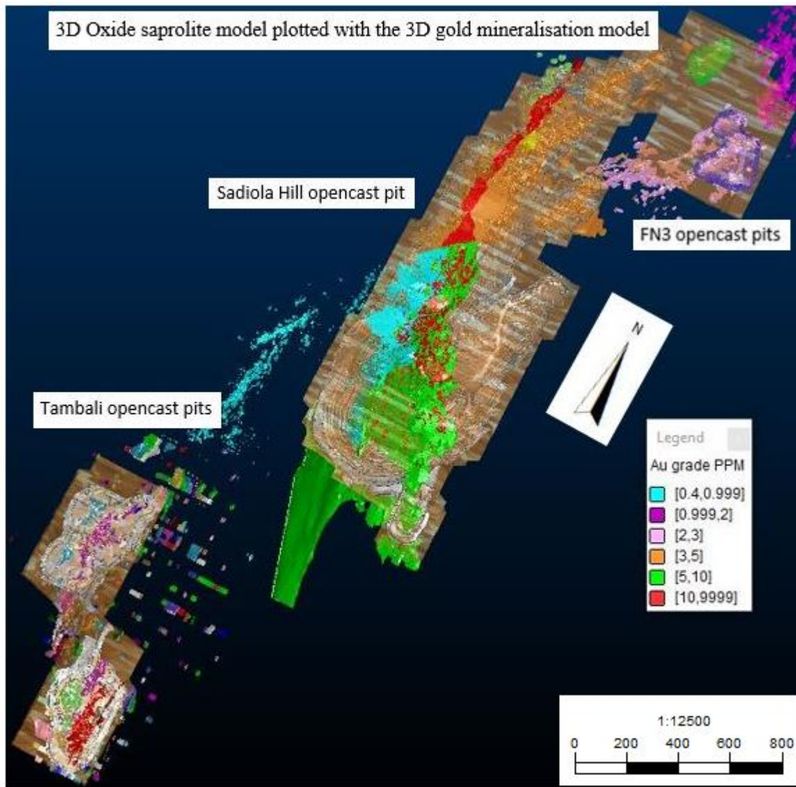
Figure 39: The 3D oxide saprolite model plotted with the 3D gold mineralisation model for Sadiola goldfield (FN3 in the northern, Sadiola Hill open cast in the middle, and the Tambali pits in the southern part).
