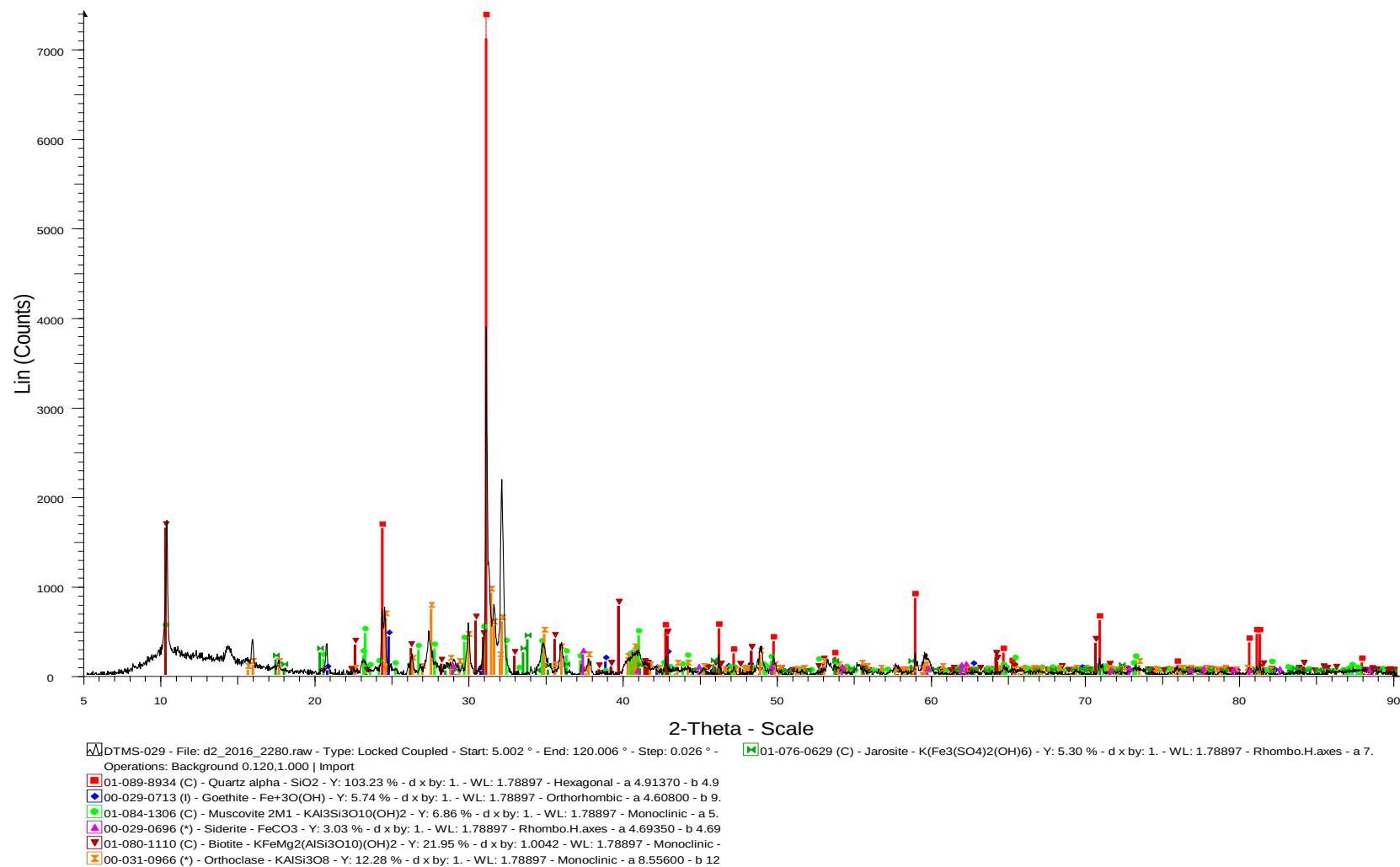
Figure 67: The result of sample DTMS-029 indicates the presents of silica, goethite, muscovite, siderite and biotite minerals.
