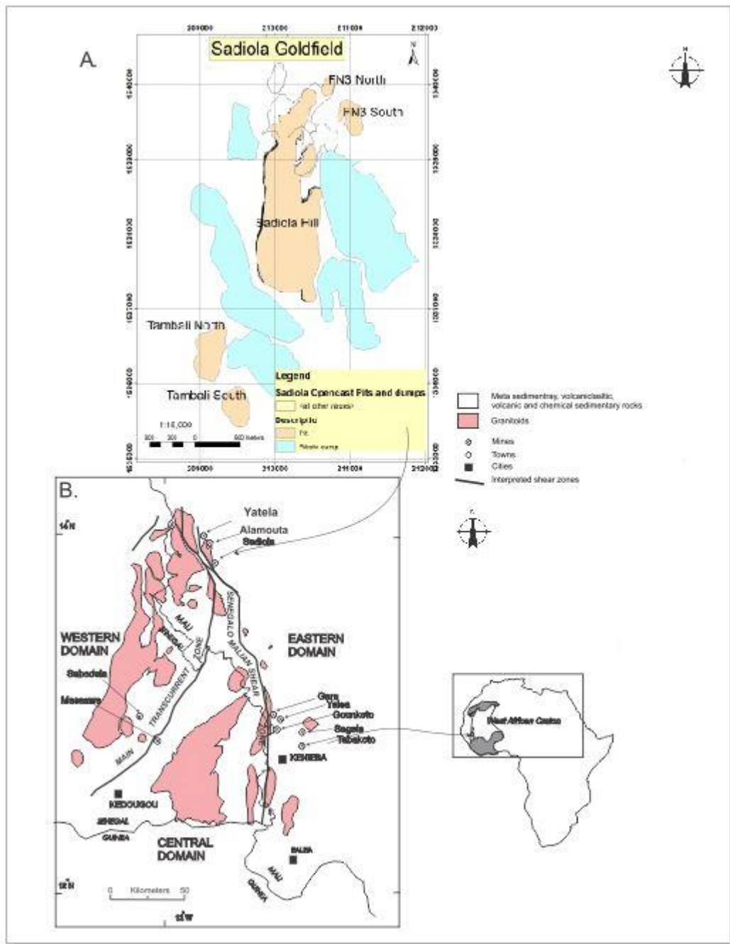
Figure 5: The inserted map shows the position of the WAC in Africa. A- Presentation of the study area in Sadiola goldfield. B- Location of the different goldfield in the Kédougou-Kénieba Inlier. In the KKI the SMSZ (Sénégal-Malian Shear Zone) is located in the east and the MTZ (Main Transcurrent Zone) at the west (after Hein et al., 2012).
