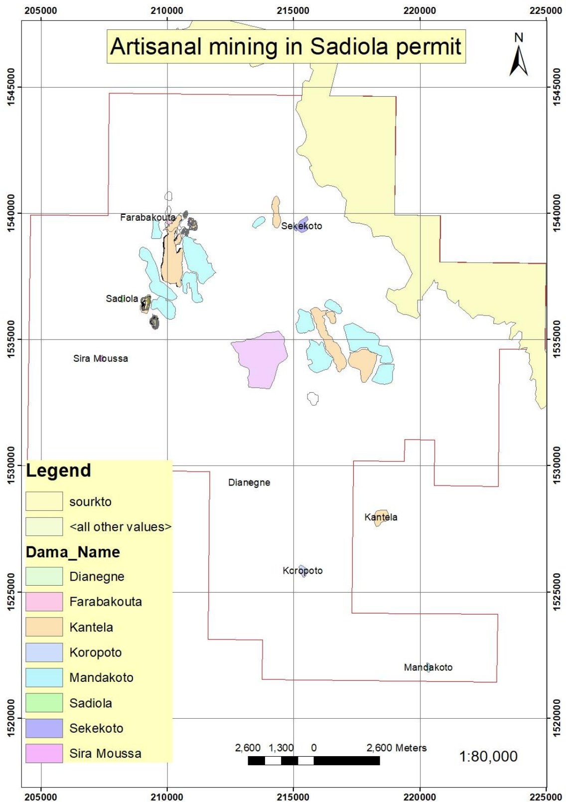
Figure 4: Position and name of artisanal mining in the Sadiola goldfield. The names of artisanal mines indicate their location, while the light blue colour represents the waste dump and the dark yellow colour represent the opencast pits. Each artisanal mine was contoured with a GPS.
