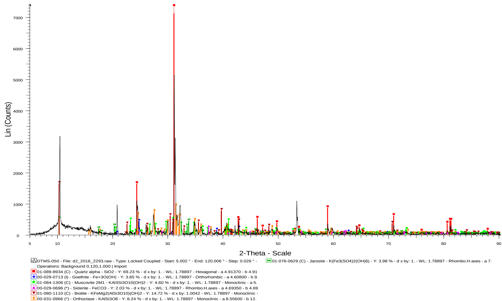
Figure 77: The result of sample DTMS-050 indicates the presents of silica, goethite, muscovite, siderite and biotite minerals.
