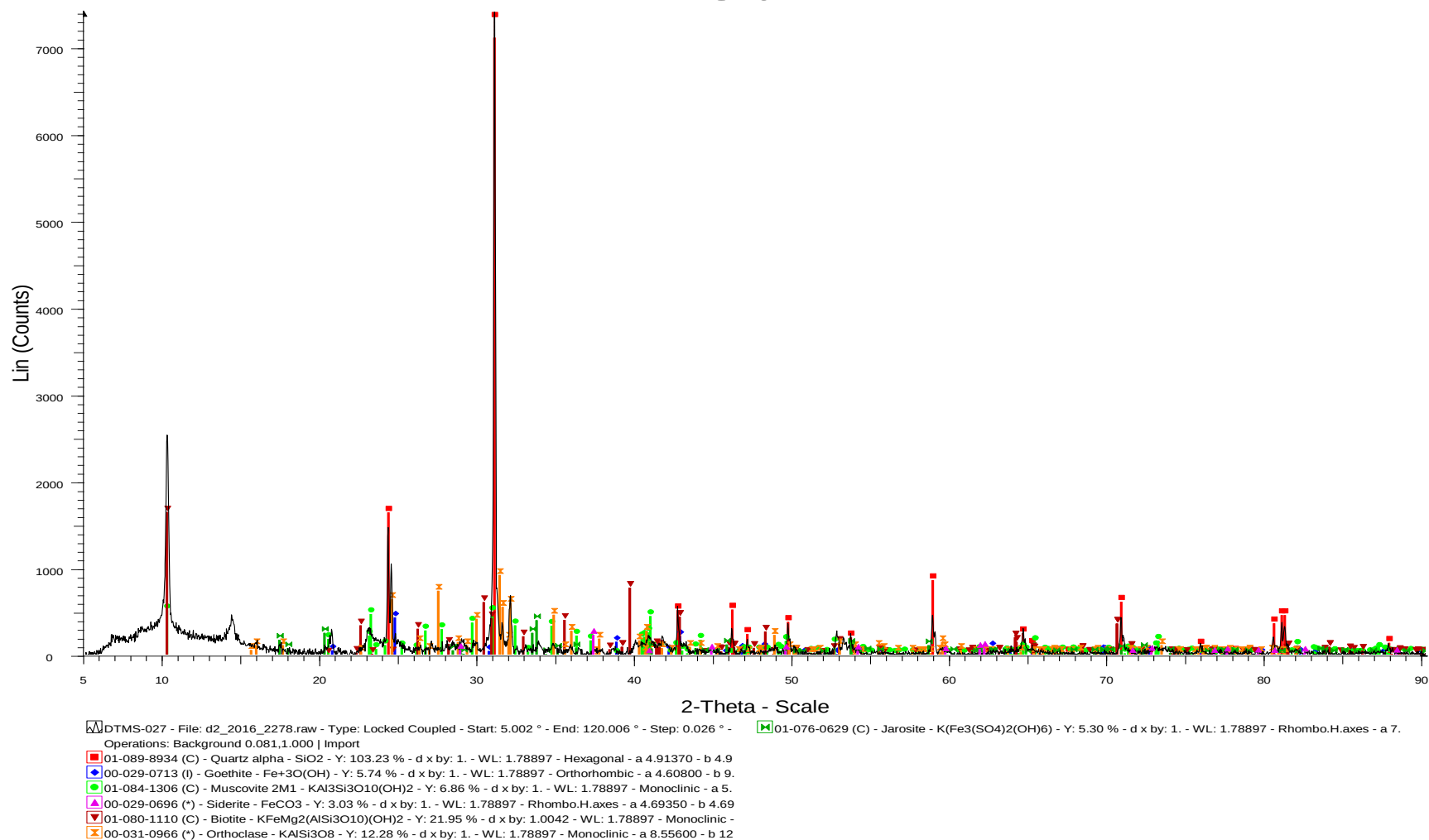
Figure 65: The result of sample DTMS-027 indicates the presents of silica, goethite, muscovite, siderite and biotite minerals.
