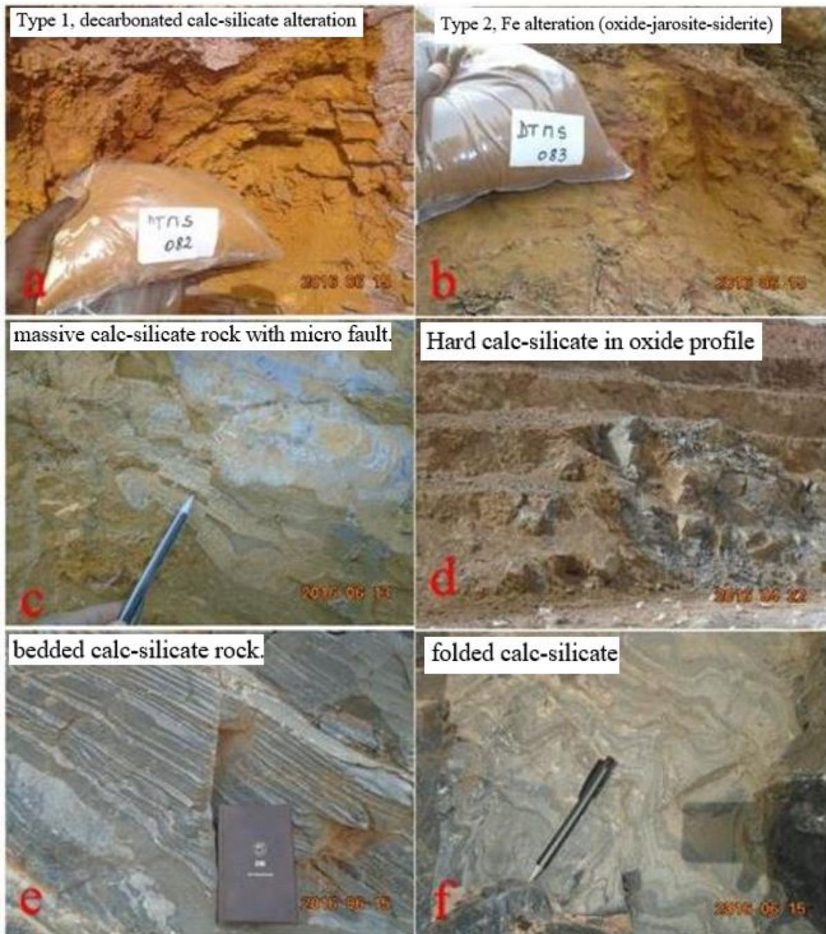
Figure 16: Photograph of the samples according to the alteration profile.
