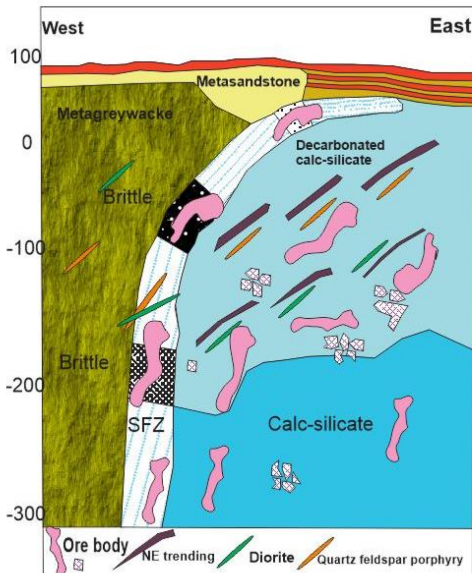
Figure 44: West-east cross-sectional sketch of the Sadiola Hill showing the results of oxidation and collapse of the oxide profile.
