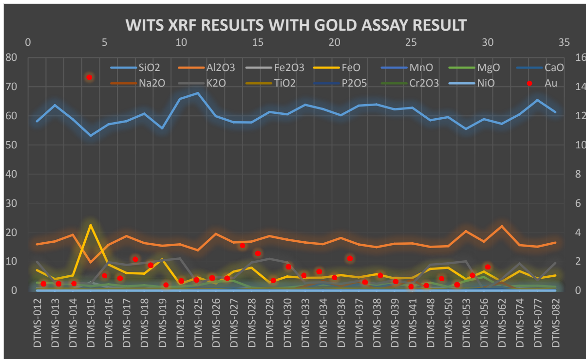
Figure 53: Diagram of the XRF result analysed in the Earth laboratory of the University of the Witwatersrand, Johannesburg. On the chart, concentrations in ppm are shown on the vertical axis, while the samples are given along the horizontal axis.
