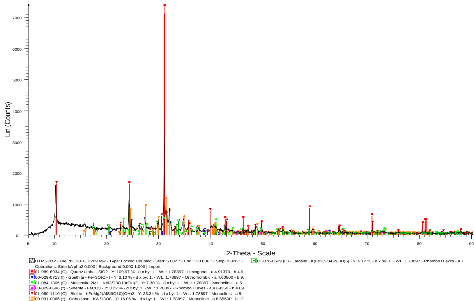
Figure 54: The result of sample DTMS-012 contains silica, goethite, muscovite, siderite and biotite minerals.
