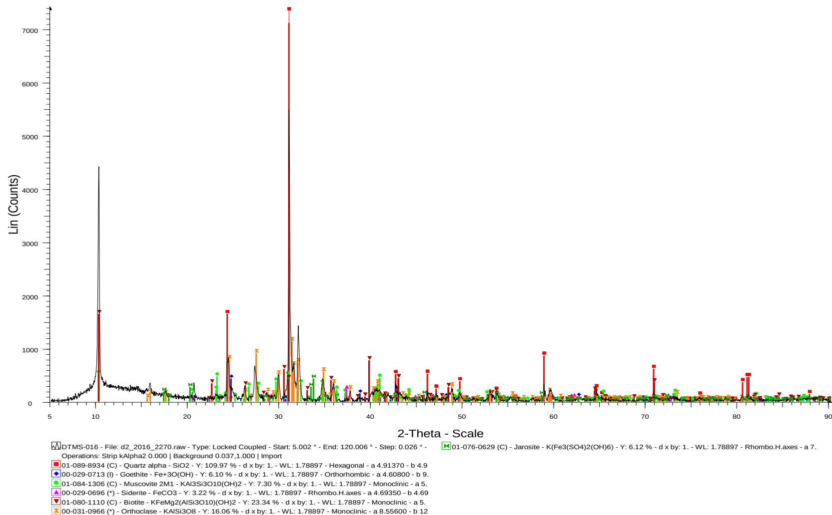
Figure 58: The result of sample DTMS-016 contains silica, goethite, muscovite, siderite and biotite minerals.
