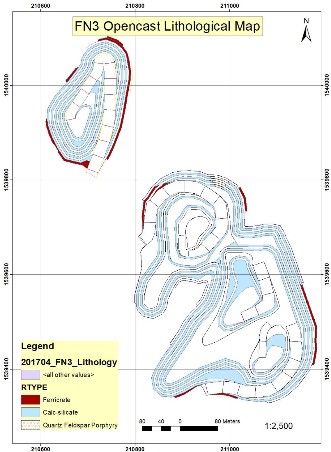
Figure 21: Lithological map of the FN3 south and north pits. The pits are dominated by altered and unaltered calc-silicate rock and crosscut by quartz-feldspar porphyry.
