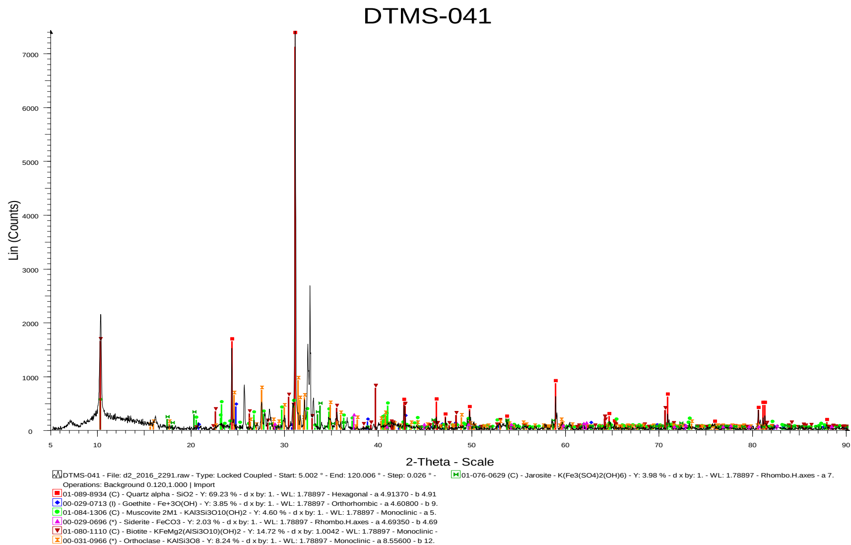
Figure 75: The result of sample DTMS-041 indicates the presents of silica, goethite, muscovite, siderite and biotite minerals.
