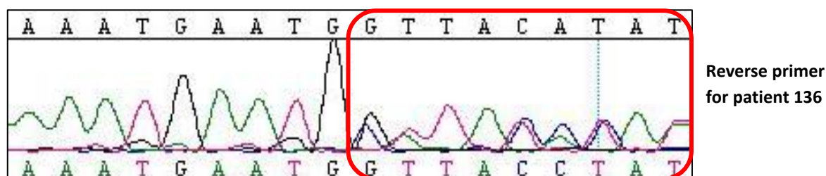
Figure 3.5: The MLH1 c.731_734delGTTA mutation in exon 9. This sequence was inspected to ensure that the correct base calling was made. The reverse primer was used to confirm the presence of the mutation and can be seen in this image.
