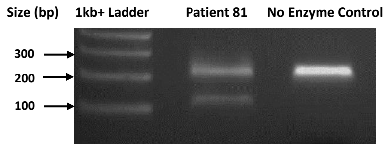
Figure 3.14: RFLP analysis with HpyCH4III performed on patient 81. This gel picture shows that patient 81 was heterozygous for c.885-1G>A as the presence of two alleles is confirmed. The 'no enzyme control' was included to ensure no contamination was present
