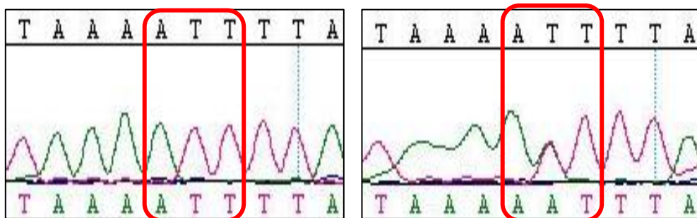
Figure 3.11: The MSH2 c.367-16T>A novel variant of intron 2. The image on the left shows the wildtype DNA sequence and the image on the right shows the heterozygous variant in patient 61.
