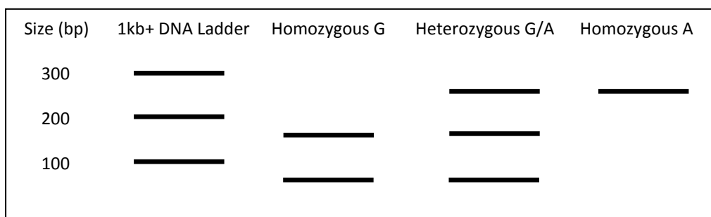
Figure 2.4: Diagram of the expected RFLP analysis using HpyCH4III to screen for the MLH1 c.885-1G>A variant. HpyCH4III will recognise and cut the wildtype allele.
