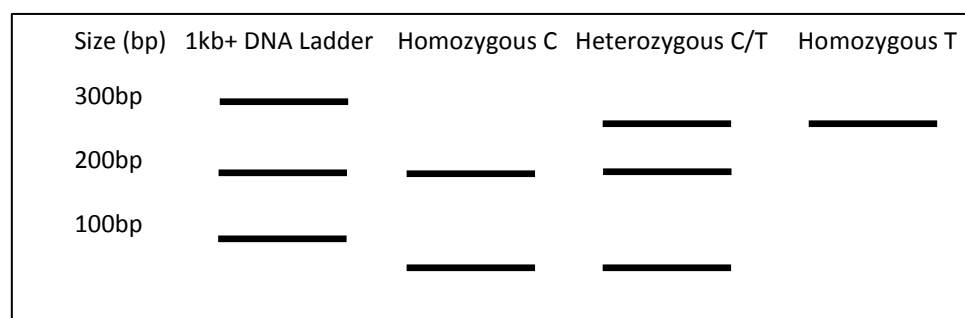
Figure 2.6: Diagram showing the expected RFLP fragments when RsaI is used to investigate the MSH2 c.1662-43C>T variant. RsaI recognises the wildtype GTAC site.
