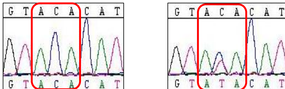
Figure 3.12: The MSH2 c.1662-43C>T novel variant located within intron 10. The image on the right shows the variant as it was detected in patient 104 and the image on the left shows the wildtype DNA sequence.
