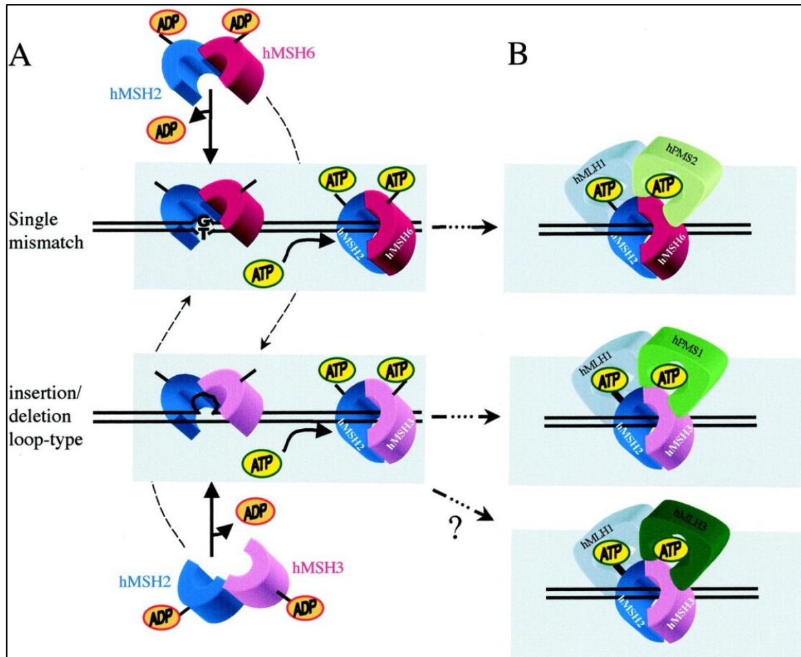
Figure 1.6: Diagram showing how the MMR proteins interact to repair mismatches in the DNA (Fishel, 2001). The MutS \alpha heterodimer (hMSH2 and hMSH6) binds to the DNA and detects single base mismatches. The MutL \alpha complex (hMLH1 and hPMS2) binds to the MutS \alpha complex. The MutS \beta heterodimer (hMSH2 and hMSH3) binds to insertion/ deletion loops in the DNA. The MutL \beta complex binds to the MutS \beta complex. In this figure, the 'h' in the protein name indicates a human protein.
