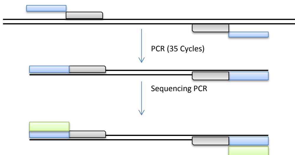
Figure 2.3: Schematic representation of PCR and sequencing reactions in this study. Universal primers (shown in blue) were included at the 5' and 3' ends of the primers (grey). The universal primers do not bind to the template DNA but are included in the amplicons. A universal sequencing primer (shown in green) can be used to sequence from either the 5' or 3' tail.
