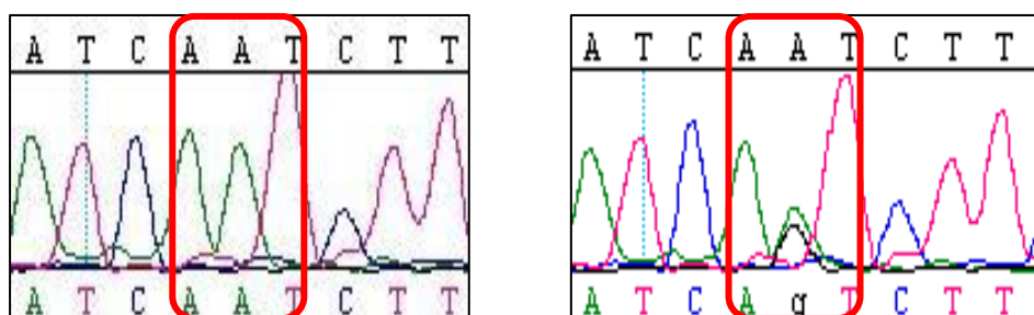
Figure 3.3: The MLH1 c.454-13A>G variant of intron 5 found in Patient 104. The wildtype sequence is displayed on the left while the image on the right shows the heterozygous variant seen in Patient 104
