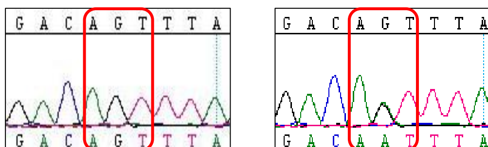
Figure 3.6: The MLH1 c.885-1G>A novel variant located within the splice acceptor site of intron 10. The wildtype DNA sequence is shown on the left. The image on the right shows the heterozygous mutation that was found in patient 81.
