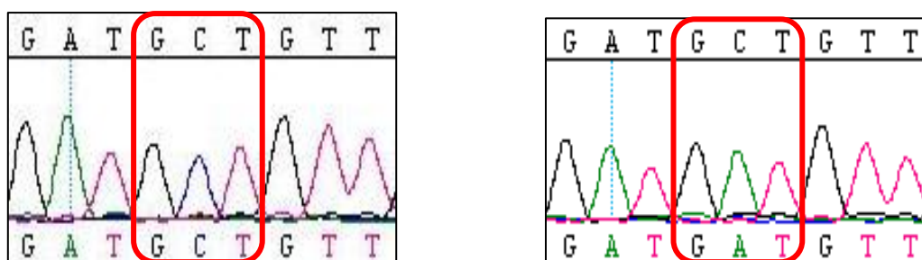
Figure 3.8: The MSH2 c.1811C>A novel variant in exon 12. This missense mutation was detected by the Wessex Regional Genetics Laboratory and was included in this study as a positive control. The image on the left shows the wildtype DNA sequence and the image on the right shows the variant.
