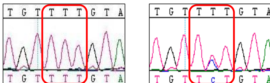
Figure 3.9: The MSH2 c.2006-6T>C pathogenic variant of intron 12. The wildtype DNA sequence for the region is seen on the left. The image on the right shows the heterozygous variant
