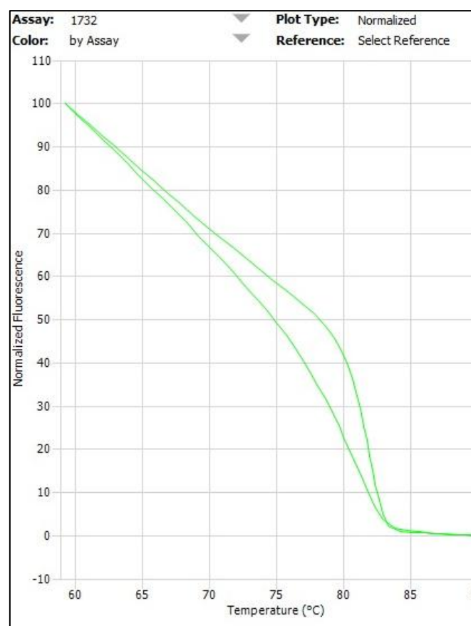
Figure 2.8: The HRM normalised melting curve obtained from control samples. The wildtype allele is the top curve and the variant ( MLH1 c.1732-19T>A) is the bottom curve. Random samples would be compared to these curves to determine allele frequency
