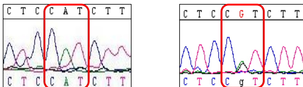
Figure 3.2: The MLH1 c.655A>G variant (p.I219V), which leads to a missense mutation, in exon 8. The wildtype DNA sequence is seen on the left while the variant can be seen on the right.
