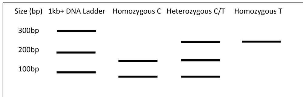
Figure 2.5: Diagram showing the expected RFLP fragments when TaqI is used to investigate the MSH2 c.1662-10C>T variant. TaqI will recognise the wildtype allele
