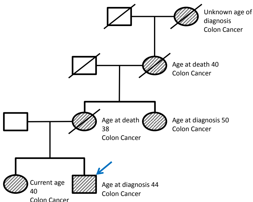
Figure G.5: The pedigree for patient 150 where the MSH2 c.1811C>A variant was found. This variant was first found by the Wessex Regional Genetics Laboratory who predicted the variant to be pathogenic. In addition, SIFT and PolyPhen also predicted this missense mutation to have a deleterious effect. The patient's sister, who also developed colon cancer, was also investigated by the Wessex Regional Genetics Laboratory and found to have the same variant. This provides strong evidence that this variant is pathogenic
