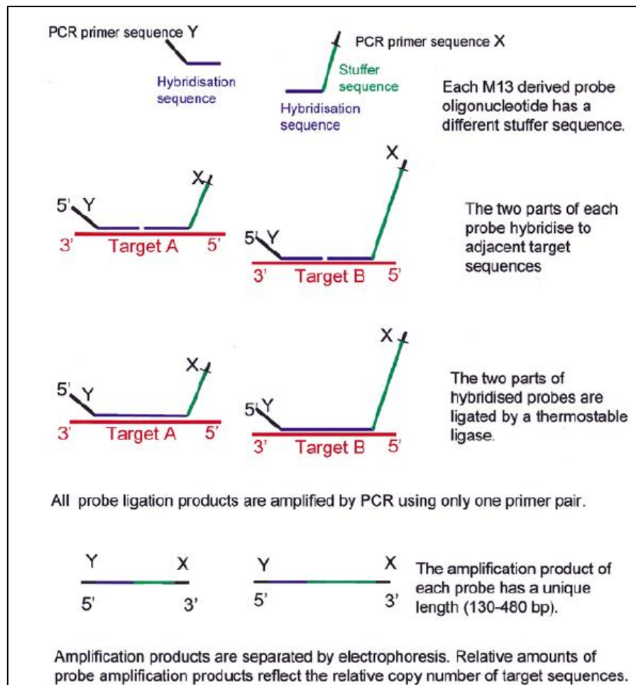
Figure 2.2: The MLPA reaction. This figure outlines the steps in an MLPA reaction.
