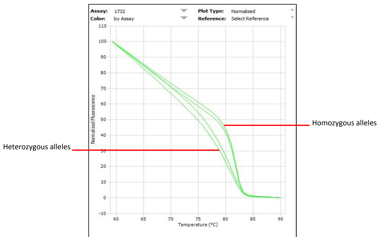
Figure 3.16: The HRM normalised melting curve for the assay of MLH1 c.1732-19T>A variant. The top curve shows the normalised curve for the homozygous control and random samples. The bottom curve shows the normalised curve for the heterozygous control and random sample
