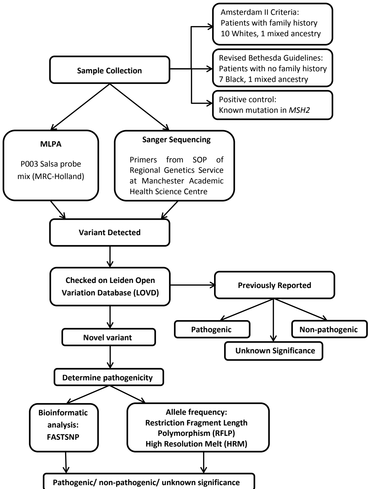
Figure 2.1: Flow Diagram outlining the approach and actions taken in this study
