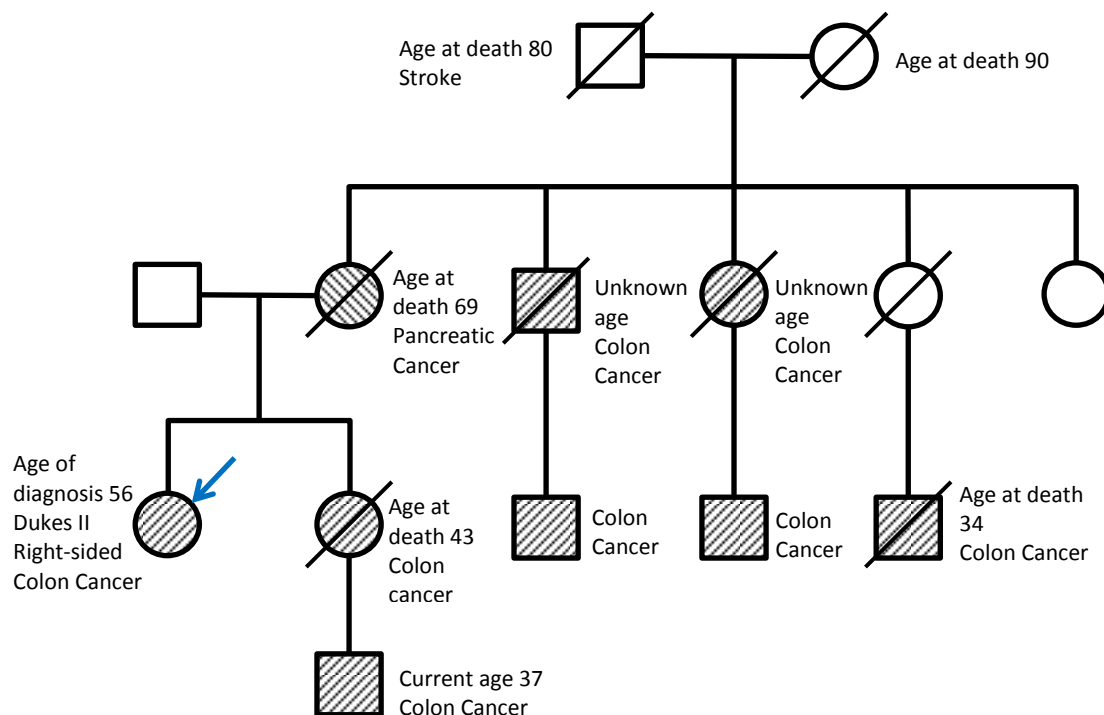
Figure G.4: Pedigree for patient 136. This white patient had a prominent family history of colon cancer and her mother had pancreatic cancer. The MLH1 c.731_734delGTTA pathogenic mutation was found in this patient, which leads frame shift and a truncated protein product. The other family members must be screened for the presence of the mutation.
