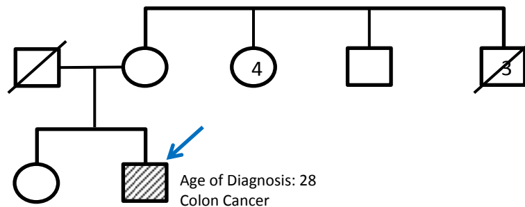
Figure G.1: The pedigree for black patient 205. This patient presented with colon cancer at 28 but has no known family history of the disease. This patient was found to have seven variants, two of which were not previously reported ( MLH1 c.1732-19T>A and MSH2 c.-185C>A). The numbers indicate multiple females and deceased males
