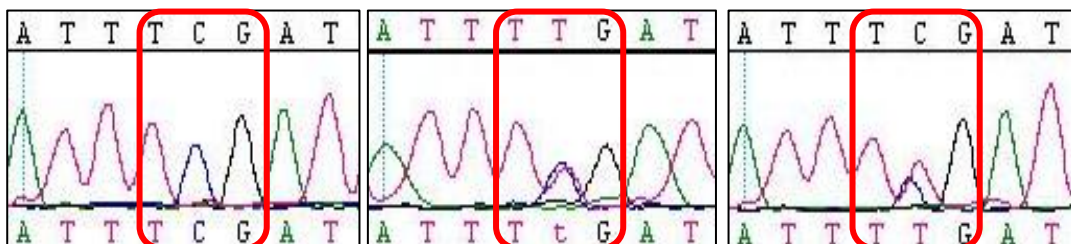
Figure 3.13: The MSH2 c.1662-10C>T novel variant located within intron 10. The image on the left shows the wildtype DNA sequence. The images in the middle and on the right show the variants that were detected in two different black African patients, 235 and 238, respectively.
