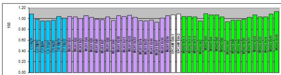
Figure 3.1: The MLPA result generated using the spread sheet from NGRL. Since all patients tested for MLPA were found to have no large insertions, deletions or duplications, all the patients MLPA results were similar to this one, with each allele being \approx 1.0 . If one allele was deleted, the bar would have been \approx 0.5 . If both alleles were deleted, the bar would be at 0. If one allele was duplicated, the bar would be \approx 1.5 , and if both alleles were duplicated, it would have been \approx 2.0 .
