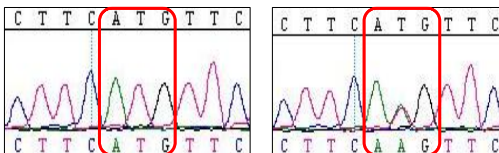
Figure 3.7: The MLH1 c.1732-19T>A novel variant that was detected in intron 15. The wildtype DNA sequence is seen on the left and the variant is seen on the right
