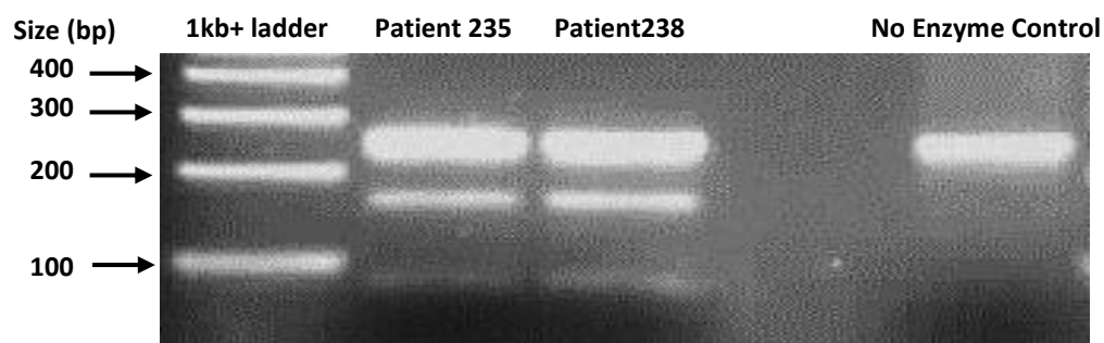
Figure 3.15: RFLP gel picture from using TaqI to investigate the MSH2 c.1662-10C>T variants in patients 235 and 238.
