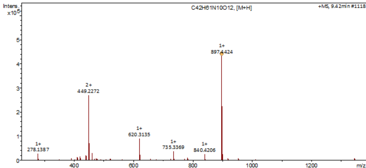
Figure A49. LC-MS analysis for 61c
