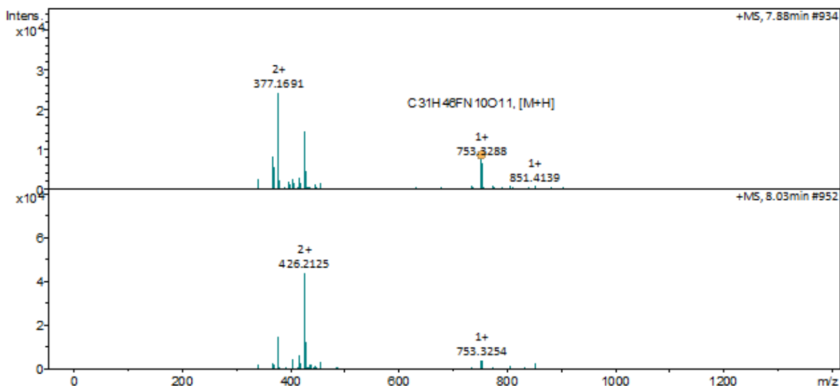
Figure A53. LC-MS analysis of 61g
