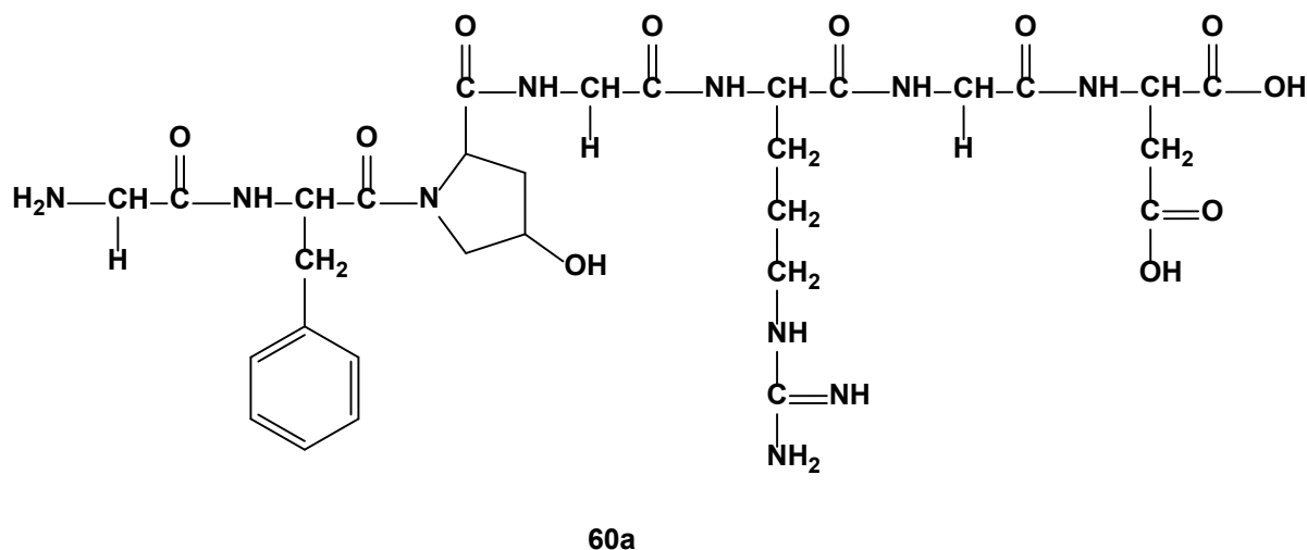
Figure 16. Structural representation of \alpha -peptide G-F-O-G-R-G-D
