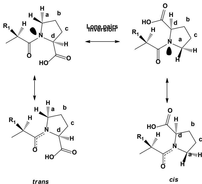
Figure 17. Conformational isomers of peptide containing proline. 143,144
