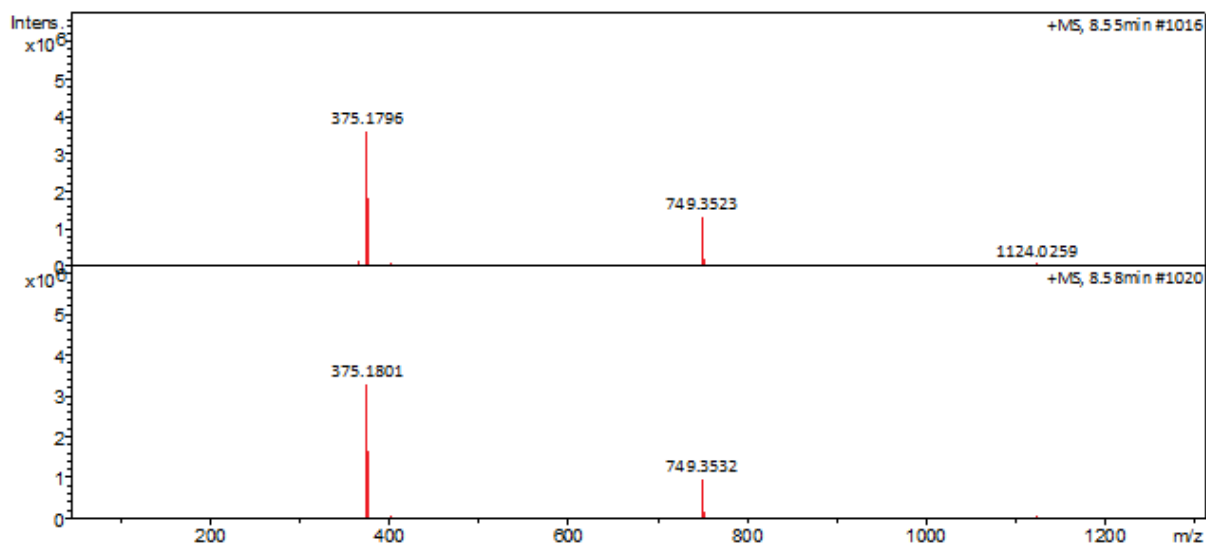
Figure A46. LC-MS analysis for G-(Me)Phe-O-G-R-G-D
