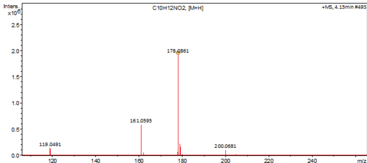
Figure A32. LC-MS analysis for hydrolysis of 54c
