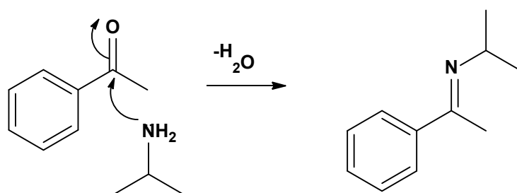
Figure A20. Mechanism for by-product formed by reaction between the isopropyl amine and acetophenone
