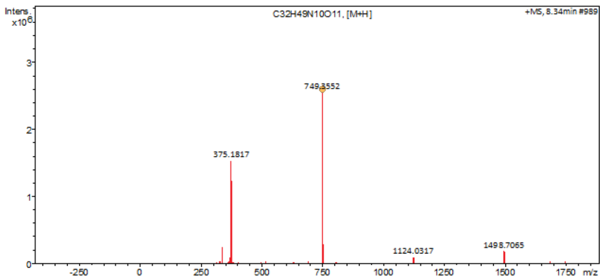
Figure A50. LC-MS analysis of 61d
