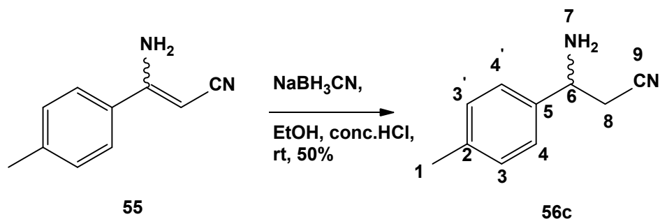
Scheme 26. Synthesis of 3-amino-3-( p -tolyl)propanenitrile 56c using NaBH 3 CN
