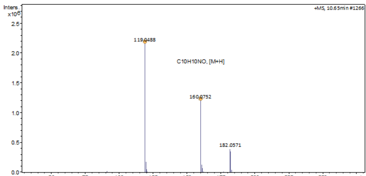
Figure A23. LC-MS analysis for standard 54c
