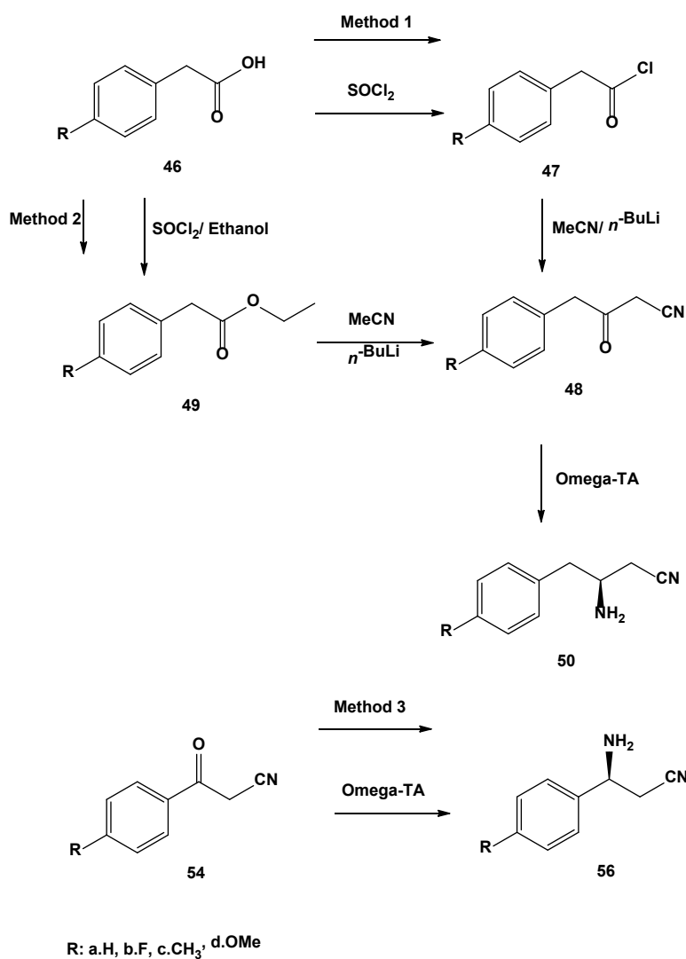
Scheme 15. Planned approach towards the synthesis of \beta -aminonitriles
