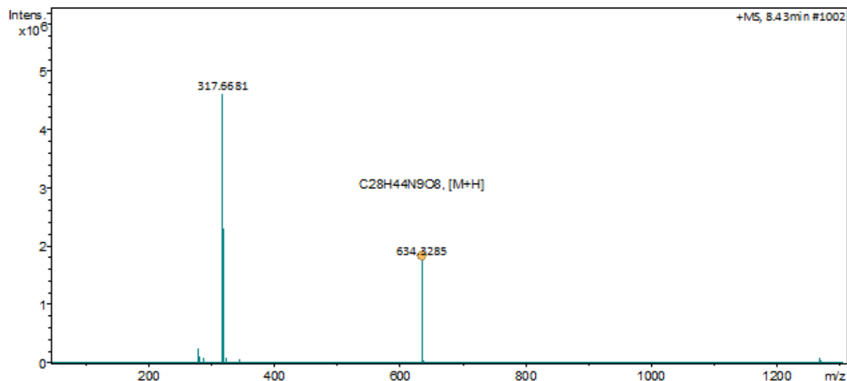
Figure A45. LC-MS analysis for G-(Me)Phe-O-G-R-G
