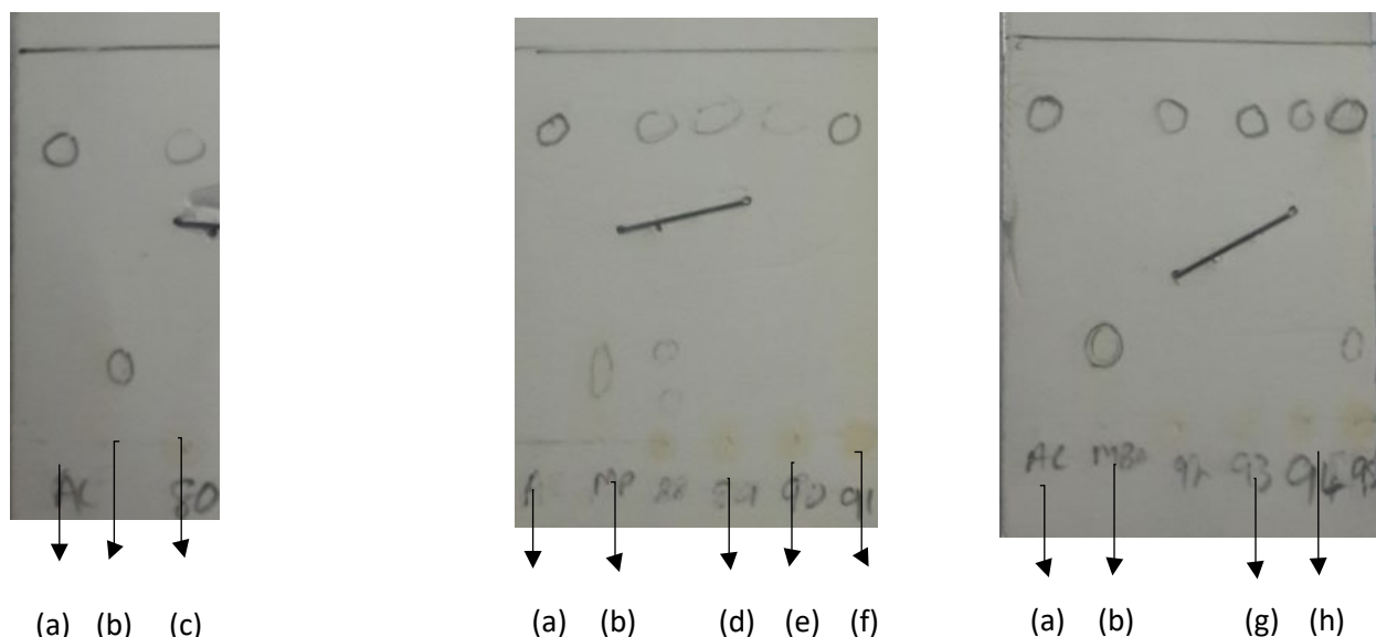
Figure A5. Reductive amination of 58 (50% EtOAc/Hexane); (a) The acetophenone standard starting material 58 . (b) The MBA standard product 57 . (c) Reaction involved Prozomix-TA020, (d) Reaction involved Prozomix-TA023. (e) Reaction involved Prozomix-TA025. (f) Reaction involved Prozomix-TA027. (g) Reaction involved Prozomix-018. (h) reaction 94 involved Prozomix-TA050
