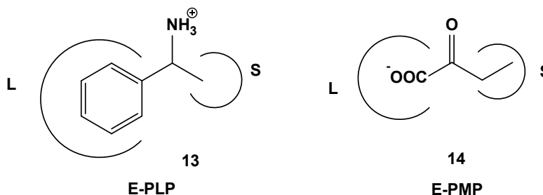
Figure 11. \omega -Transaminase substrate binding depicting the large (L) and small (S) pockets of the PLP form of the enzyme occupied by methylbenzylamine ( 13 ) and 2-oxobutyrate ( 14 ). 87
