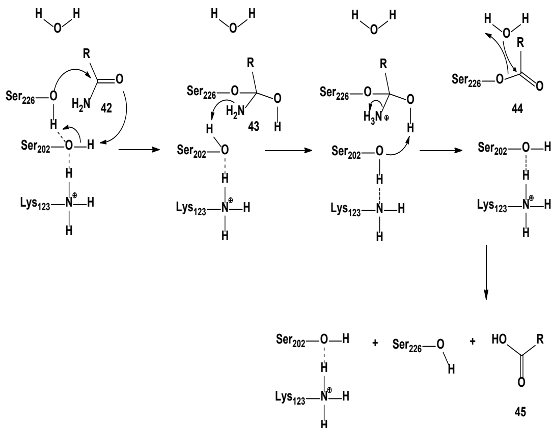
Scheme 13. Amidase mechanism for the biotransformation of amide into acid. 107
