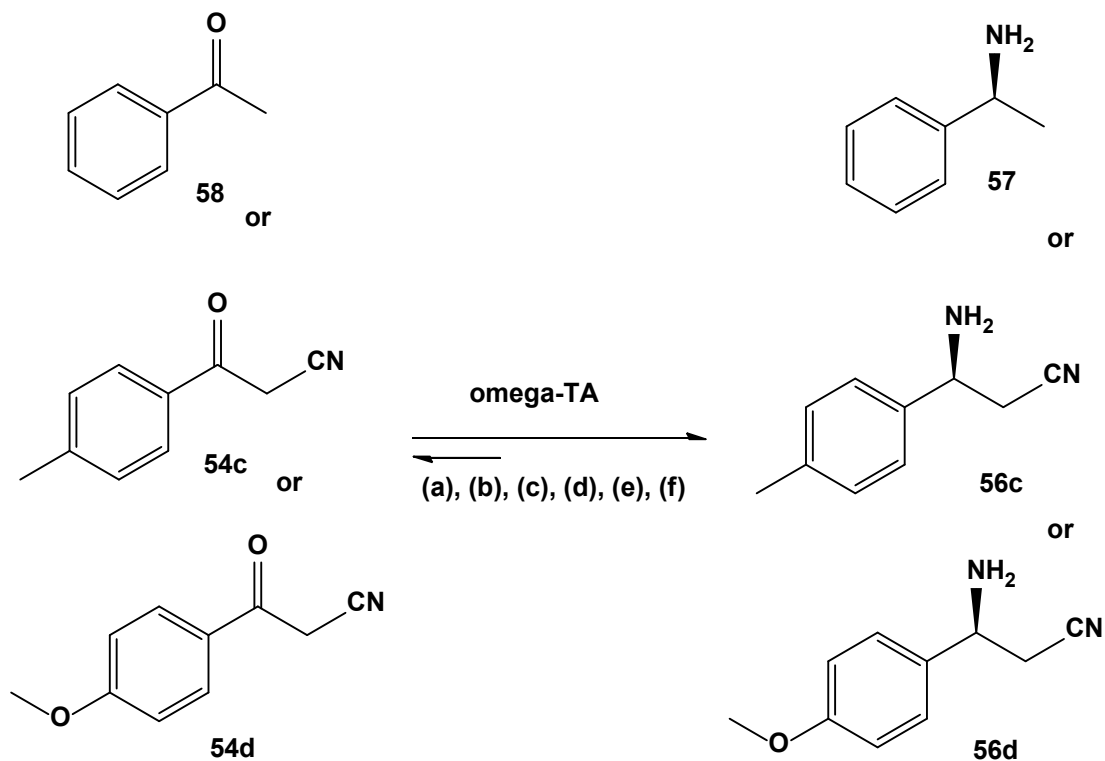
Scheme 27. Biotransformation of \beta -ketonitriles using omega-transaminase; (a) and (b) Screening of transaminase activity using 57 and 58 . (c) and (d) Investigating substrate and product inhibition using 57 and 58 . (e) Displacing unfavourable equilibrium by testing LDH system and different amine donors on 58 . (f) Asymmetric synthesis of \beta -aminonitriles using diamine donor on 58 , 54c and 54d .
