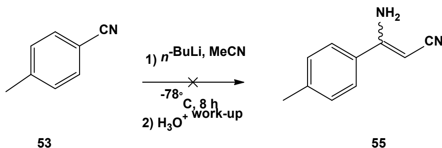
Scheme 23. Synthesis of the enamine using n -BuLi
