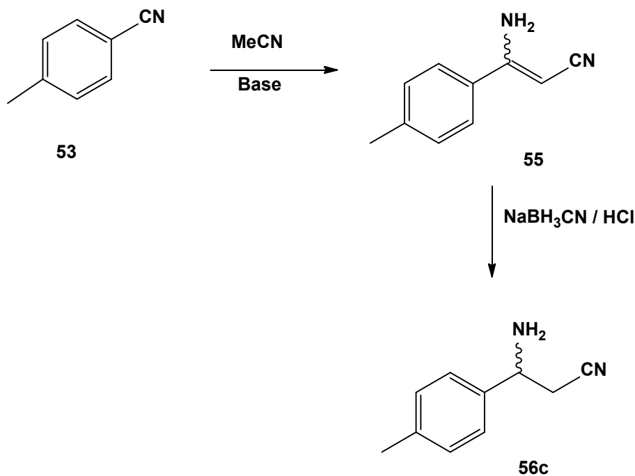
Scheme 22. Planned approach towards synthesis of 3-amino-3-( p -tolyl)propanenitrile 56c
