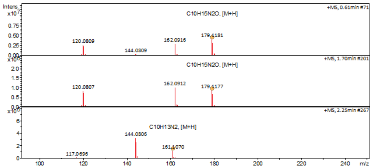
Figure A31. LC-MS analysis for hydrolysis of 56c
