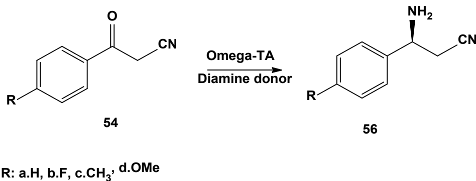
Figure 13. Biotransformation of beta -ketonitriles using omega-transaminases
