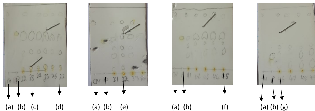
Figure A25. TLC for reductive amination of 54c (10 mM) using diamine donor (10% MeOH/EtOAc); (a) Standard substrate 54c . (b) Standard amine product 56c . (c) Reaction involved Prozomix-TA011. (d) Reaction involved prozomix-TA005. (e) Reaction involved Prozomix-TA010. (f) Reaction involved Prozomix-TA045. (g) Reaction 46 involved Prozomix-TA042 (40%. EtOAc/Hexane)
