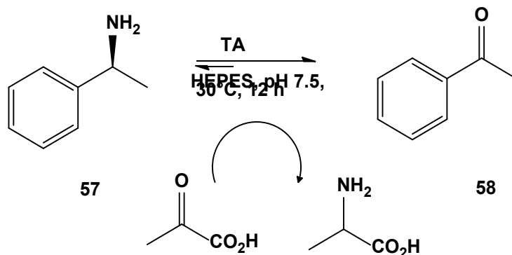
Scheme 28. Deamination of methylbenzylamine using pyruvate
