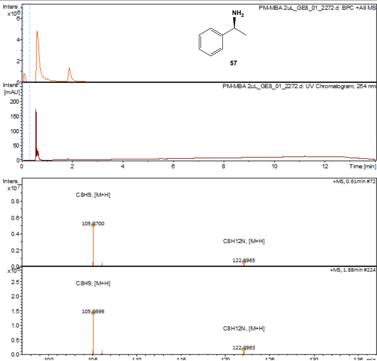
Figure A1. LC-MS data for the standard MBA 57
