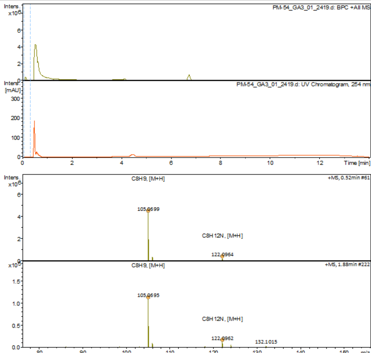
Figure A10. LC-MS analysis for deamination reaction involving Prozomix-TA045 at 250 mM
