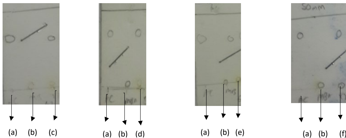
Figure A3. TLC for deamination of MBA (50 mM) (30 %EtOAc/Hexane); (a) The acetophenone standard product. (b) The MBA standard starting material. (c) Reaction involving Prozomix-TA016, (d) Reaction involving Prozomix-TA030, (e) Reaction involving Prozomix-TA037, (f) Reaction involving Prozomix-TA045.
