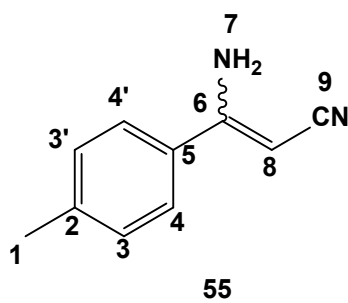
1 H NMR of 55
