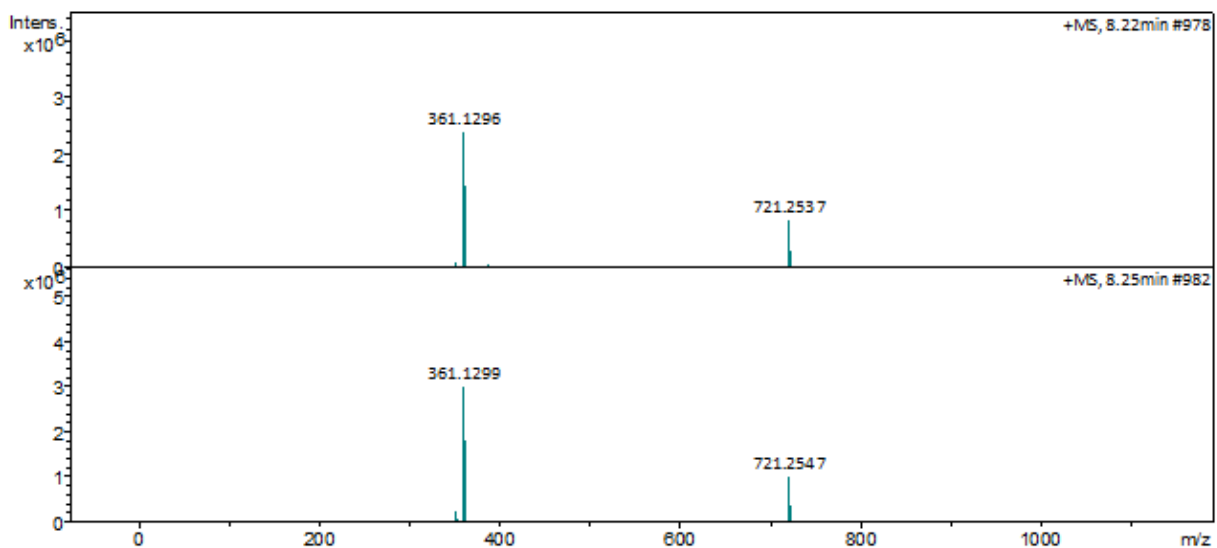
Figure A39. LC-MS analysis of 60a
