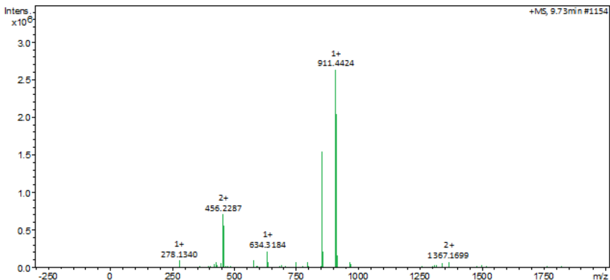
Figure A52. LC-MS analysis of 61f
