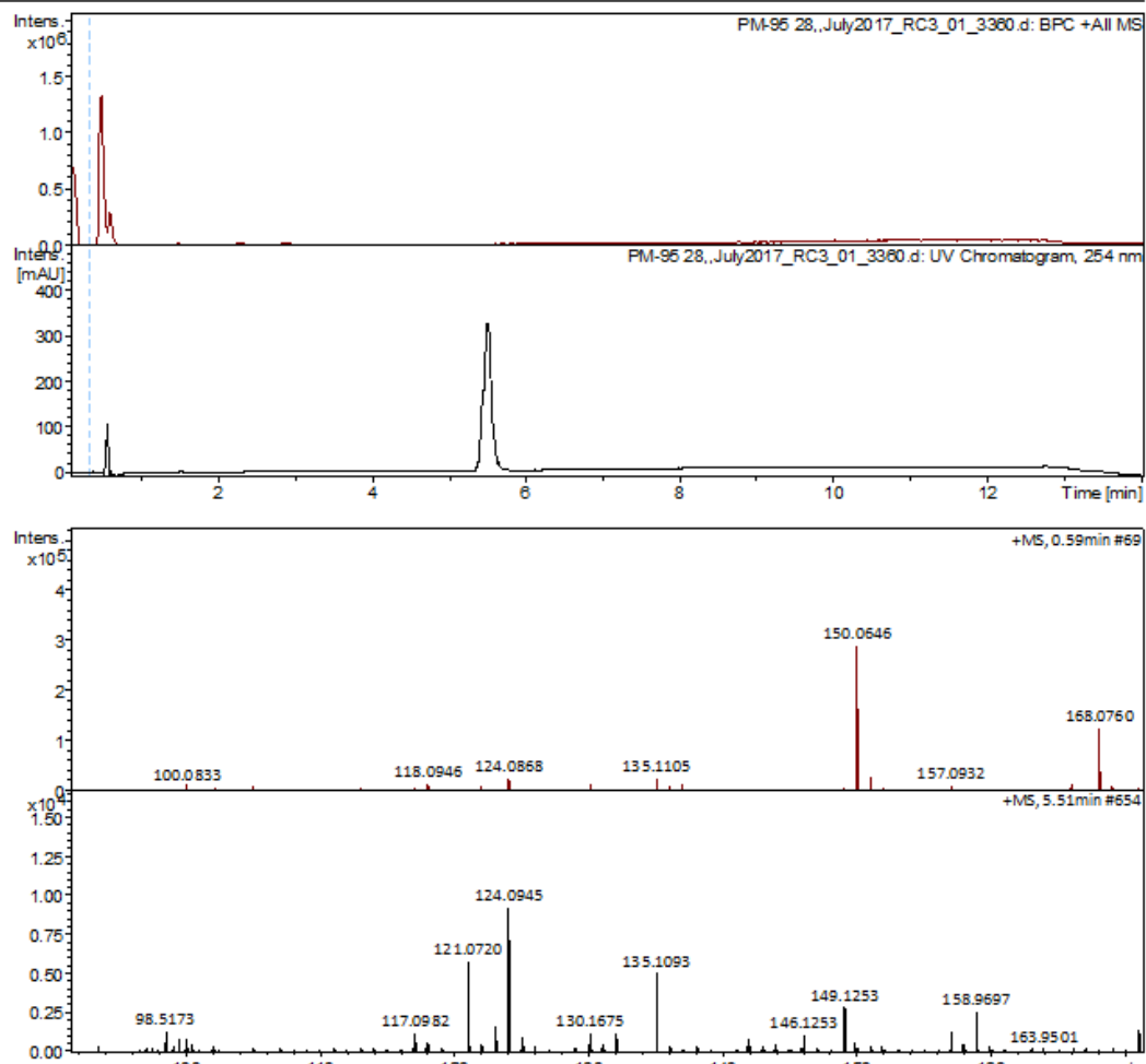
Figure A16. LC-MS analysis for reductive amination reaction involving Prozomix-TA038 at 100 mM of acetophenone
