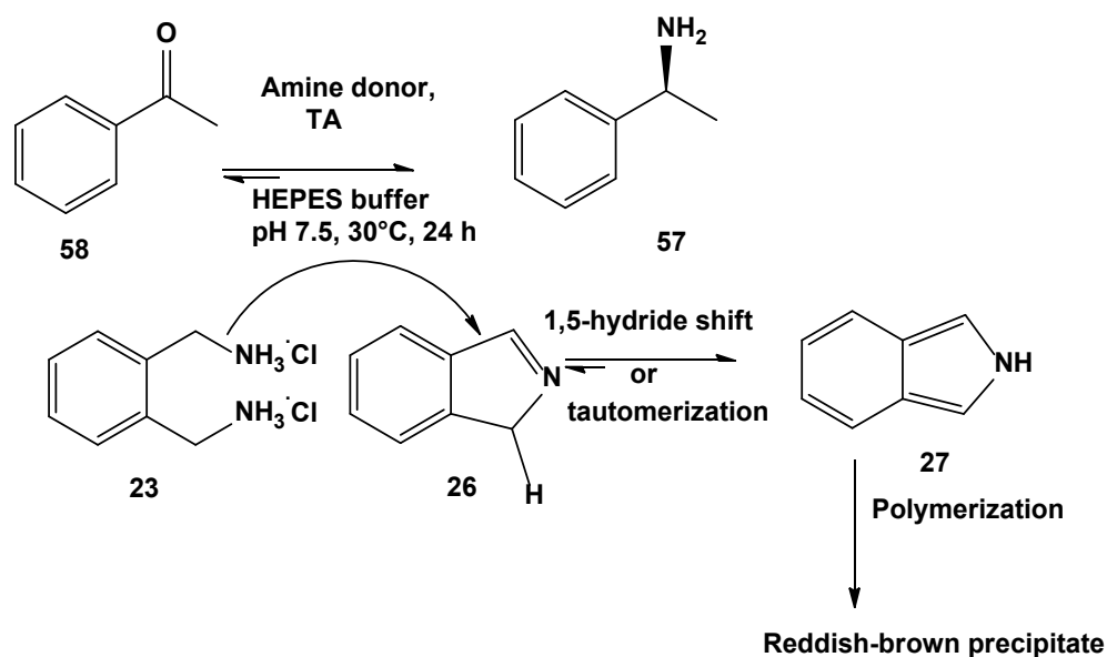
Scheme 30. Synthesis of MBA using diamine donor
