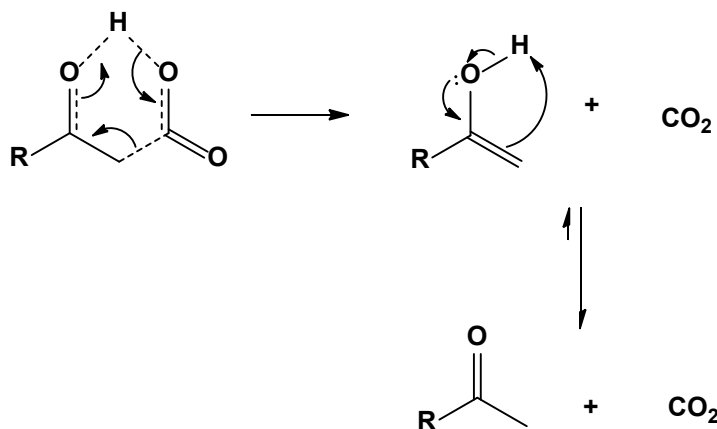
Figure 12. Decarboxylation mechanism through a cyclic transition state mechanism. 53
