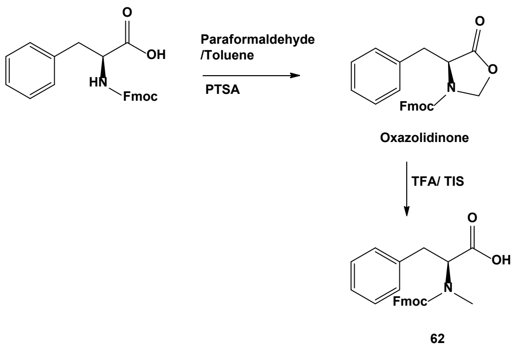
Scheme 36. Synthesis of N -methylated phenylalanine 62
