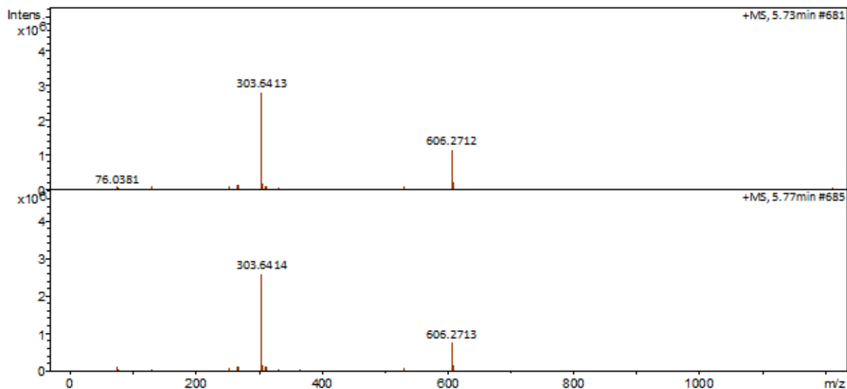
Figure A37. LC-MS analysis for GFOGRG
