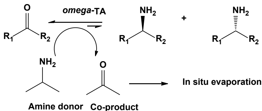
Scheme 8. Selected example for larger scale reaction using isopropylamine. 99
