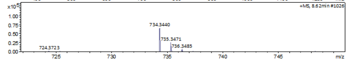
Figure A47. HRSM analysis for 61a
