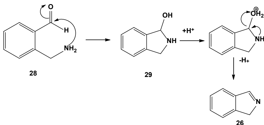
Scheme 31. 5-exo-trig cyclisation of 2-(aminomethyl) benzaldehyde
