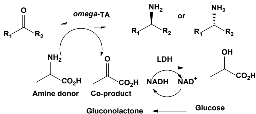
Scheme 7. Example of the removal of coproduct using LDH coupled with omega-transaminase. 77
