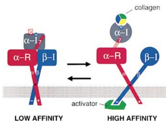
Figure 6. Diagram depicting the integrin binding site. 19
