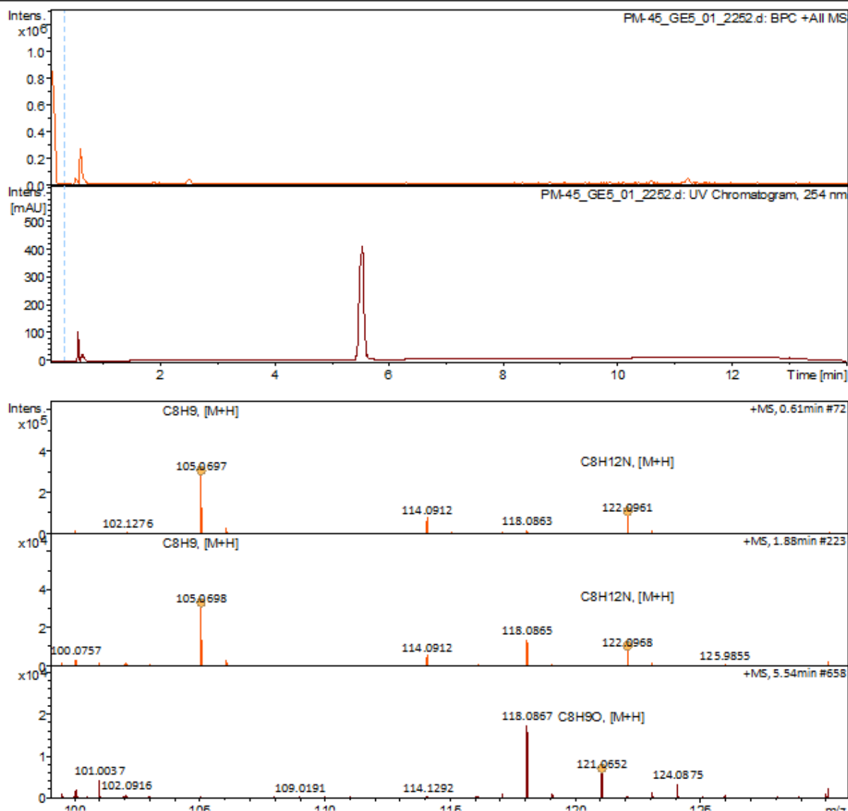
Figure A12. LC-MS analysis for reductive amination reaction involving Prozomix-TA022 at 25 mM of acetophenone
