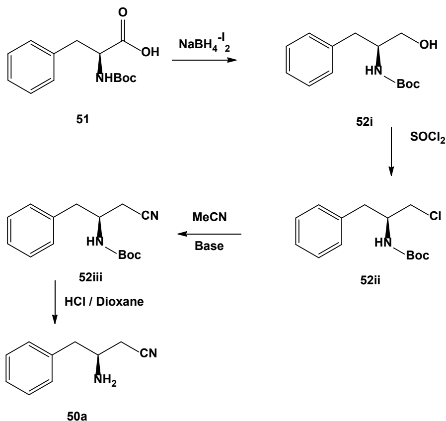
Scheme 19. Proposed route for the synthesis of 3-amino-4-phenylbutanenitrile 50a
