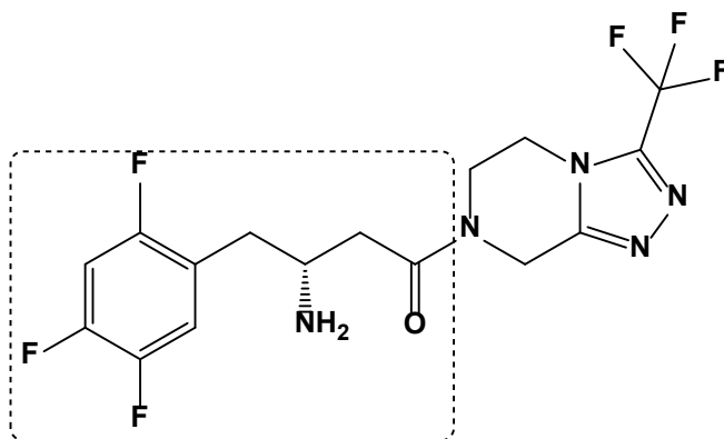
Figure 9. Structural representation of Sitagliptin.
