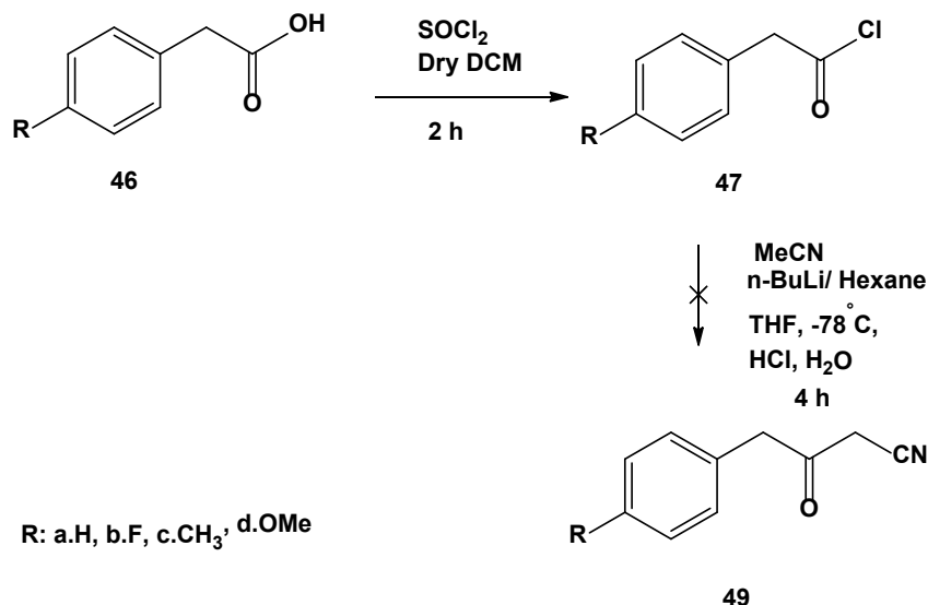
Scheme 16. Proposed synthesis of beta -ketonitriles via acyl chloride.
