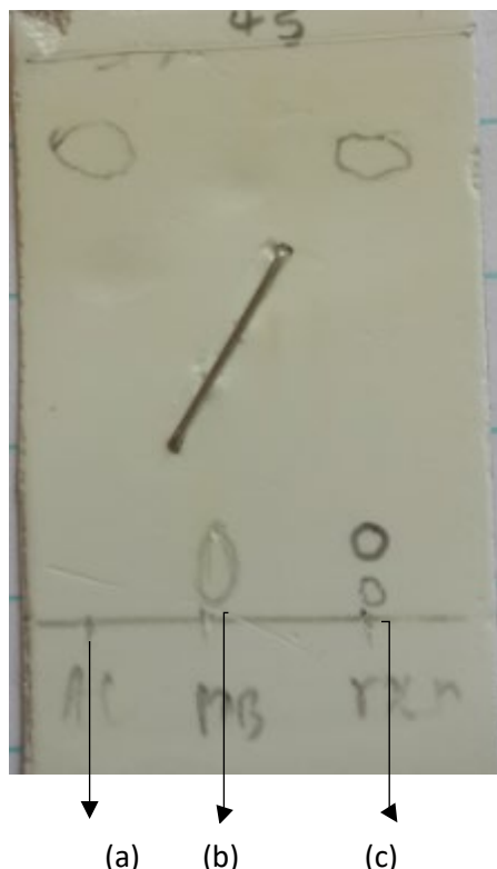
Figure A11. TLC analysis for reductive amination of 58 (30% EtOAc/hexane). (a) The acetophenone standard starting material 58 . (b) The MBA standard product 57 . (c) Reaction involving Prozomix-TA022 at 25 mM of 58 .
