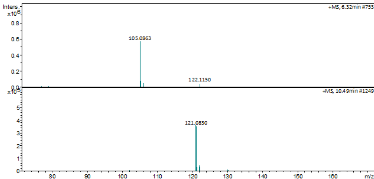
Figure A22. LC-MS analysis for reductive amination reaction involving ECS-TA06 at 10 mM of 58 using diamine donor
