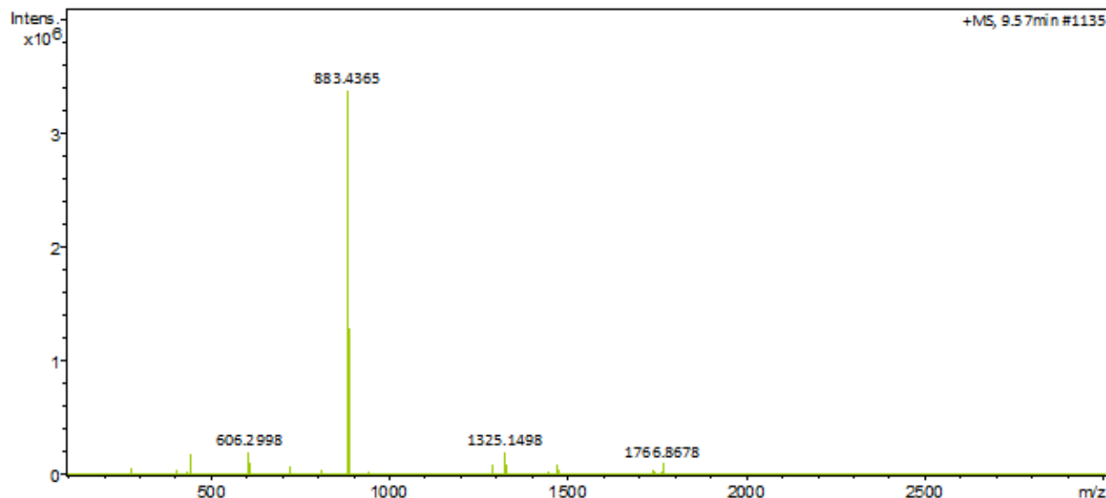
Figure A41. LC-MS analysis for GFOGRGD-Ada 60c
