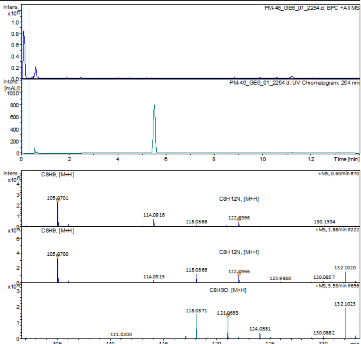
Figure A7. LC-MS analysis for reductive amination reaction involving ECS-TA02
