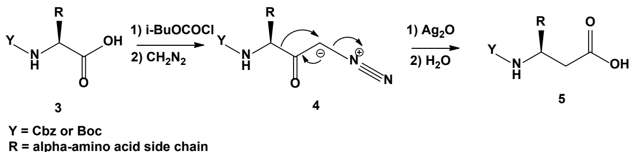
Scheme 1. Synthesis of \beta -amino acids from \alpha -amino acids via Wolff rearrangement. 61
