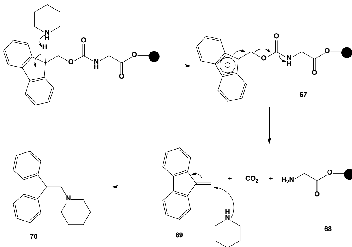
Scheme 34. Fmoc-deprotection mechanism using piperidine 139
