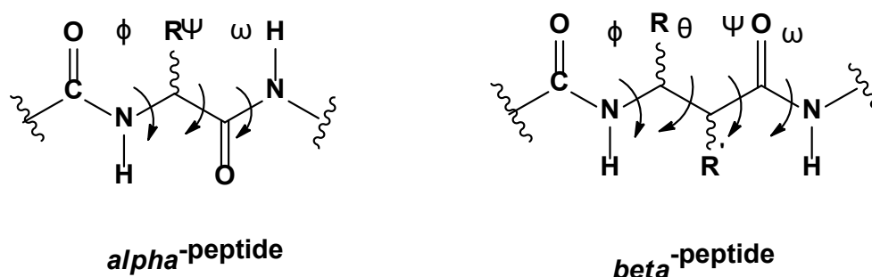
Figure 8. A diagram depicting torsion angles for alpha and beta -peptide. 3a
