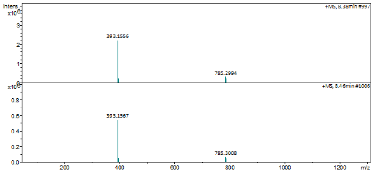
Figure A35. LC-MS analysis of GFOG
