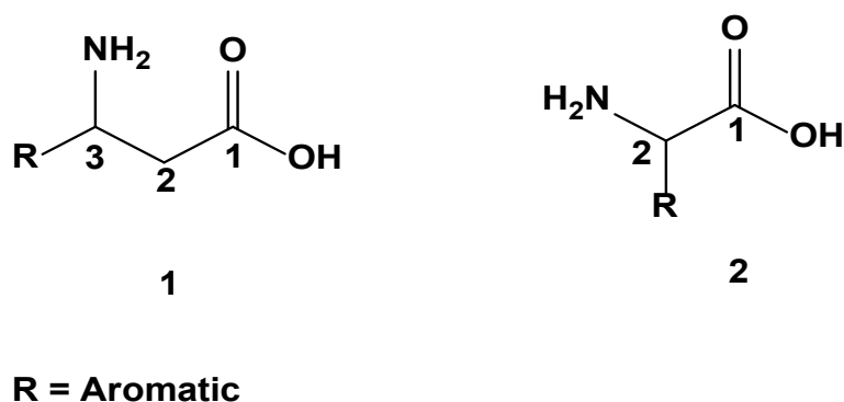
Figure 1. Illustration of \beta -amino acid ( 1 ) and \alpha -amino acid ( 2 )
