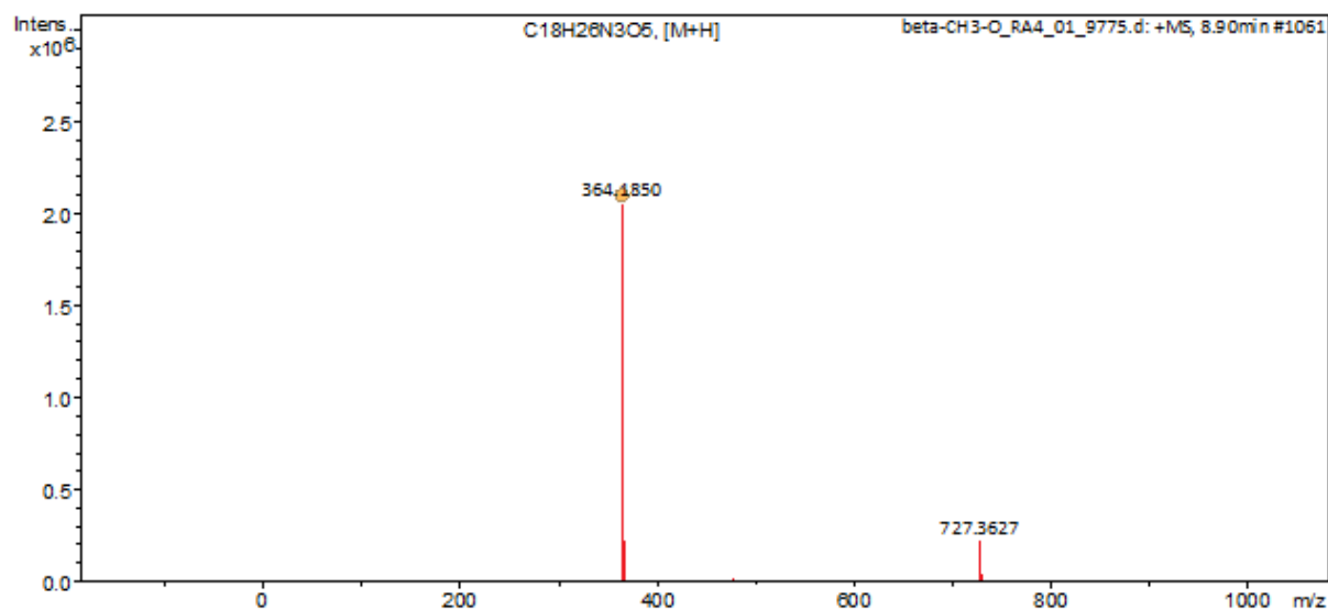
Figure A42. HMRS analysis for G-(Me)Phe-O
