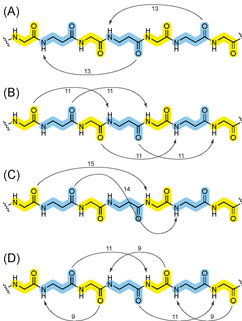
Figure 7. Intramolecular hydrogen bonding possibilities in helices of alpha and beta -amino acid containing peptides. The alpha amino acid residues are highlighted yellow while the
