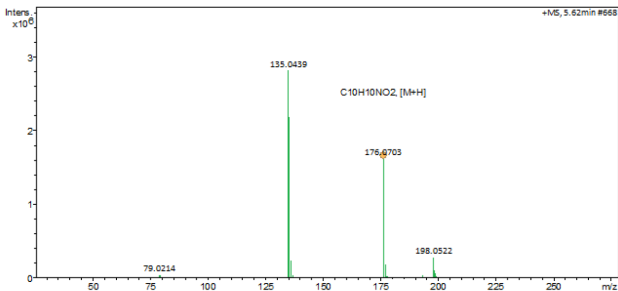
Figure A27. LC-MS analysis of standard 54b
