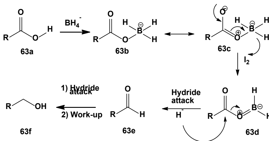
Scheme 21. Proposed mechanism involving NaBH 4 -I 2
