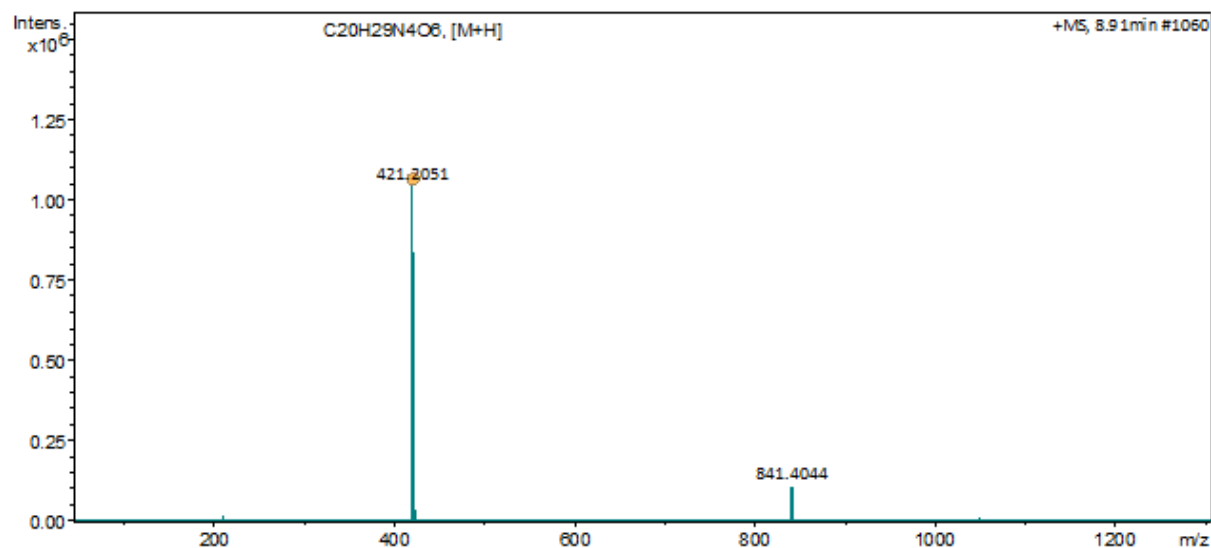
Figure A43. LC-MS analysis for G-(Me)Phe-O-G
