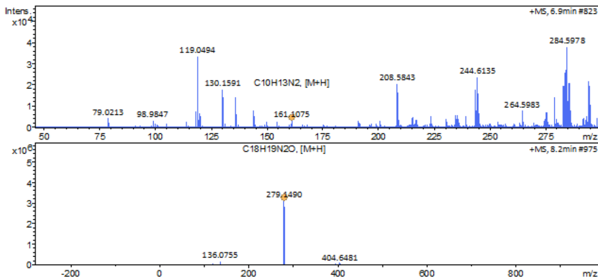
Figure A26. LC-MS analysis for reductive amination reaction involving Prozomix-TA042 at 10 mM of 54a using diamine donor
