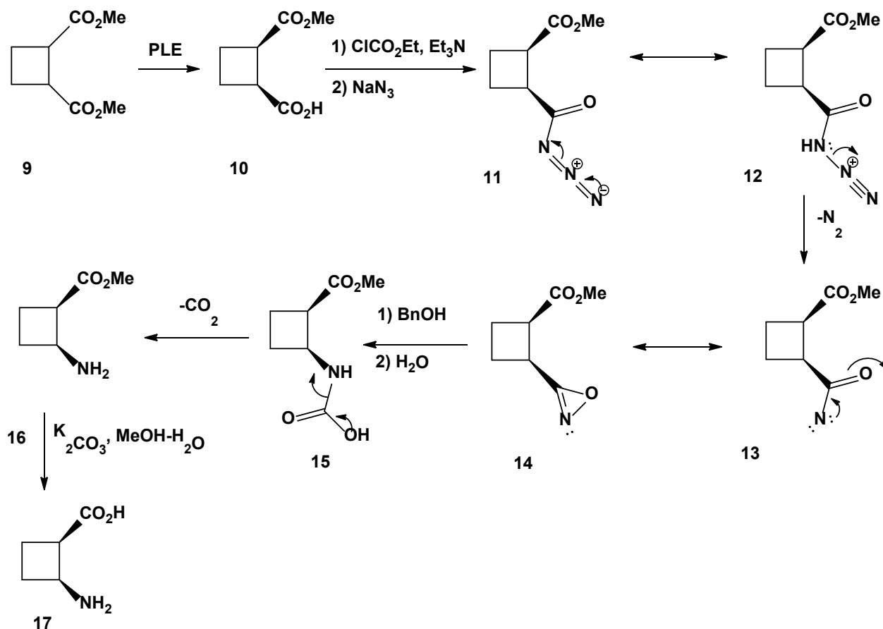
Scheme 3. A stepwise Curtius rearrangement of di-esters 9 . 64,65,66
