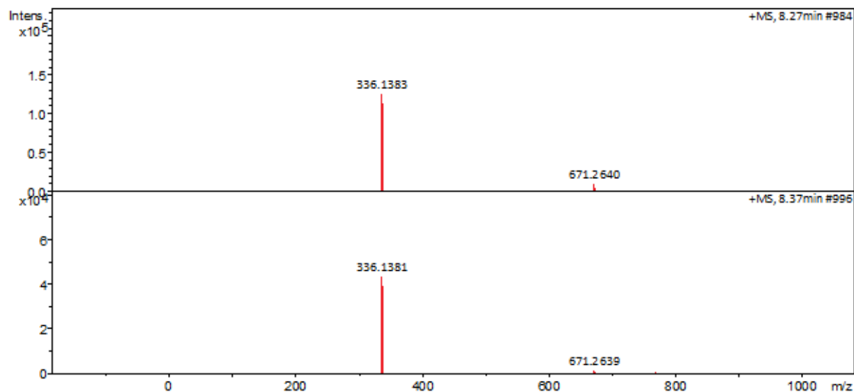
Figure A34. LC-MS analysis of GFO
