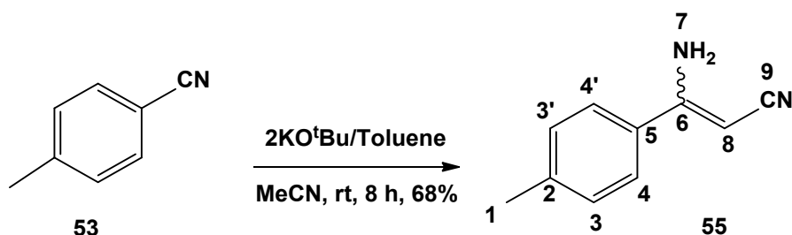
Scheme 25. Synthesis of enamine using \text{KO}^t\text{Bu} /toluene
