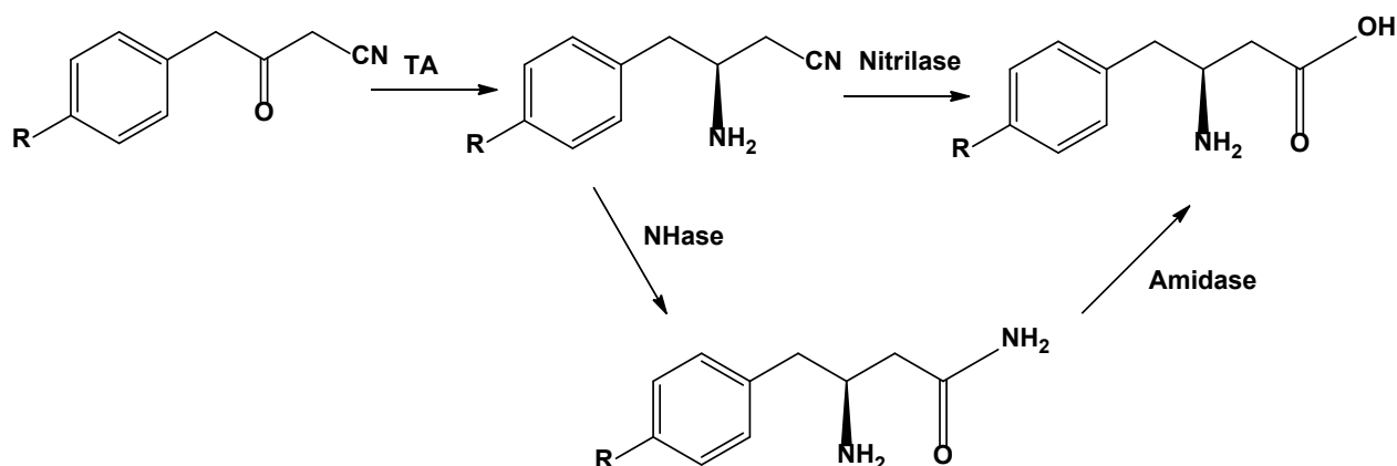
Scheme 14. RAH reaction cascade
