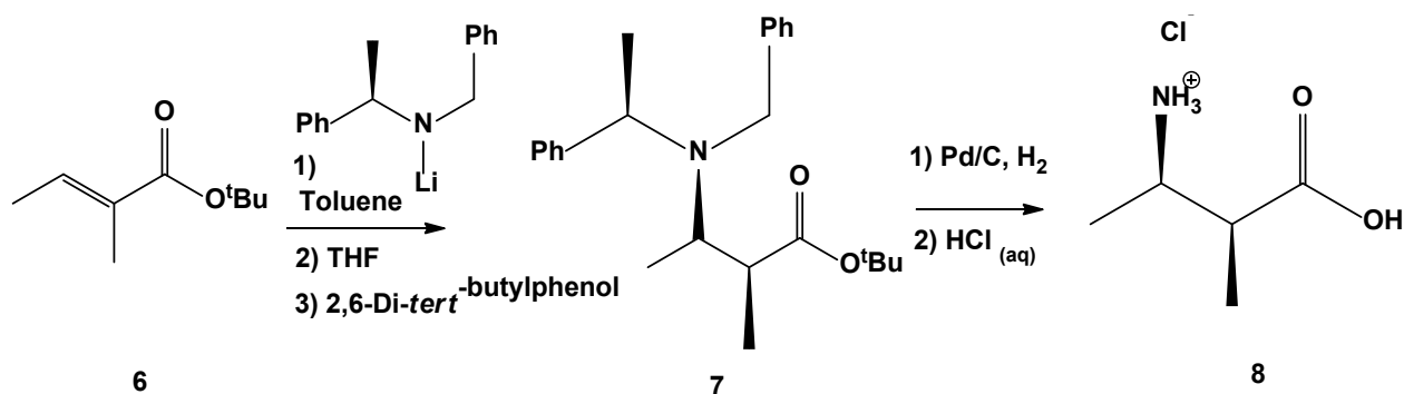
Scheme 2. Michael addition of the enantiopure amine. 41
