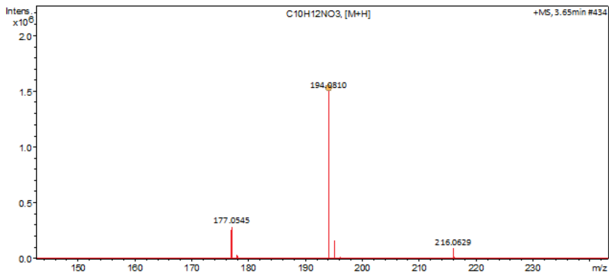
Figure A33. LC-MS of hydrolysis of 54d
