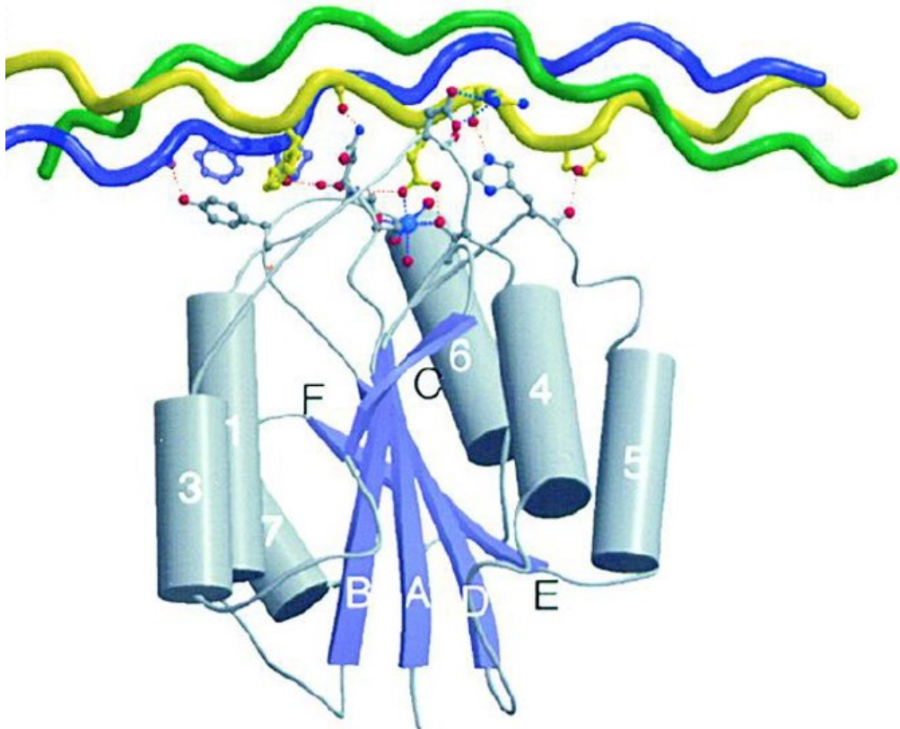
Figure 4. A schematic of the detailed collagen-integrin interface, reproduced from Ref 19,19
