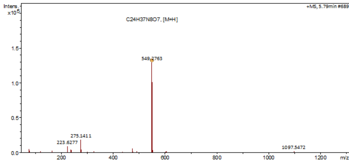
Figure A36. LC-MS analysis of GFOGR
