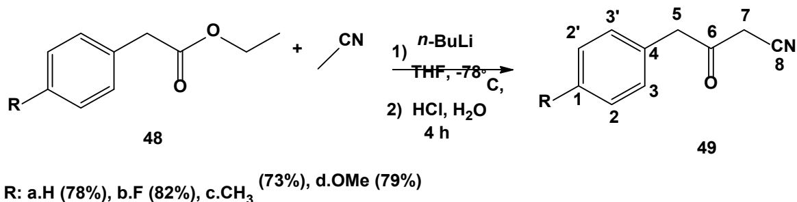
Scheme 18. Synthesis of \beta -ketonitriles from ester precursors
