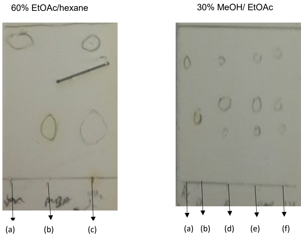
Figure A17. TLC for reductive amination of acetophenone using LDH mixture; (a) Acetophenone standard starting material . (b) MBA standard product . (c) Reaction involving ECS-TA05 with Acetophenone (50 mM) . (d) Reaction involved Prozomix-TA016 with Acetophenone (50 mM) . (e) Reaction involved Prozomix-TA045 with Acetophenone (50 mM) . (f) Reaction involved Aspergillus fumigatus with Acetophenone (50 mM) .
