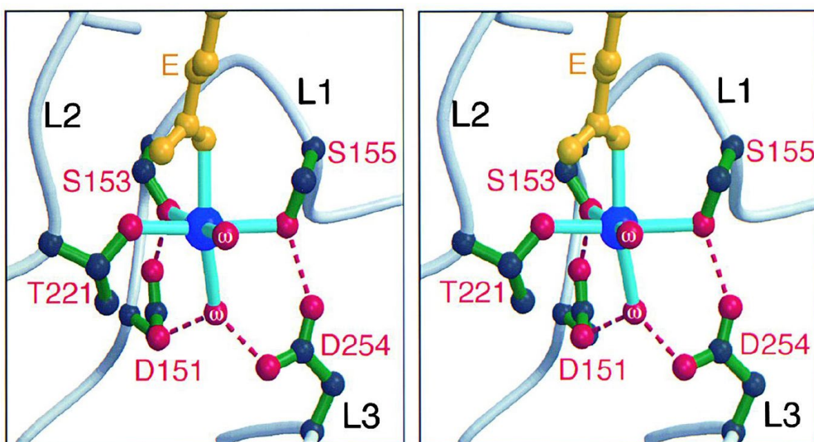
Figure 5. A stereo molecular diagram representing MIDAS. Reproduced from Ref 19 .
