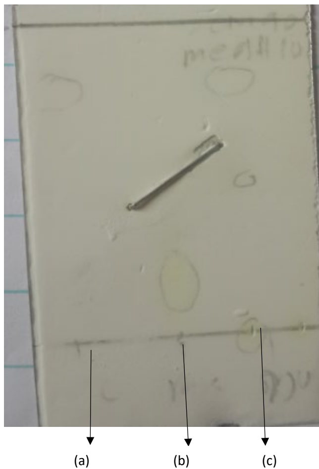
Figure A18. TLC analysis of reaction involving Prozomix-048 with 58 (10 mM) (c) (10% MeOH/EtOAc). (a) Acetophenone standard , (b) MBA standard
