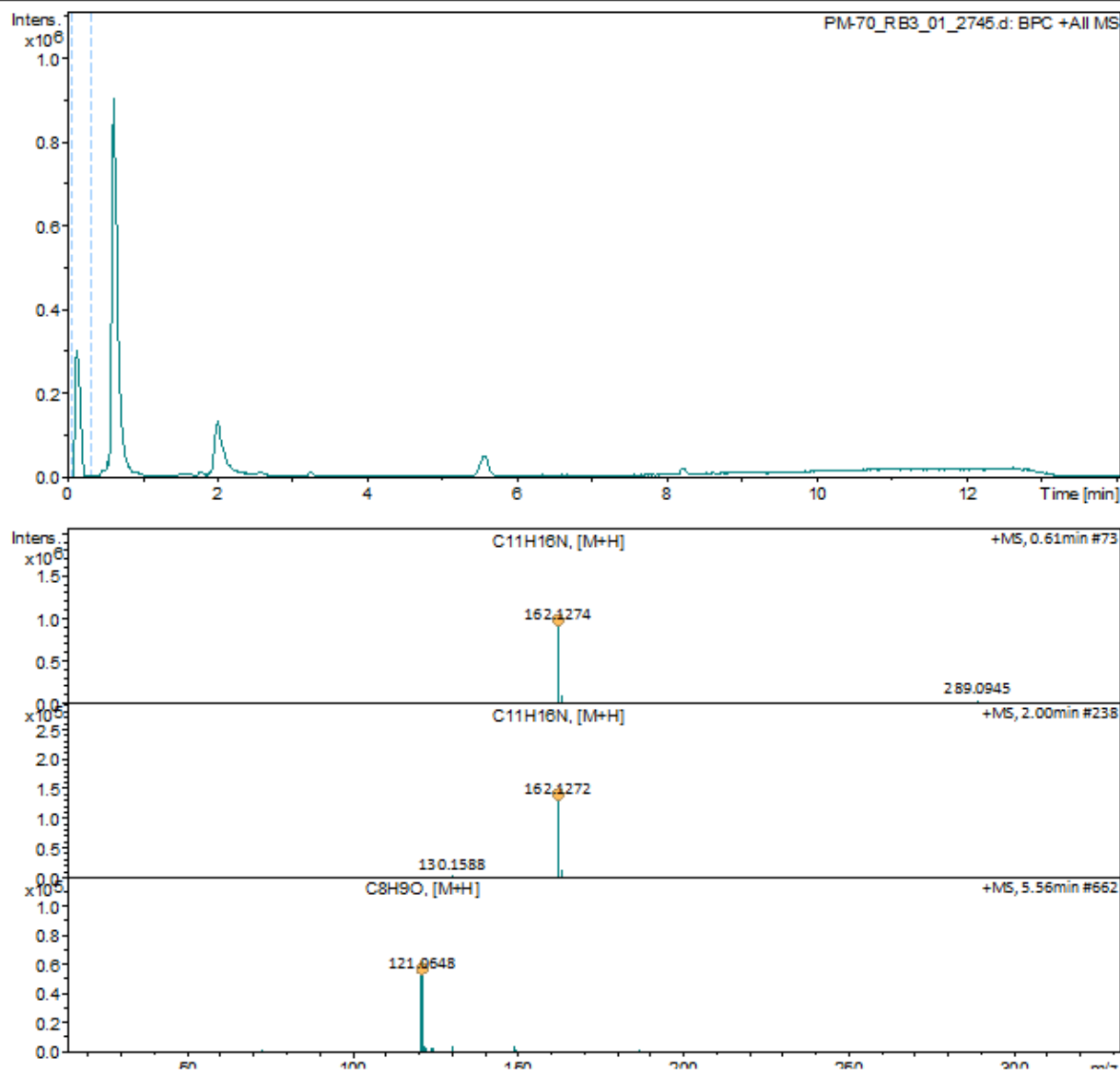
Figure A19. LC-MS analysis for reductive amination reaction involving Prozomix-TA048 with 58 (10 mM)
