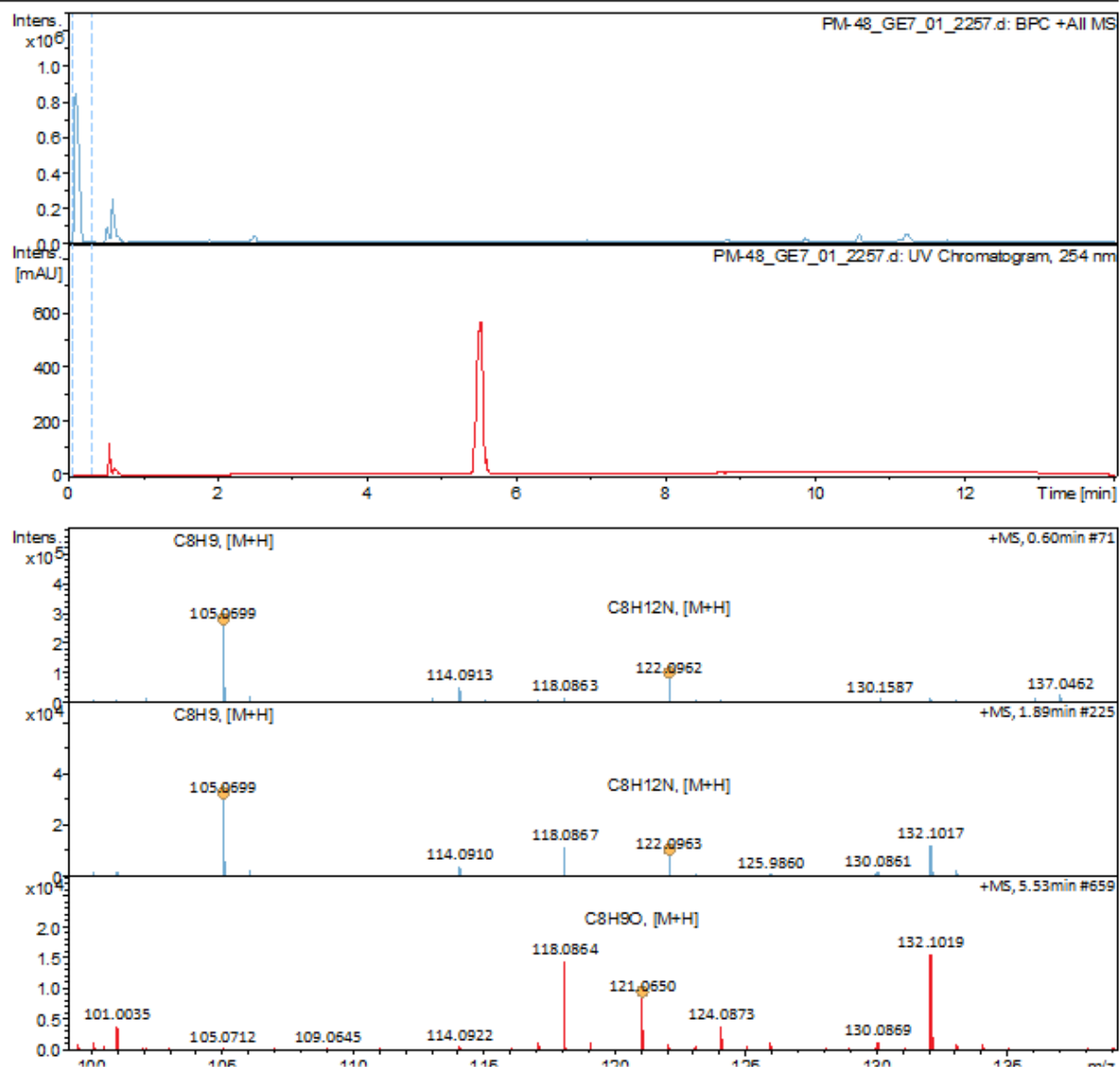
Figure A8. LC-MS analysis for reductive amination reaction involving Prozomix-TA024
