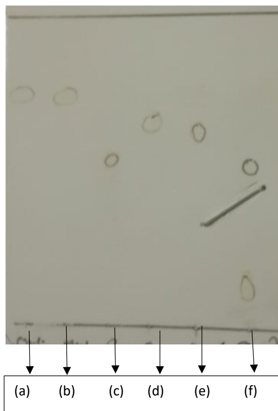
Figure A30. TLC analysis for hydrolysis of 56c and 66 (40% EtOAc/Hexane); (a) Standard starting material 54c . (b) Standard starting material 54d . (c) Standard starting material 56c . (d) Reaction for hydrolysis of 54c . (e) Reaction for hydrolysis of 54d . (f) Reaction for hydrolysis of 56c .
