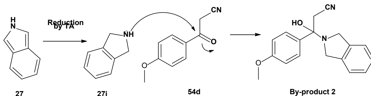
Scheme 33. Mechanism of the side-reaction between starting material 54d and the isoindole
