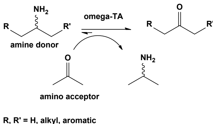
Scheme 4. Deamination of amino group involving transaminases. 78
