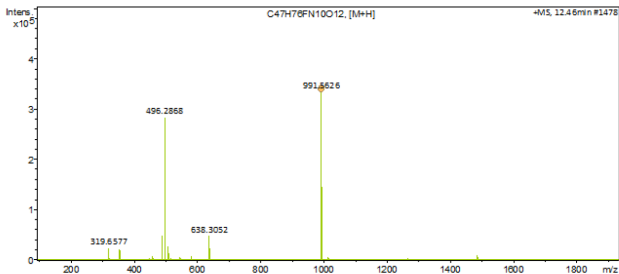
Figure A54. LC-MS analysis of 61h
