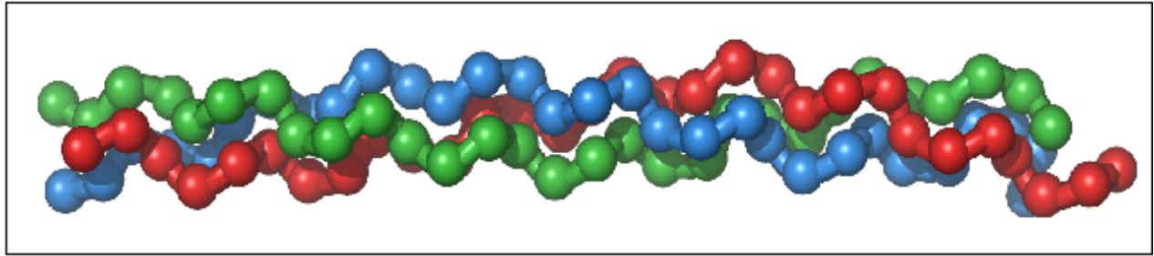
Figure 3. A diagram of collagen peptides triple helix in complex ( http://www.ebi.ac.uk/interpro/potm/2009_1/Protein_focus_2009_01-Collagen.html ).
