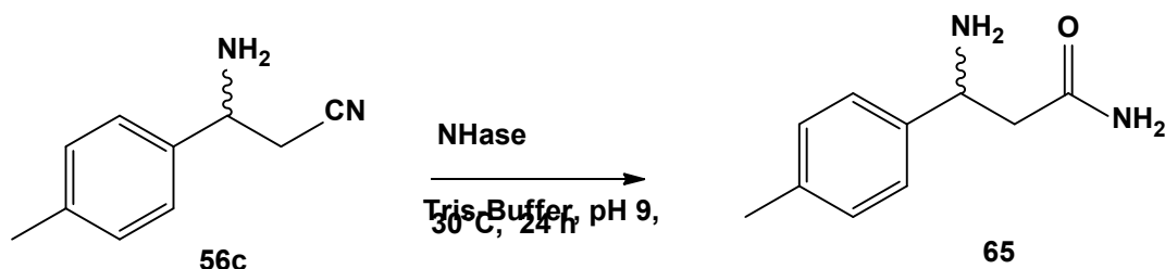
Scheme 34. Hydrolysis of \beta -aminonitrile 56c using NHase
