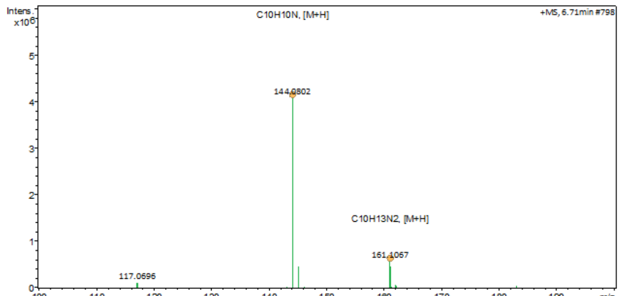
Figure A24. LC-MS analysis for standard 56c
