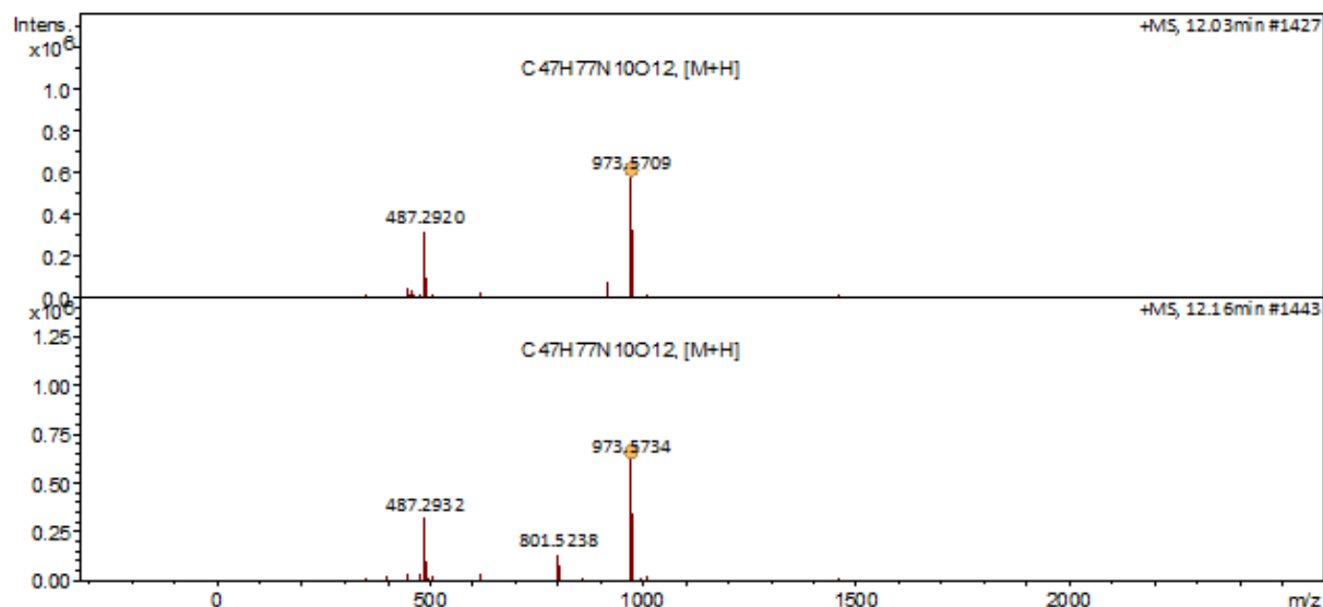
Figure A48. LC-MS analysis for 61b
