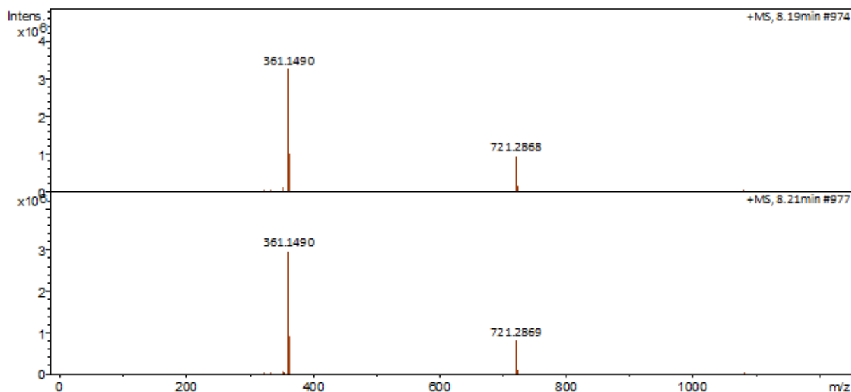
Figure A38. LC-MS analysis of GFOGRGD
