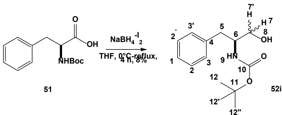
Scheme 20. Reduction of Boc-phenylalanine using \text{NaBH}_4\text{-I}_2 , 8% yield.
