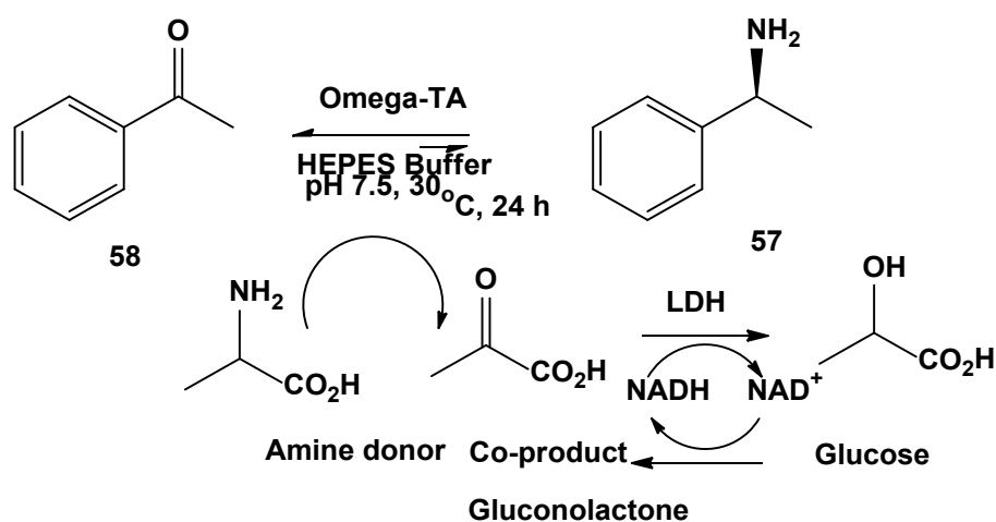
Scheme 29. Reductive amination of acetophenone using LDH mixture
