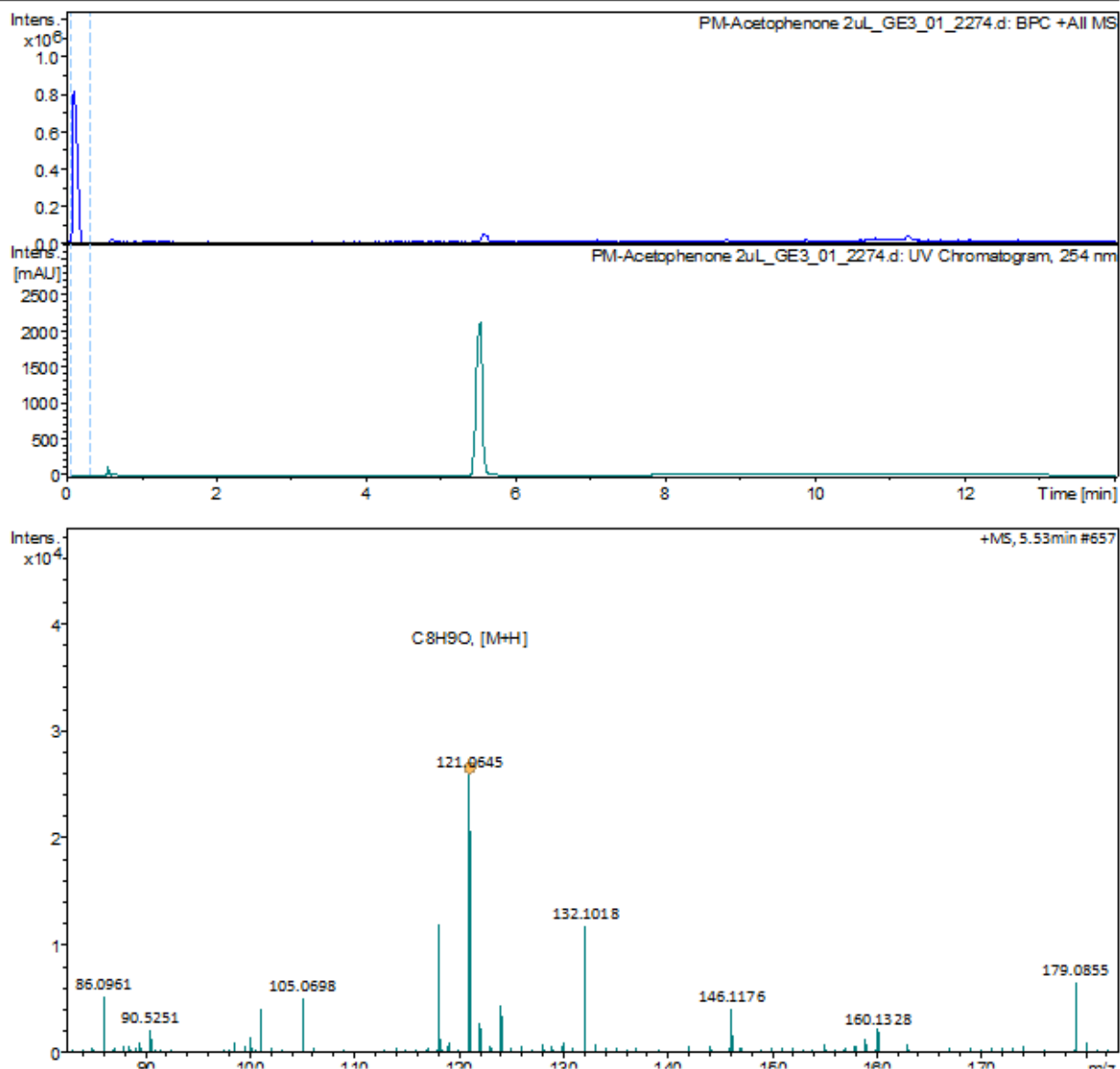
Figure A2. LC-MS data for the standard acetophenone 58
