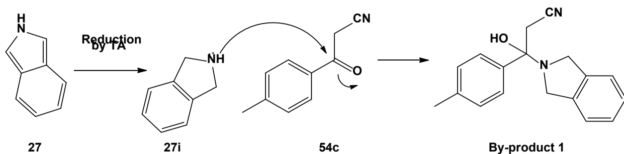
Scheme 32. Mechanism of the side-reaction between starting material 54c and the isoindole
