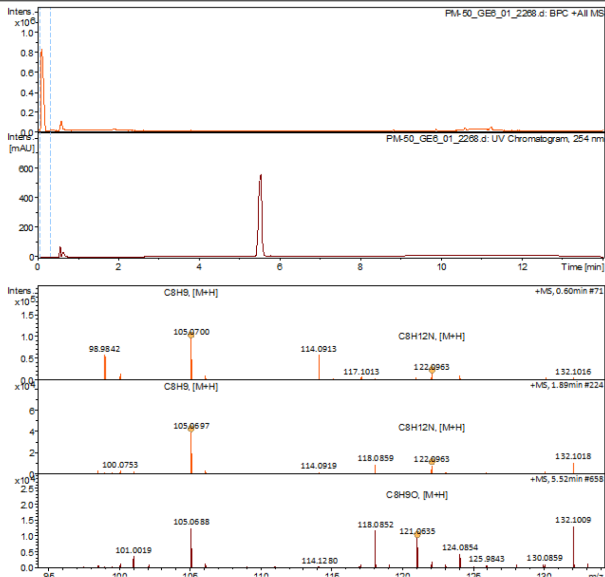
Figure A14. LC-MS analysis for reductive amination reaction involving Prozomix-TA024 at 50 mM of acetophenone
