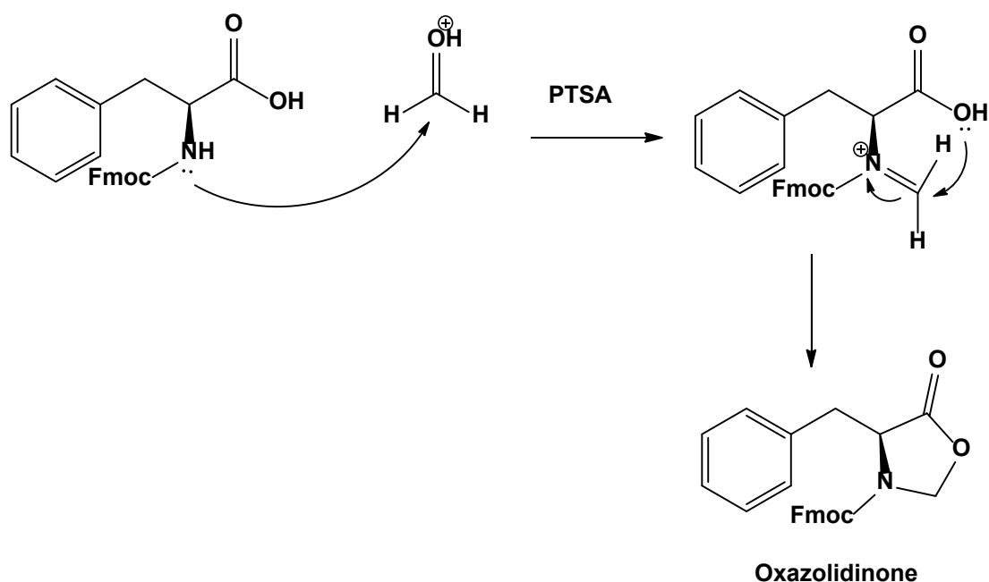
Scheme 37. Proposed mechanism of the formation of oxazolidinone
