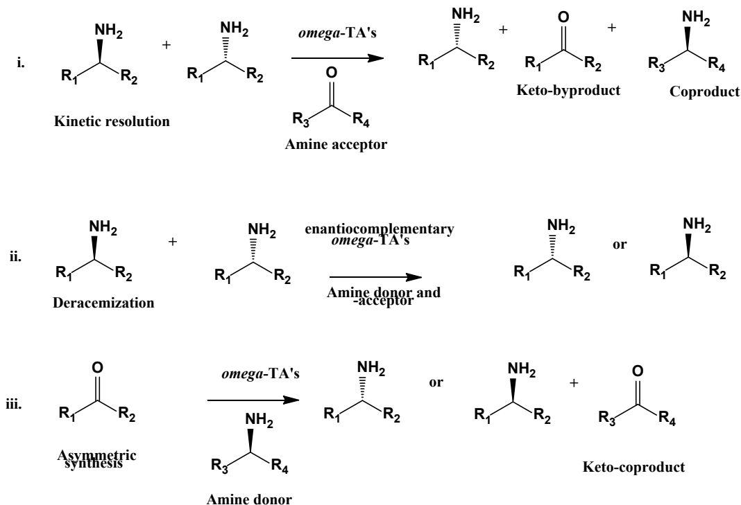
Scheme 6. Different methods for the biotransformation of substrates into pure enantiomers. 74
