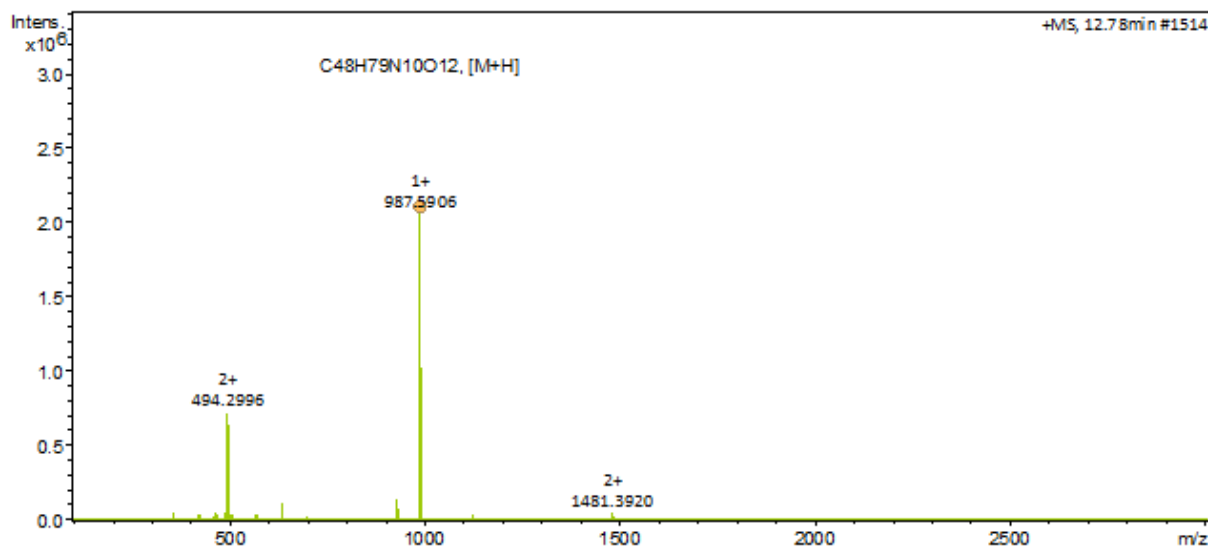
Figure A51. LC-MS analysis of 61e
