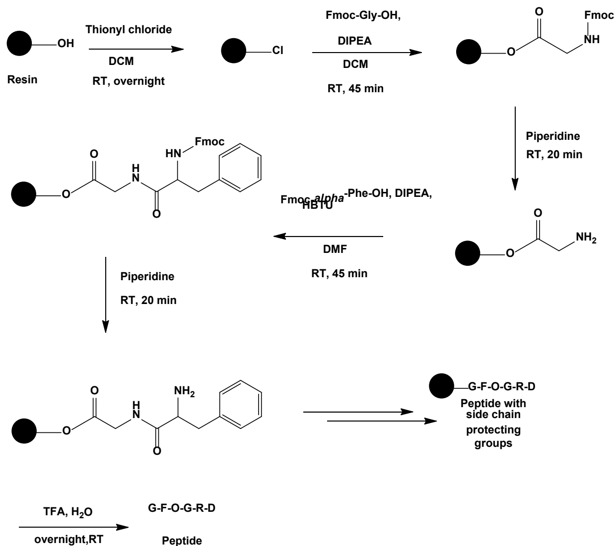
Scheme 33. Synthesis of wound healing peptides
