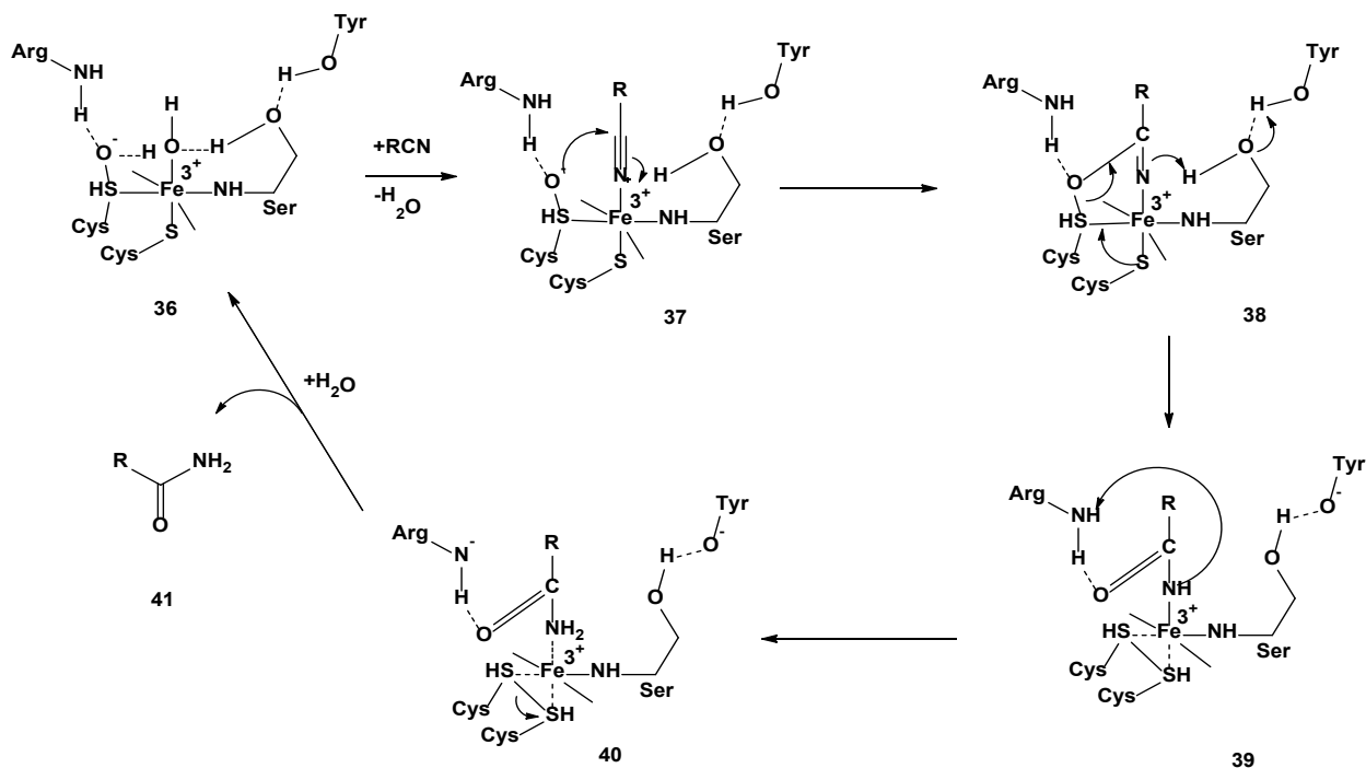
Scheme 12. The NHase mechanism for conversion of nitrile to amide. 106
