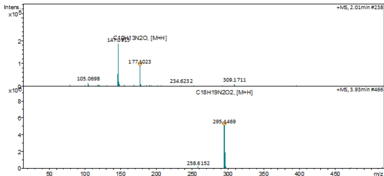
Figure A29. LC-MS analysis for reductive amination reaction involving Prozomix-TA011 at 10 mM of 54b using diamine donor
