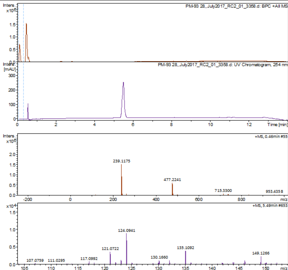
Figure A6. LC-MS analysis for Prozomix-TA018 reduction amination reaction of 58
