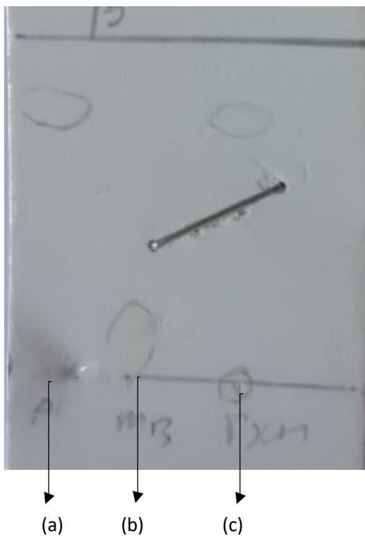
Figure A15. TLC analysis for reductive amination of 58 (30% EtOAc/hexane). (a) Acetophenone standard starting material. (b) MBA standard product. (c) Reaction involving Prozomix-TA038 at 100 mM of acetophenone
