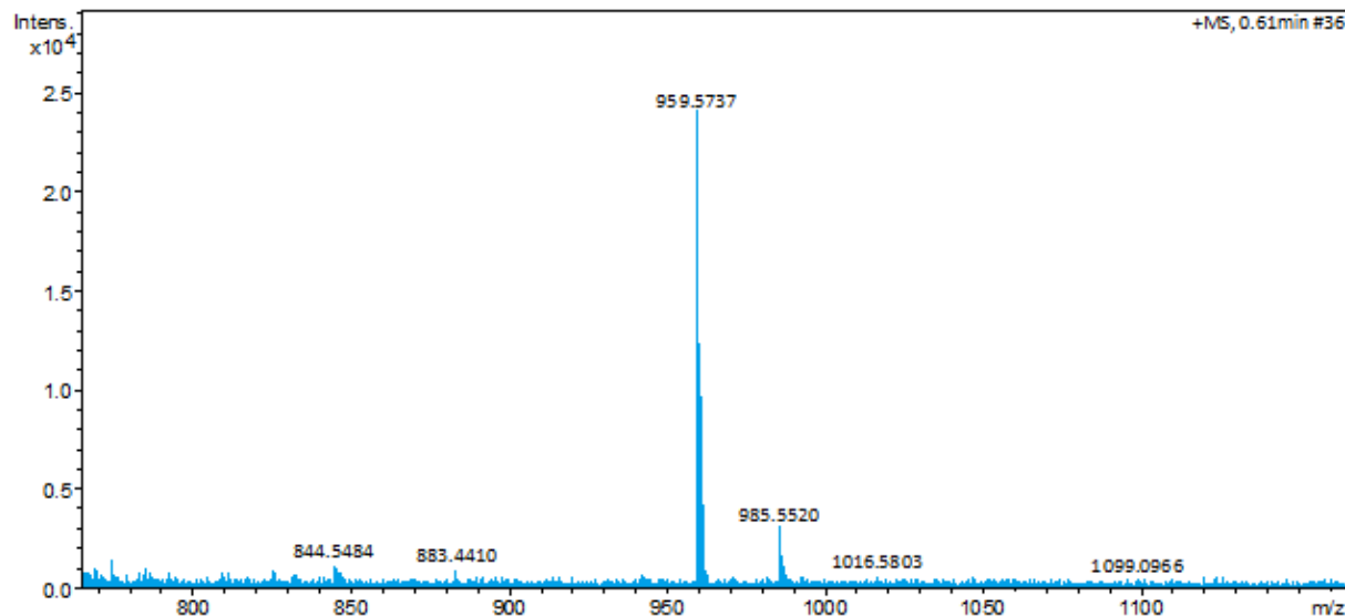
Figure A40. LC-MS analysis of GFOGRGD-Pal 60b
