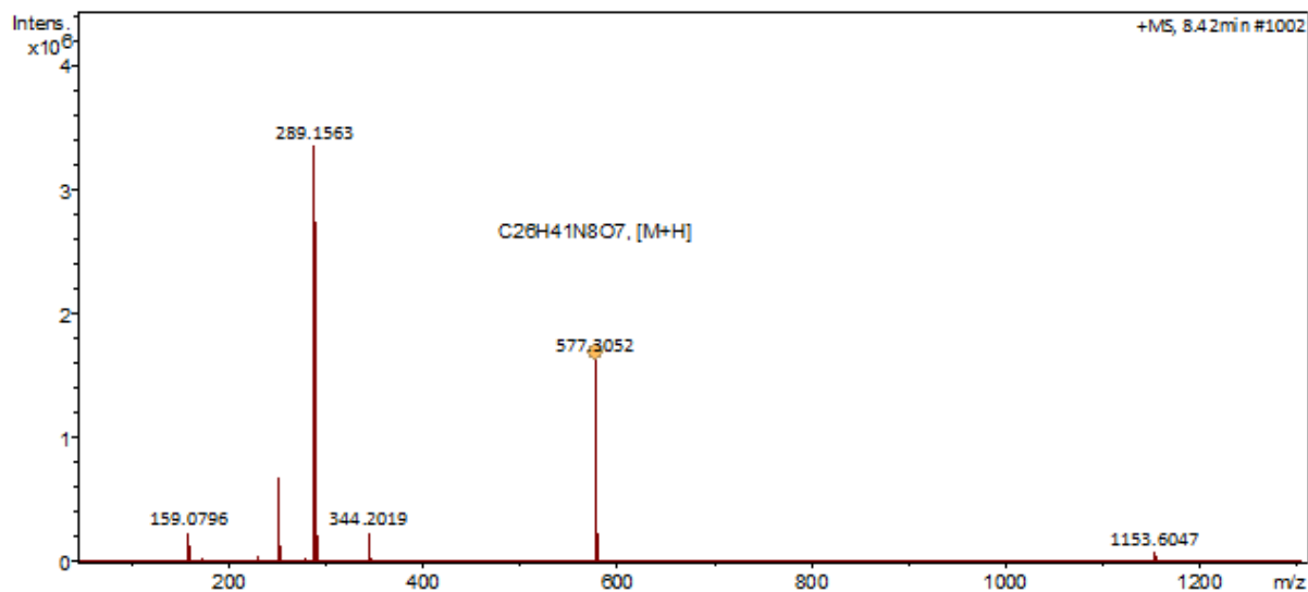
Figure A44. LC-MS analysis for G-(Me)Phe-O-G-R
