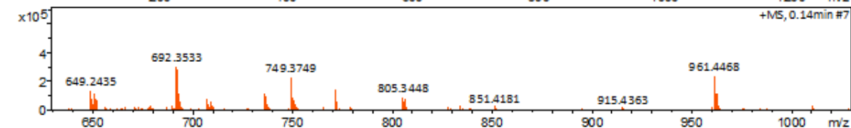
Figure A55. LC-MS analysis of 61i
