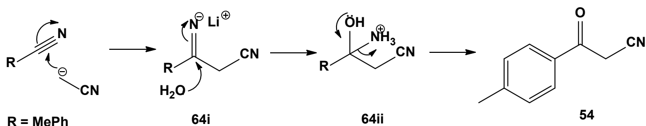
Scheme 24. Proposed mechanism for the formation of ketone during work-up
