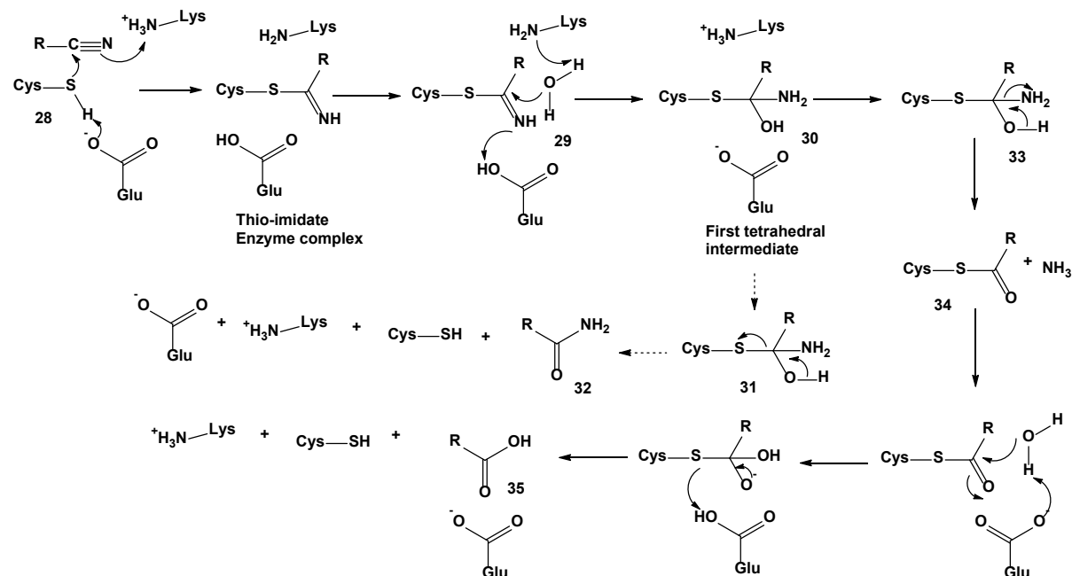
Scheme 11. Nitrilase hydrolysis mechanism for nitrile substrates. 101
