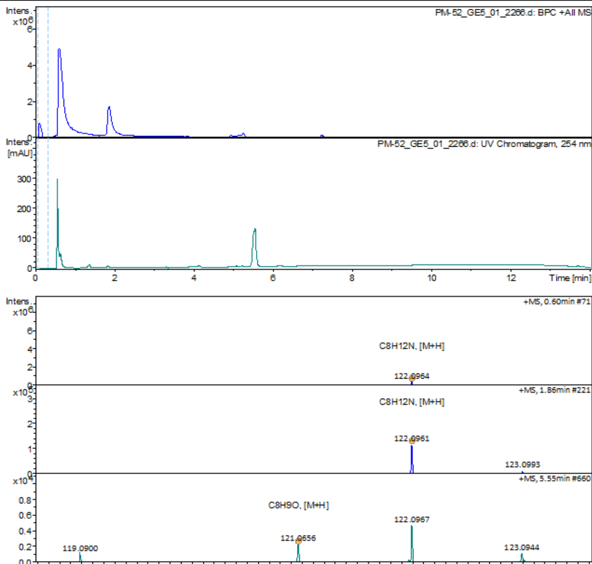
Figure A4. LC-MS analysis for deamination reaction of S-MBA involving Prozomix-TA045
