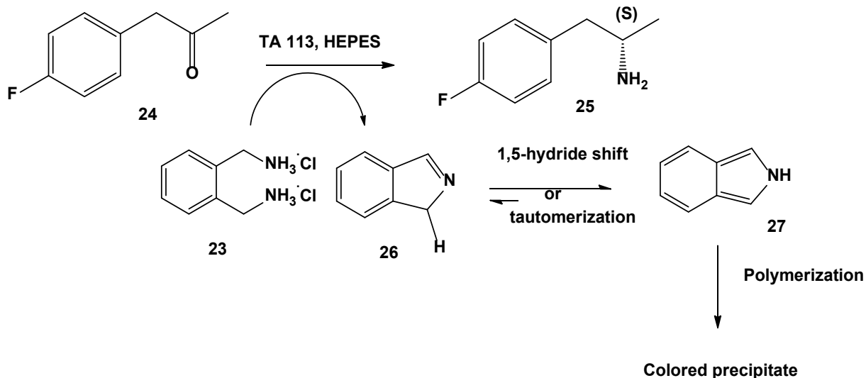
Scheme 9. Conversion of 24 into (S)- 25 using diamine donor ( 23 ) at 1.1 equivalent. HEPES = 4-(2-hydroxyethyl)-piperazine-1-ethanesulfonic acid. 99
