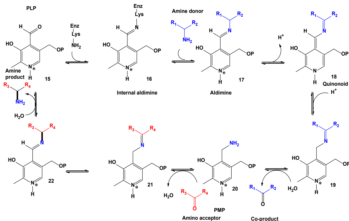
Scheme 5. The schematic representation of transaminases mechanism involving the PLP cofactor. 84
