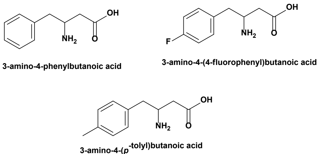
Figure 18. Purchased aromatic \beta -amino acids
