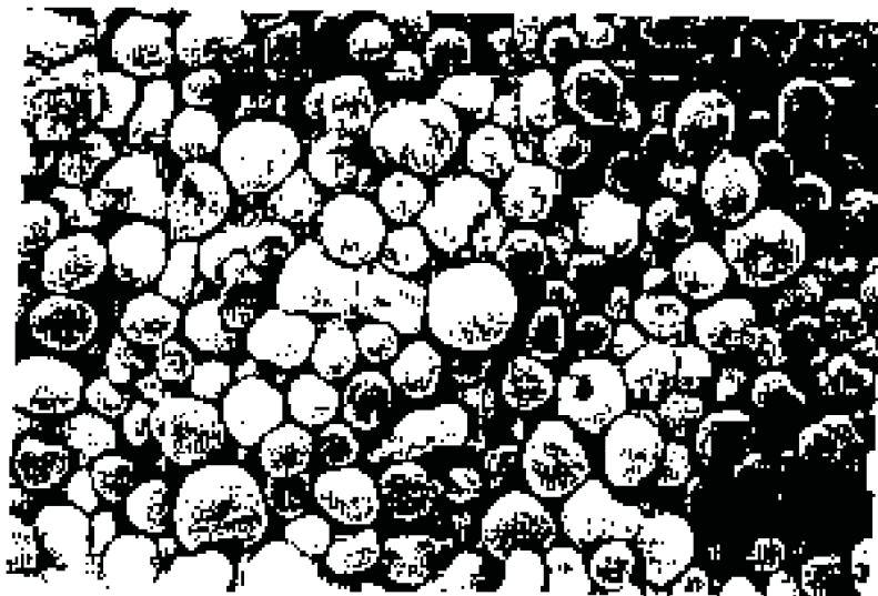
Figure 3.18 : Scanning Electron Micrograms of catalyst prepared with the commercial cobalt nitrate
