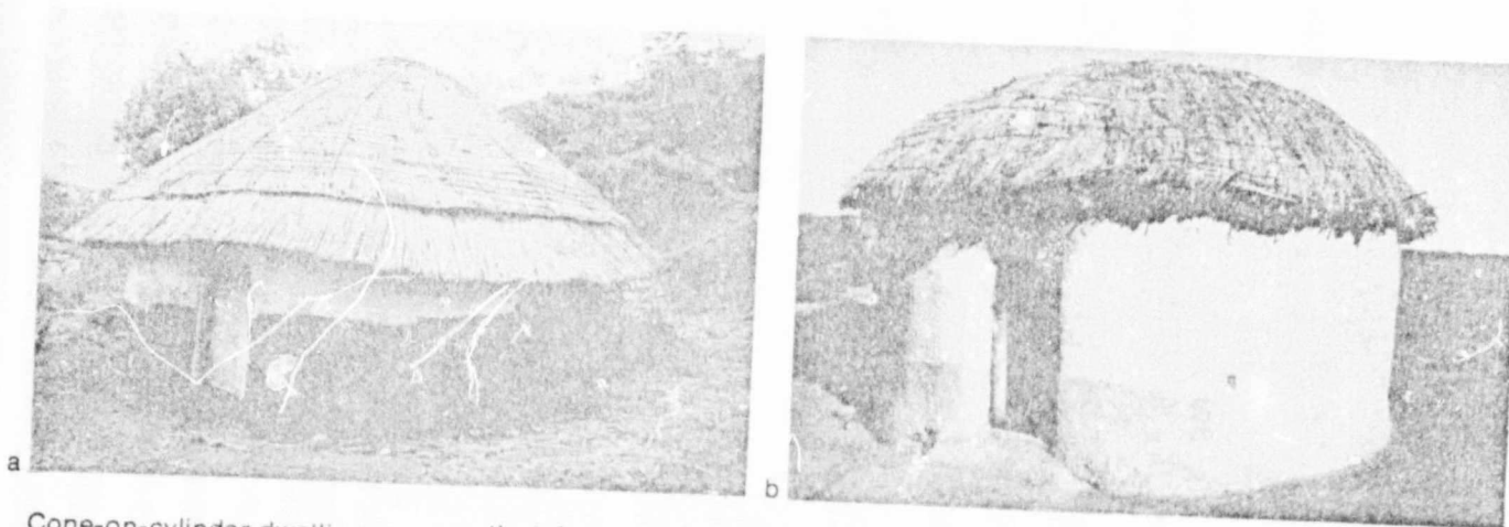
Cone-on-cylinder dwellings, thatch held down by a rope network:
