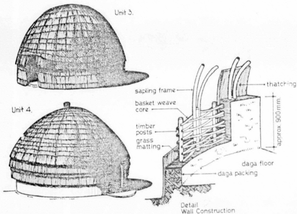
Beehive dome on minor cylinder: Units 3 and 4.
