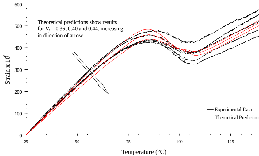
Figure G.9: Comparison between predicted strain variation and experimental data
