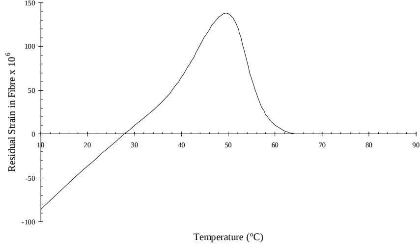
Figure 4.4: Variation in the residual strain in the fibre with temperature
