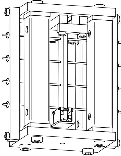
Figure 5.24: Final configuration of test frame
