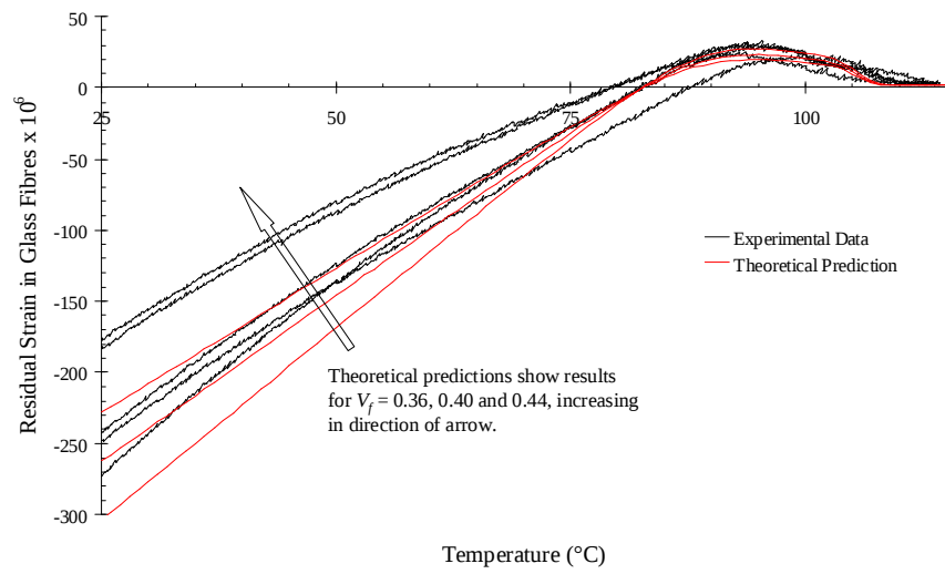
Figure G.6: Comparison between predicted residual strain variation and experimental data
