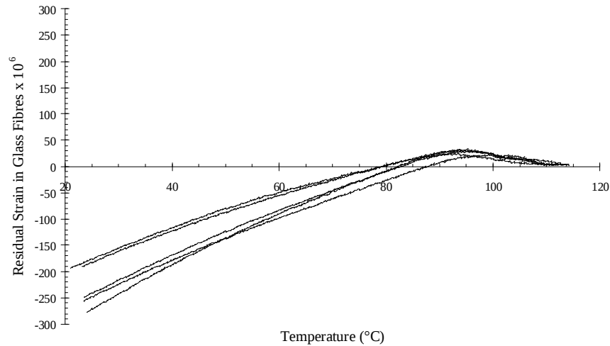
Figure F.5: Residual strain in glass fibres of unloaded specimens
