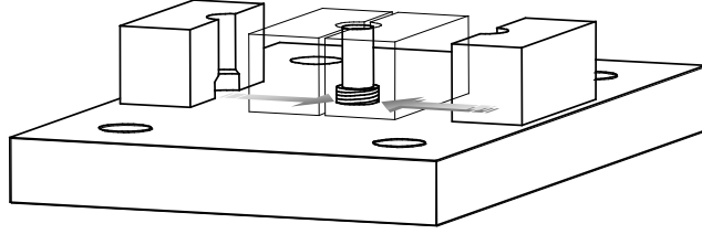
Figure 5.25: Fitment of spacer blocks around sensor
