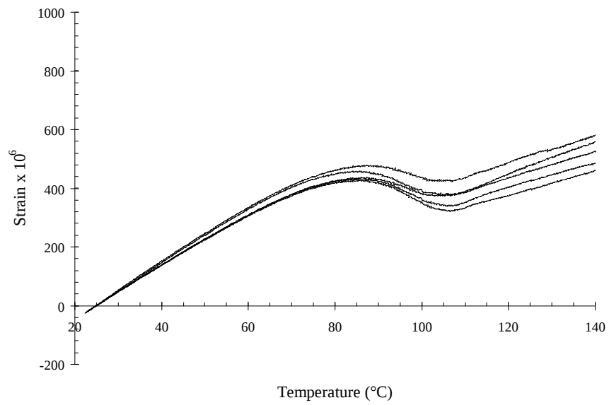
Figure 6.4: Measured strain in preloaded specimens
