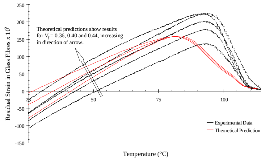
Figure 6.25: Comparison between predicted residual strain variation and experimental data - Annealed specimens
