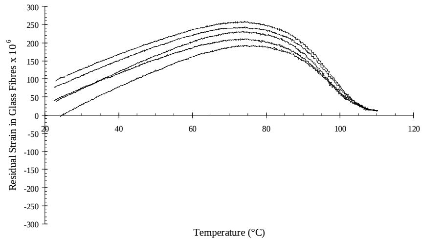
Figure 6.18: Residual strain in glass fibres of preloaded specimens
