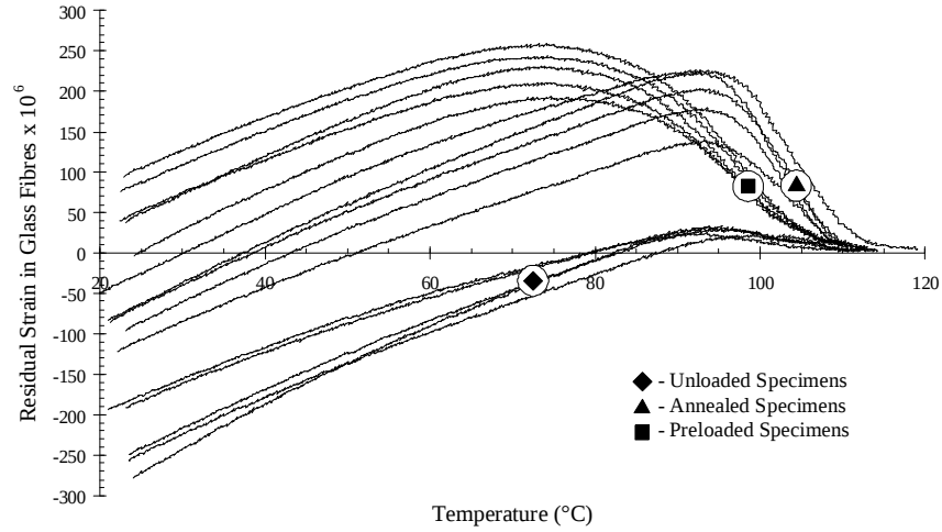
Figure 6.20: Comparison between residual strains in glass fibres of different specimen types
