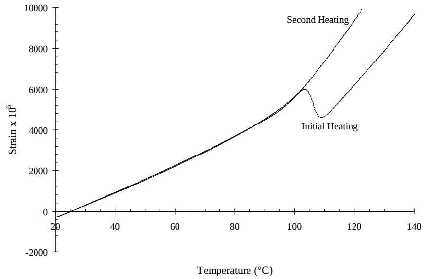
Figure 6.1: Measured strain in cast resin as a function of temperature
