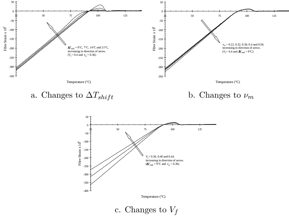
Figure G.3: Response of the fibre strain to changes in matrix and laminate properties
