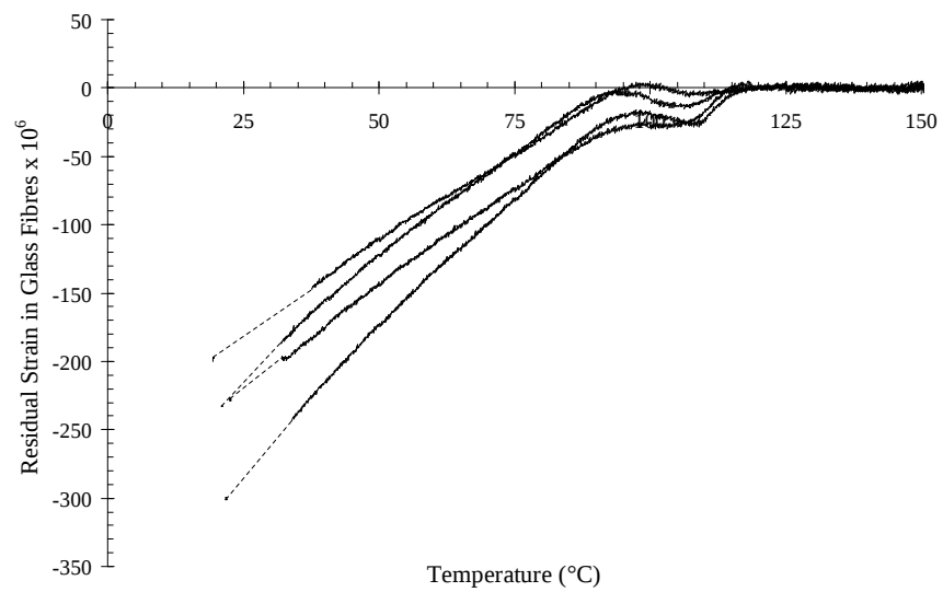
Figure 5.20: Residual strain in glass fibres of unloaded specimens
