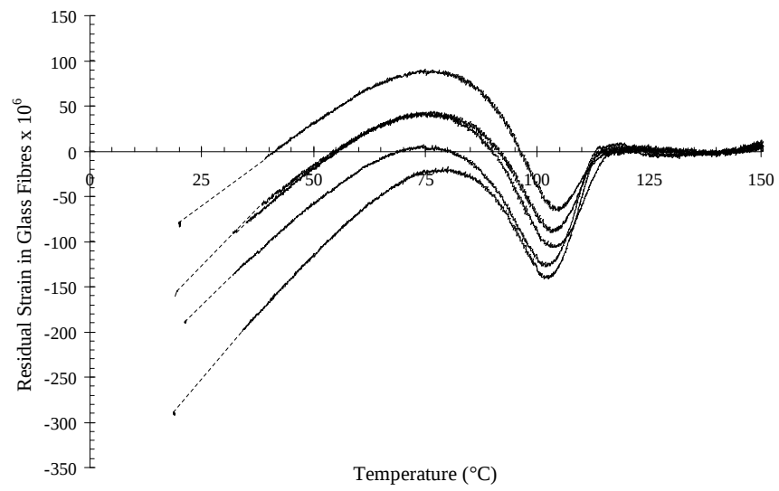
Figure 5.21: Residual strain in glass fibres of preloaded specimens
