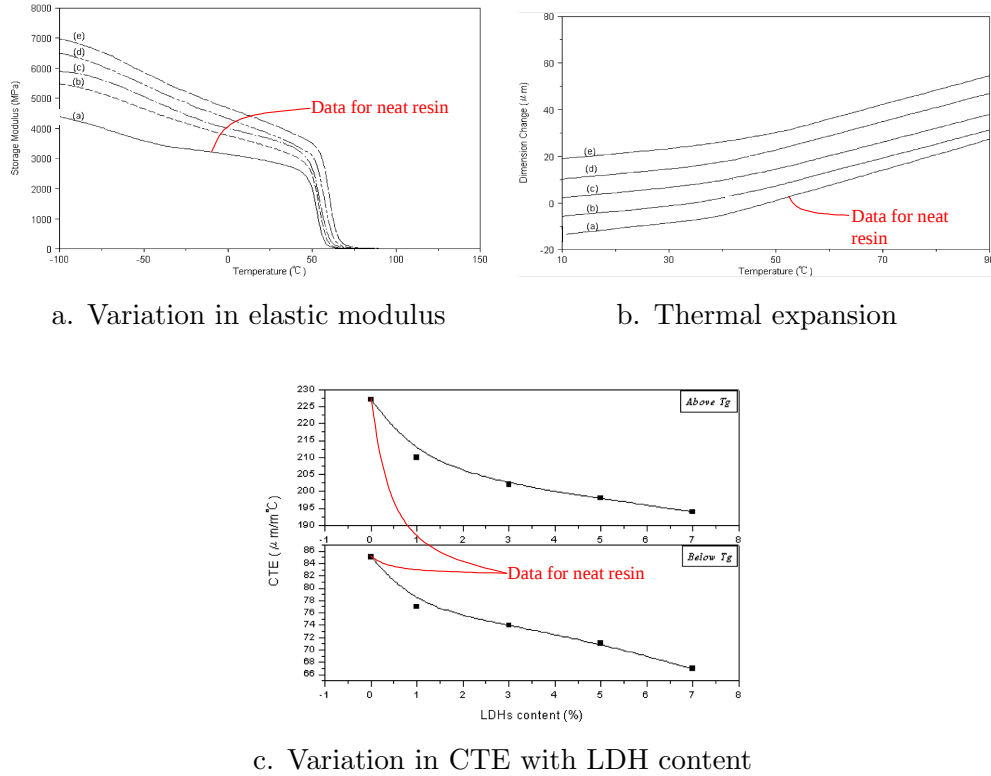
Figure A.4: Properties of EPON 828 cured with Jeffamine D400
