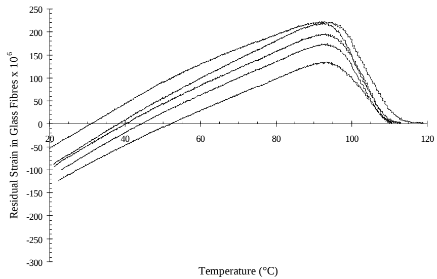
Figure 6.15: Residual strain in glass fibres of annealed specimens
