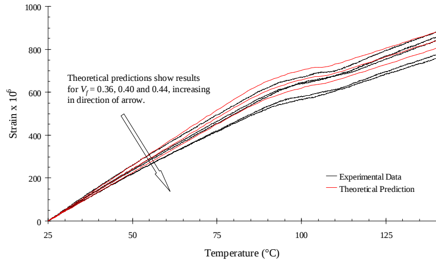
Figure 6.22: Comparison between predicted strain variation and experimental data - Unloaded specimens
