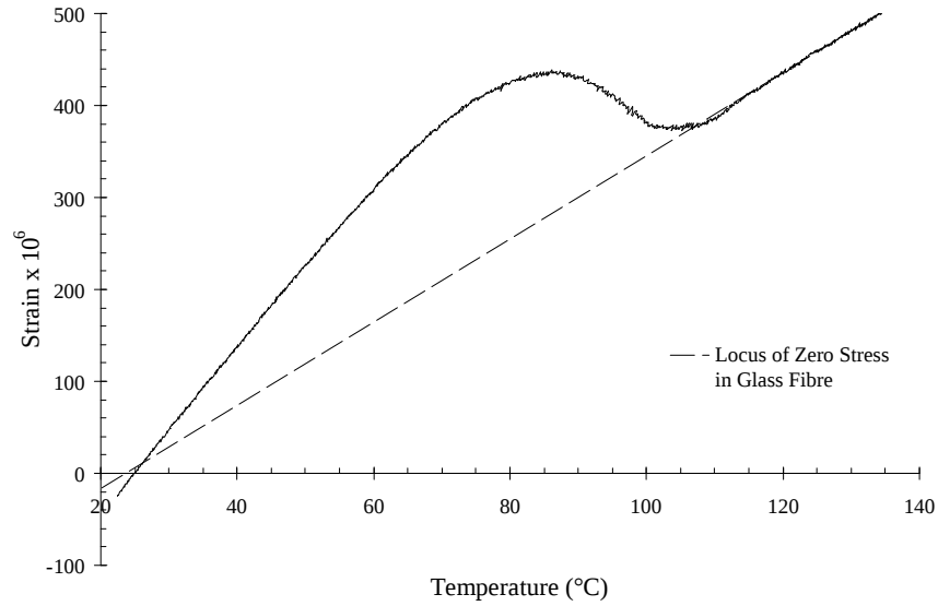
Figure 6.7: Locus of zero stress in glass fibre
