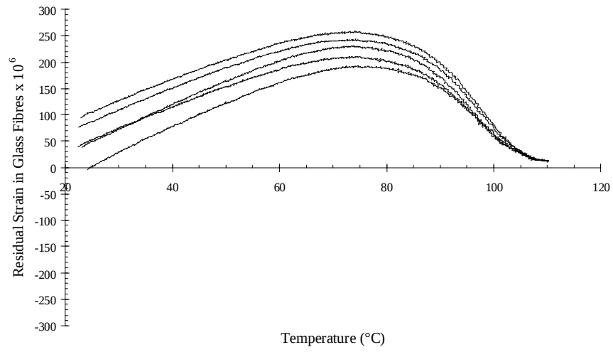
Figure F.6: Residual strain in glass fibres of preloaded specimens
