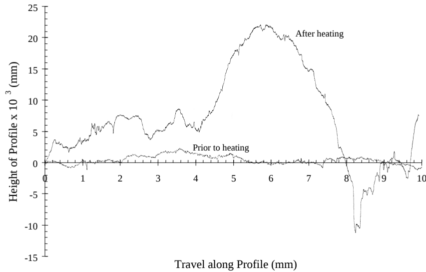
Figure 5.23: Surface roughness profile on the end face of preloaded specimens
