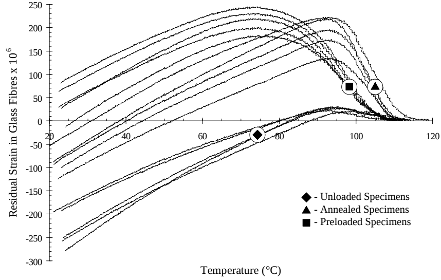
Figure 6.16: Comparison between residual strains in glass fibres of different specimen types
