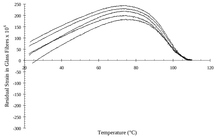
Figure 6.14: Residual strain in glass fibres of preloaded specimens
