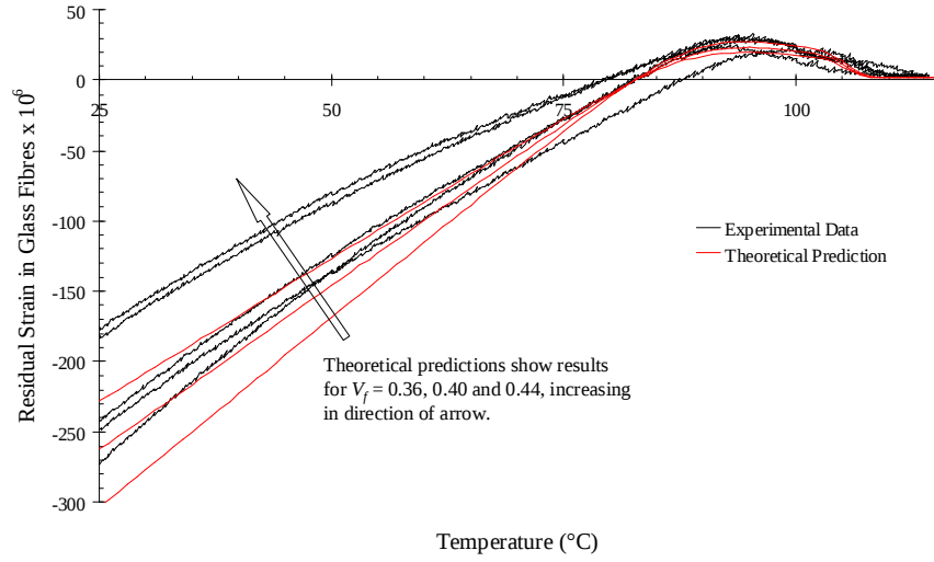
Figure 6.21: Comparison between predicted residual strain variation and experimental data - Unloaded specimens
