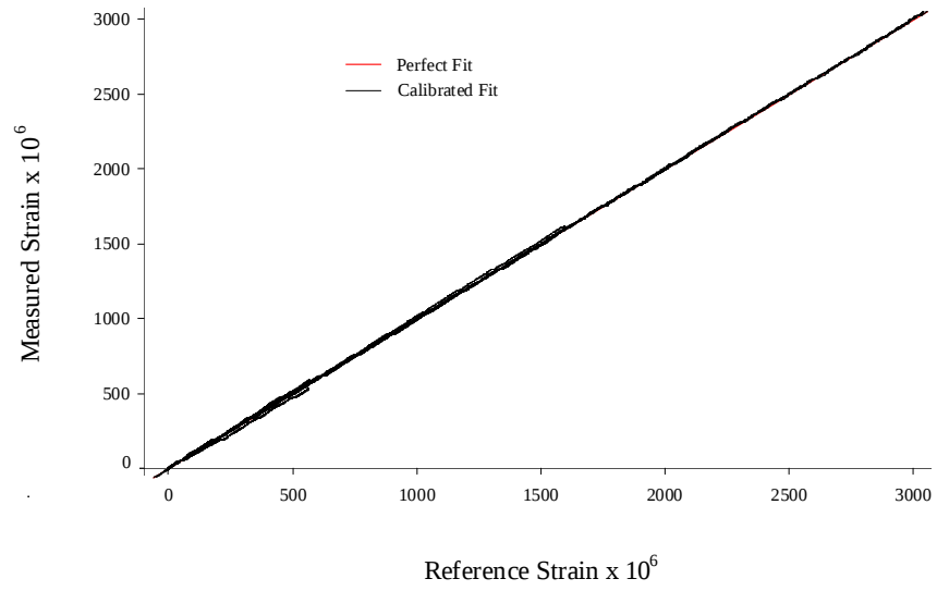
Figure D.2: Comparison of measured strains with reference strains
