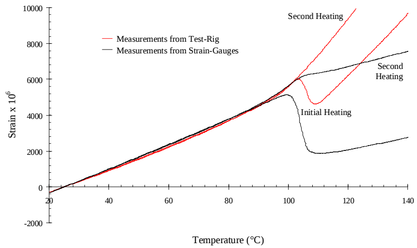
Figure 6.2: Comparison of the measured thermal strain of cast resin obtained using the final test rig and strain gauges
