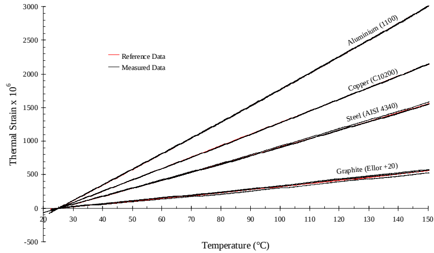
Figure 5.33: Comparison between reference thermal strains and calibrated measurements
