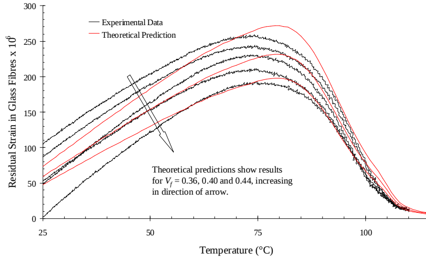
Figure G.8: Comparison between predicted residual strain variation and experimental data
