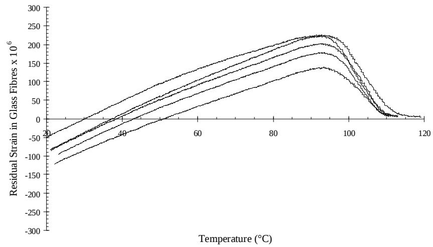
Figure F.7: Residual strain in glass fibres of annealed specimens
