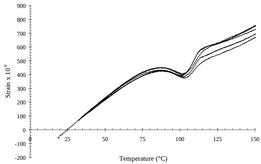
Figure 5.17: Measured strain in preloaded specimens as a function of temperature
