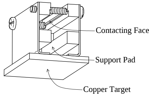
Figure 5.28: Configuration of target support
