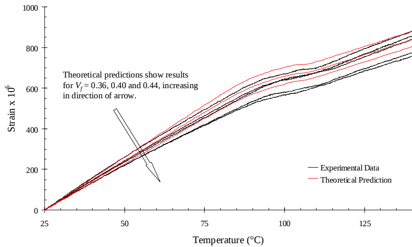
Figure G.7: Comparison between predicted strain variation and experimental data
