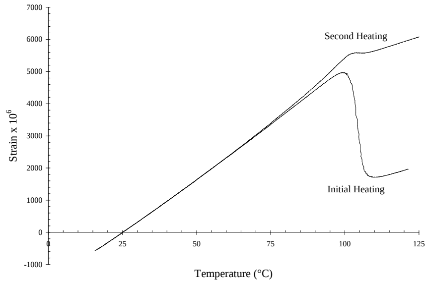
Figure 5.2: Apparent strain in cast resin - Gauges affixed with cyanoacrylate
