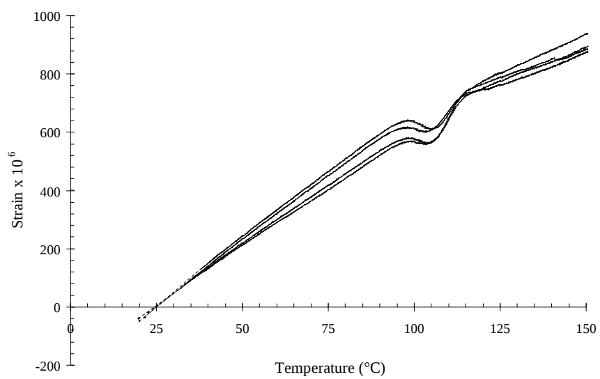
Figure 5.18: Measured strain in annealed specimens as a function of temperature
