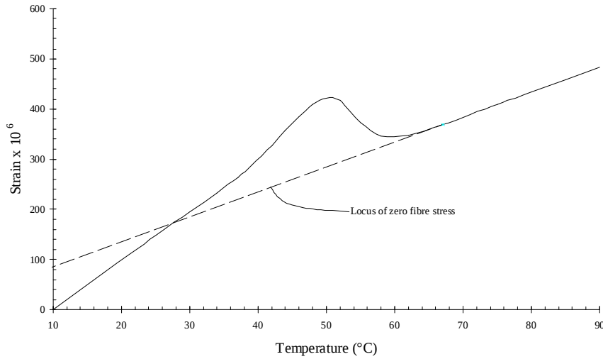
Figure 4.3: Extrapolation of the linear response at high temperatures defines the locus of zero fibre stress
