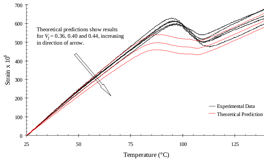
Figure 6.26: Comparison between predicted strain variation and experimental data - Annealed specimens
