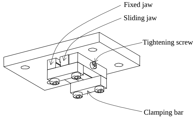
Figure 5.12: Configuration of grip assembly on backing plate
