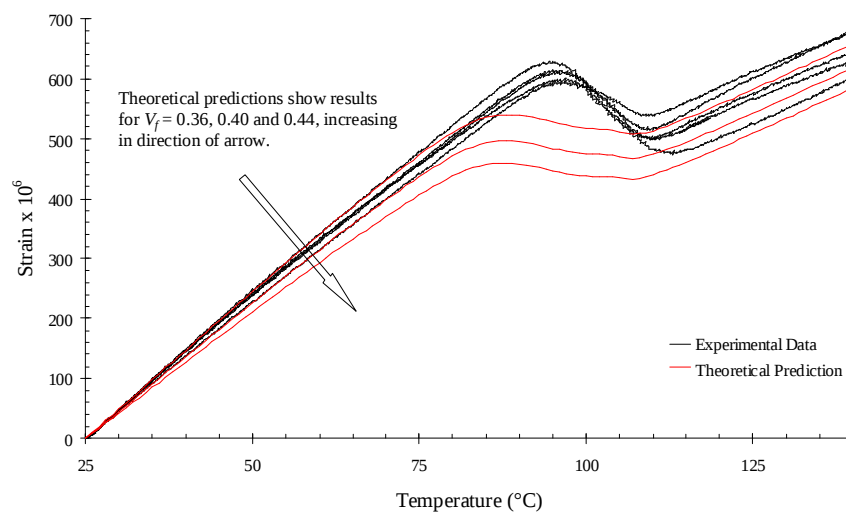
Figure G.12: Comparison between predicted residual strain variation and experimental data
