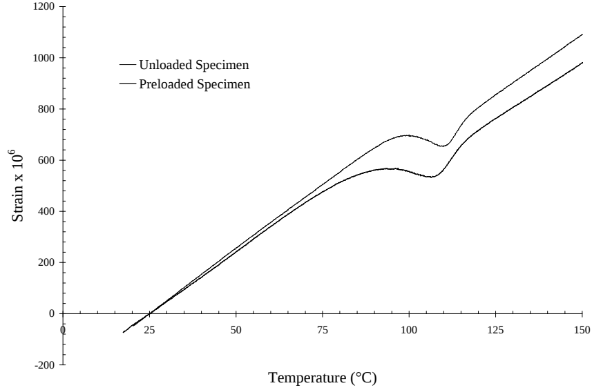
Figure 5.4: Apparent strain in glass fibre reinforced specimens
