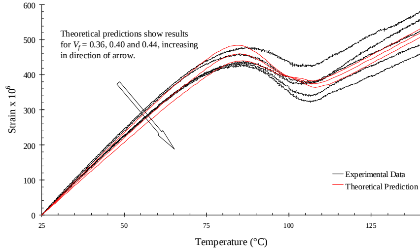
Figure 6.24: Comparison between predicted strain variation and experimental data - Preloaded specimens
