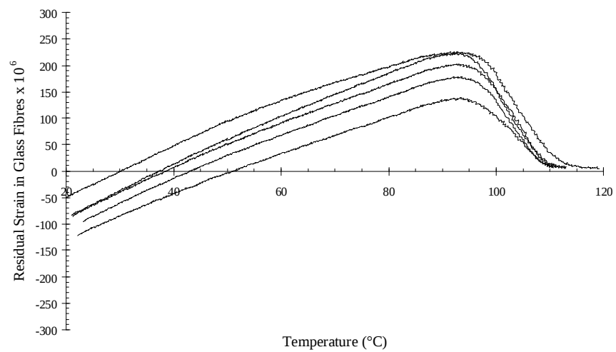
Figure 6.19: Residual strain in glass fibres of annealed specimens
