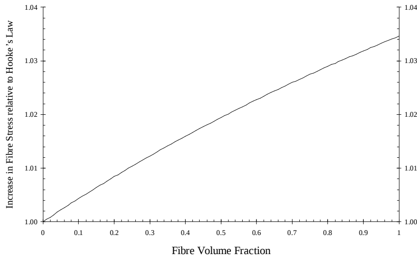
Figure B.4: Increase in fibre stress relative to that found using Hooke's Law
