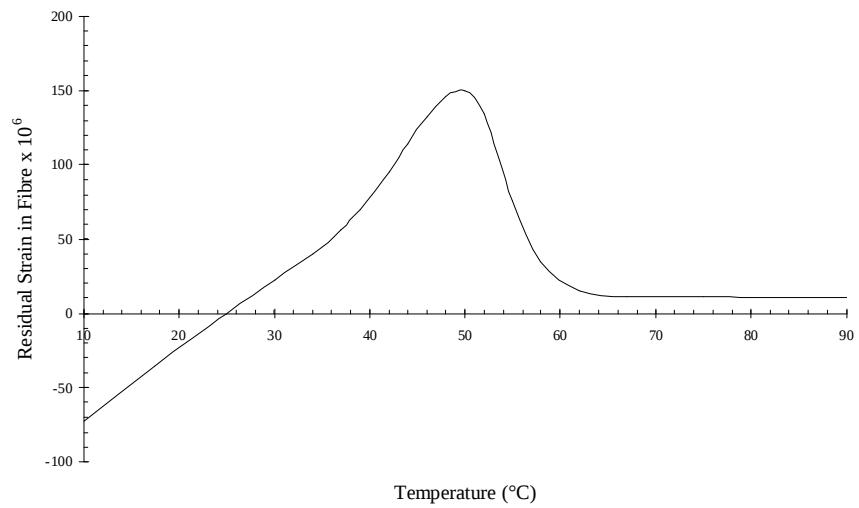
Figure 4.6: Corrected variation of residual fibre strain
