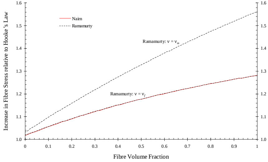
Figure B.2: Increase in fibre stress relative to that found using Hooke's Law
