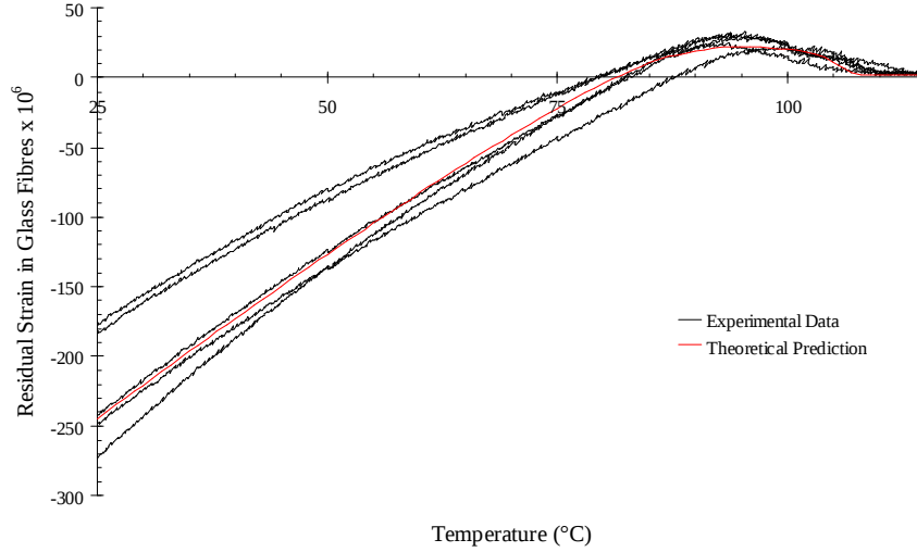
Figure 7.2: Predicted response of unloaded specimens when using manufacturer's data for CTE
