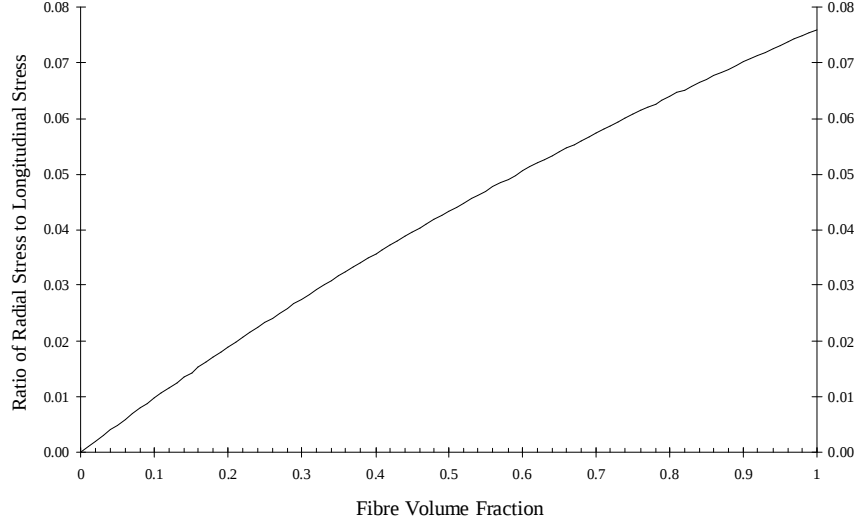
Figure B.3: Variation in ratio between radial and longitudinal stress in the fibres
