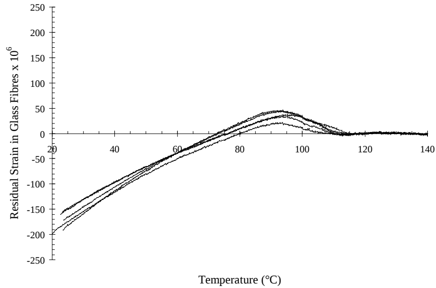
Figure 6.7: Locus of zero stress in glass fibre
