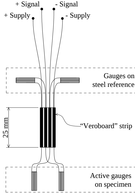
Figure 5.1: Schematic layout of Wheatstone bridge connections
