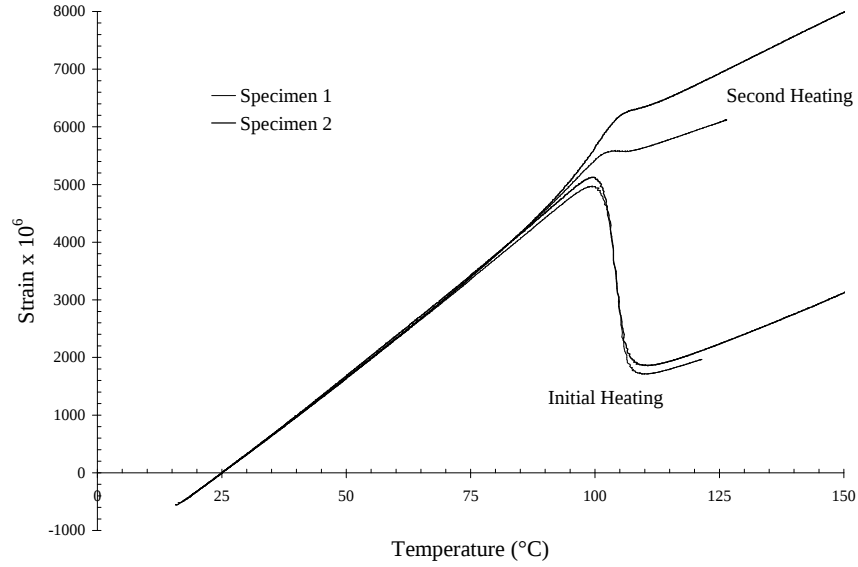
Figure 5.3: Comparison between apparent strains obtained from specimens with different strain-gauge adhesives
