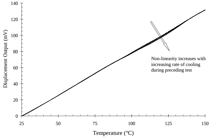
Figure 5.32: Effect of rate of oven cooling on measurement linearity
