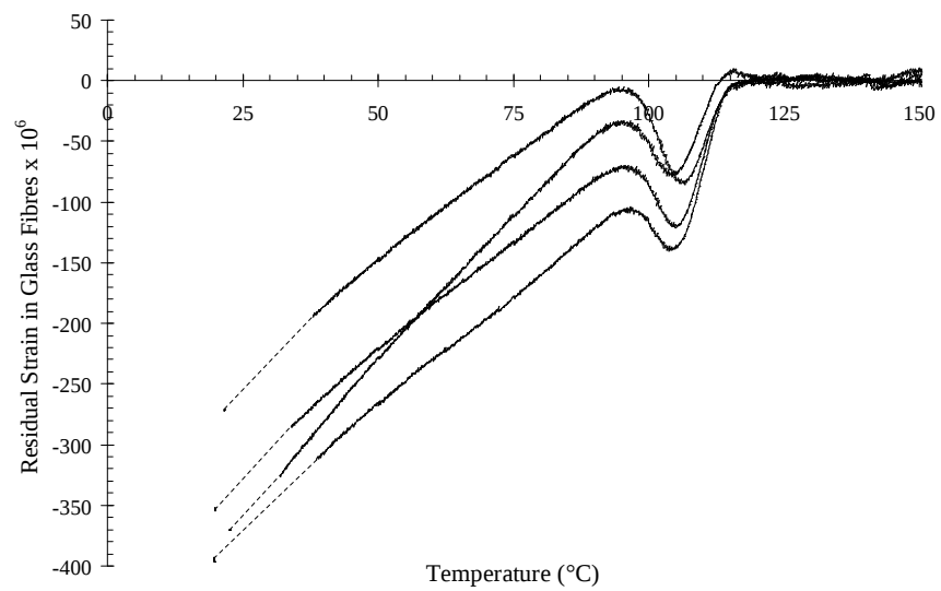
Figure 5.22: Residual strain in glass fibres of annealed specimens
