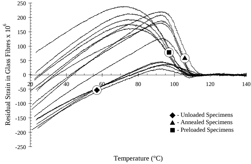
Figure 6.11: Comparison between residual strains in glass fibres of different specimen types
