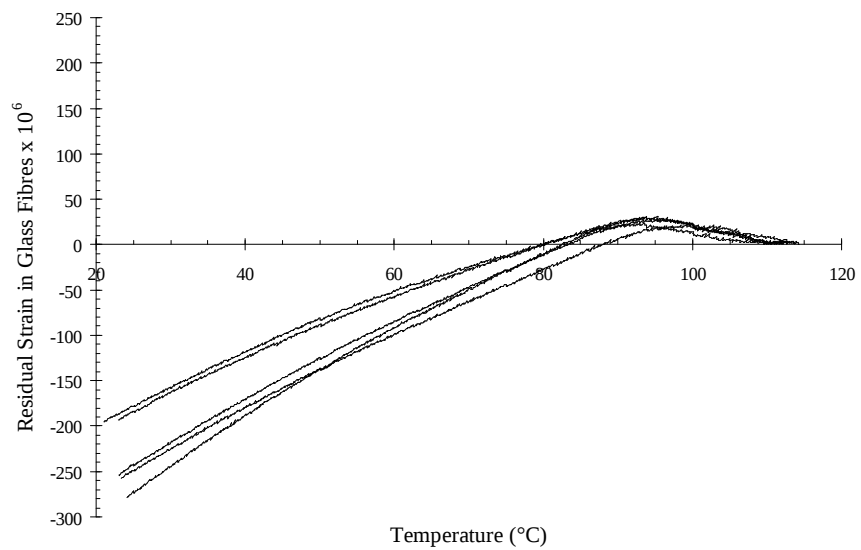
Figure 6.13: Residual strain in glass fibres of unloaded specimens
