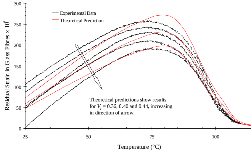
Figure 6.23: Comparison between predicted residual strain variation and experimental data - Preloaded specimens
