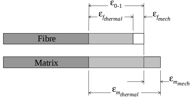
Figure A.2: Development of thermal strains in GFRP
