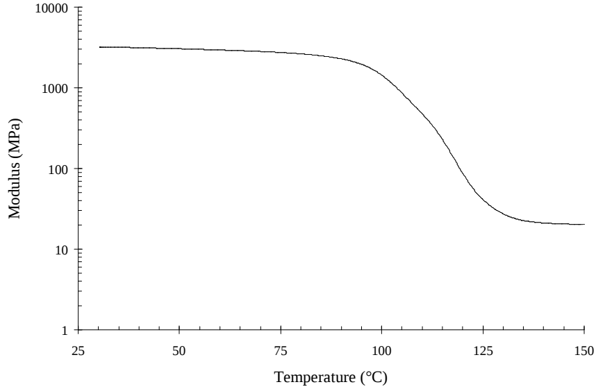
Figure 4.1: Temperature variation of modulus in Derakane 411-350
