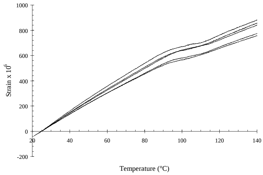
Figure 6.3: Measured strain in unloaded specimens
