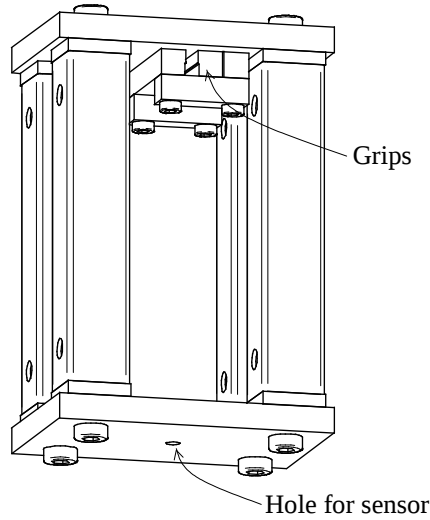
Figure 5.9: Configuration of test frame
