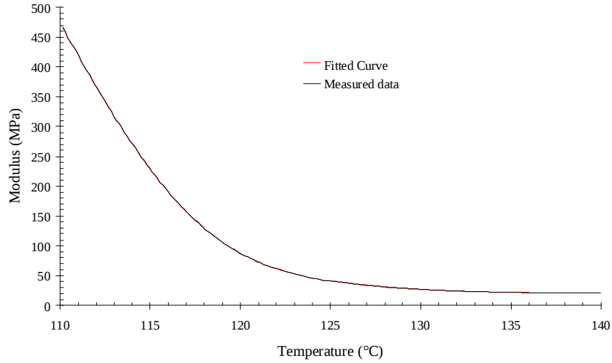
Figure F.3: Correlation between measured matrix modulus and fitted curve
