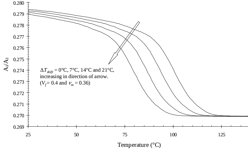
Figure G.4: Variation of \frac{A_1}{A_3} as function of temperature and \Delta T_{shift}
