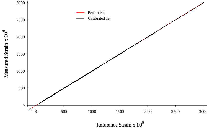
Figure D.1: Comparison of measured strains with reference strains
