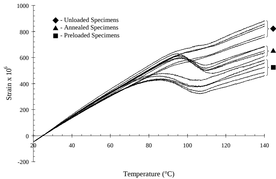
Figure 6.6: Comparison between measured strains in different specimen types
