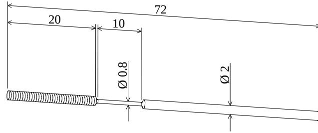
Figure 5.30: Rods used to provide rotational restraint
