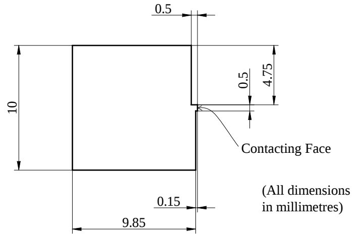
Figure 5.10: Cross-section through a jaw of the “knife-edge” grips
