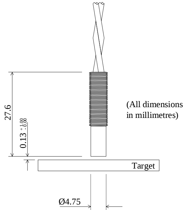
Figure 5.5: Position of displacement sensor relative to target
