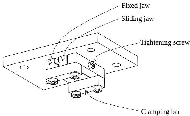
Figure 5.26: Configuration of grip assembly
