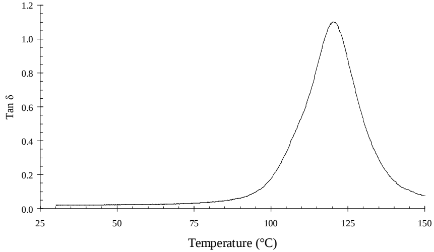
Figure F.4: Temperature variation of \tan \delta in Derakane 411-350
