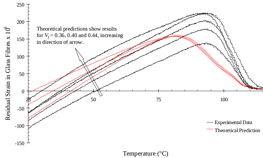
Figure G.11: Comparison between predicted residual strain variation and experimental data
