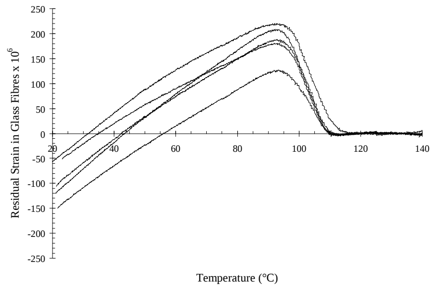
Figure 6.10: Residual strain in glass fibres of annealed specimens
