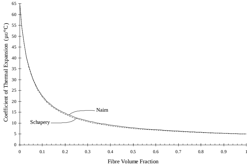
Figure A.1: Predicted longitudinal CTE for unidirectional GFRP
