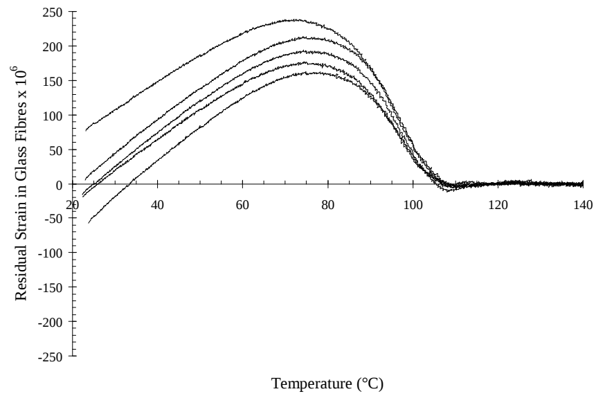
Figure 6.9: Residual strain in glass fibres of preloaded specimens
