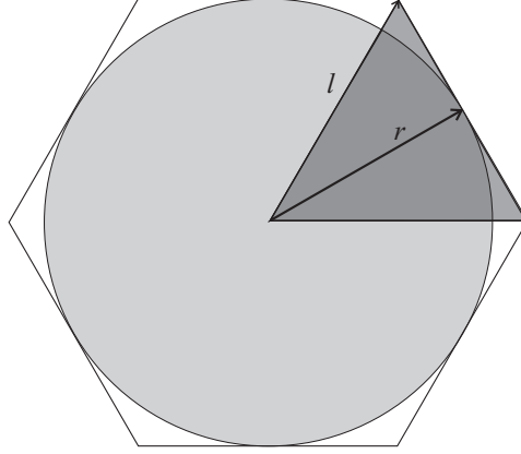
Figure E.1: Fibre within hexagonal unit cell
