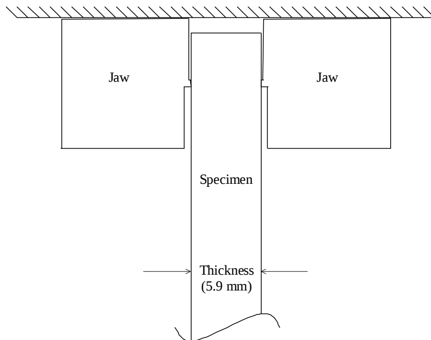
Figure 5.11: Specimen positioned within clamping jaws
