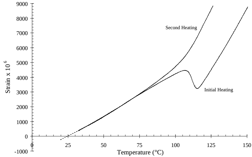
Figure 5.15: Measured strain in cast resin as a function of temperature
