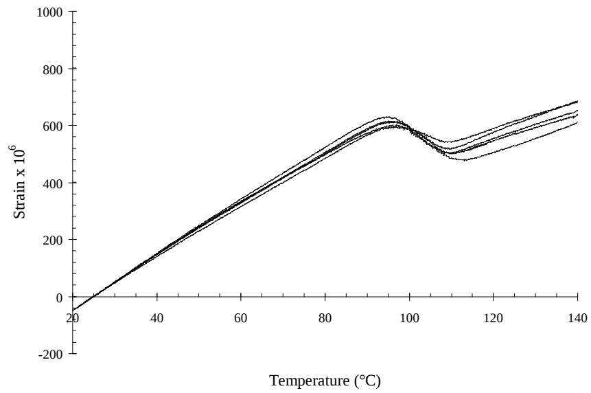
Figure 6.5: Measured strain in annealed specimens
