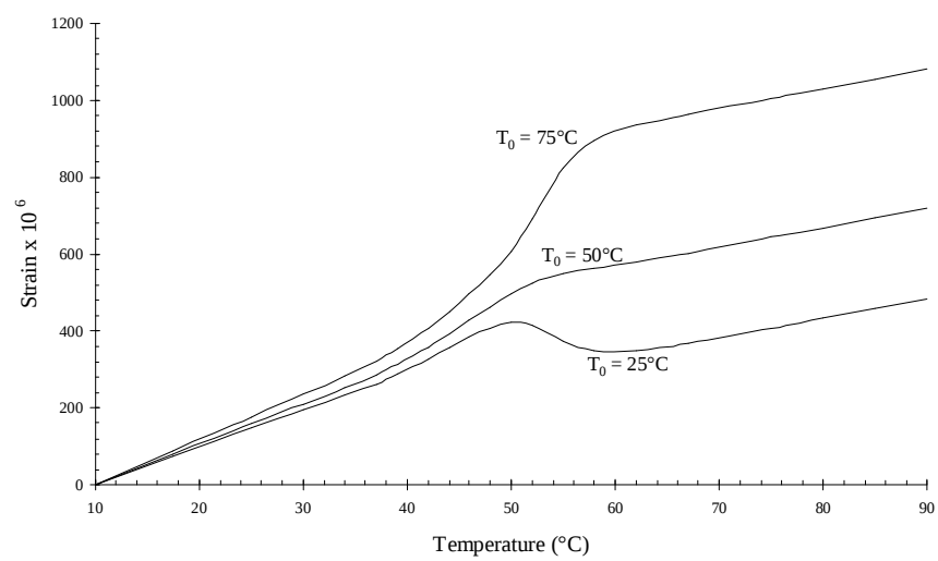
Figure A.5: Illustrative longitudinal thermal response of EPON 828/E-glass laminate
