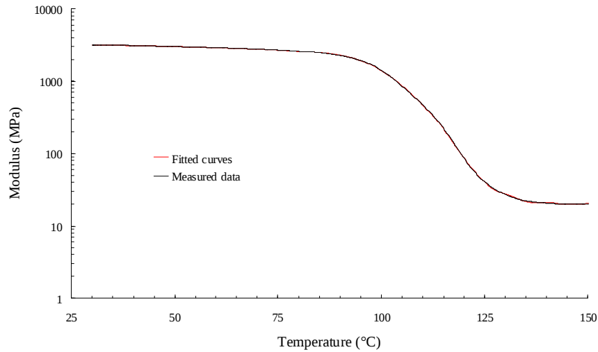
Figure G.1: Correlation between measured modulus and fitted curves
