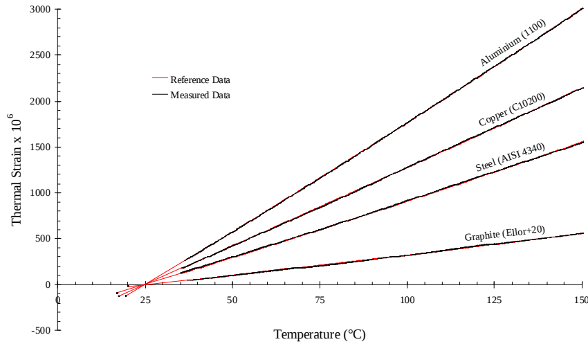
Figure 5.14: Comparison between reference thermal strains and calibrated measurements
