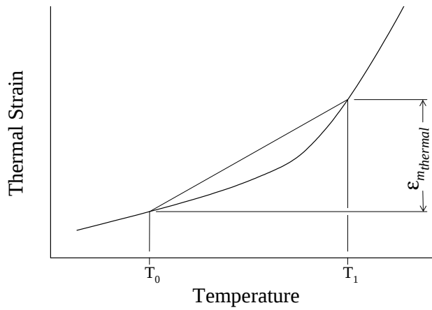
Figure A.3: Illustrative thermal strains in polymer matrix
