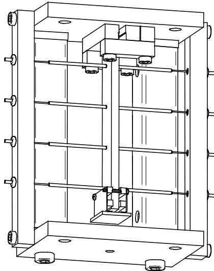
Figure 5.31: Arrangement of rods providing rotational restraint - Front spacing legs are omitted for clarity
