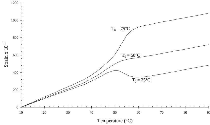
Figure 4.2: Illustrative longitudinal thermal response of EPON 828/E-glass laminate
