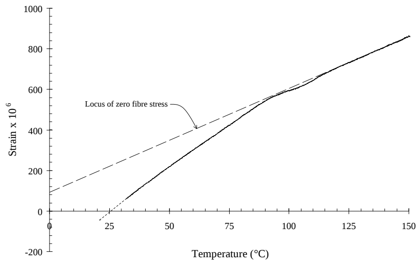
Figure 5.19: Locus of zero stress in glass fibres
