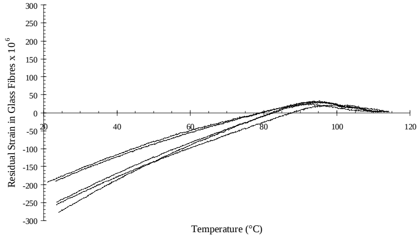
Figure 6.17: Residual strain in glass fibres of unloaded specimens
