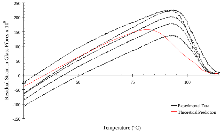
Figure G.10: Comparison between predicted residual strain variation and experimental data
