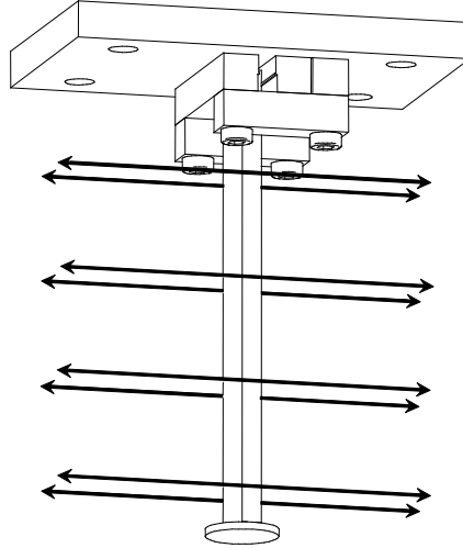
Figure 5.13: Tensioned carbon threads attached to specimen - Spacing legs are not shown in the interests of clarity
