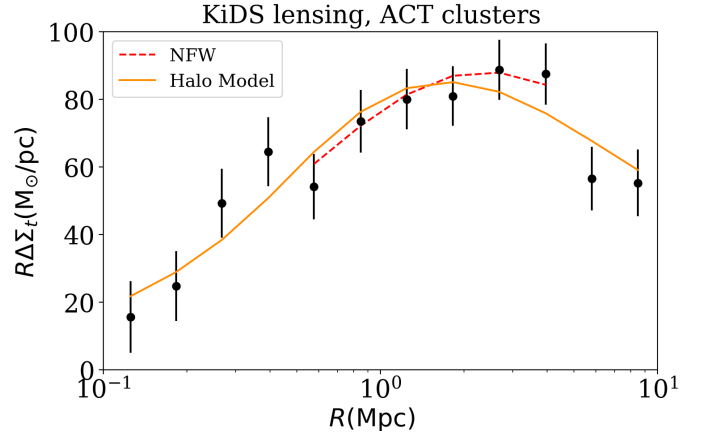
Fig. 3. ESD profile ( \Delta\Sigma ) multiplied by the radius R as a function of radius R for the complete stack of 157 SZ-detected clusters. The signal is detected at 25\sigma significance. The best-fitting model is shown using a single NFW, shown in red, and the halo model, shown in orange. A limited range of scales is used for the NFW model to avoid the impact of mis-centring at small scales and the contribution from large-scale structure at scales greater than 5 Mpc. Both models give good fits to the data.
