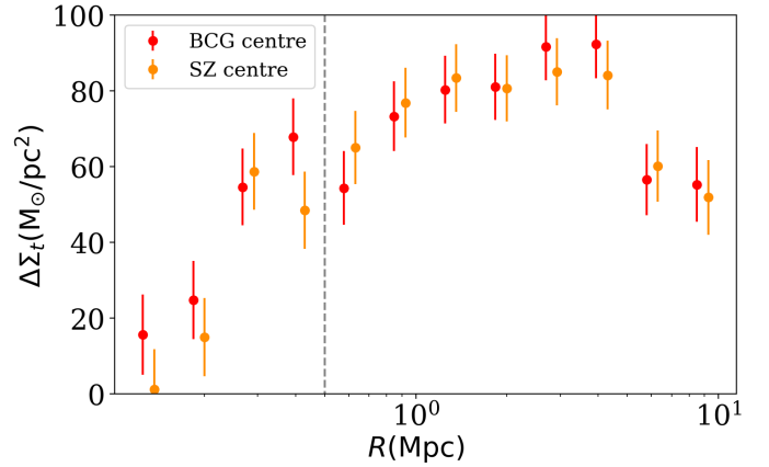
Fig. A.1. Tests of mis-centring: comparison of the ESD measured around the peak in the SZ emission and the BCG. The ratio between the BCG and SZ centred signal averaged R > 0.5 is unity.
