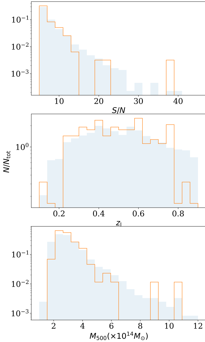
Fig. 2. Upper: normalised SZ signal-to-noise distribution of the ACT clusters found in the KiDS-1000 region. Middle: normalised redshift distribution of these clusters. Lower: normalised SZ-derived mass distribution of these clusters, estimated from the SZ observable Compton- \gamma values. The blue shaded region corresponds to clusters selected to have an SZ signal-to-noise greater than 5 and in the redshift range 0.1–0.9 across the full ACT footprint. The orange line corresponds to the selection of 157 clusters used in this analysis that lie within the KiDS footprint.
