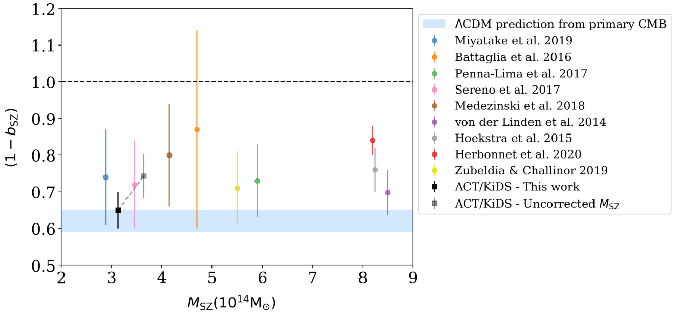
Fig. 4. Estimated (1 - b_{SZ}) bias parameter from this analysis (ACT SZ-detected clusters calibrated with KiDS weak lensing), compared to other recent results. Shown on this figure at the lower mass range, the analyses of ACT and Planck clusters using HSC (Miyatake et al. 2019; Medezinski et al. 2018), ACT/CS82 (Battaglia et al. 2016), CLASH (Penna-Lima et al. 2017), PSZ2LenS (Sereno et al. 2017), WtG (von der Linden et al. 2014), CCCP (Hoekstra et al. 2015) which has recently been updated to CCCP and MENaCS (Herbonnet et al. 2020) and Planck clusters with Planck CMB lensing (Zubeldia & Challinor 2019) analyses. The blue band indicates the prediction from Planck primary CMB measurements if the \Lambda CDM model is correct (Planck Collaboration VI 2020), given the SZ clusters observed by Planck . This value is computed using a Planck Collaboration VI (2020) primary CMB best fit cosmology, however using the cosmology derived from ACT DR6 lensing, Madhavacheril et al. (2023), would give the same result.
