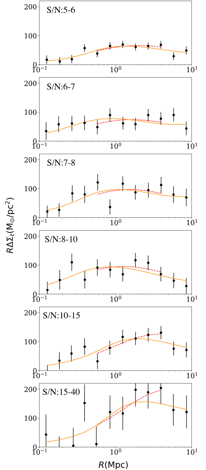
Fig. 5. ESD profile ( \Delta\Sigma ) as a function of radius R , for each sub-sample of clusters. The best fit lines are also plotted shown in red for the single NFW and orange for the halo model.
