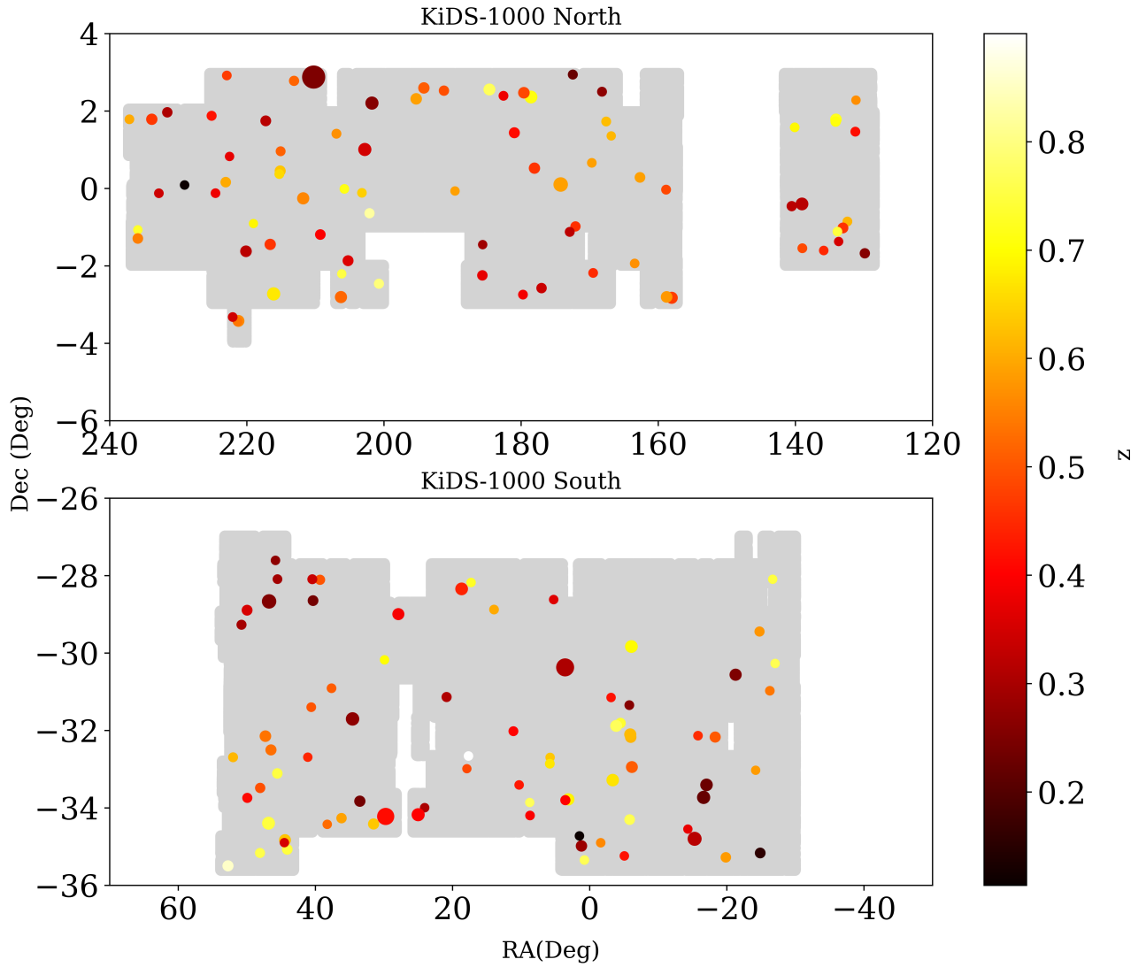
Fig. 1. KiDS North and South survey areas are shown in light grey in the upper and lower panels, respectively. The positions of ACT clusters used in this analysis are indicated by each circle. The colour of the circles corresponds to cluster redshift, with yellow indicating high redshift and black indicating low redshift. The size of each circle scales with the SZ signal-to-noise, which is correlated with the cluster mass when the noise is the same everywhere, such that larger circles represent clusters with a greater SZ signal-to-noise than smaller circles.
