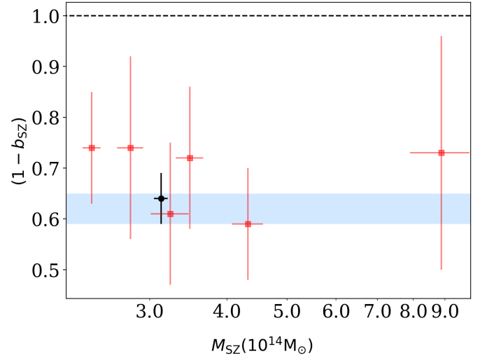
Fig. 6. Estimated (1 - b_{\text{SZ}}) bias parameter from the total cluster stack shown in black, and in red for six individual SZ signal-to-noise bins. These values are reported in Table 1. The blue band indicates the prediction from Planck primary CMB measurements if the \Lambda CDM model is correct (Planck Collaboration VI 2020), given the SZ clusters observed by Planck .
