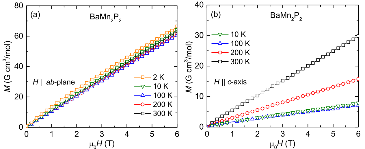
FIG. 7. Isothermal magnetization M vs applied magnetic field H of BaMn 2 P 2 measured for two different crystal orientations; (a) H \parallel ab plane and (b) H \parallel c axis.
