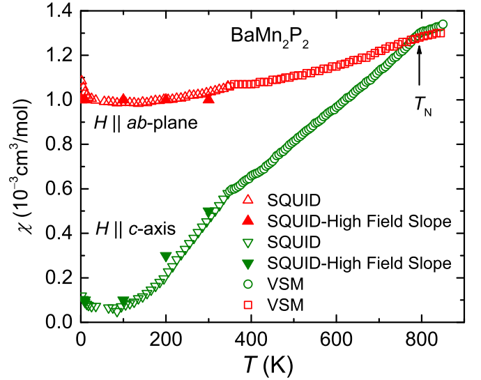
FIG. 5. Anisotropic magnetic susceptibilities \chi_{ab,c} \equiv M/H vs temperature T of \text{BaMn}_2\text{P}_2 measured using a SQUID-magnetometer at \mu_0 H = 3 \text{ T} for T \leq 350 \text{ K} , determined from high-field slopes of the isothermal magnetization measurements and measured using a vibrating sample magnetometer for T \geq 350 \text{ K} .
