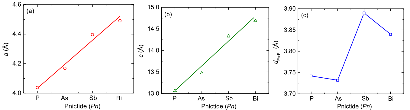
FIG. 2. Variation of tetragonal lattice parameters (a) a , (b) c , and (c) the distance between adjacent pnictogen layers d_{Pn-Pn} in BaMn 2 Pn 2 ( Pn = P, As, Sb, Bi ) with the type of pnictide ion present in the unit cell.
