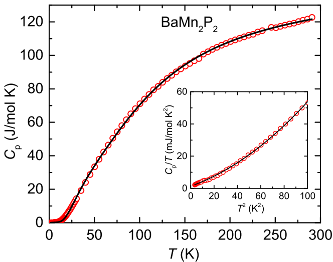
FIG. 4. Heat capacity C_p vs temperature T along with the Debye-Einstein fit as described in the text. Inset: C_p/T vs T^2 data for T \leq 10 \text{ K} along with the fit as described in the text.
