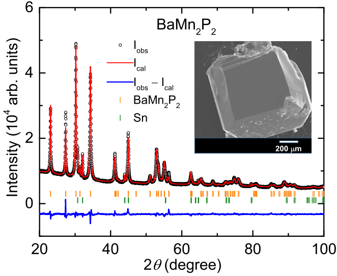
FIG. 1. Room temperature powder x-ray diffraction data collected on Sn-grown crushed crystals of BaMn 2 P 2 , two-phase Rietveld refinement profile, difference profile, and Bragg positions of BaMn 2 P 2 as well as adventitious Sn. Inset: Scanning electron microscope image of a crystal of BaMn 2 P 2 .
