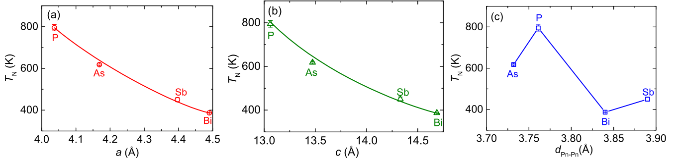
FIG. 6. Variation of antiferromagnetic transition temperature T_N with tetragonal unit cell parameters (a) a , (b) c , and (c) distance between adjacent pnictogen layers d_{Pn-Pn} in BaMn 2 Pn 2 ( Pn = P, As, Sb, Bi ).
