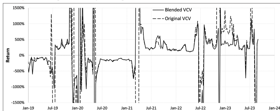
Figure 8: Comparison of original sample and blended covariance matrices via return metric
