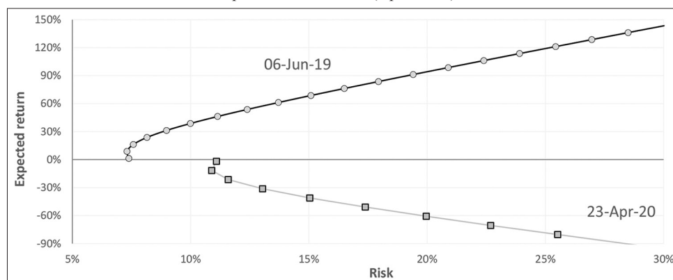
Figure 1: “Normal” efficient frontier when market conditions were non-turbulent (June 2019) AND during the turbulent initial phase of COVID-19 (April 2020)
