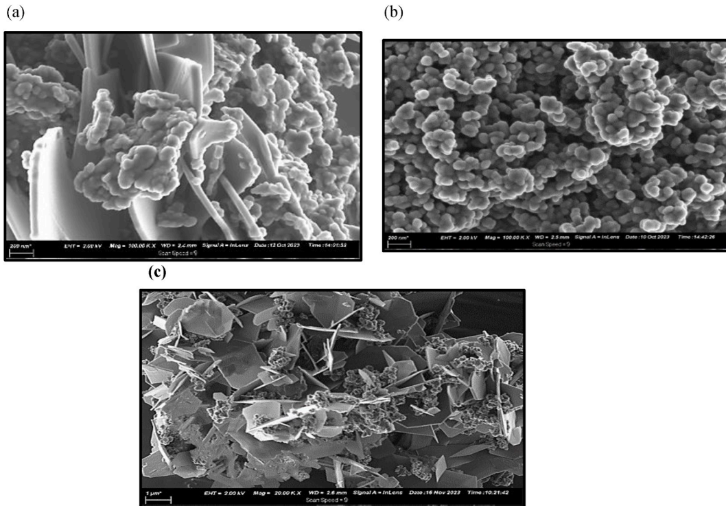
Fig. 6. SEM Analysis of nanoparticle morphology: (a) \text{Fe}_3\text{O}_4 (20–30nm), (b) \text{Ti O}_2 (18 nm) nanoparticles, and (c) \text{Fe}_3\text{O}_4/\text{Ti O}_2 hybrid configuration.
