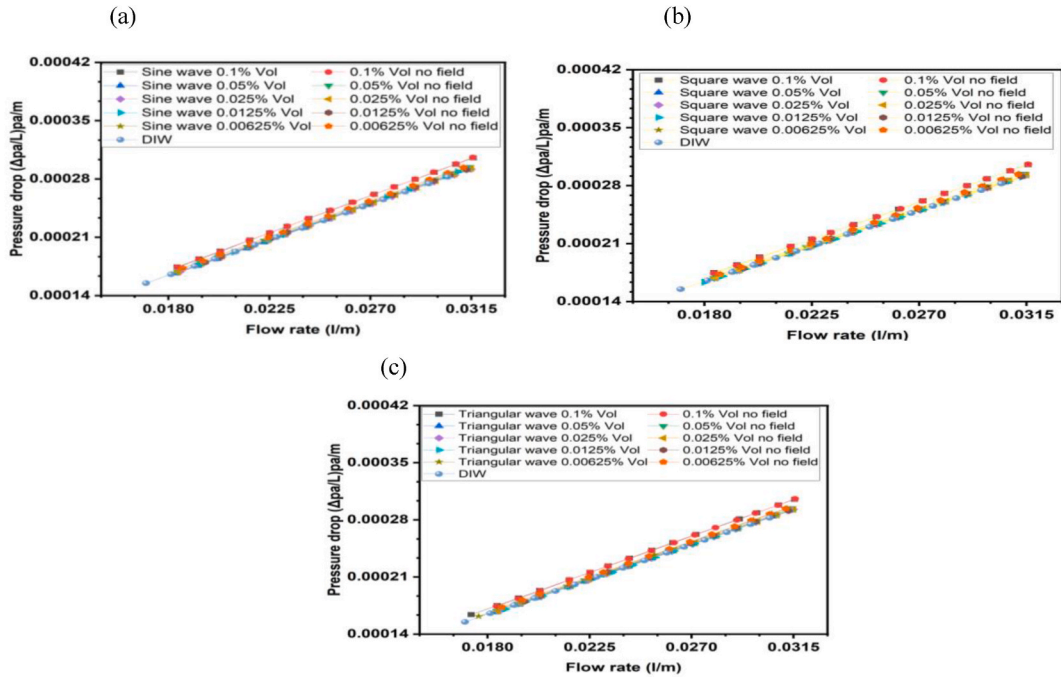
Fig. 18. (a) Effect of volumetric fractions and magnetic field sine wave on pressure drop in Fe 3 O 4 /TiO 2 nanofluids across different flow rates (b) Effect of volumetric fractions and magnetic field square wave on pressure drop in Fe 3 O 4 /TiO 2 nanofluids across different flow rates (c) Effect of volumetric fractions and magnetic field triangular wave on pressure drop in Fe 3 O 4 /TiO 2 nanofluids across different flow rates.
