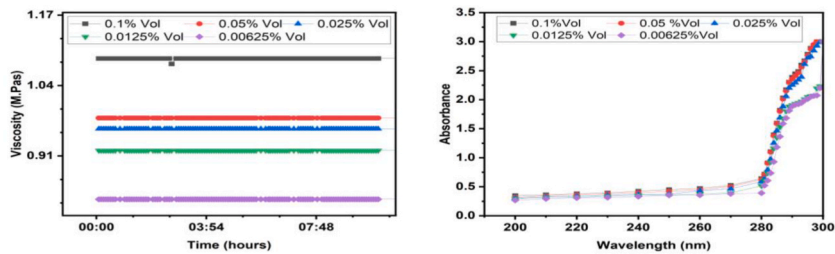
Fig. 7. (a) Time-dependent assessment of stability (b) Influence of \text{Fe}_3\text{O}_4/\text{Ti O}_2 density on light absorption across various wavelengths.
