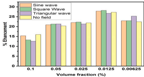
Fig. 16. Comparative analysis of heat transfer enhancement with different waveforms at varied volume fractions.
