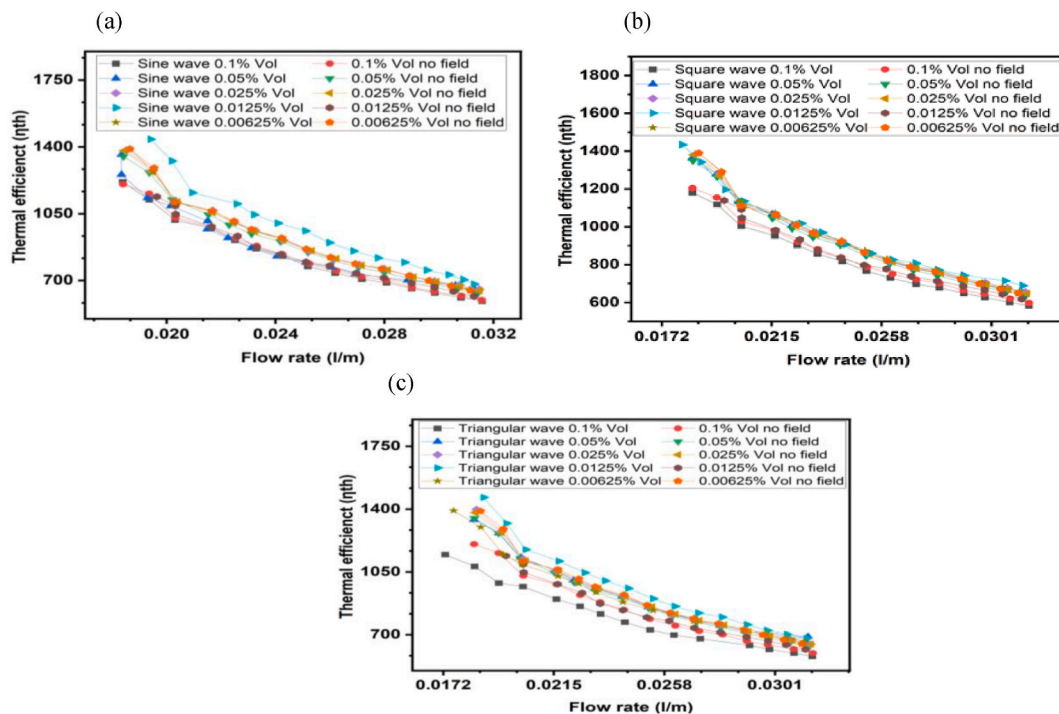
Fig. 19. (a) Effect of magnetic field sine waveform and volume fractions on thermal efficiency of \text{Fe}_3\text{O}_4/\text{TiO}_2 nanofluids across various flow rates (b) Effect of magnetic field square waveform and volume fractions on thermal efficiency of \text{Fe}_3\text{O}_4/\text{TiO}_2 nanofluids across various flow rates (c) Effect of magnetic field triangular waveform and volume fractions on thermal efficiency of \text{Fe}_3\text{O}_4/\text{TiO}_2 nanofluids across various flow rate.
