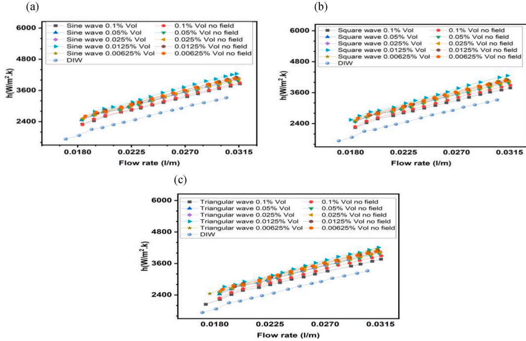
Fig. 17. (a) Effect of volumetric fractions, comparison of mean heat transfer coefficient for Fe 3 O 4 /TiO 2 nanofluid under sine wave and flow rates, including no magnetic condition (b) Effect of volumetric fractions, comparison of mean heat transfer coefficient for Fe 3 O 4 /TiO 2 nanofluid under square wave and flow rates, including no magnetic condition (c) Effect of volumetric fractions, comparison of mean heat transfer coefficient for Fe 3 O 4 /TiO 2 nanofluid under triangular wave and flow rates, including no magnetic condition.
