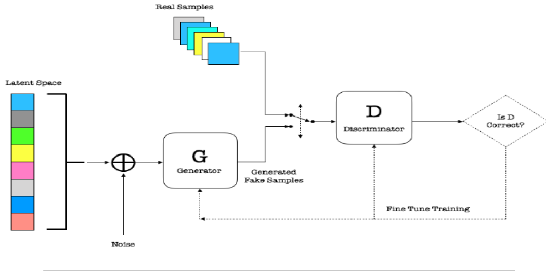
FIGURE 2.3: GAN operation
