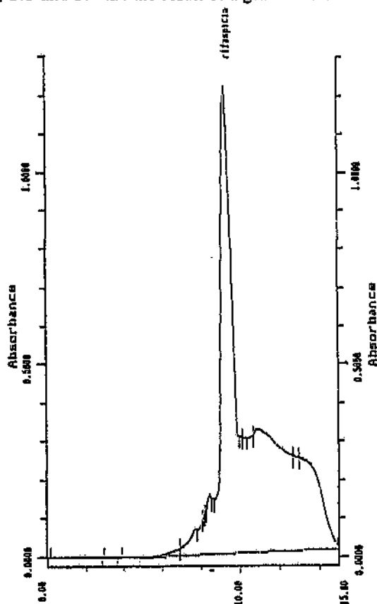
Figure 3.2 UV chromatogram of rifampicin
