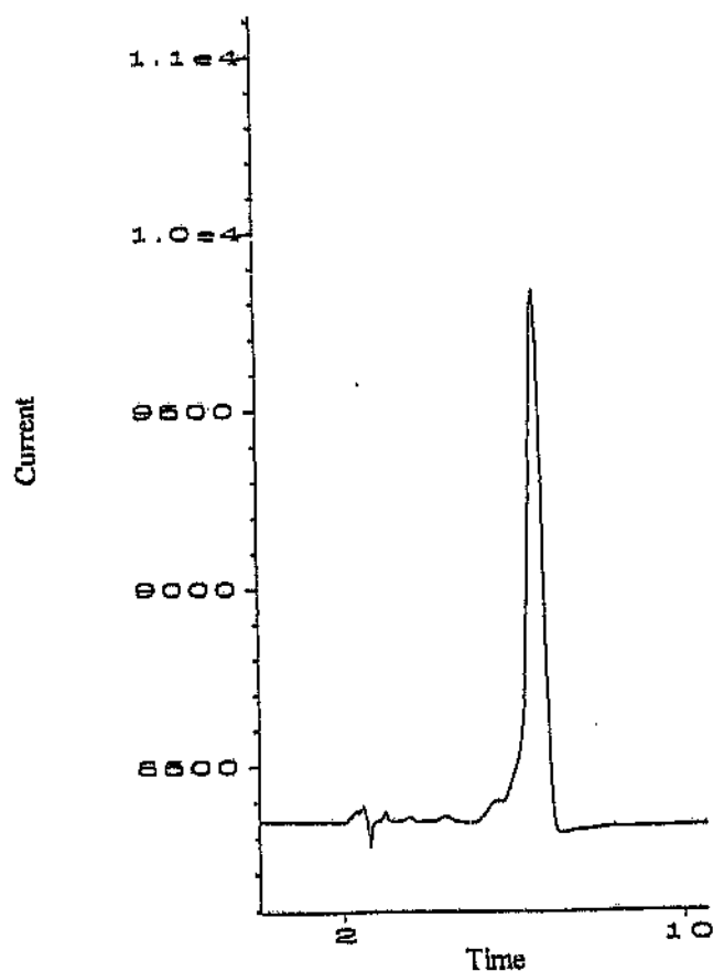
Figure 3.9 ECD chromatogram of rifampicin
