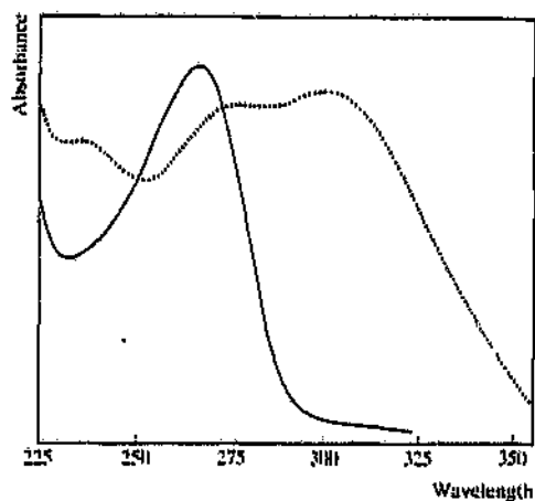
Figure 1.4 UV spectrum of isoniazid
