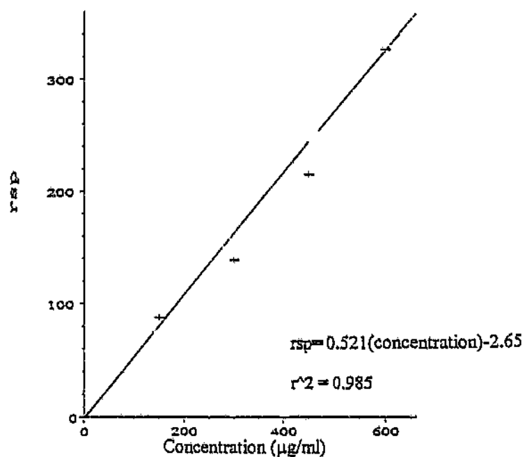
Figure 3.14 Calibration curve of rifampicin (electrochemical detection)
