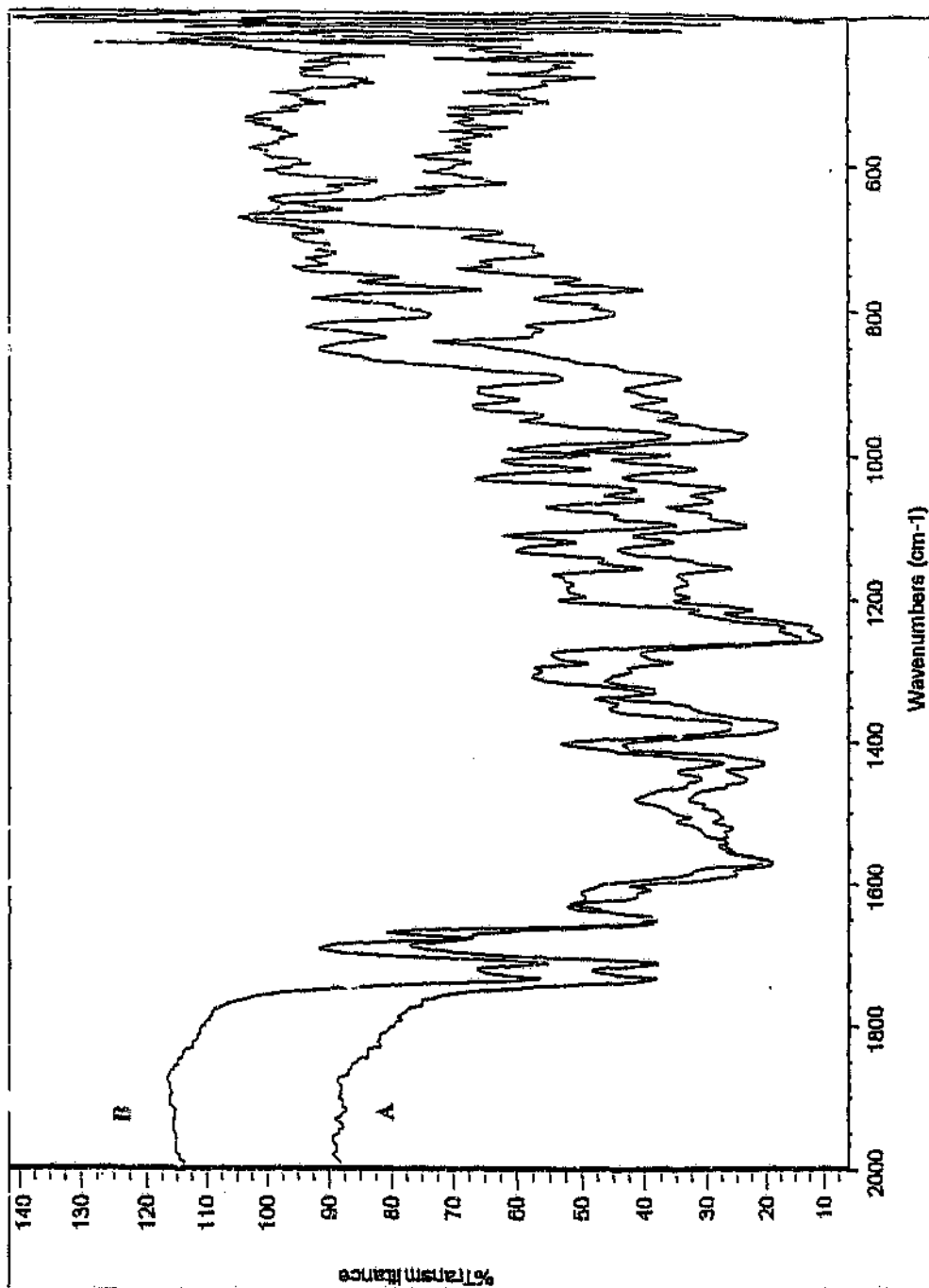
Figure 3.15 FT-IR spectrum of rifampicin (A) and differential spectrum of a physical mixture of rifampicin/isoniazid (B)
