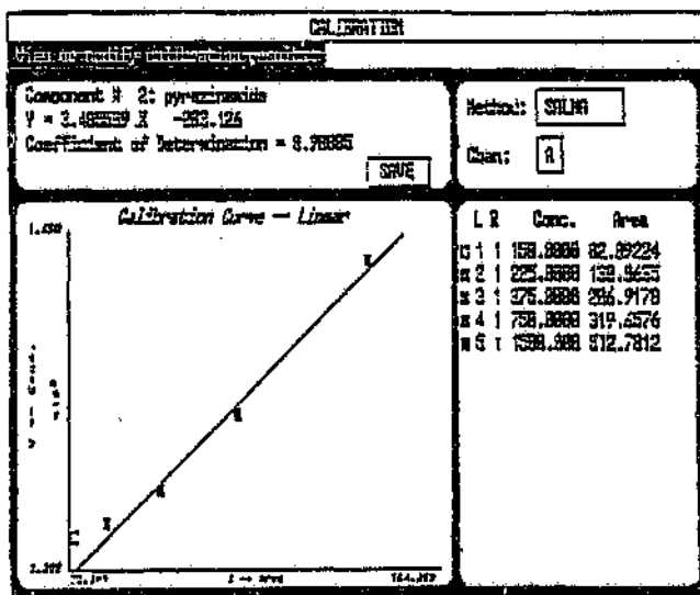
Figure 3.7 Calibration curve of pyrazinamide (UV detection)
