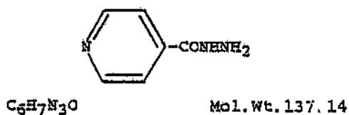
Figure 1.3 Structural formula of isoniazid. (Brewer, 1977).
