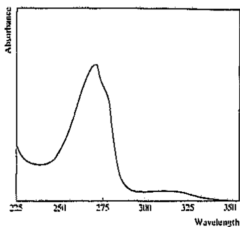
Figure 1.6 UV spectrum of pyrazinamide
