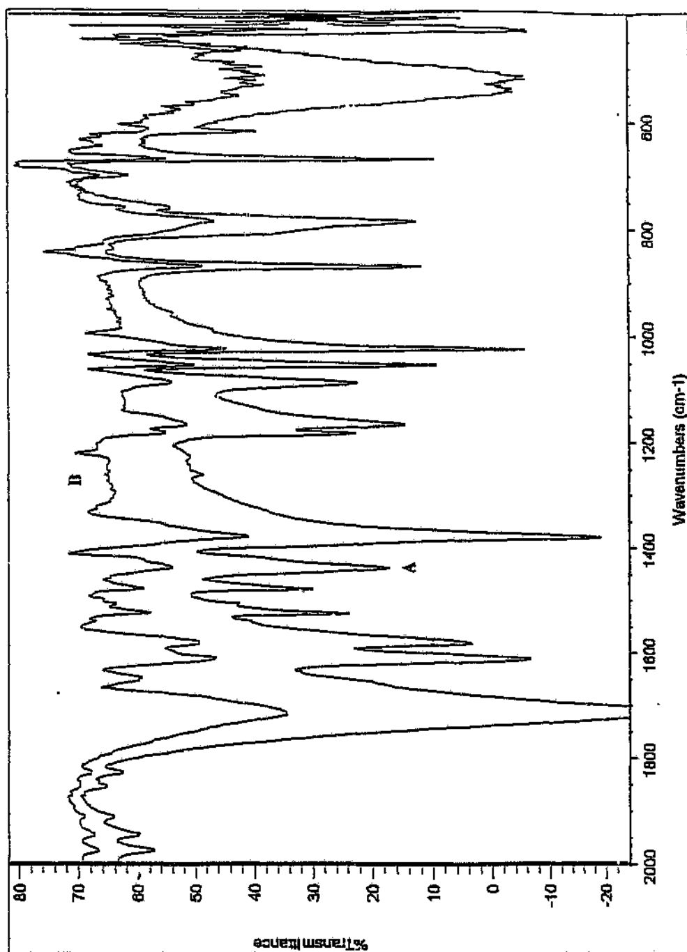
Figure 3.22 FT-IR spectrum of pyrazinamide (A) and differential spectrum of a physical mixture of pyrazinamide/isoniazid (B)
