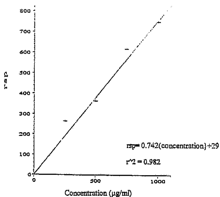
Figure 3.13 Calibration curve of ethambutol HCl (electrochemical detection)
