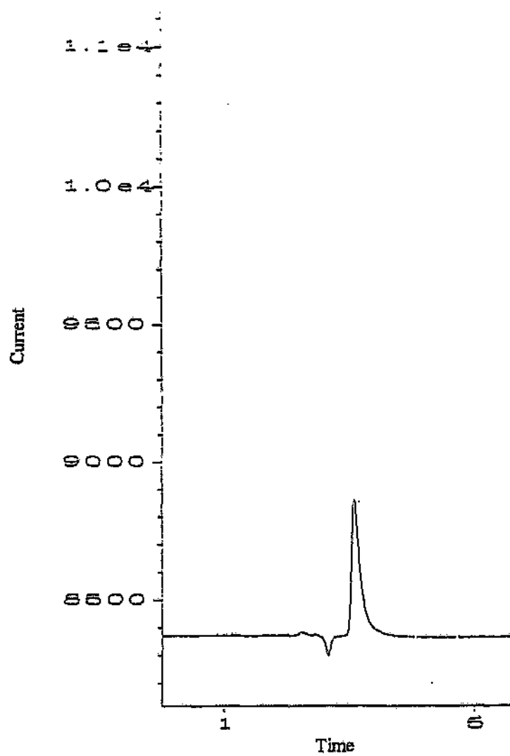
Figure 3.11 ECD chromatogram of ethambutol HCl
