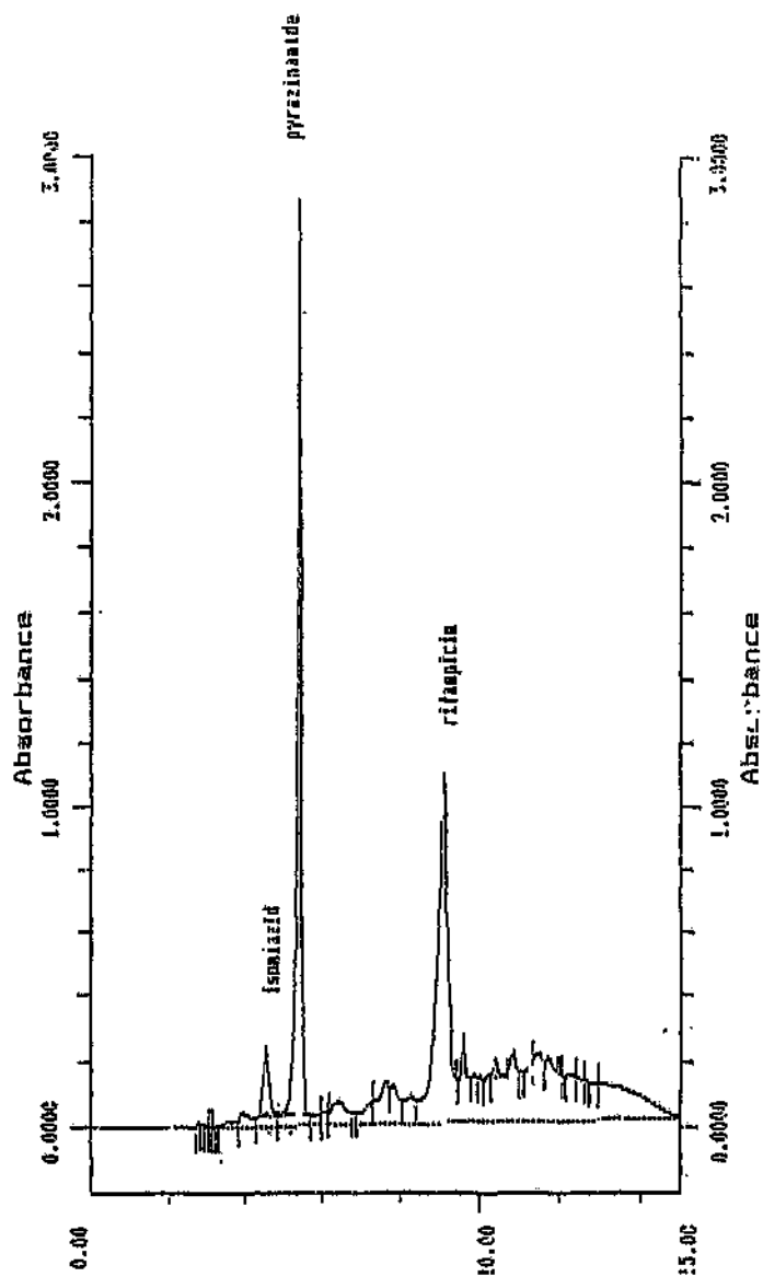
Figure 3.1 UV chromatogram of rifampicin, isoniazid and pyrazinamide
