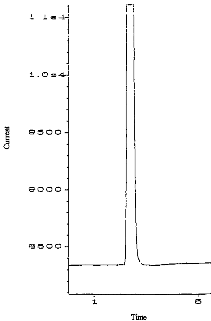
Figure 3.10 ECD chromatogram of isoniazid
